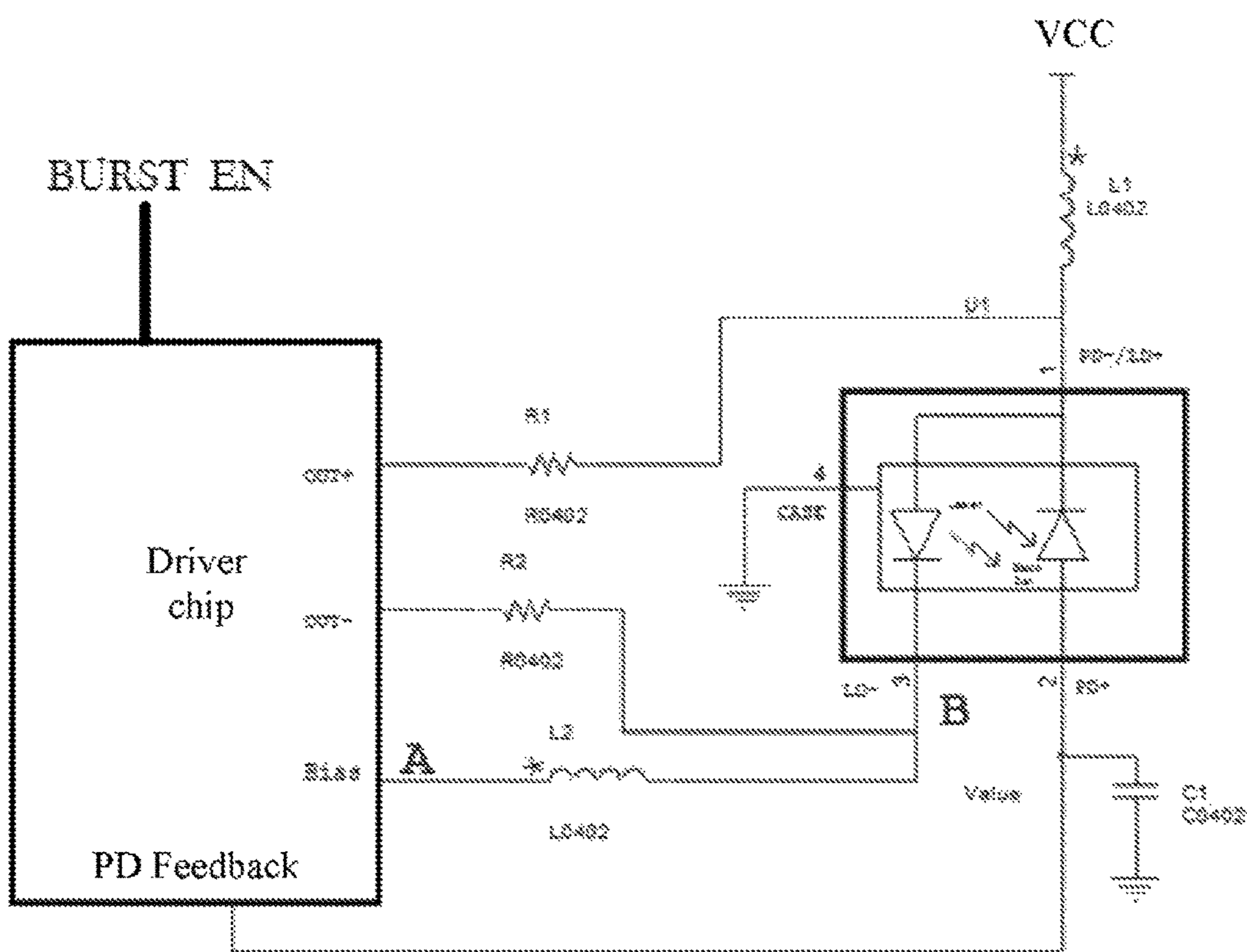
FIG. 1 (Prior Art)
