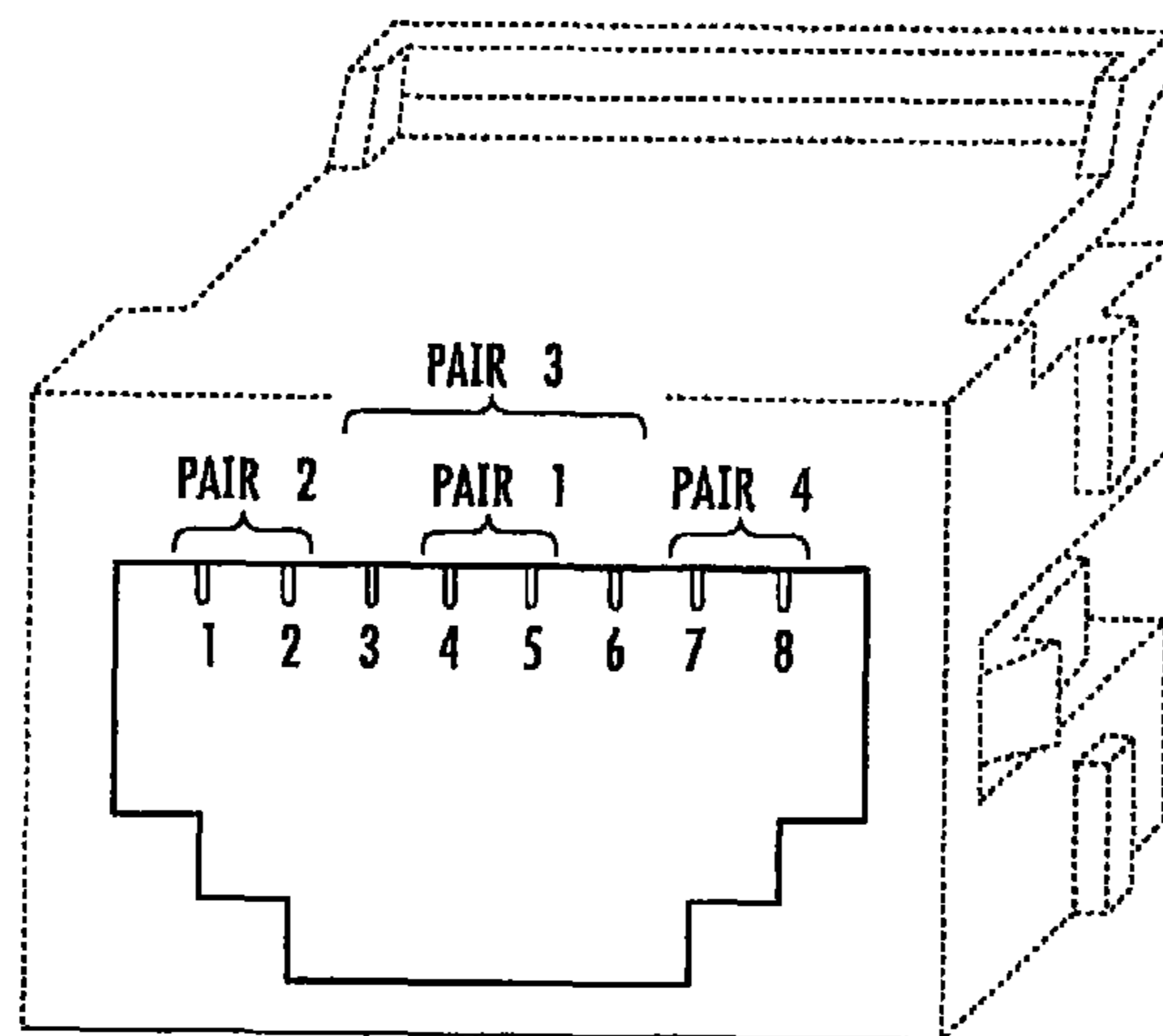
FIG. 2 (PRIOR ART)
