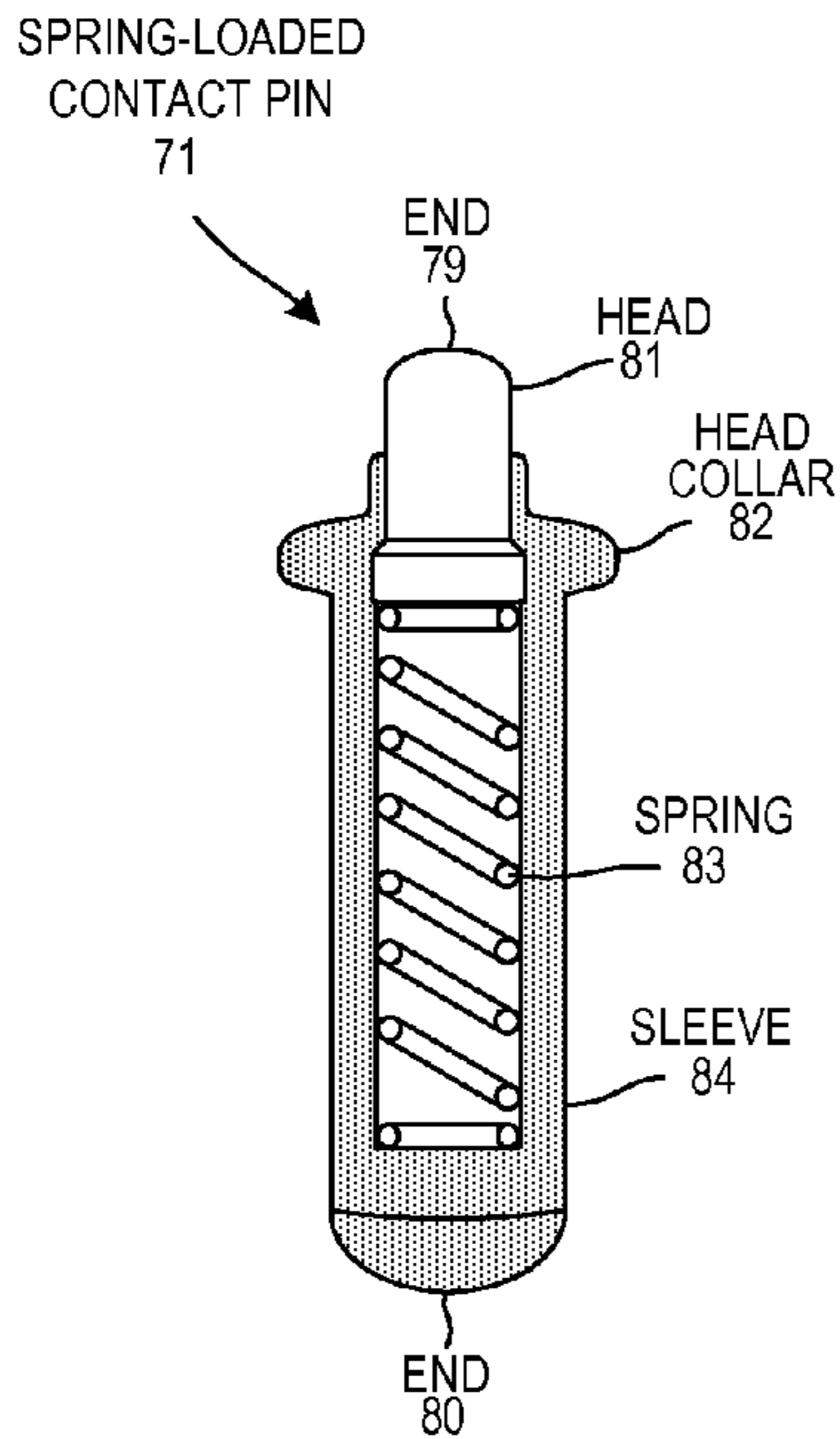
SPRING-LOADED CONTACT PIN
