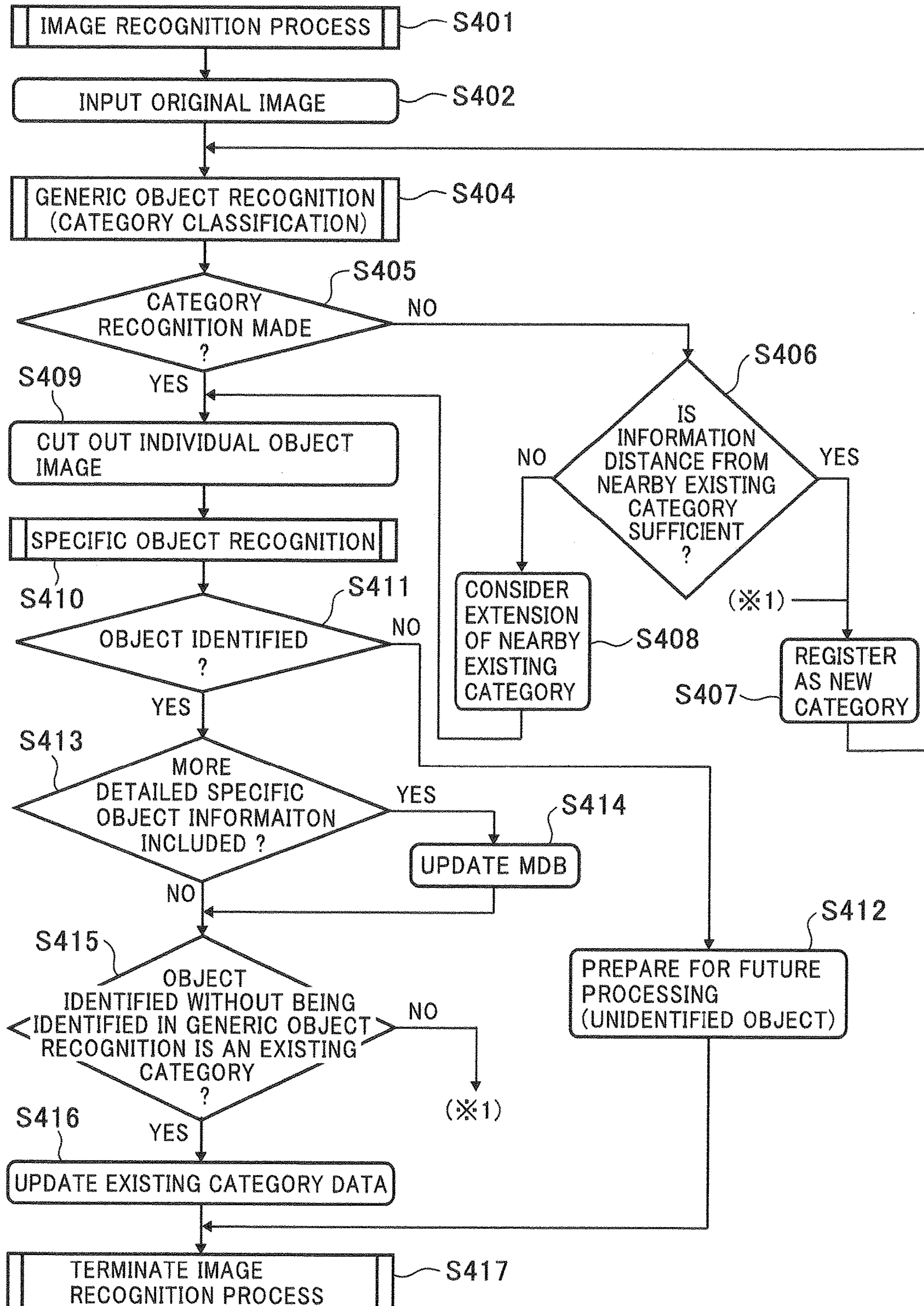
FIG.4 (ENTIRE RECOGNITION FLOW)
