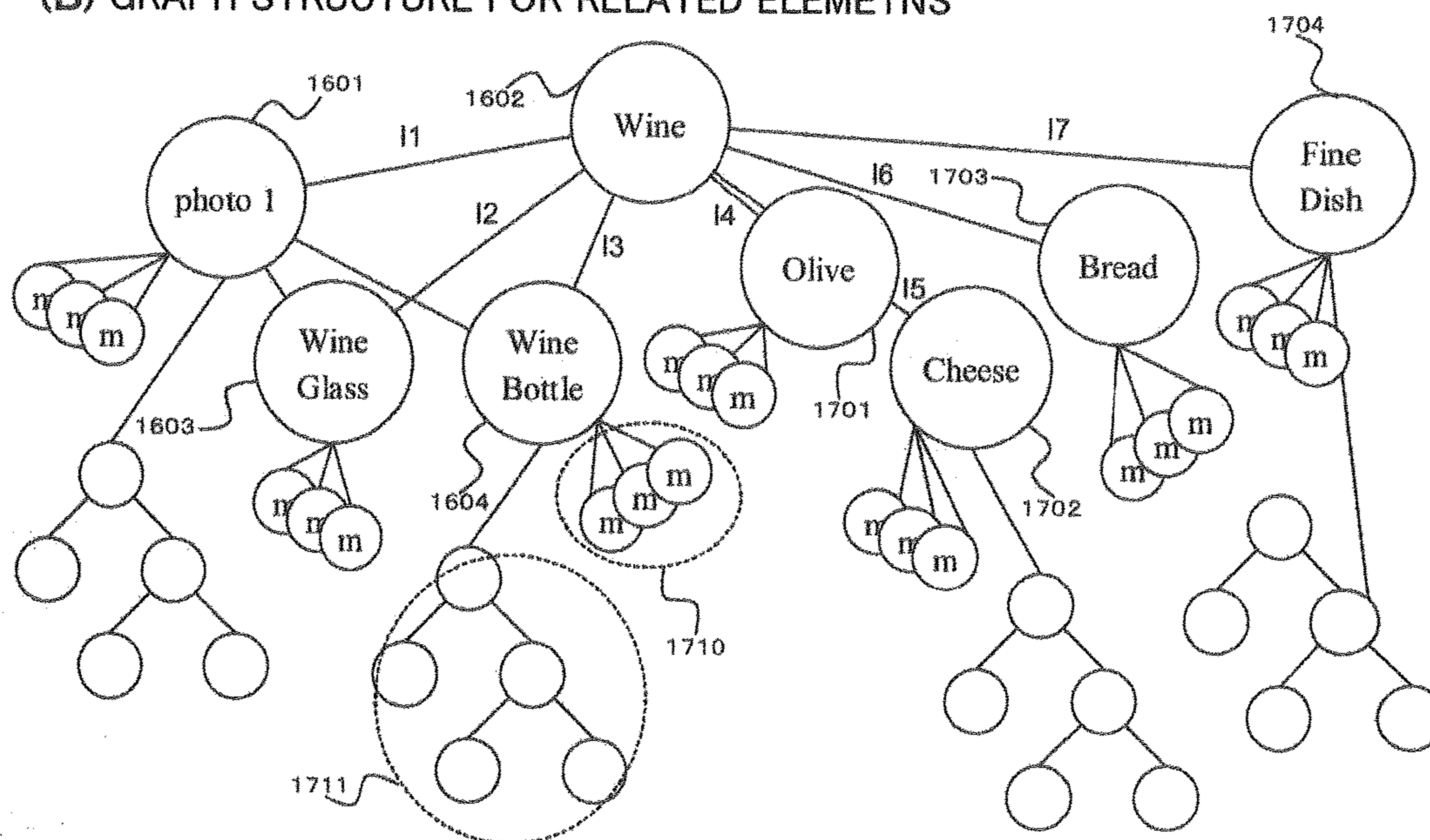
(B) GRAPH STRUCTURE FOR RELATED ELEMENTS
