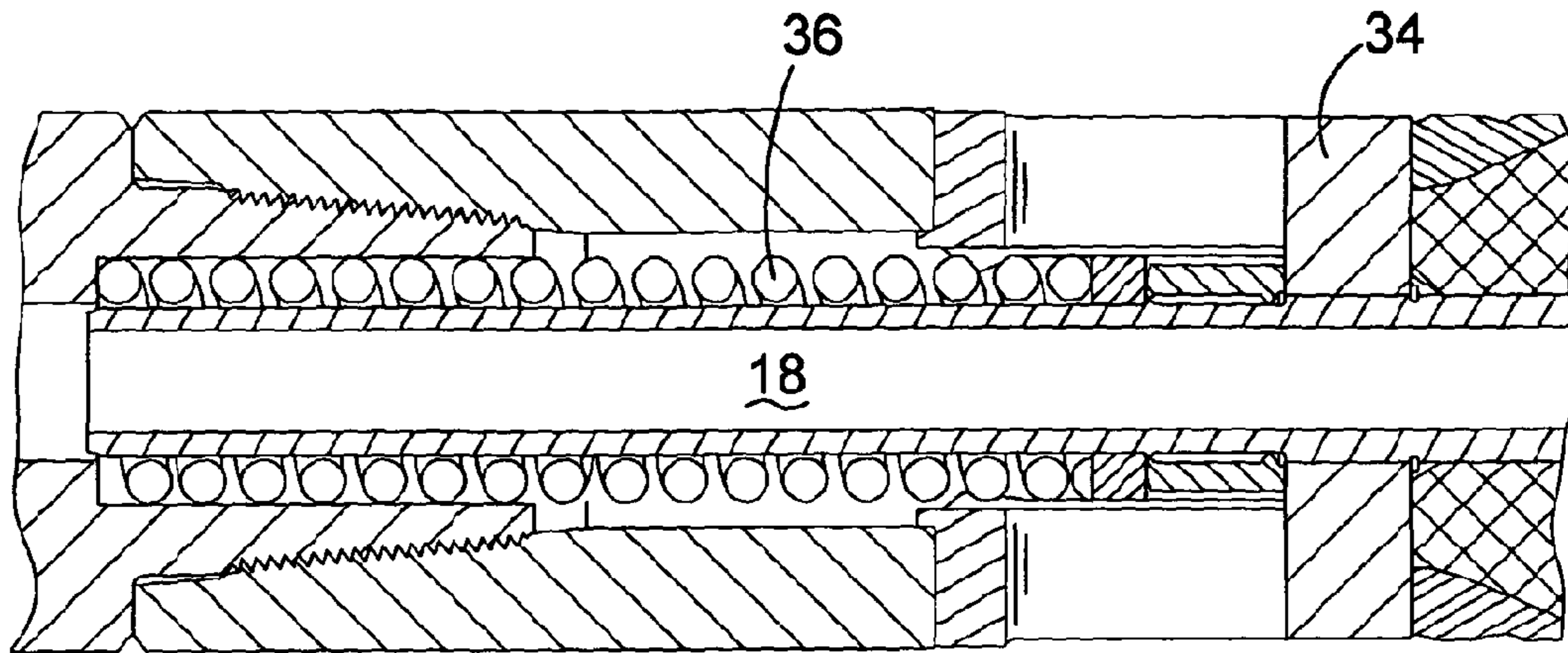
FIG.6a
