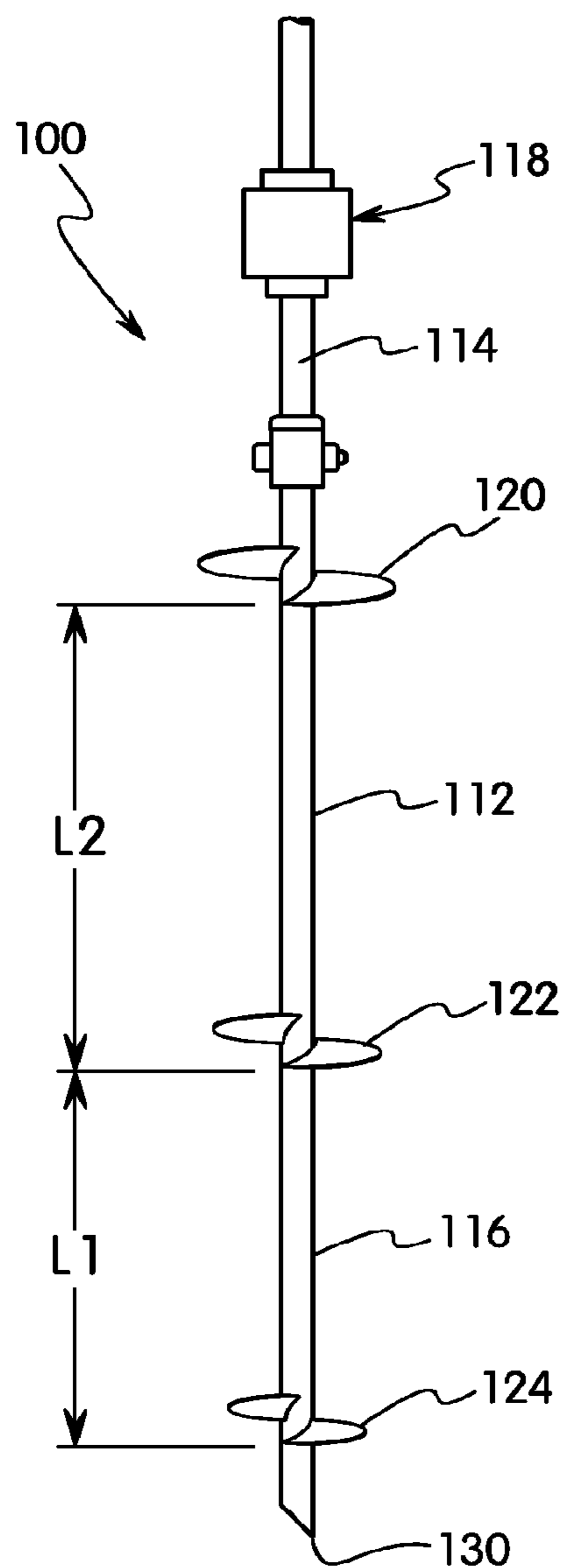
FIG. 1 (PRIOR ART)
