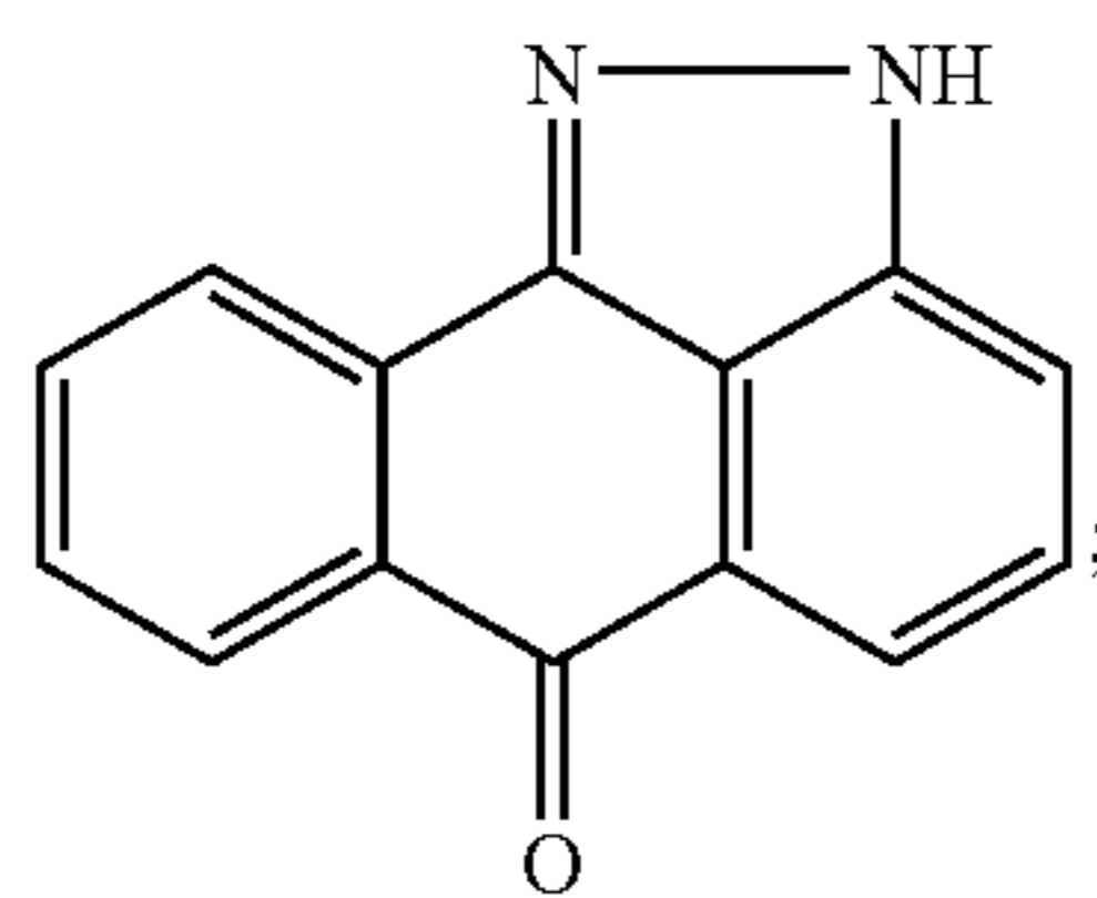
2H-Dibenzo[cd,g] indazol-6-one
