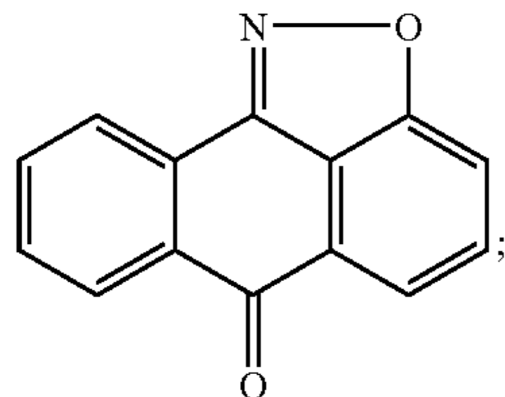
2-Oxa-1-aza-aceanthrylen-6-one
