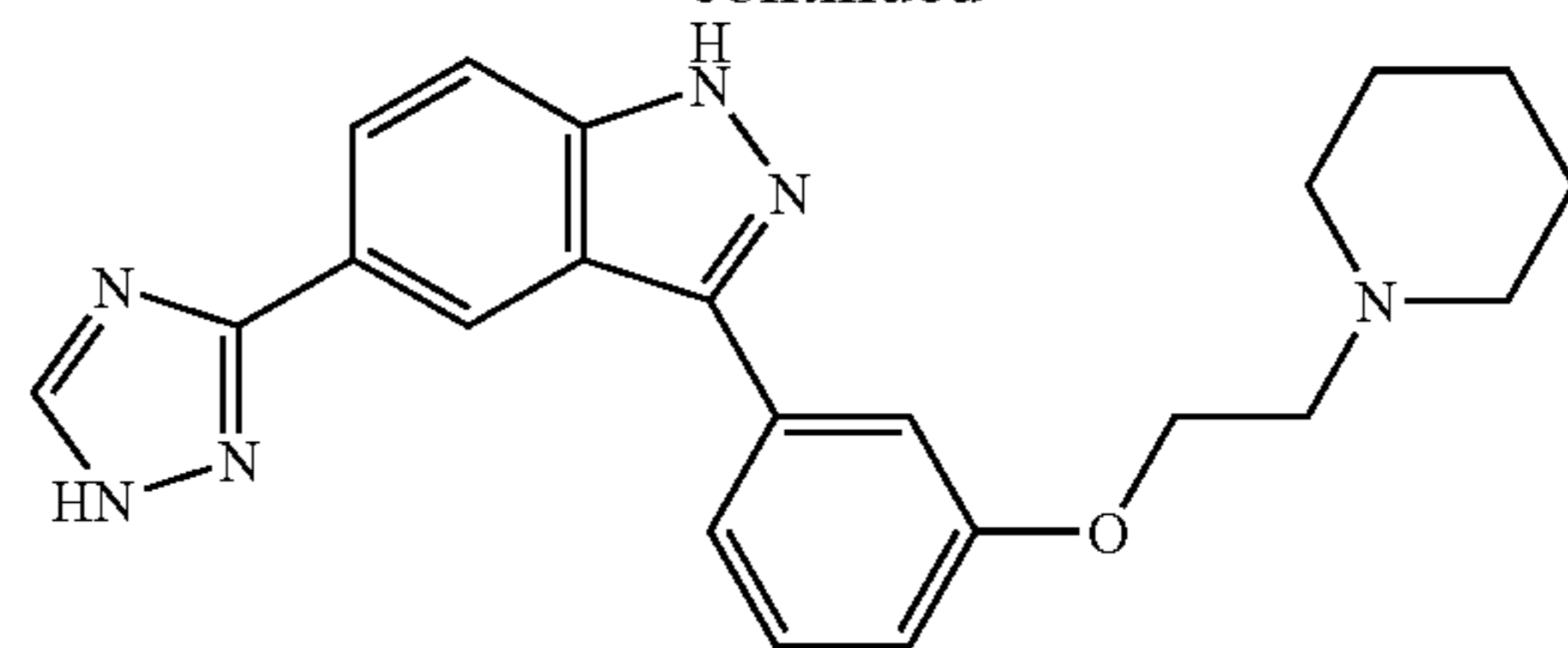
3-[3-(2-Piperidin-1-yl-ethoxy)-phenyl]-5-(1H-[1,2,4]triazol-3-yl)-1H-indazole
