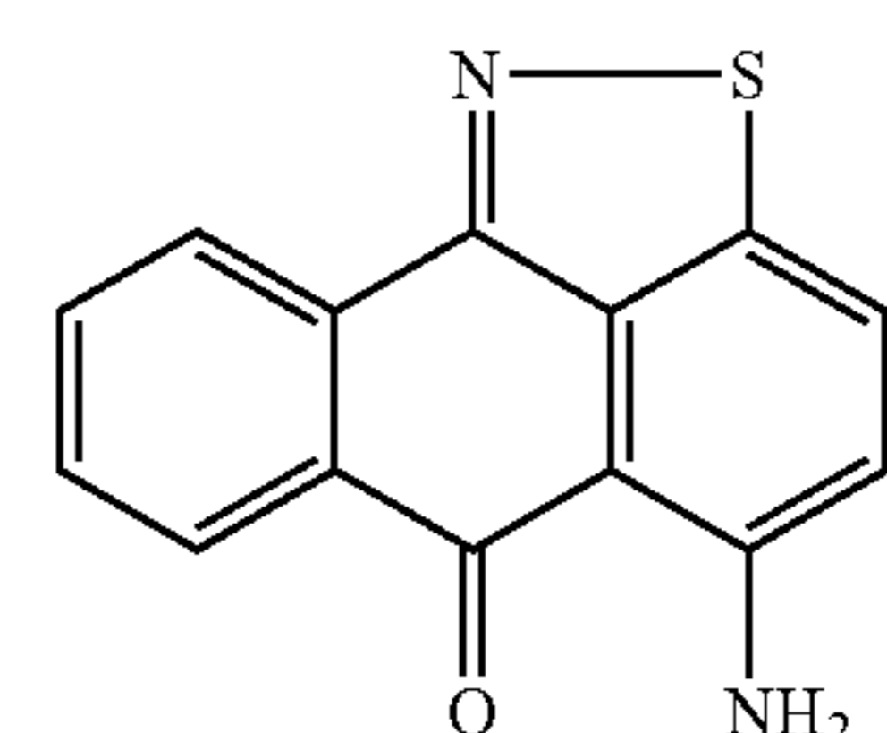
5-Amino-anthra[9,1- cd]isothiazol-6-one
