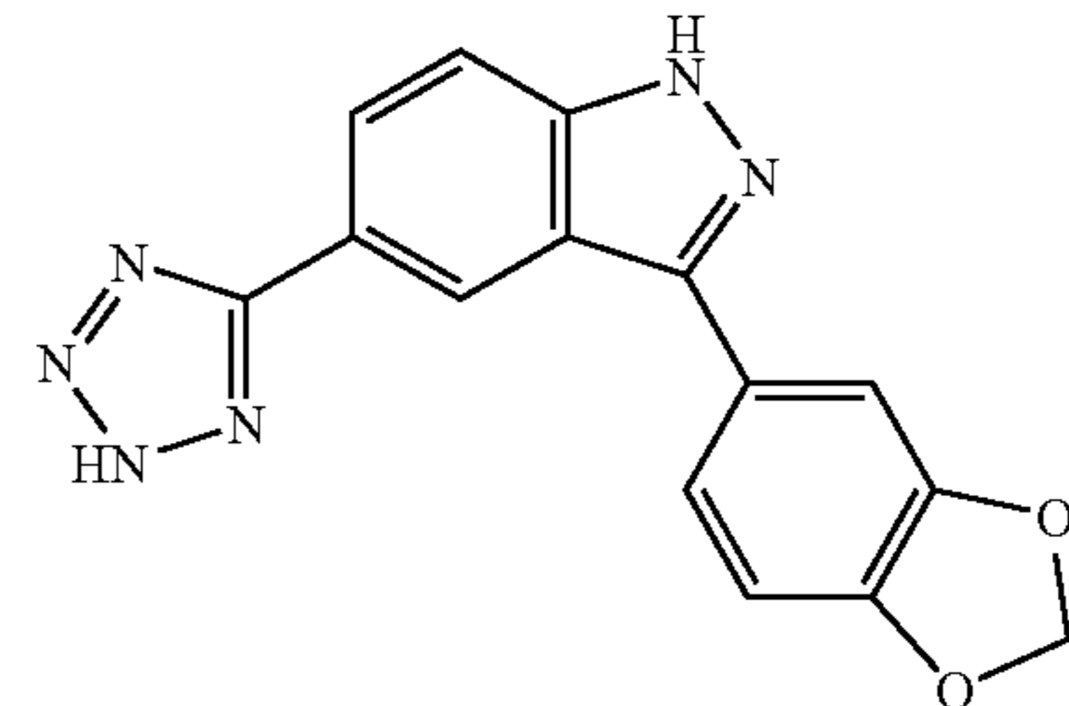
3-Benzo[1,3]dioxol-5-yl-5-(2H-tetrazol-5-yl)-1H-indazole
