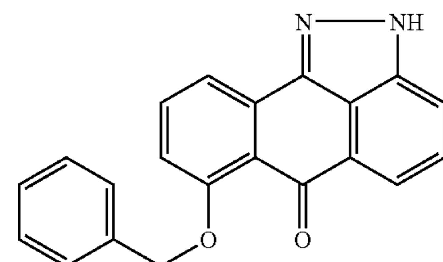
7-Benzyloxy-2H-dibenzo[cd,g]indazol- 6-one
