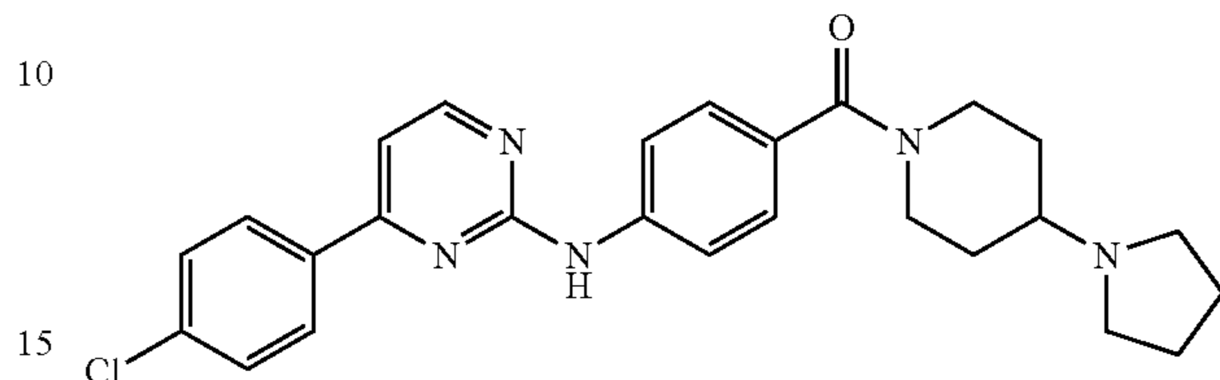
{4-[4-(4-Chloro-phenyl)-pyrimidin-2-ylamino]-phenyl}-(4-pyrrolidin-1-yl-piperidin-1-yl)-methanone
