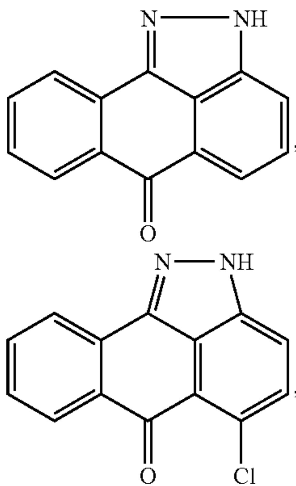
5-Chloroanthra[1,9cd]pyrazol-6(2H)-one
