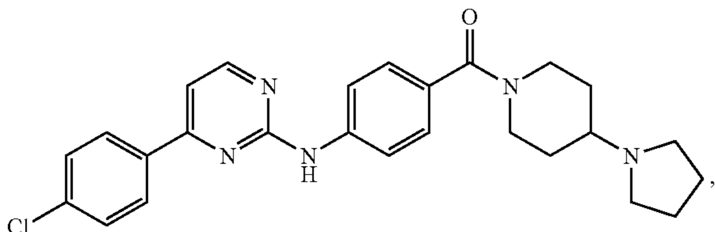
{4-[4-(4-Chloro-phenyl)-pyrimidin-2-ylamino]-phenyl}-(4-pyrrolidin-1-yl-piperidin-1-yl)-methanone
