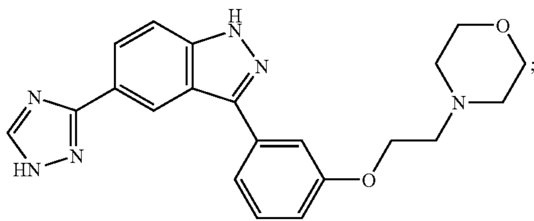
3-[3-(2-Morpholin-4-yl-ethoxy)-phenyl]-5-(1H-[1,2,4]triazol-3-yl)-1H-indazole
