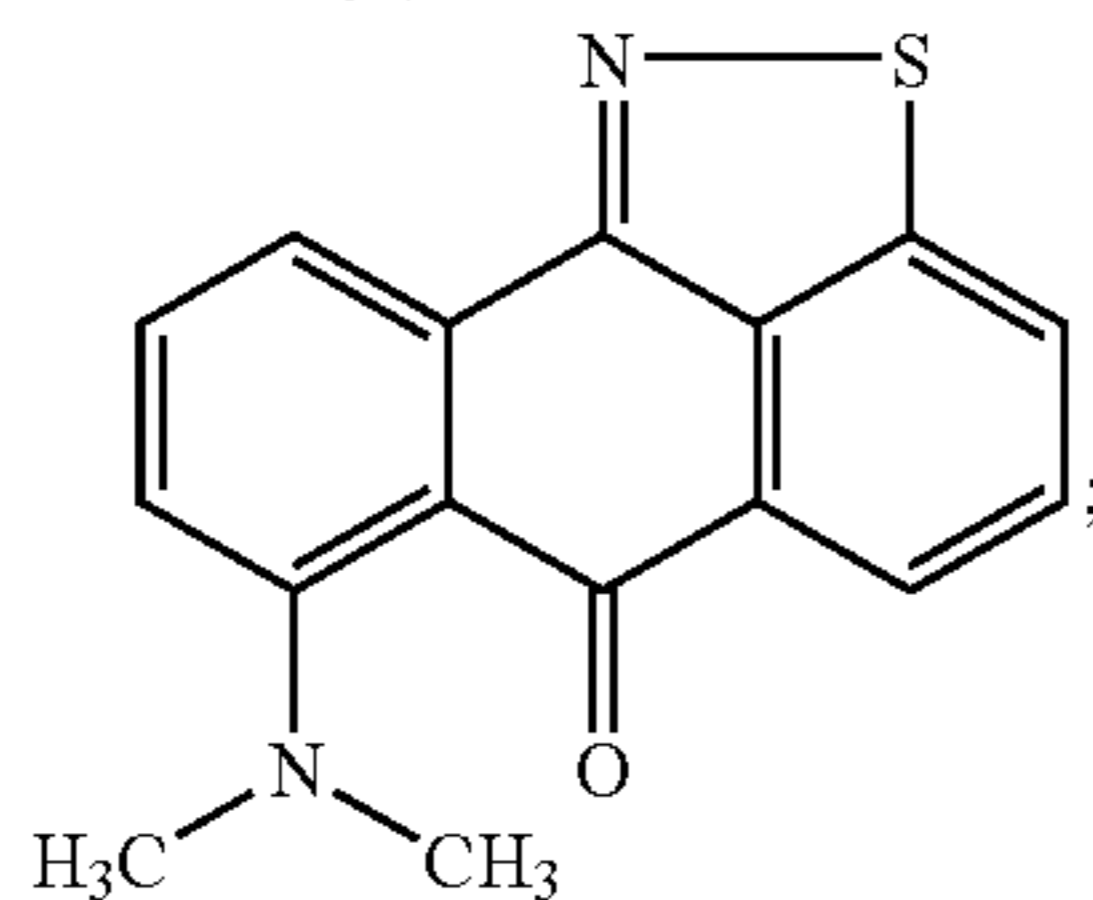
7-Dimethylamino-anthra[9,1-cd]isothiazol-6-one
