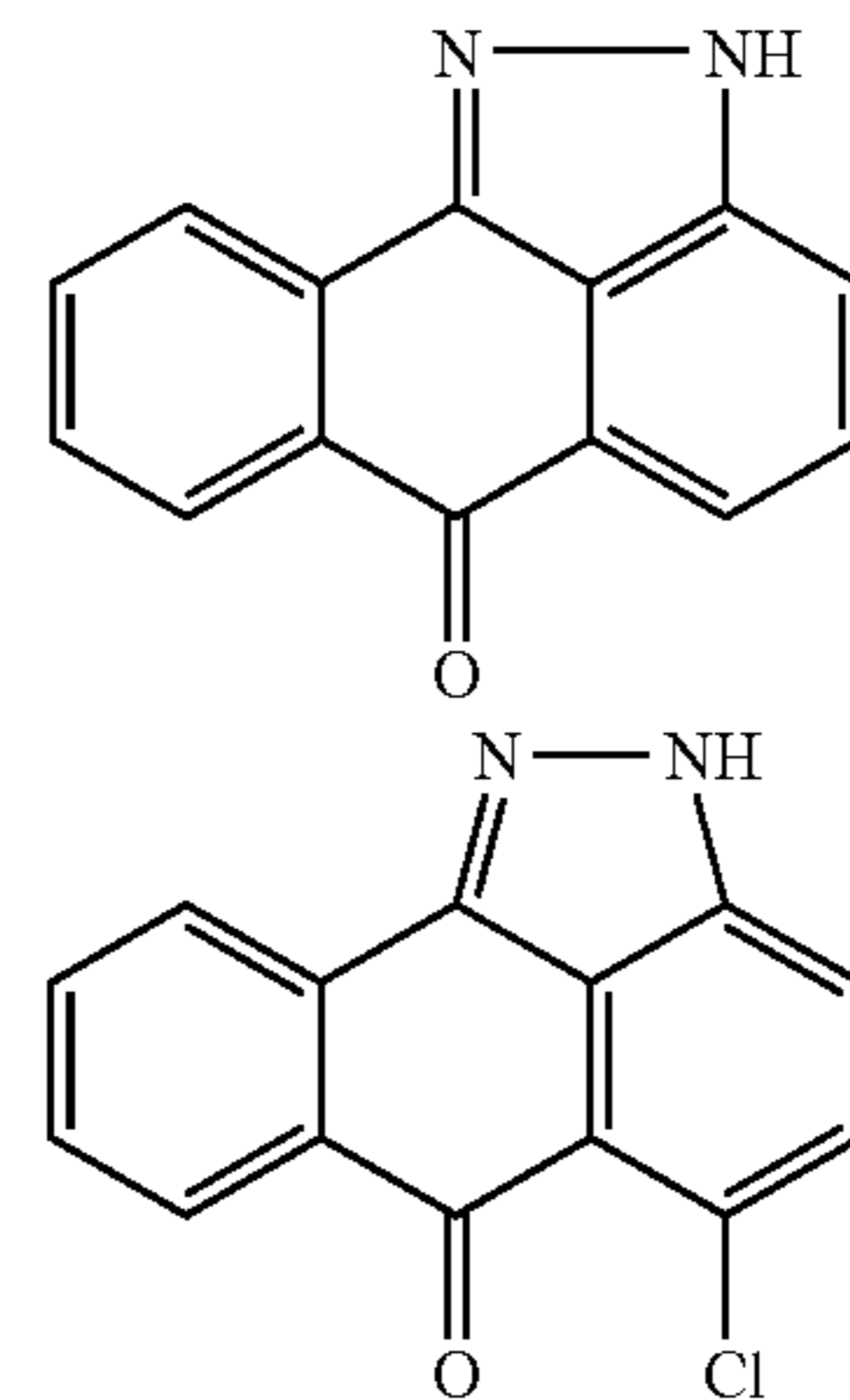
5-Chloroanthra[1,9cd]pyrazol-6(2H)-one
