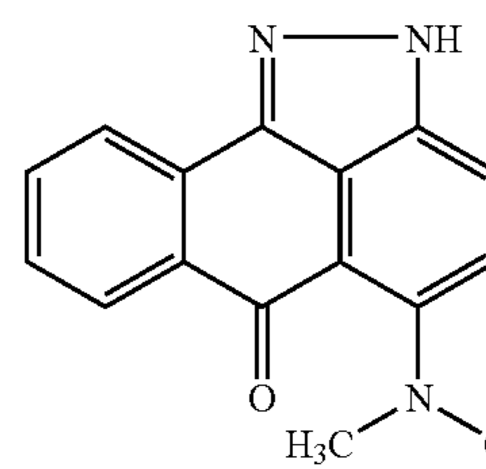
5-Dimethylamino-2H- dibenzo[cd,g]indazol-6-one
