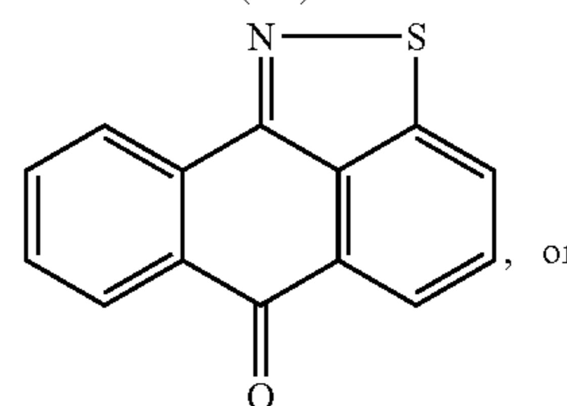
5-Chloroanthra[1,9cd]pyrazol-6(2H)-one
