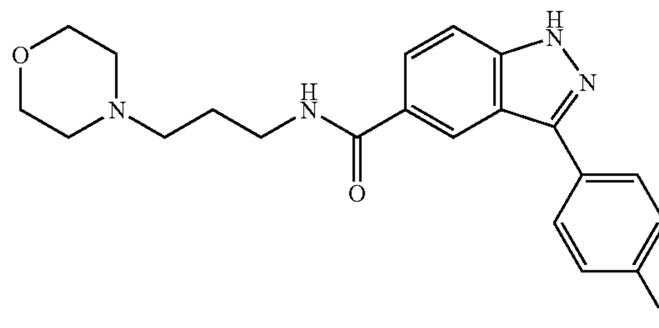
3-(4-Fluoro-phenyl)-1H-indazole-5-carboxylic acid (3-morpholin-4-yl-propyl)-amide
