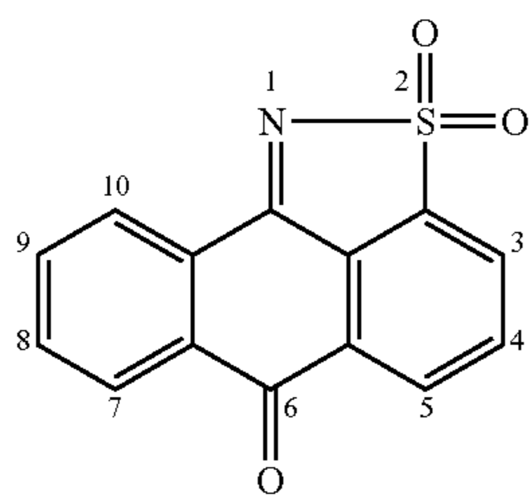
2,2-Dioxo-2H-2l 6 -anthra [9,1-cd]isothiazol-6-one
