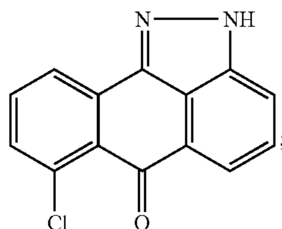
7-Chloro-2H-dibenzo[cd,g] indazol-6-one
