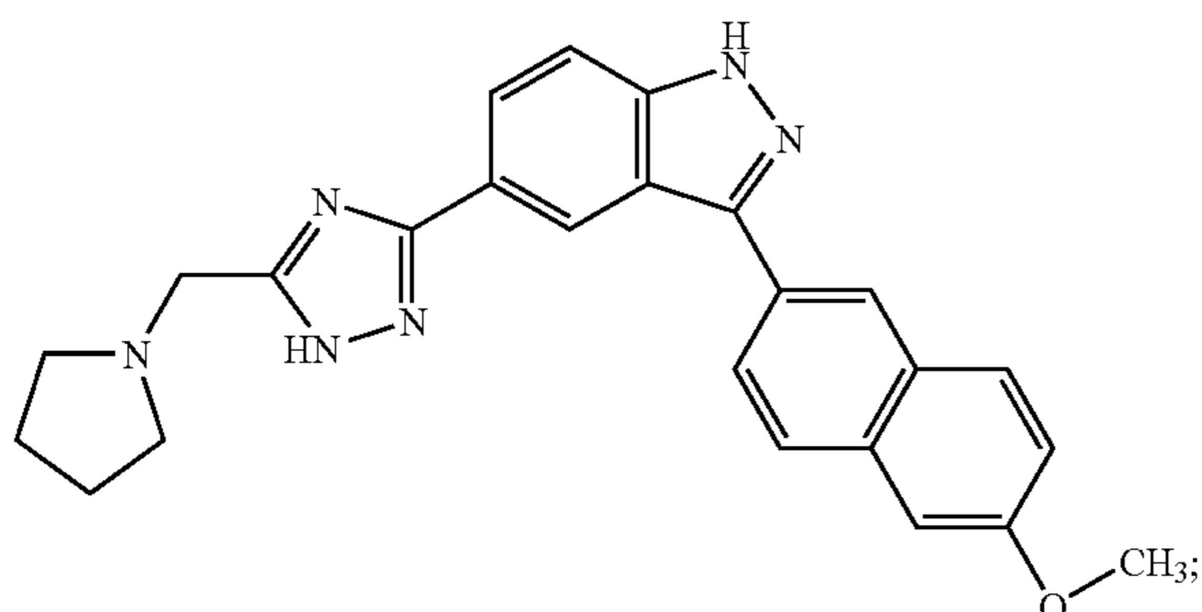
3-(6-Methoxy-naphthalen-2-yl)-5-(5-pyrrolidin-1-ylmethyl-1H-[1,2,4]triazol-3-yl)-1H-indazole
