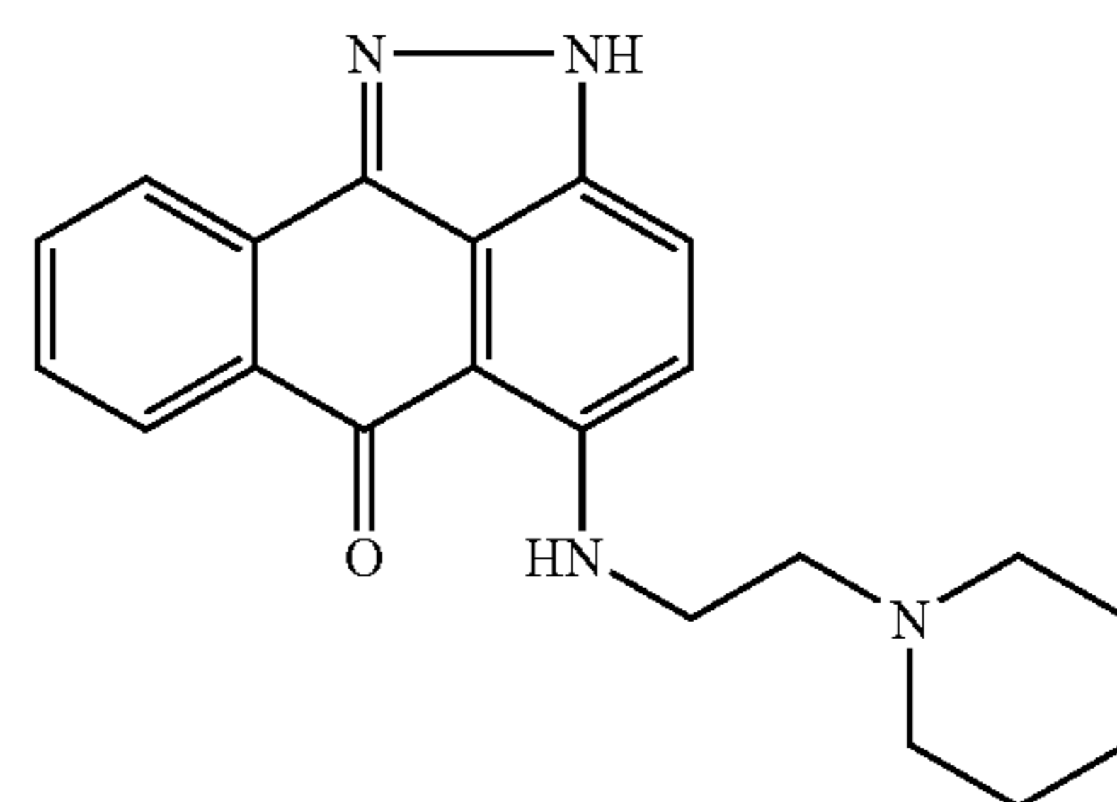
5-(2-Piperidin-1-yl-ethylamino)-2H- dibenzo[cd,g]indazole-6-one
