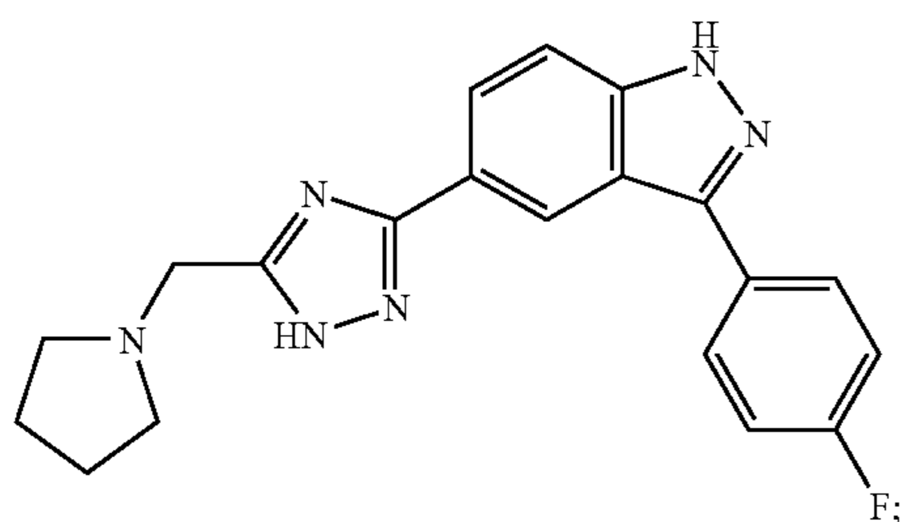
3-(4-Fluoro-phenyl)-5-(5-pyrrolidin-1-ylmethyl-1H-[1,2,4]triazol-3-yl)-1H-indazole
