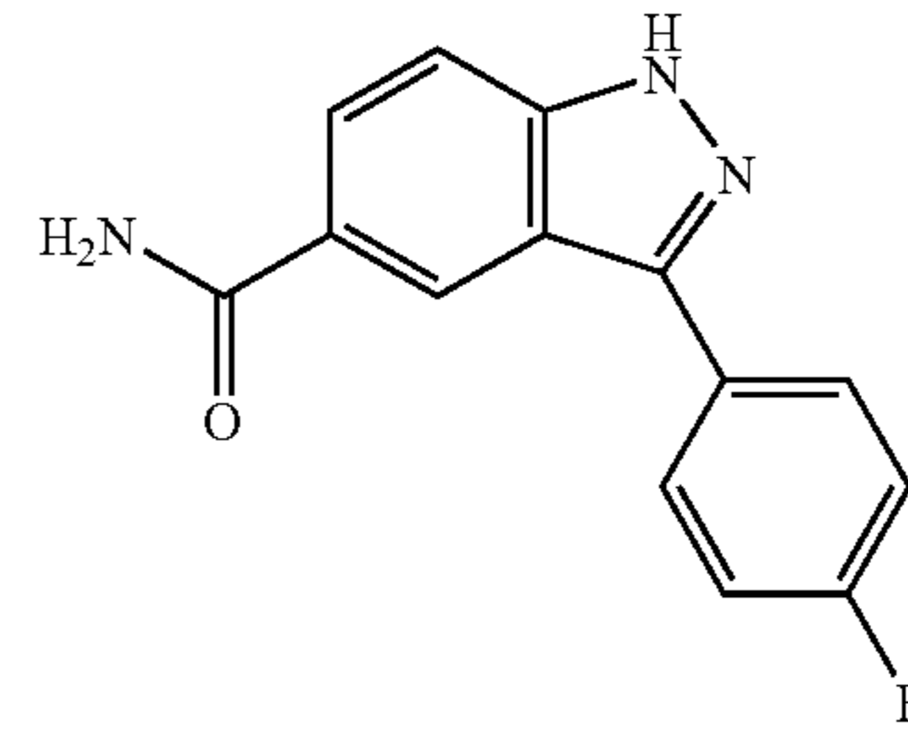
3-(4-Fluoro-phenyl)-1H-indazole-5-carboxylic acid amide
