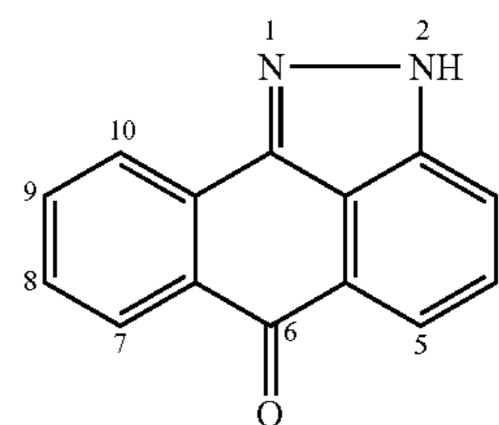
2H-Dibenzo[cd,g]indazol-6-one
