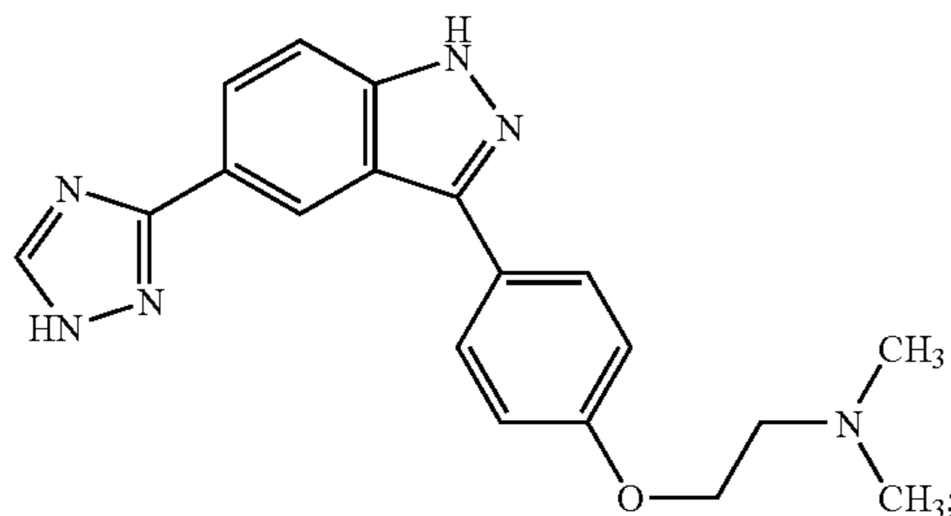
Dimethyl-(2-{4-[5-(1H-[1,2,4]triazol-3-yl)-1H-indazol-3-yl]-phenoxy}-ethyl)-amine
