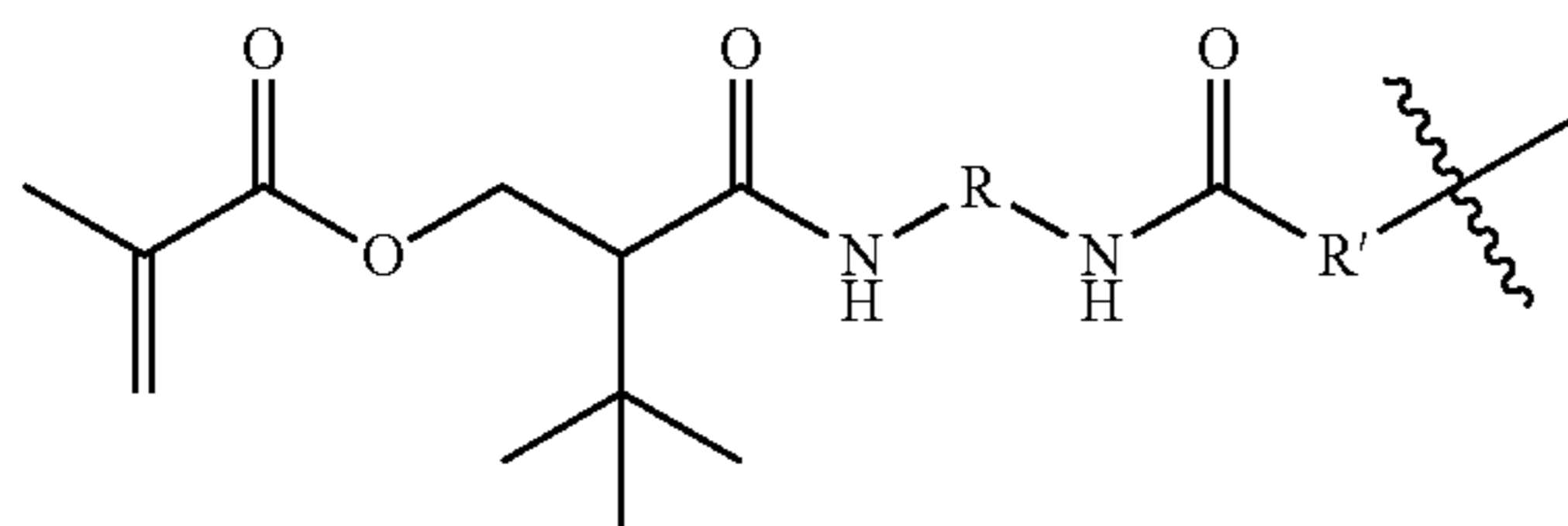
Formula (XI)
