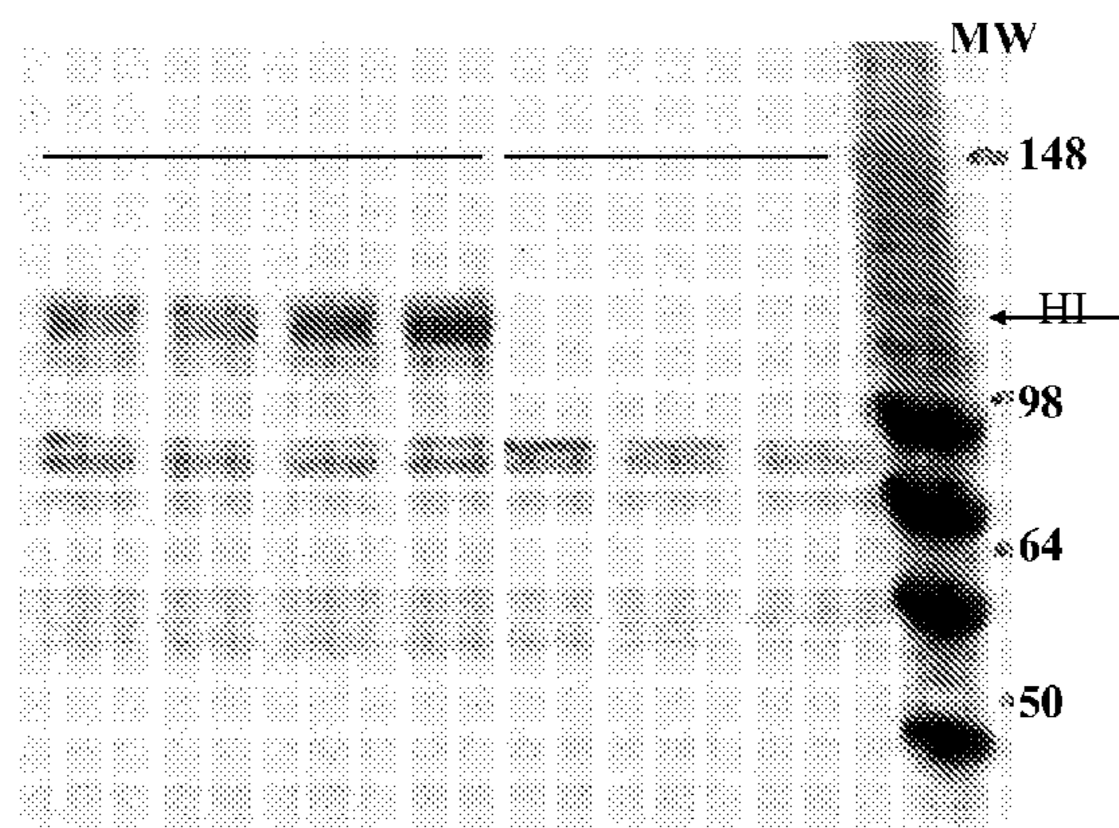
Immunoblot analysis of nuclear extracts demonstrating stabilization of HIF-1 \alpha in mouse liver by {[5-(3-chlorophenyl)-3-hydroxypyridine-2-carbonyl]amino}-acetic acid
