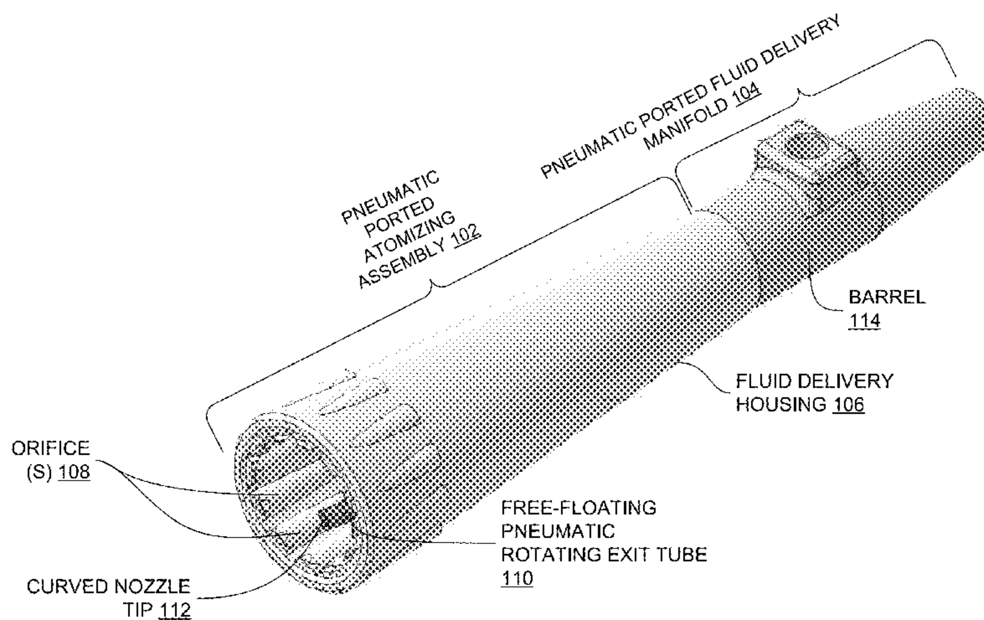
PNEUMATIC PORTED ATOMIZING FLUID DELIVERY MANIFOLD 100
