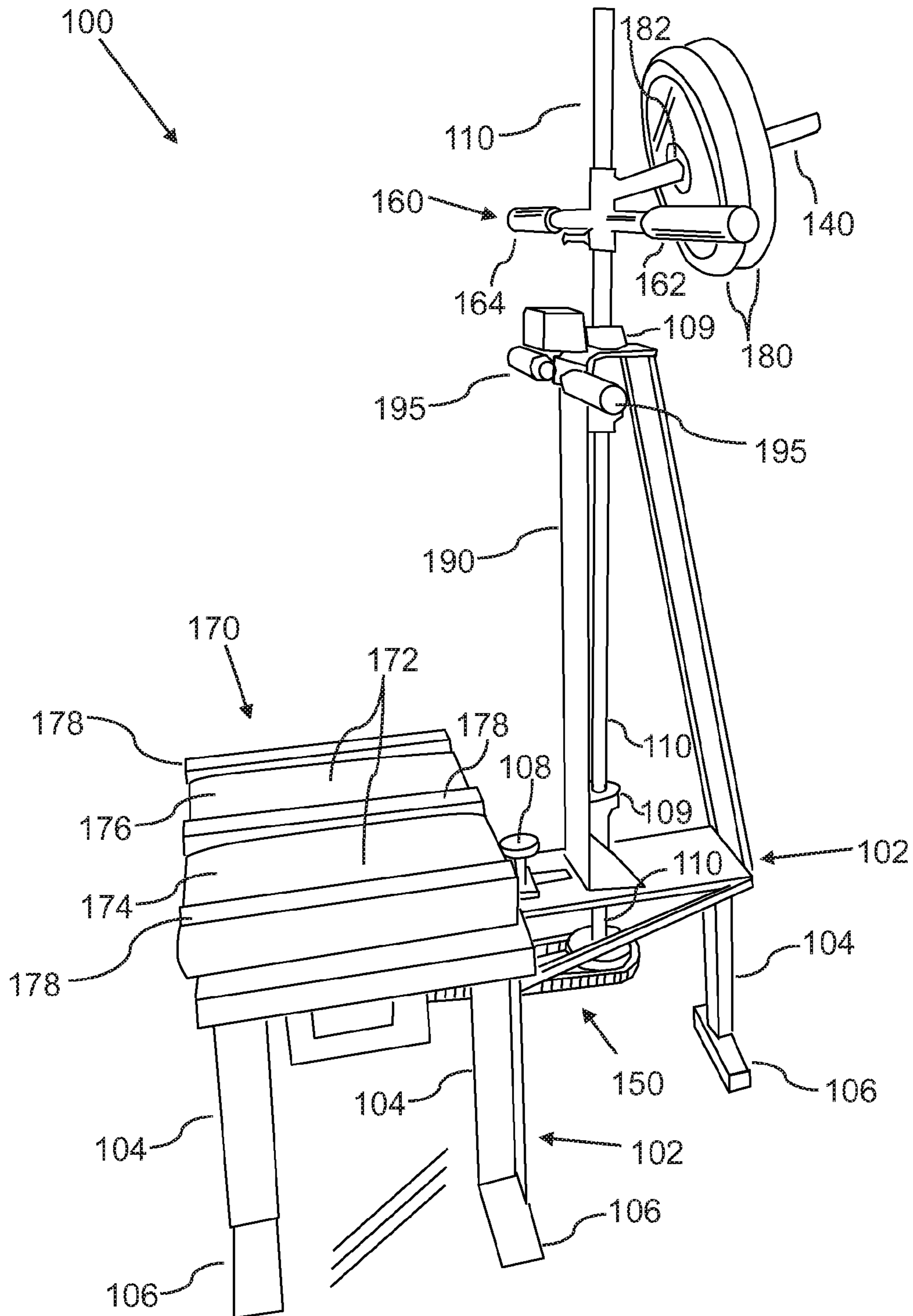
FIG. 1 Abdominal Twist Exercise Device
