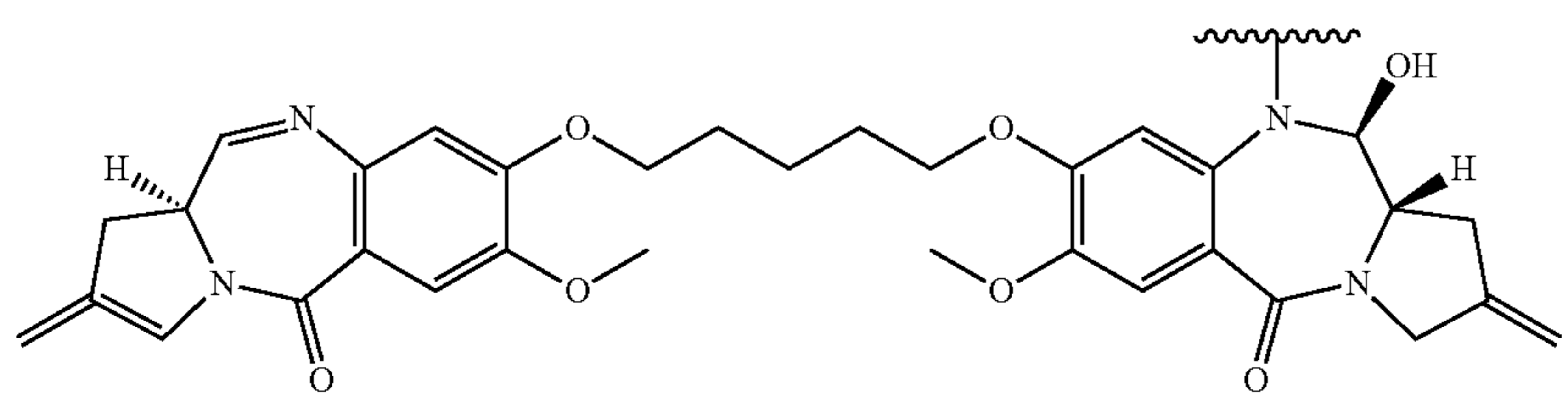
PBD dimer
