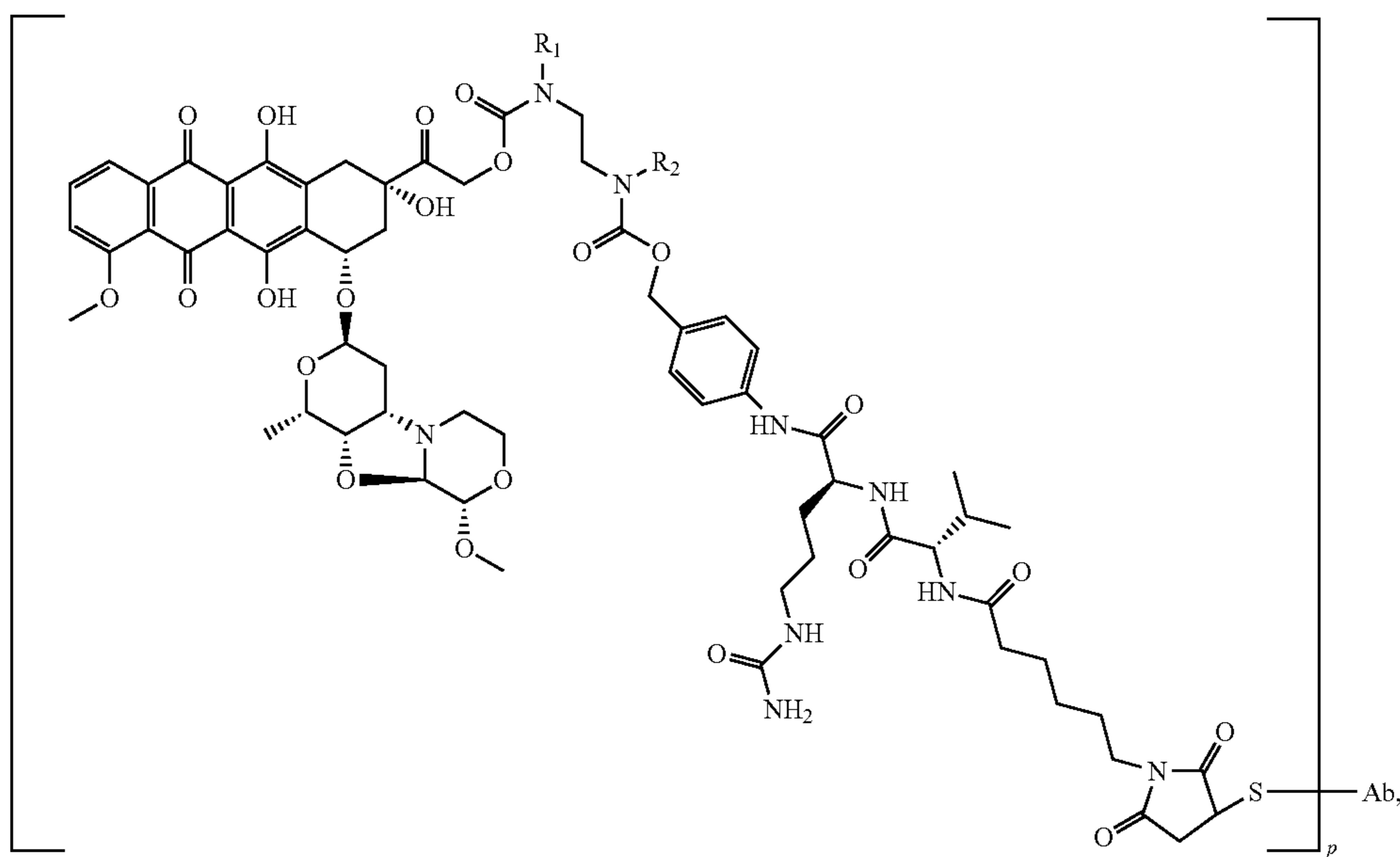
PNU-159682-val-cit-PAB-spacer-Ab
