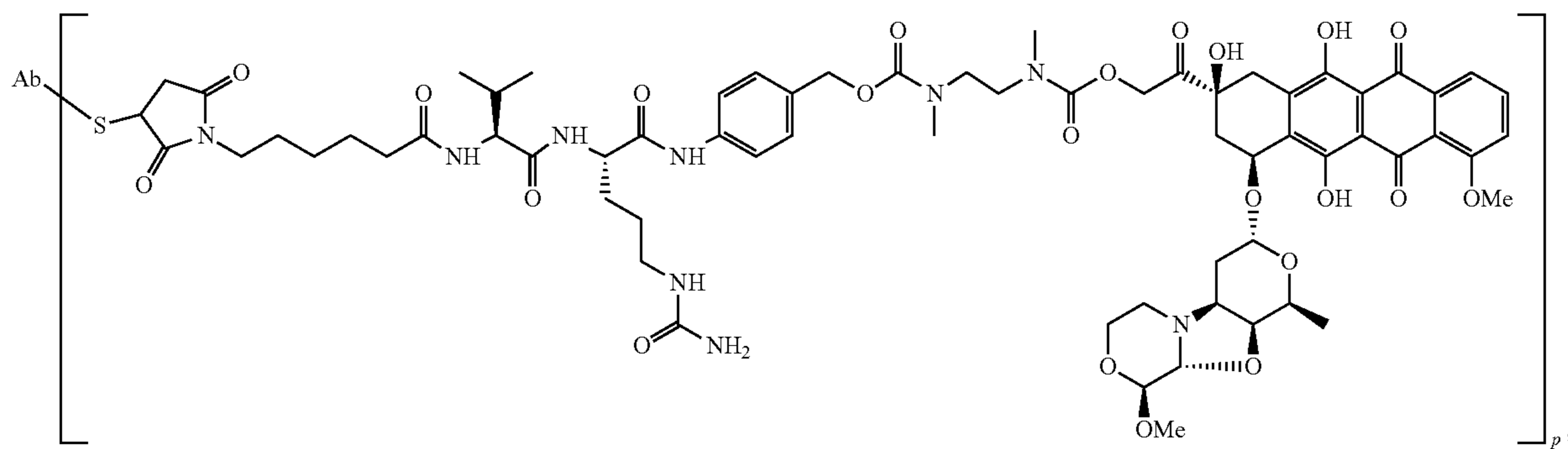
PNU-159682-val-cit-PAB-Ab
