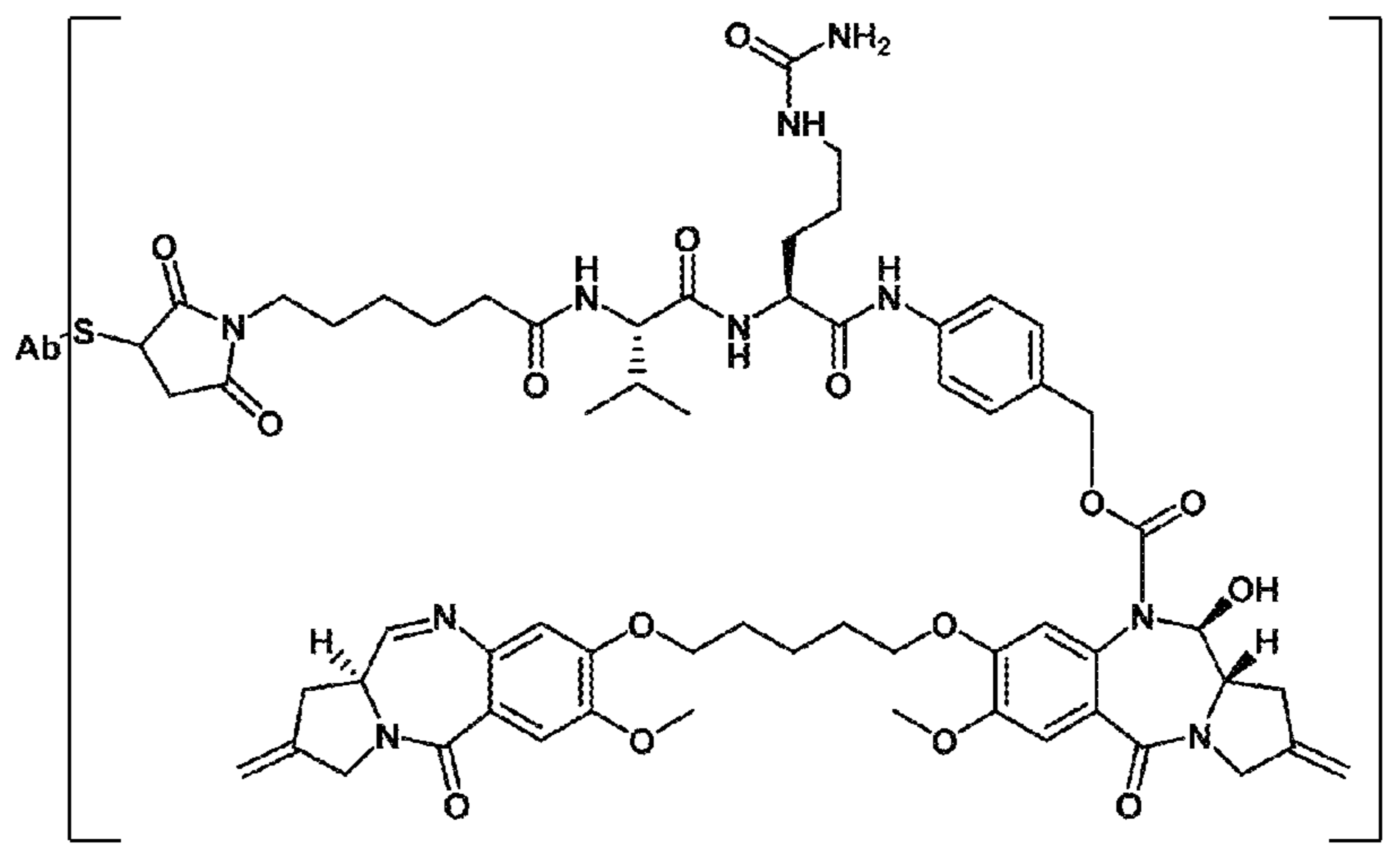
FIG. 15D Ab-MC-val-cit-PAB-PBD
