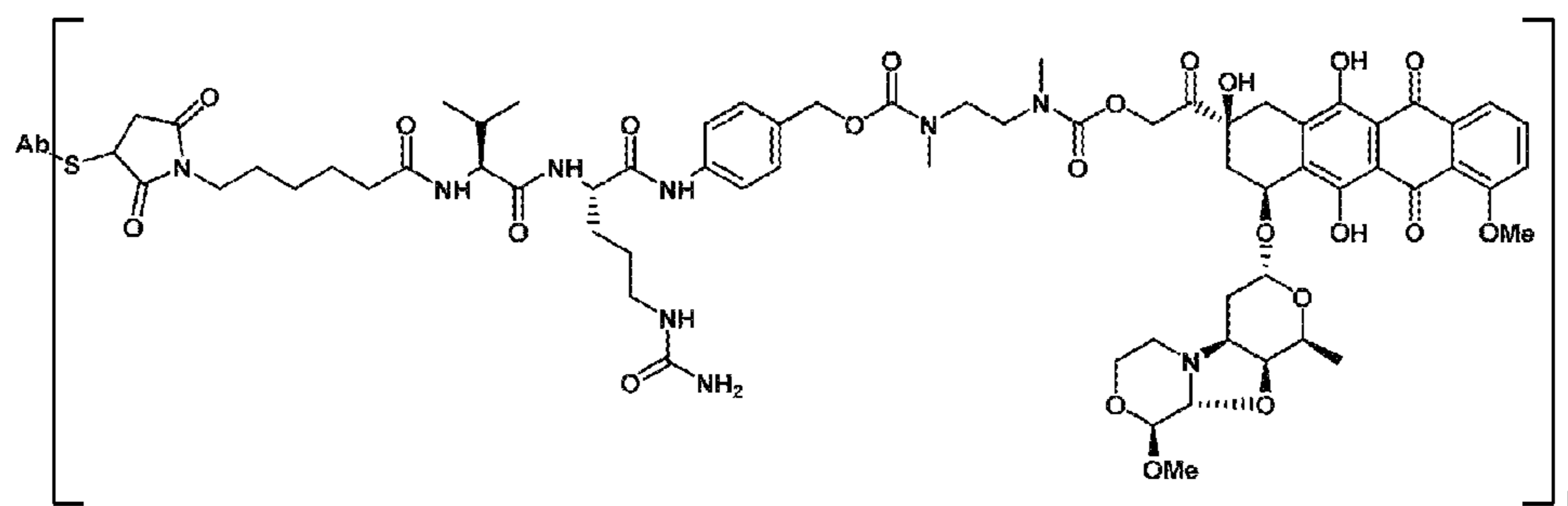
FIG. 15C Ab-MC-val-cit-PAB-PNU-159682
