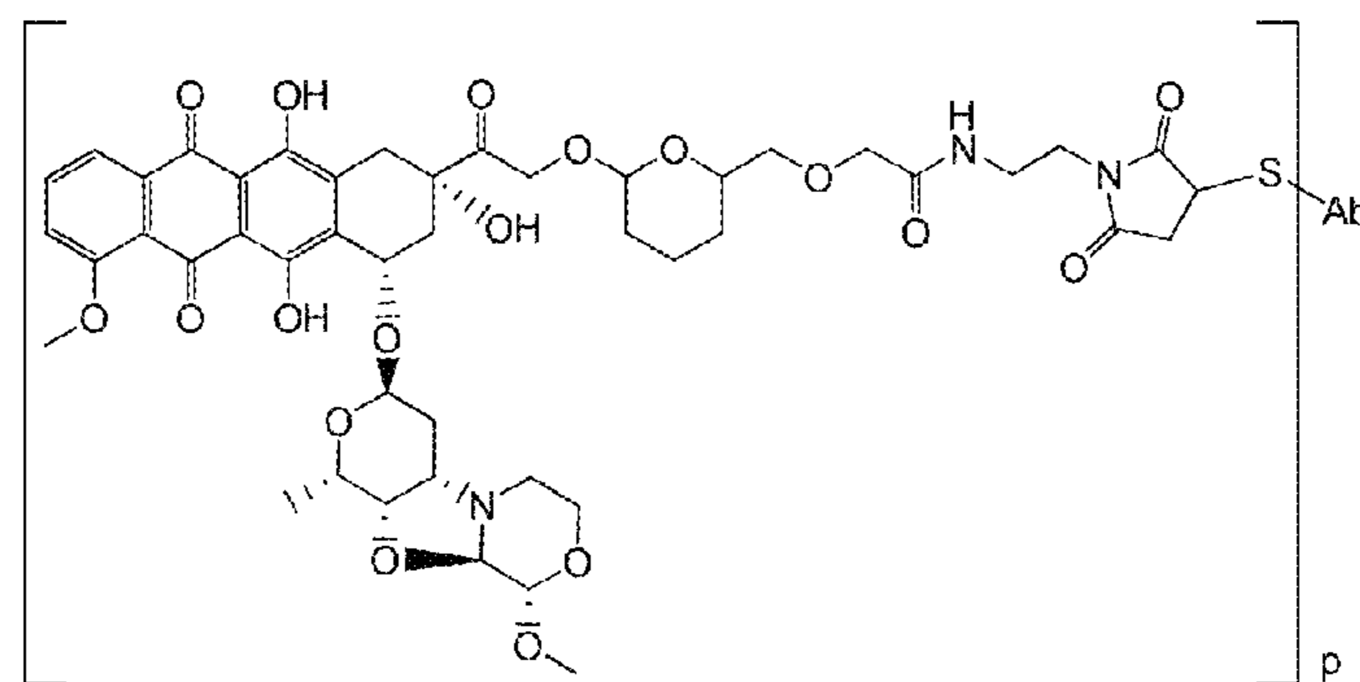
FIG. 15B Ab-MC-acetal-PNU-159682
