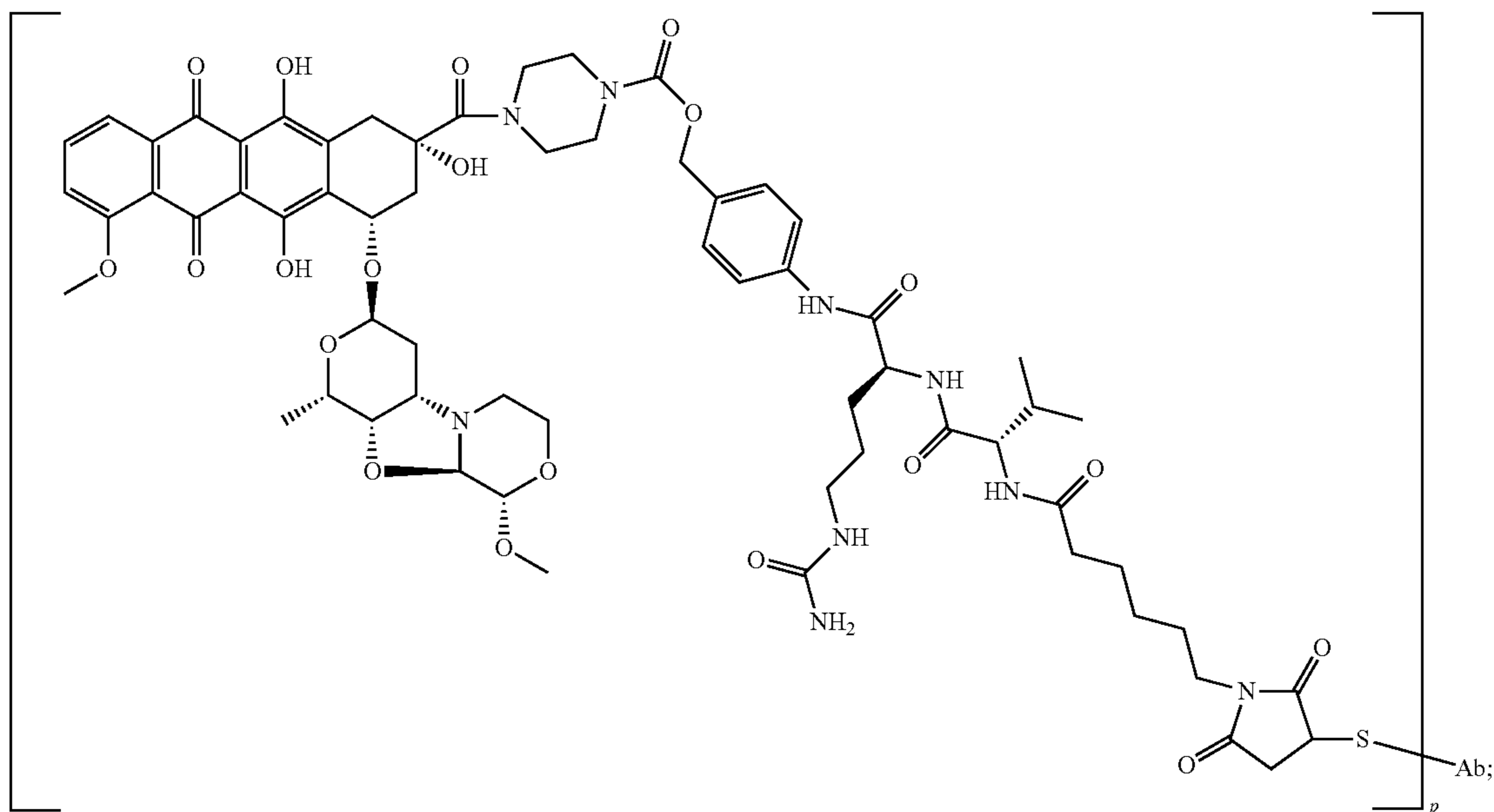
PNU-159682-val-cit-PAB-Ab
