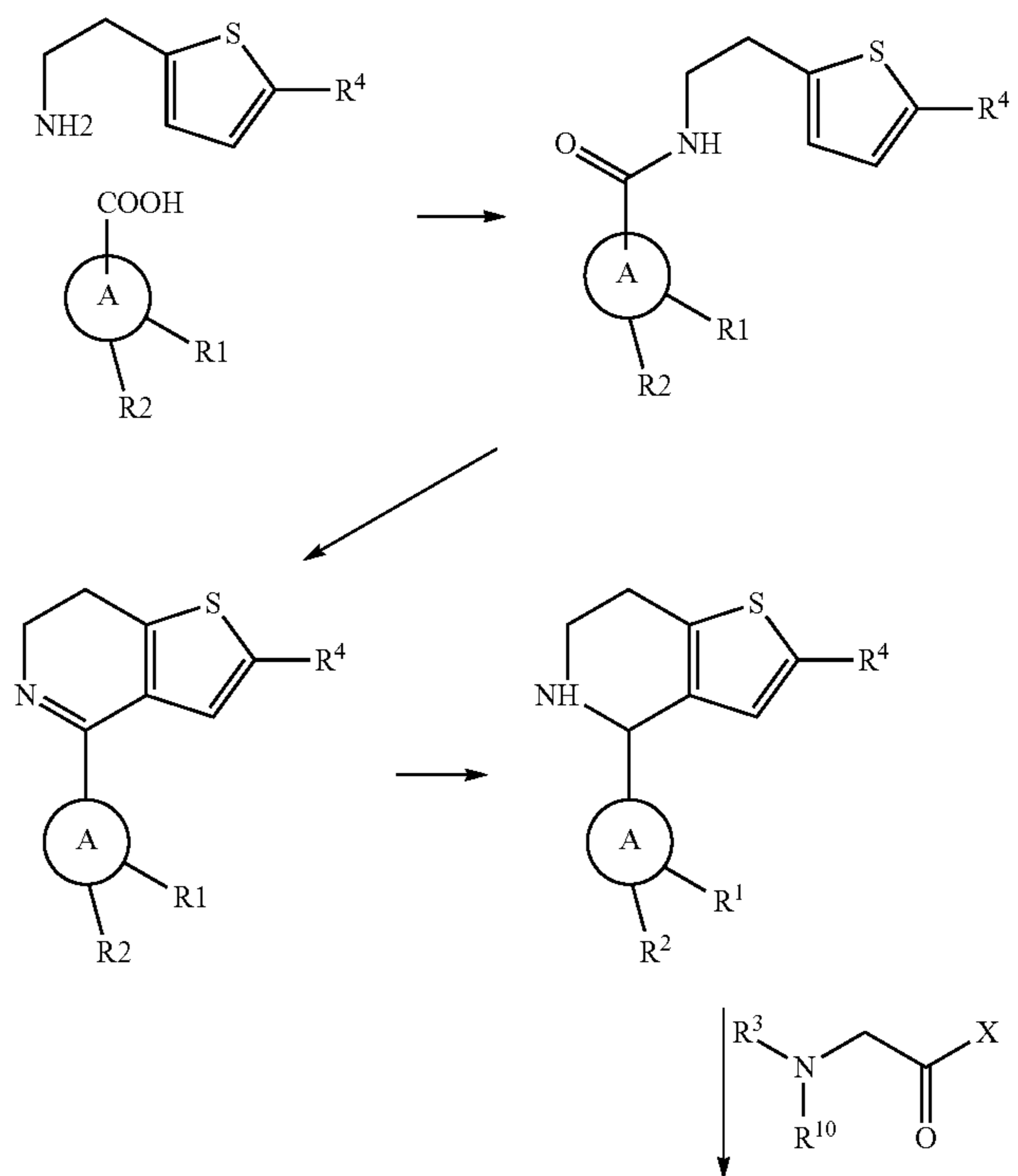
SCHEME 2
