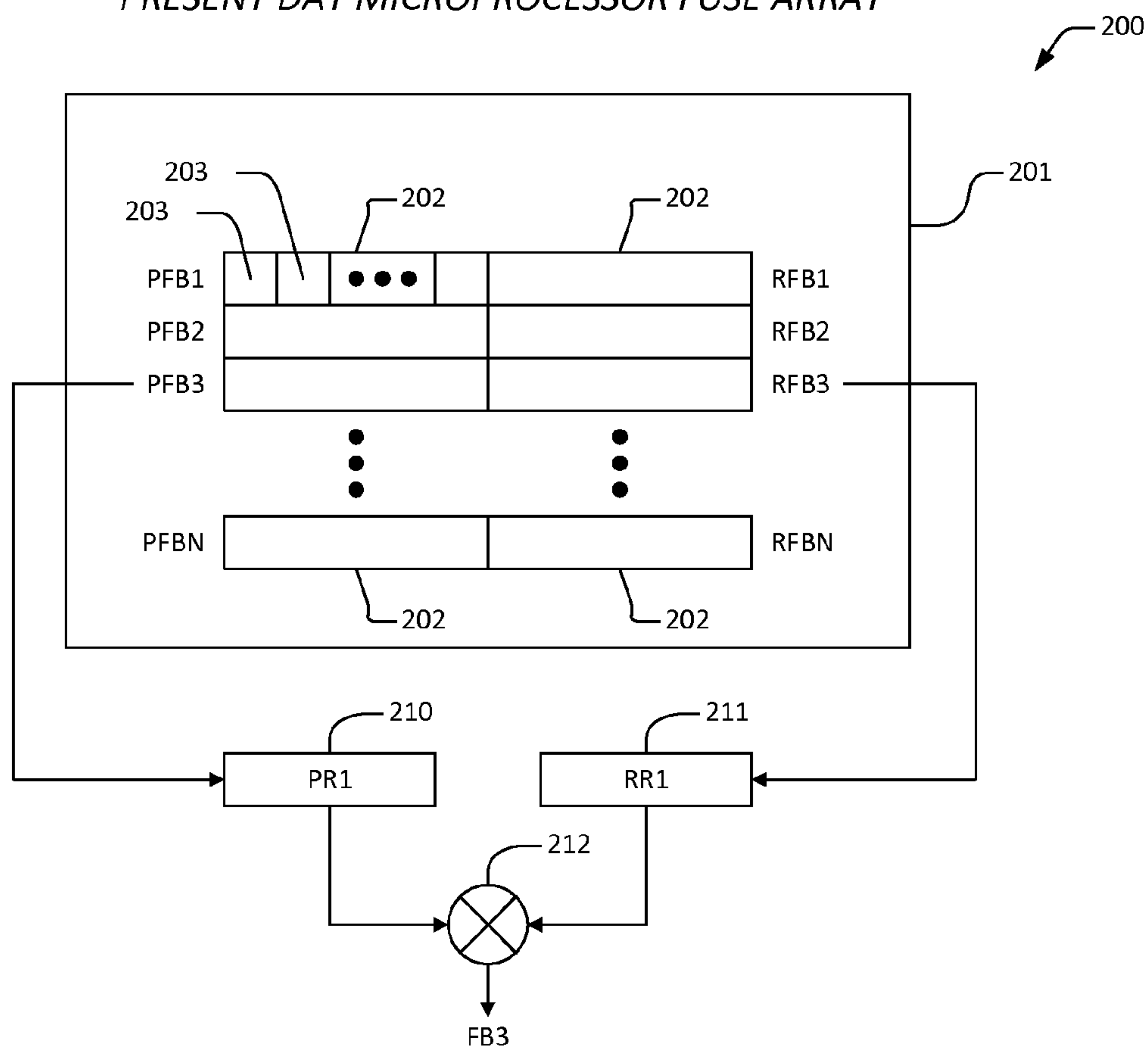
FIG. 2 (Prior Art)
