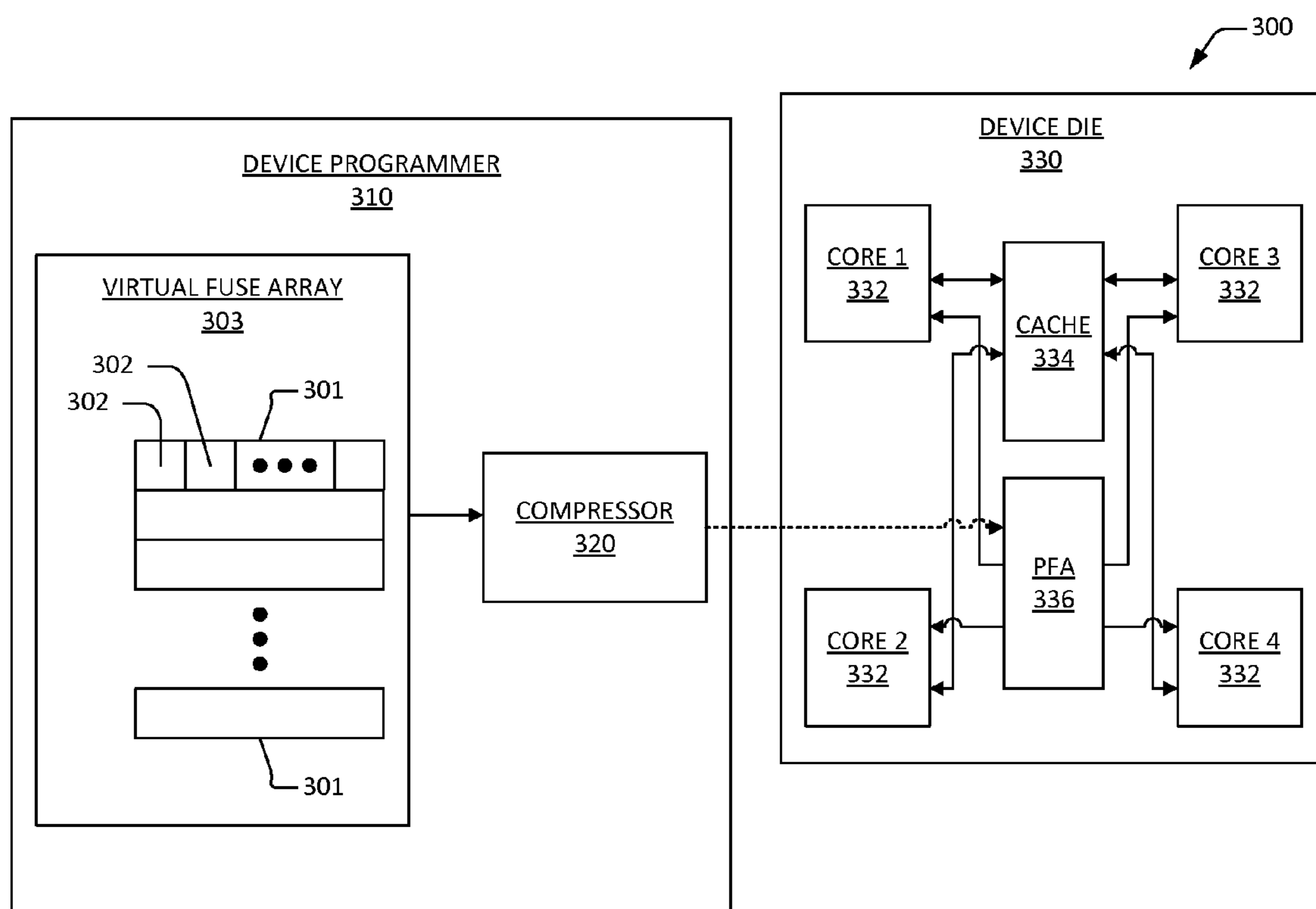
MICROPROCESSOR FUSE ARRAY COMPRESSION SYSTEM
