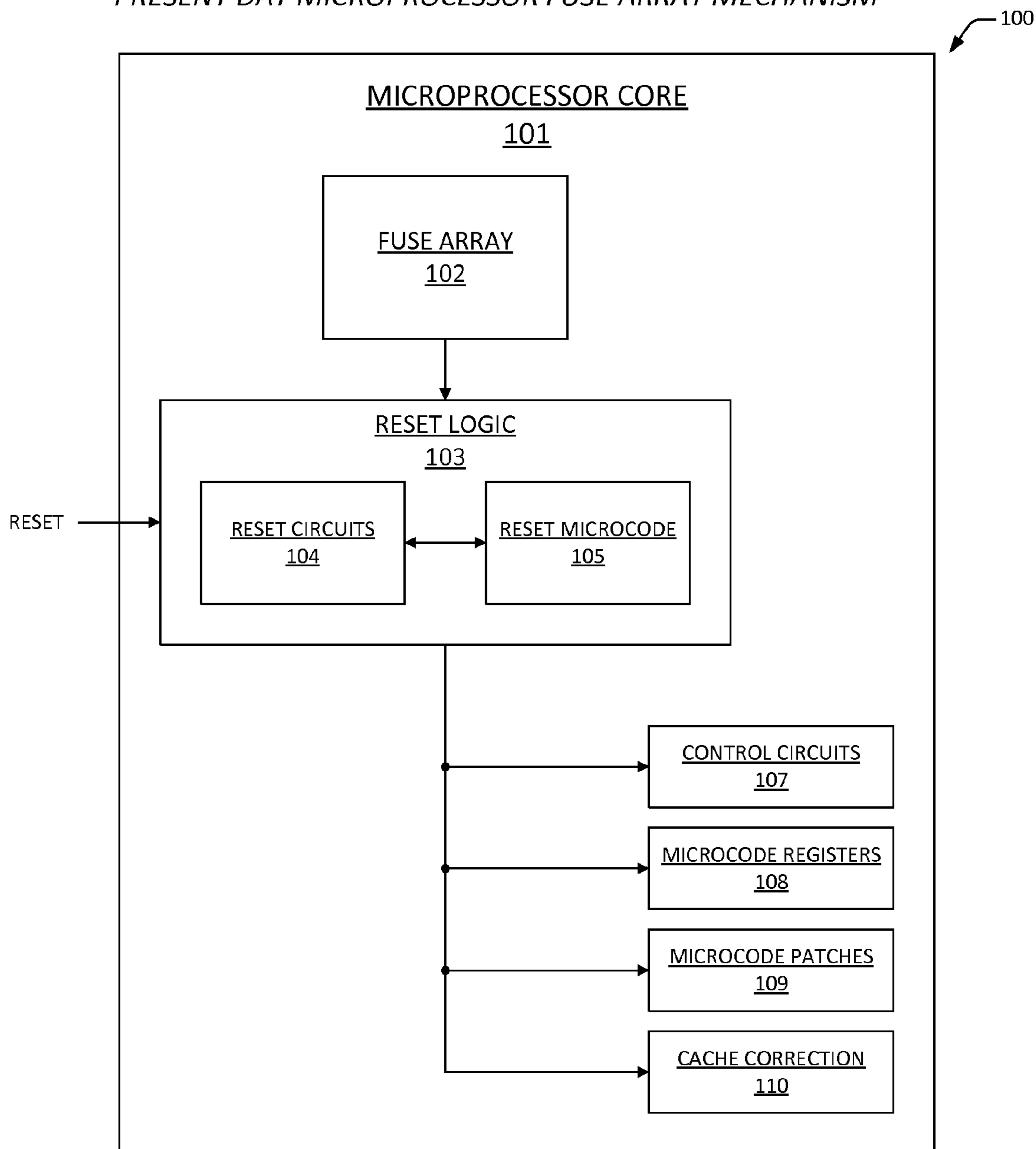
PRESENT DAY MICROPROCESSOR FUSE ARRAY MECHANISM
