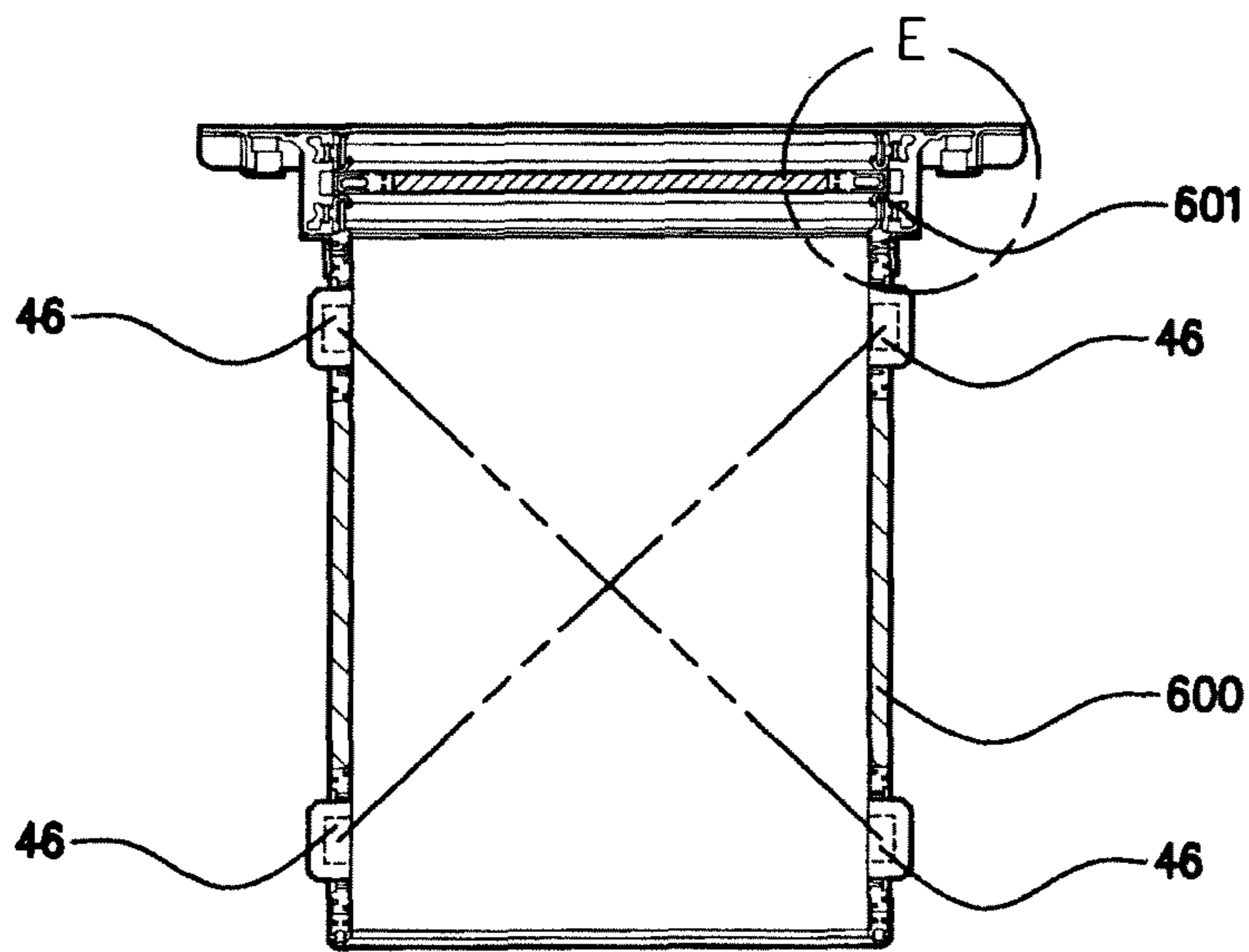
SECTION B-B
