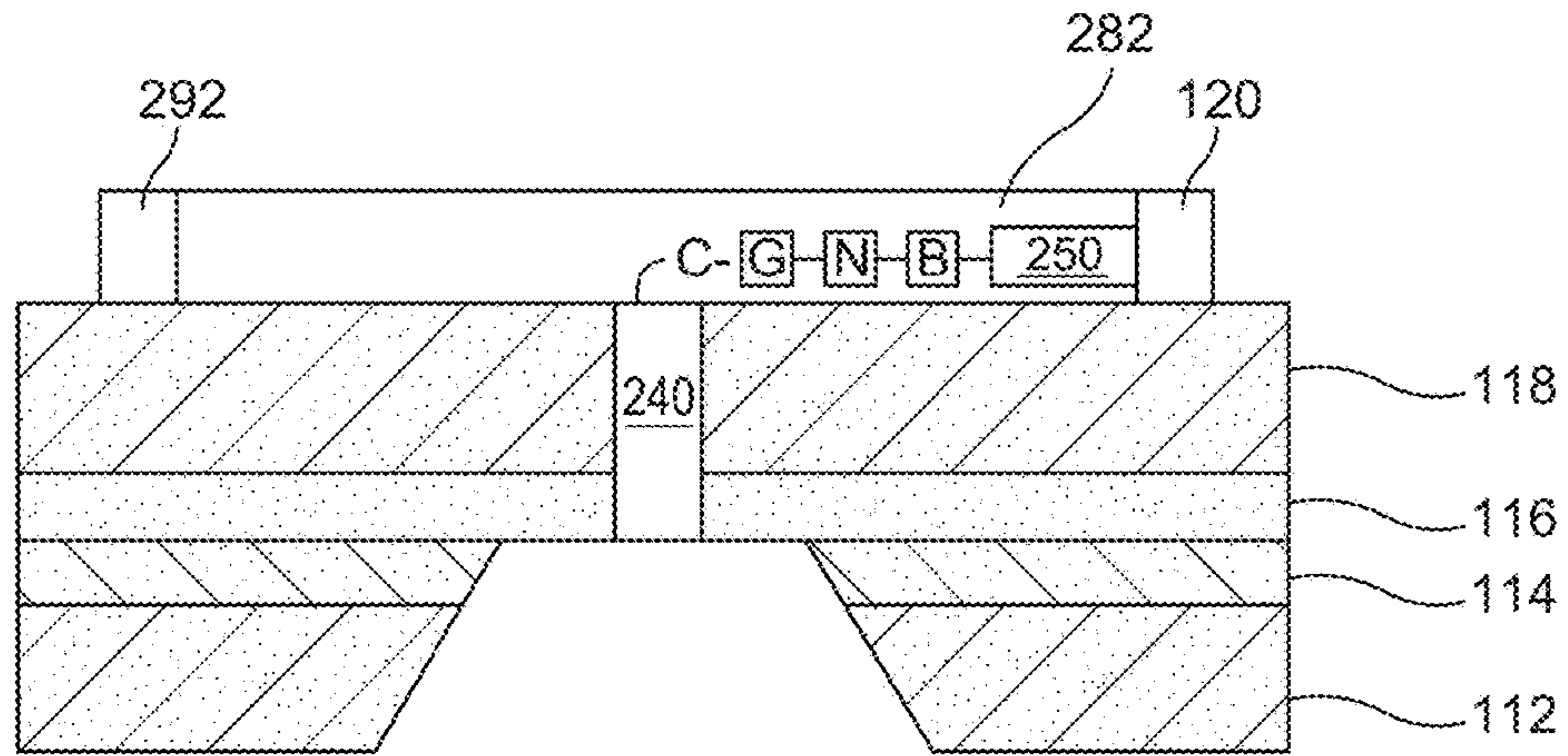
Add Ring-shaped Pd Connecting Layer FIG. 2L
