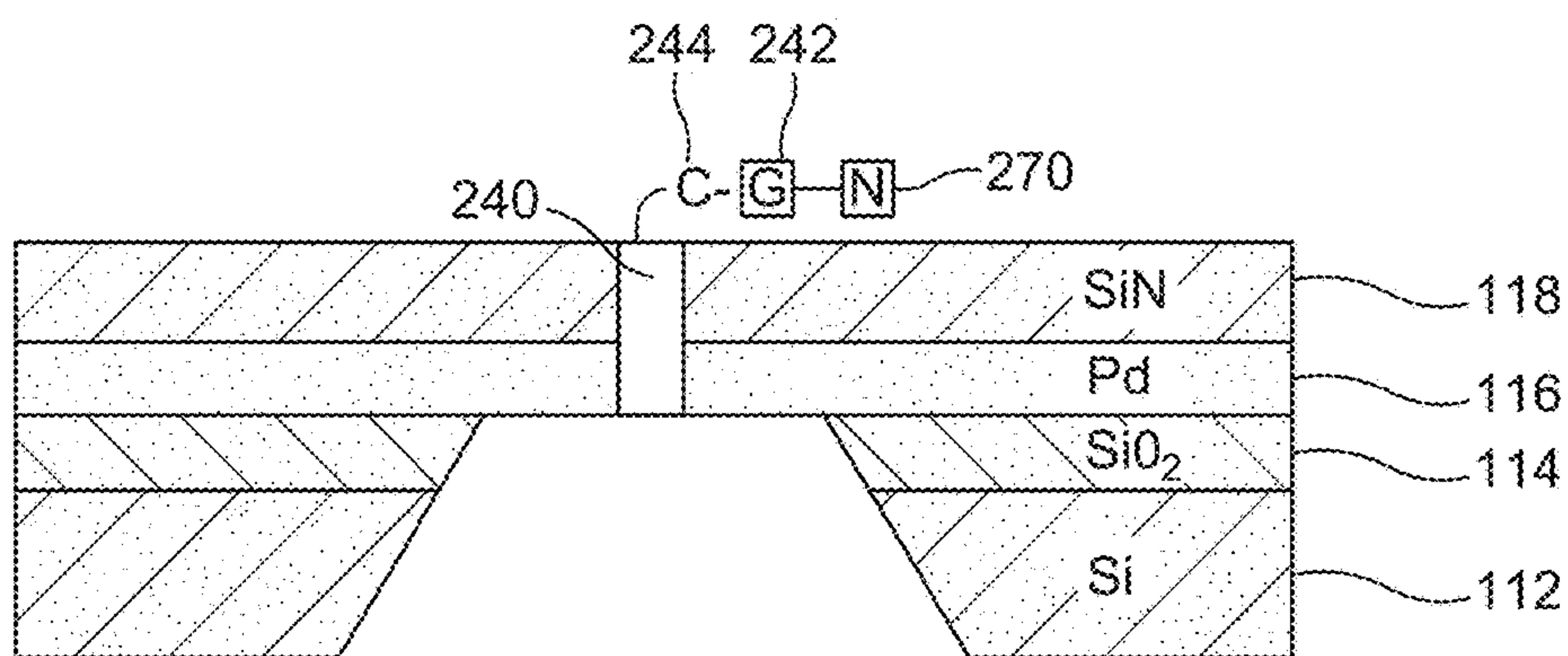
Attach Nucleotide to Guanidinium
