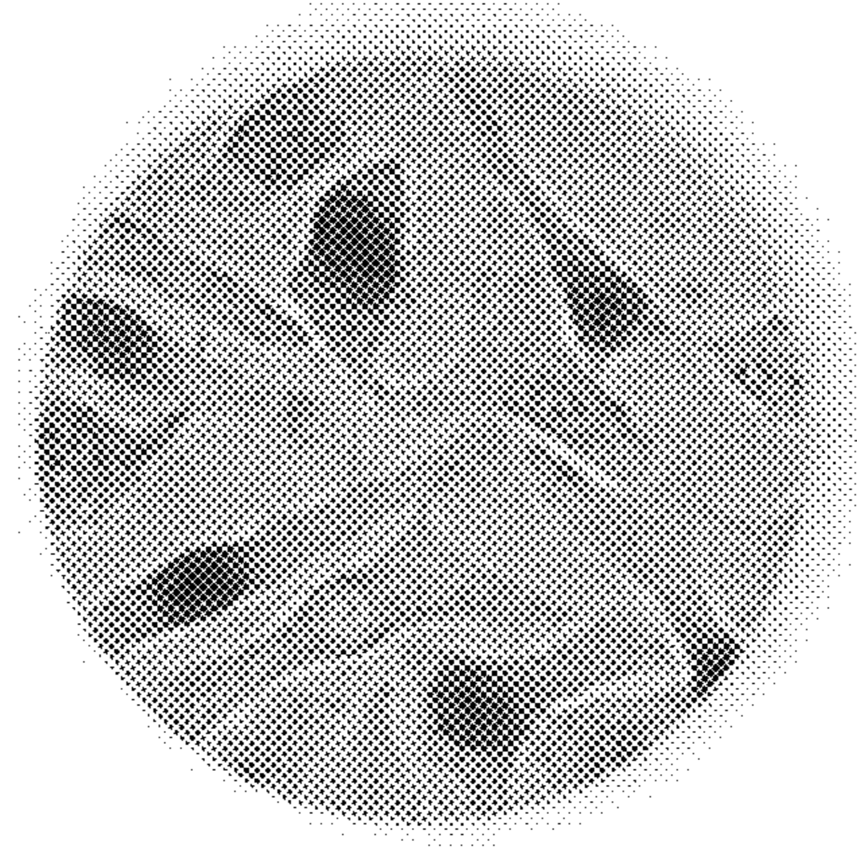
CRE Recombinase Plasmid
