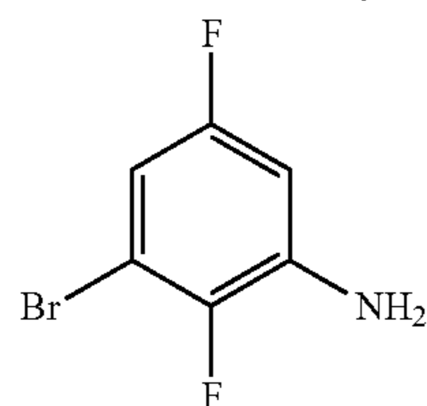
3-bromo-2,5-difluoroaniline
