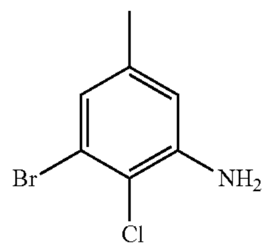
3-bromo-2-chloro-5-methylaniline
