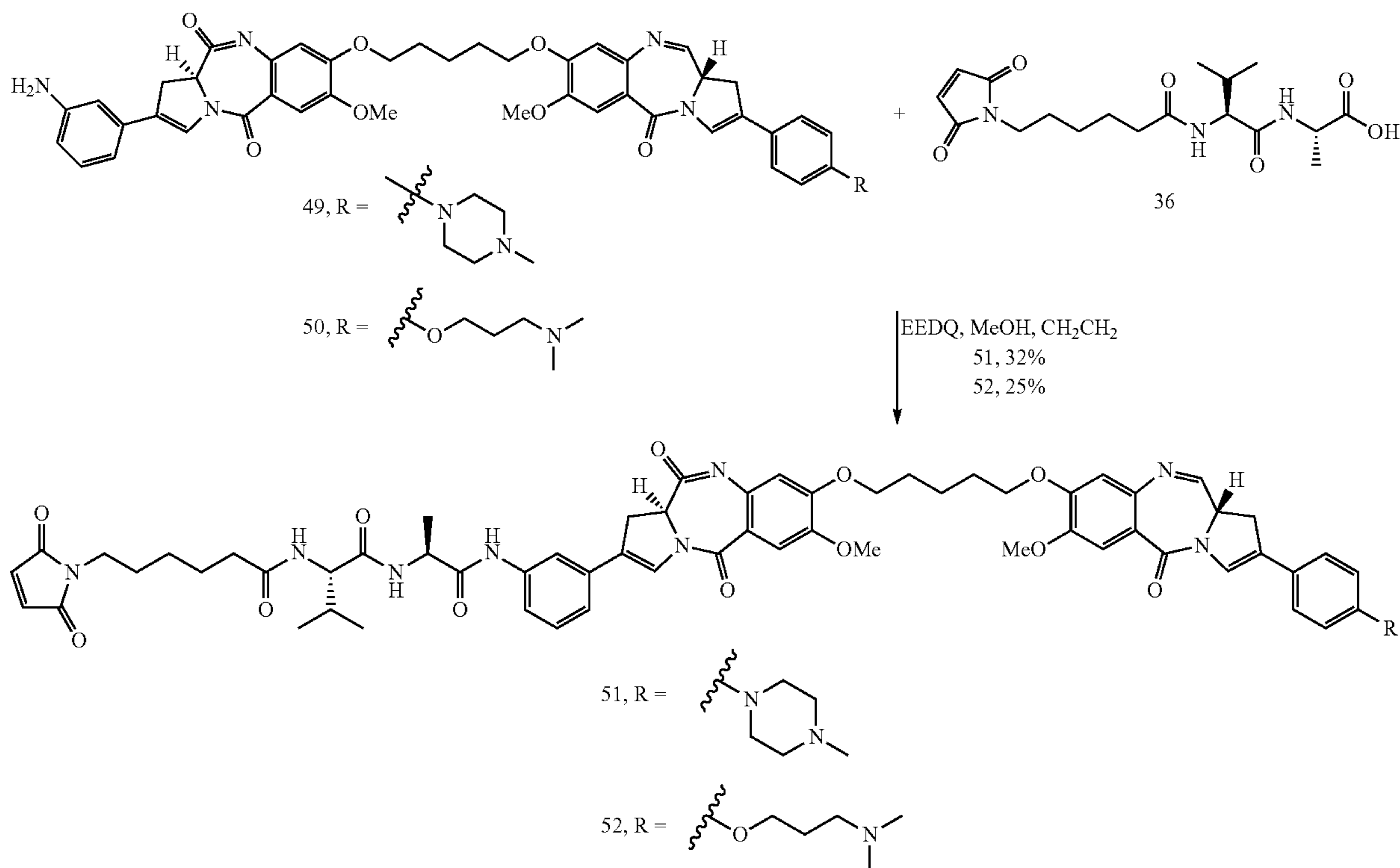
Scheme 7
