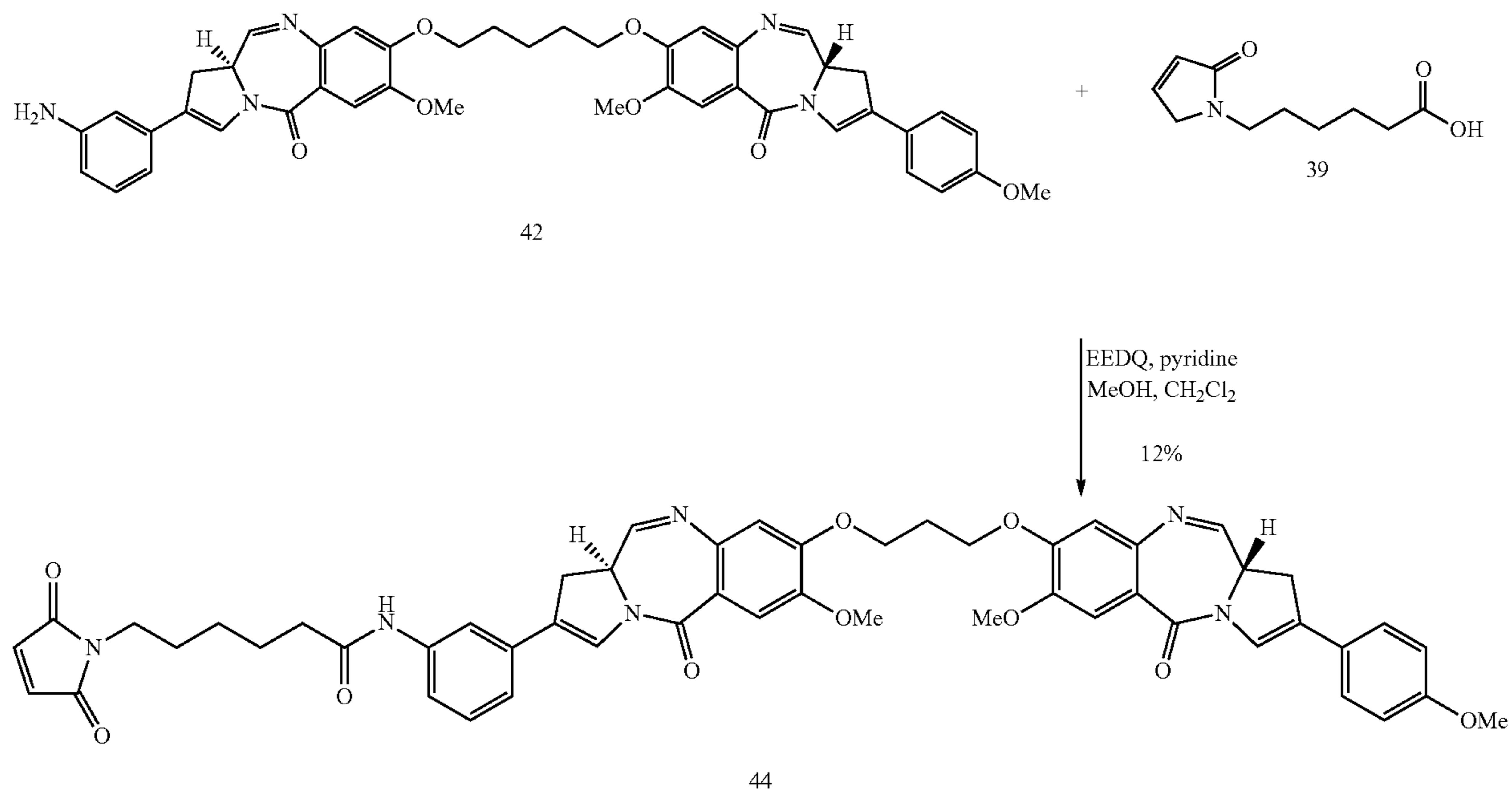
Scheme 5
