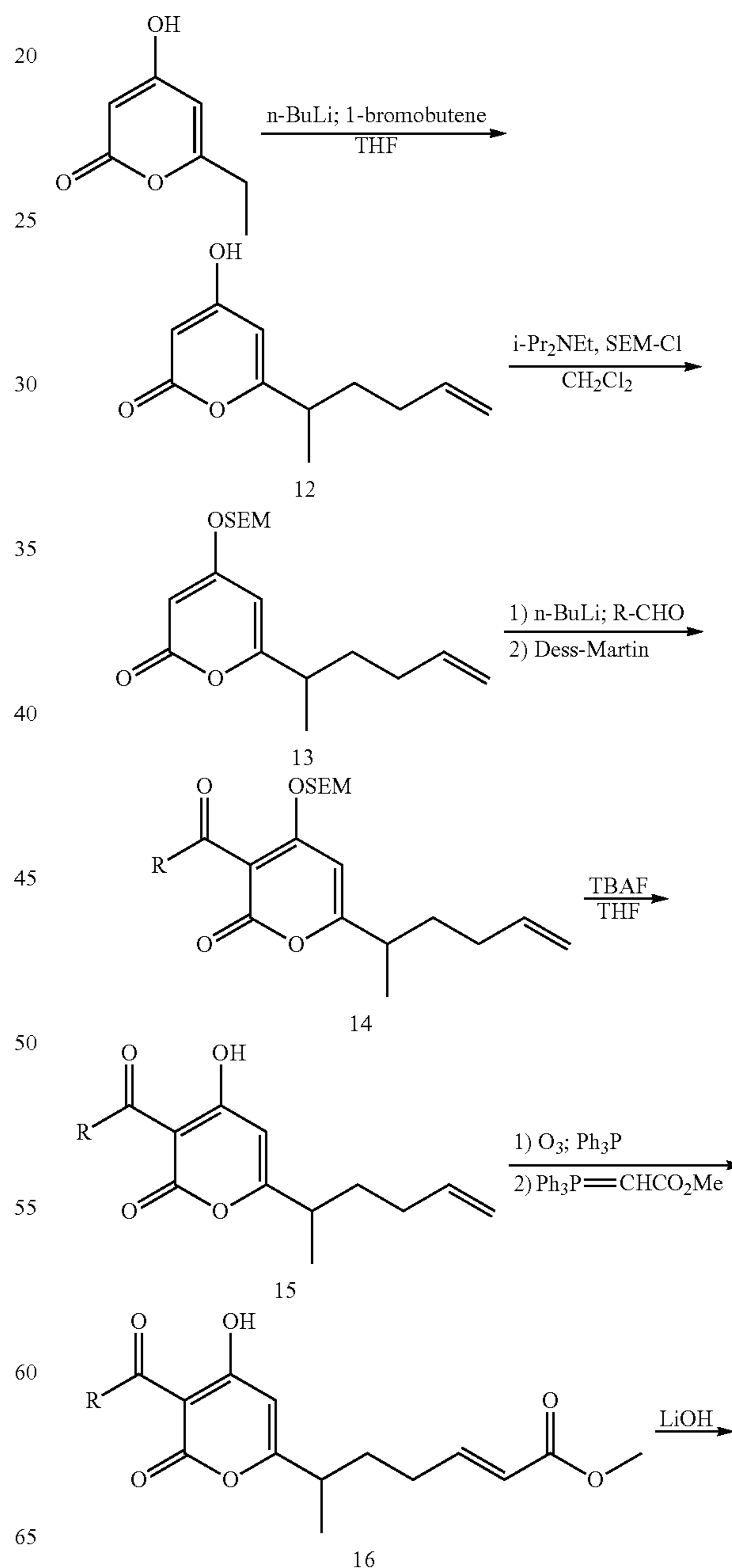
Scheme 4: General Scheme for Preparing Certain Compounds of Formulae Ia-Ic: Method D
