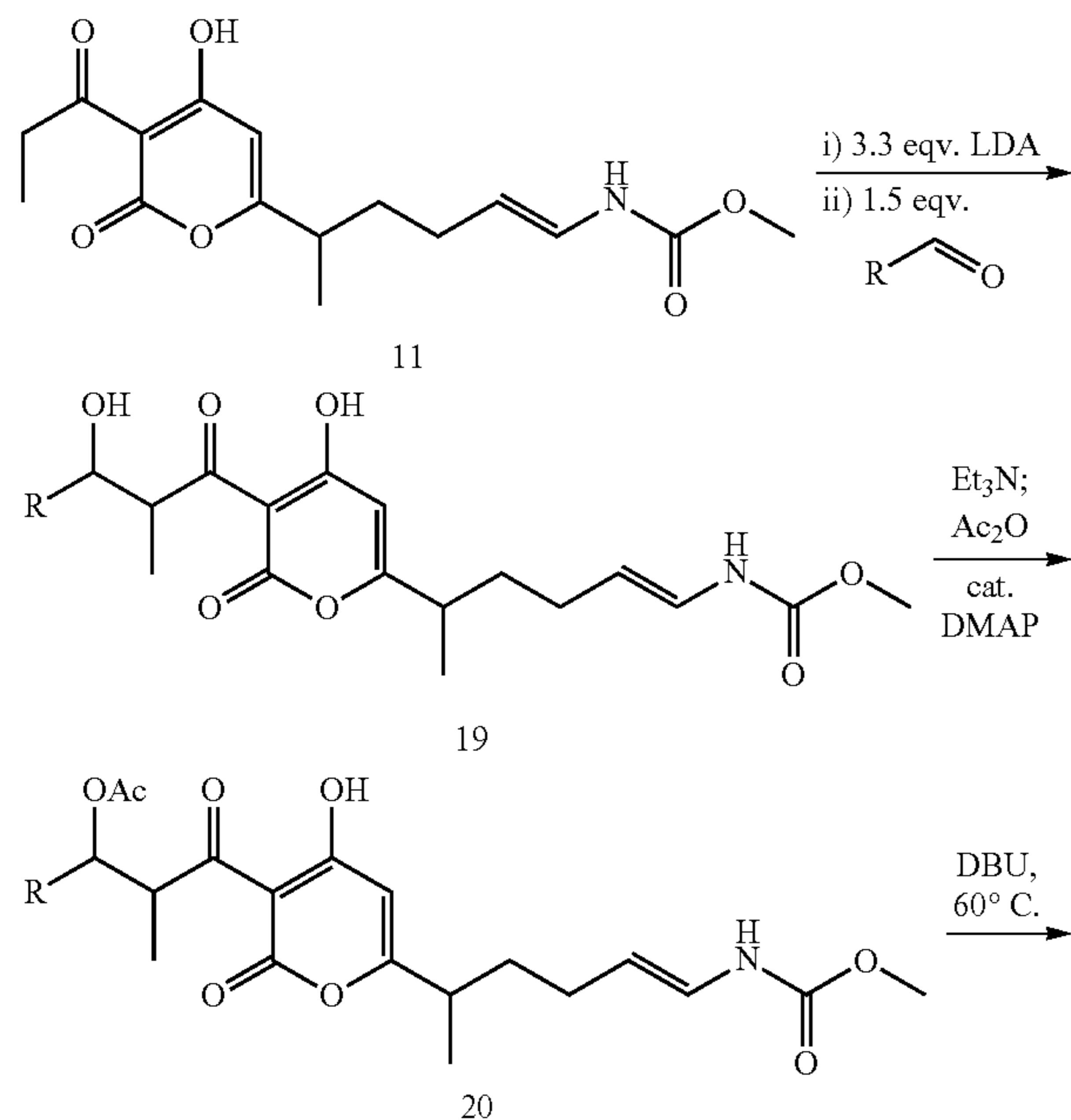
Scheme 5: General Scheme for Preparing Certain Compounds of Formulae Ia-Ic: Method E
