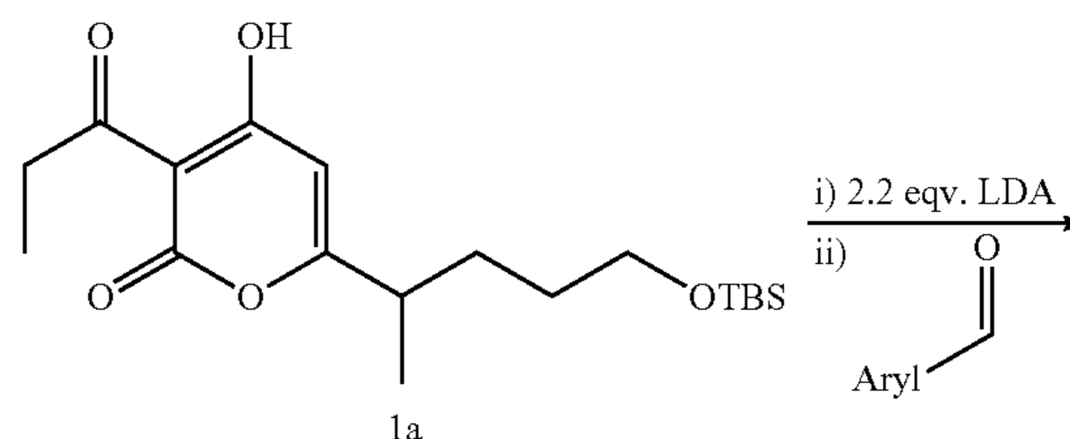
Scheme 1: General Scheme for Preparing Certain Compounds of Formulae Ia-Ic: Method A
