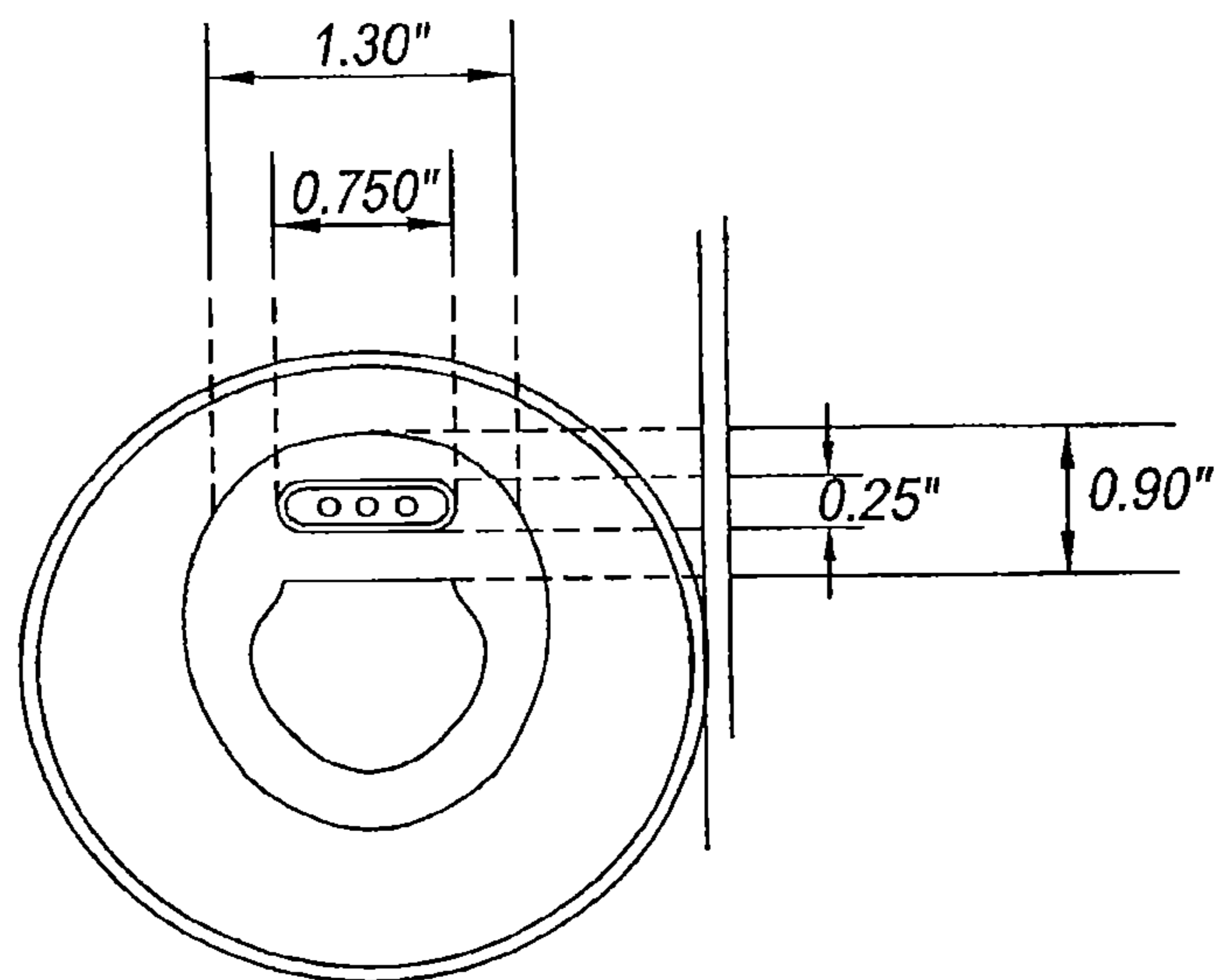
Fig. 20 (Prior Art)
