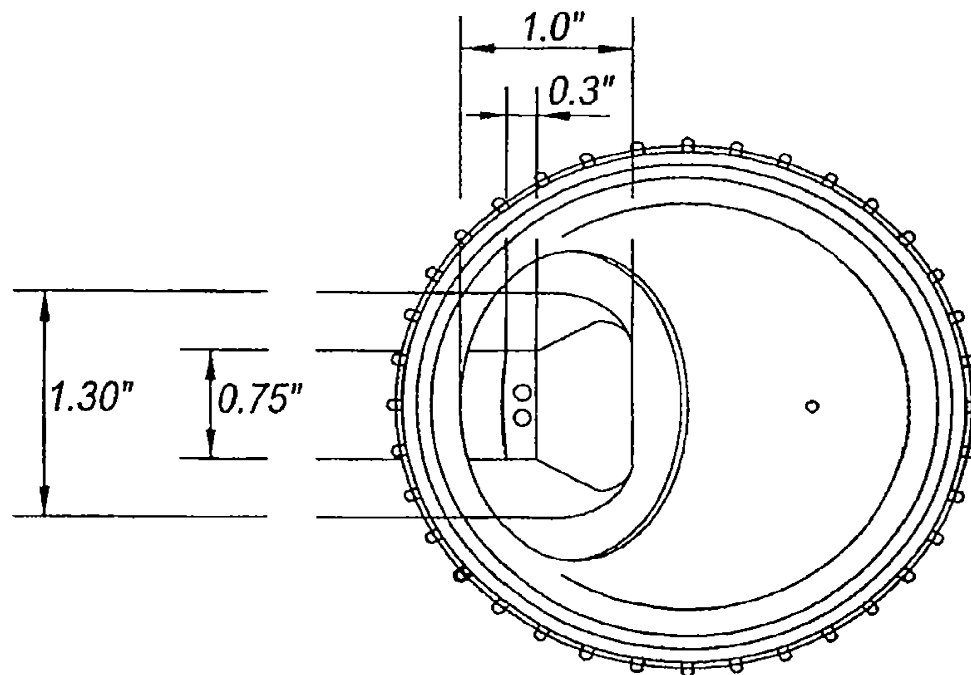
Fig. 17 (Prior Art)
