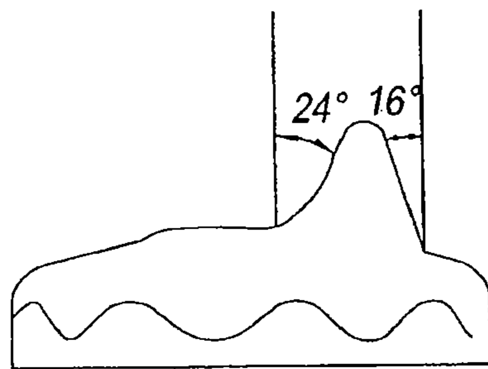
Fig. 19 (Prior Art)
