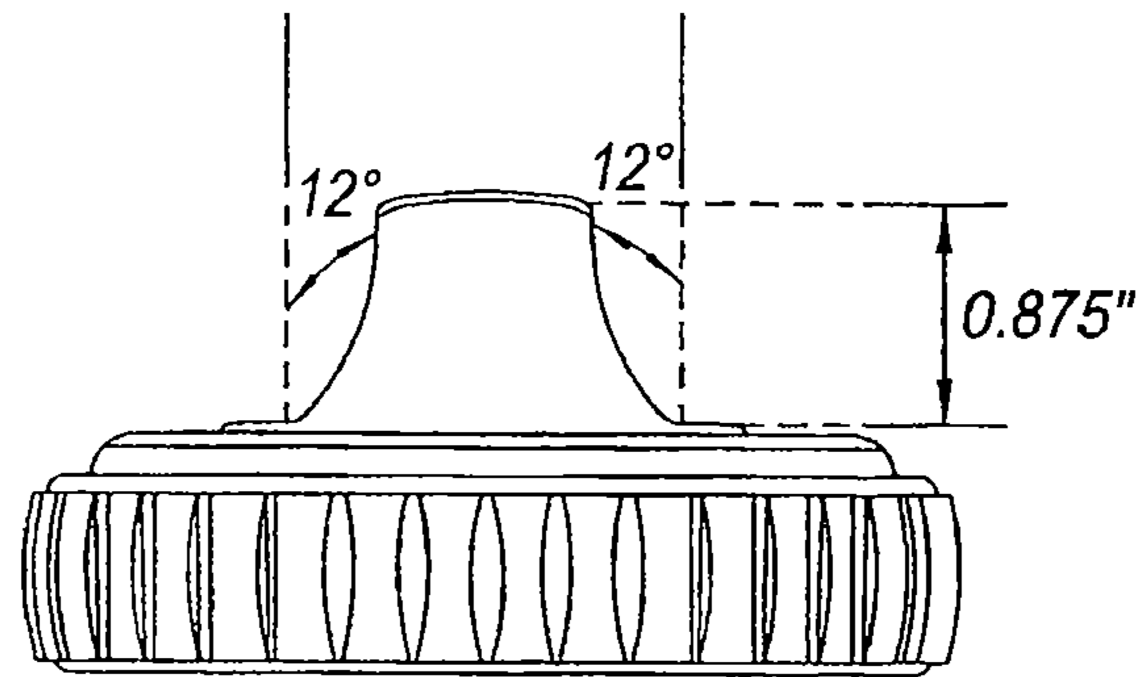
Fig. 15 (Prior Art)
