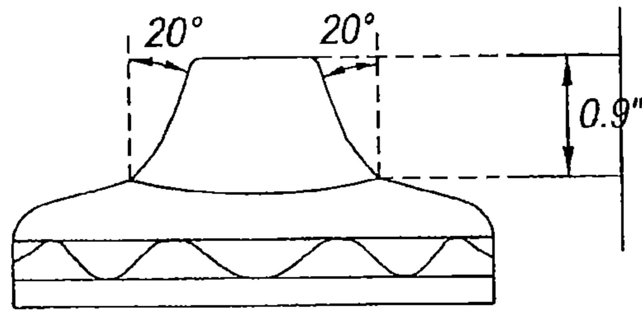
Fig. 18 (Prior Art)
