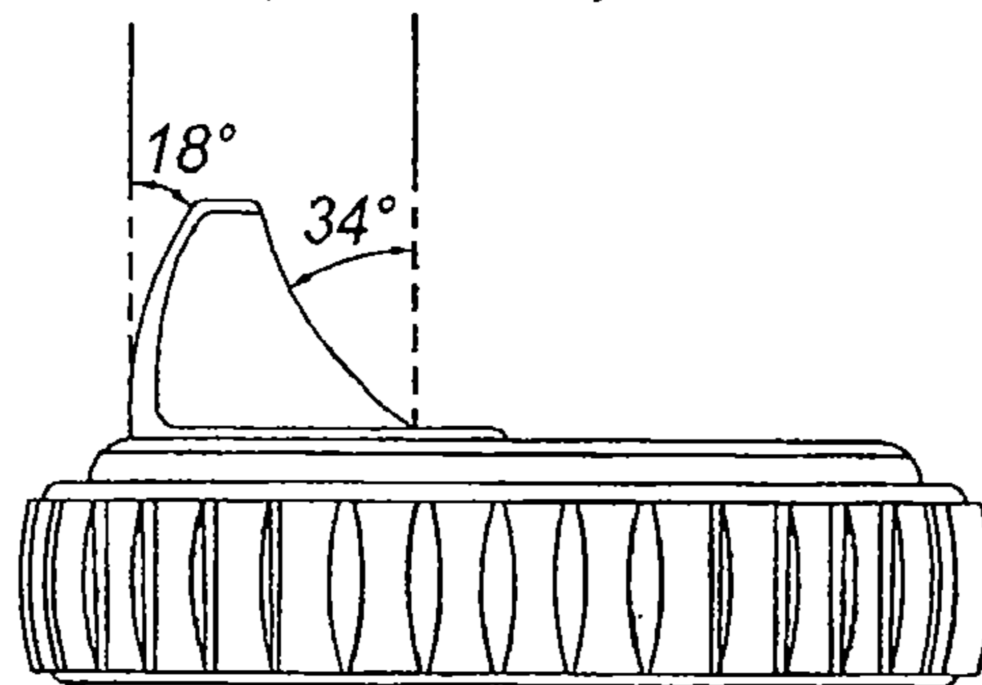
Fig. 16 (Prior Art)
