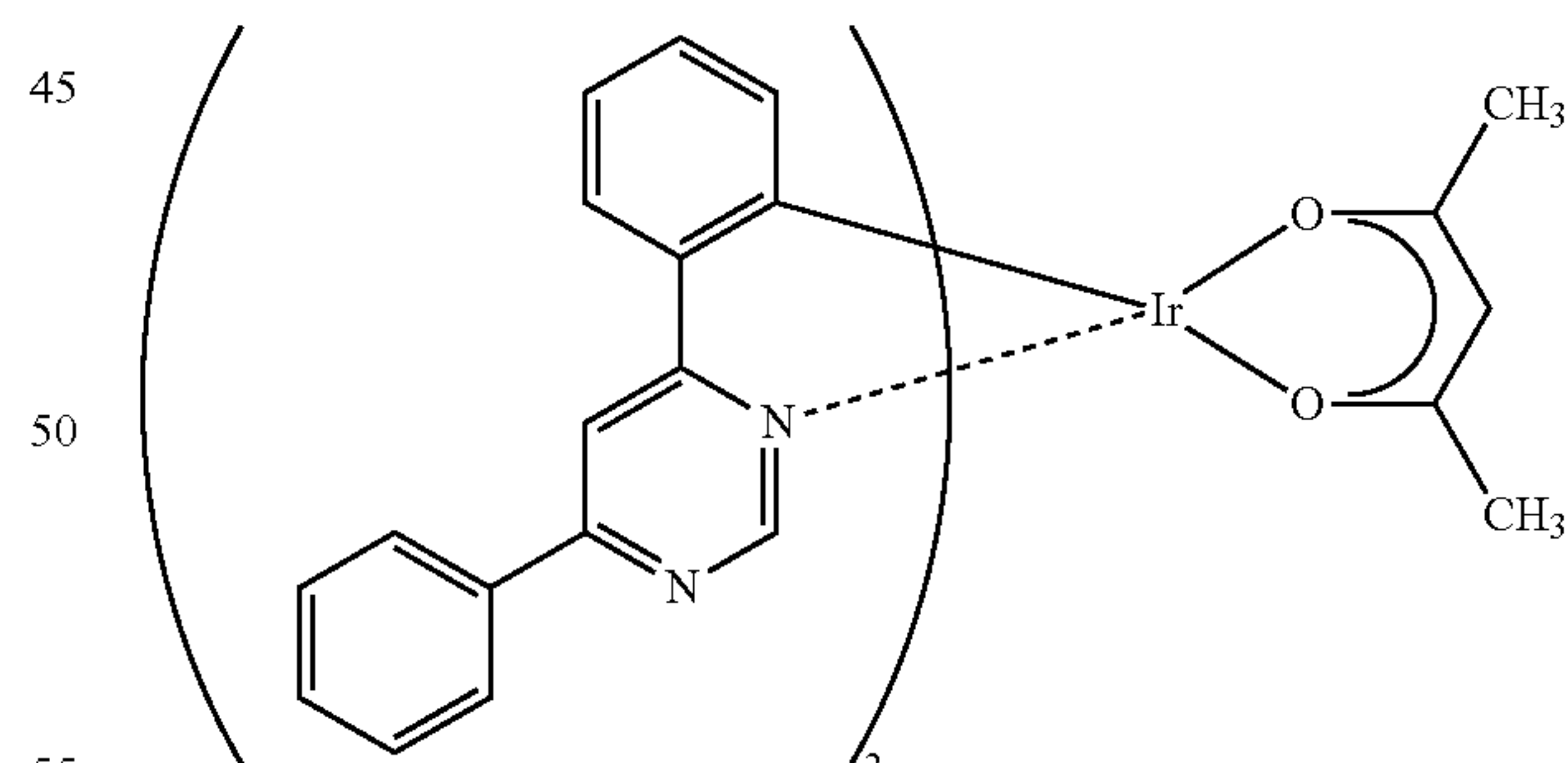
[Ir(dppm) 2 (acac)]
