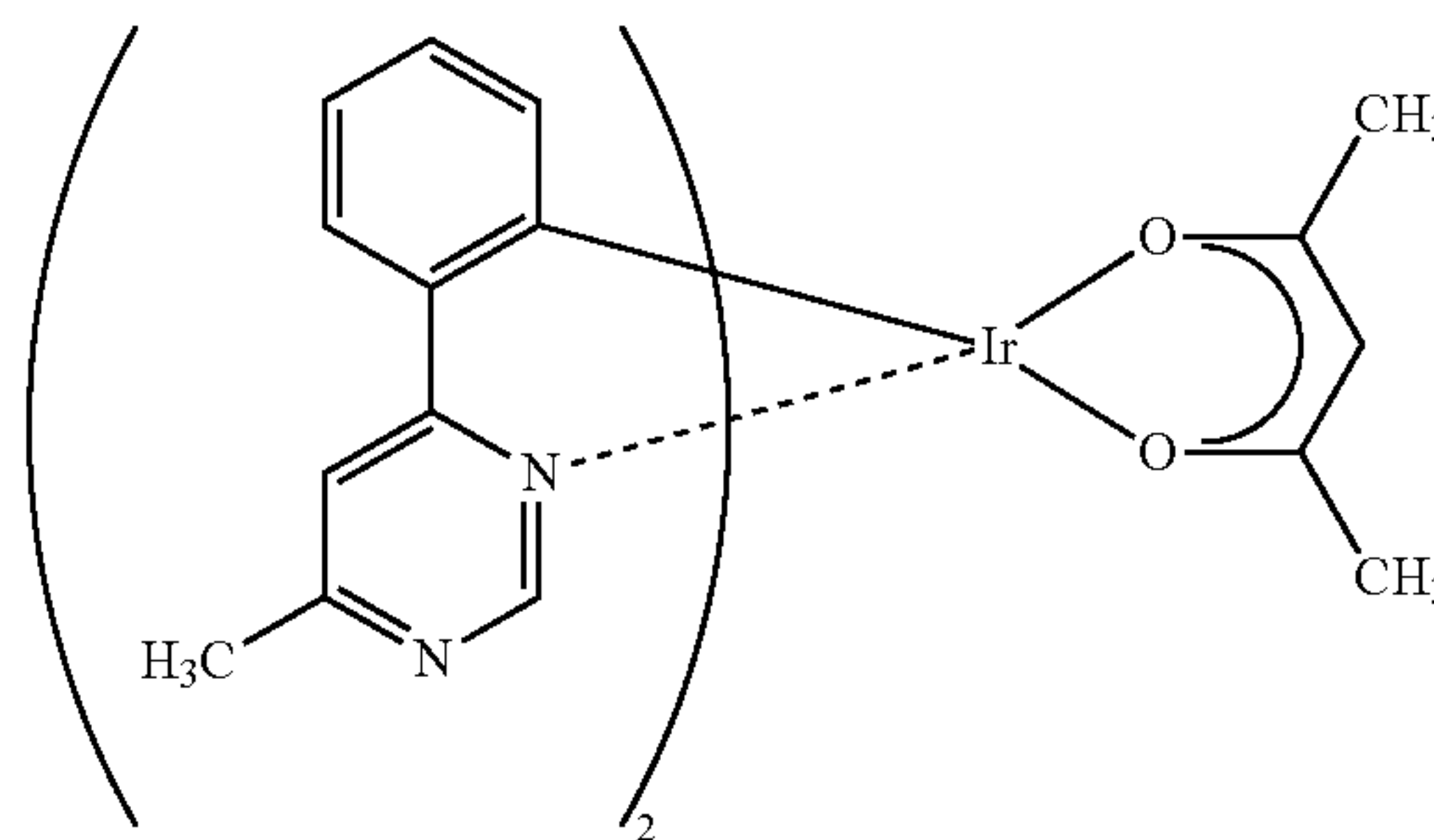
[\text{Ir}(\text{mppm})_2(\text{acac})]
