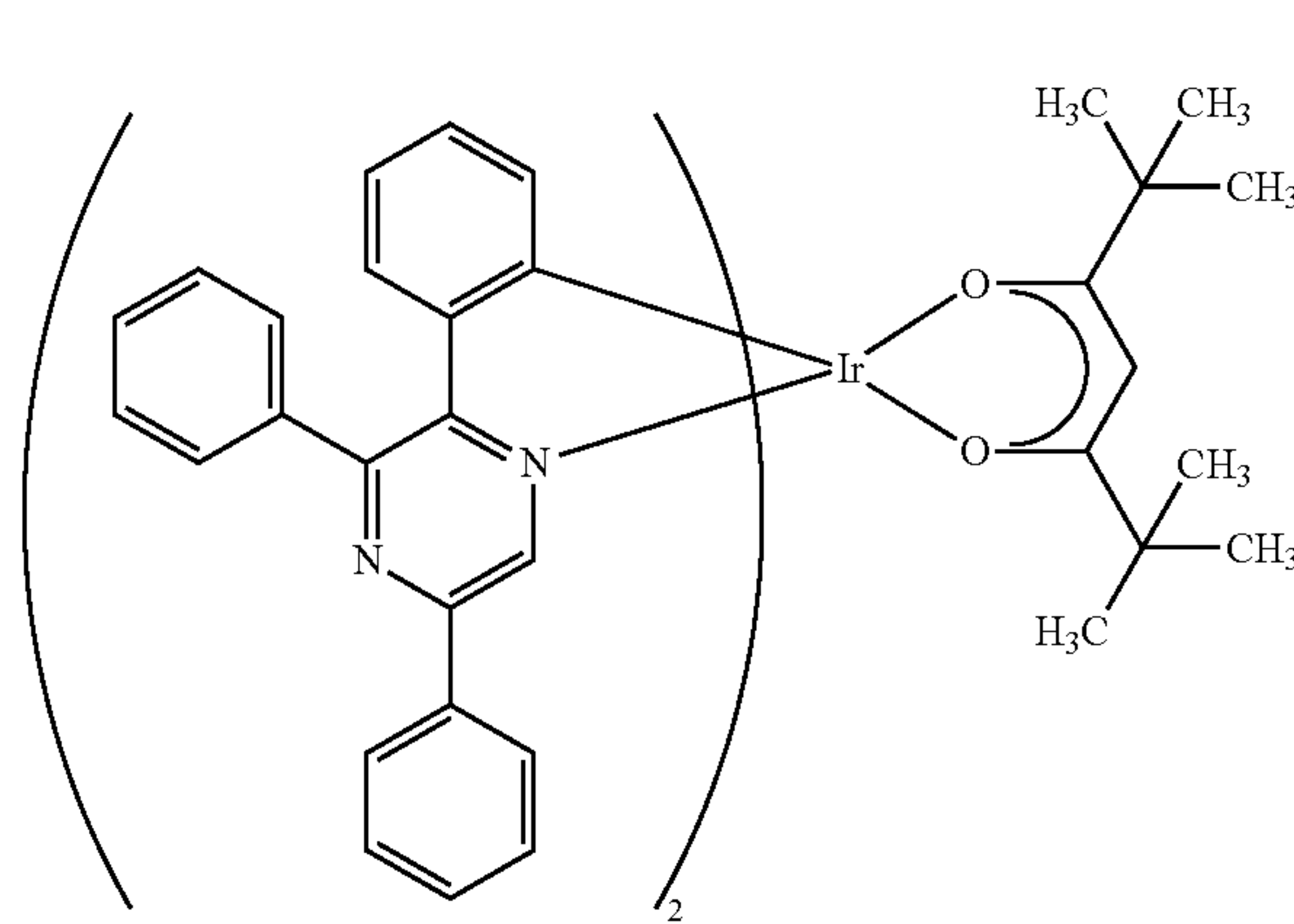
[\text{Ir}(\text{tppr})_2(\text{dpm})]
