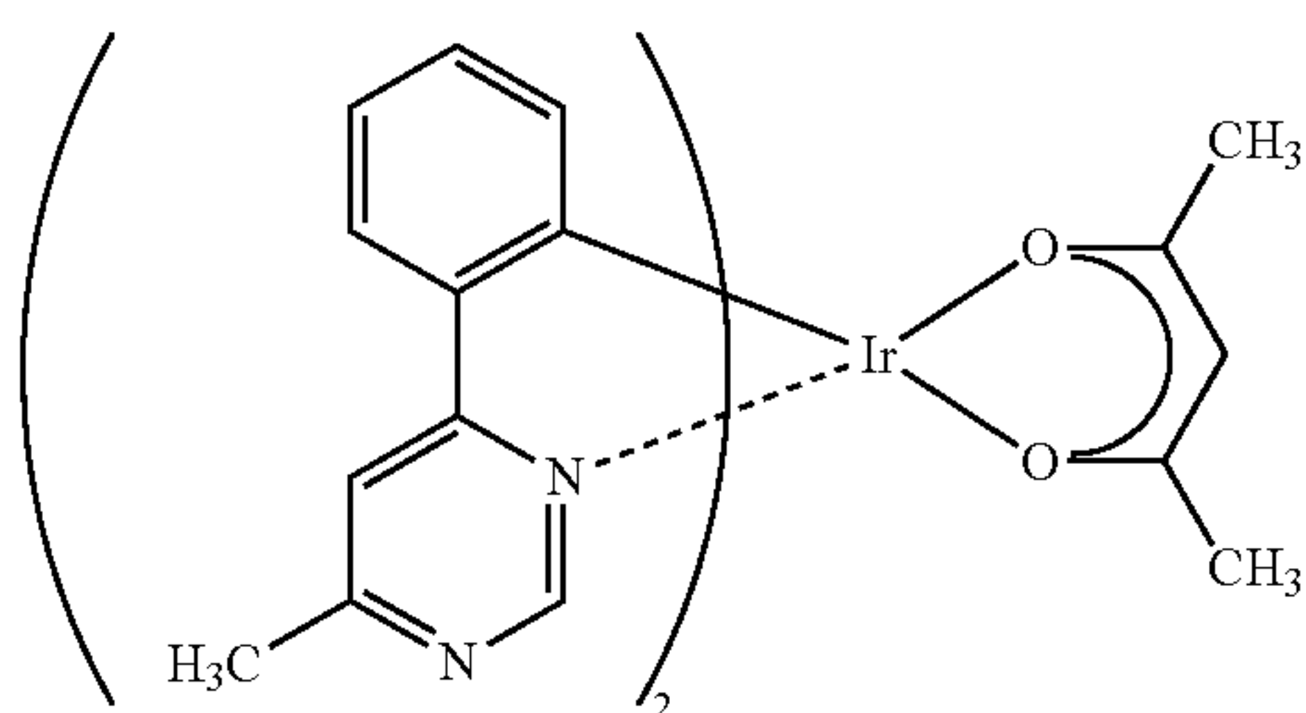
[Ir(mppm) 2 (acac)]
