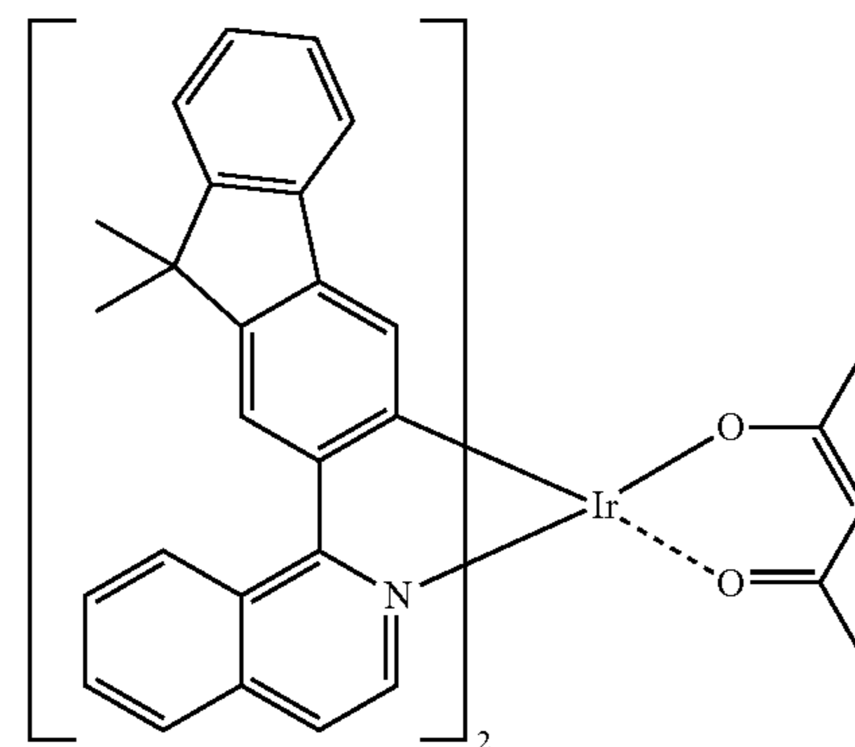
It(fliq) 2 (acac)
