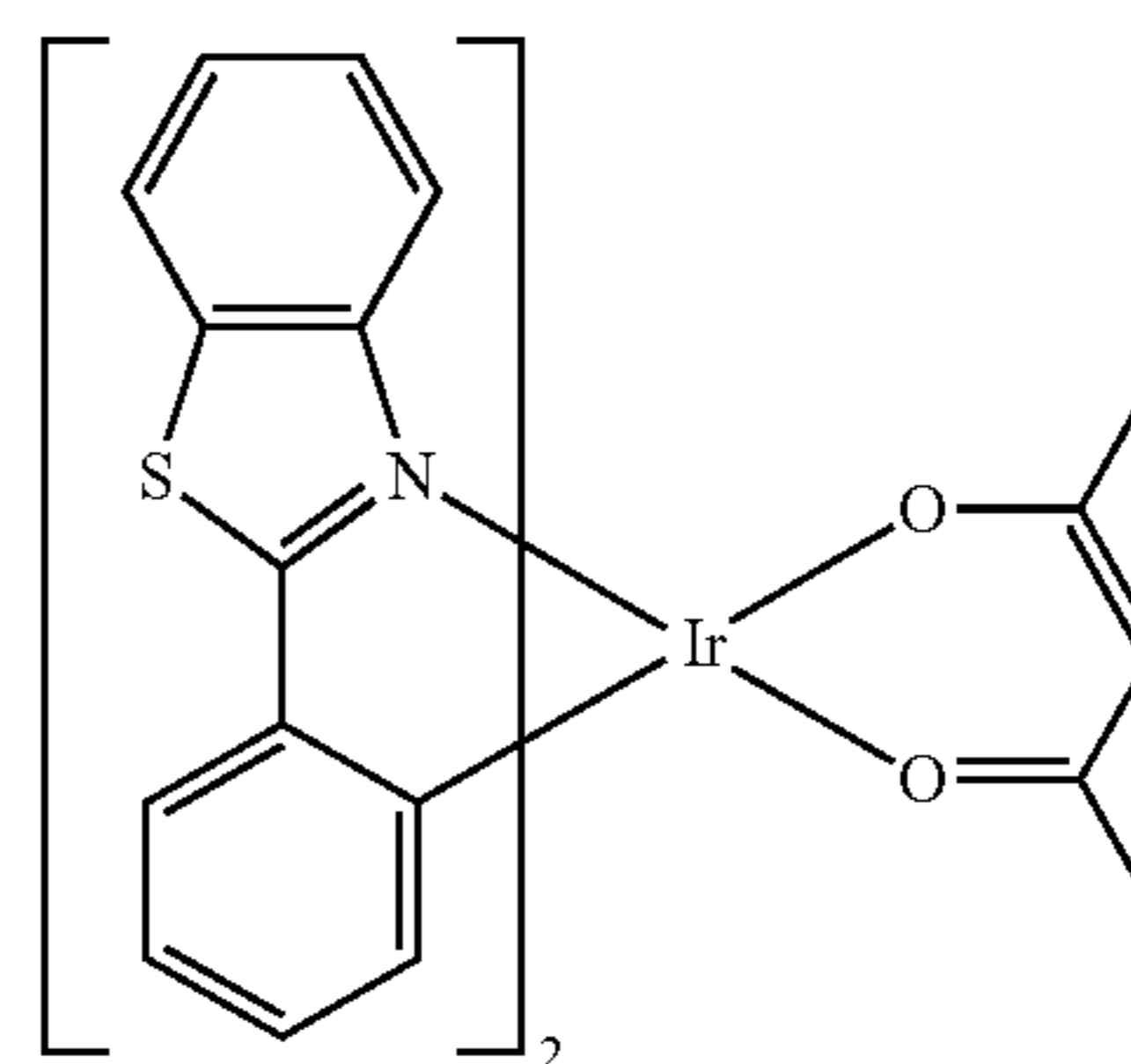
Ir(BT) 2 (acac)
