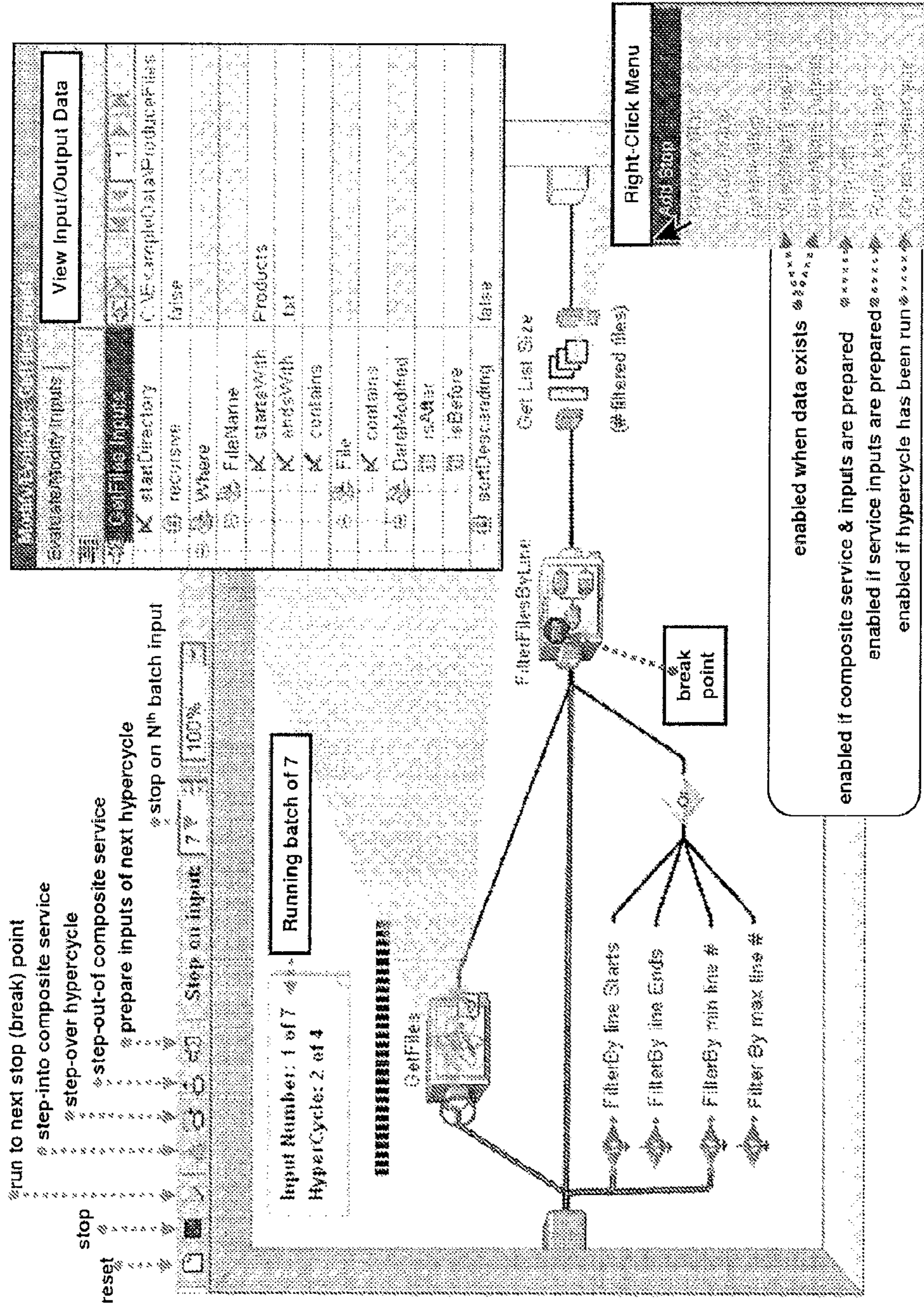
FIG. 14 Semantic-Based Debugger
