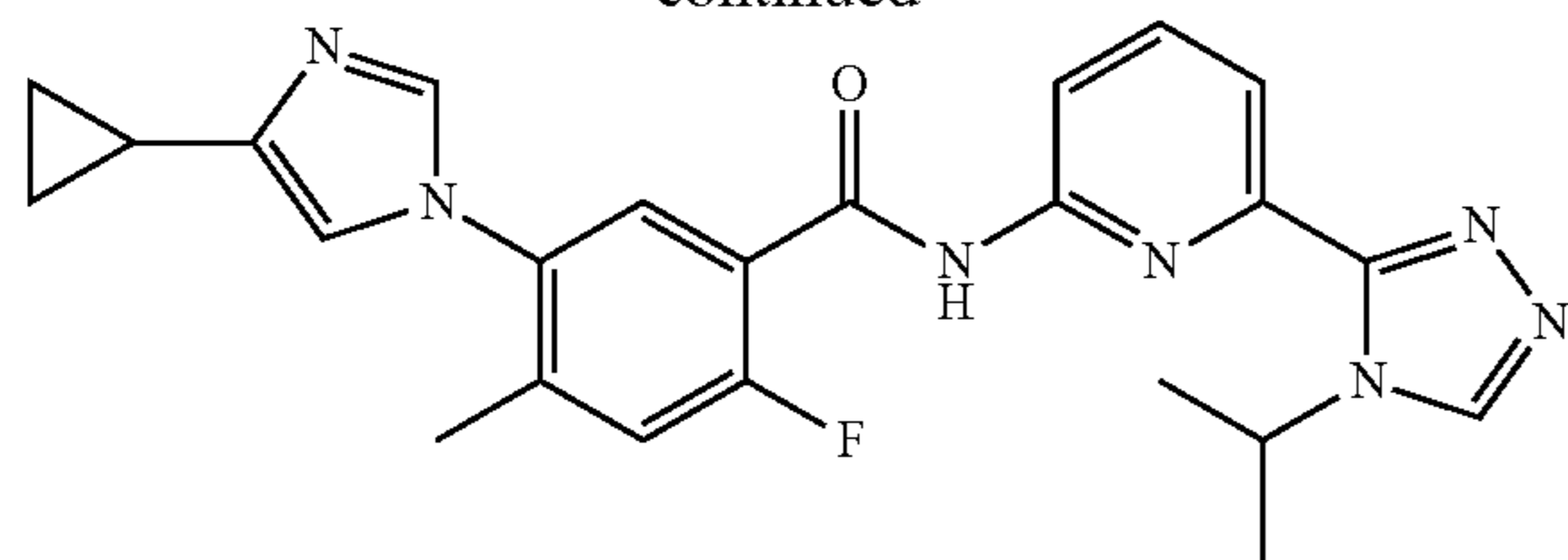
Compound (A)
