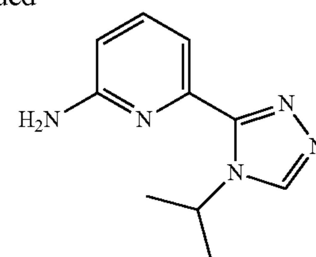
Compound (C)
