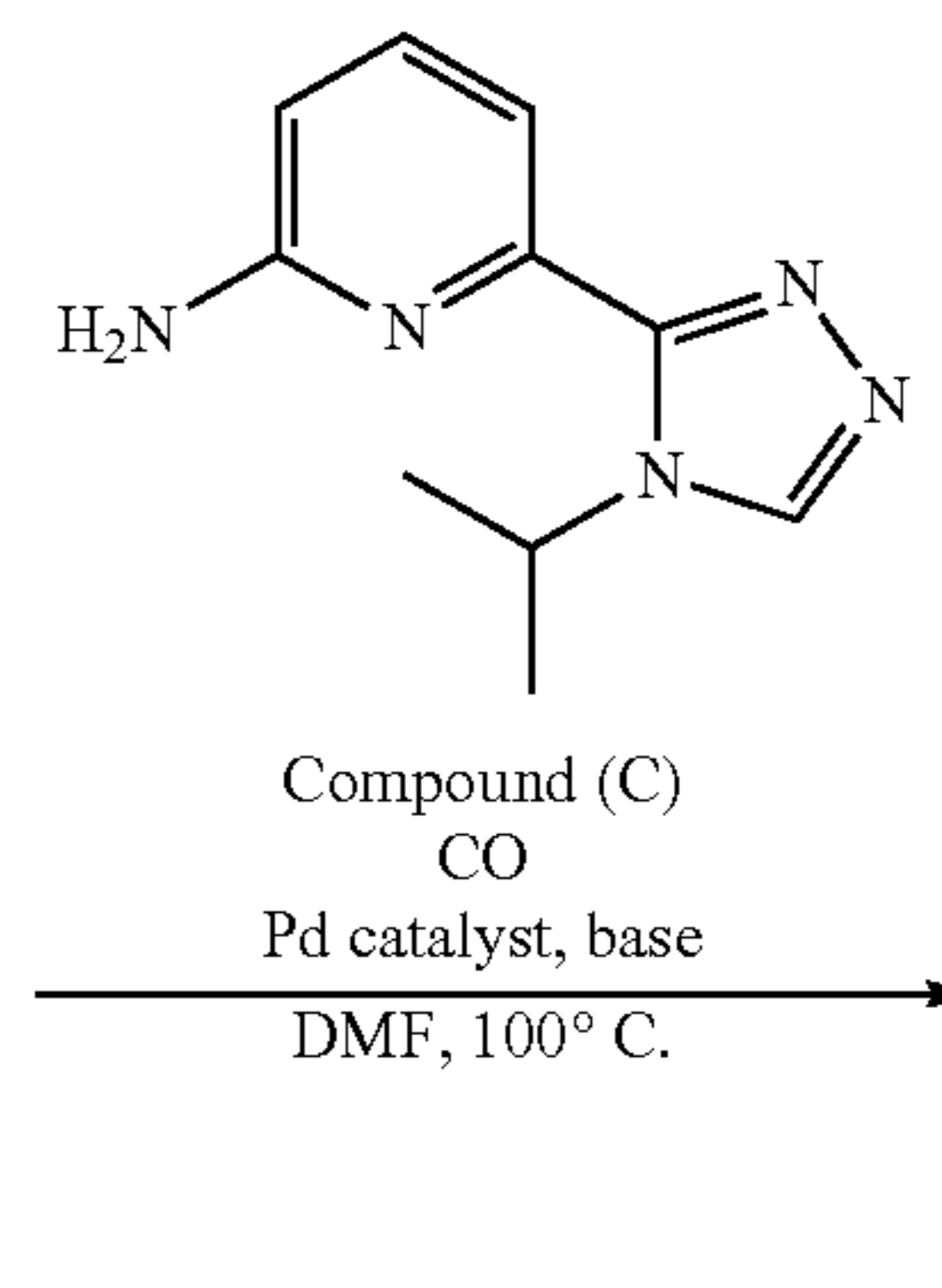
Scheme 3
