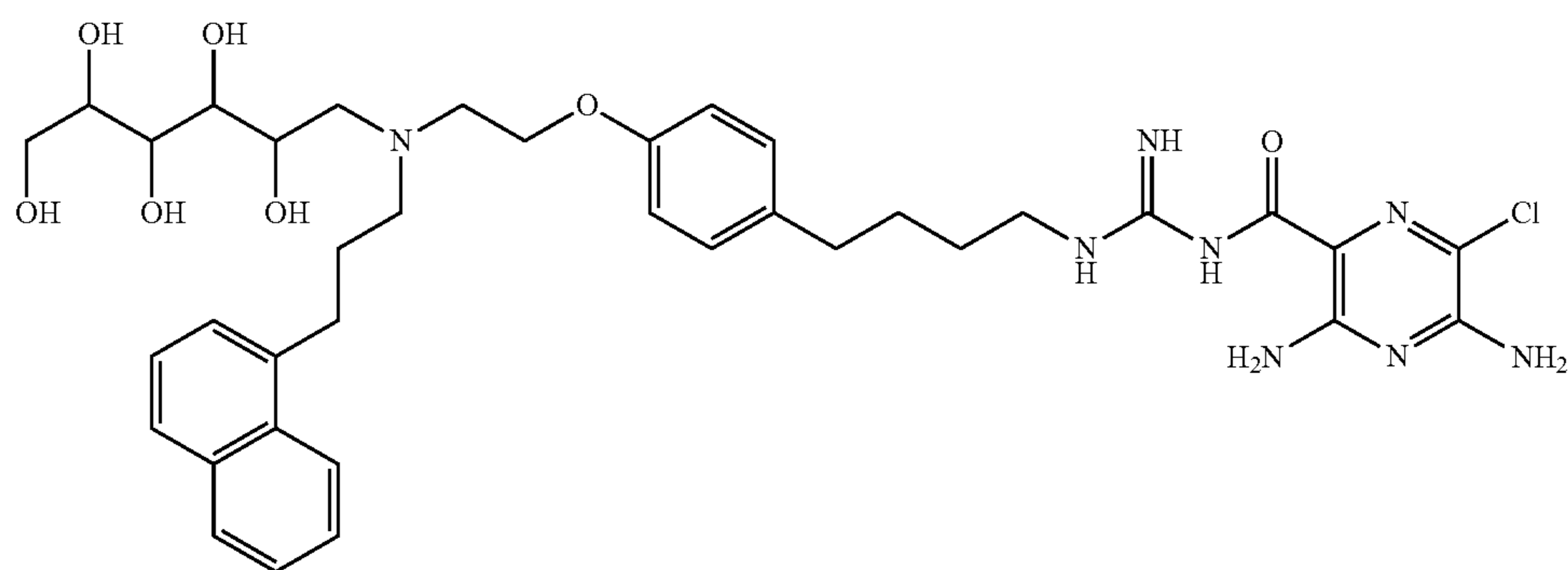
50 3,5-diamino-6-chloro-N-(N-(4-(4-(2-((3-(naphthalen-1-yl)propyl)(2,3,4,5,6-pentahydroxyhexyl)amino)ethoxy)phenyl)butyl)carbamimidoyl)pyrazine-2-carboxamide;
