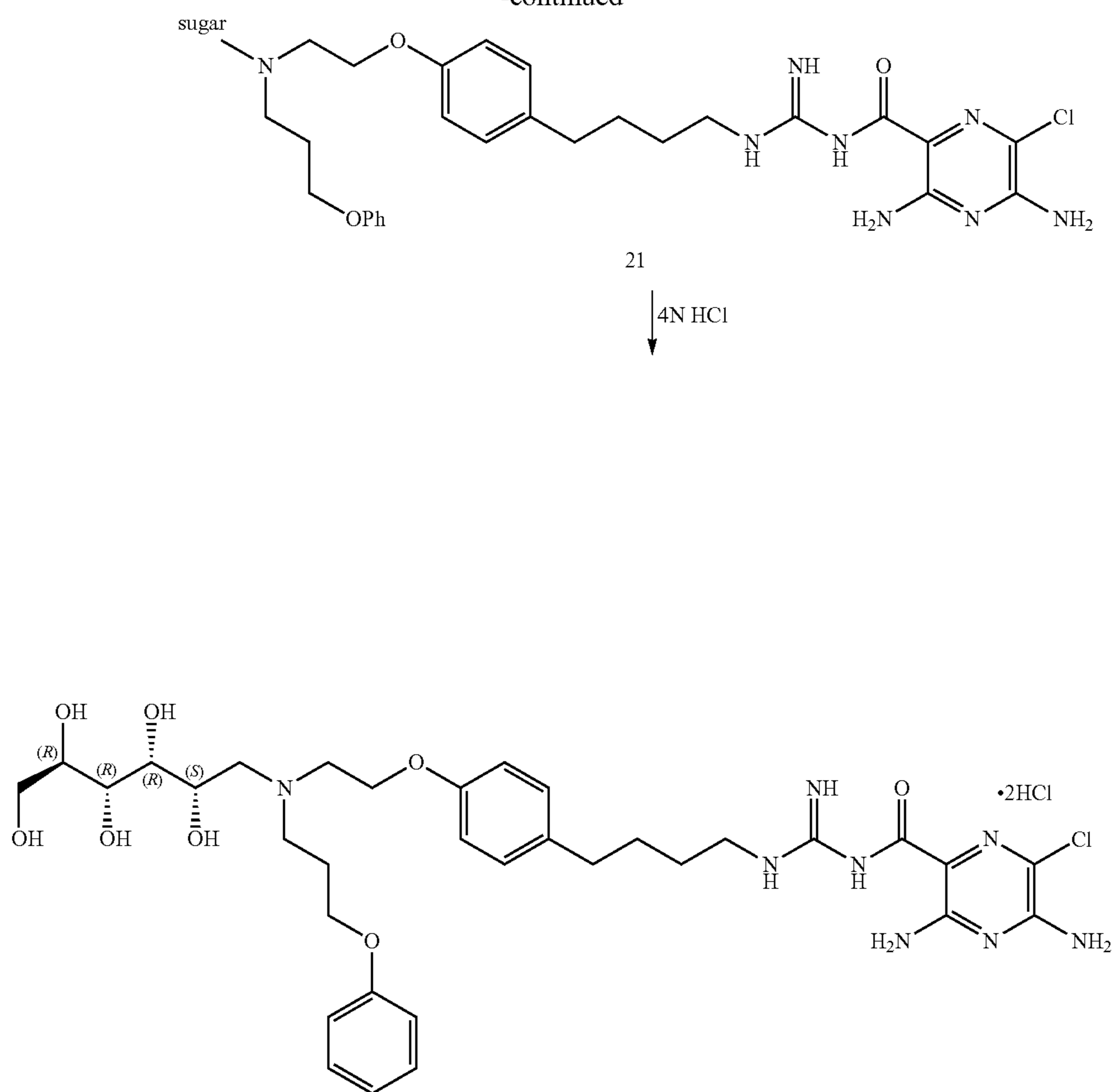
Compound 22
