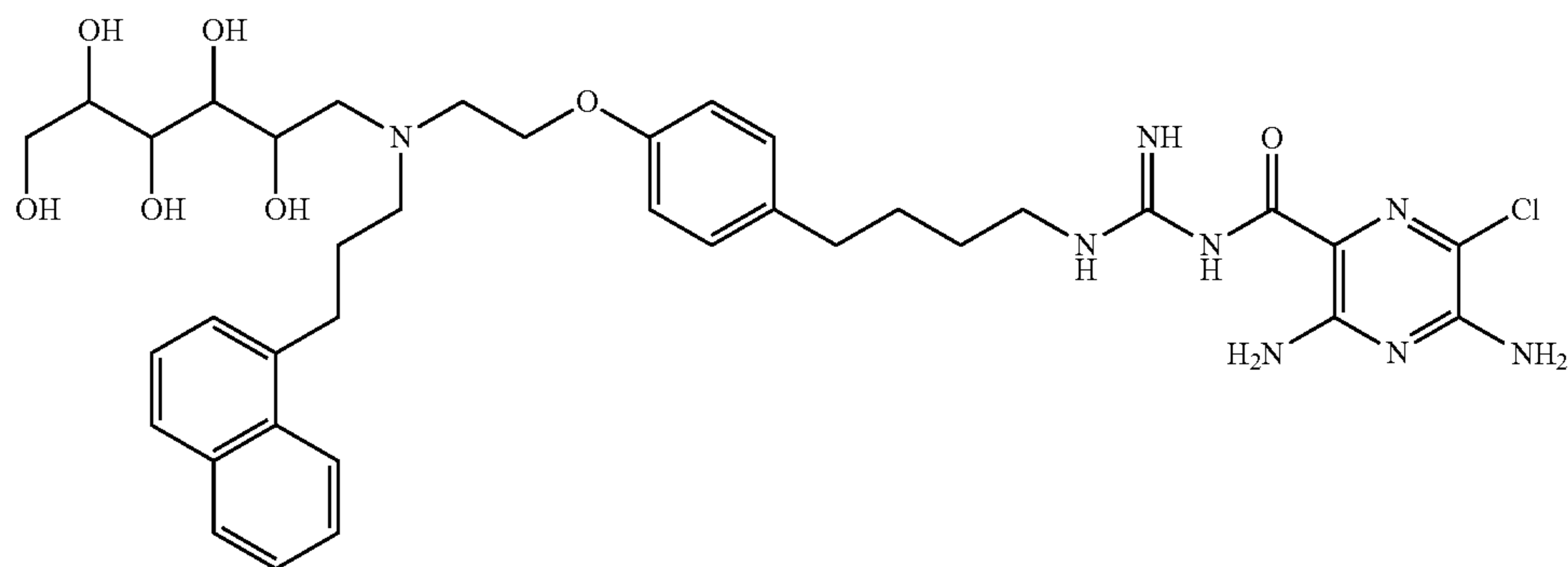
50 3,5-diamino-6-chloro-N-(N-(4-(4-(2-((3-(naphthalen-1-yl)propyl)(2,3,4,5,6-pentahydroxyhexyl)amino)ethoxy)phenyl)butyl)carbamimidoyl)pyrazine-2-carboxamide;
