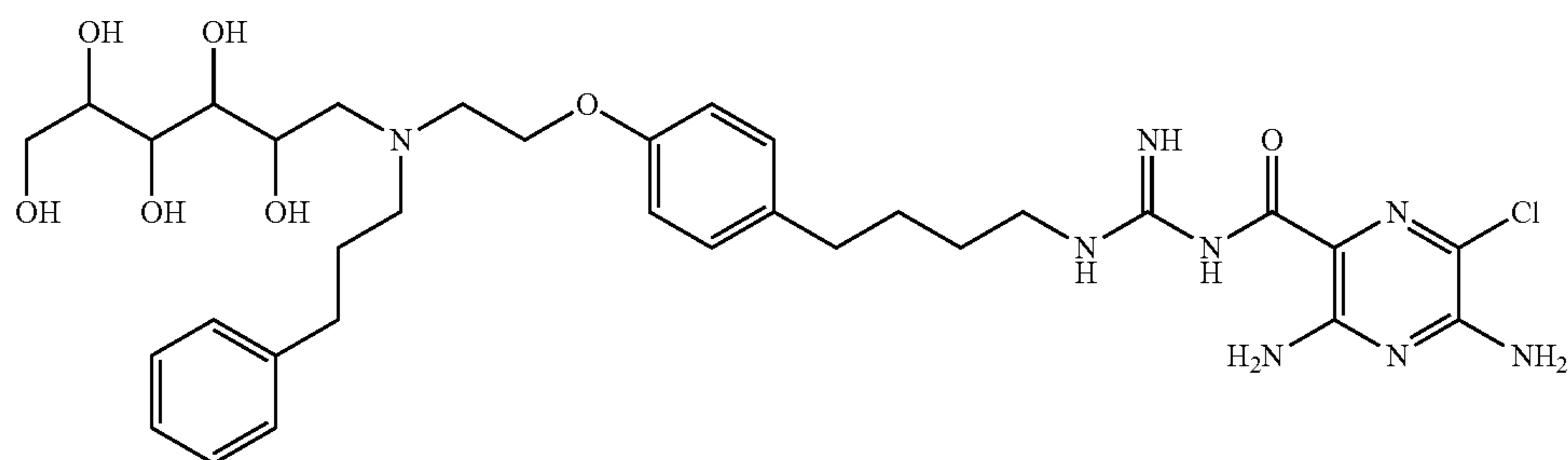
30 3,5-diamino-6-chloro-N-(N-(4-(4-(2-((2,3,4,5,6-pentahydroxyhexyl)(3-phenylpropyl)amino)ethoxy)phenyl)butyl)carbamimidoyl)pyrazine-2-carboxamide;
