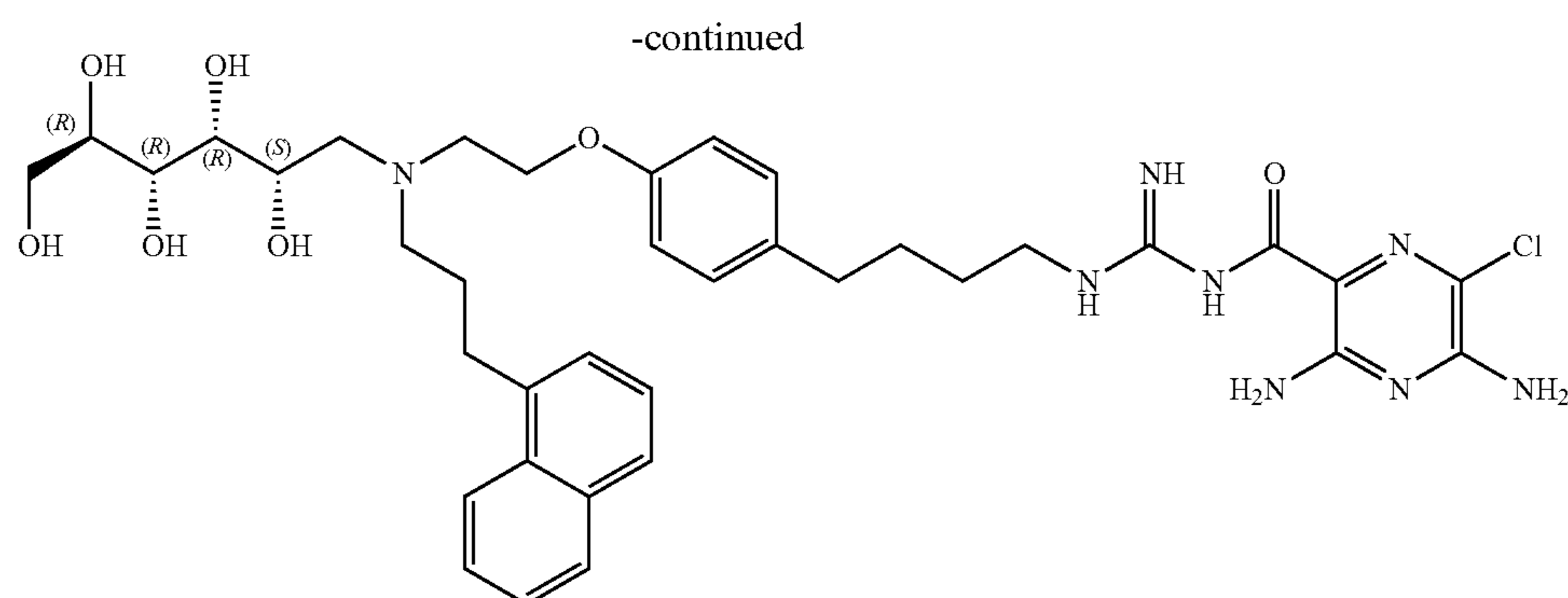
Compound 27
