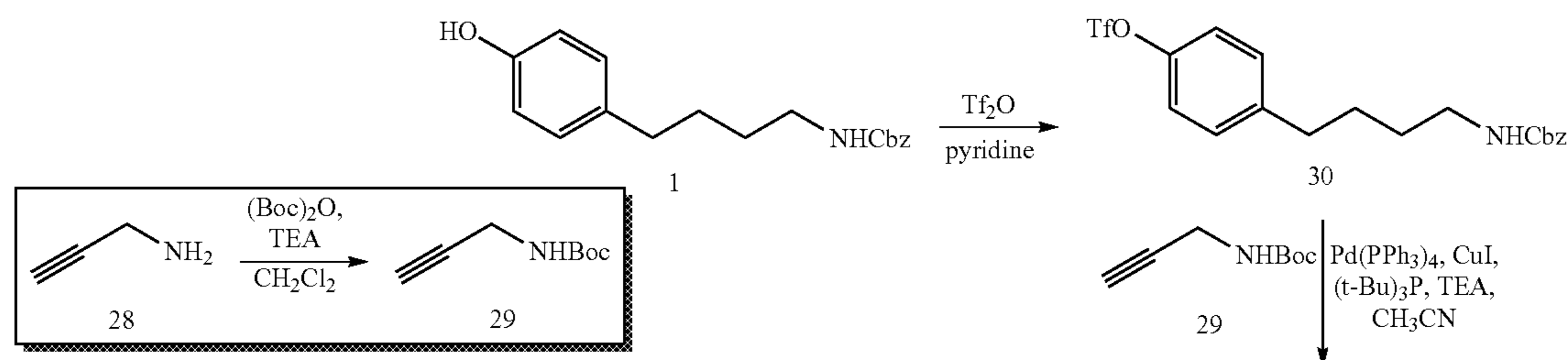
Scheme 5. The Preparation of the Hydrochloride salt of 3,5-diamino-6-chloro-N-(N-(4-(4-(3-(((2S,3R,4R,5R)-2,3,4,5,6-pentahydroxyhexyl)(3-phenylpropyl)amino)propyl)phenyl)butyl)carbamimidoyl)pyrazine-2-carboxamide (Compound 35):
