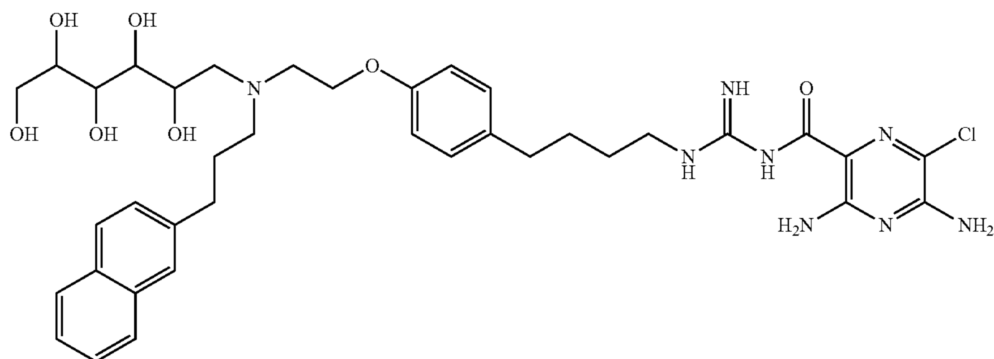
50 3,5-diamino-6-chloro-N-(N-(4-(4-(2-((3-(naphthalen-1-yl)propyl)(2,3,4,5,6-pentahydroxyhexyl)amino)ethoxy)phenyl)butyl)carbamimidoyl)pyrazine-2-carboxamide;
