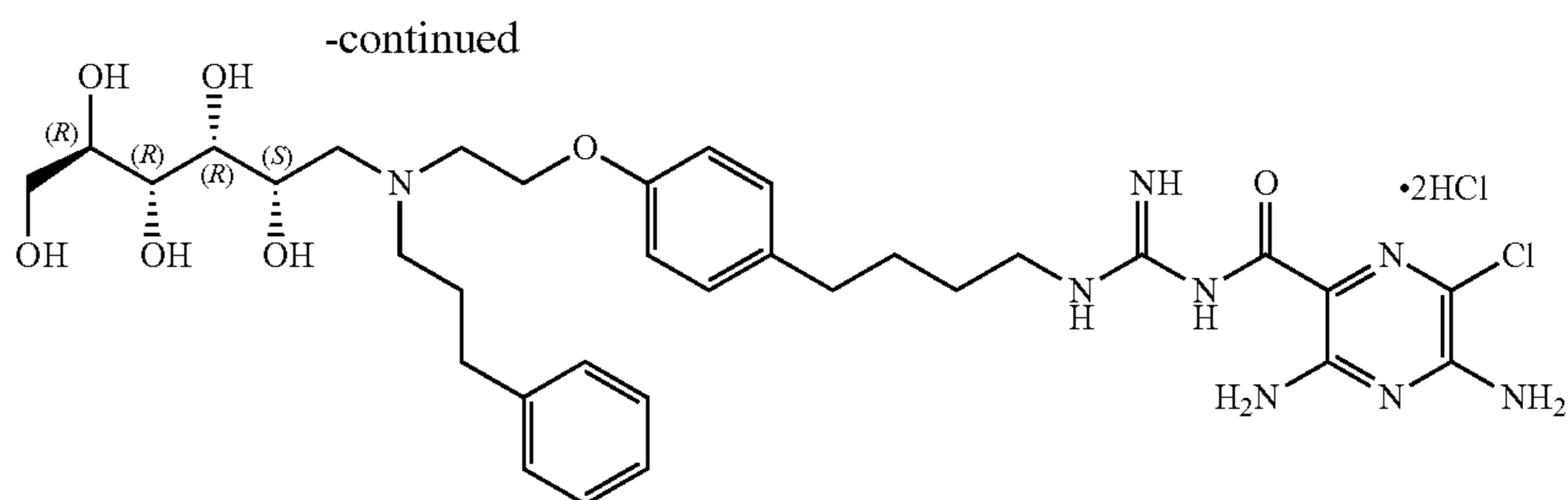
Compound 40
