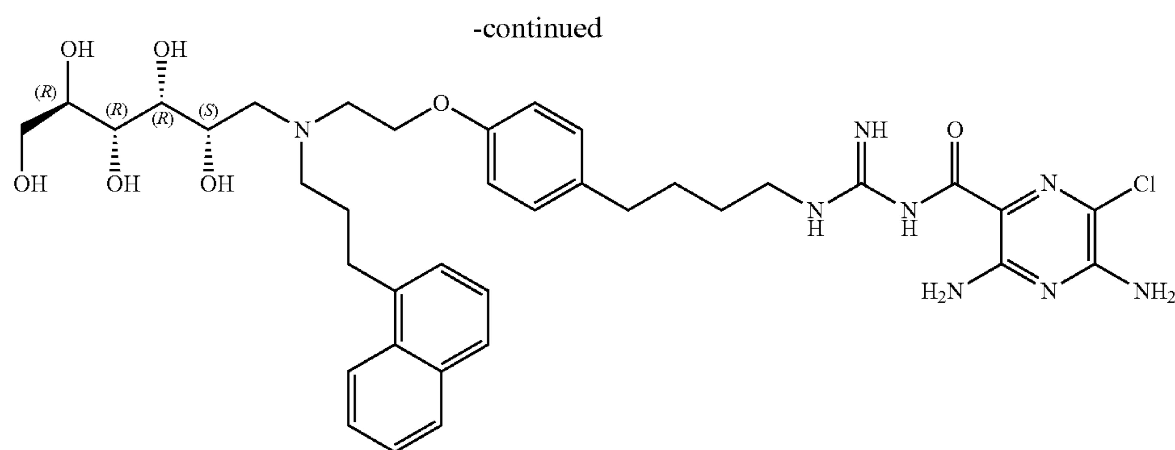
Compound 27
