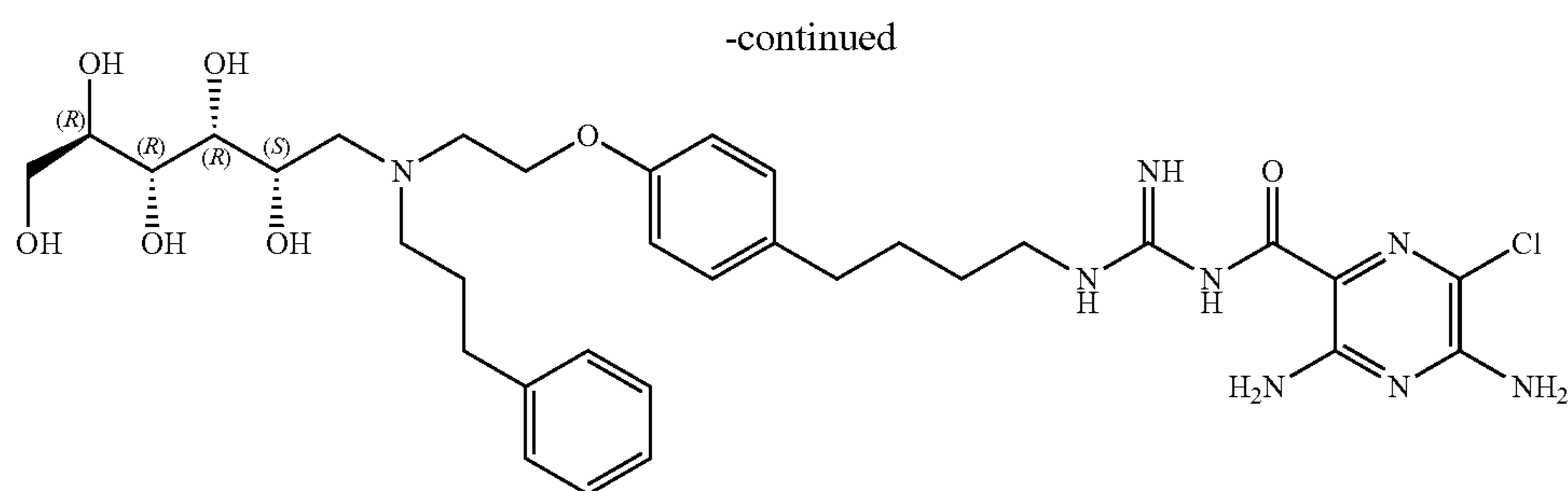
Compound 12
