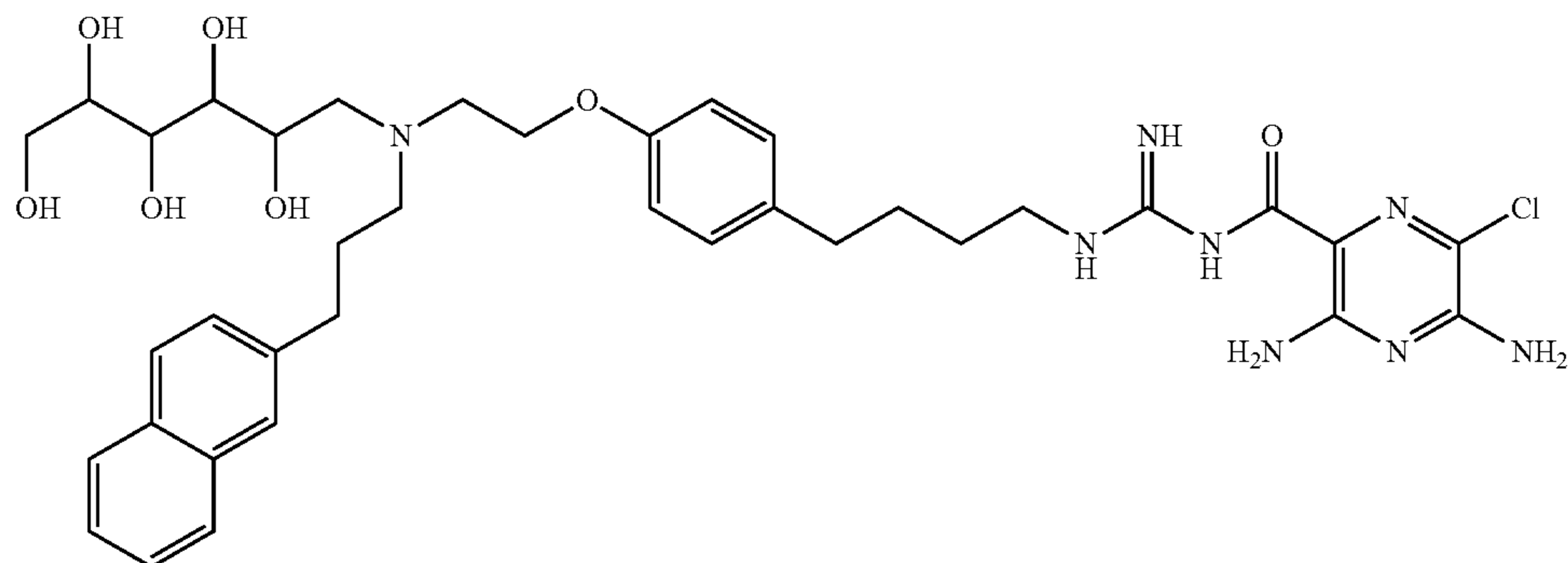
50 3,5-diamino-6-chloro-N-(N-(4-(4-(2-((3-(naphthalen-1-yl)propyl)(2,3,4,5,6-pentahydroxyhexyl)amino)ethoxy)phenyl)butyl)carbamimidoyl)pyrazine-2-carboxamide;
