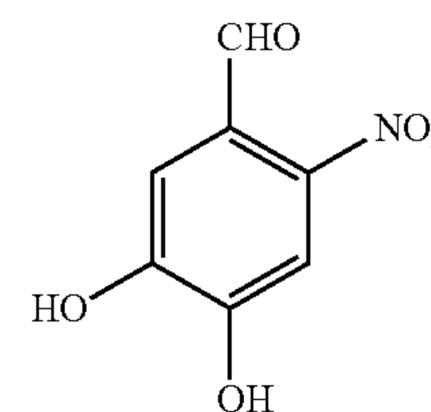
3,4-Dihydroxy-6-nitrobenzaldehyde (DH6NB)
