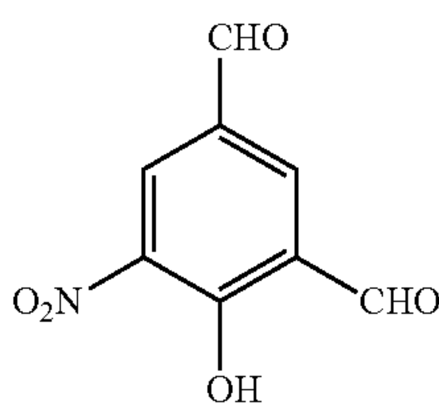
4-Hydroxy-3-Nitro-m- Phthalaldehyde
