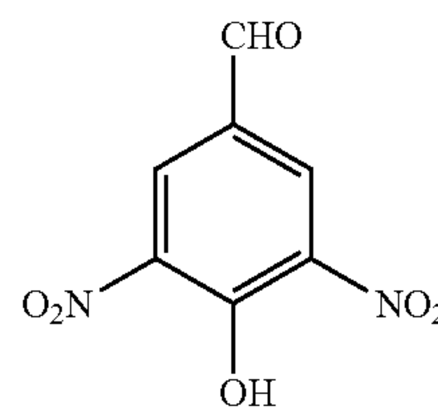
4-Hydroxy-3,5-Dinitrobenzaldehyde (DHNBA)
