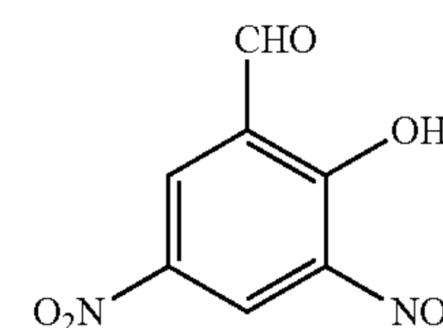
3,5-Dinitrosalicylaldehyde (DNSA)
