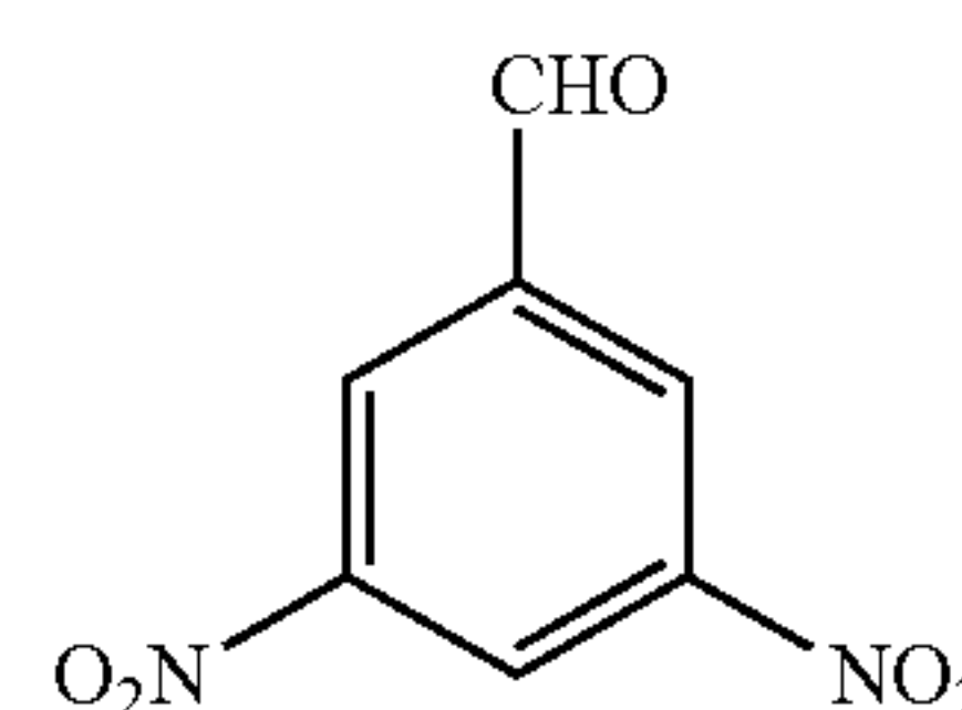
3,5-Dinitrobenzaldehyde
