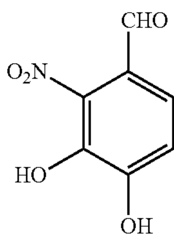
3,4-Dihydroxy-2- nitrobenzaldehyde
