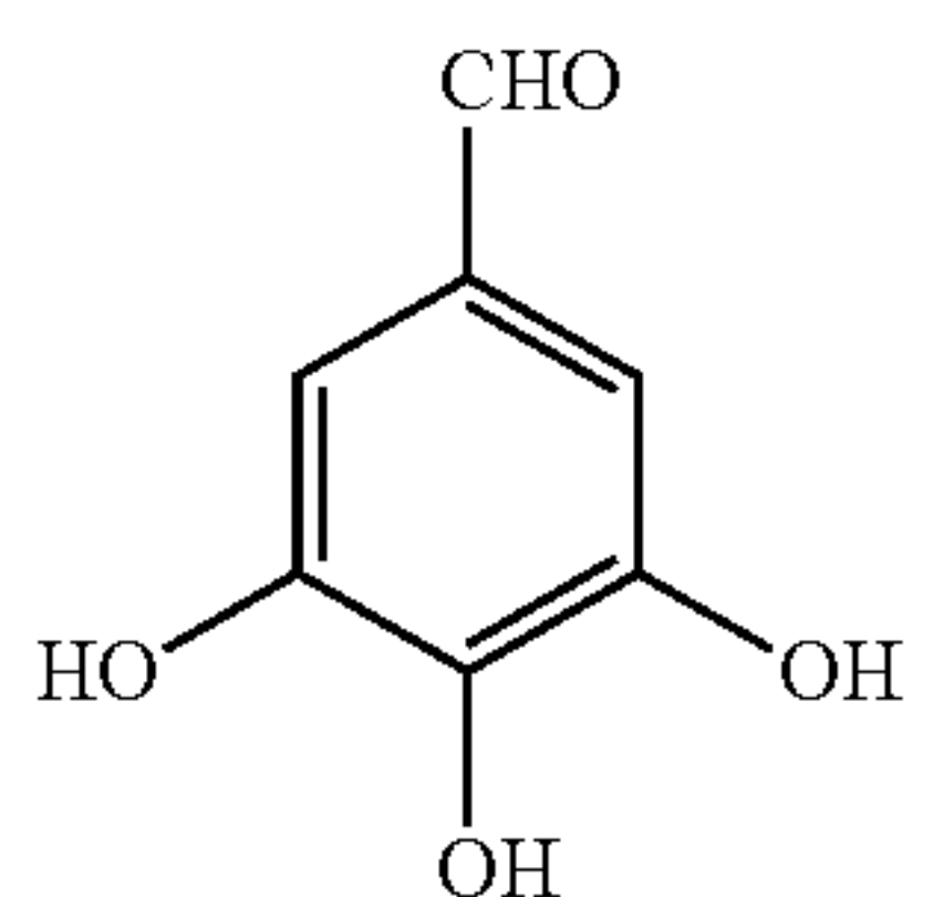
3,4,5-Trihydroxybenzaldehyde (THB-CHO)
