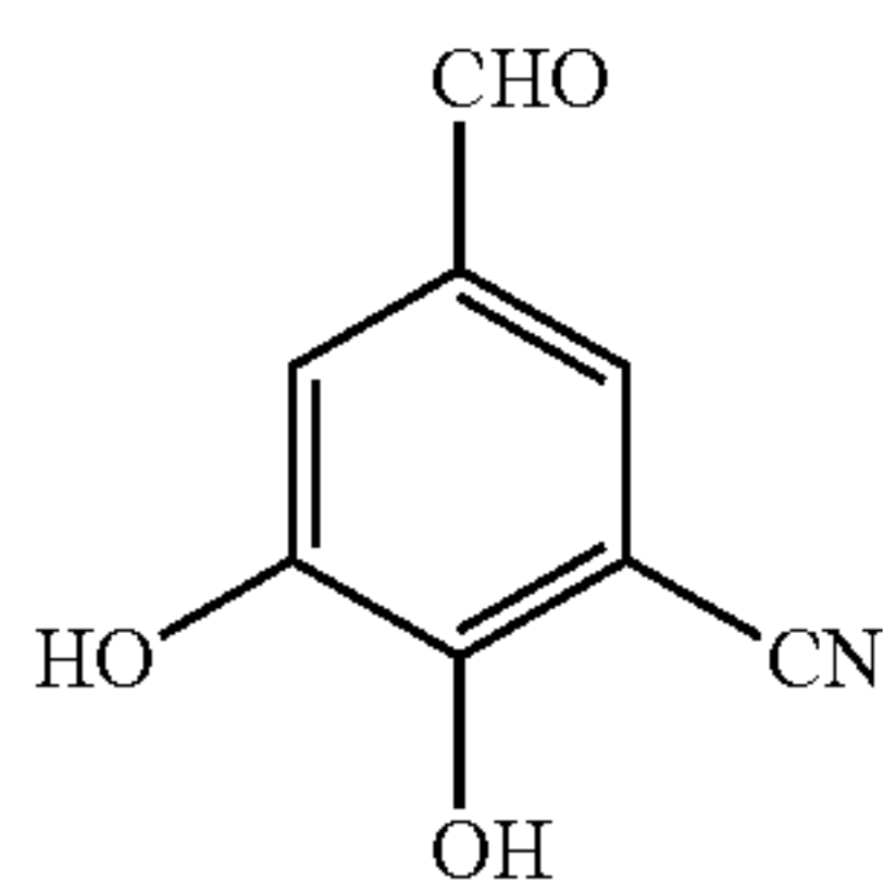
5-Formyl-2,3- dihydroxybenzonitrile
