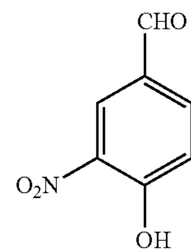
4-Hydroxy-3-Nitrobenzaldehyde (NHBA)
