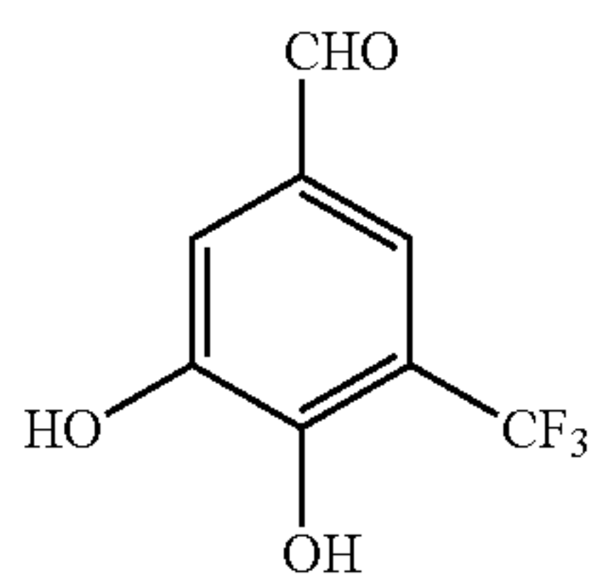
3,4-Dihydroxy-5- (trifluoromethyl)benzaldehyde
