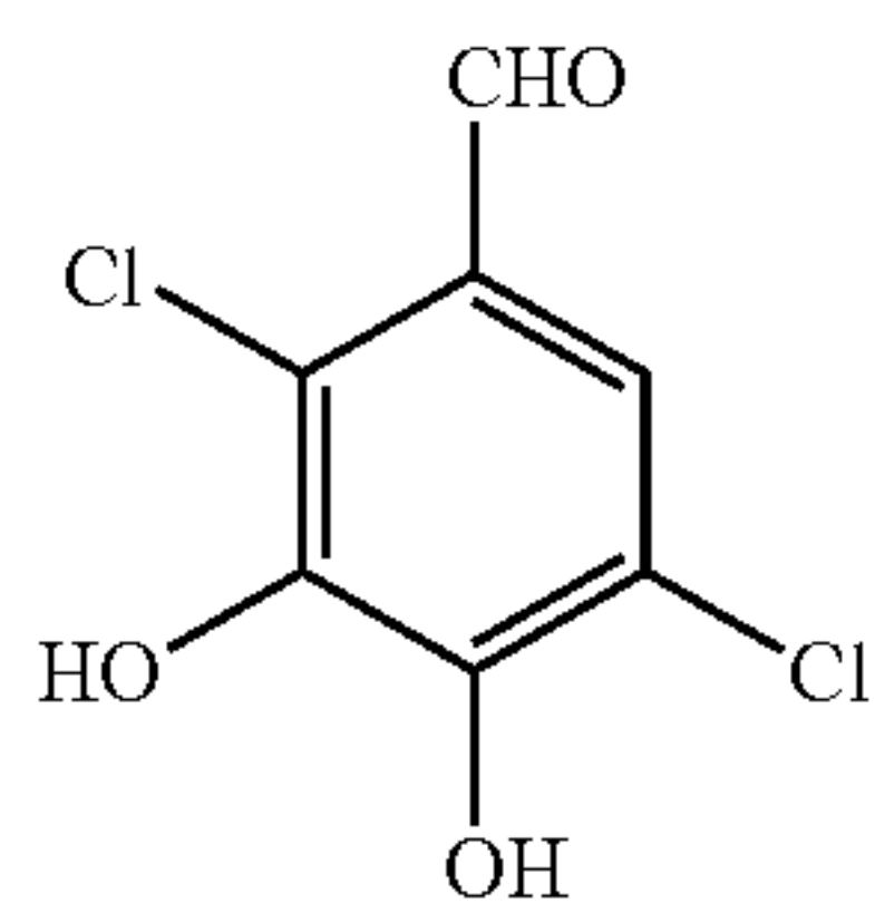
2,5-Dichloro-3,4- dihydroxybenzaldehyde
