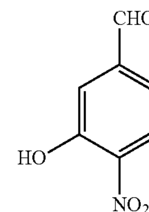
3-Hydroxy-4-Nitrobenzaldehyde (HNBA)
