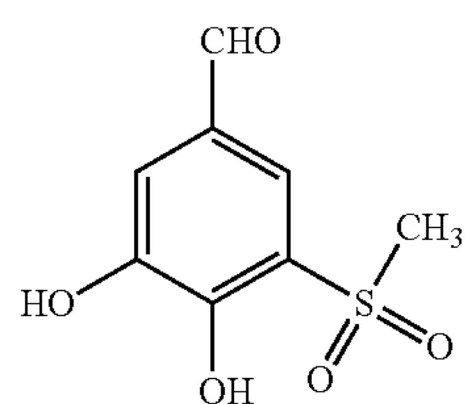
3,4-Dihydroxy-5- (methylsulfonyl)benzaldehyde
