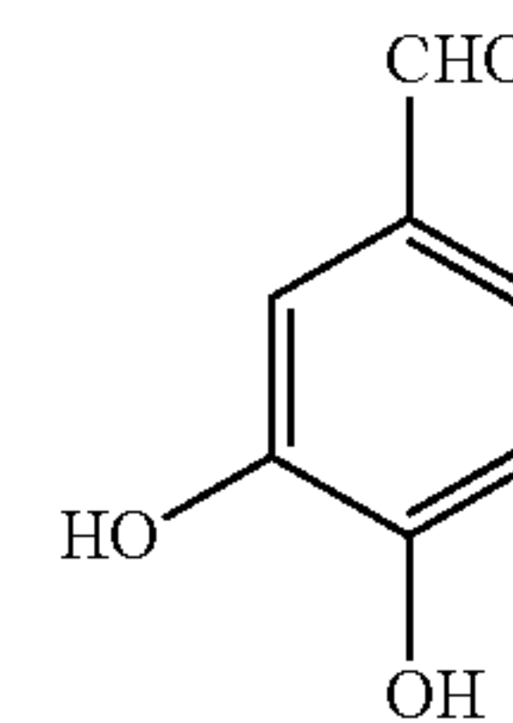
3,4-Dihydroxybenzaldehyde (DHB-CHO)
