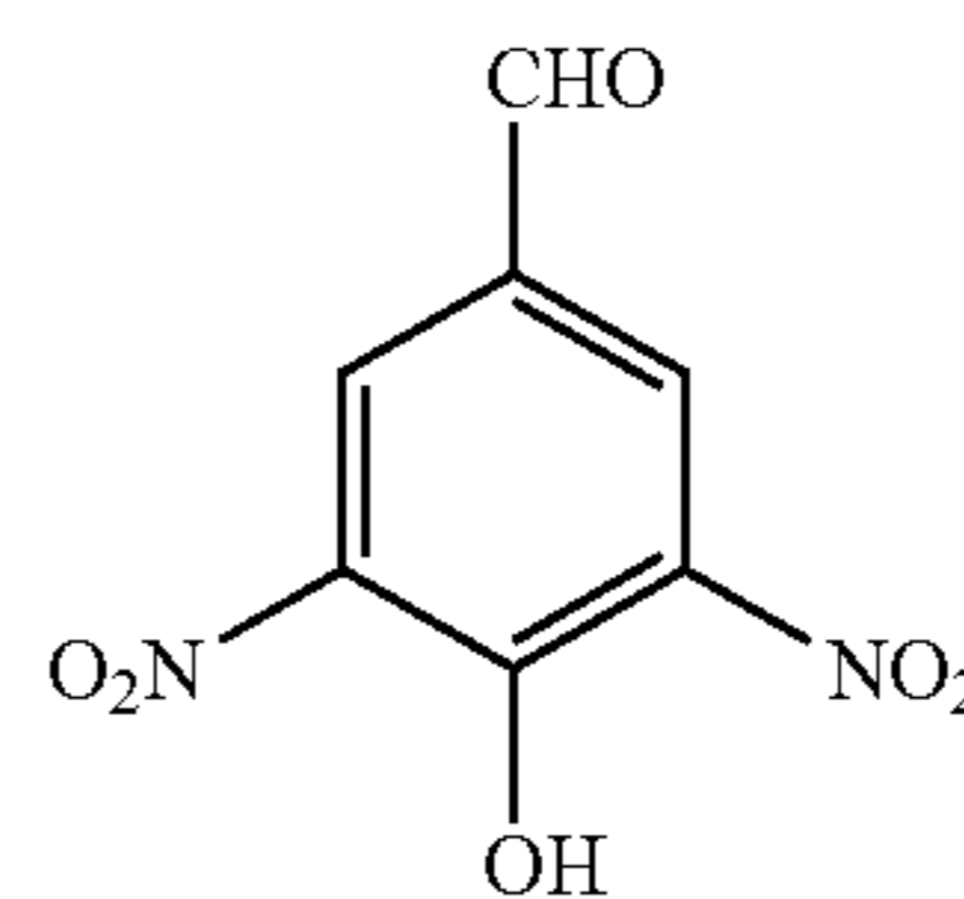
4-Hydroxy-3,5-Dinitrobenzaldehyde (DNHBA)
