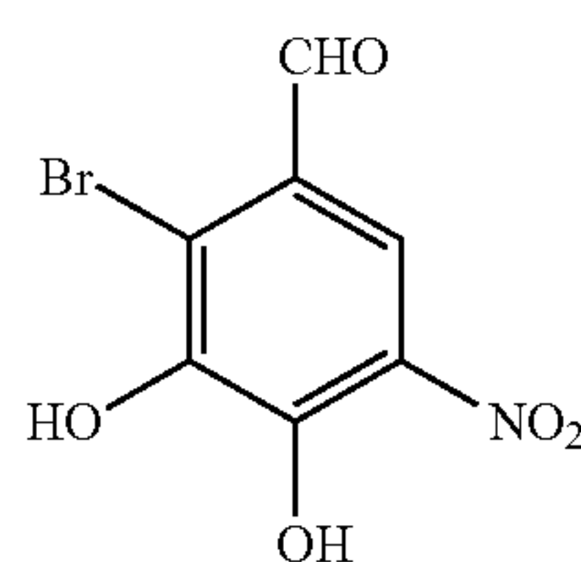
2-Bromo-3,4- dihydroxy-5- nitrobenzaldehyde
