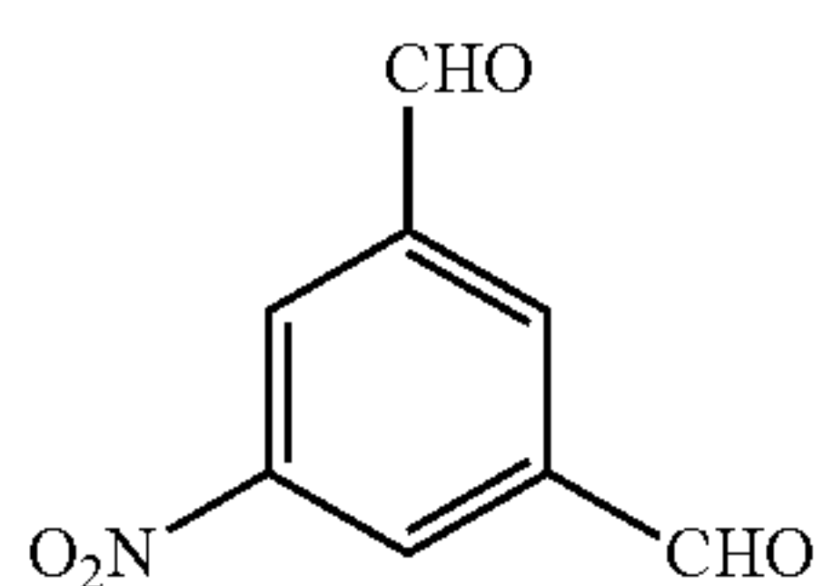
3-Nitro-m- Phthalaldehyde
