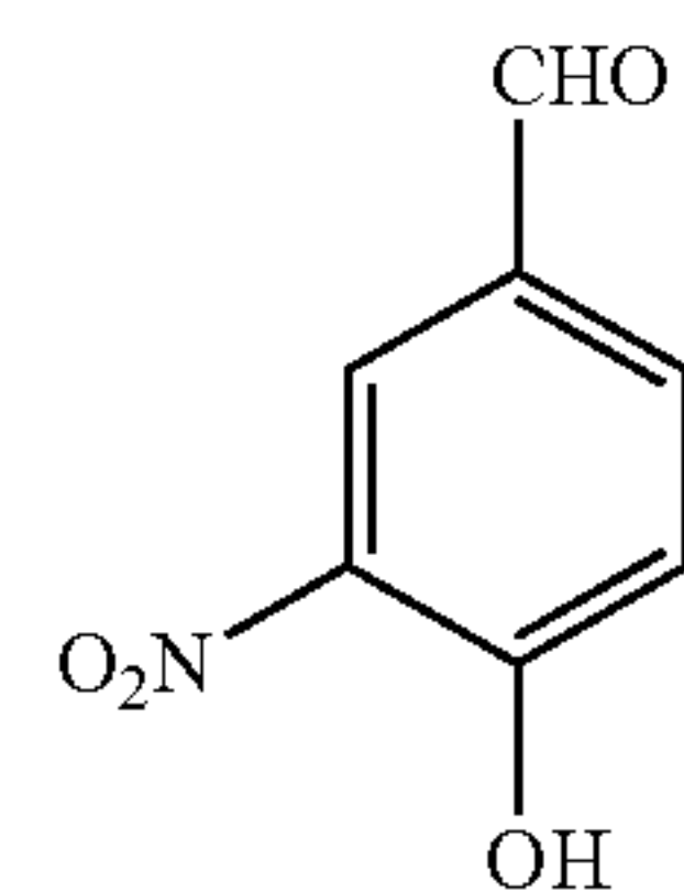
4-Hydroxy-3-Nitrobenzaldehyde (NHBA)
