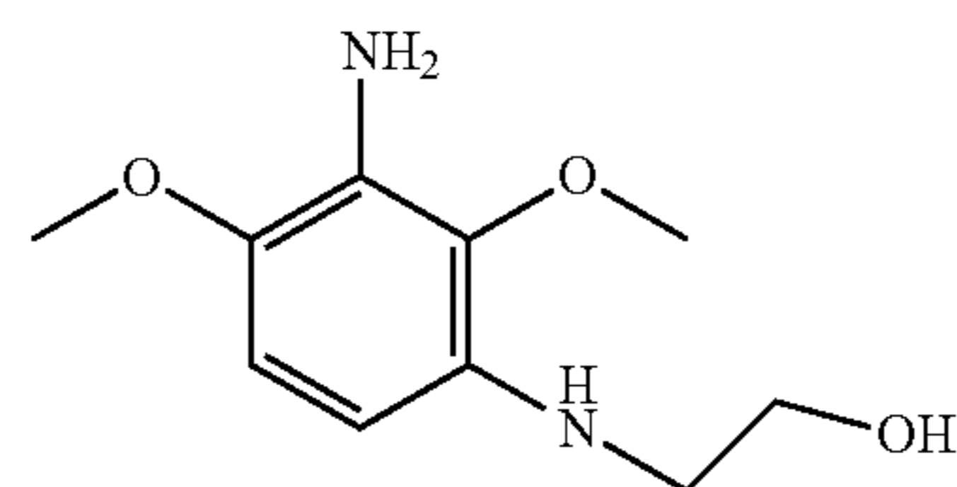
2-(3-amino-2,4-dimethoxyphenylamino)ethanol
