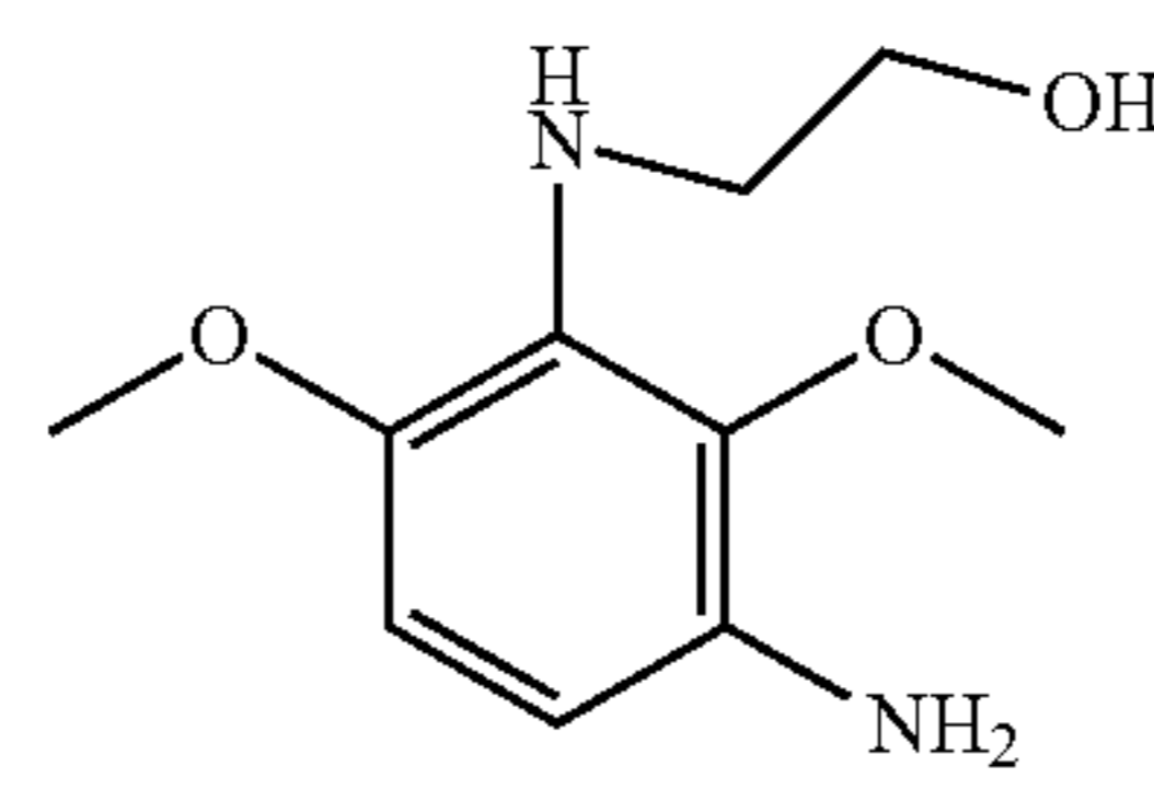
2-(3-amino-2,6-dimethoxyphenylamino)ethanol
