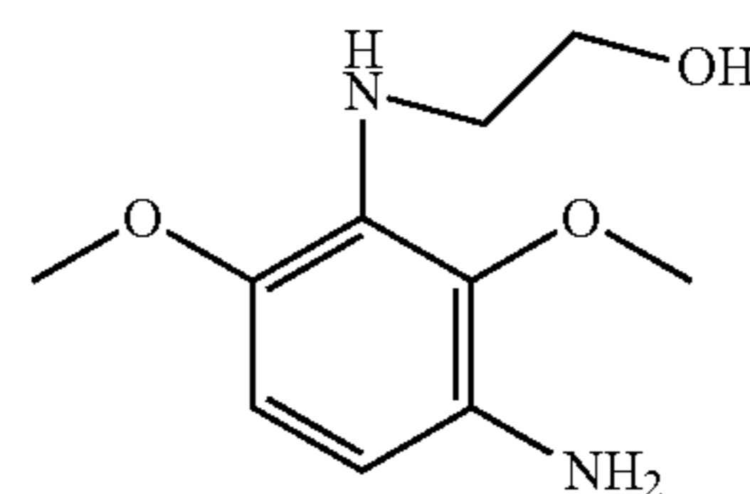
2-(3-amino-2,6-dimethoxyphenylamino)ethanol
