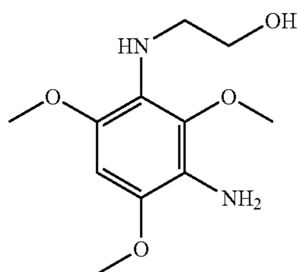
2-(3-amino-2,4,6-trimethoxyphenylamino)ethanol
