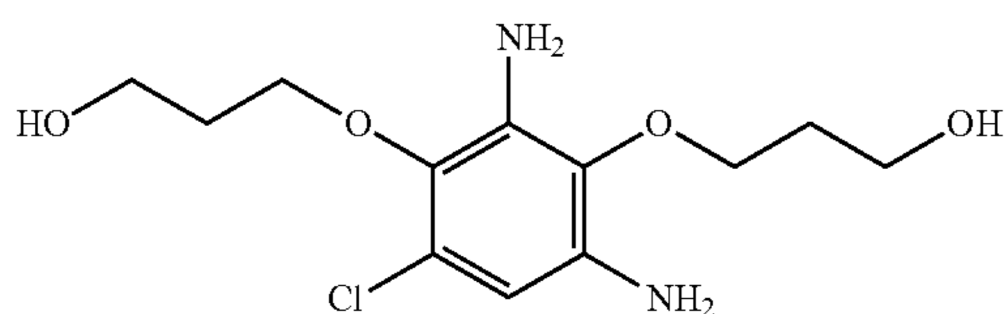
3-[2,6-diamino-4-chloro-3-(3-hydroxypropoxy)phenoxy]propan-1-ol
