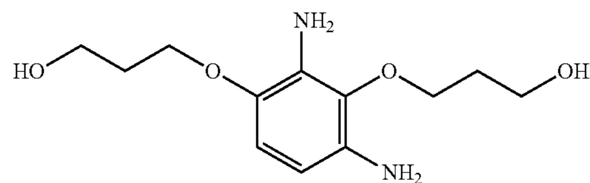
3-[2,6-diamino-3-(3-hydroxypropoxy)phenoxy]propan-1-ol
