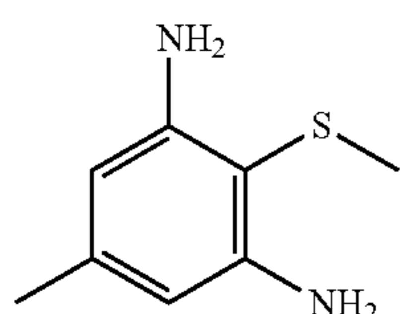
5-methyl-2-methylsulfanylbenzene-1,3-diamine
