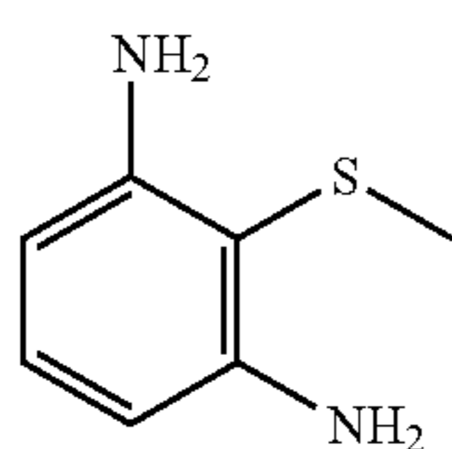
2-methylsulfanylbenzene-1,3-diamine
