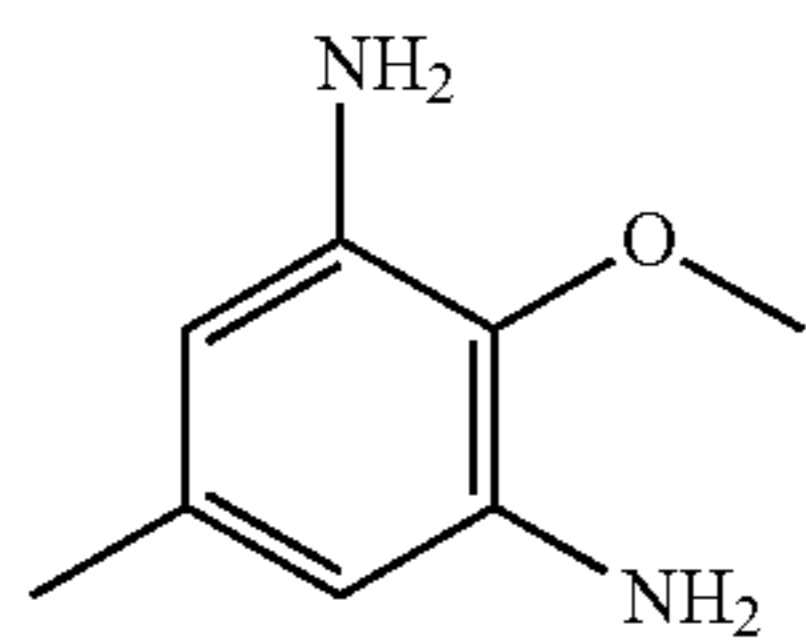
2-methoxy-5-methylbenzene-1,3-diamine
