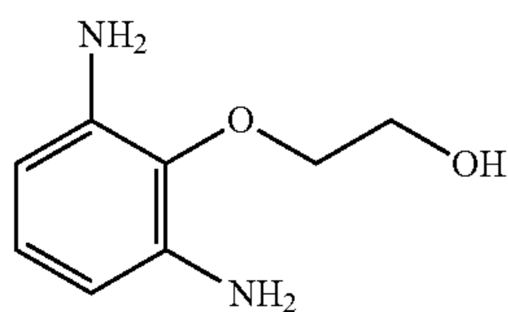
2-(2,6-diaminophenoxy)ethanol
