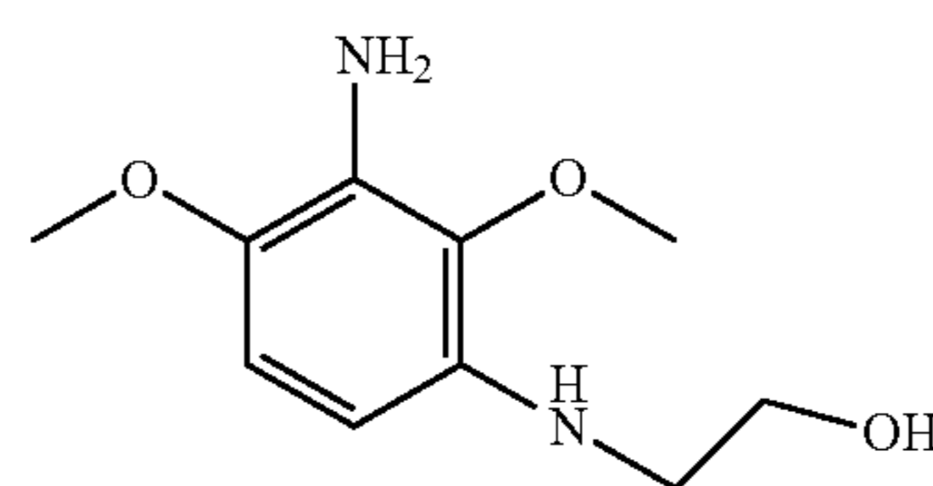
2-(3-amino-2,4-dimethoxyphenylamino)ethanol
