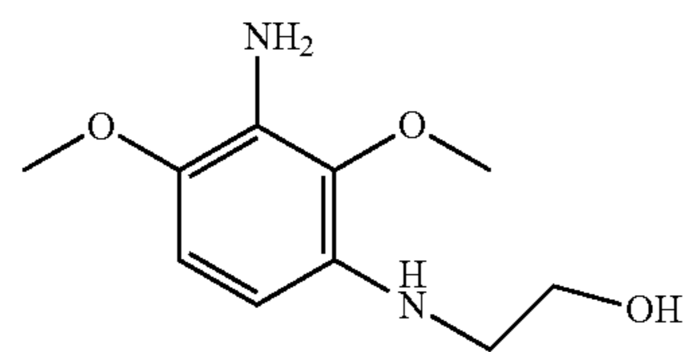
2-(3-amino-2,4-dimethoxyphenylamino)ethanol
