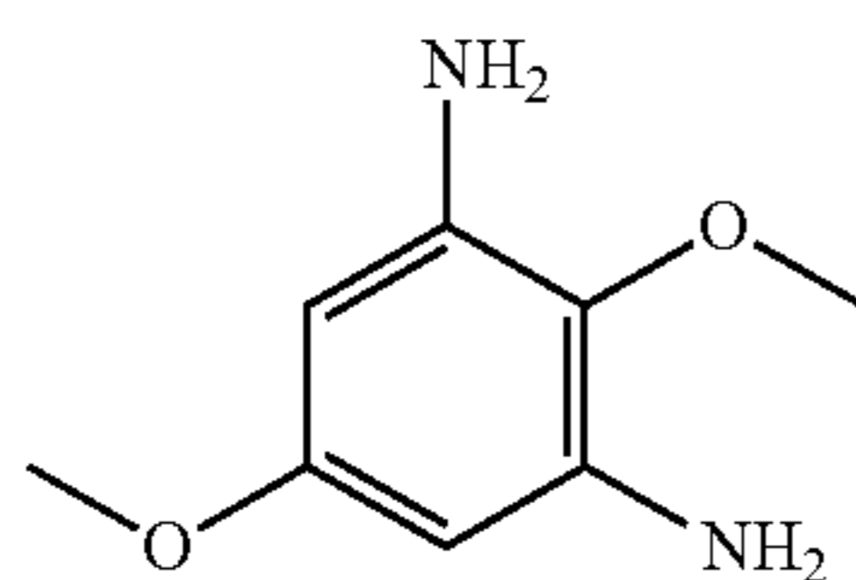
2,5-dimethoxybenzene- 1,3-diamine
