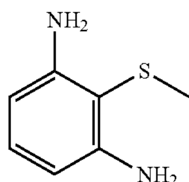
2-methylsulfanylbenzene-1,3-diamine
