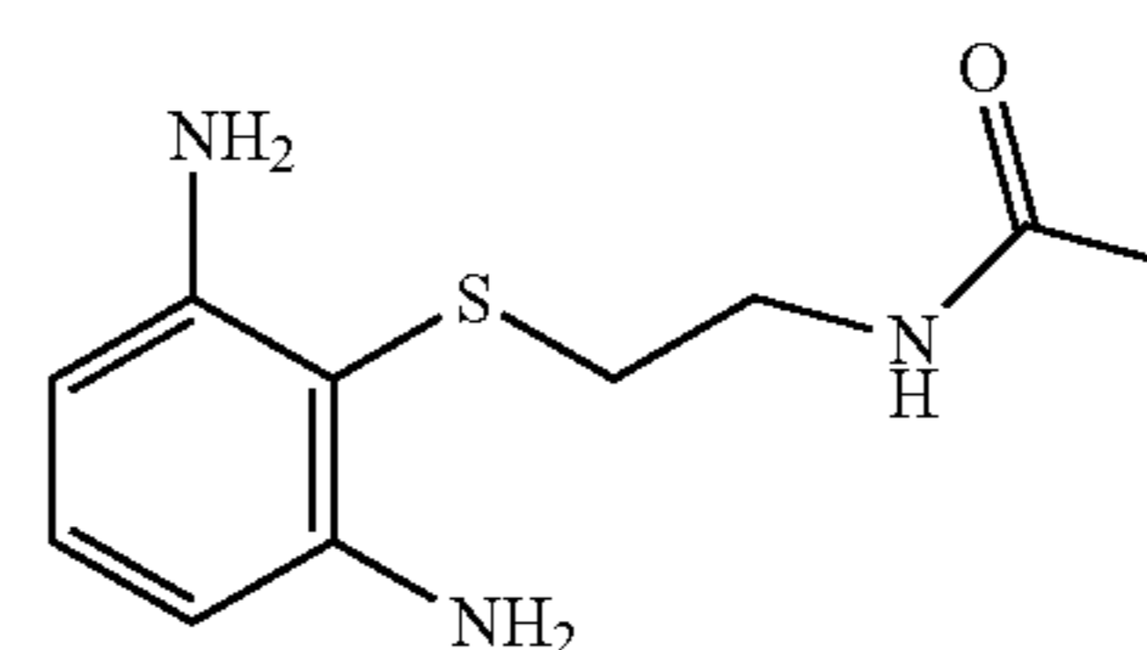
N-[2-(2,6-diaminophenyl)sulfanyl]ethyl acetamide
