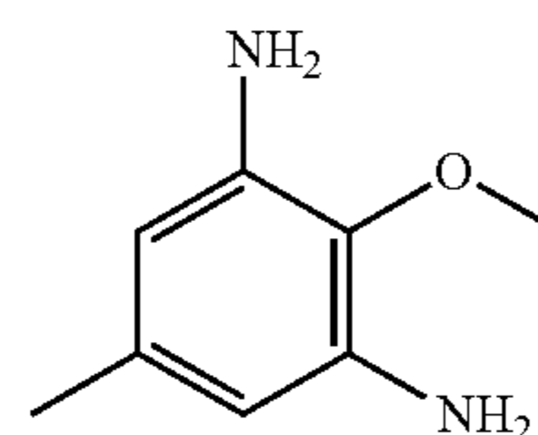
2-methoxy-5-methylbenzene-1,3-diamine
