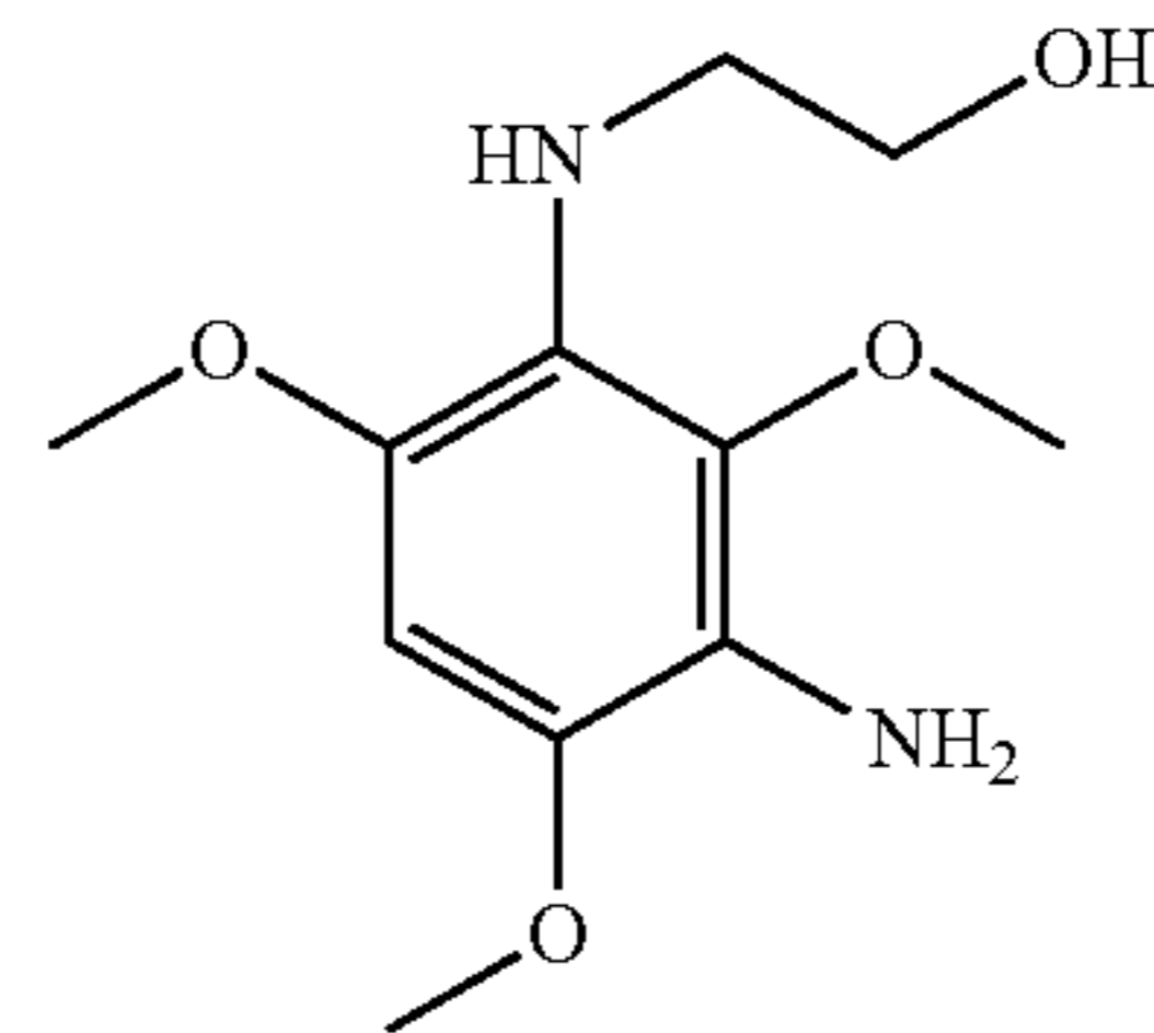
2-(3-amino-2,4,6-trimethoxyphenylamino)ethanol
