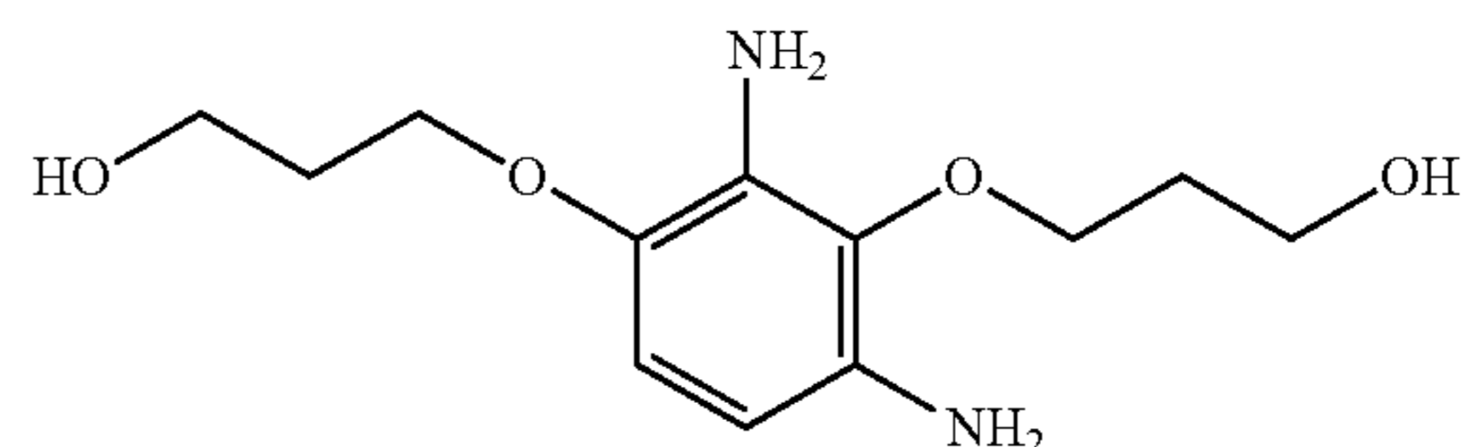
3-[2,6-diamino-3-(3-hydroxypropoxy)phenoxy]propan-1-ol
