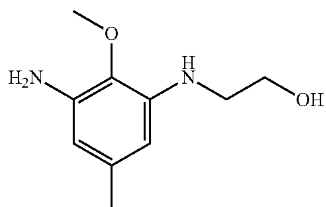
2-(3-amino-2-methoxy-5-methylphenylamino)ethanol
