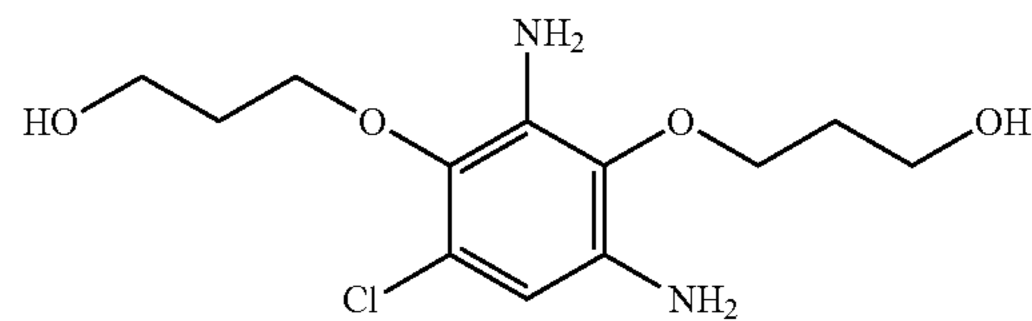
3-[2,6-diamino-4-chloro-3-(3-hydroxypropoxy)phenoxy]propan-1-ol
