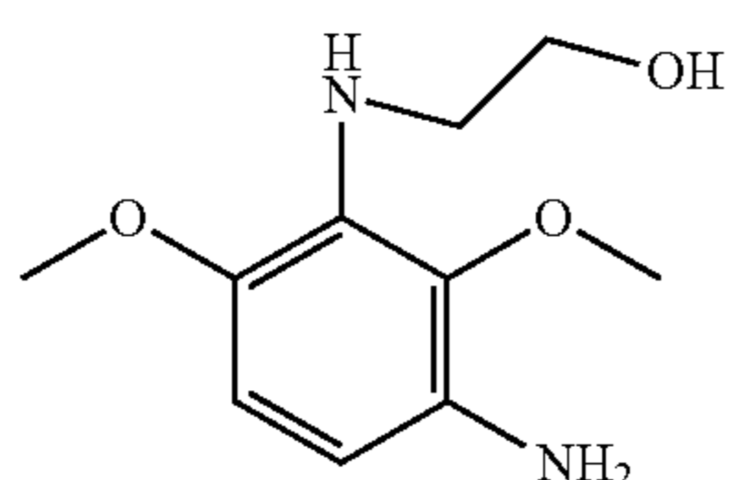
2-(3-amino-2,6-dimethoxyphenylamino)ethanol
