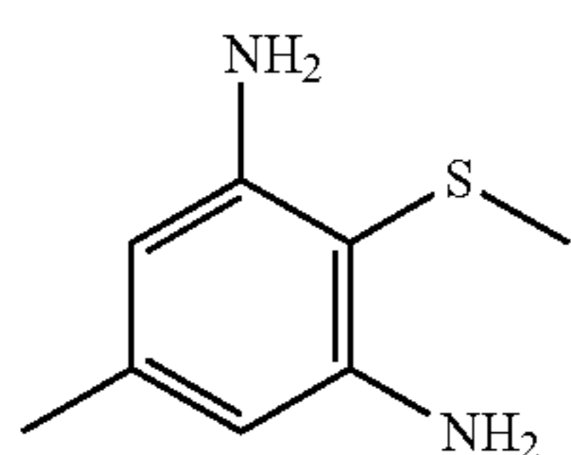
5-methyl-2-methylsulfanylbenzene-1,3-diamine
