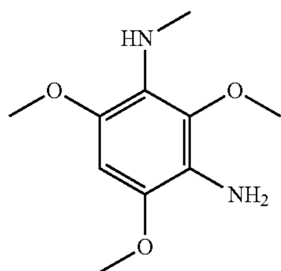
2,4,6-trimethoxy-N-methylbenzene-1,3-diamine
