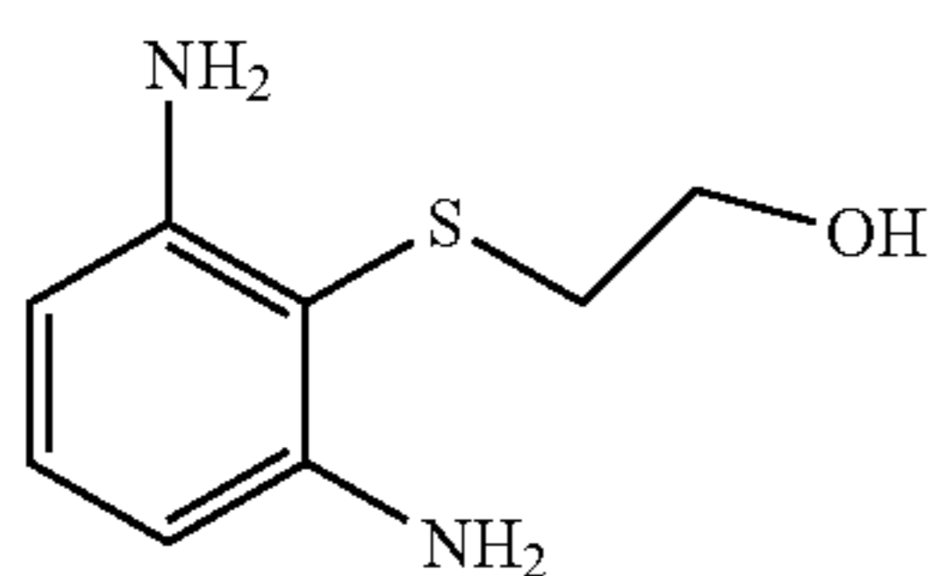
2-(2,6-diaminophenylsulfanyl)ethanol
