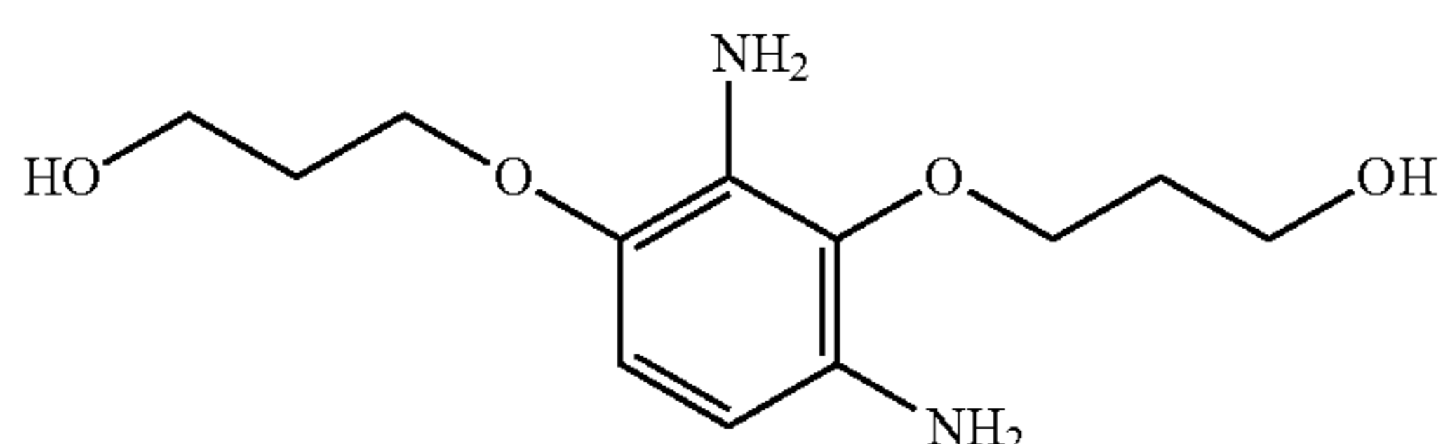
3-[2,6-diamino-3-(3-hydroxypropoxy)phenoxy]propan-1-ol
