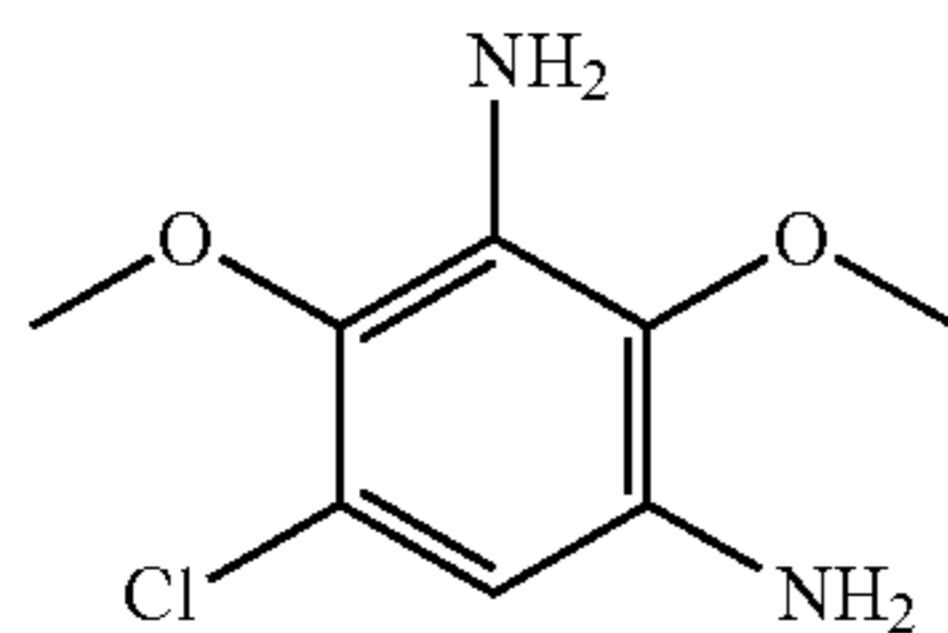
5-chloro-2,4-dimethoxybenzene-1,3-diamine
