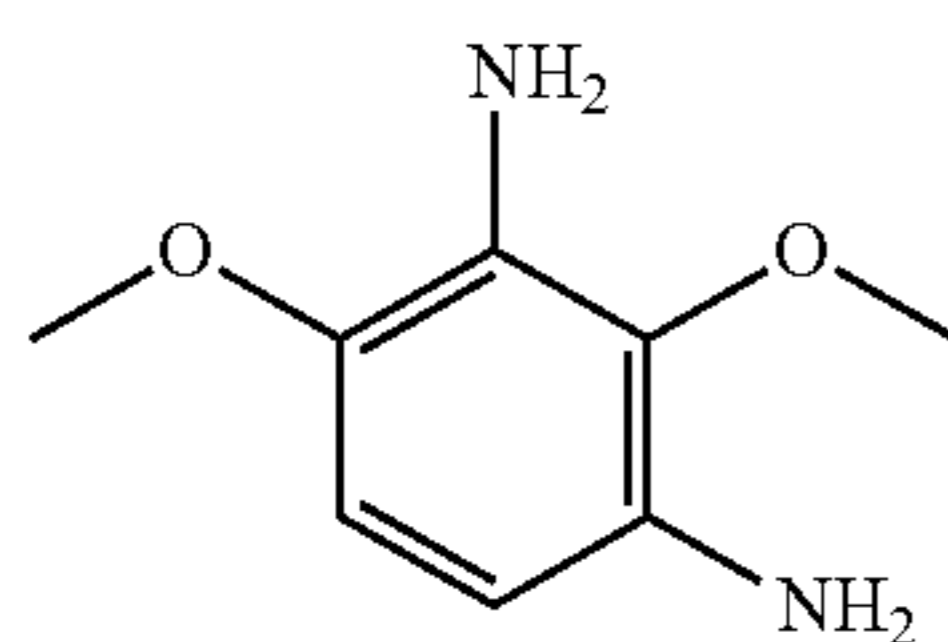
2,4-dimethoxybenzene- 1,3-diamine
