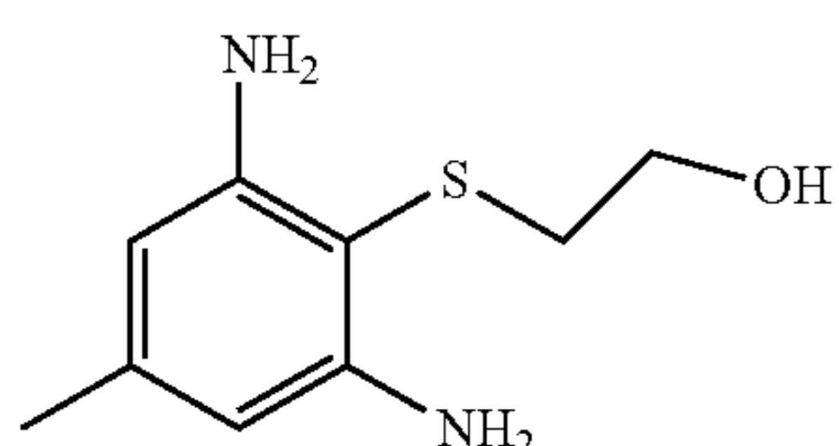
2-(2,6-diamino-4-methylphenylsulfanyl)ethanol
