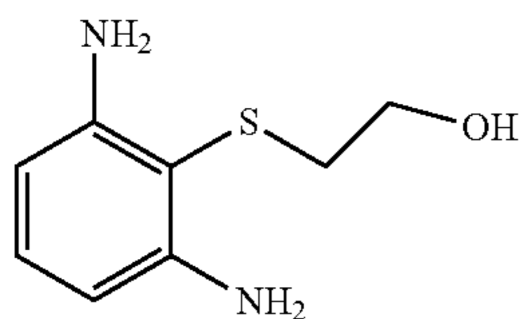
2-(2,6-diaminophenylsulfanyl)ethanol
