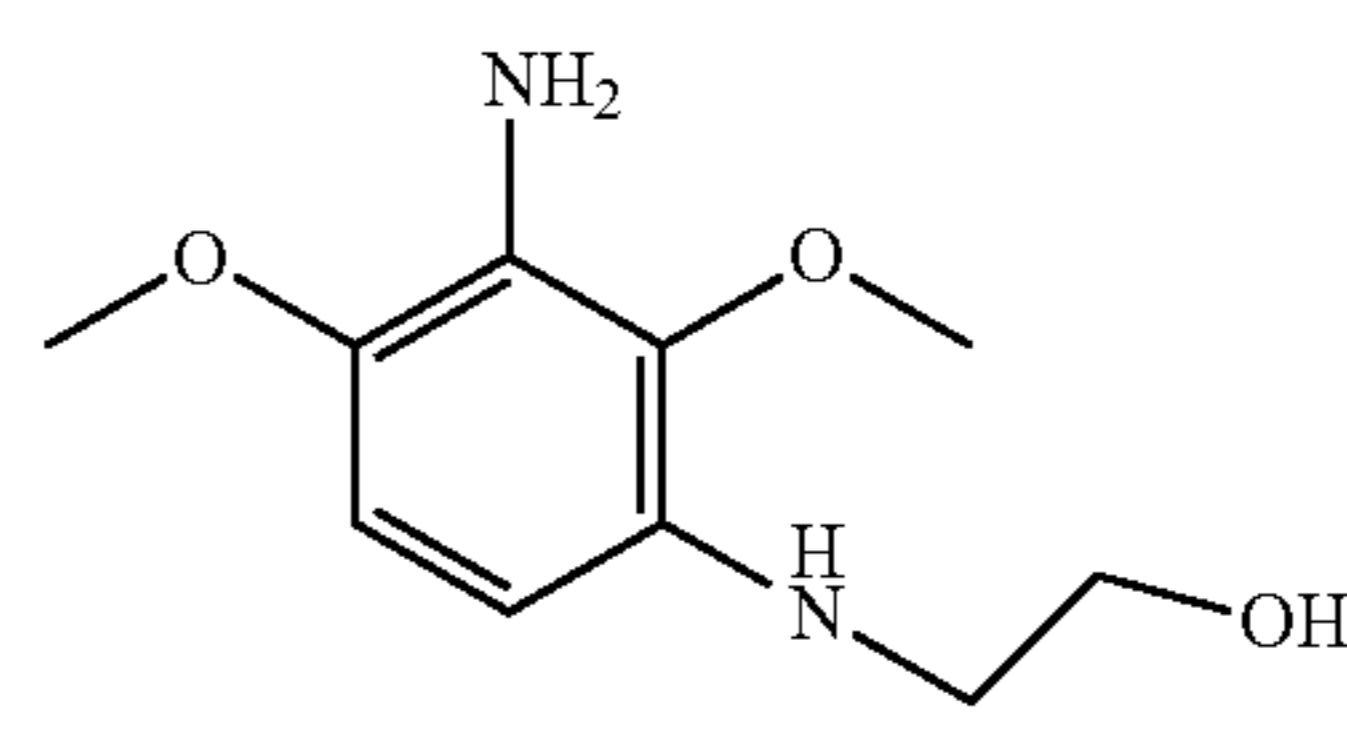
2-(3-amino-2,4-dimethoxyphenylamino)ethanol
