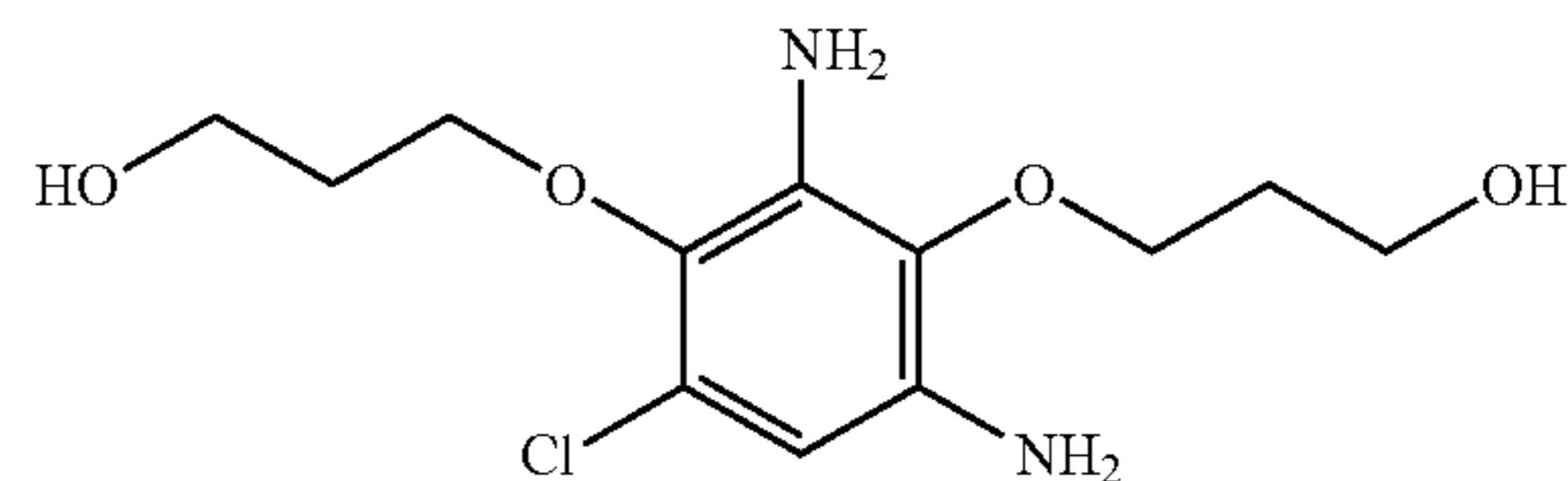
3-[2,6-diamino-4-chloro-3-(3-hydroxypropoxy)phenoxy]propan-1-ol
