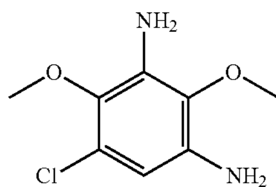
5-chloro-2,4-dimethoxy- benzene-1,3-diamine
