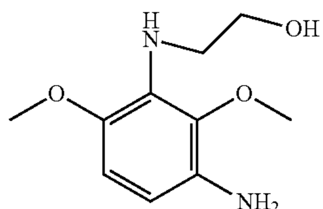
2-(3-amino-2,6-dimethoxyphenylamino)ethanol
