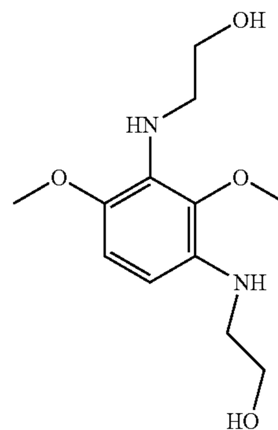
2-[3-(2-hydroxyethylamino)-2,6-dimethoxyphenylamino]ethanol
