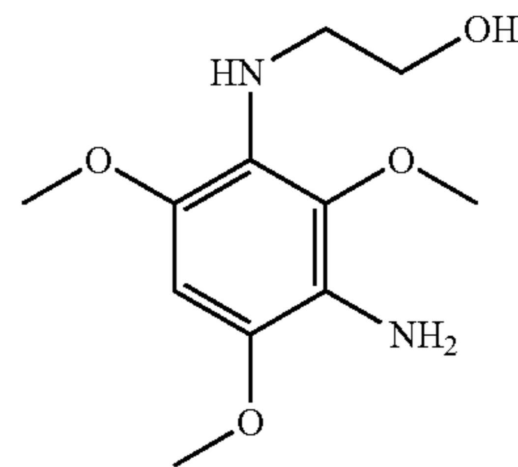
2-(3-amino-2,4,6-trimethoxyphenylamino)ethanol
