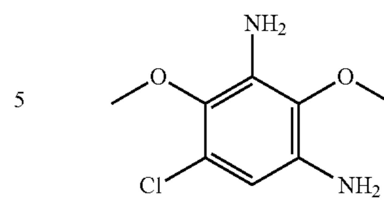
5-chloro-2,4-dimethoxy- benzene-1,3-diamine
