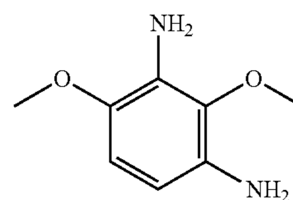
2,4-dimethoxybenzene-1,3-diamine
