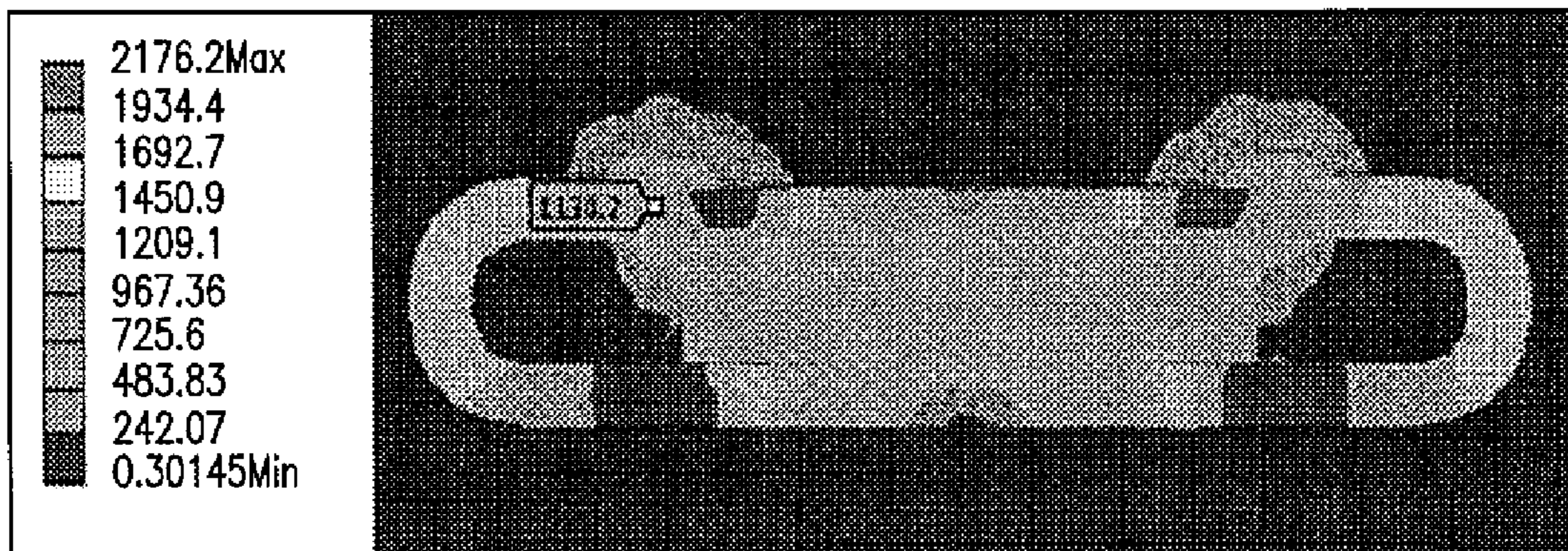
FIG. 9 PRIOR ART
