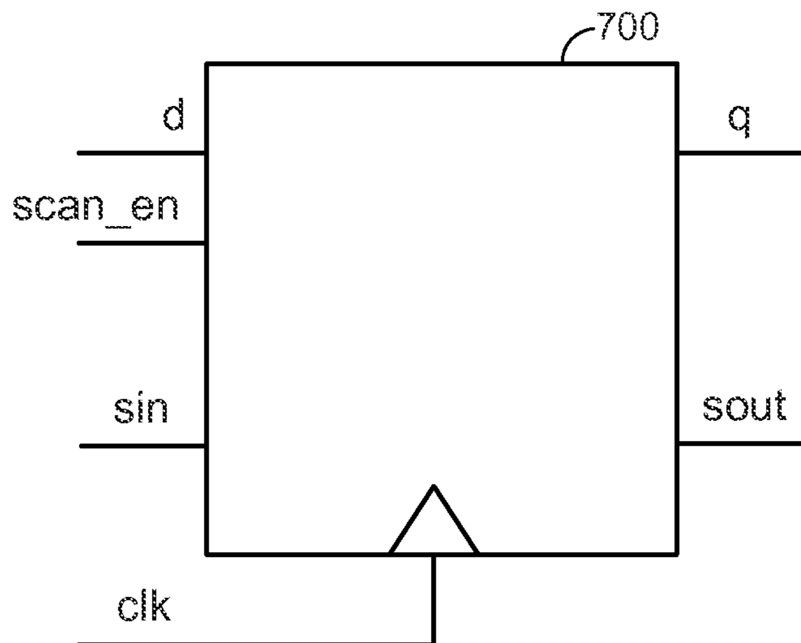
A regular SFF (without async. set/reset)
