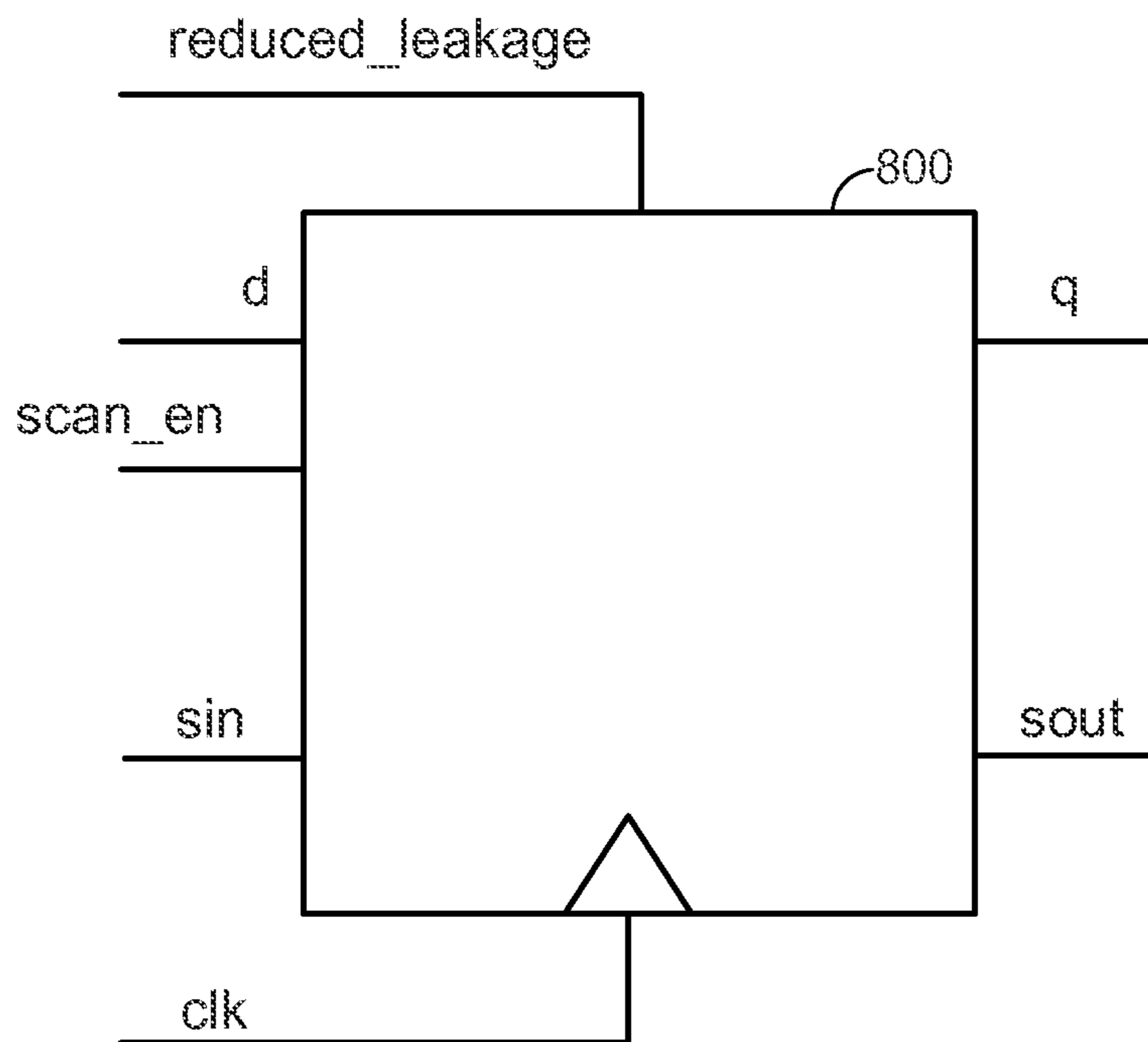
An equivalent 0/1-Gated SFF
