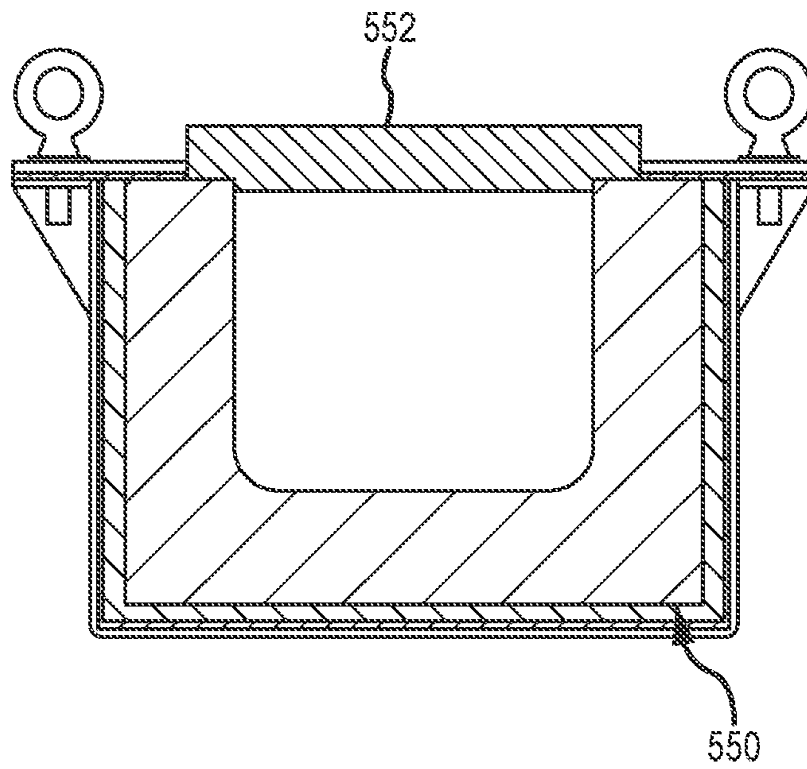
SECTION B-B
