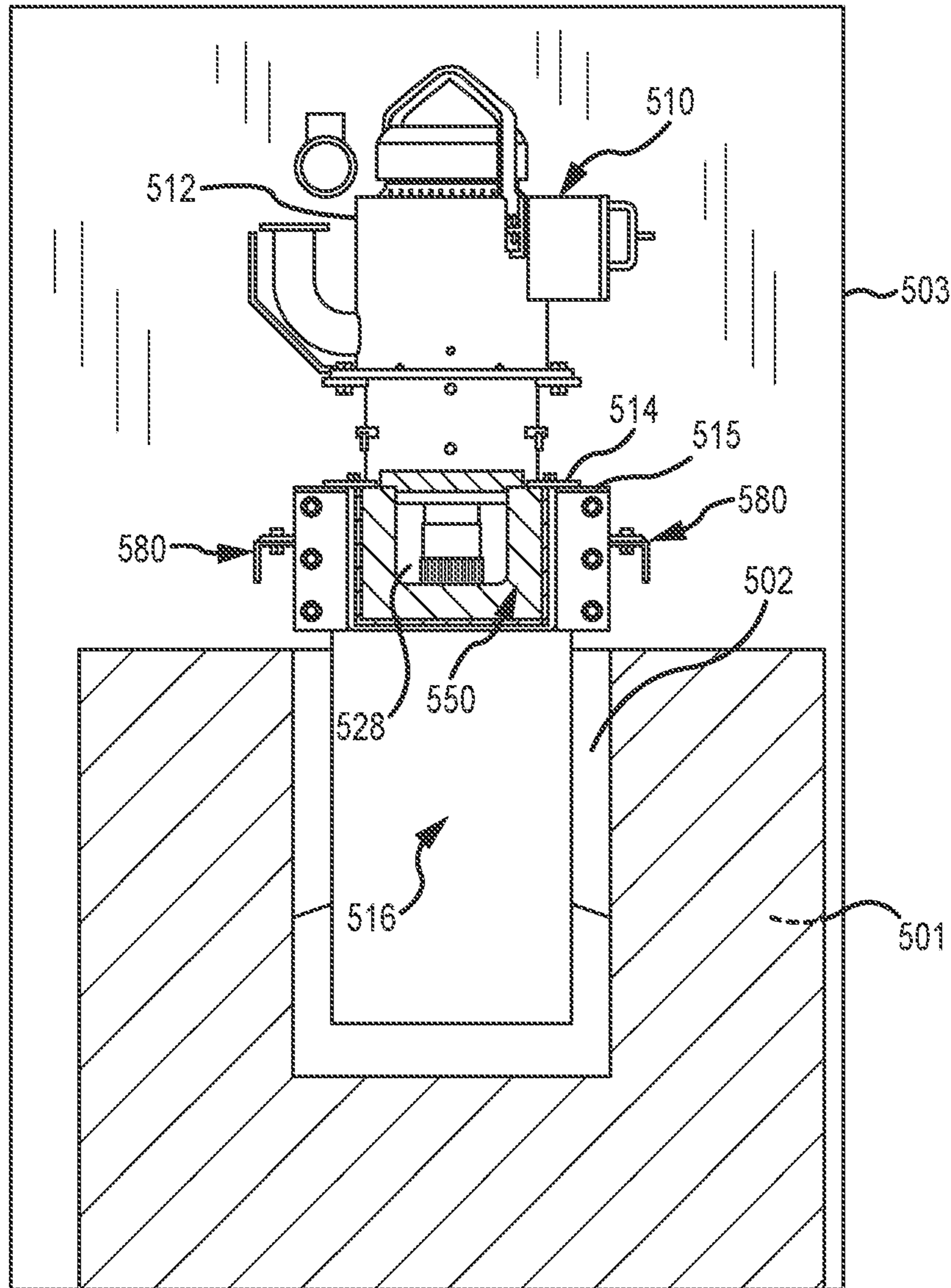
SECTION C-C
