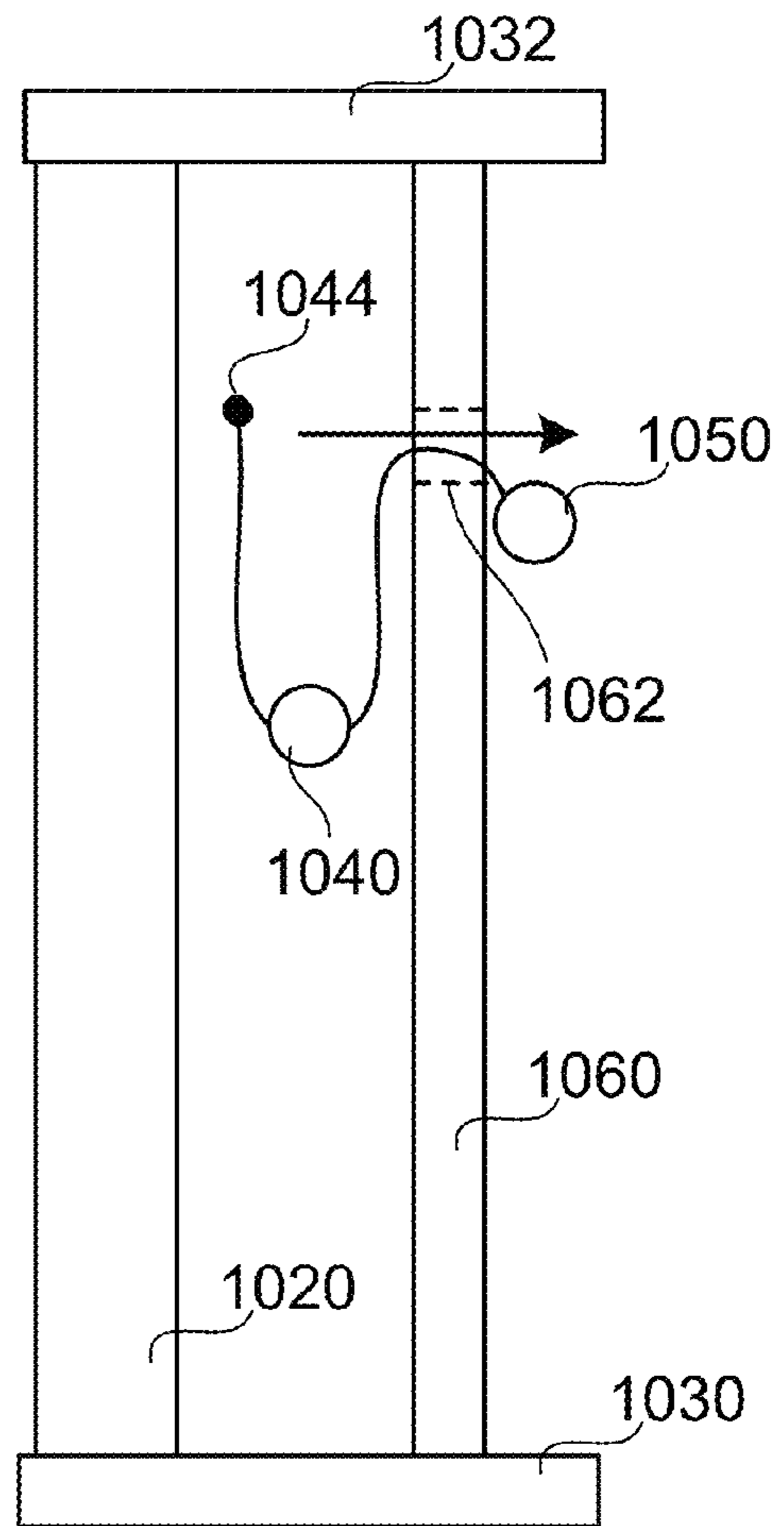
Fig. 14B Venting
