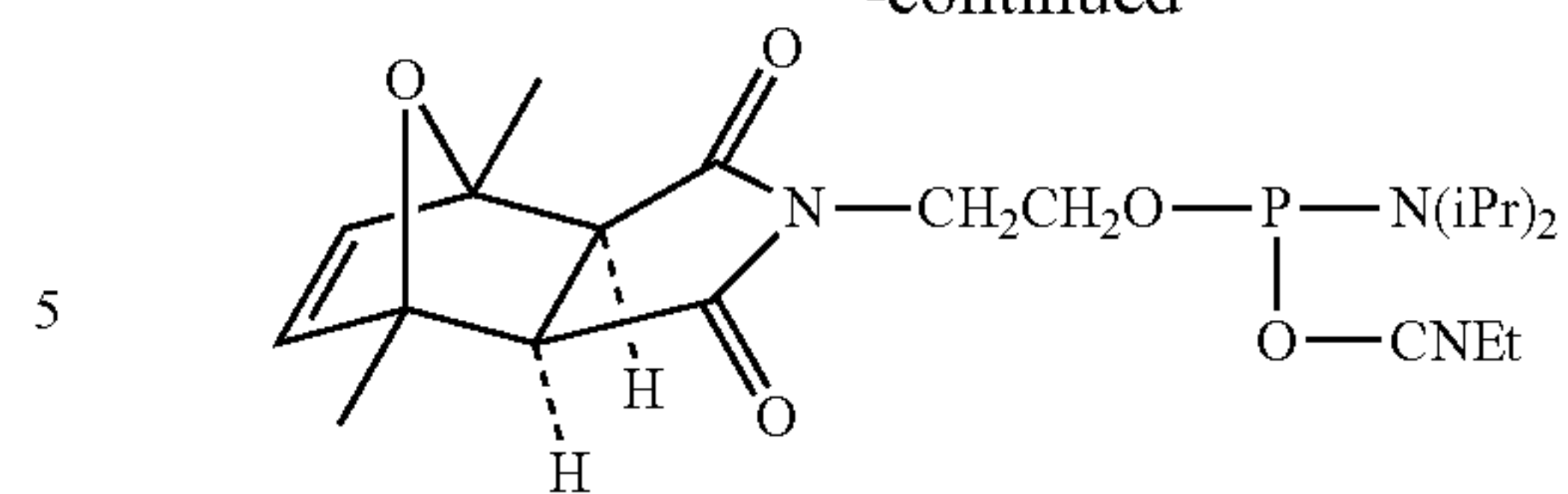
5'-Maleimide-Modifier Phosphoramidite
