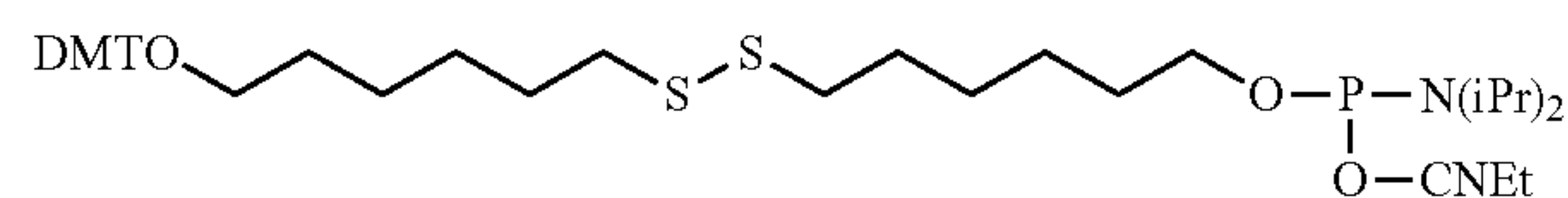
Thiol-Modifier C6 S—S
