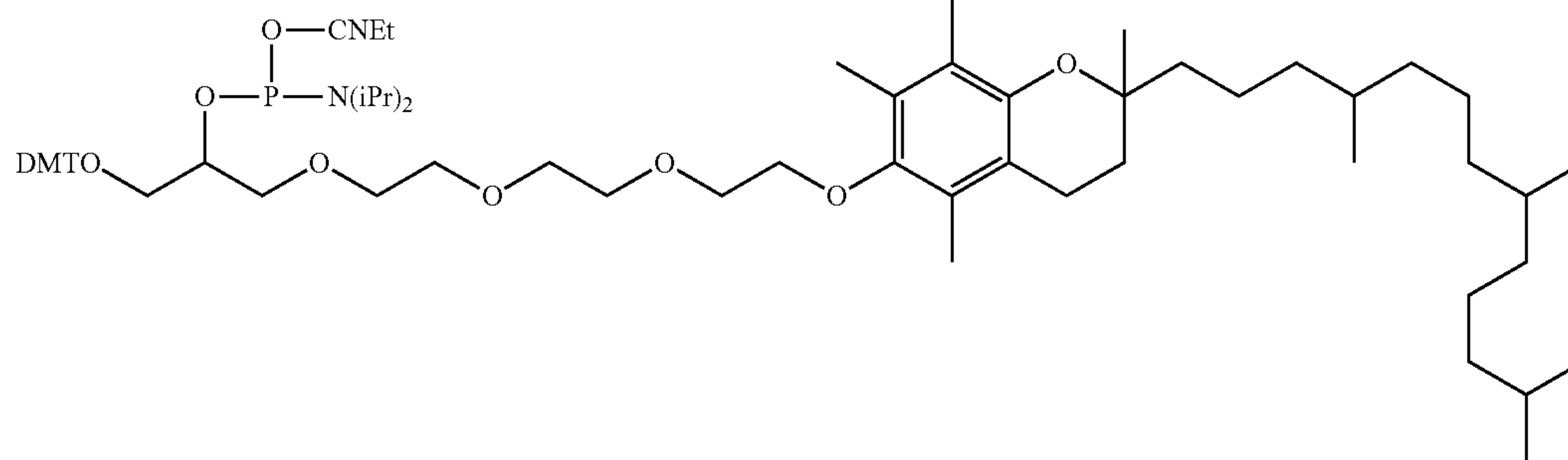
\alpha -Tocopherol-TEG Phosphoramidite
