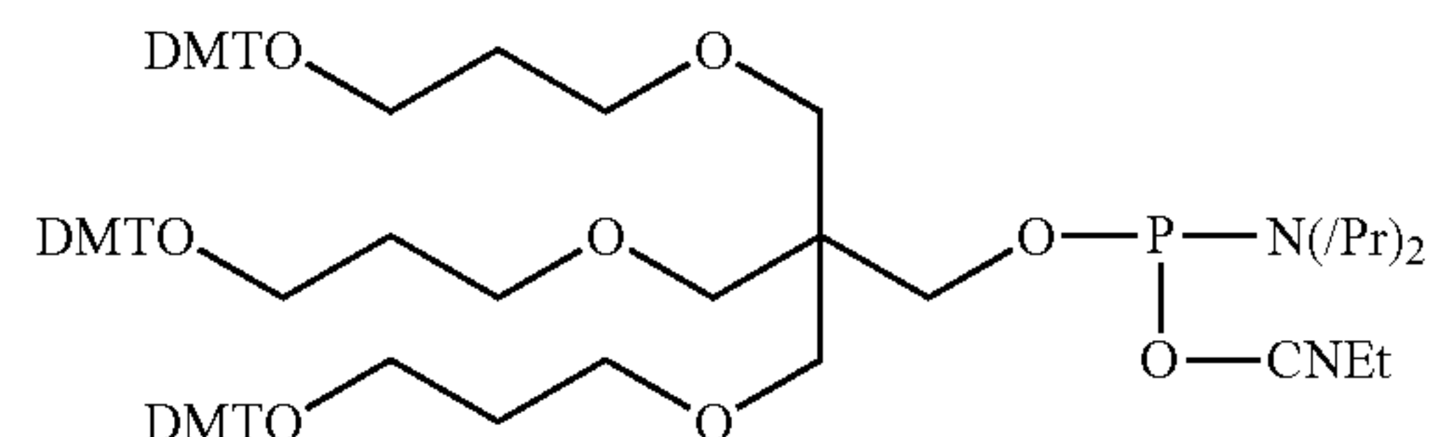
Formula X
