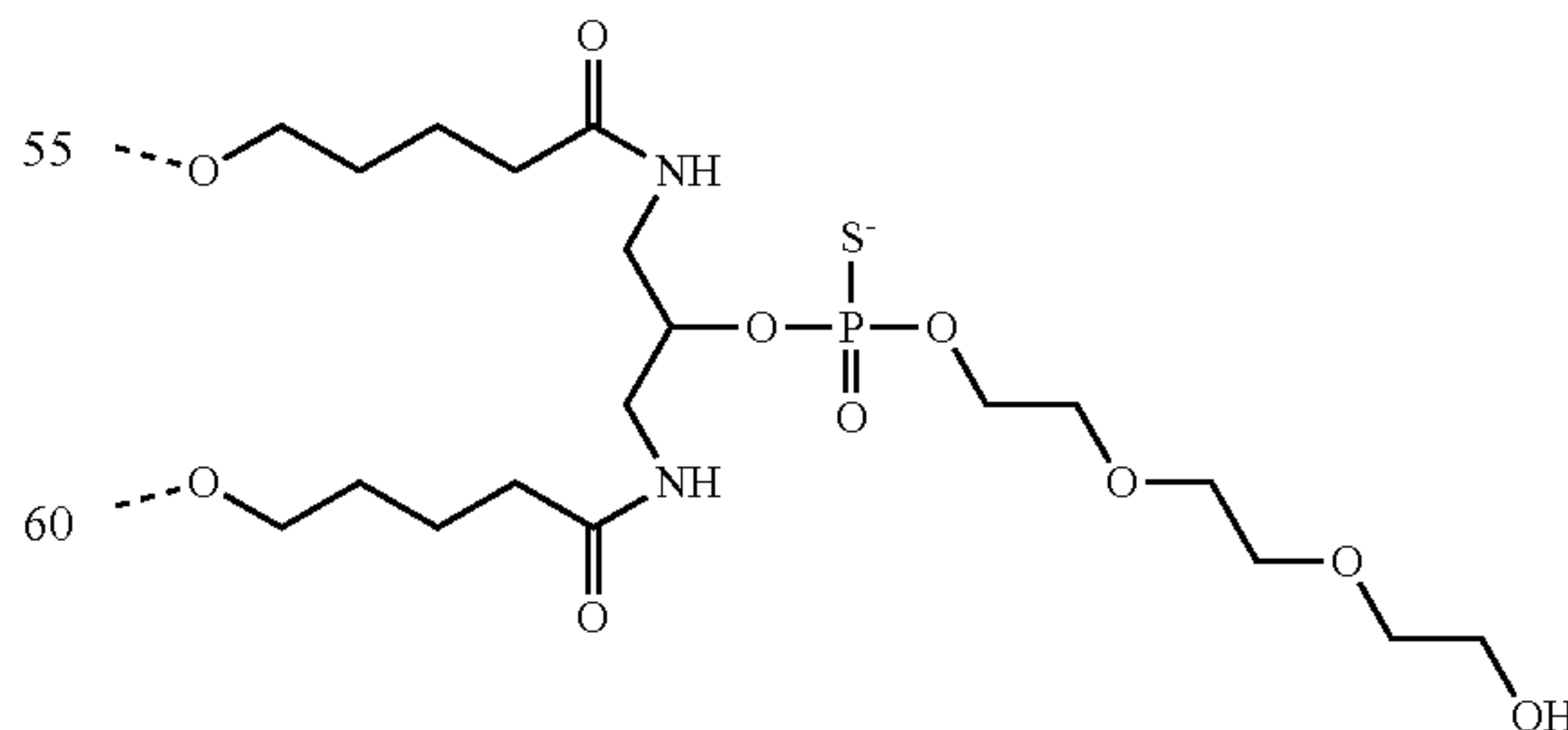
(Formula XI)
