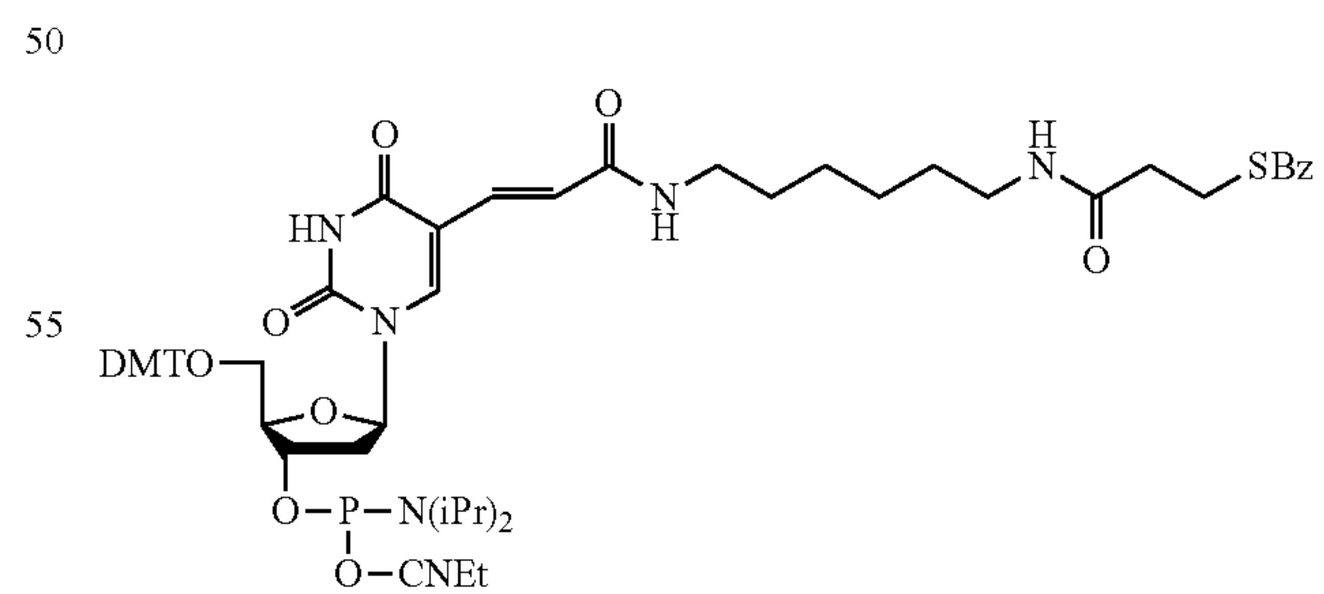
S-Bz-Thiol-Modifier C6 dT
