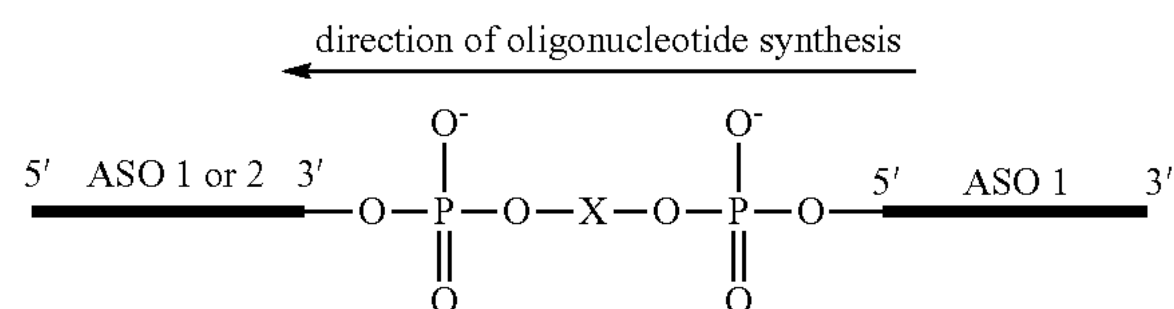
Formula I
