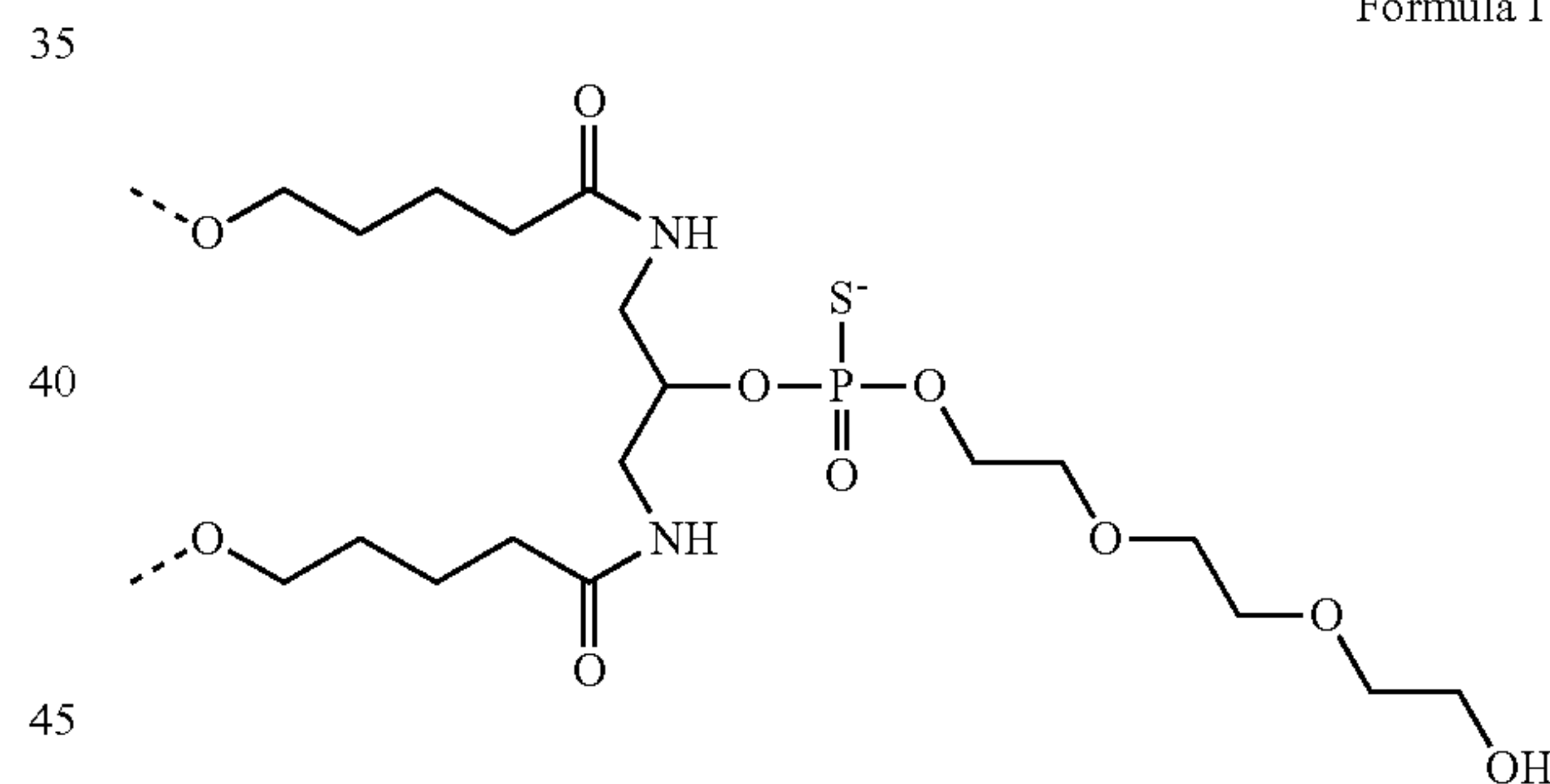
Formula IV
