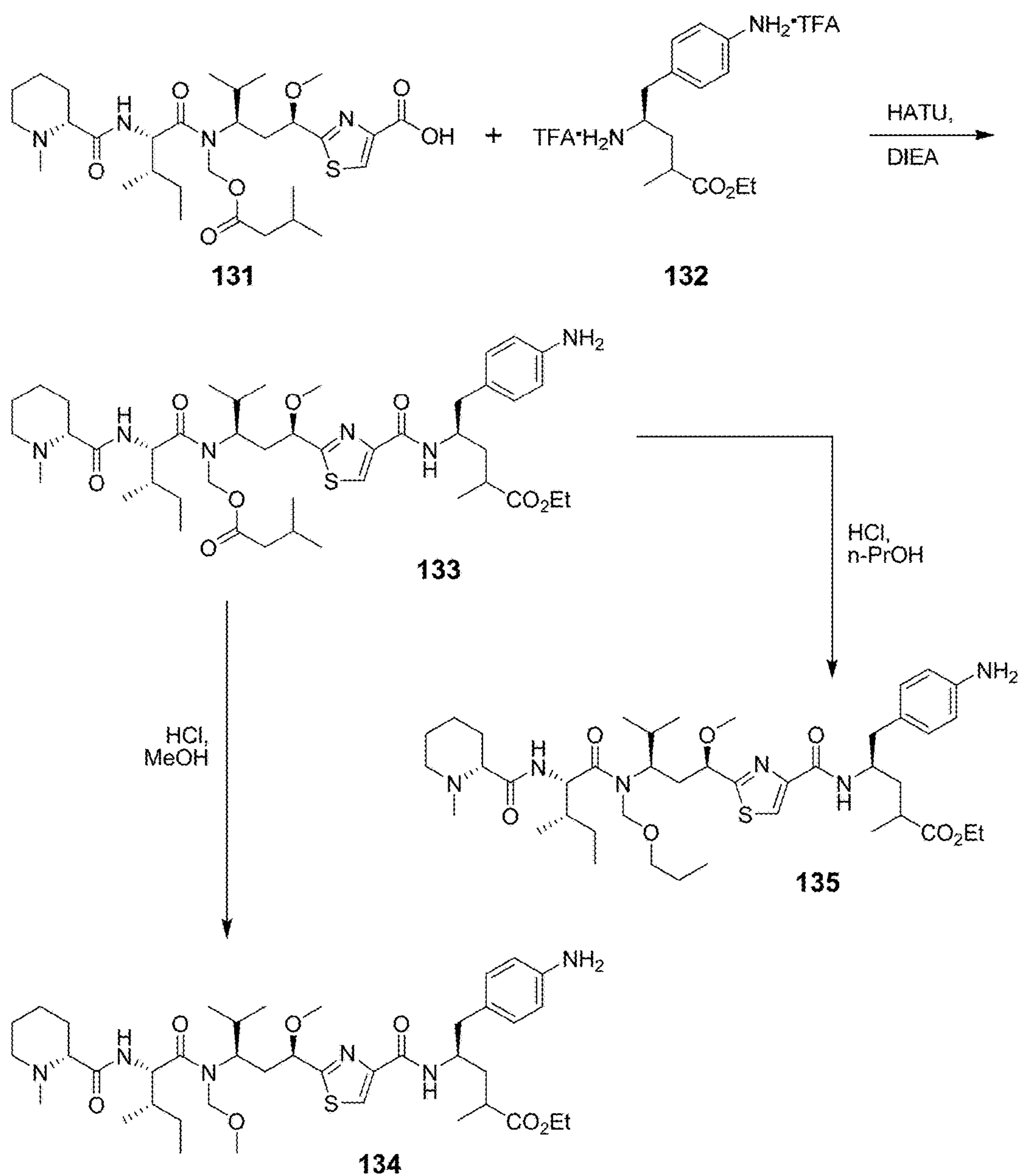
Scheme 21
