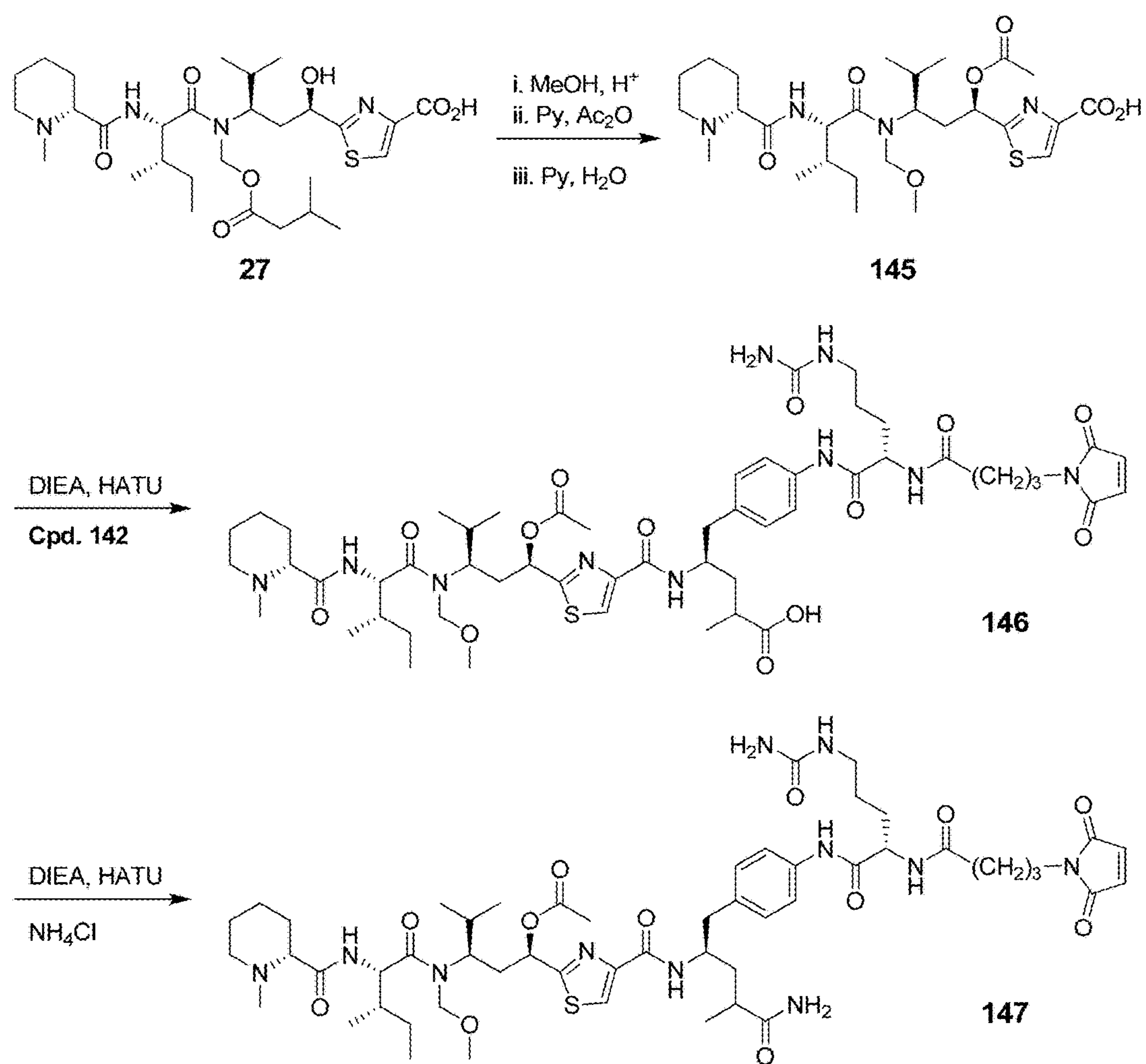
Scheme 23
