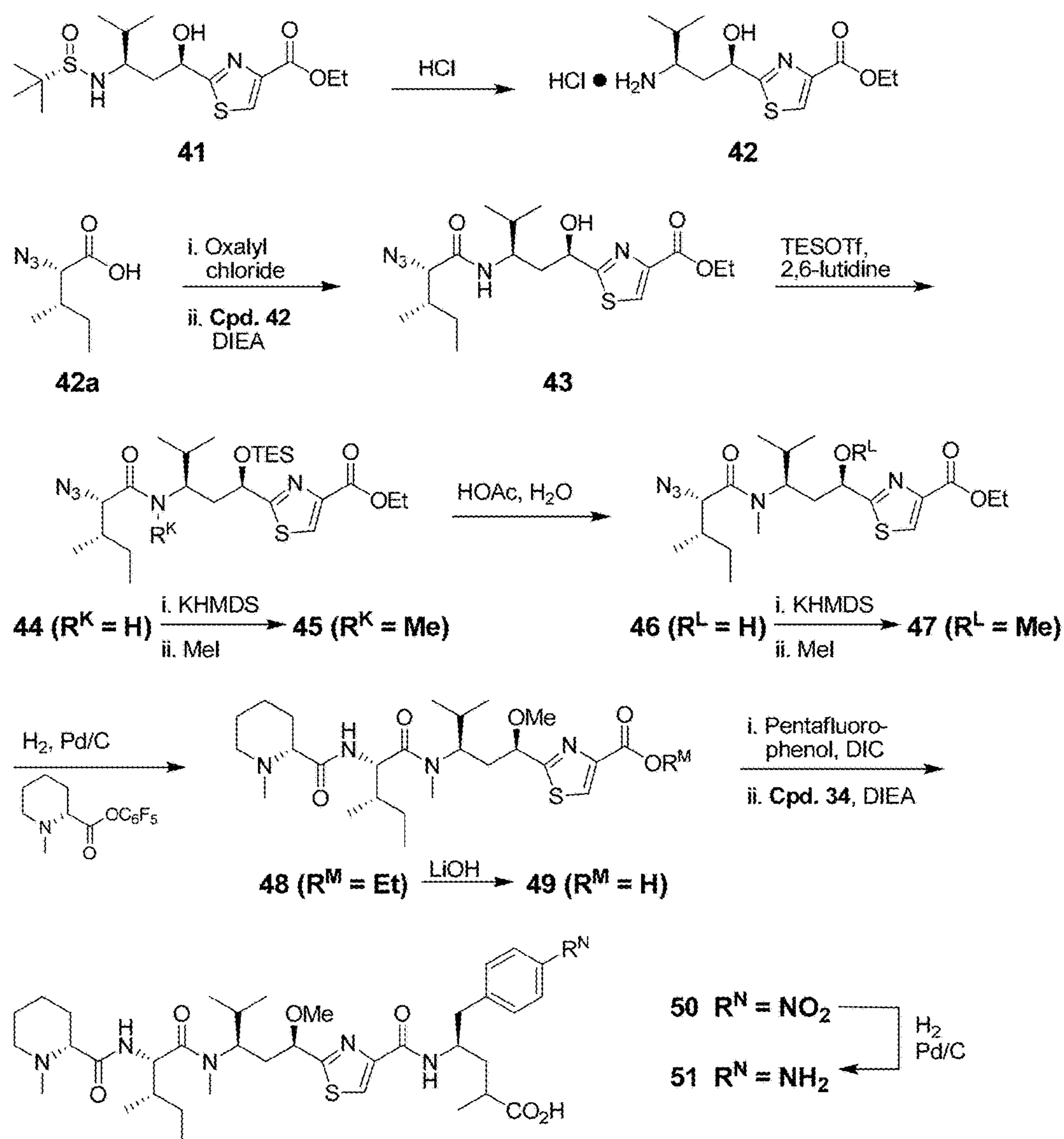
Scheme 5
