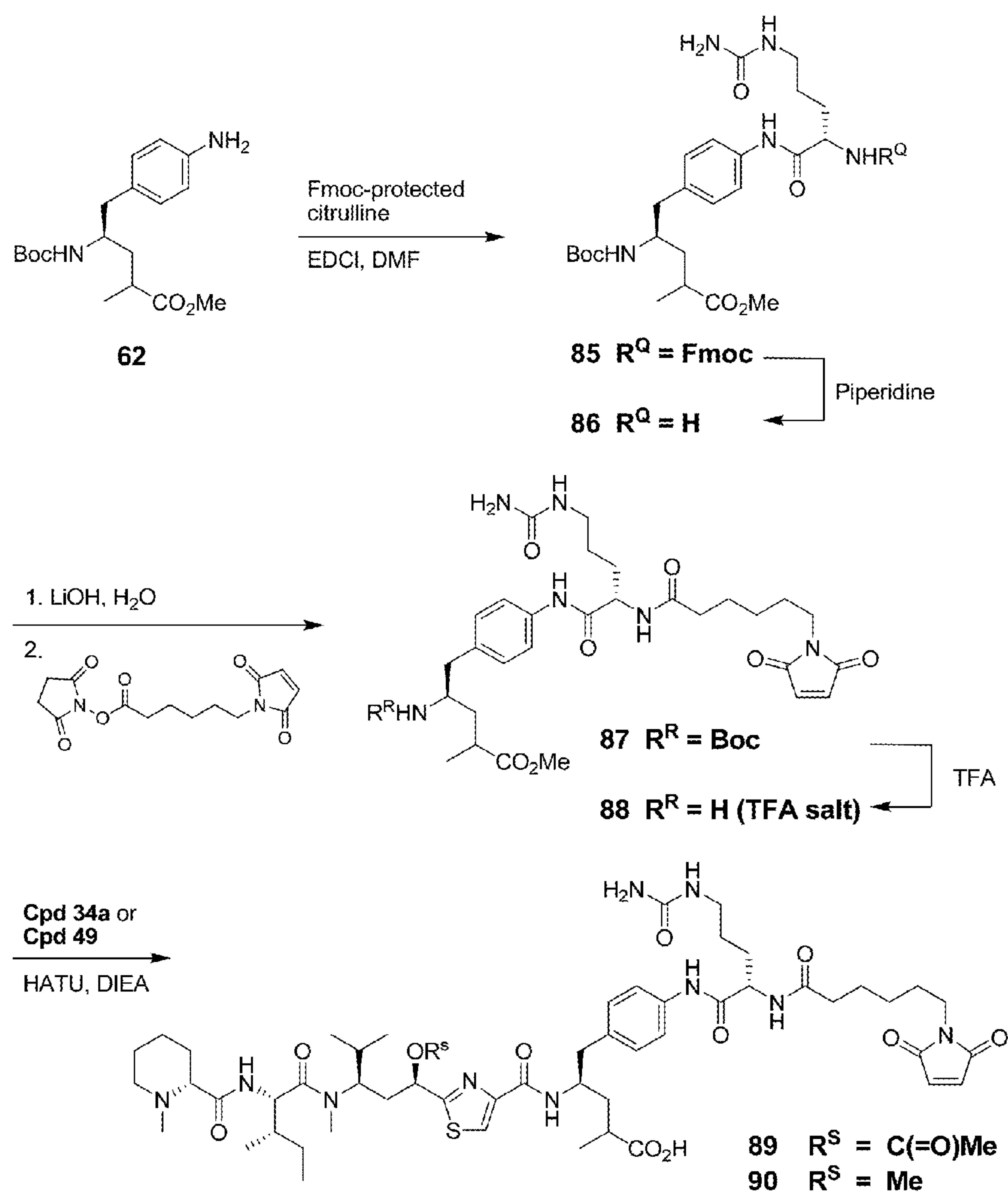
Scheme 15
