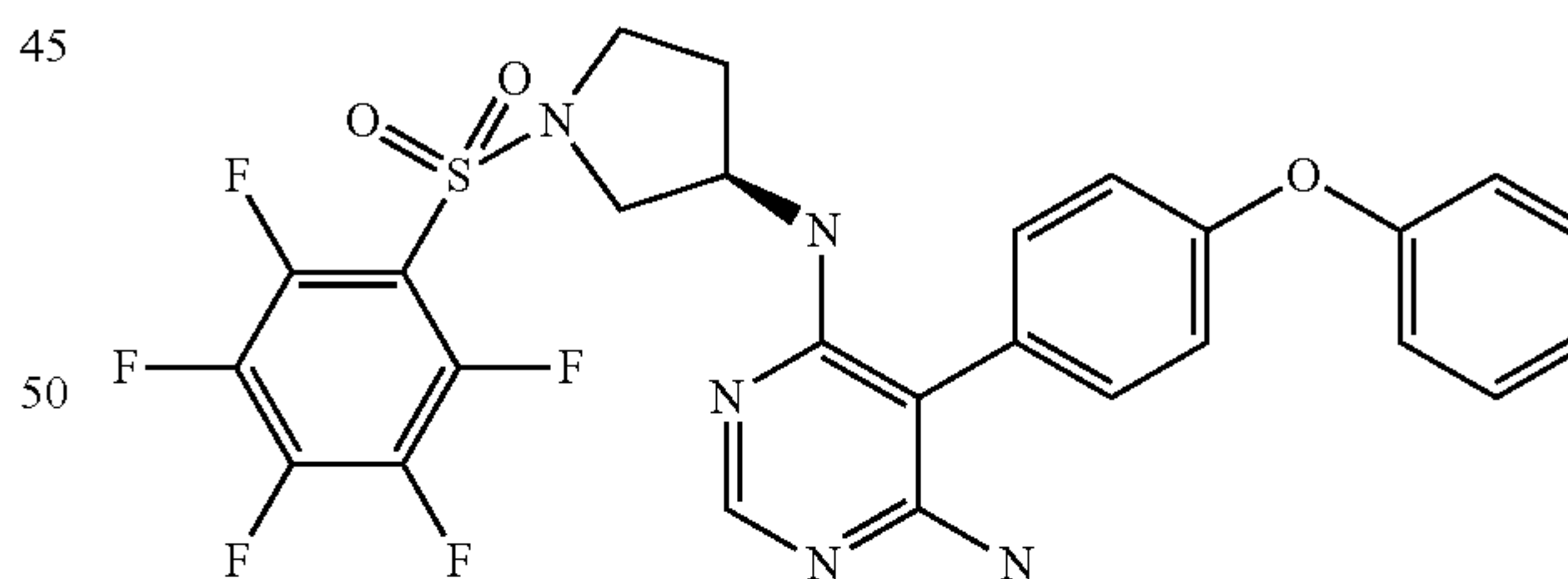
(R)-N4-(1-((perfluorophenyl)sulfonyl)pyrrolidin-3-yl)-5-(4-phenoxyphenyl)pyrimidine-4,6-diamine (A178)
