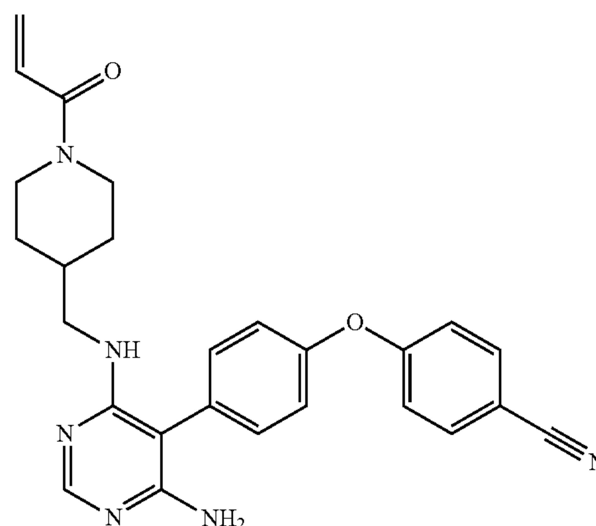
4-(4-(4-(((1-acryloylpiperidin-4-yl)methyl)amino)-6-aminopyrimidin-5-yl)phenoxy)benzonitrile (A86)
