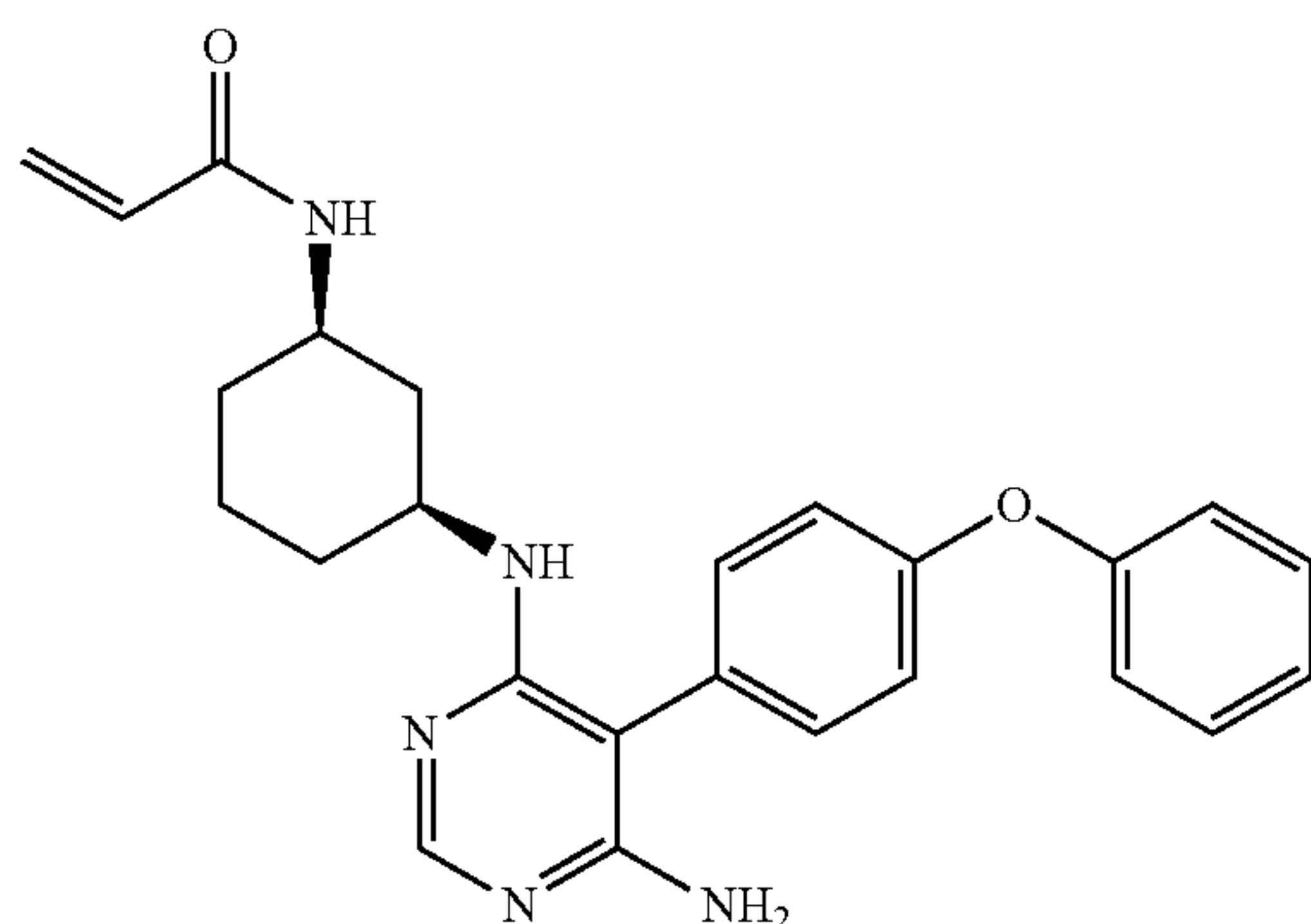
N-(cis-3-((6-amino-5-(4-phenoxyphenyl)pyrimidin-4-yl)amino)cyclohexyl)acrylamide (A51)
