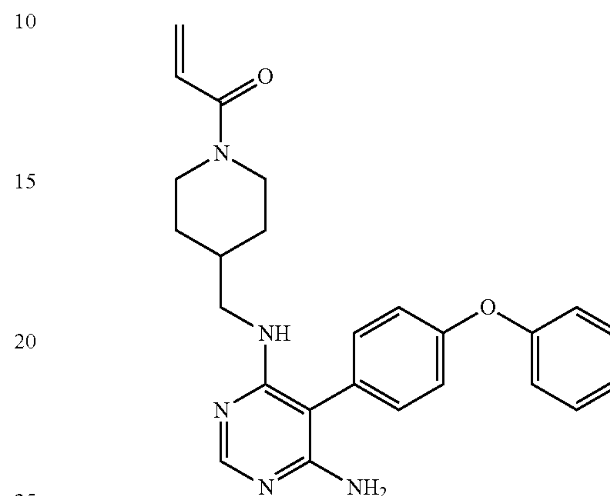
N-[(1-acryloylpiperidin-4-yl)methyl]-5-(4-phenoxyphenyl)pyrimidine-4,6-diamine
