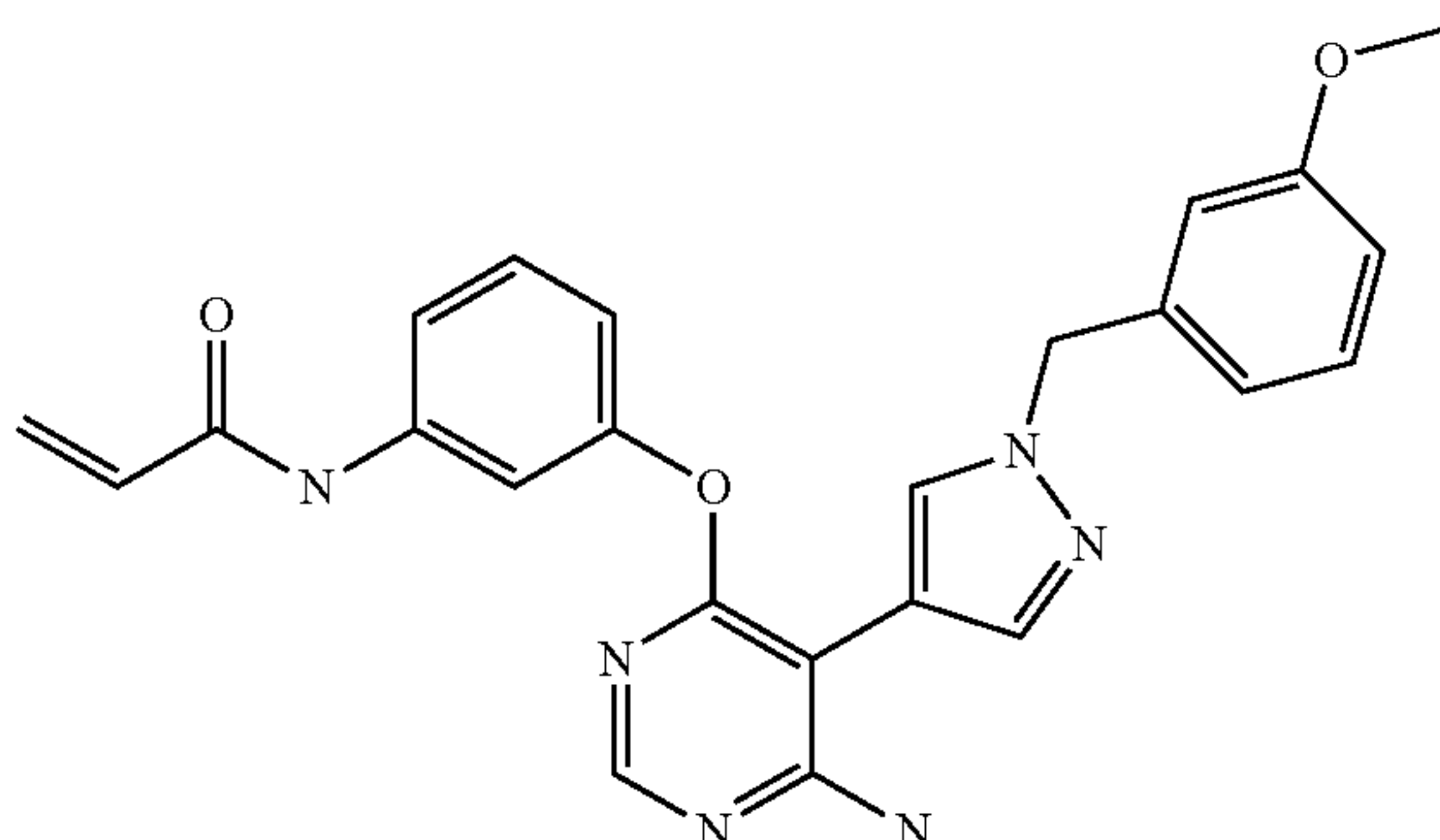
N-(3-((6-amino-5-(1-(3-methoxybenzyl)-1H-pyrazol-4-yl)pyrimidin-4-yl)oxy)phenyl)acrylamide (A198)
