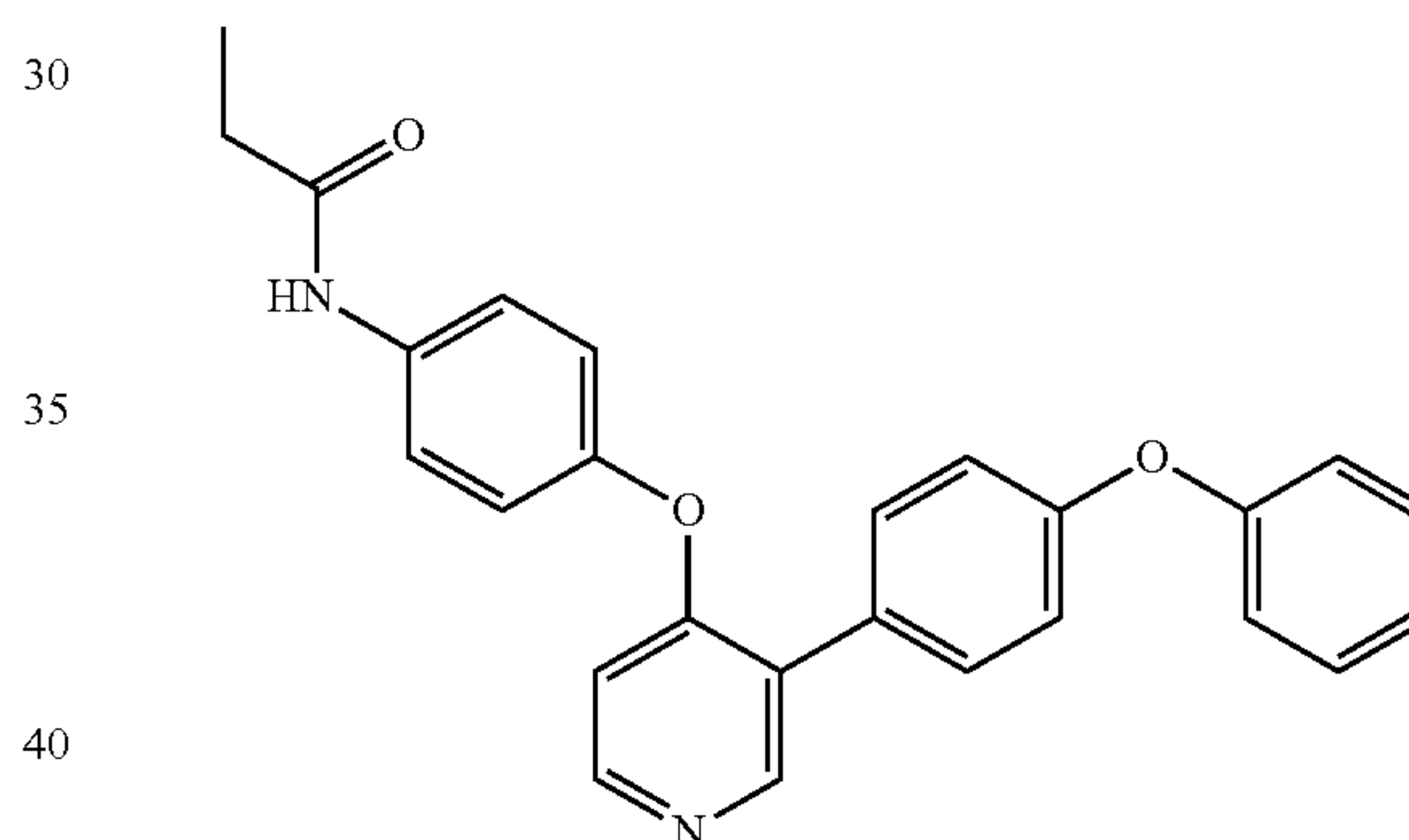
N-(4-((3-(4-phenoxyphenyl)pyridin-4-yl)oxy)phenyl)propionamide (A321)
