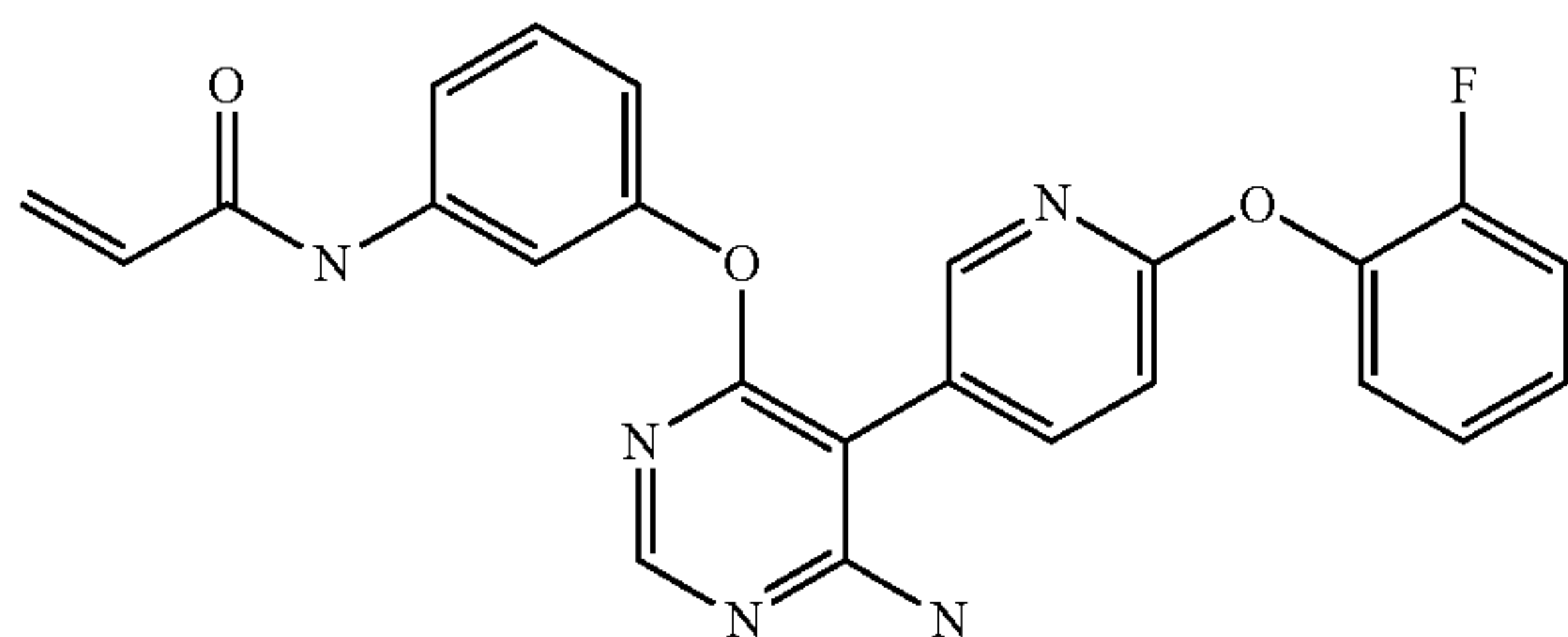
N-(3-((6-amino-5-(6-(2-fluorophenoxy)pyridin-3-yl)pyrimidin-4-yl)oxy)phenyl)acrylamide (A165)
