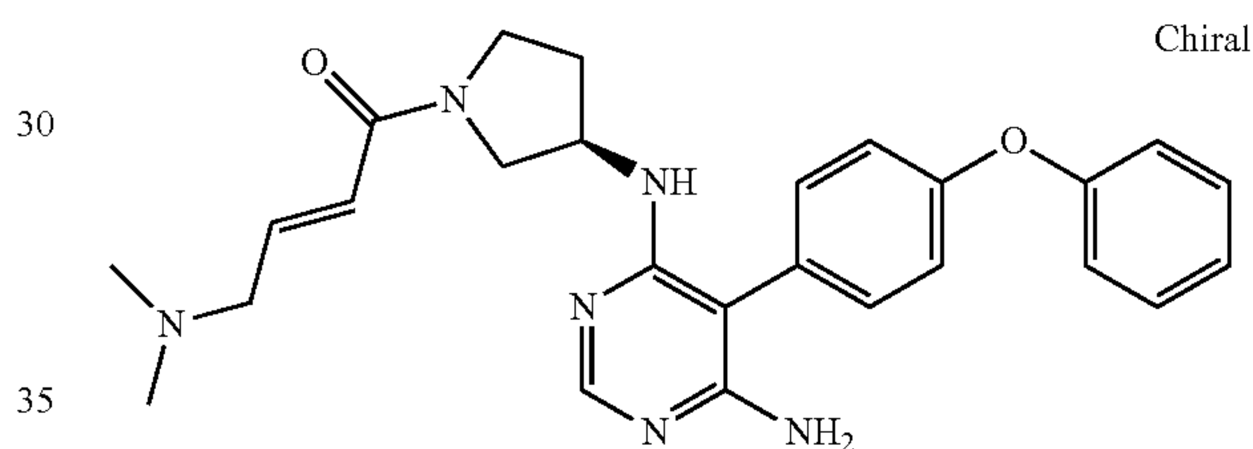
(R,E)-1-(3-((6-amino-5-(4-phenoxyphenyl)pyrimidin-4-yl)amino)pyrrolidin-1-yl)-4-(dimethylamino)but-2-en-1-one (A73)
