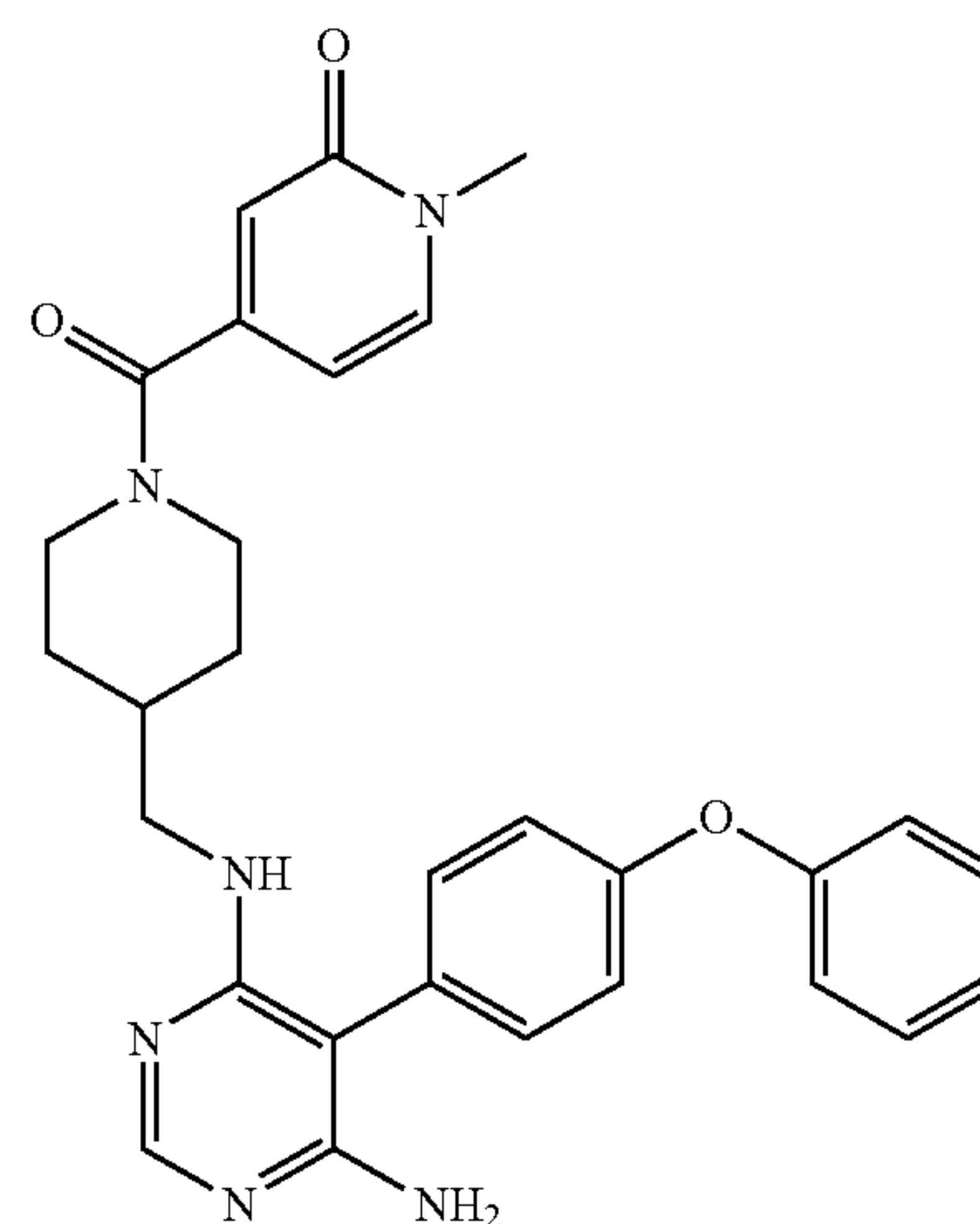
4-(4-(((6-amino-5-(4-phenoxyphenyl)pyrimidin-4-yl)amino)methyl)piperidine-1-carbonyl)-1-methylpyridin-2(1H)-one (A8)
