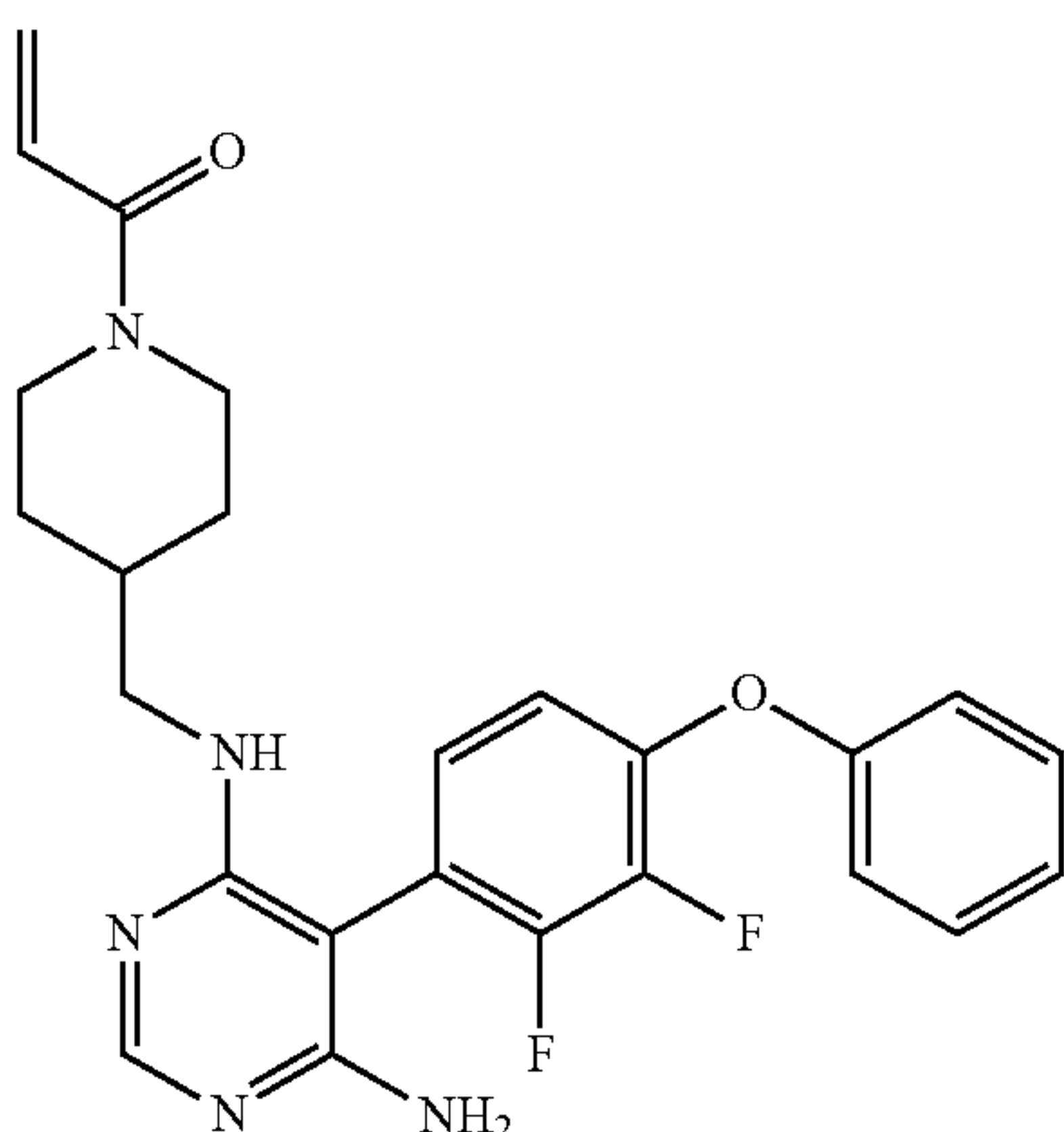
1-(4-(((6-amino-5-(2,3-difluoro-4-phenoxyphenyl)pyrimidin-4-yl)amino)methyl)piperidin-1-yl)prop-2-en-1-one (A88)
