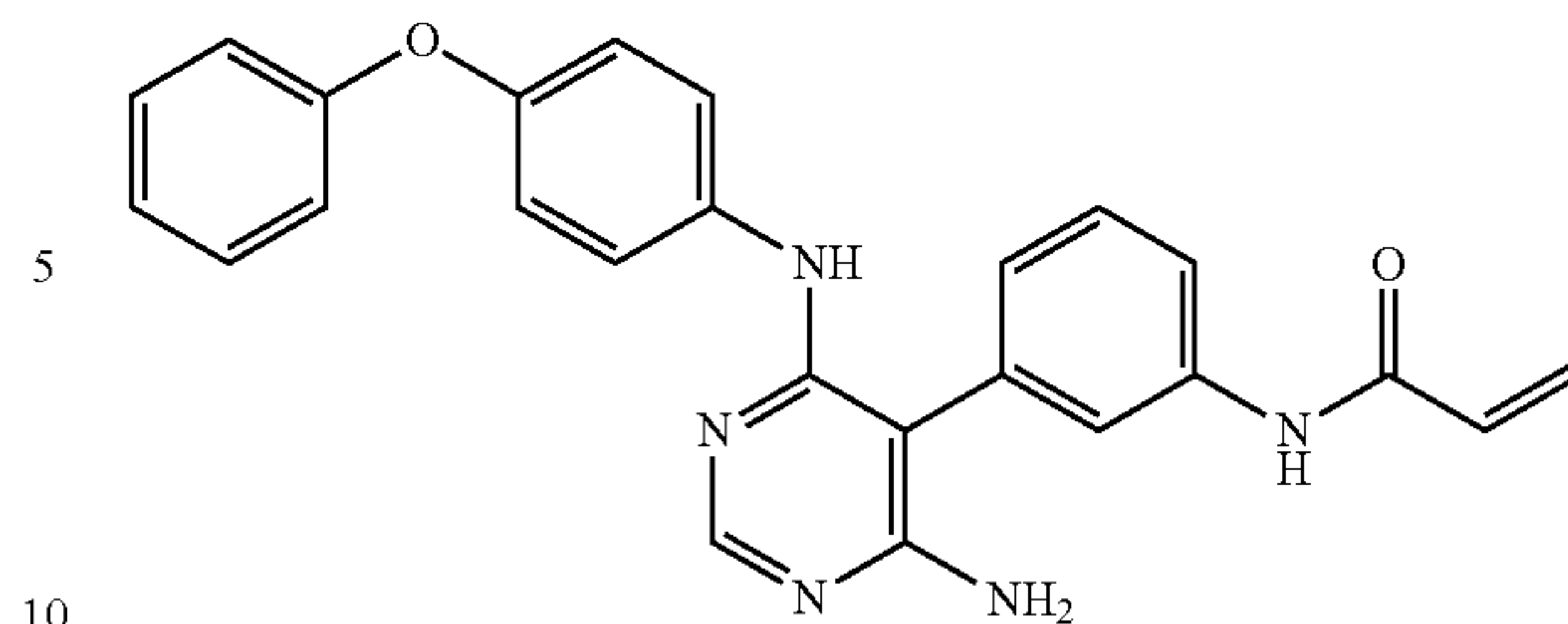
N-(3-(4-amino-6-((4-phenoxyphenyl)amino)pyrimidin-5-yl)phenyl)acrylamide (A241)
