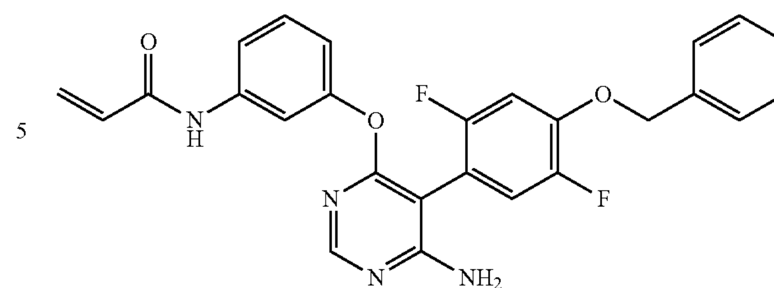
N-(3-((6-amino-5-(4-(benzyloxy)-2,5-difluorophenyl)pyrimidin-4-yl)oxy)phenyl)acrylamide (A339)
