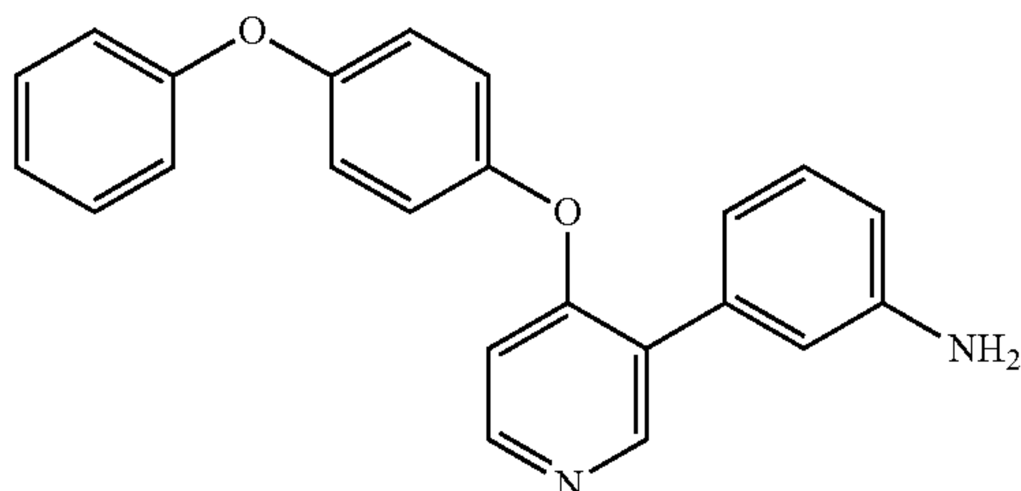
3-(4-(4-phenoxyphenoxy)pyridin-3-yl)aniline (A312)
