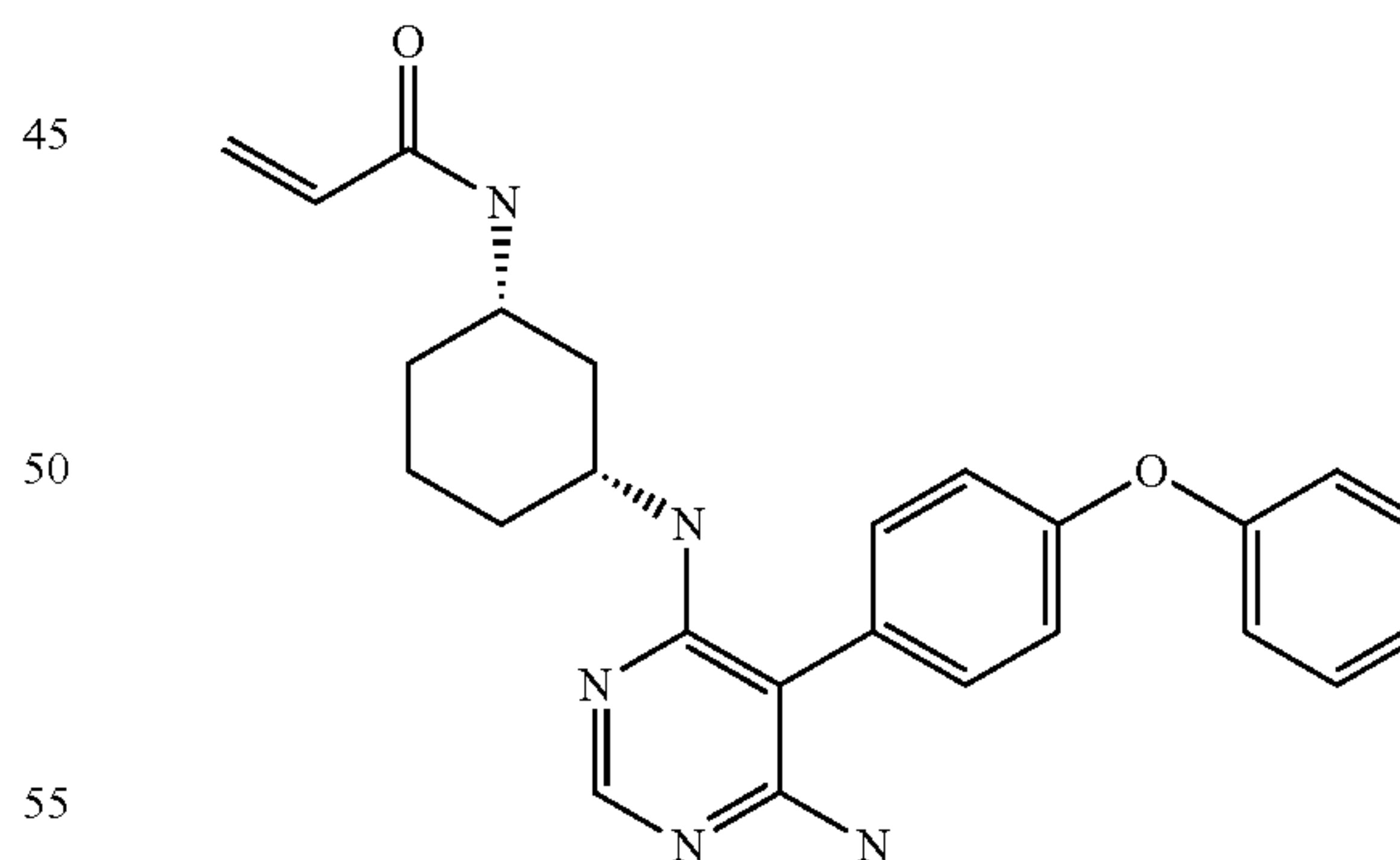
N-((1S,3R)-3-(((6-amino-5-(4-phenoxyphenyl)pyrimidin-4-yl)amino)cyclohexyl)acrylamide (A173)
