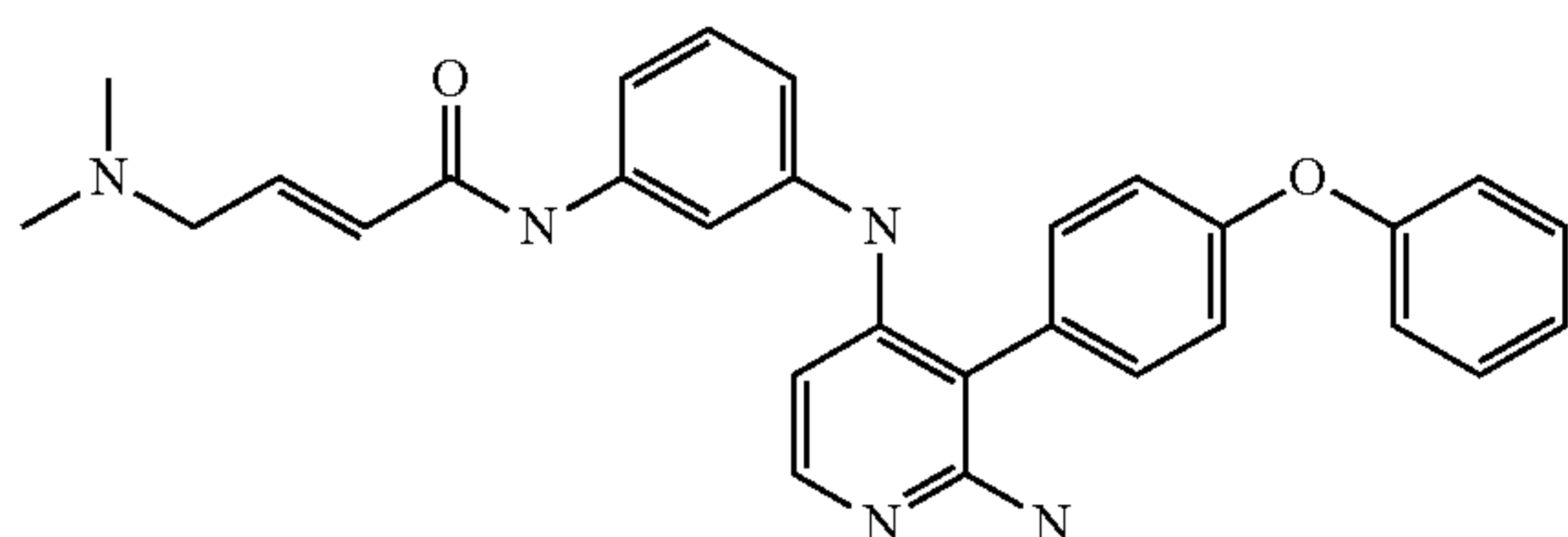
(E)-N-(3-((2-amino-3-(4-phenoxyphenyl)pyridin-4-yl)oxy)phenyl)-4-(dimethylamino)but-2-enamide (A151)
