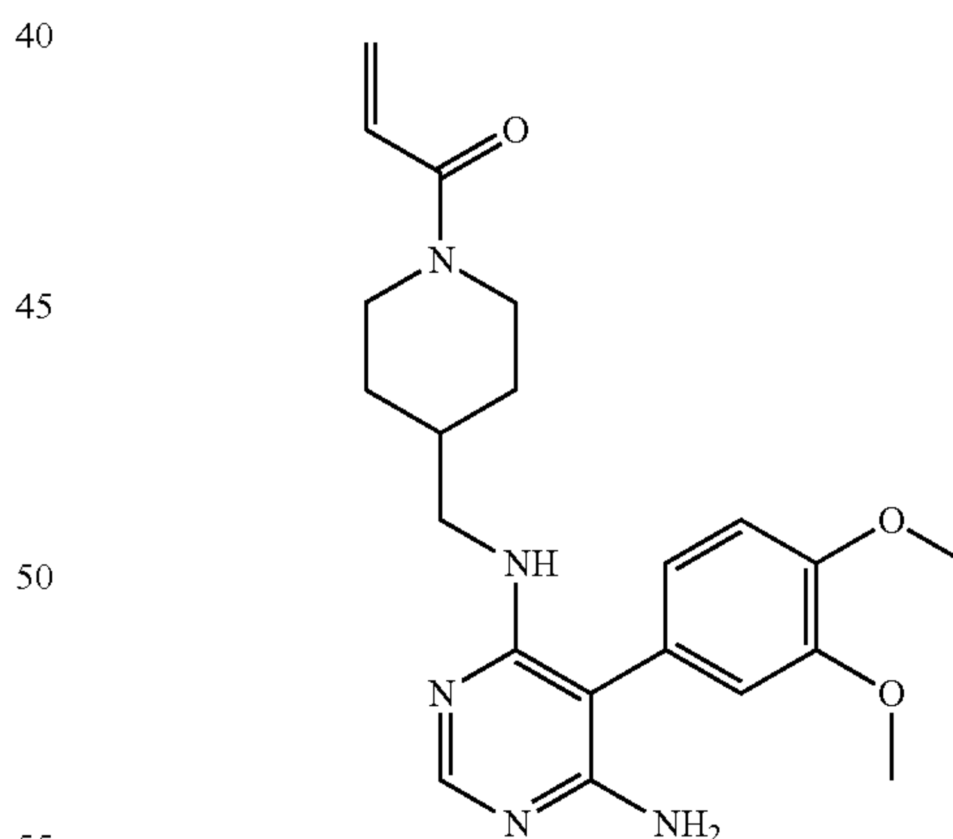
1-(4-(((6-amino-5-(3,4-dimethoxyphenyl)pyrimidin-4-yl)amino)methyl)piperidin-1-yl)prop-2-en-1-one (A82)
