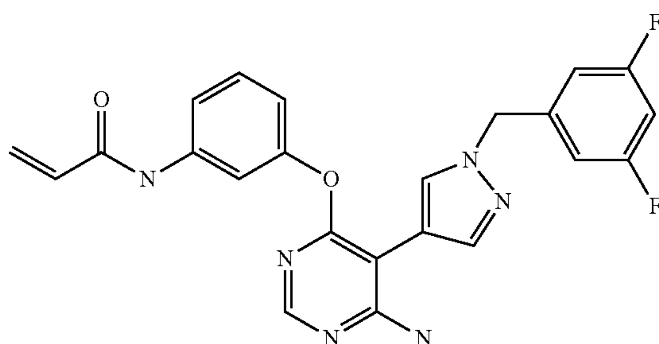
N-(3-((6-amino-5-(1-(3,5-difluorobenzyl)-1H-pyrazol-4-yl)pyrimidin-4-yl)oxy)phenyl)acrylamide (A183)
