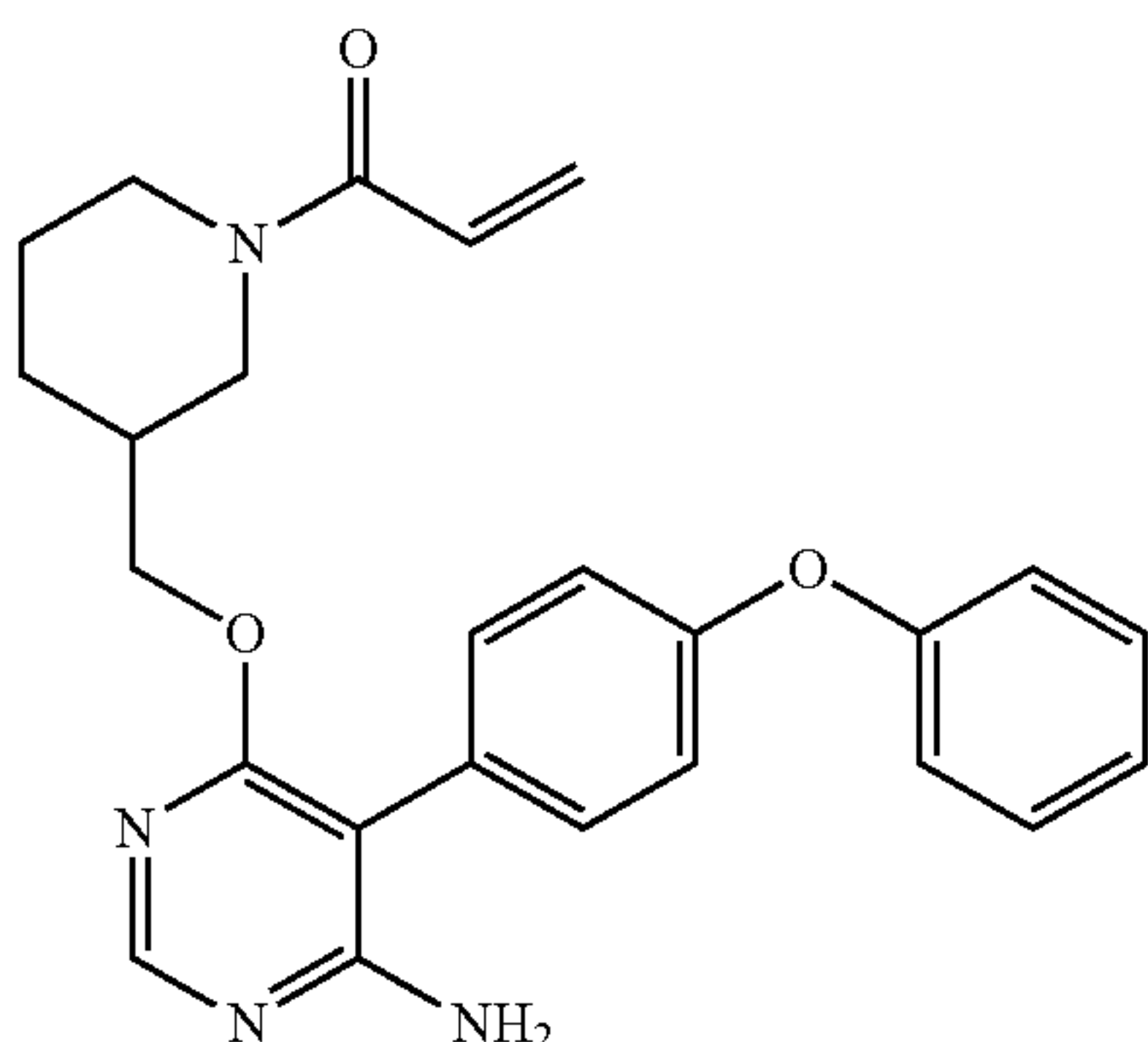
1-(3-(((6-amino-5-(4-phenoxyphenyl)pyrimidin-4-yl)oxy)methyl)piperidin-1-yl)prop-2-en-1-one (A17)
