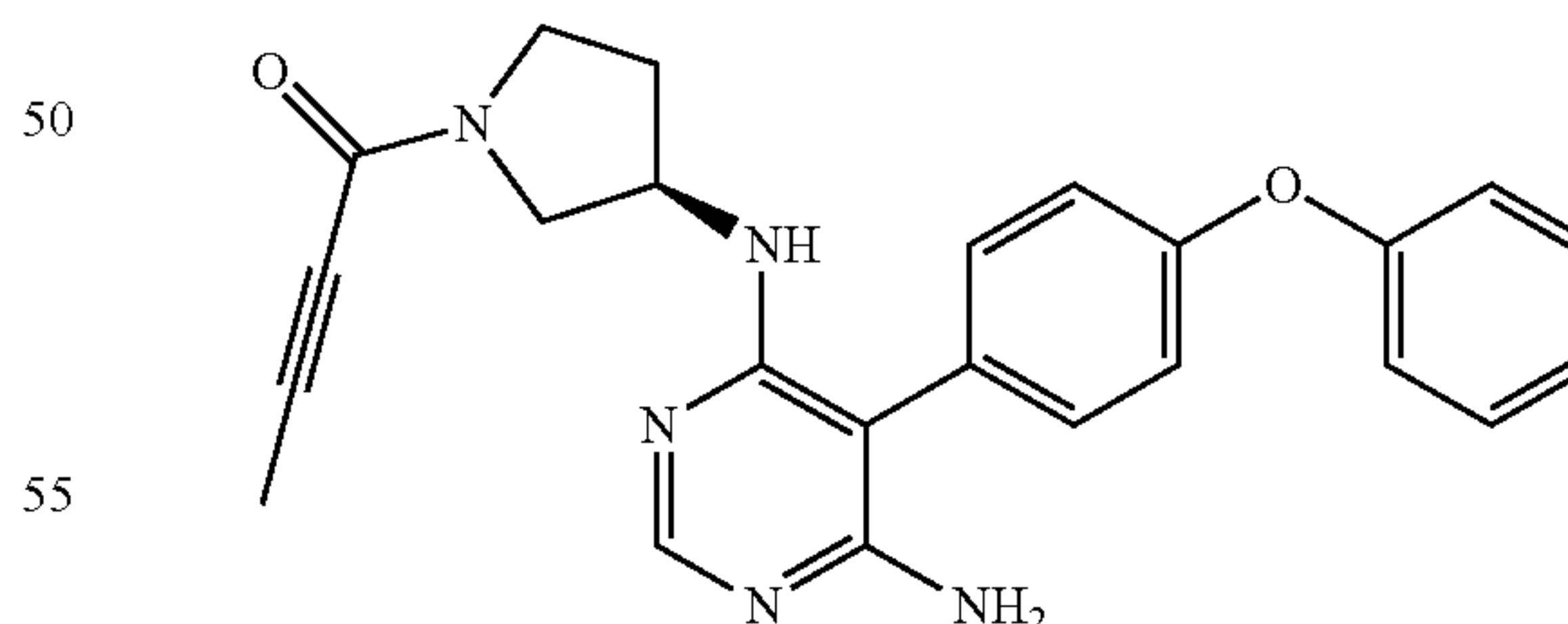
(R)-1-(3-((6-amino-5-(4-phenoxyphenyl)pyrimidin-4-yl)amino)pyrrolidin-1-yl)but-2-yn-1-one (A341)
