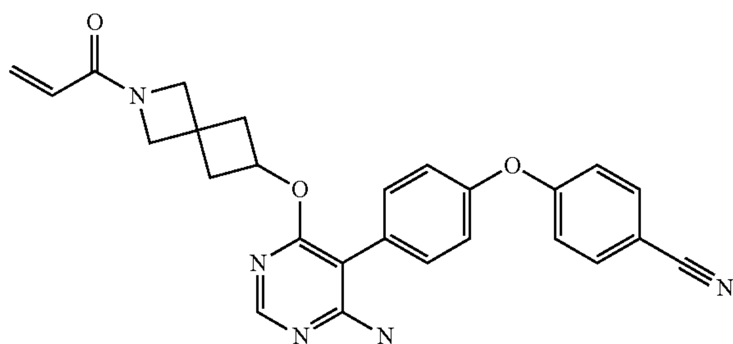
4-(4-(4-((2-acryloyl-2-azaspiro[3.3]heptan-6-yl)oxy)-6-aminopyrimidin-5-yl)phenoxy)benzonitrile (A202)
