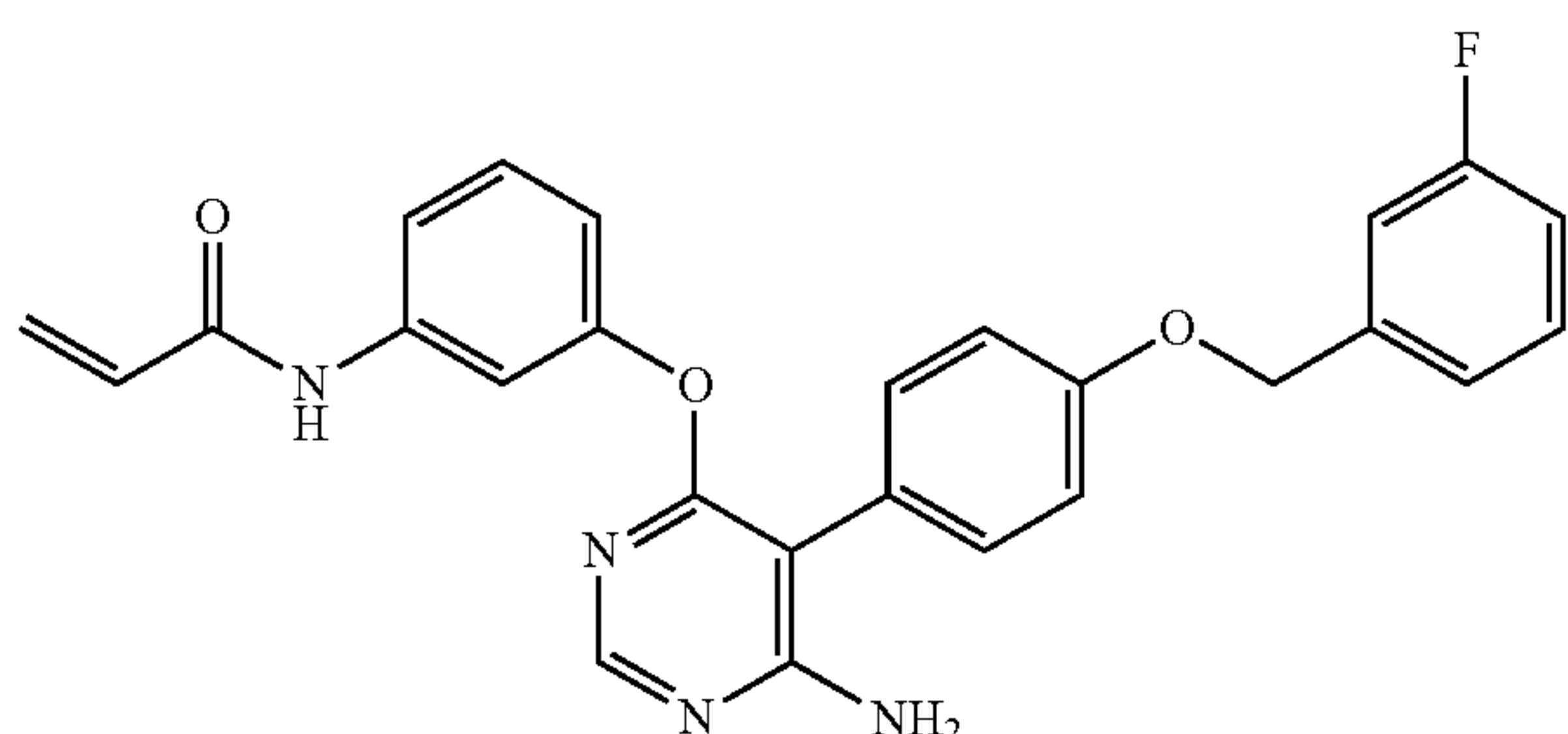
N-(3-((6-amino-5-(4-((3-fluorobenzyl)oxy)phenyl)pyrimidin-4-yl)oxy)phenyl)acrylamide (A260)
