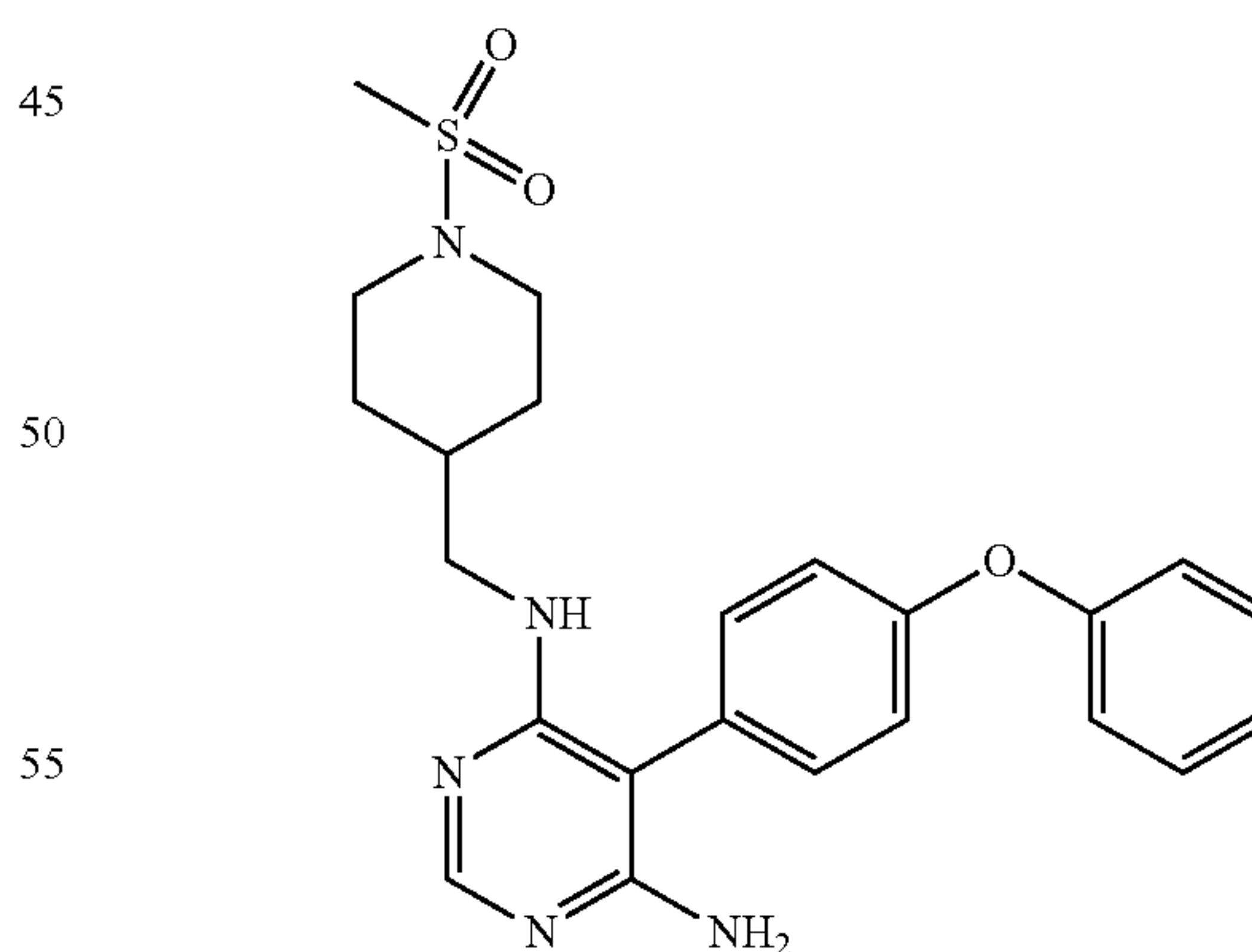
N4-((1-(methylsulfonyl)piperidin-4-yl)methyl)-5-(4-phenoxyphenyl)pyrimidine-4,6-diamine (A55)
