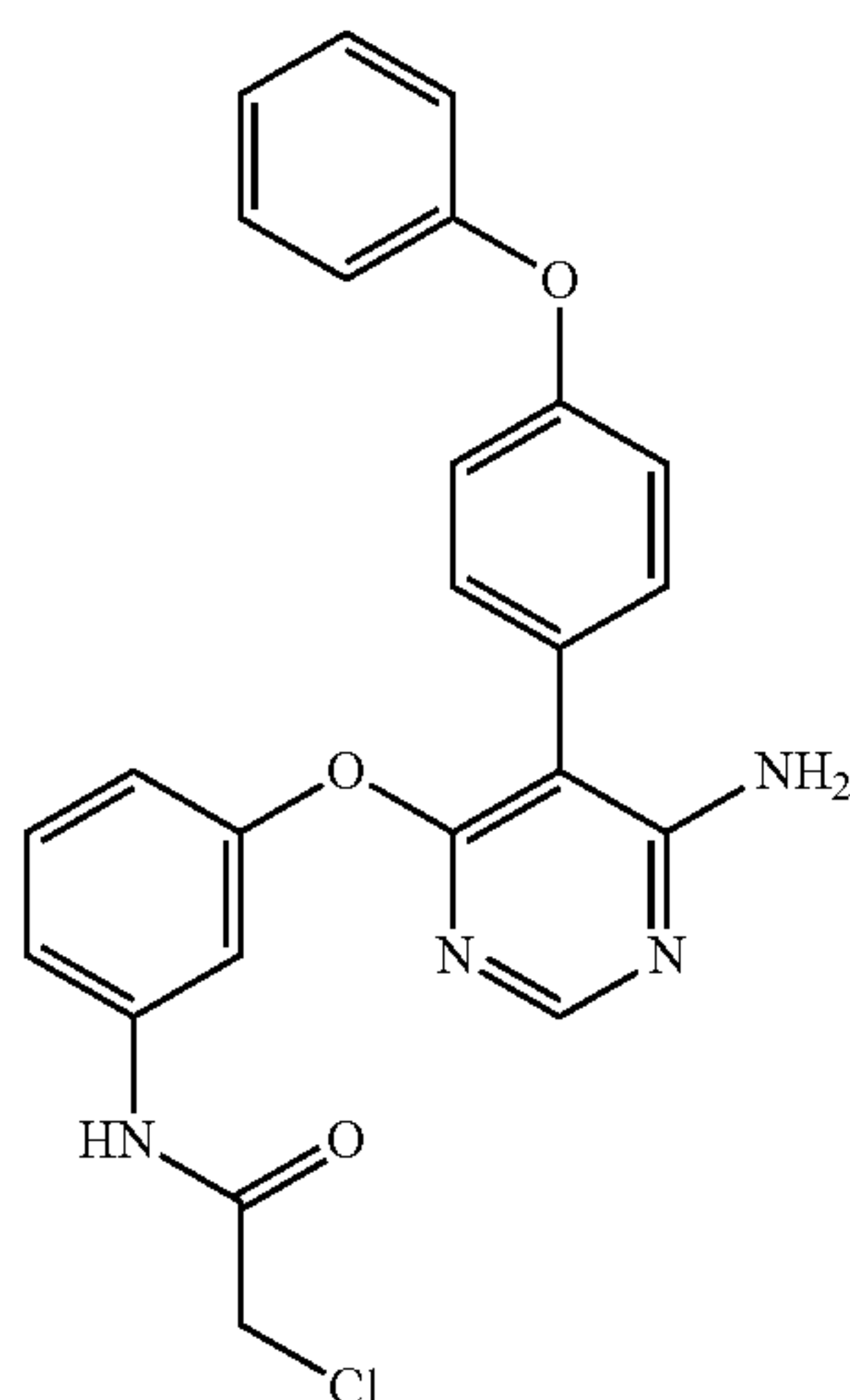
N-{3-[6-Amino-5-(4-phenoxy-phenyl)-pyrimidin-4-yloxy]-phenyl}-2-chloroacetamide (A342)
