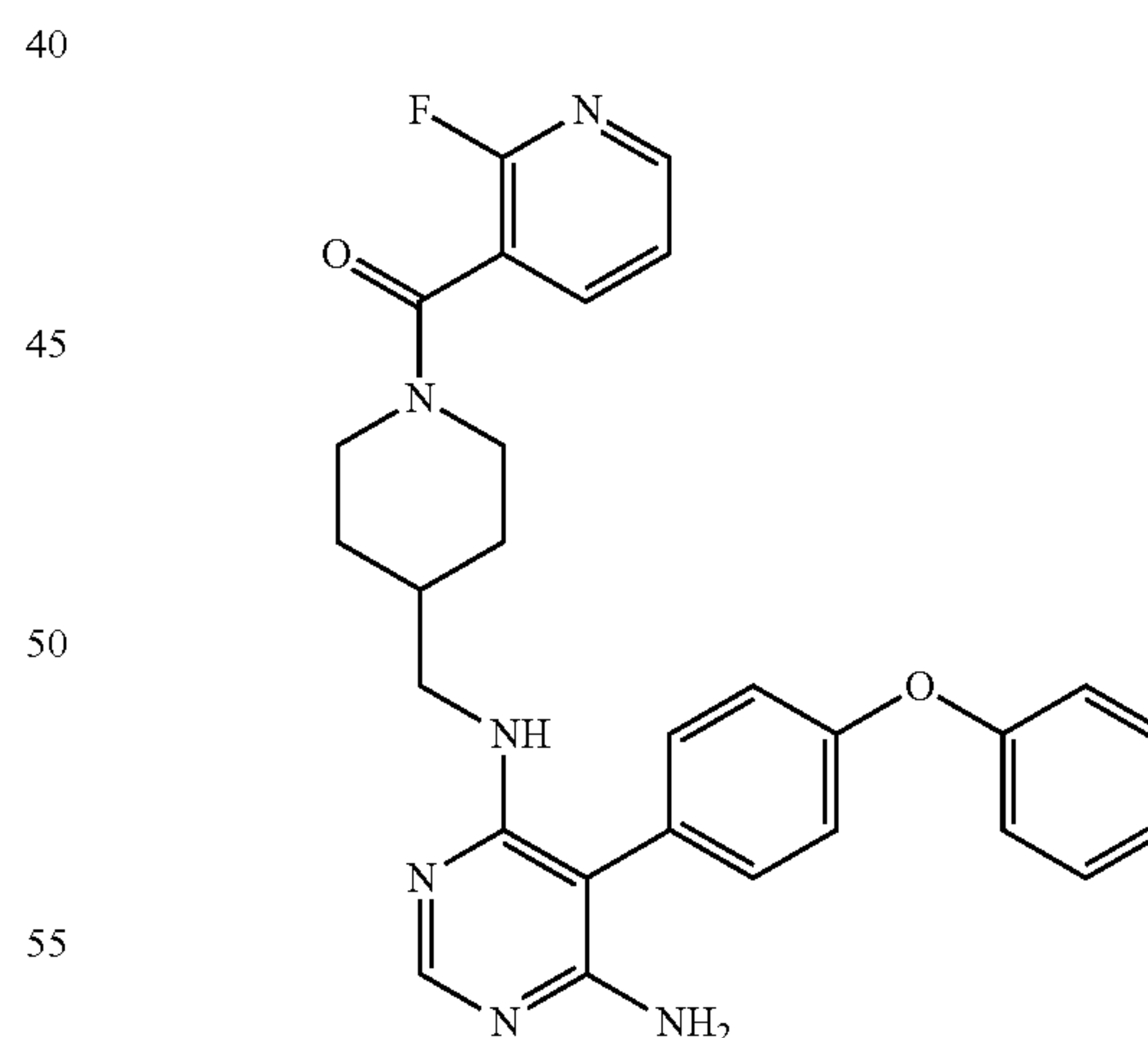
4-(((6-amino-5-(4-phenoxyphenyl)pyrimidin-4-yl)amino)methyl)piperidin-1-yl(2-fluoropyridin-3-yl)methanone (A12)
