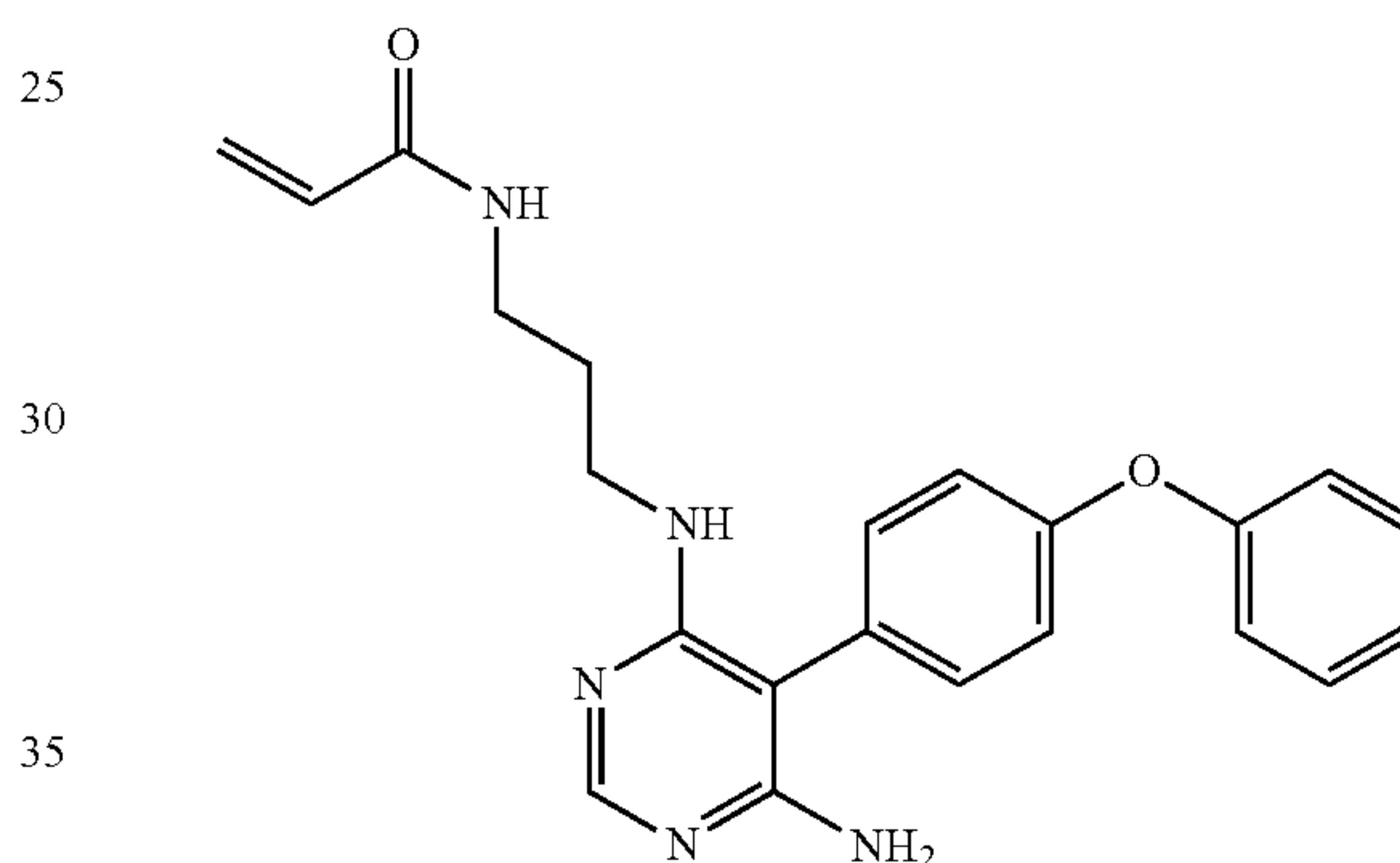
N-(3-(((6-amino-5-(4-phenoxyphenyl)pyrimidin-4-yl)amino)propyl)acrylamide (A59)
