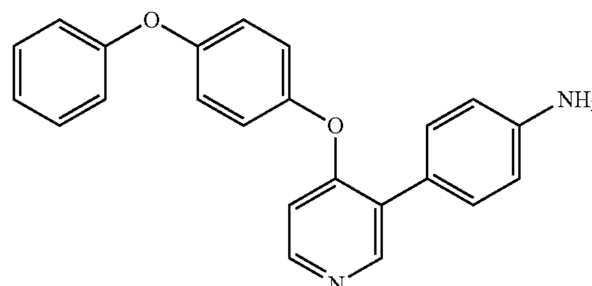
4-(4-(4-phenoxyphenoxy)pyridin-3-yl)aniline (A314)
