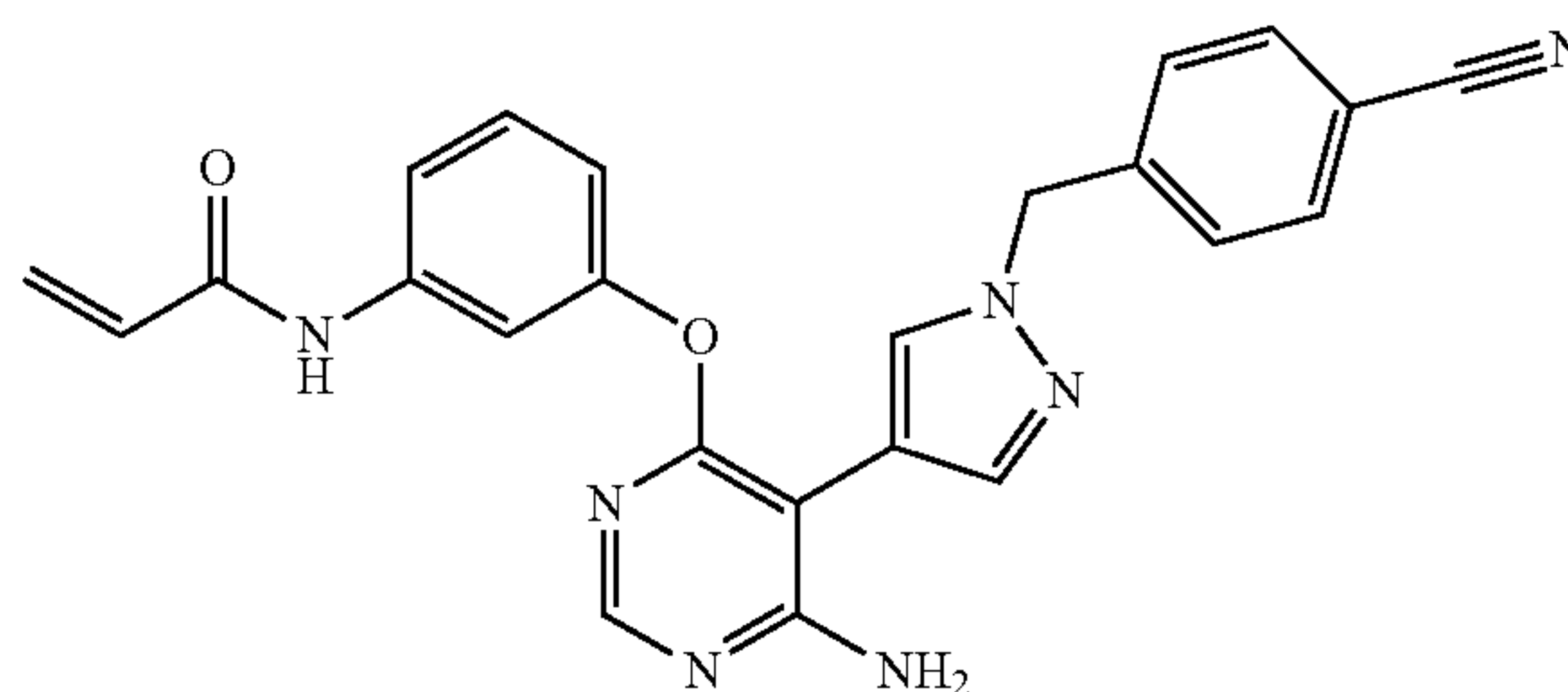
N-(3-(((6-amino-5-(1-(4-cyanobenzyl)-1H-pyrazol-4-yl)pyrimidin-4-yl)oxy)phenyl)acrylamide (A69)
