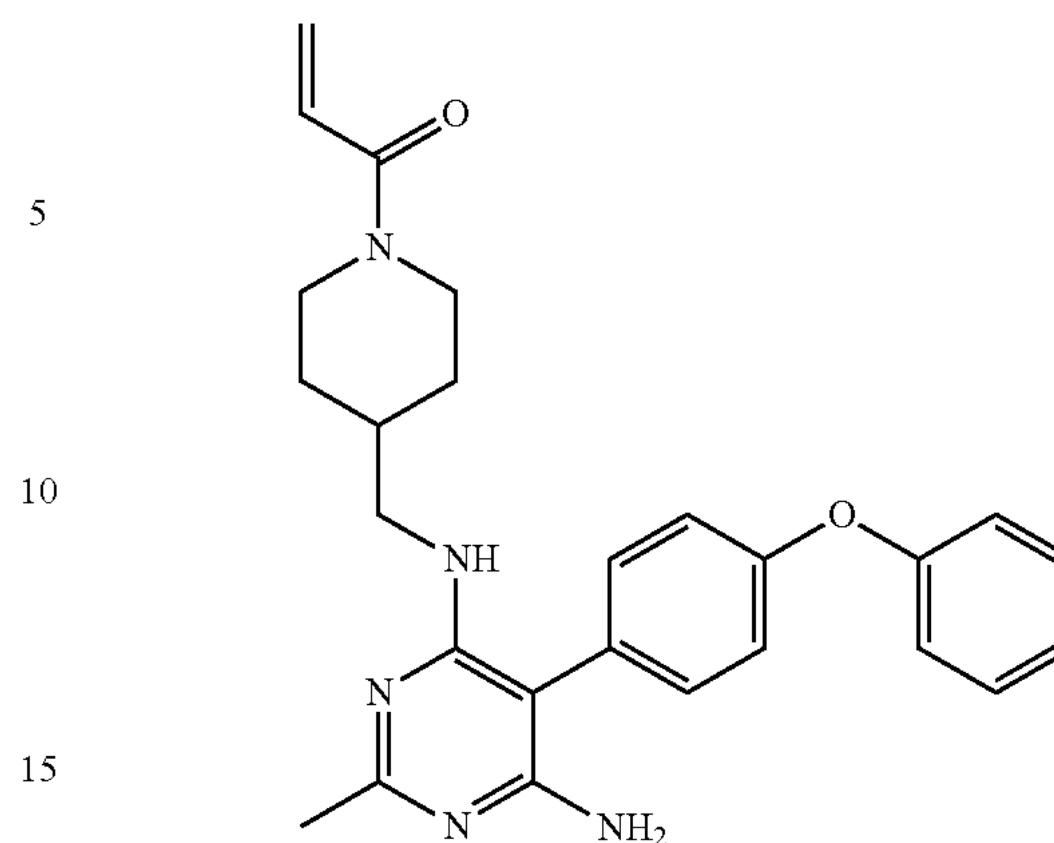
1-(4-(((6-amino-2-methyl-5-(4-phenoxyphenyl)pyrimidin-4-yl)amino)methyl)piperidin-1-yl)prop-2-en-1-one (A36)
