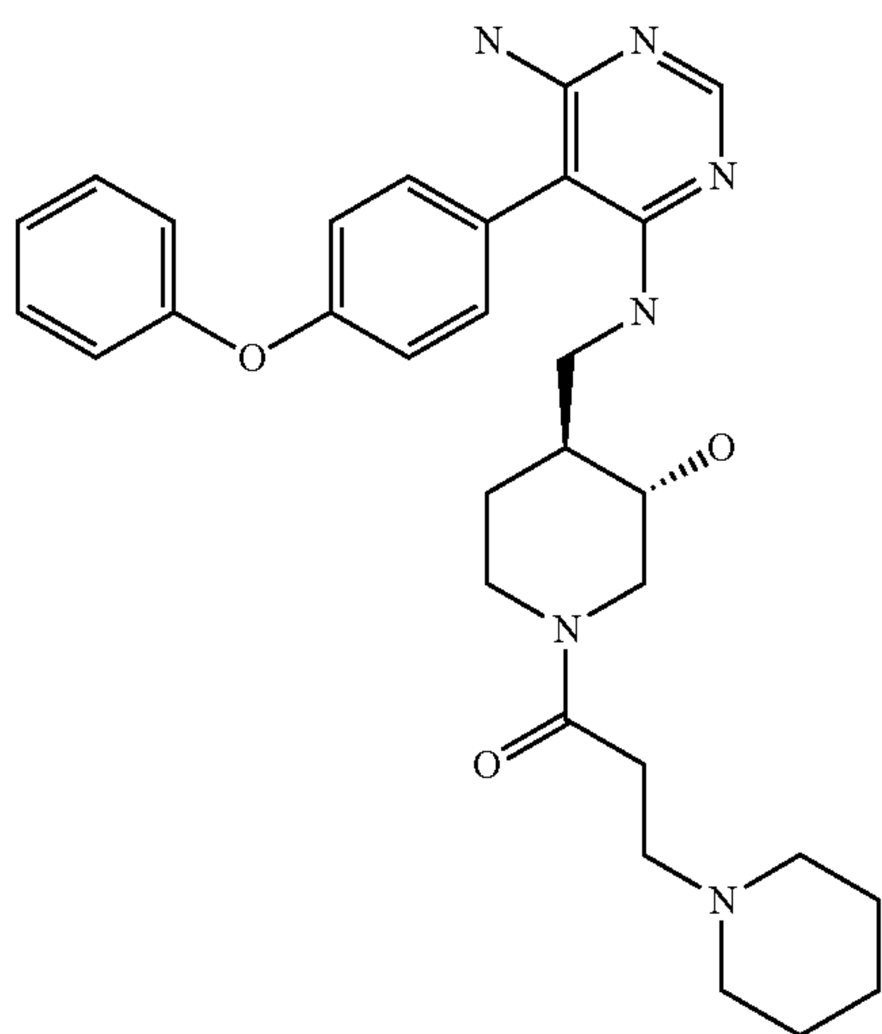
1-((3S,4S)-4-(((6-amino-5-(4-phenoxyphenyl)pyrimidin-4-yl)amino)methyl)-3-hydroxypiperidin-1-yl)-3-(piperidin-1-yl)propan-1-one (A233)
