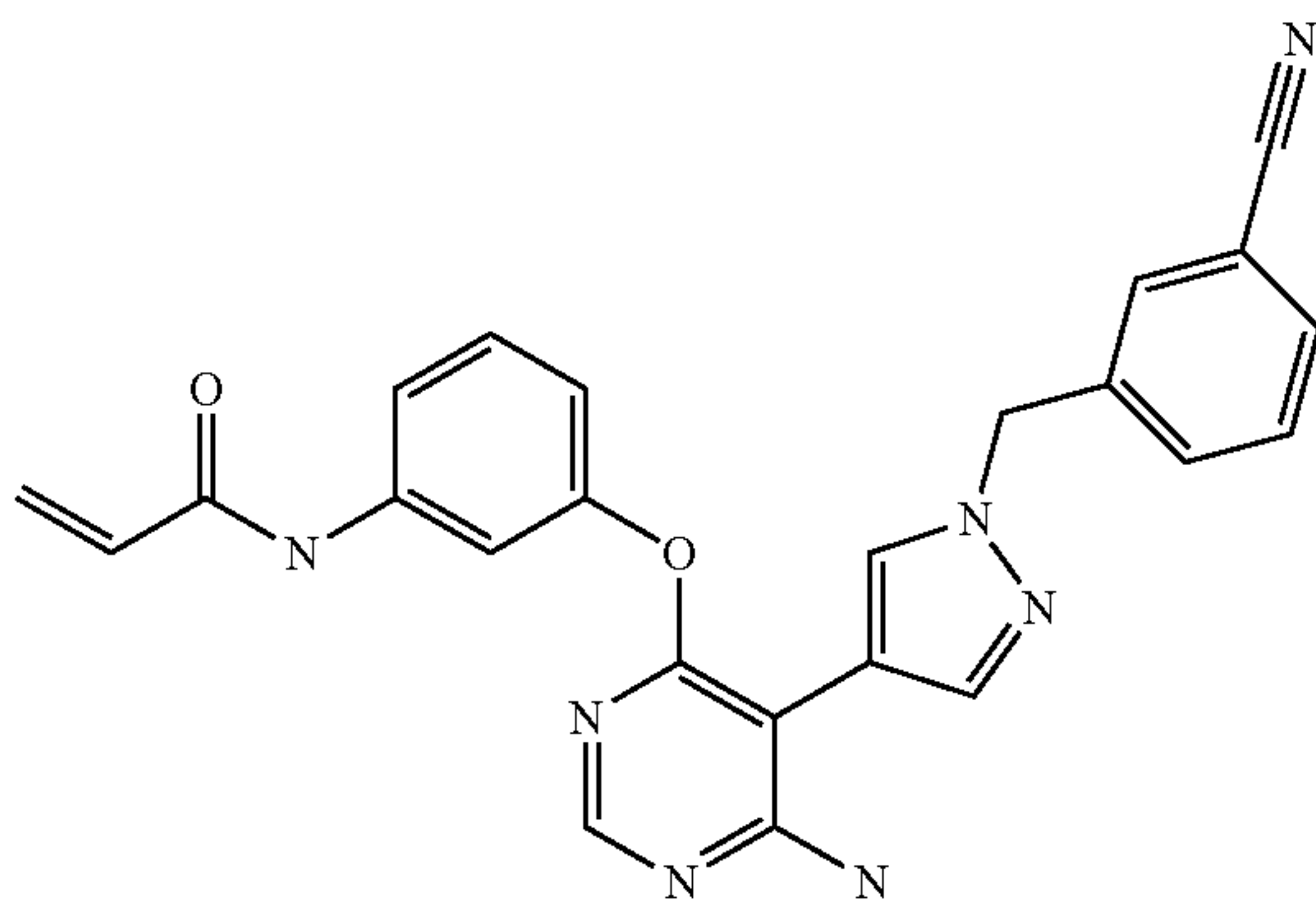
N-(3-((6-amino-5-(1-(3-cyanobenzyl)-1H-pyrazol-4-yl)pyrimidin-4-yl)oxy)phenyl)acrylamide (A203)
