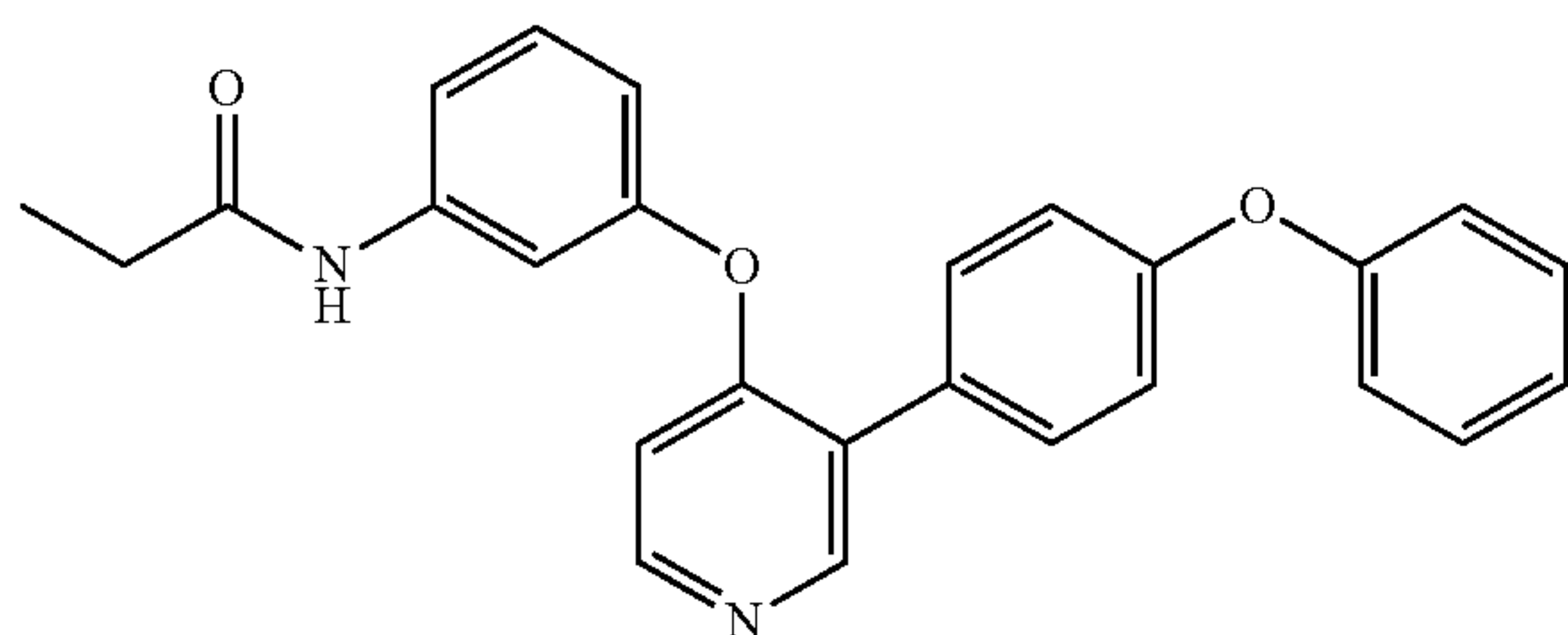
N-(3-((3-(4-phenoxyphenyl)pyridin-4-yl)oxy)phenyl)propionamide (A318)
