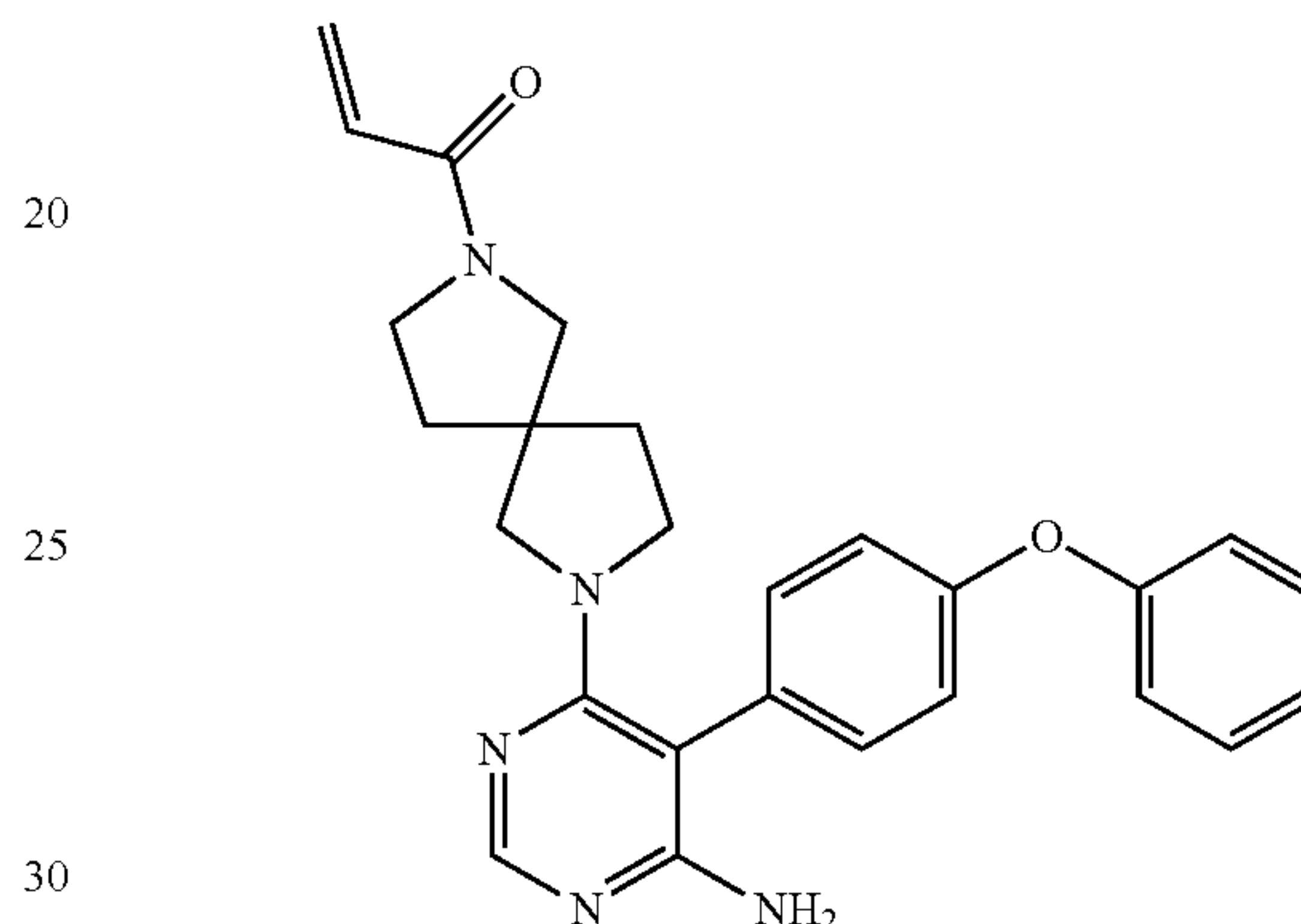
1-(7-(6-amino-5-(4-phenoxyphenyl)pyrimidin-4-yl)-2,7-diazaspiro[4.4]nonan-2-yl)prop-2-en-1-one (A93)
