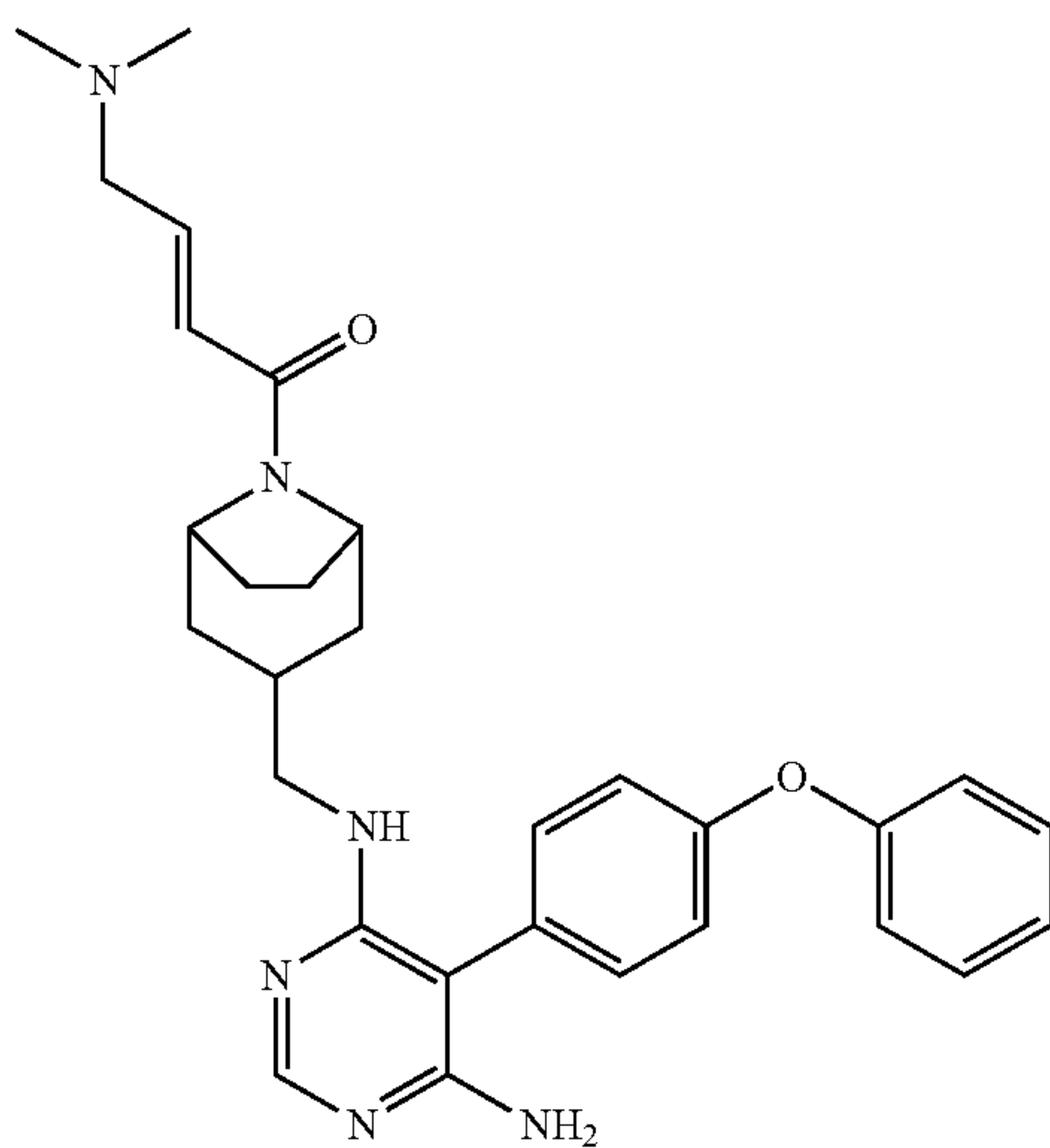
(E)-1-(3-(((6-amino-5-(4-phenoxyphenyl)pyrimidin-4-yl)amino)methyl)-8-azabicyclo[3.2.1]octan-8-yl)-4-(dimethylamino)but-2-en-1-one (A71)
