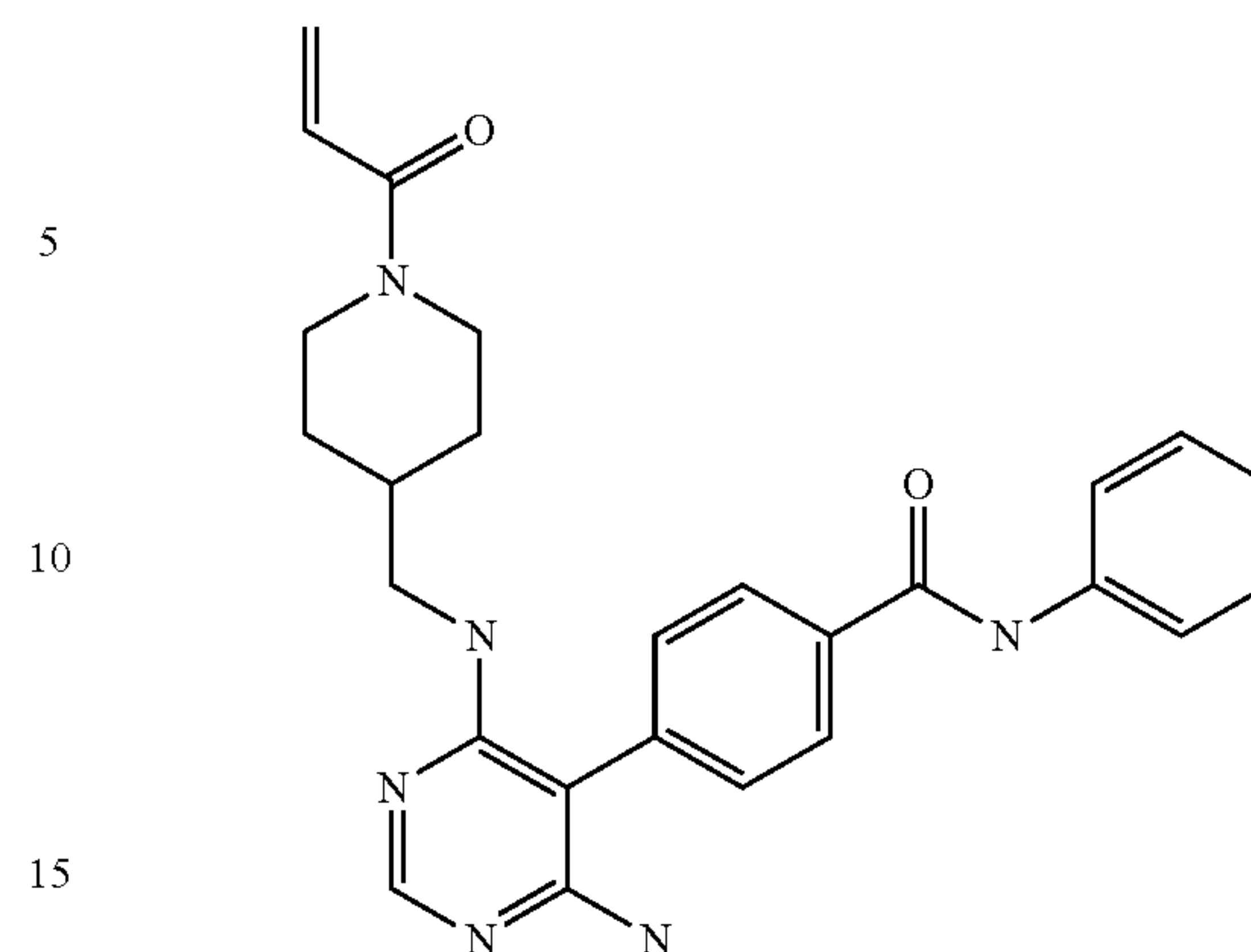
4-(4-(((1-acryloylpiperidin-4-yl)methyl)amino)-6-aminopyrimidin-5-yl)-N-phenylbenzamide (A157)
