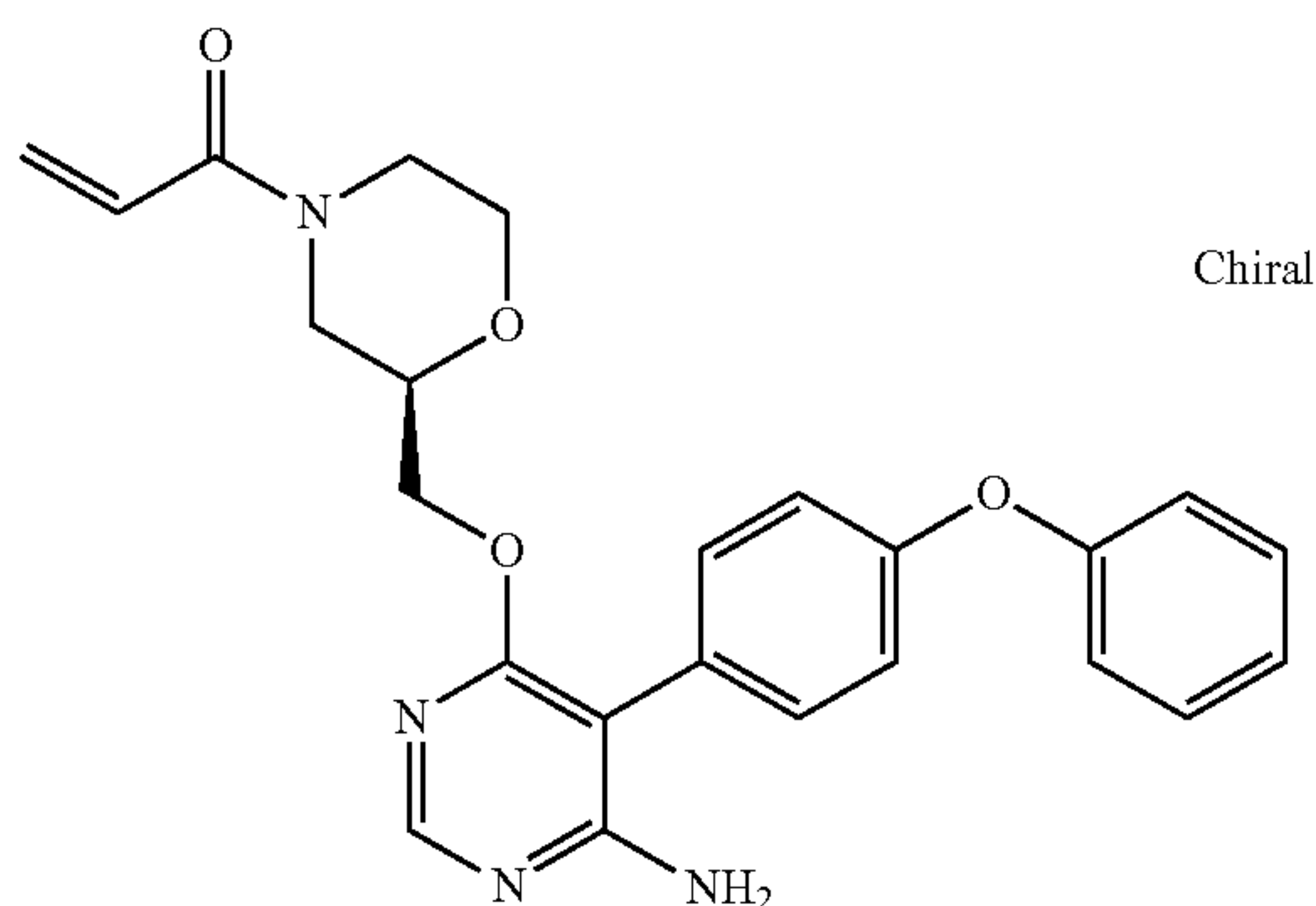
(R)-1-(2-(((6-amino-5-(4-phenoxyphenyl)pyrimidin-4-yl)oxy)methyl)morpholino)prop-2-en-1-one (A66)
