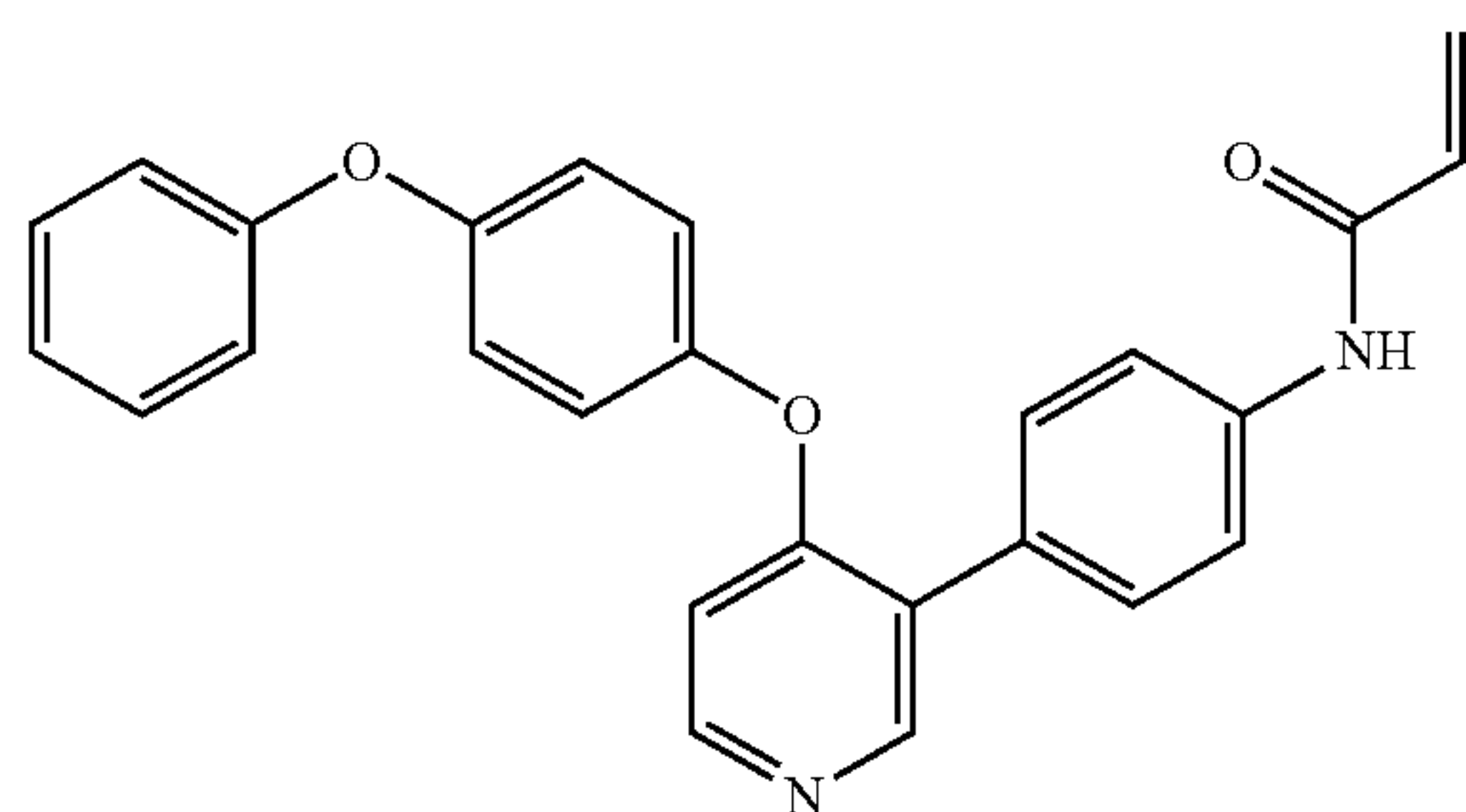
N-(4-(4-(4-phenoxyphenoxy)pyridin-3-yl)phenyl)acrylamide (A281)
