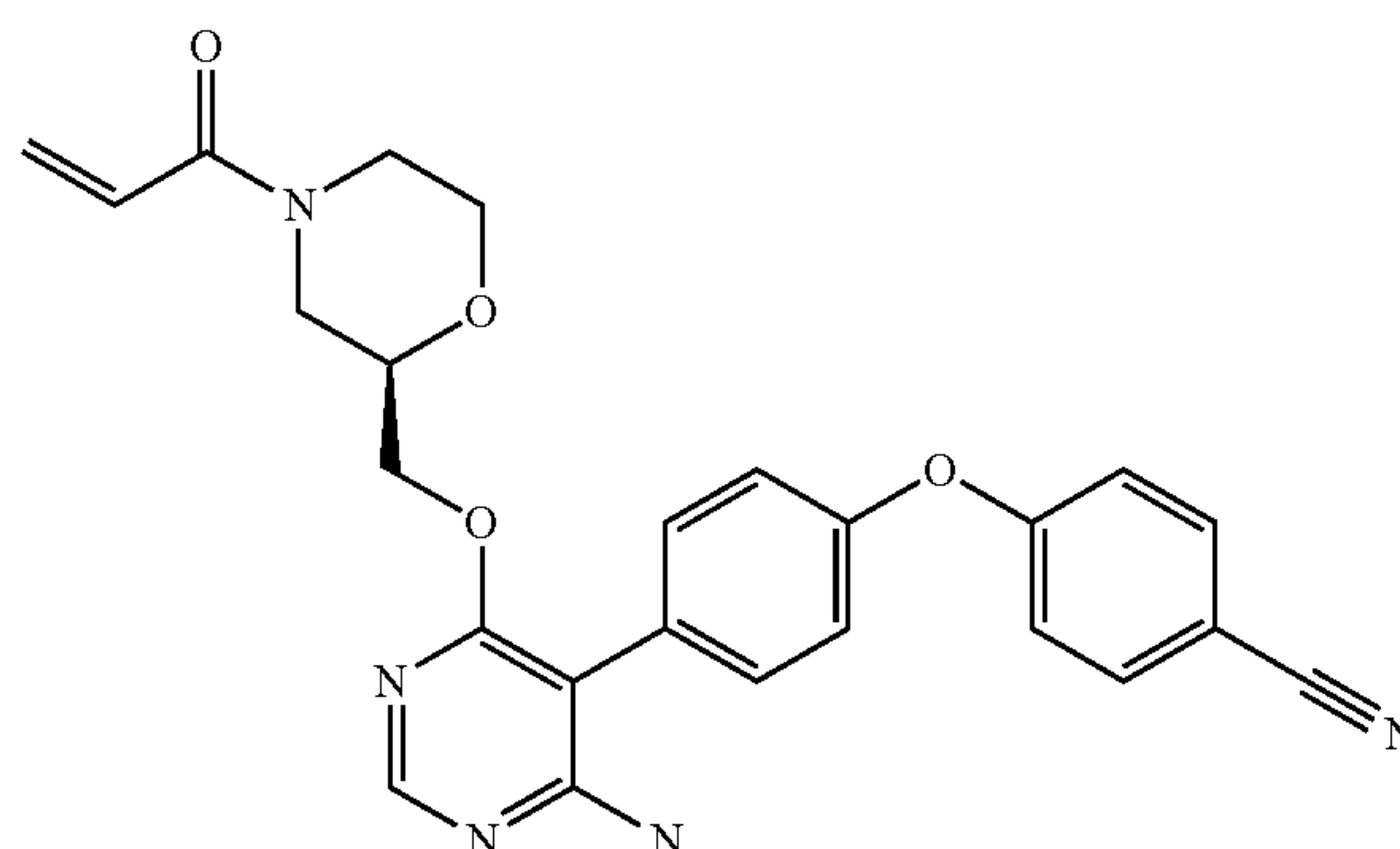
(R)-4-(4-(4-((4-acryloylmorpholin-2-yl)methoxy)-6-aminopyrimidin-5-yl)phenoxy)benzonitrile (A200)
