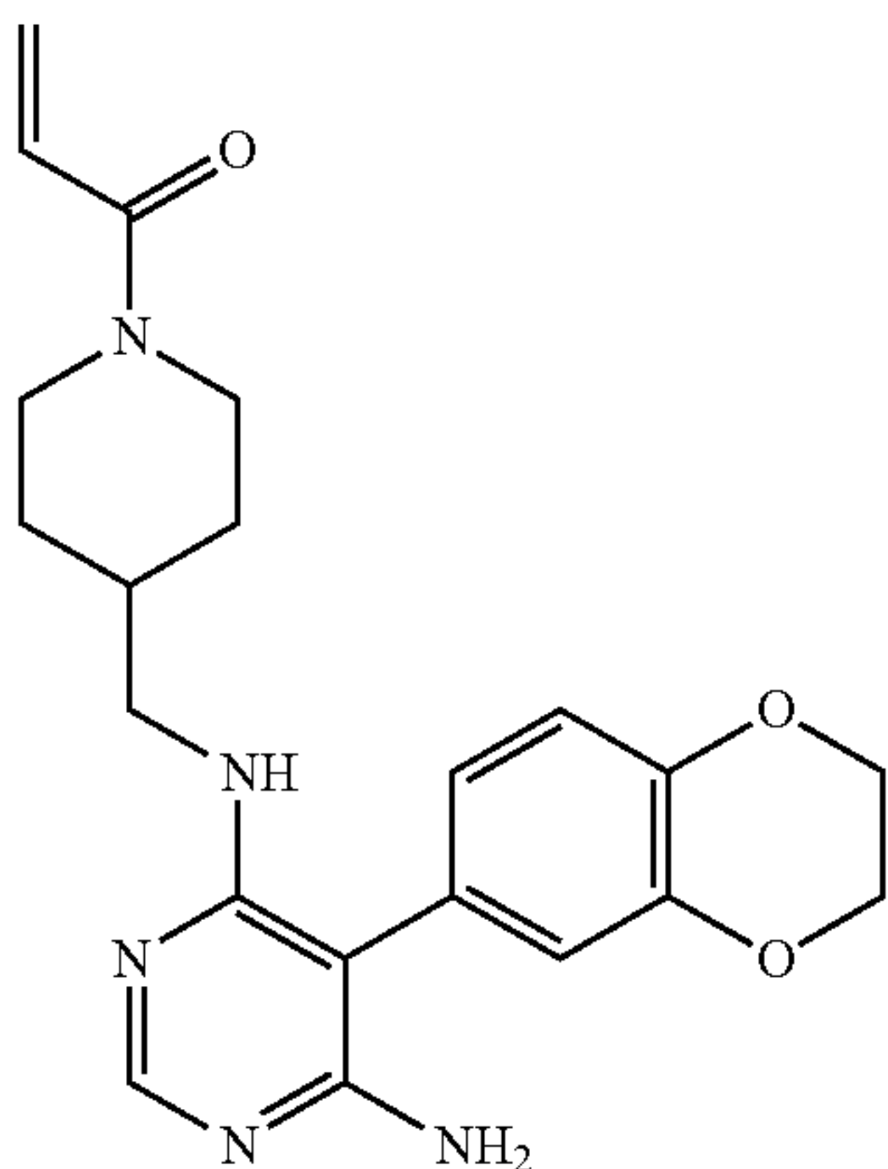
1-(4-(((6-amino-5-(2,3-dihydrobenzo[b][1,4]dioxin-6-yl)pyrimidin-4-yl)amino)methyl)piperidin-1-yl)prop-2-en-1-one (A84)
