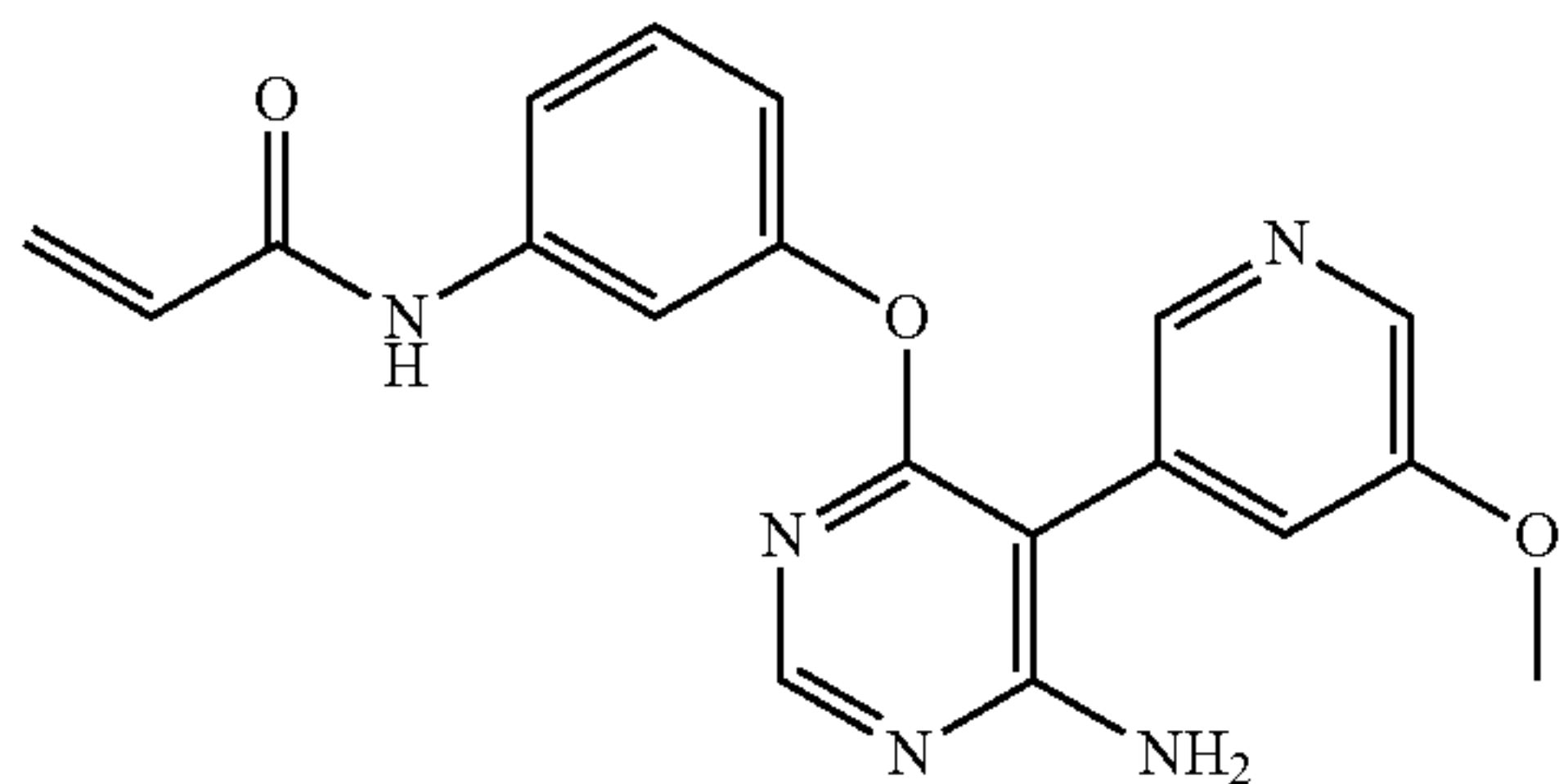
N-(3-((6-amino-5-(5-methoxypyridin-3-yl)pyrimidin-4-yl)oxy)phenyl)acrylamide (A291)
