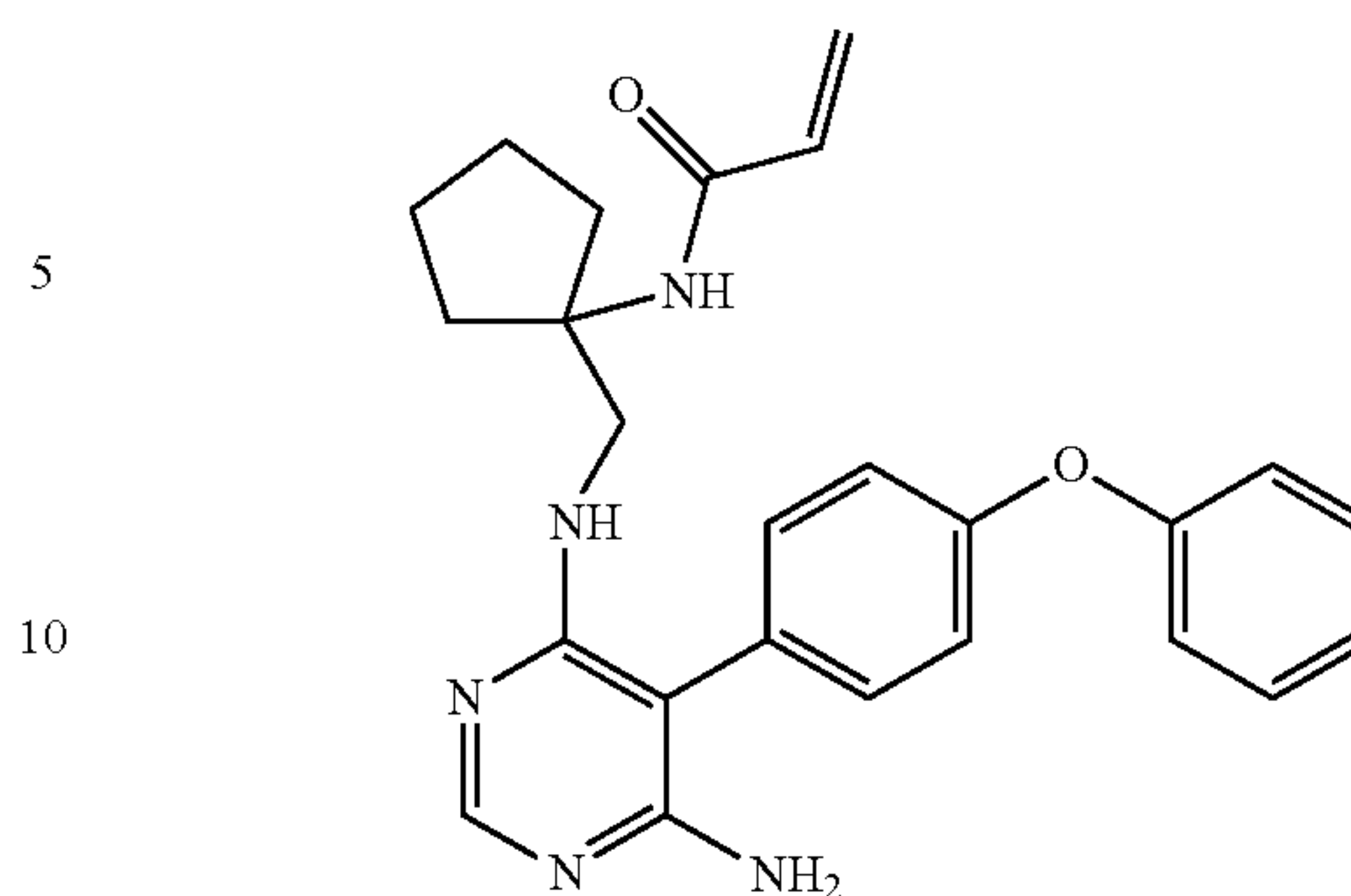
N-(1-(((6-amino-5-(4-phenoxyphenyl)pyrimidin-4-yl)amino)methyl)cyclopentyl)acrylamide (A20)
