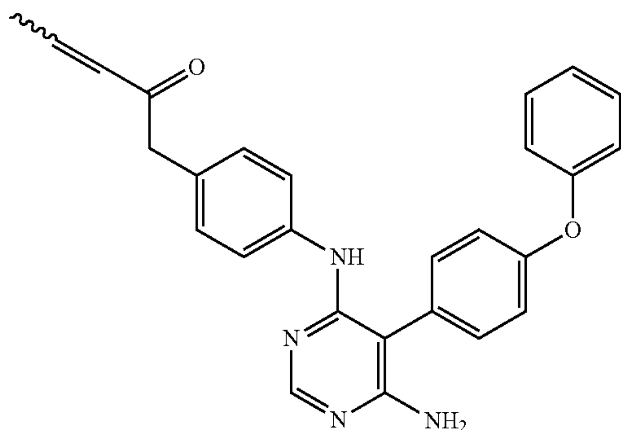
1-(4-(6-Amino-5-(4-phenoxyphenyl)-pyrimidin-4-ylamino)-phenyl)-pent-3-en-2-one
