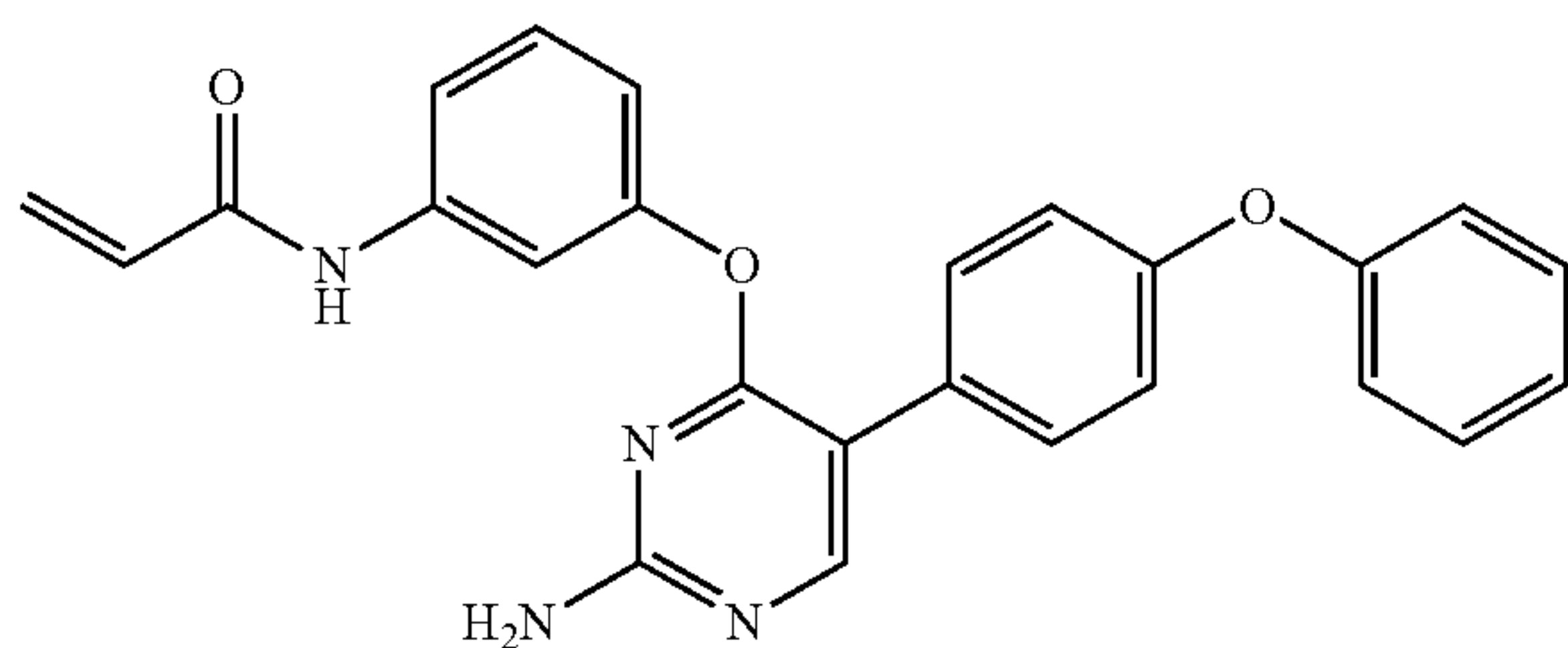
N-(3-((2-amino-5-(4-phenoxyphenyl)pyrimidin-4-yl)oxy)phenyl)acrylamide (A271)
