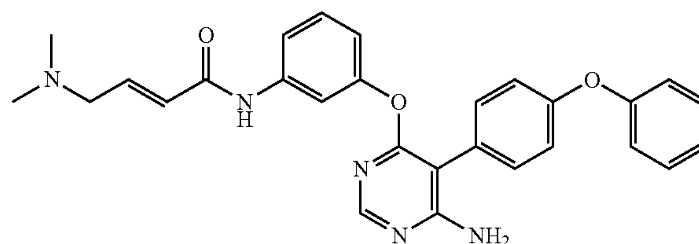
(E)-N-(3-(((6-amino-5-(4-phenoxyphenyl)pyrimidin-4-yl)oxy)phenyl)-4-(dimethylamino)but-2-enamide (A252)
