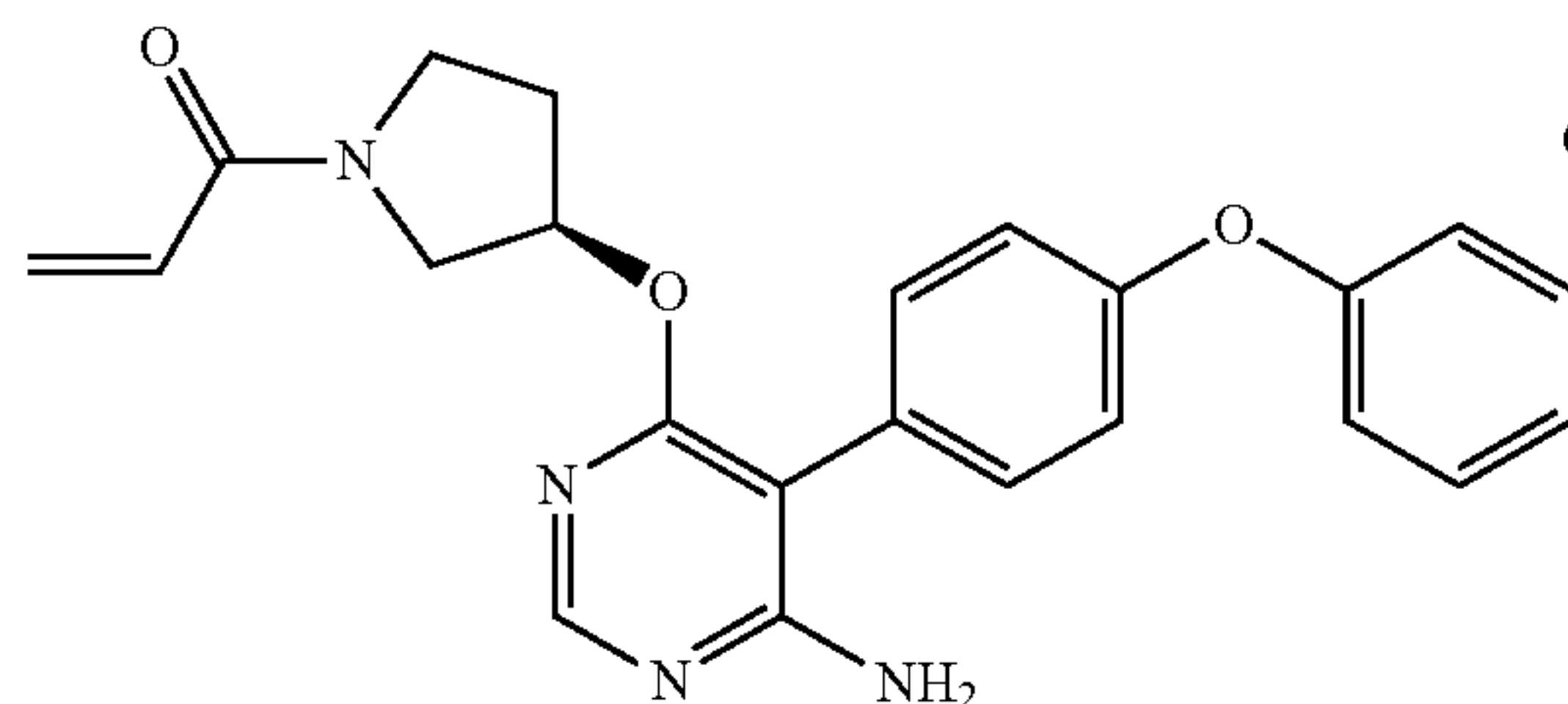
(R)-1-(3-(((6-amino-5-(4-phenoxyphenyl)pyrimidin-4-yl)oxy)pyrrolidin-1-yl)prop-2-en-1-one (A19)
