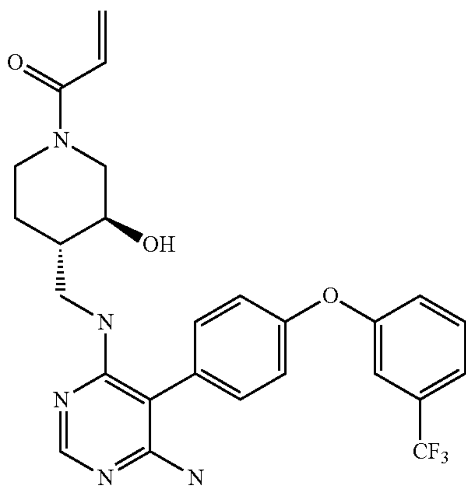
1-((3S,4S)-4-(((6-amino-5-(4-(3-(trifluoromethyl)phenoxy)phenyl)pyrimidin-4-yl)amino)methyl)-3-hydroxypiperidin-1-yl)prop-2-en-1-one (A170)
