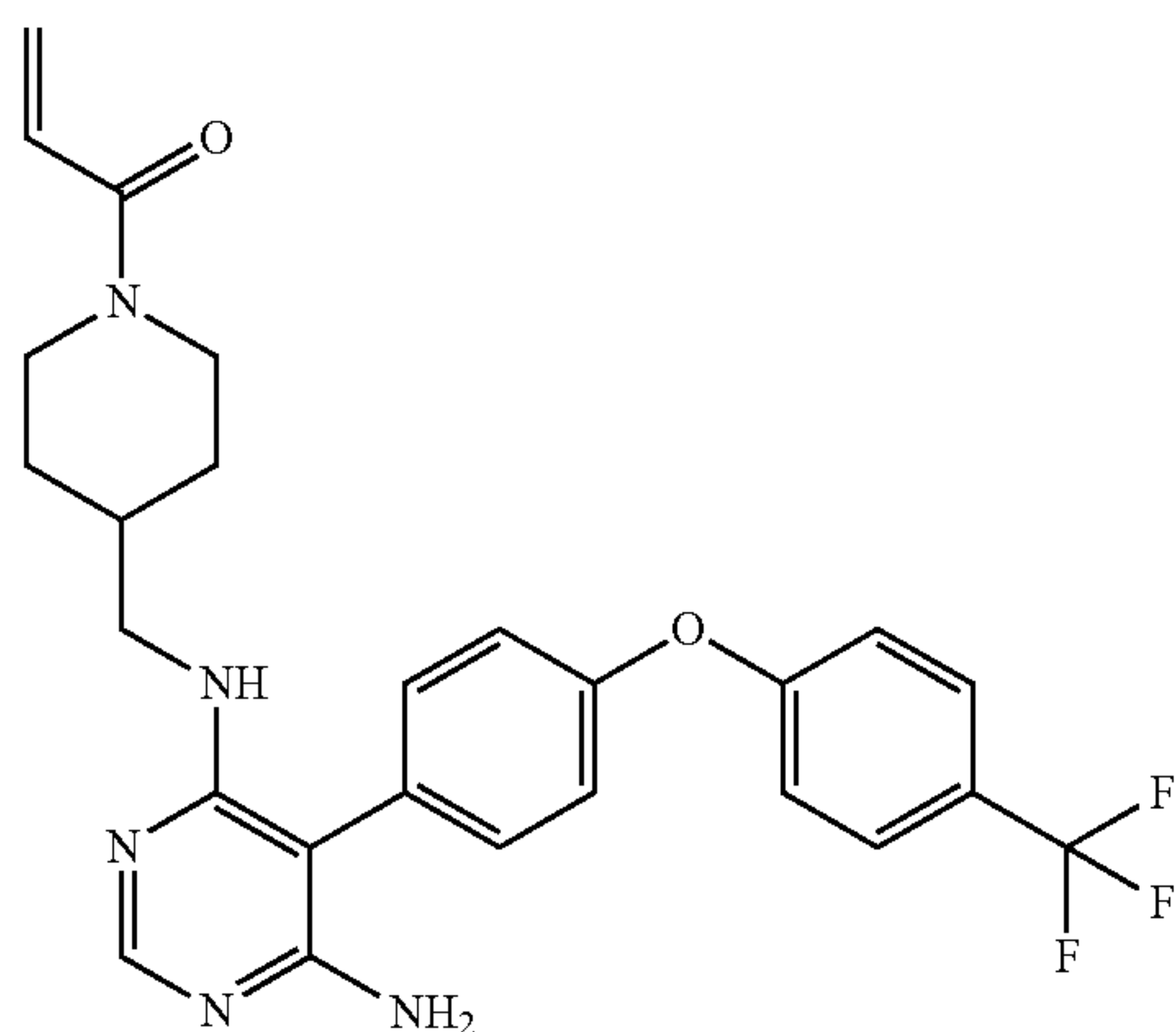
1-(4-(((6-amino-5-(4-(4-(trifluoromethyl)phenoxy)phenyl)pyrimidin-4-yl)amino)methyl)piperidin-1-yl)prop-2-en-1-one (A79)
