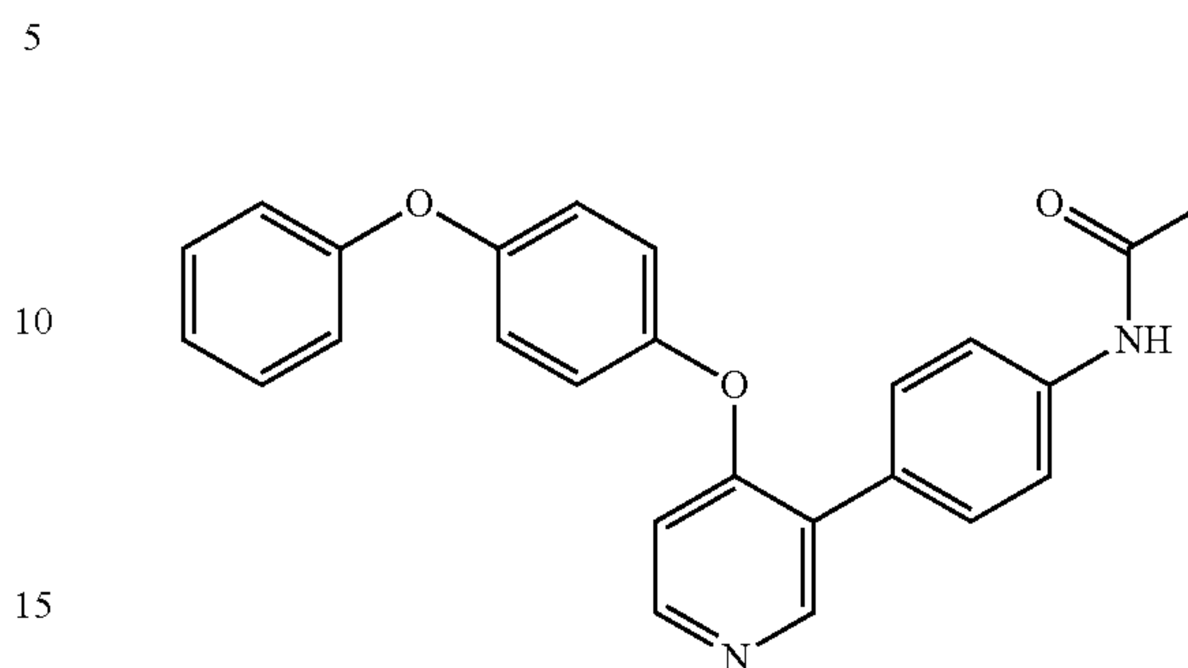
N-(4-(4-(4-phenoxyphenoxy)pyridin-3-yl)phenyl)propionamide (A320)
