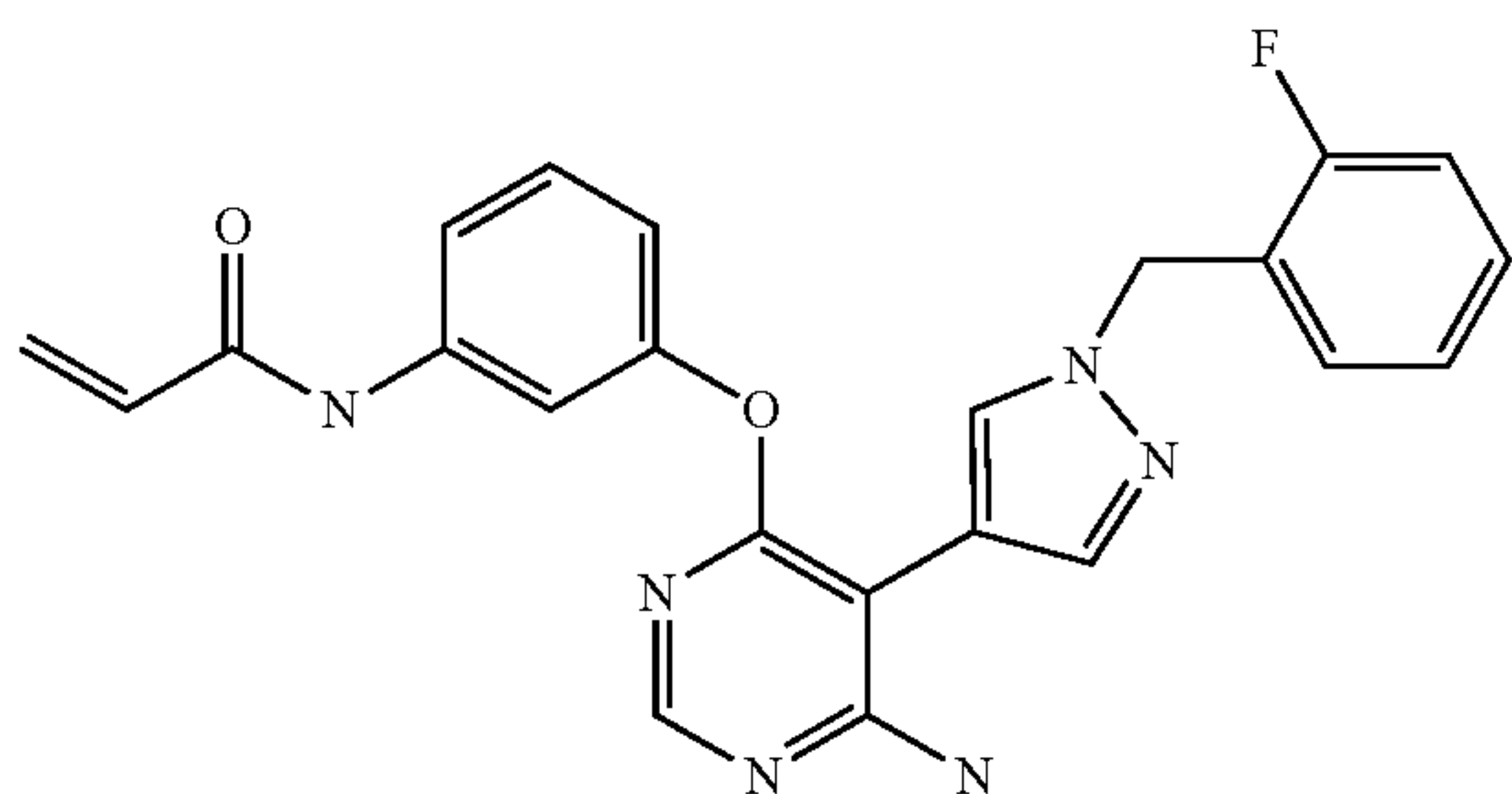
N-(3-((6-amino-5-(1-(2-fluorobenzyl)-1H-pyrazol-4-yl)pyrimidin-4-yl)oxy)phenyl)acrylamide (A184)
