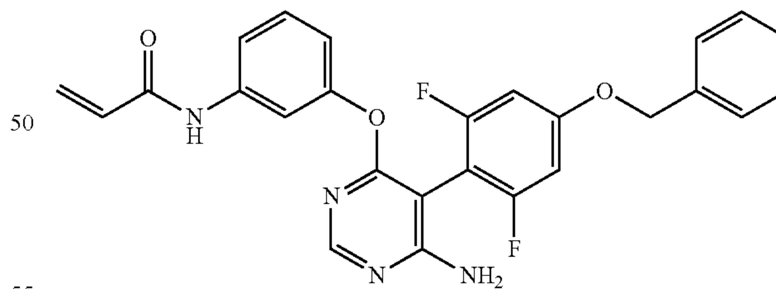
N-(3-((6-amino-5-(4-(benzyloxy)-2,6-difluorophenyl)pyrimidin-4-yl)oxy)phenyl)acrylamide (A294)
