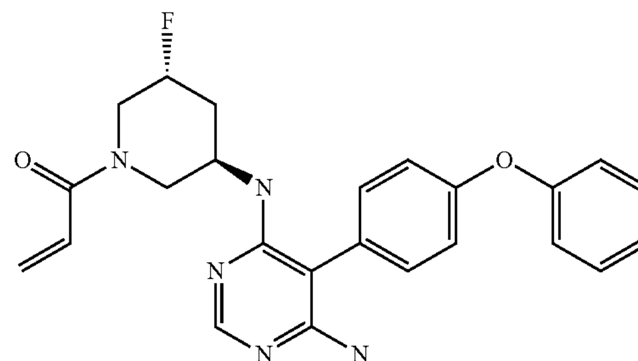
1-((3R,5R)-3-((6-amino-5-(4-phenoxyphenyl)pyrimidin-4-yl)amino)-5-fluoropiperidin-1-yl)prop-2-en-1-one (A205)
