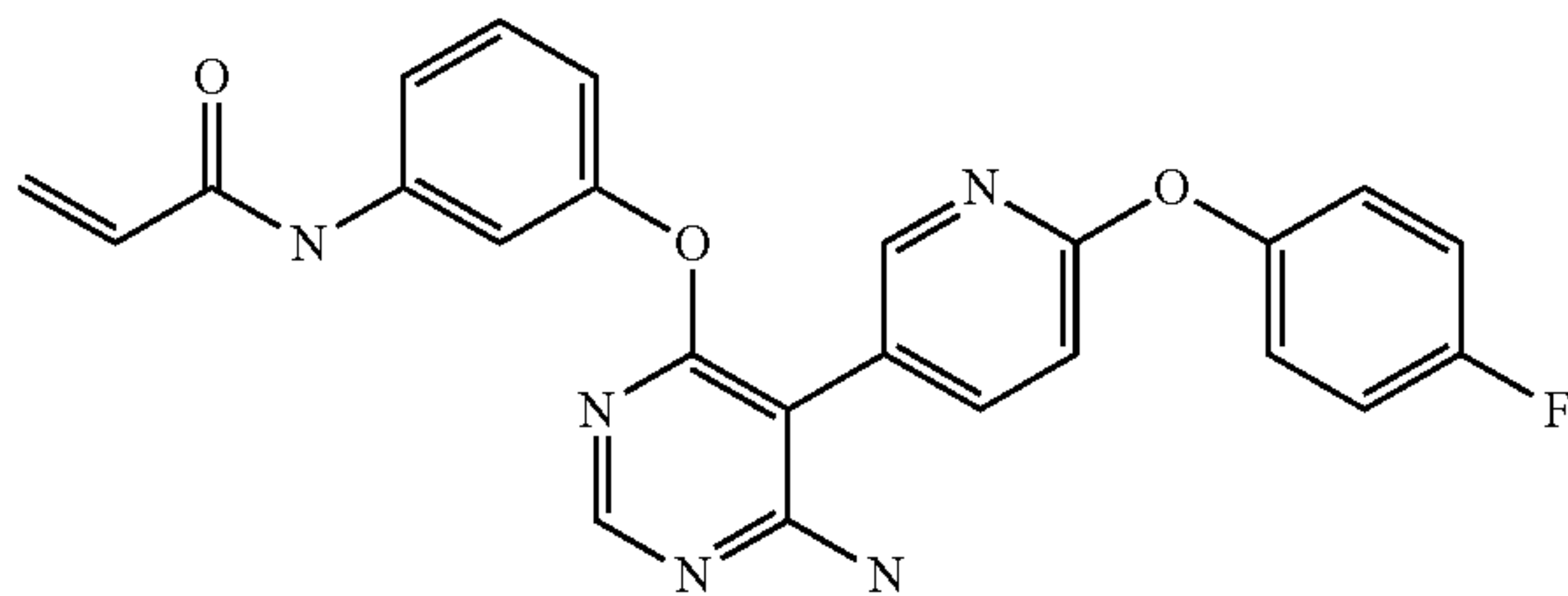
N-(3-((6-amino-5-(6-(4-fluorophenoxy)pyridin-3-yl)pyrimidin-4-yl)oxy)phenyl)acrylamide (A166)
