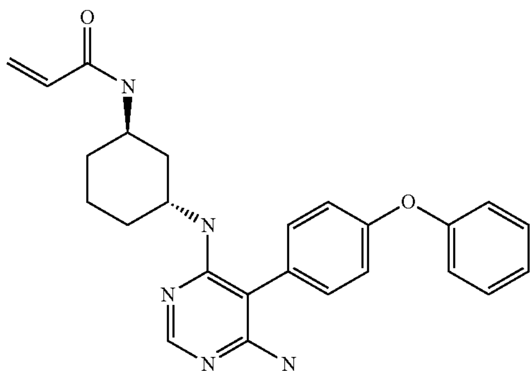
N-((1R,3R)-3-((6-amino-5-(4-phenoxyphenyl)pyrimidin-4-yl)amino)cyclohexyl)acrylamide (A175)
