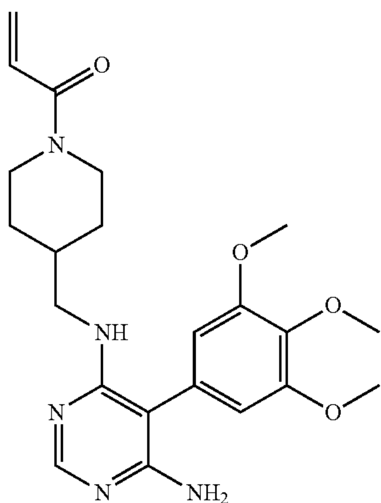
1-(4-(((6-amino-5-(3,4,5-trimethoxyphenyl)pyrimidin-4-yl)amino)methyl)piperidin-1-yl)prop-2-en-1-one (A83)
