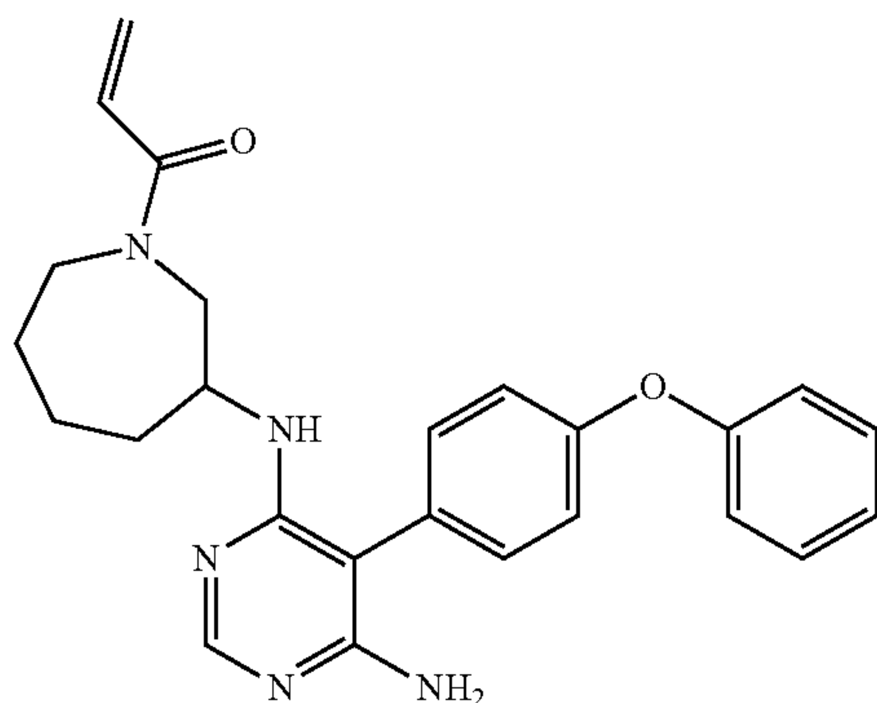
1-(3-((6-amino-5-(4-phenoxyphenyl)pyrimidin-4-yl)amino)azepan-1-yl)prop-2-en-1-one (A52)
