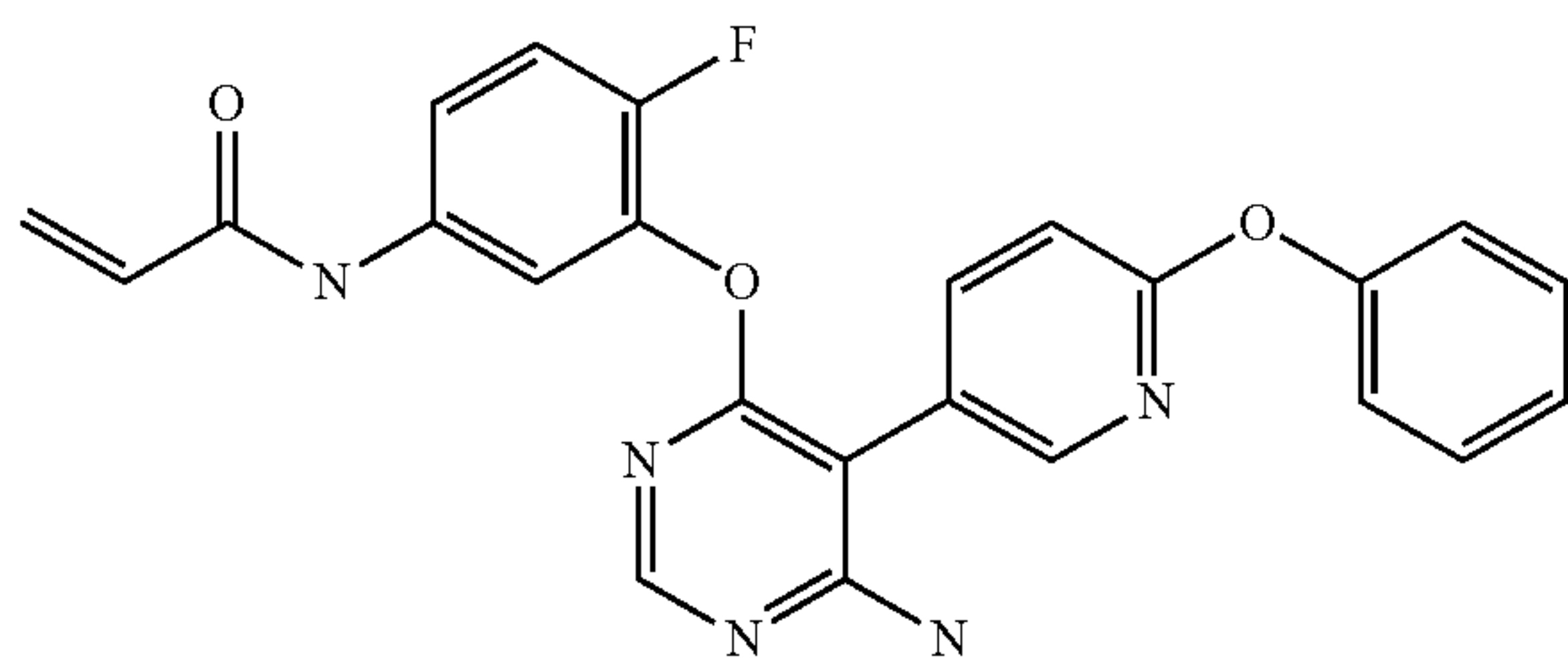
N-(3-((6-amino-5-(6-phenoxy-3-fluoropyridin-3-yl)pyrimidin-4-yl)oxy)-4-fluorophenyl)acrylamide (A161)
