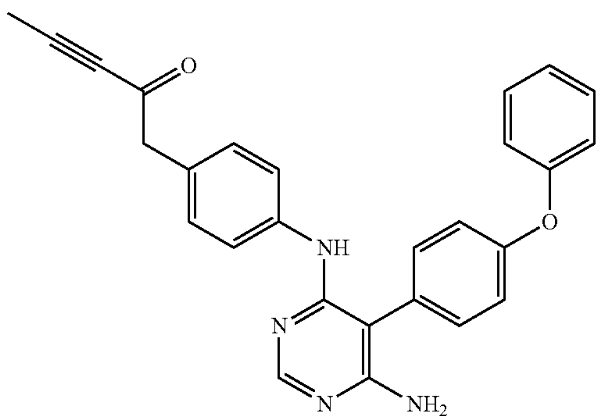
1-(4-(6-Amino-5-(4-phenoxyphenyl)-pyrimidin-4-ylamino)-phenyl)-pent-3-yn-2-one
