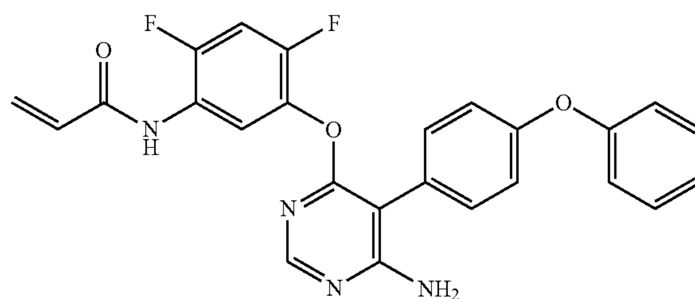
N-(5-(((6-amino-5-(4-phenoxyphenyl)pyrimidin-4-yl)oxy)-2,4-difluorophenyl)acrylamide (A251)
