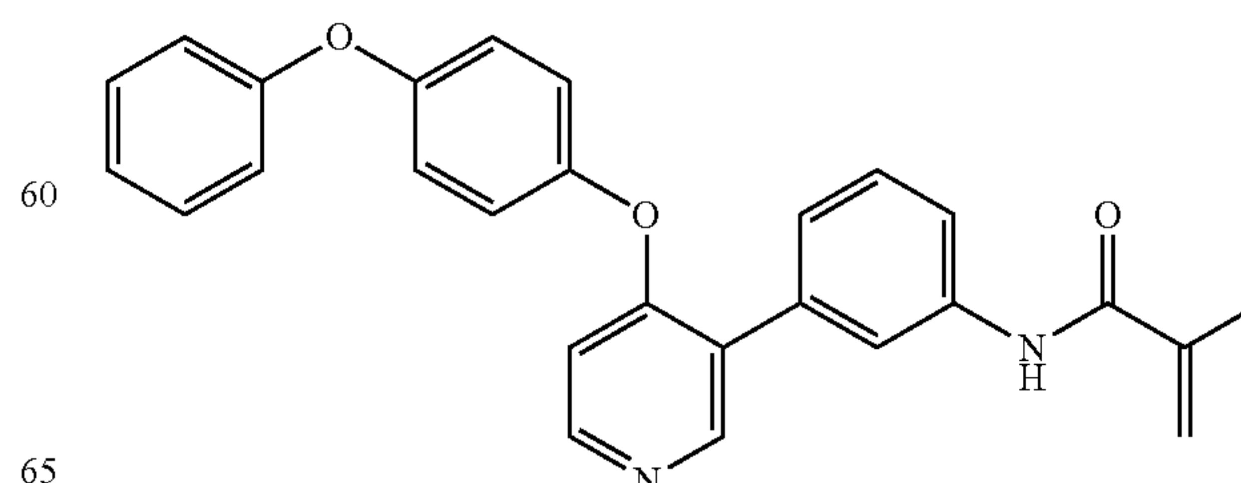
N-(3-(4-(4-phenoxyphenoxy)pyridin-3-yl)phenyl)propionamide (A319)
