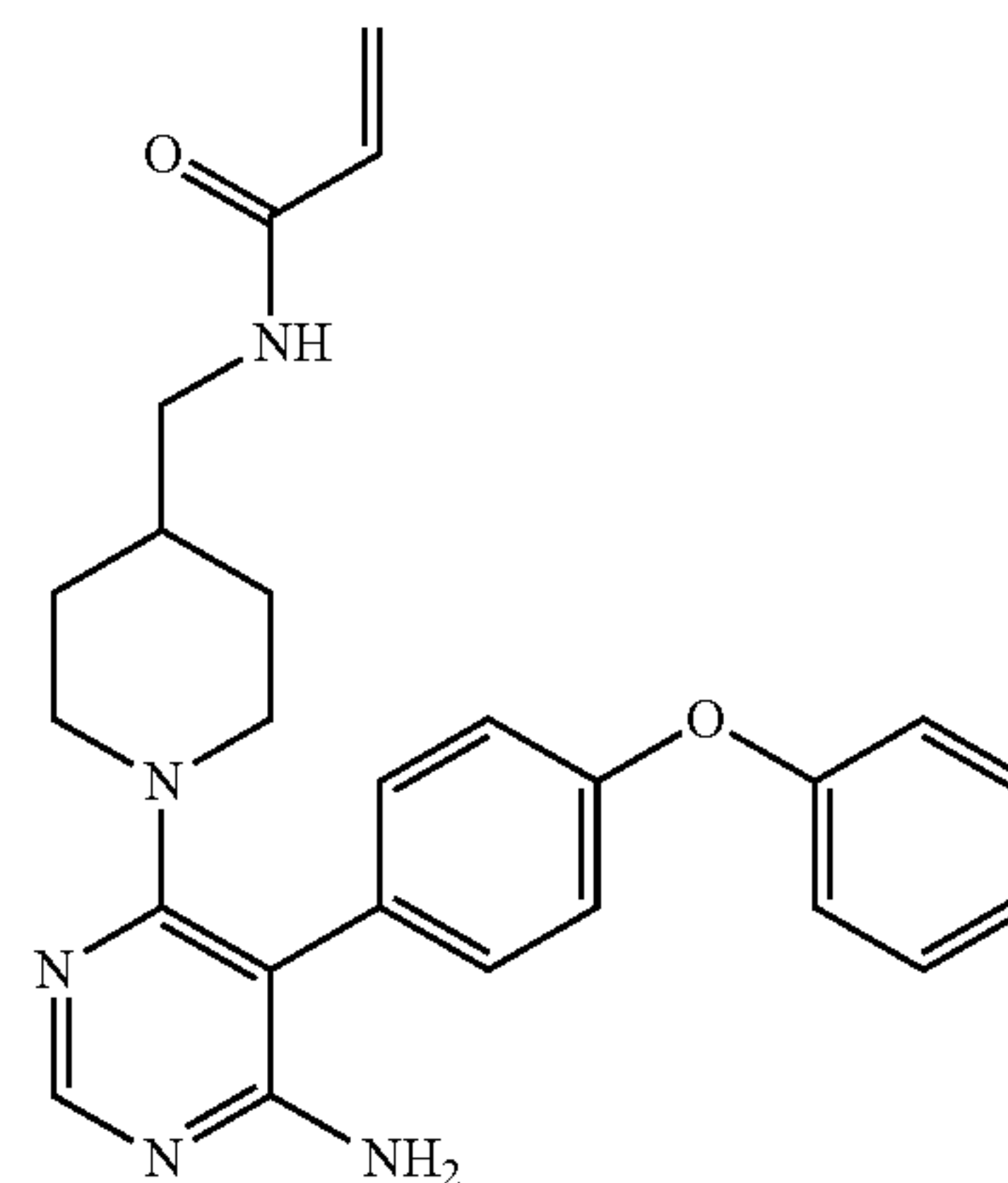
N-((1-(6-amino-5-(4-phenoxyphenyl)pyrimidin-4-yl)piperidin-4-yl)methyl)acrylamide (A7)
