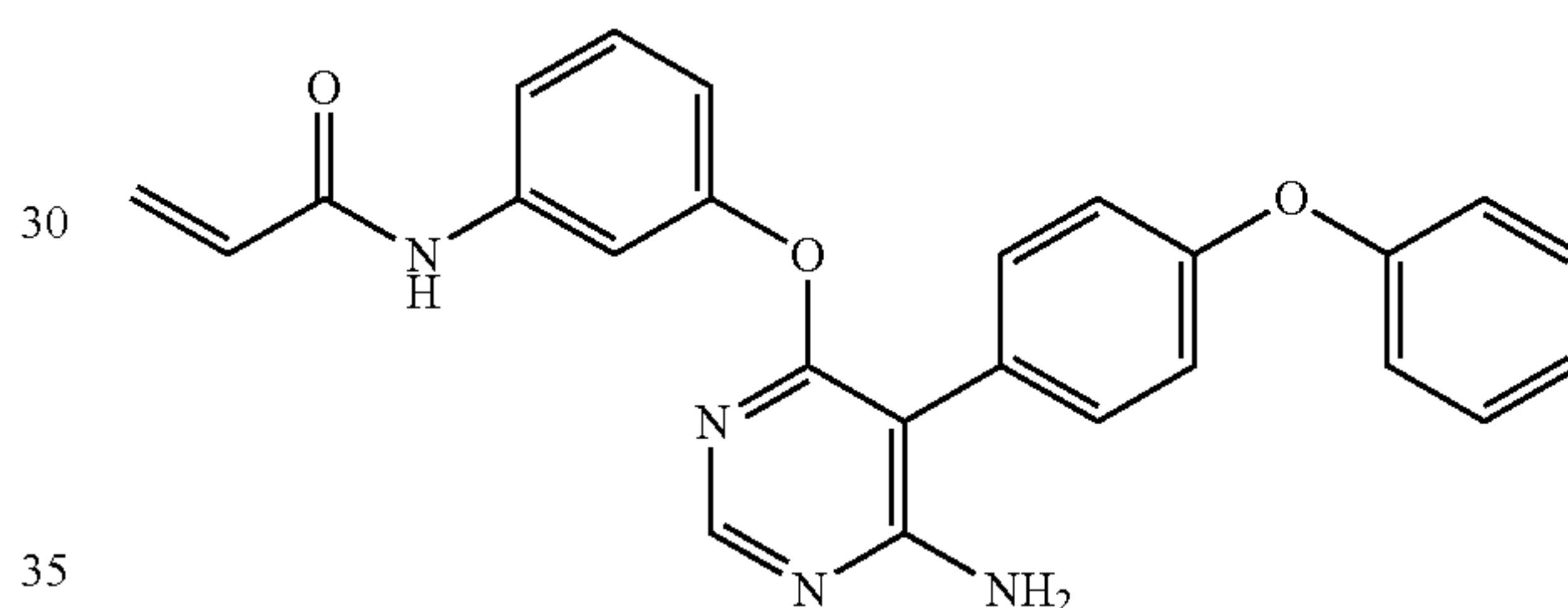
N-(3-(((6-amino-5-(4-phenoxyphenyl)pyrimidin-4-yl)oxy)phenyl)acrylamide (A242)
