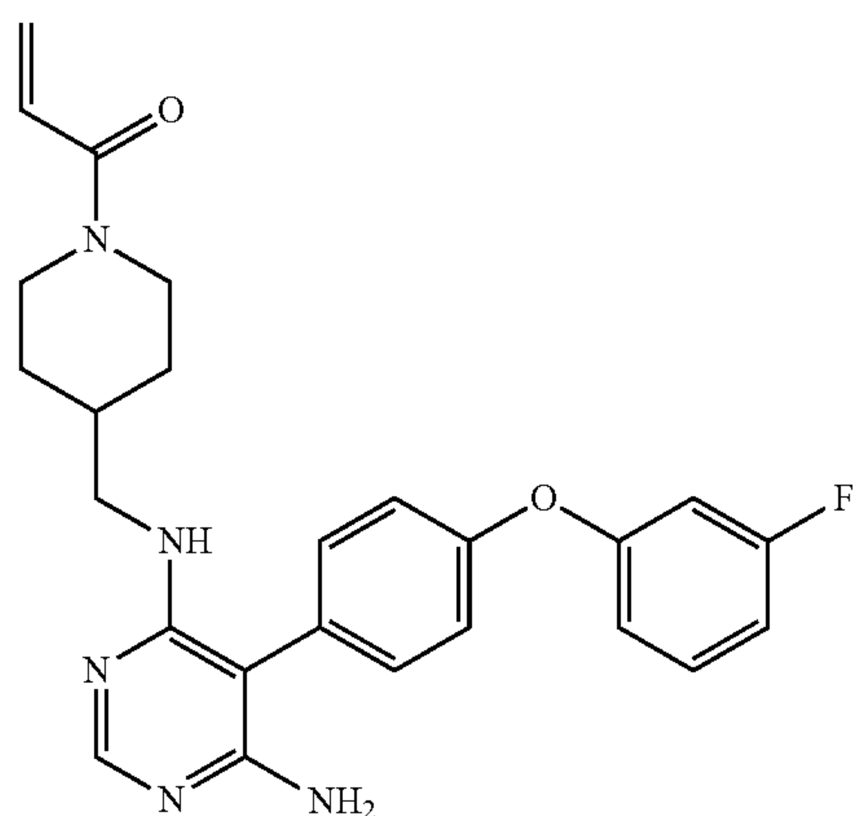
1-(4-(((6-amino-5-(4-(3-fluorophenoxy)phenyl)pyrimidin-4-yl)amino)methyl)piperidin-1-yl)prop-2-en-1-one (A34)
