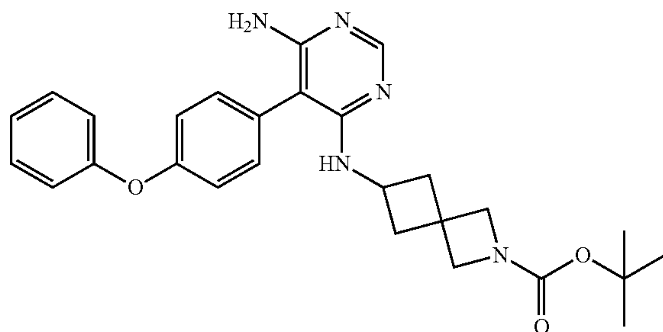
tert-butyl 6-((6-amino-5-(4-phenoxyphenyl)pyrimidin-4-yl)amino)-2-azaspiro[3.3]heptane-2-carboxylate
