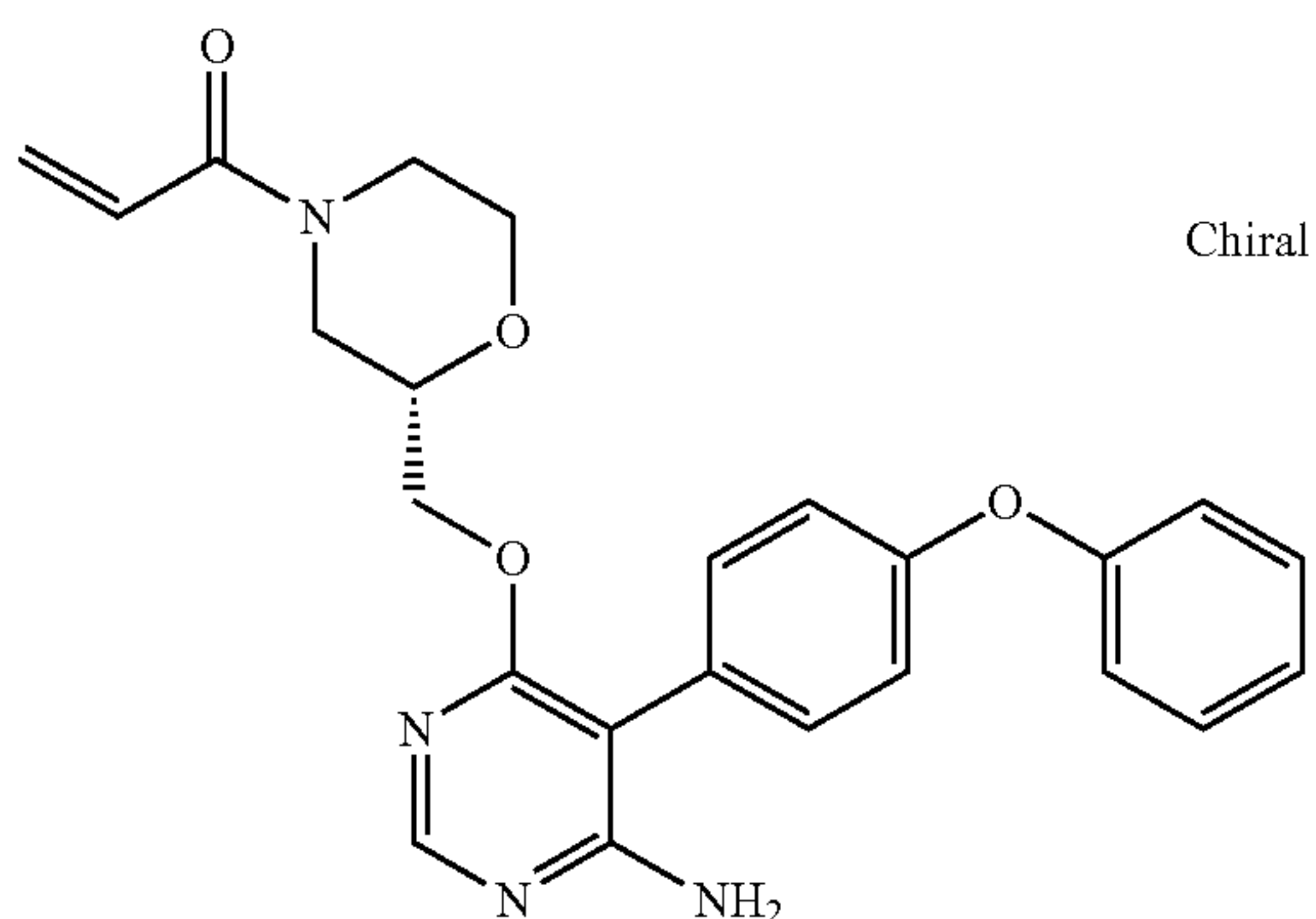
(S)-1-(2-(((6-amino-5-(4-phenoxyphenyl)pyrimidin-4-yl)oxy)methyl)morpholino)prop-2-en-1-one (A65)
