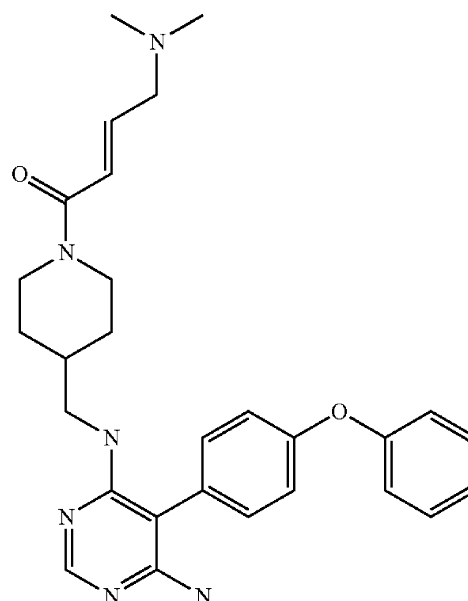
(E)-1-(4-(((6-amino-5-(4-phenoxyphenyl)pyrimidin-4-yl)amino)methyl)piperidin-1-yl)-4-(dimethylamino)but-2-en-1-one (A153)
