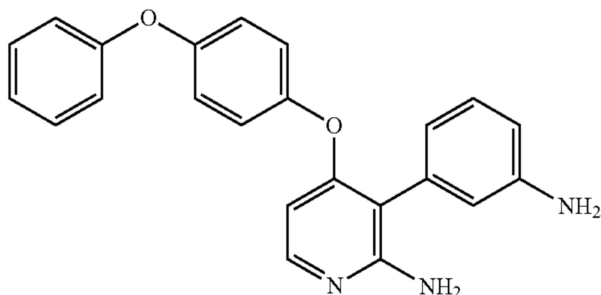
3-(3-aminophenyl)-4-(4-phenoxyphenoxy)pyridin-2-amine (A300)
