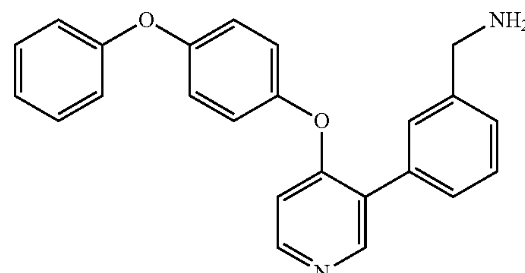
(3-(4-(4-phenoxyphenoxy)pyridin-3-yl)phenyl)methanamine (A316)
