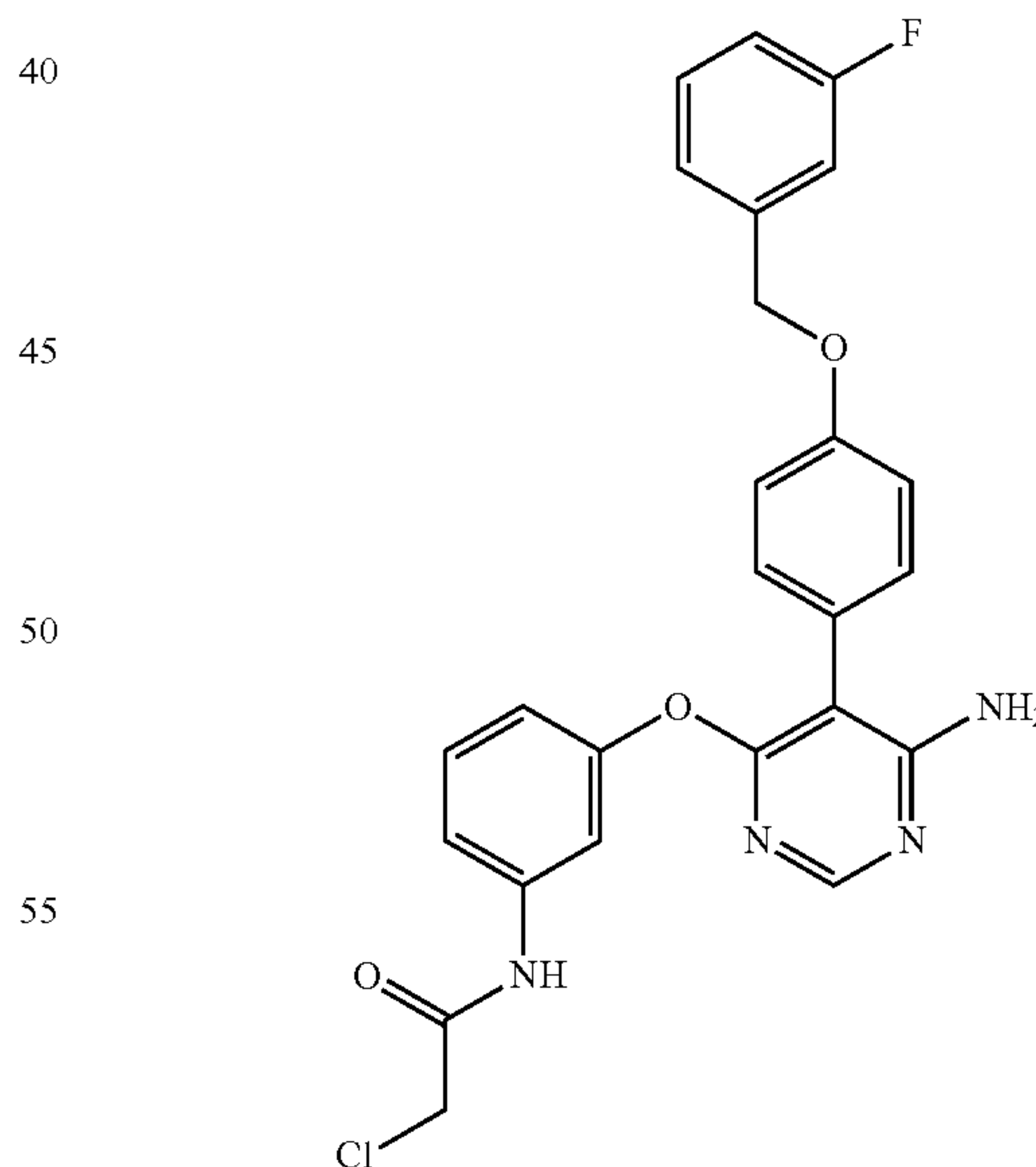
N-(3-{6-Amino-5-[4-(3-fluoro-benzyloxy)-phenyl]-pyrimidin-4-yloxy}-phenyl)-2-chloro-acetamide (A345)
