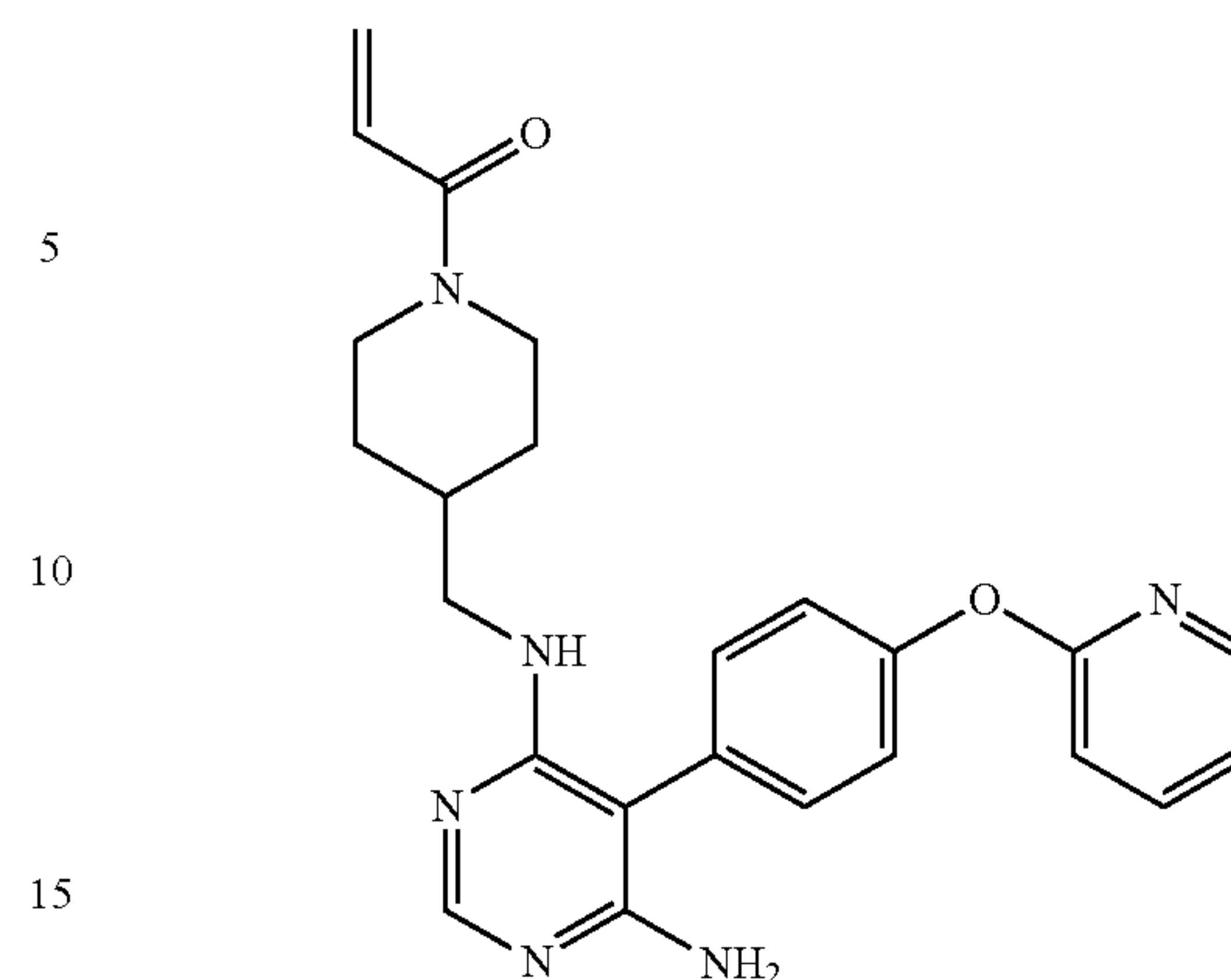
1-(4-(((6-amino-5-(4-(pyridin-2-yloxy)phenyl)pyrimidin-4-yl)amino)methyl)piperidin-1-yl)prop-2-en-1-one (A335)
