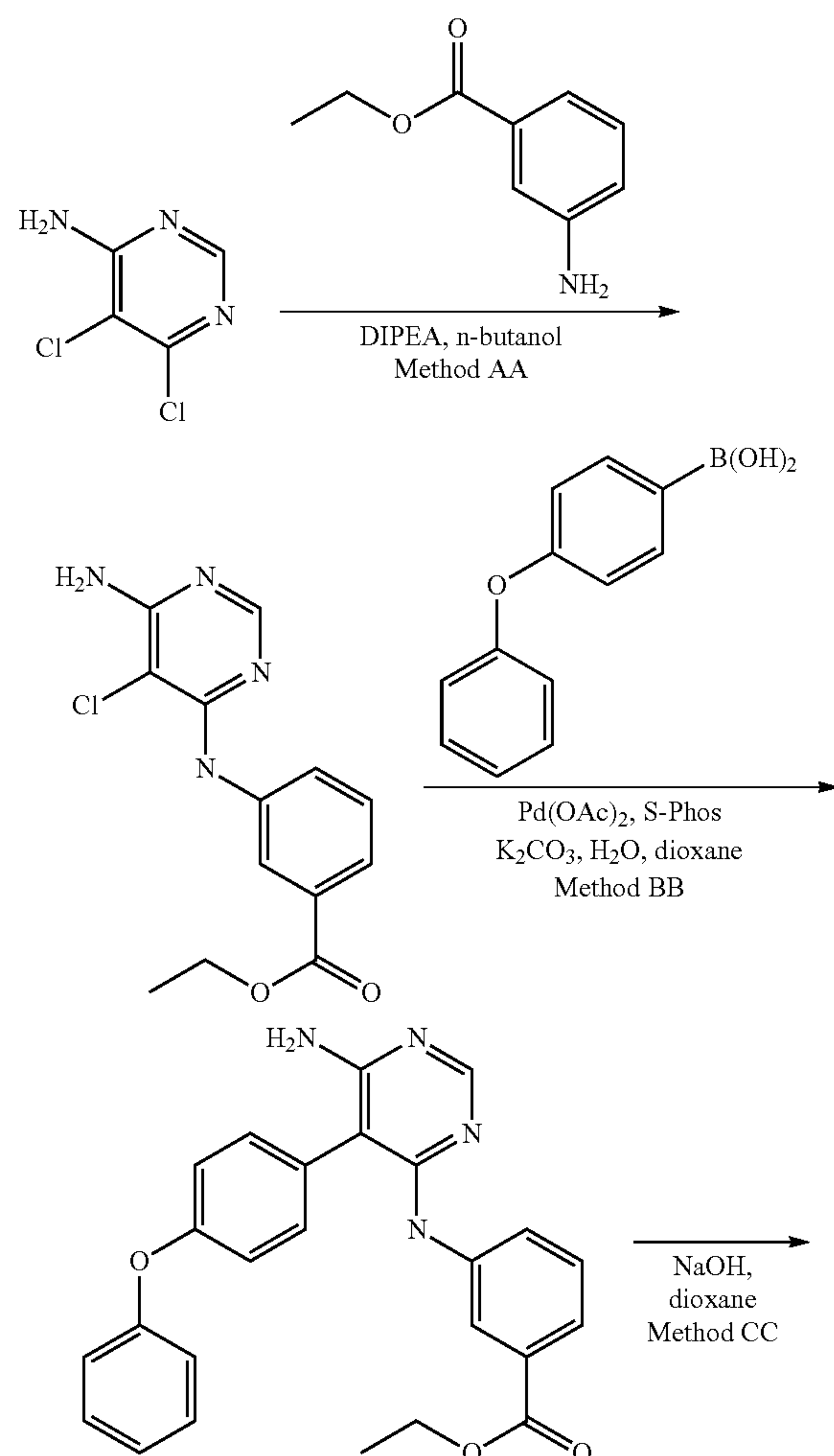
Scheme 4
