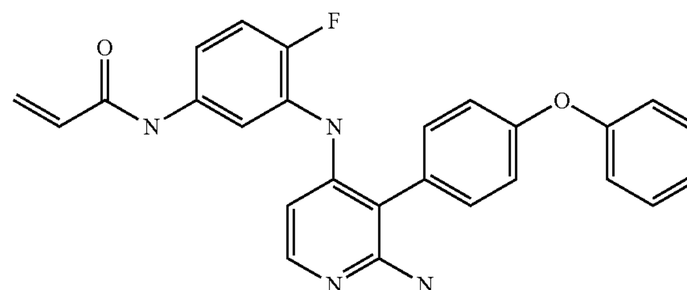
N-(3-((2-amino-3-(4-phenoxyphenyl)pyridin-4-yl)oxy)-4-fluorophenyl)acrylamide (A158)
