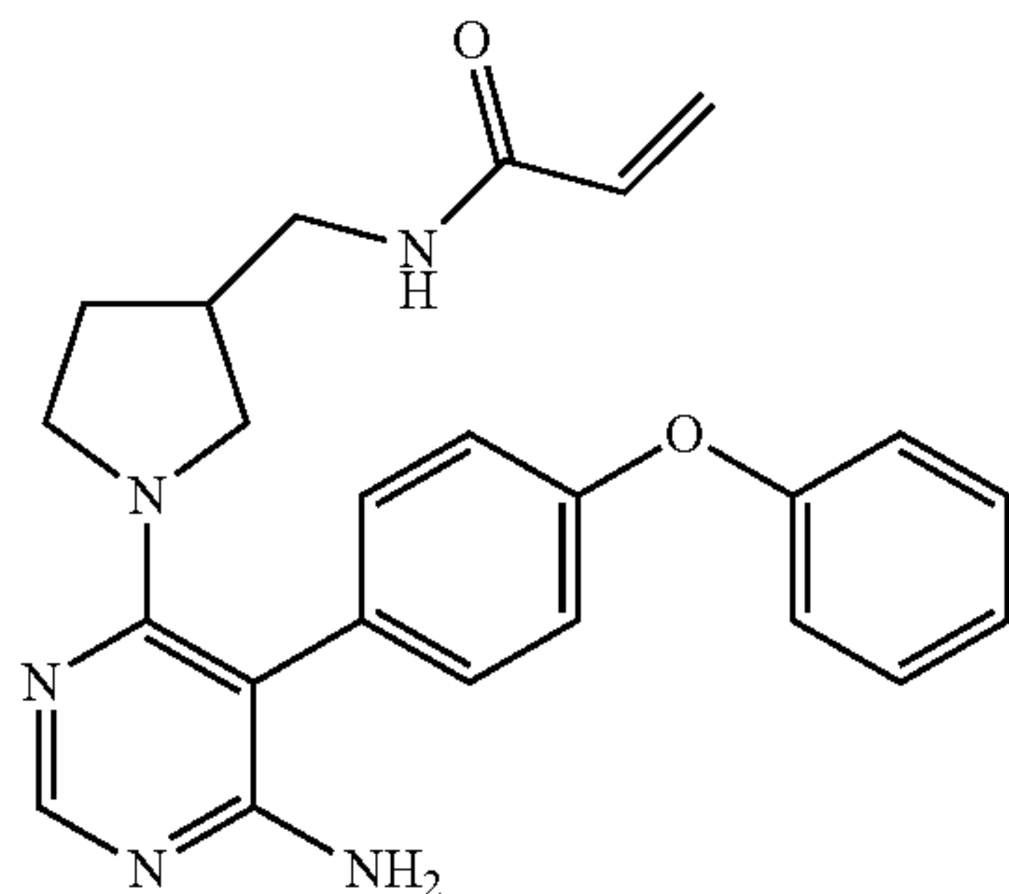
N-((1-(6-amino-5-(4-phenoxyphenyl)pyrimidin-4-yl)pyrrolidin-3-yl)methyl)acrylamide (A5)
