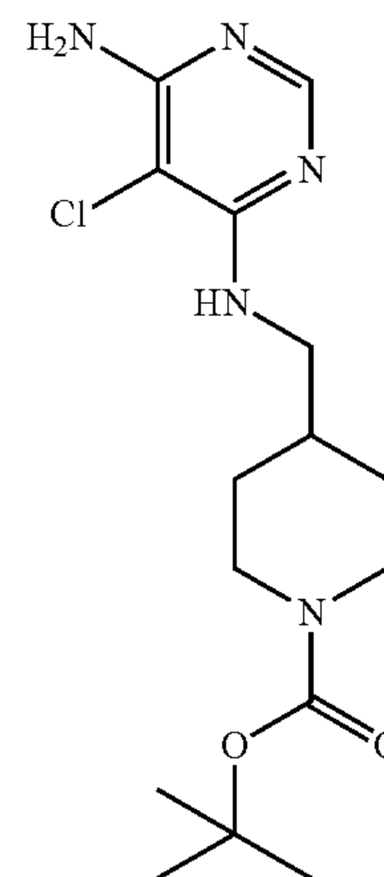
tert-butyl 4-([(6-amino-5-chloropyrimidin-4-yl)amino]methyl)piperidine-1-carboxylate
