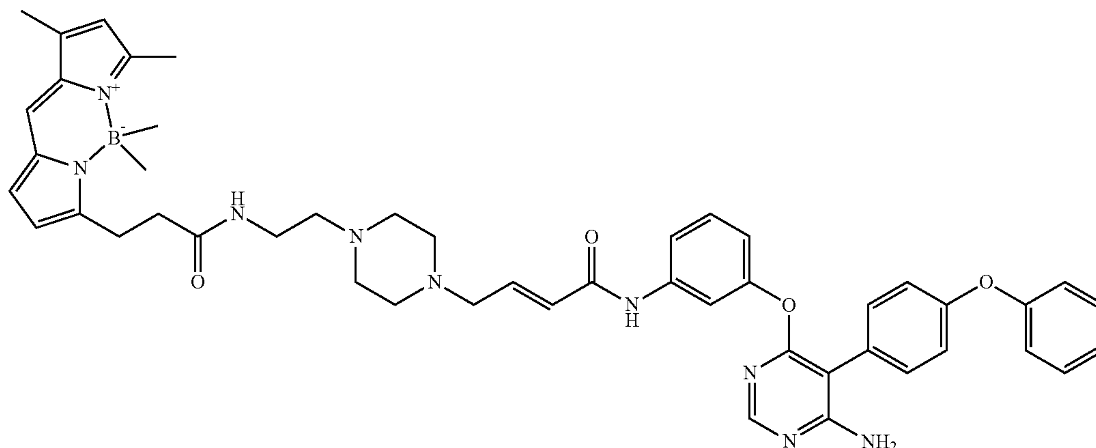
(E)-7-(3-((2-(4-(4-((3-((6-amino-5-(4-phenoxyphenyl)pyrimidin-4-yl)oxy)phenyl)amino)-4-oxobut-2-en-1-yl)piperazin-1-yl)ethyl)amino)-3-oxopropyl)-5,5-difluoro-1,3-dimethyl-5H-dipyrrolo[1,2-c:2',1'-f][1,3,2]diazaborinin-4-ium-5-uide (A35)
