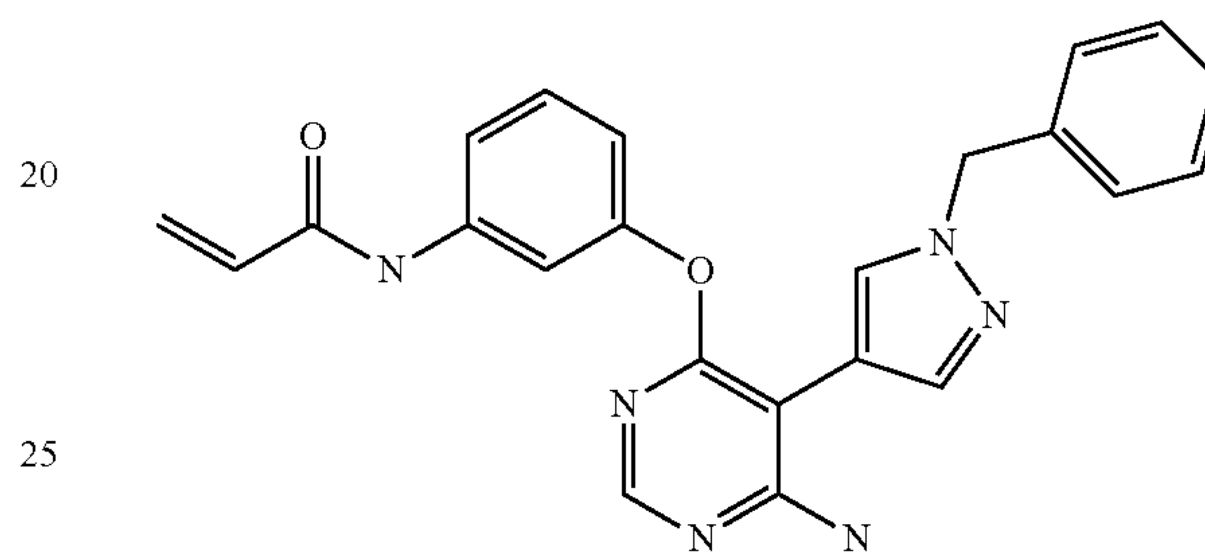
N-(3-(((6-amino-5-(1-benzyl-1H-pyrazol-4-yl)pyrimidin-4-yl)oxy)phenyl)acrylamide (A172)
