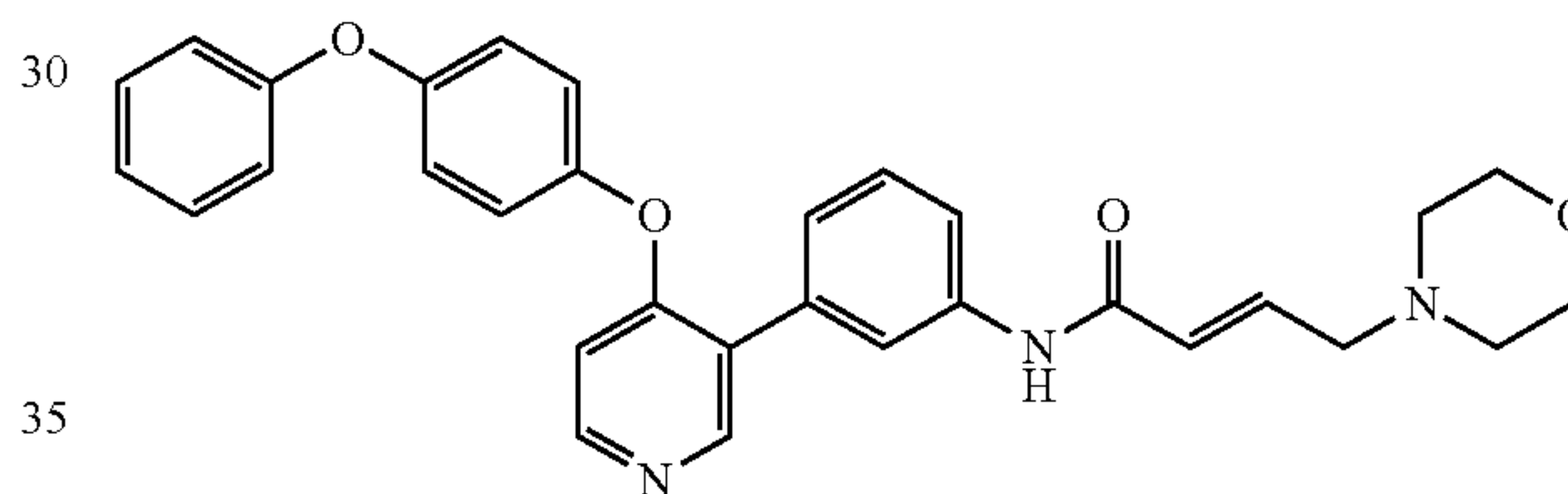
(E)-4-morpholino-N-(3-(4-(4-phenoxyphenoxy)pyridin-3-yl)phenyl)but-2-enamide (A293)
