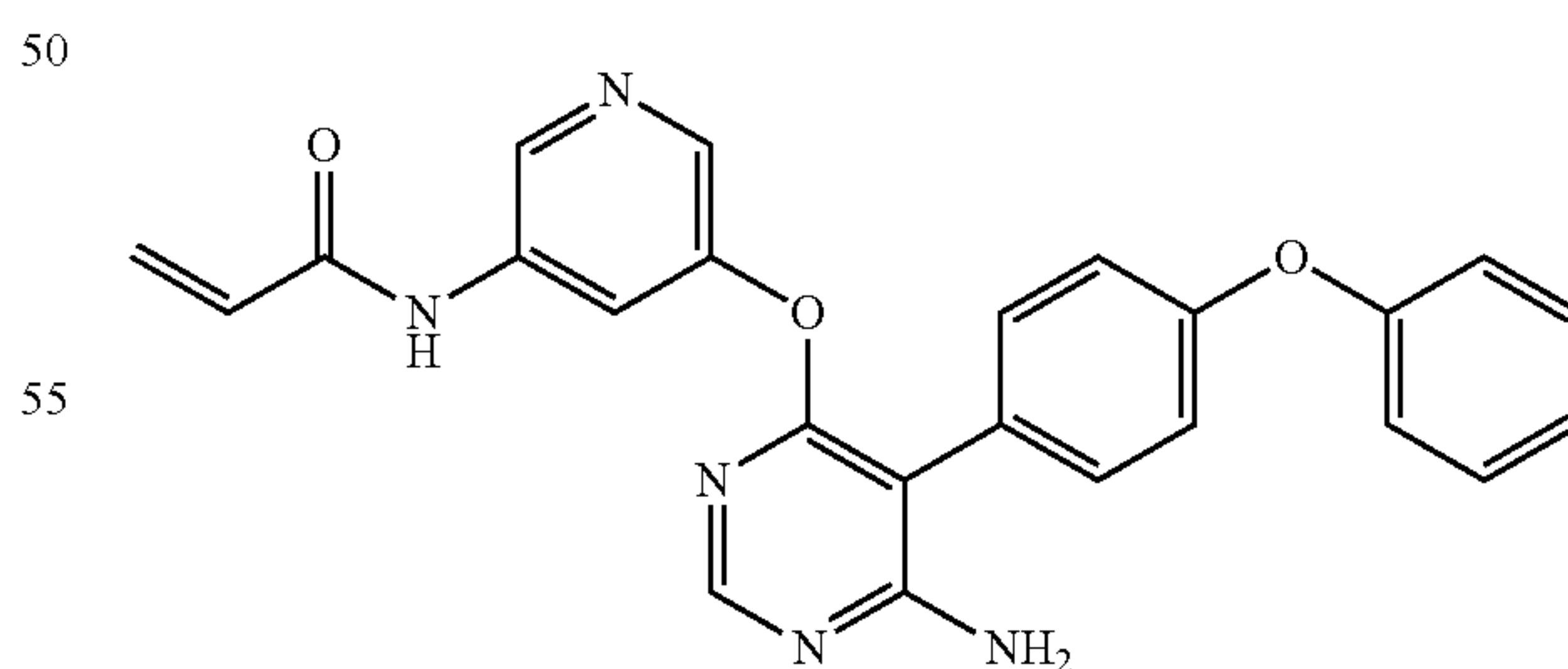
N-(5-(((6-amino-5-(4-phenoxyphenyl)pyrimidin-4-yl)oxy)pyridin-3-yl)acrylamide (A60)
