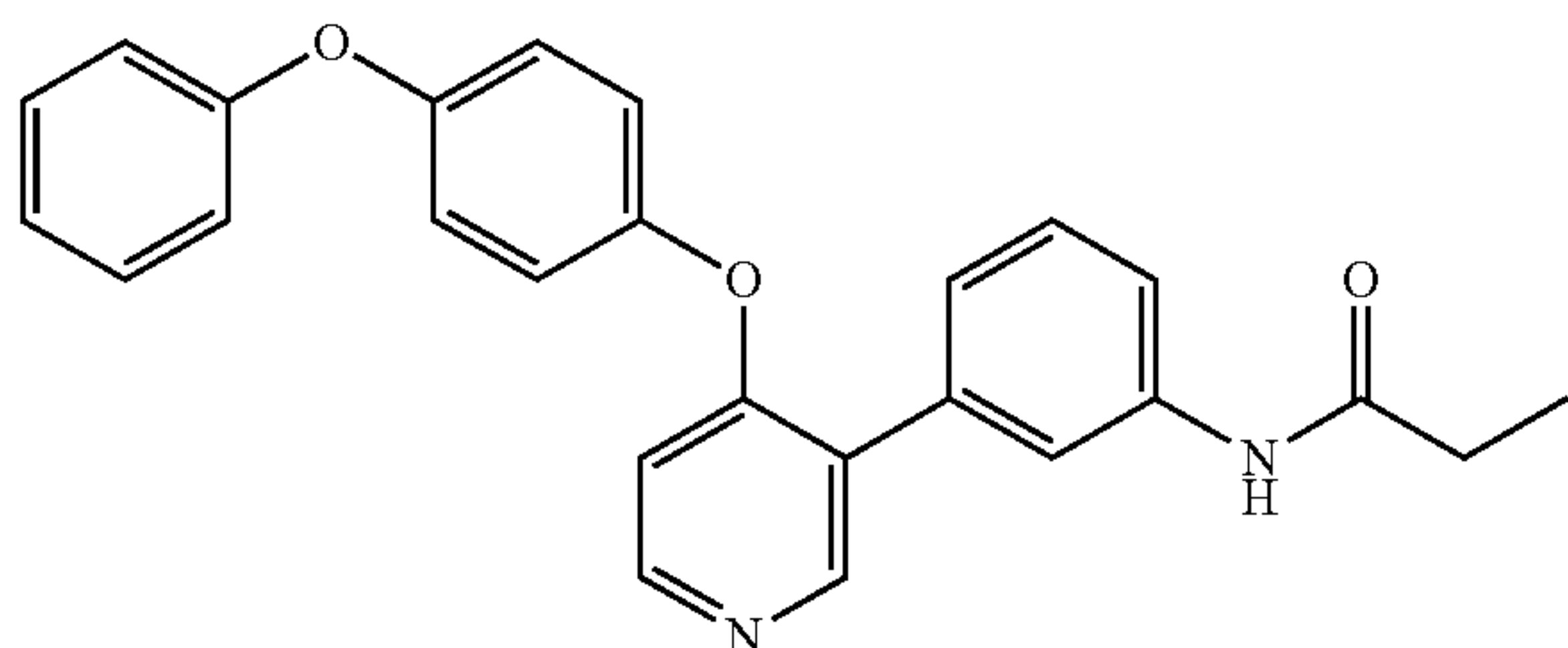
N-(3-(4-(4-phenoxyphenoxy)pyridin-3-yl)phenyl)propionamide (A319)
