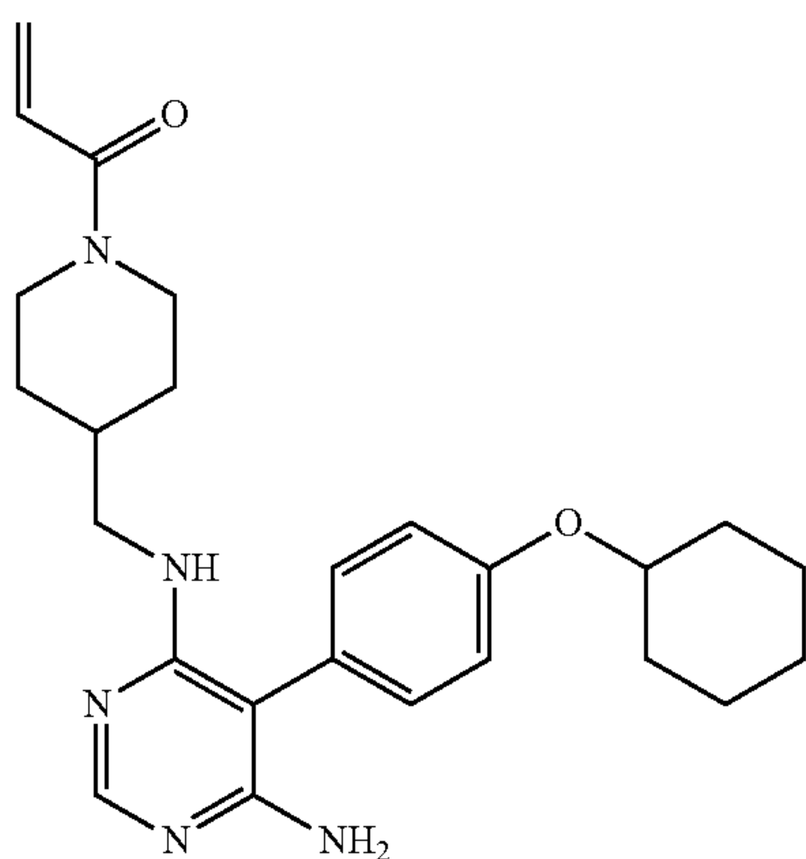
1-(4-(((6-amino-5-(4-(cyclohexyloxy)phenyl)pyrimidin-4-yl)amino)methyl)piperidin-1-yl)prop-2-en-1-one (A99)
