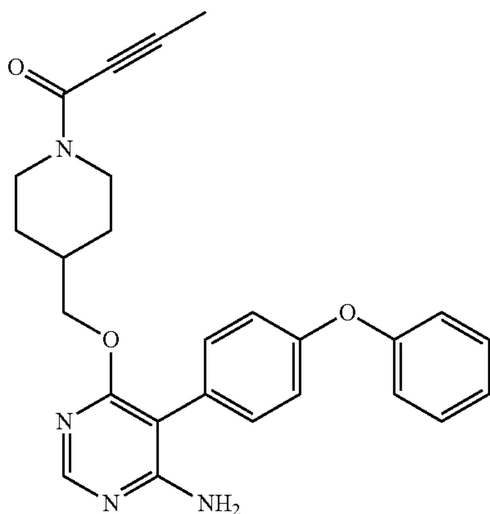
1-(4-(((6-amino-5-(4-phenoxyphenyl)pyrimidin-4-yl)oxy)methyl)piperidin-1-yl)but-2-yn-1-one (A9)
