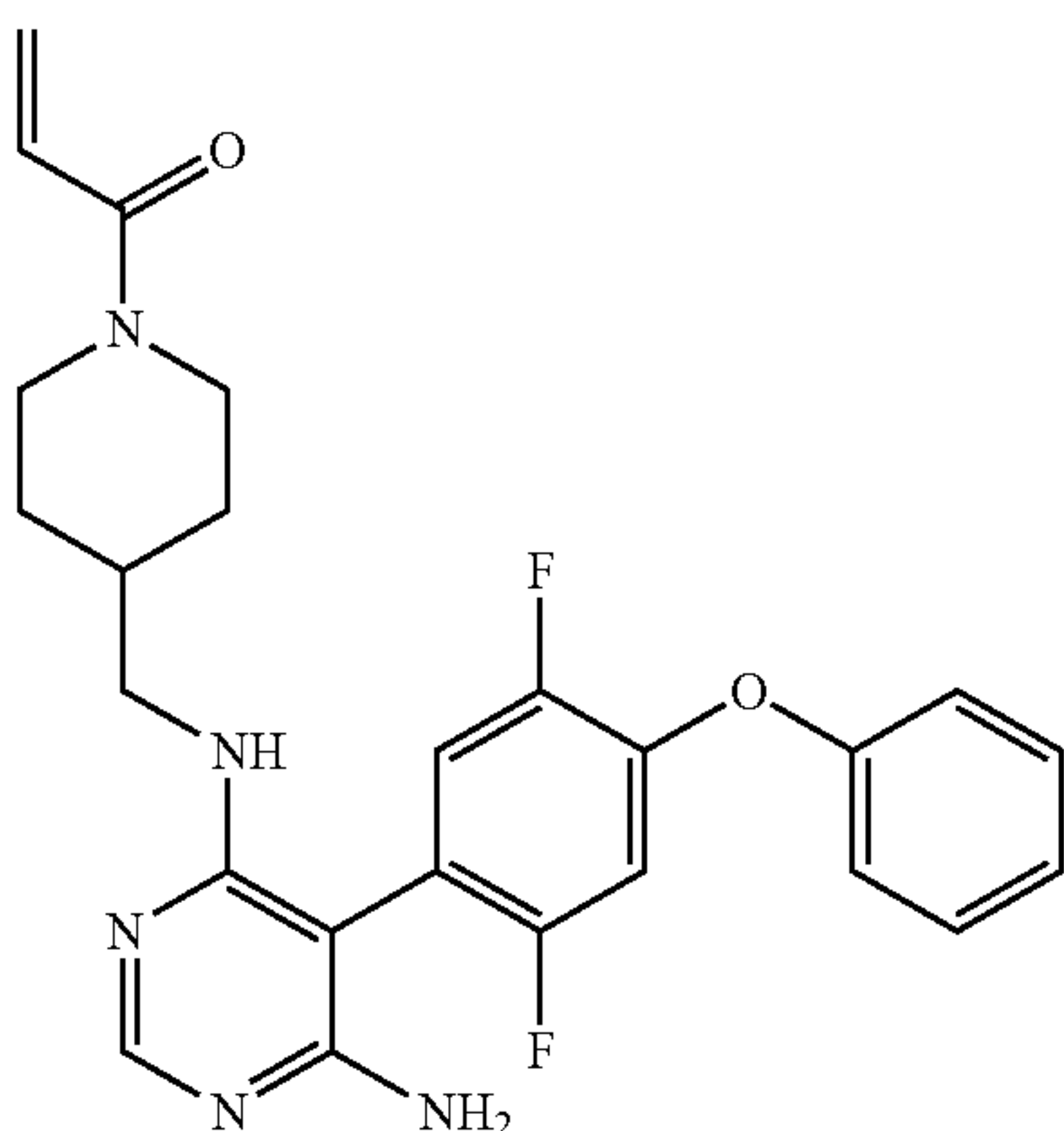
1-(4-(((6-amino-5-(2,5-difluoro-4-phenoxyphenyl)pyrimidin-4-yl)amino)methyl)piperidin-1-yl)prop-2-en-1-one (A87)
