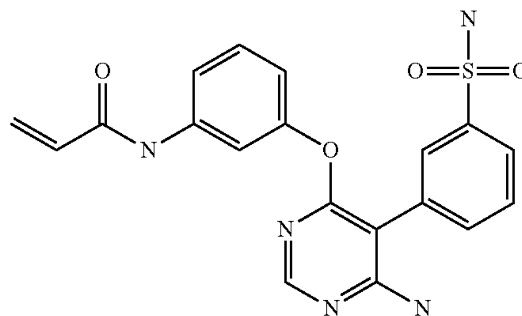
N-(3-((6-amino-5-(3-sulfamoylphenyl)pyrimidin-4-yl)oxy)phenyl)acrylamide (A163)
