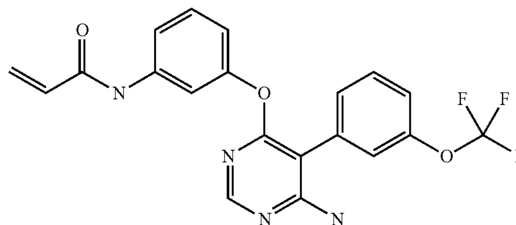
N-(3-((6-amino-5-(3-(trifluoromethoxy)phenyl)pyrimidin-4-yl)oxy)phenyl)acrylamide (A164)
