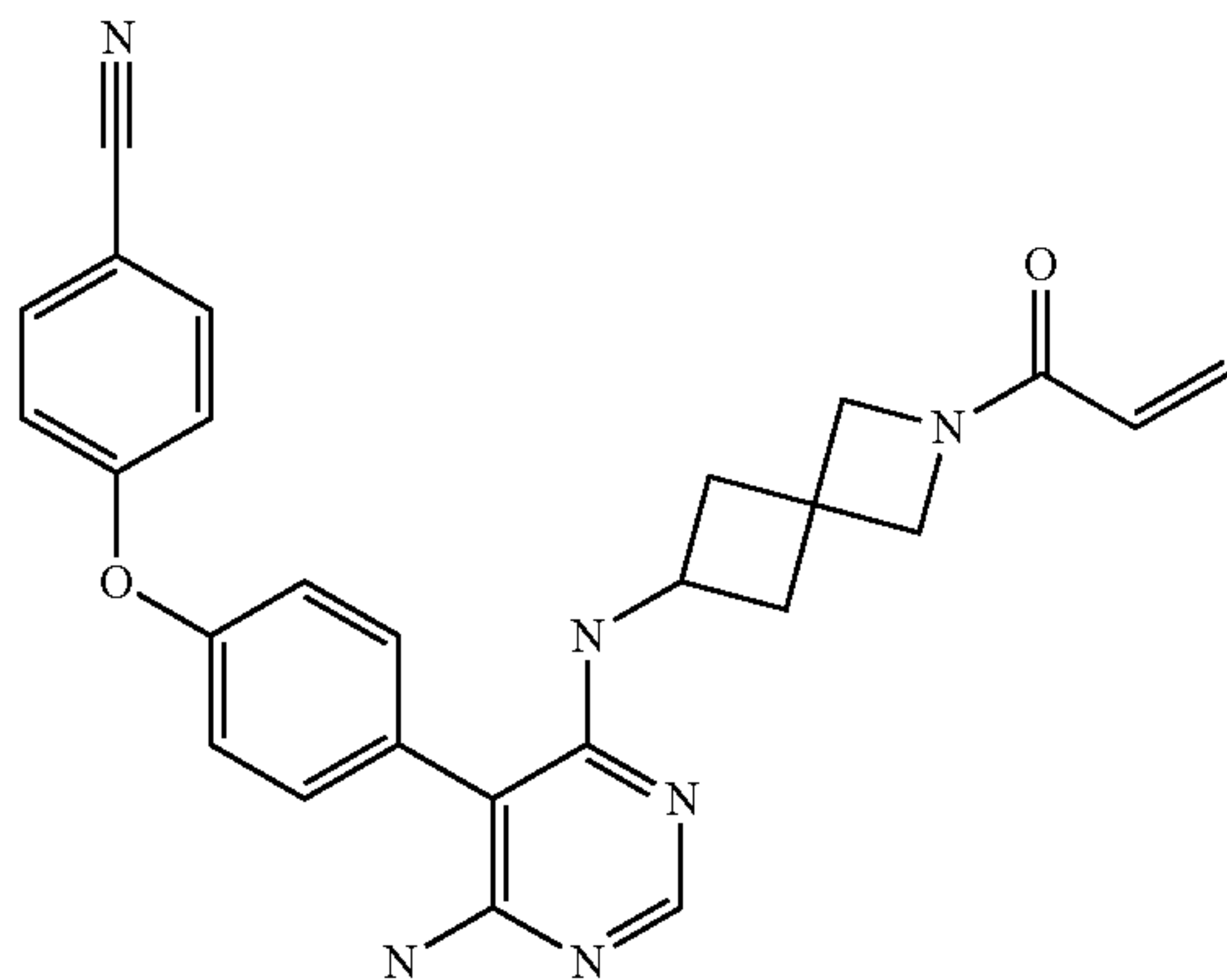
4-(4-(4-((2-acryloyl-2-azaspiro[3.3]heptan-6-yl)amino)-6-aminopyrimidin-5-yl)phenoxy)benzonitrile (A207)
