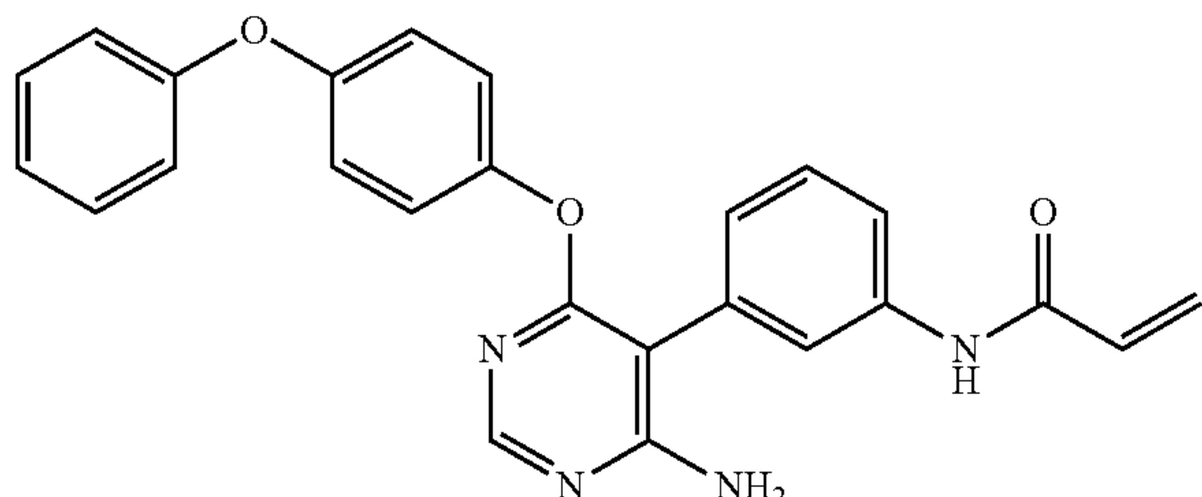
N-(3-(4-amino-6-(4-phenoxyphenoxy)pyrimidin-5-yl)phenyl)acrylamide (A245)
