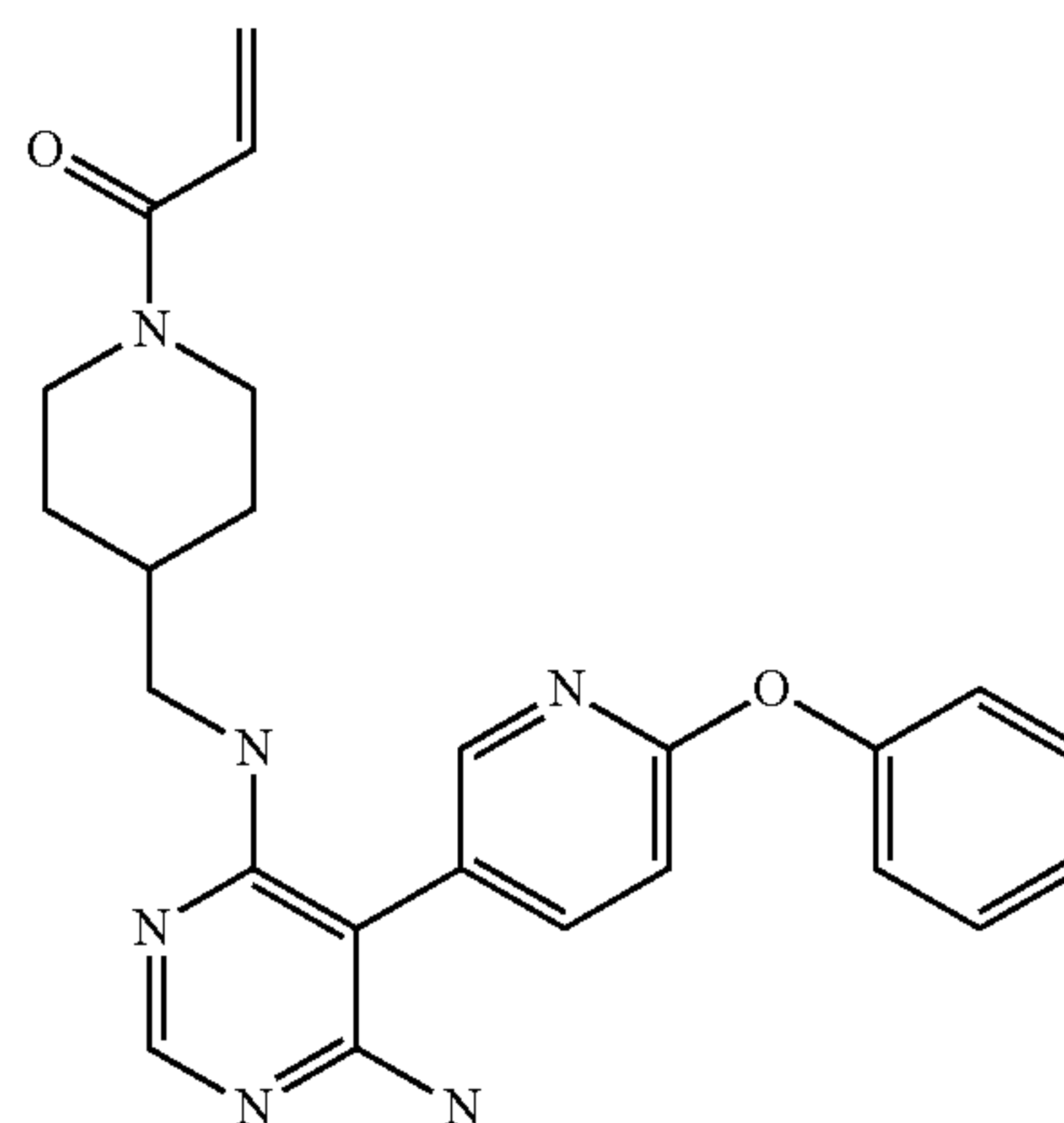
1-(4-(((6-amino-5-(6-phenoxy)pyridin-3-yl)pyrimidin-4-yl)amino)methyl)piperidin-1-yl)prop-2-en-1-one (A168)
