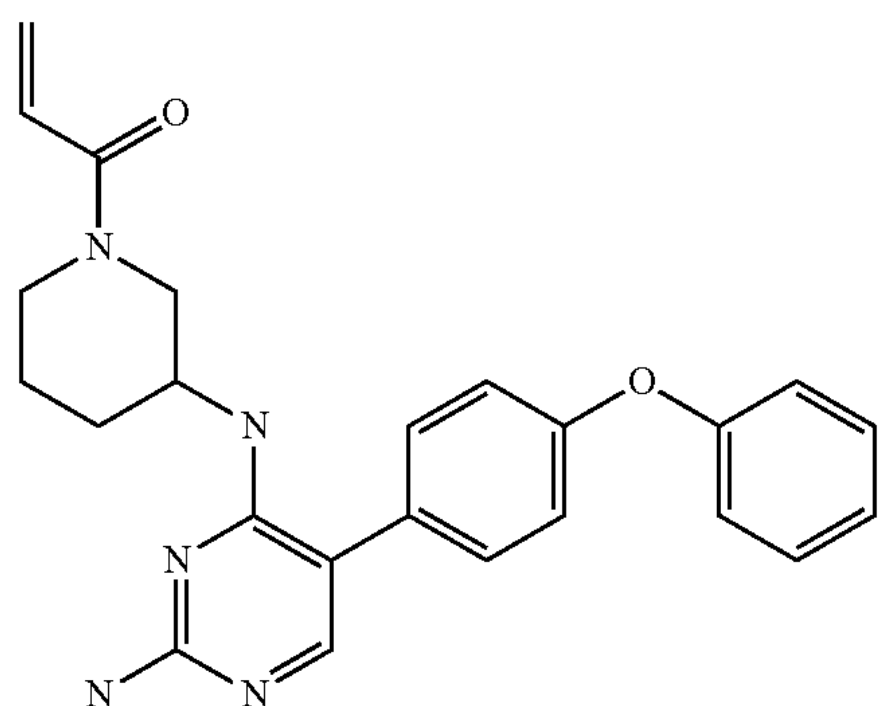
1-(3-((2-amino-5-(4-phenoxyphenyl)pyrimidin-4-yl)amino)piperidin-1-yl)prop-2-en-1-one (A150)
