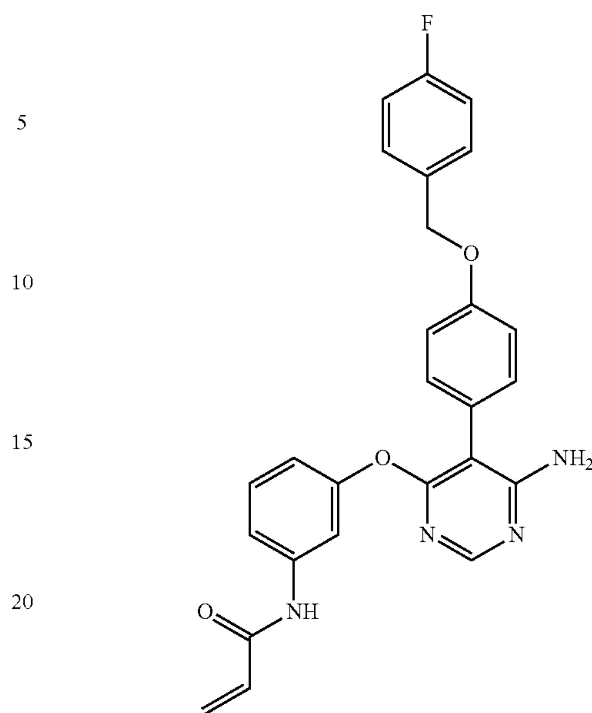
N-(3-{6-Amino-5-[4-(4-fluoro-benzyloxy)-phenyl]-pyrimidin-4-yloxy}-phenyl)-acrylamide (A344)
