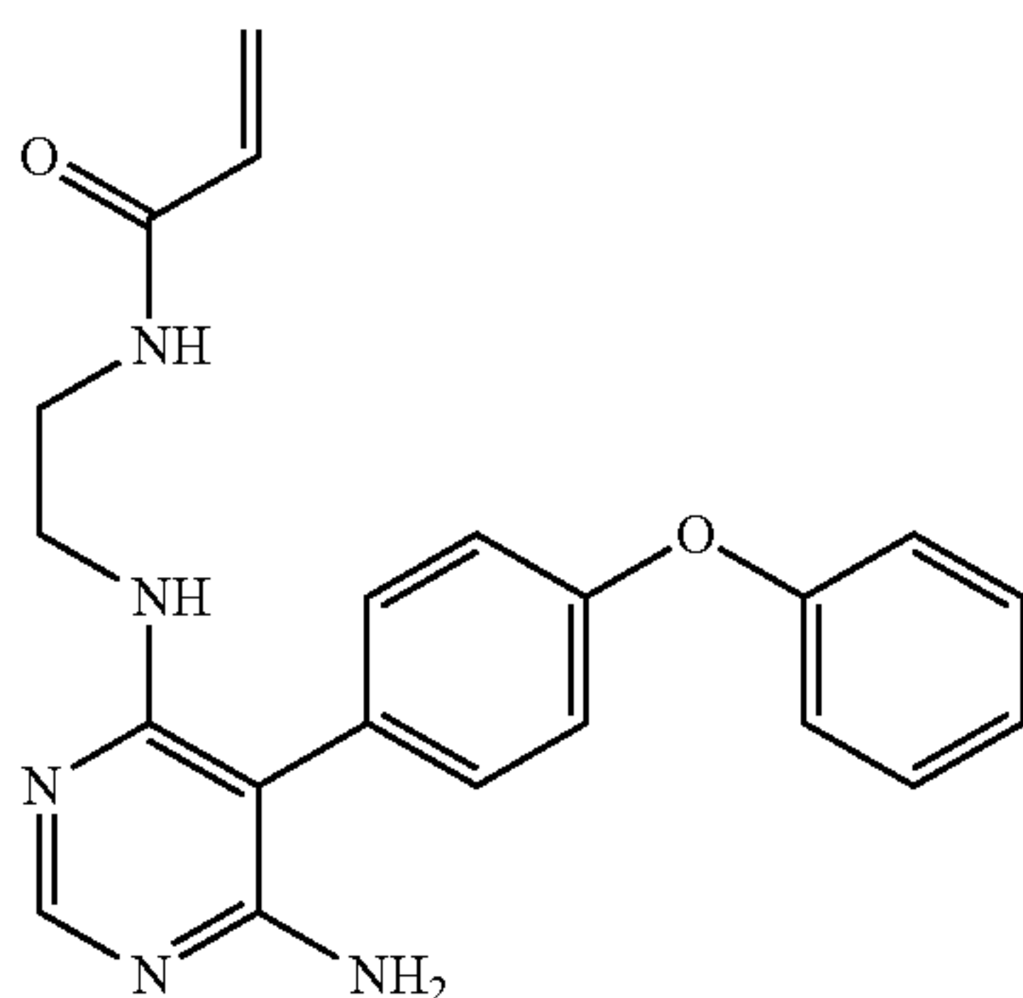
N-(2-(((6-amino-5-(4-phenoxyphenyl)pyrimidin-4-yl)amino)ethyl)acrylamide (A18)
