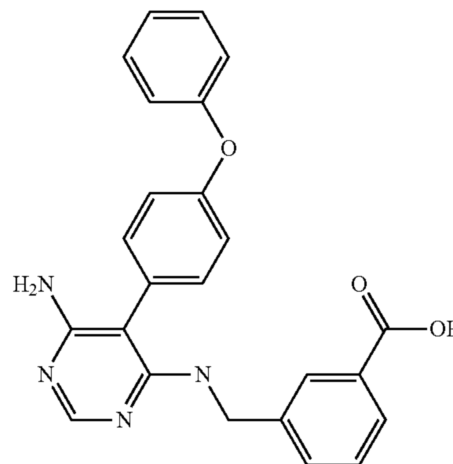
3-((6-Amino-5-(4-phenoxy-phenyl)-pyrimidin-4-ylamino)-methyl)-benzoic acid (134)
