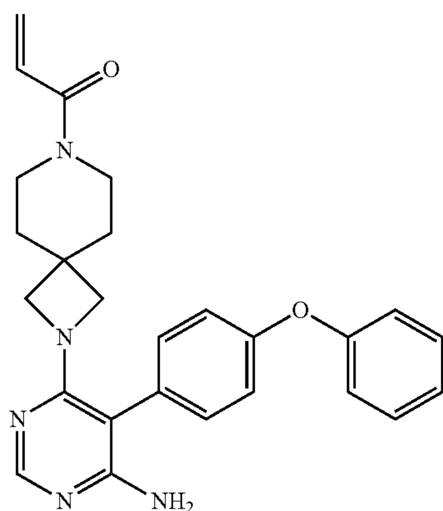
1-(2-(6-amino-5-(4-phenoxyphenyl)pyrimidin-4-yl)-2,7-diazaspiro[3.5]nonan-7-yl)prop-2-en-1-one (A91)
