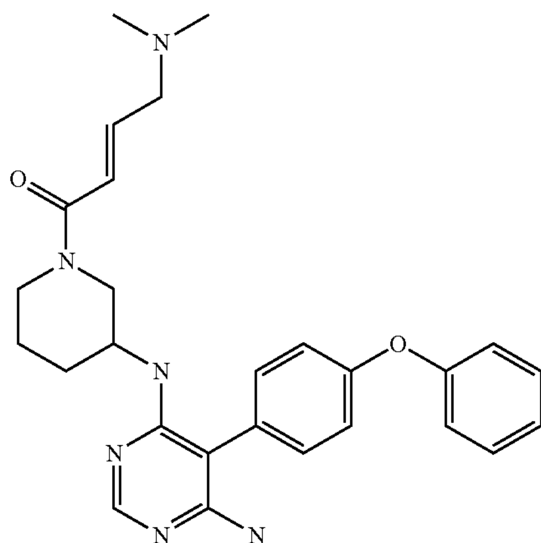
(E)-1-(3-((6-amino-5-(4-phenoxyphenyl)pyrimidin-4-yl)amino)piperidin-1-yl)-4-(dimethylamino)but-2-en-1-one (A160)
