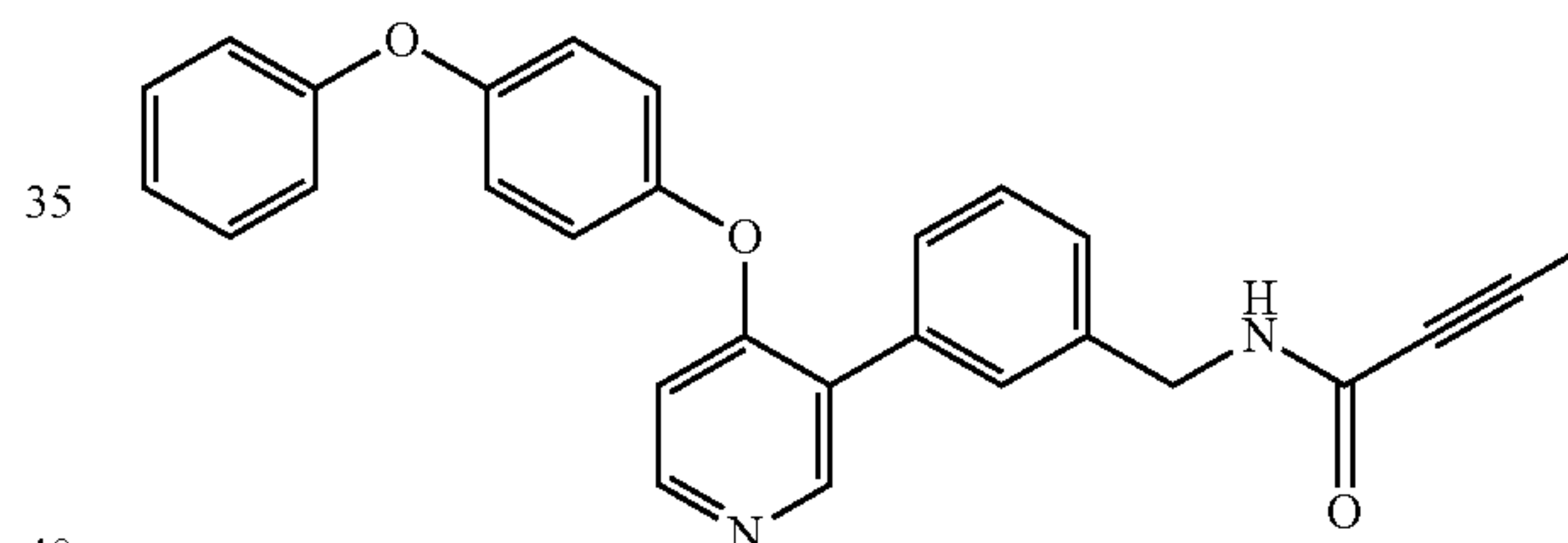
N-(3-(4-(4-phenoxyphenoxy)pyridin-3-yl)benzyl)but-2-ynamide (A304)
