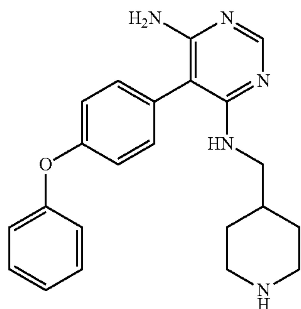
5-(4-phenoxyphenyl)-N-(piperidin-4-ylmethyl)pyrimidine-4,6-diamine
