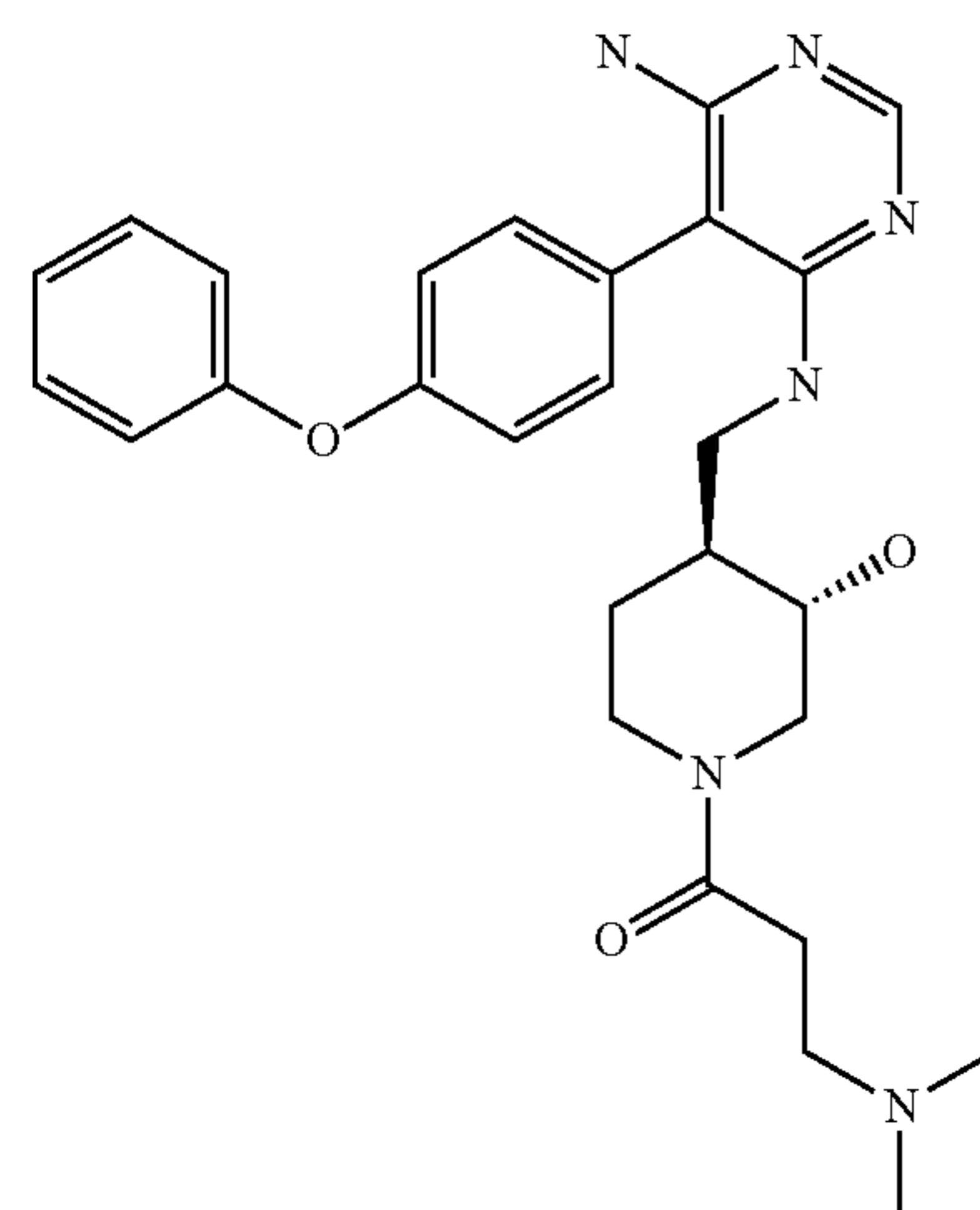
1-(((3S,4S)-4-(((6-amino-5-(4-phenoxyphenyl)pyrimidin-4-yl)amino)methyl)-3-hydroxypiperidin-1-yl)-3-(dimethylamino)propan-1-one (A232)
