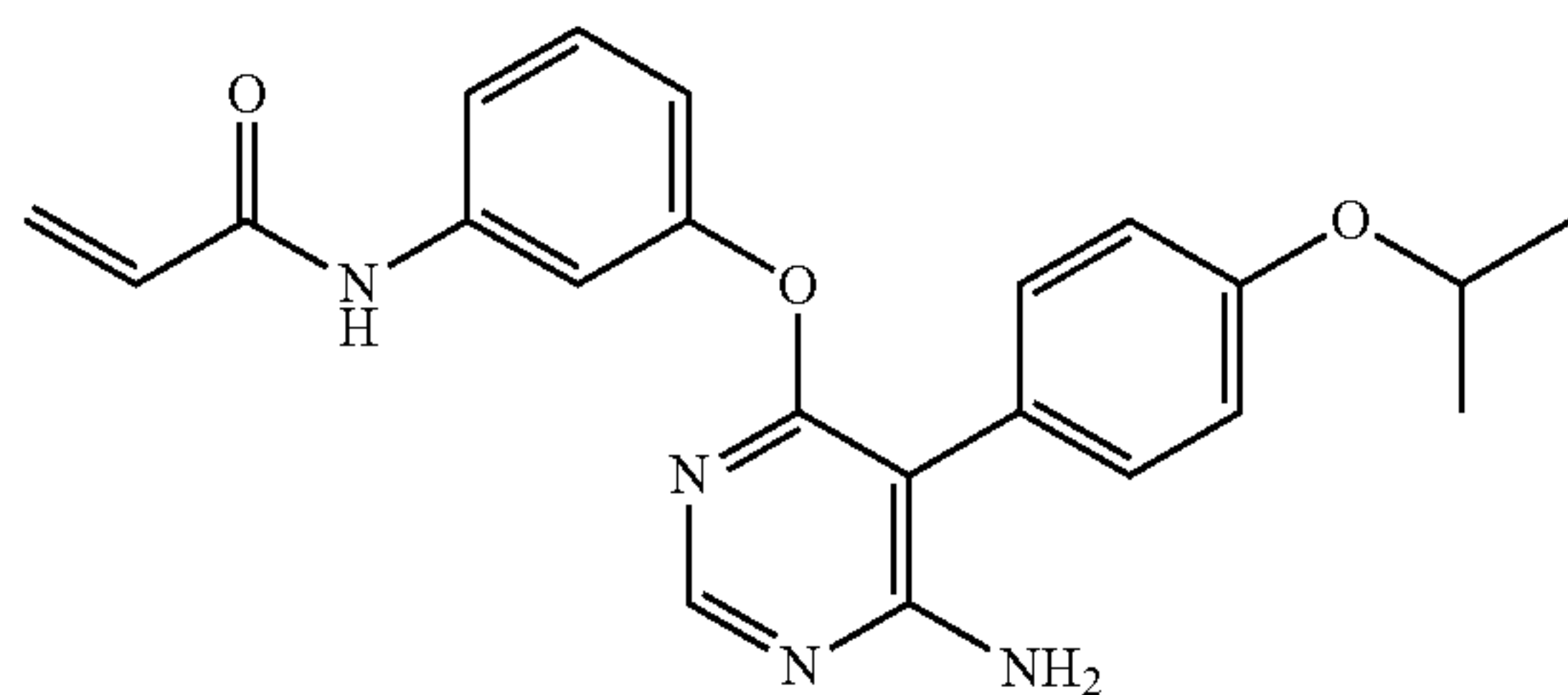
N-(3-((6-amino-5-(4-isopropoxyphenyl)pyrimidin-4-yl)oxy)phenyl)acrylamide (A289)
