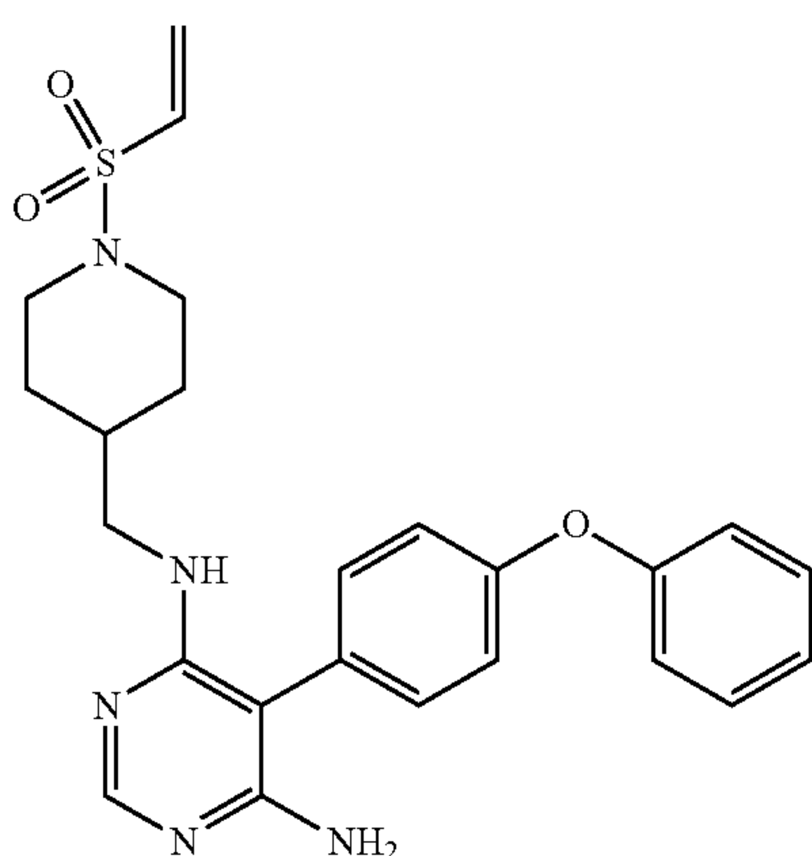
5-(4-phenoxyphenyl)-N4-((1-(vinylsulfonyl)piperidin-4-yl)methyl)pyrimidine-4,6-diamine (A10)
