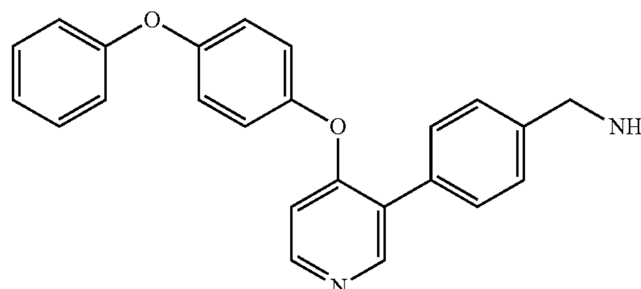
(4-(4-(4-phenoxyphenoxy)pyridin-3-yl)phenyl)methanamine (A315)
