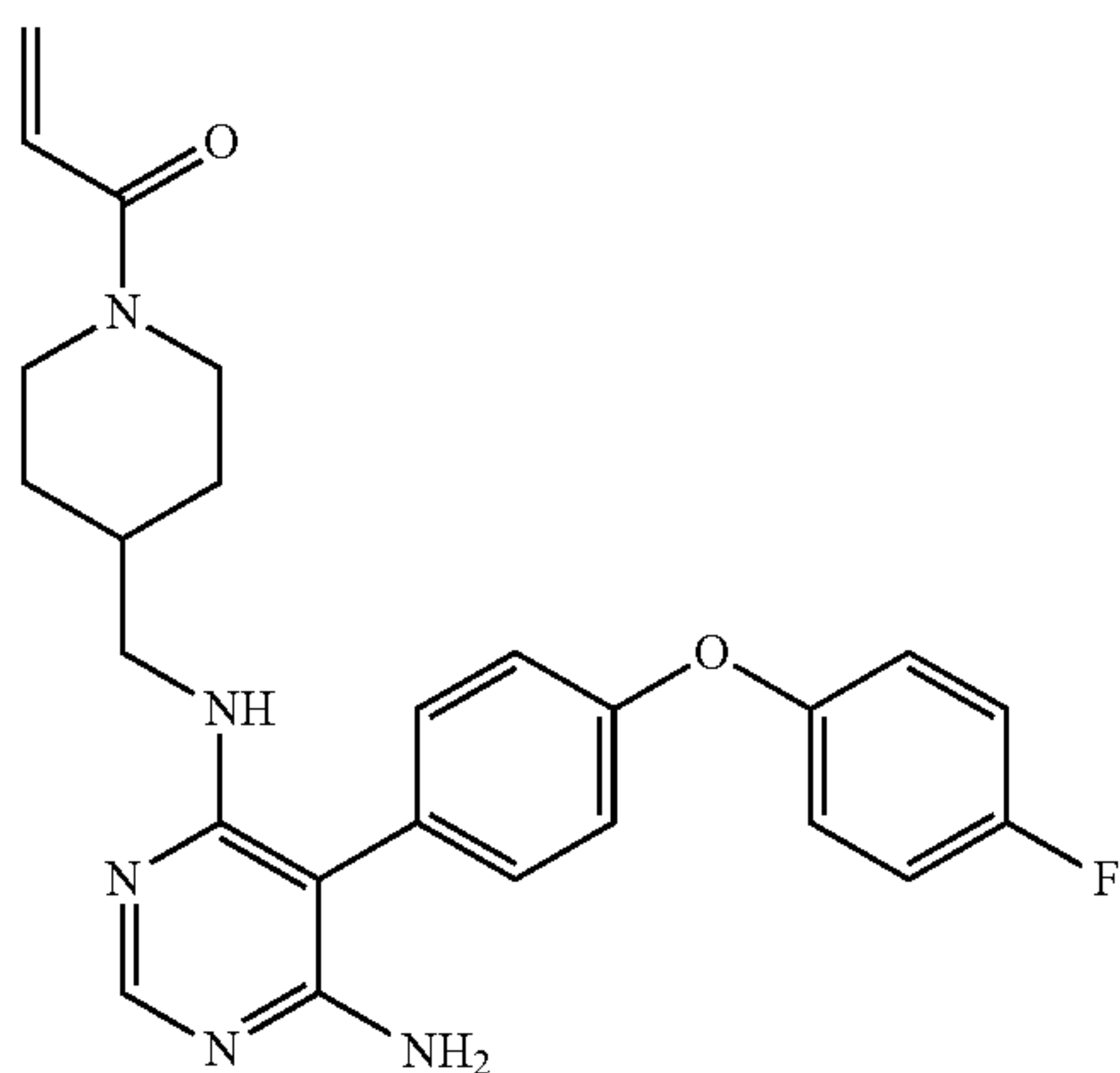
1-(4-(((6-amino-5-(4-(4-(fluorophenoxy)phenyl)pyrimidin-4-yl)amino)methyl)piperidin-1-yl)prop-2-en-1-one (A80)
