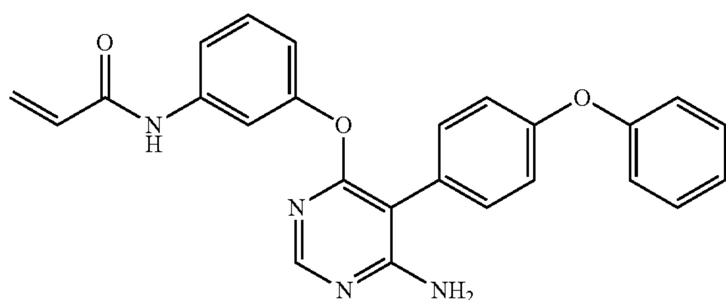
N-(3-{[6-amino-5-(4-phenoxyphenyl)pyrimidin-4-yl]oxy}phenyl)acrylamide
