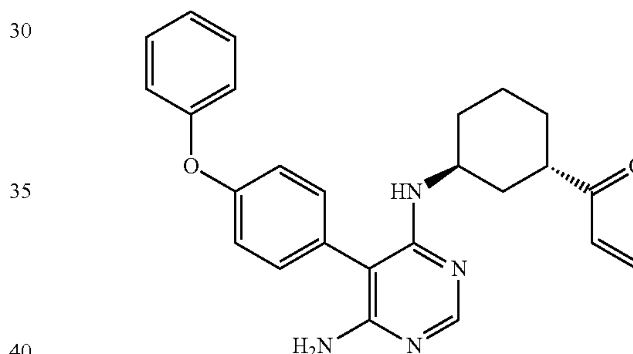
1-((1S,3S)-3-(6-Amino-5-(4-phenoxyphenyl)-pyrimidin-4-ylamino)-cyclohexyl)-propenone (A143)
