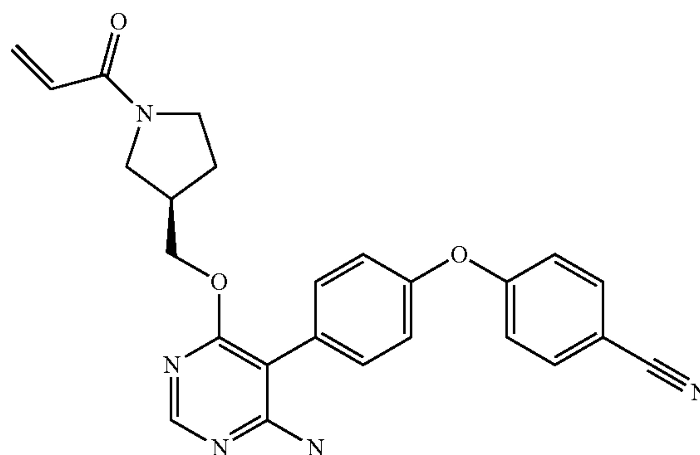
(R)-4-(4-(4-((1-acryloylpyrrolidin-3-yl)methoxy)-6-aminopyrimidin-5-yl)phenoxy)benzonitrile (A201)
