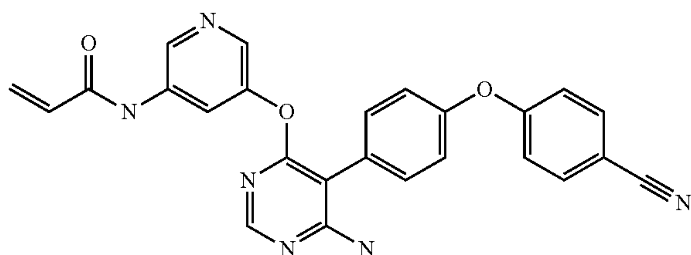
N-(5-((6-amino-5-(4-(4-cyanophenoxy)phenyl)pyrimidin-4-yl)oxy)pyridin-3-yl)acrylamide (A197)
