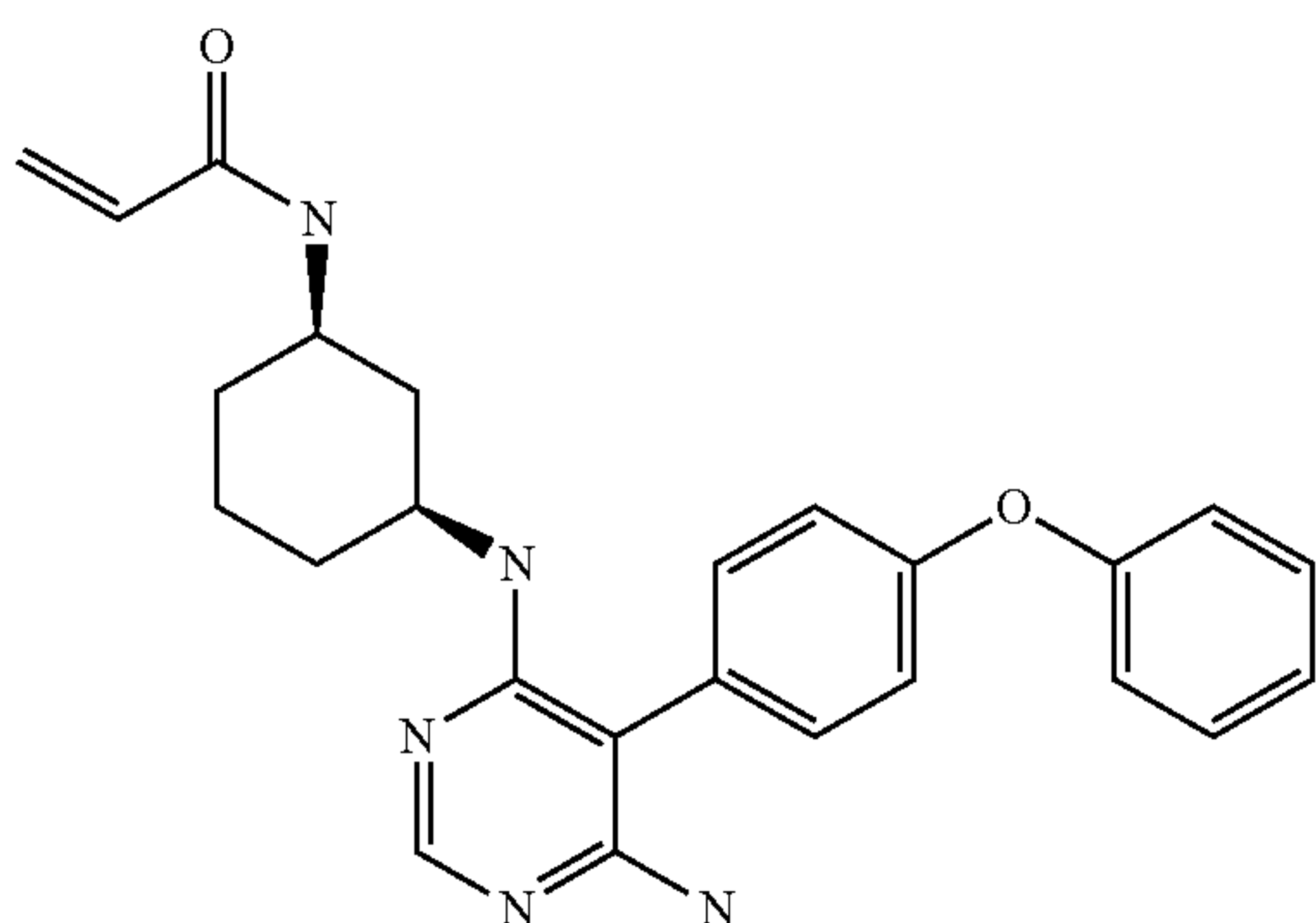
N-((1R,3S)-3-((6-amino-5-(4-phenoxyphenyl)pyrimidin-4-yl)amino)cyclohexyl)acrylamide (A174)
