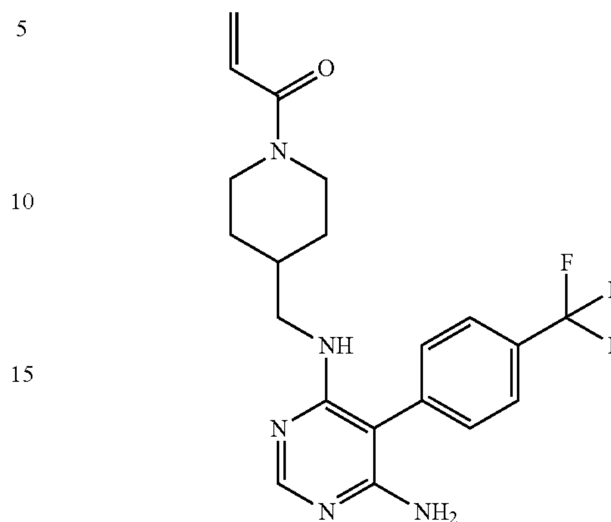
1-(4-(((6-amino-5-(4-(4-(trifluoromethyl)phenyl)pyrimidin-4-yl)amino)methyl)piperidin-1-yl)prop-2-en-1-one (A81)
