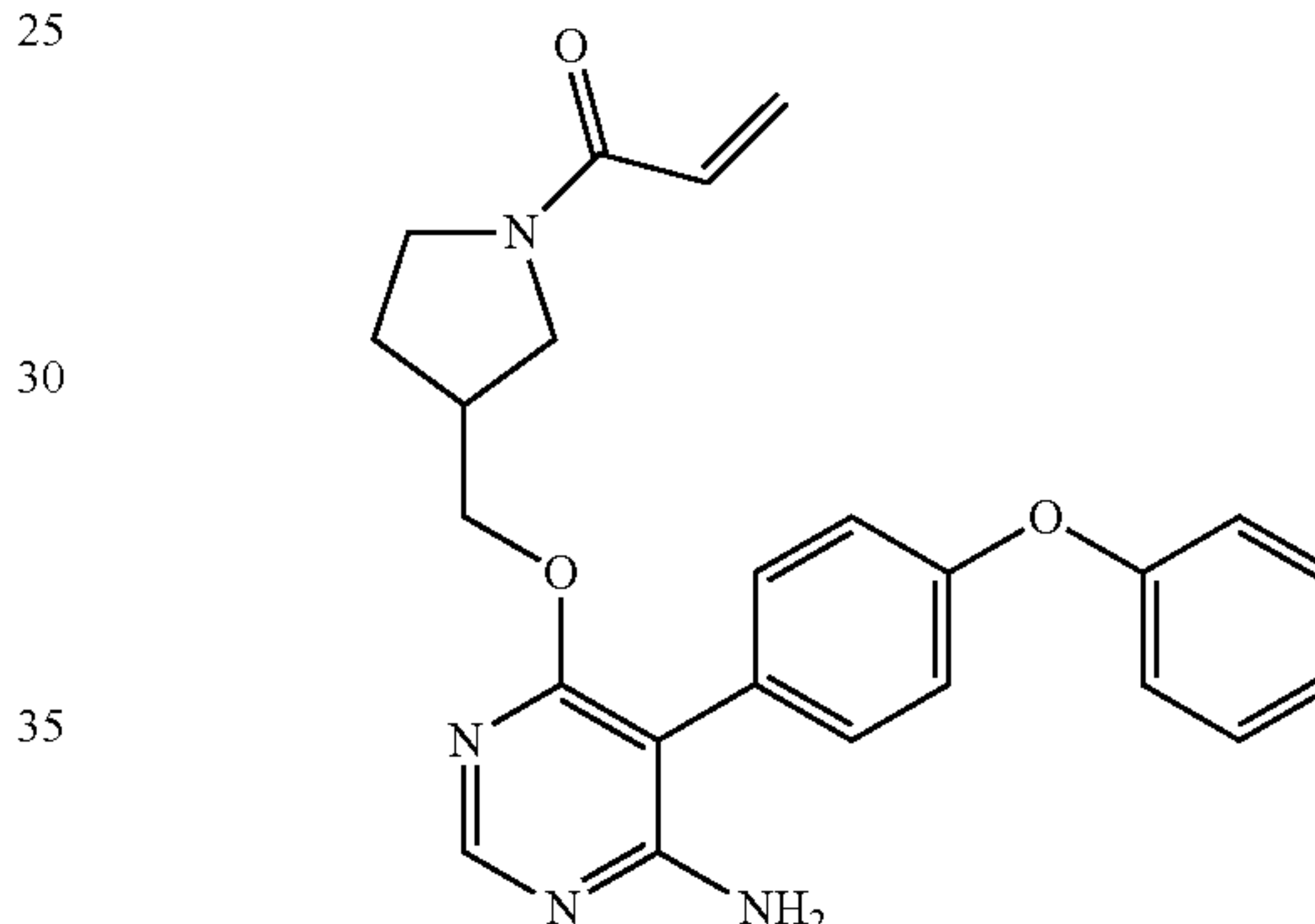
1-(3-(((6-amino-5-(4-phenoxyphenyl)pyrimidin-4-yl)oxy)methyl)pyrrolidin-1-yl)prop-2-en-1-one (A21)
