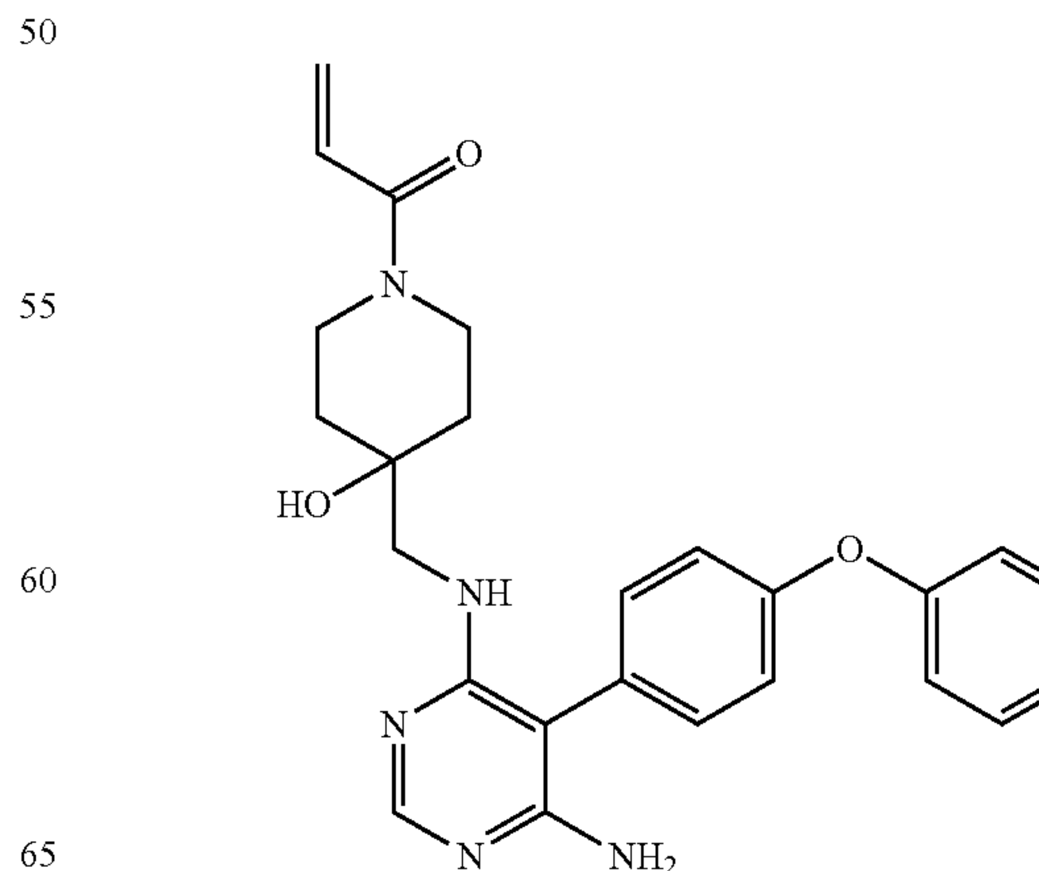
(E)-7-(3-((2-(4-(4-((3-((6-amino-5-(4-phenoxyphenyl)pyrimidin-4-yl)oxy)phenyl)amino)-4-oxobut-2-en-1-yl)piperazin-1-yl)ethyl)amino)-3-oxopropyl)-5,5-difluoro-1,3-dimethyl-5H-dipyrrolo[1,2-c:2',1'-f][1,3,2]diazaborinin-4-ium-5-uide (A35)
