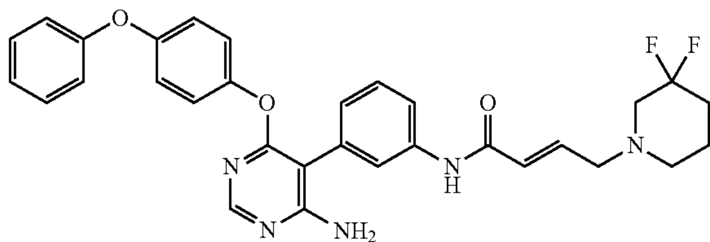
(E)-N-(3-(4-amino-6-(4-phenoxyphenoxy)pyrimidin-5-yl)phenyl)-4-(3,3-difluoropiperidin-1-yl)but-2-enamide (A301)
