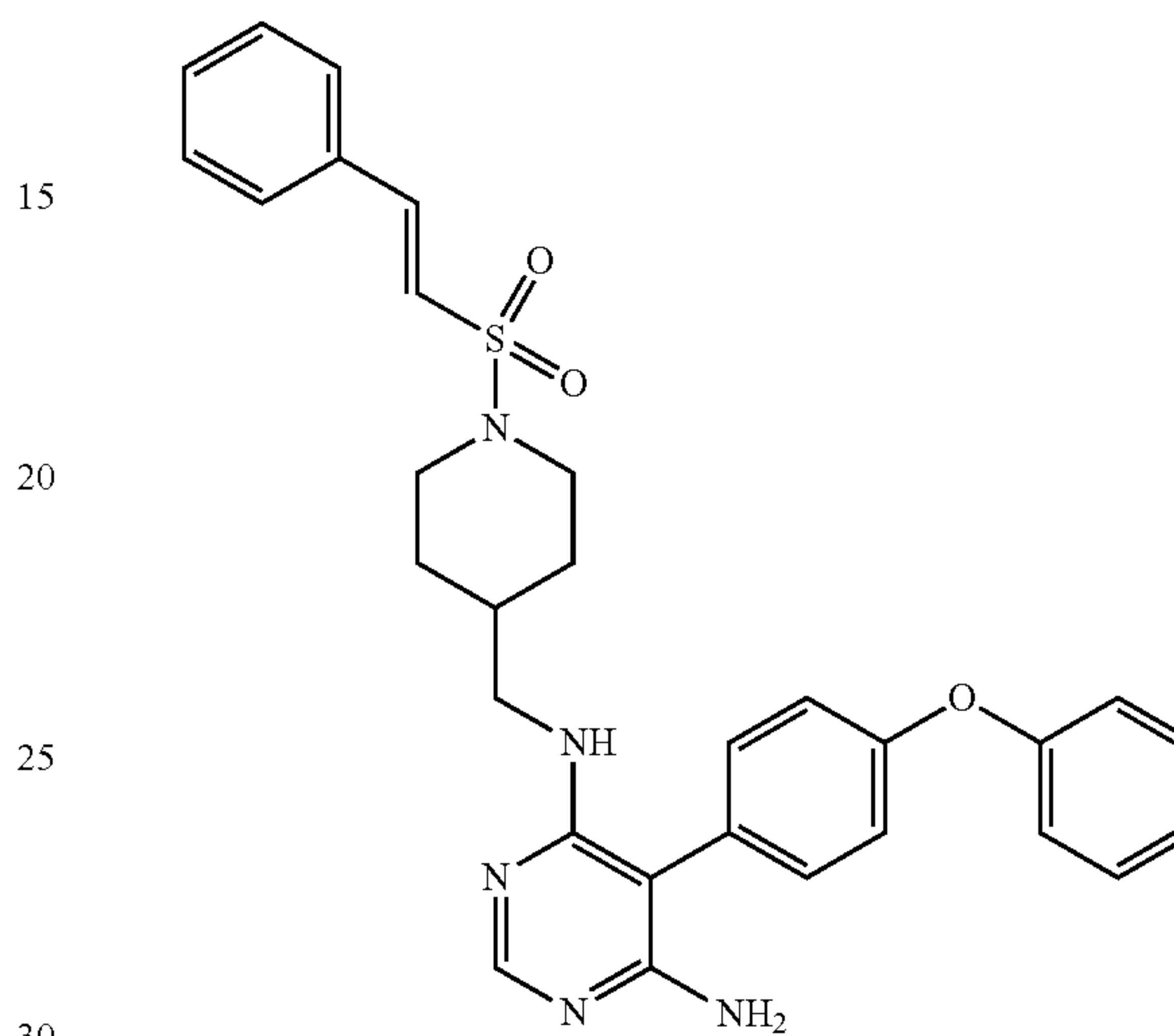
(E)-5-(4-phenoxyphenyl)-N4-((1-(styrylsulfonyl)piperidin-4-yl)methyl)pyrimidine-4,6-diamine (A54)
