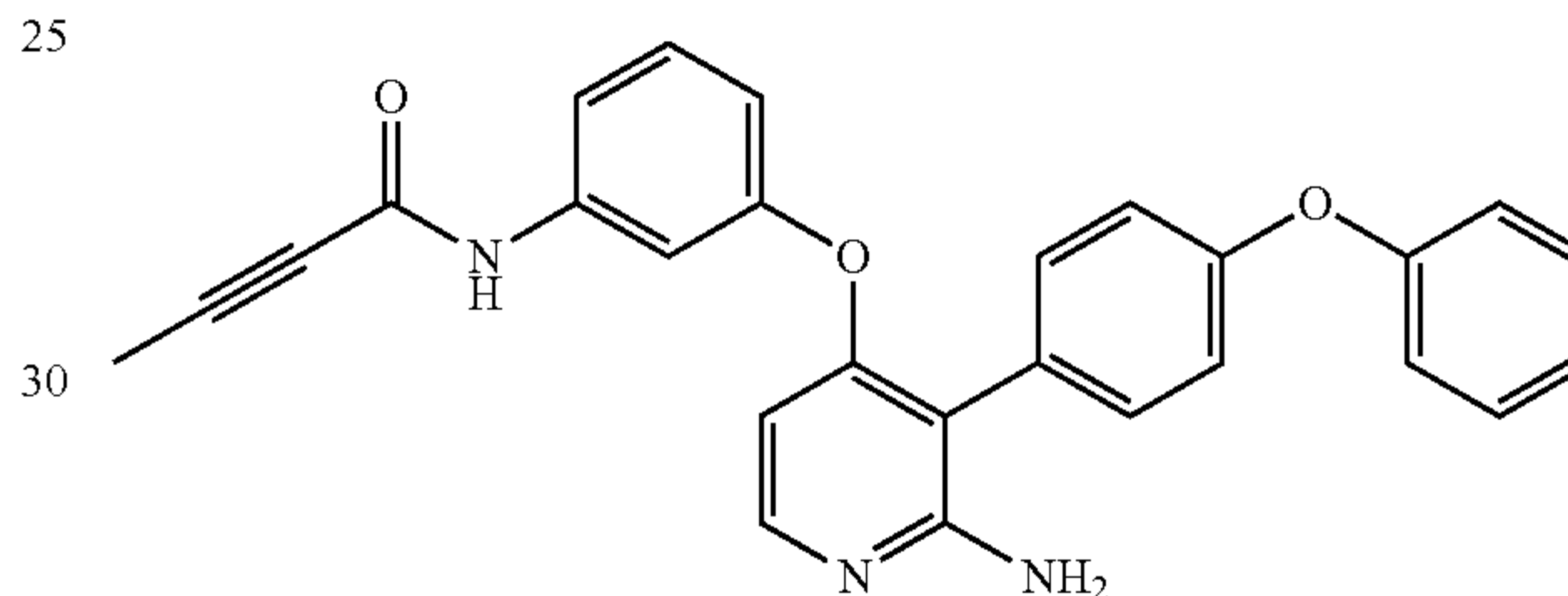
N-(3-((2-amino-3-(4-phenoxyphenyl)pyridin-4-yl)oxy)phenyl)but-2-ynamide (A340)
