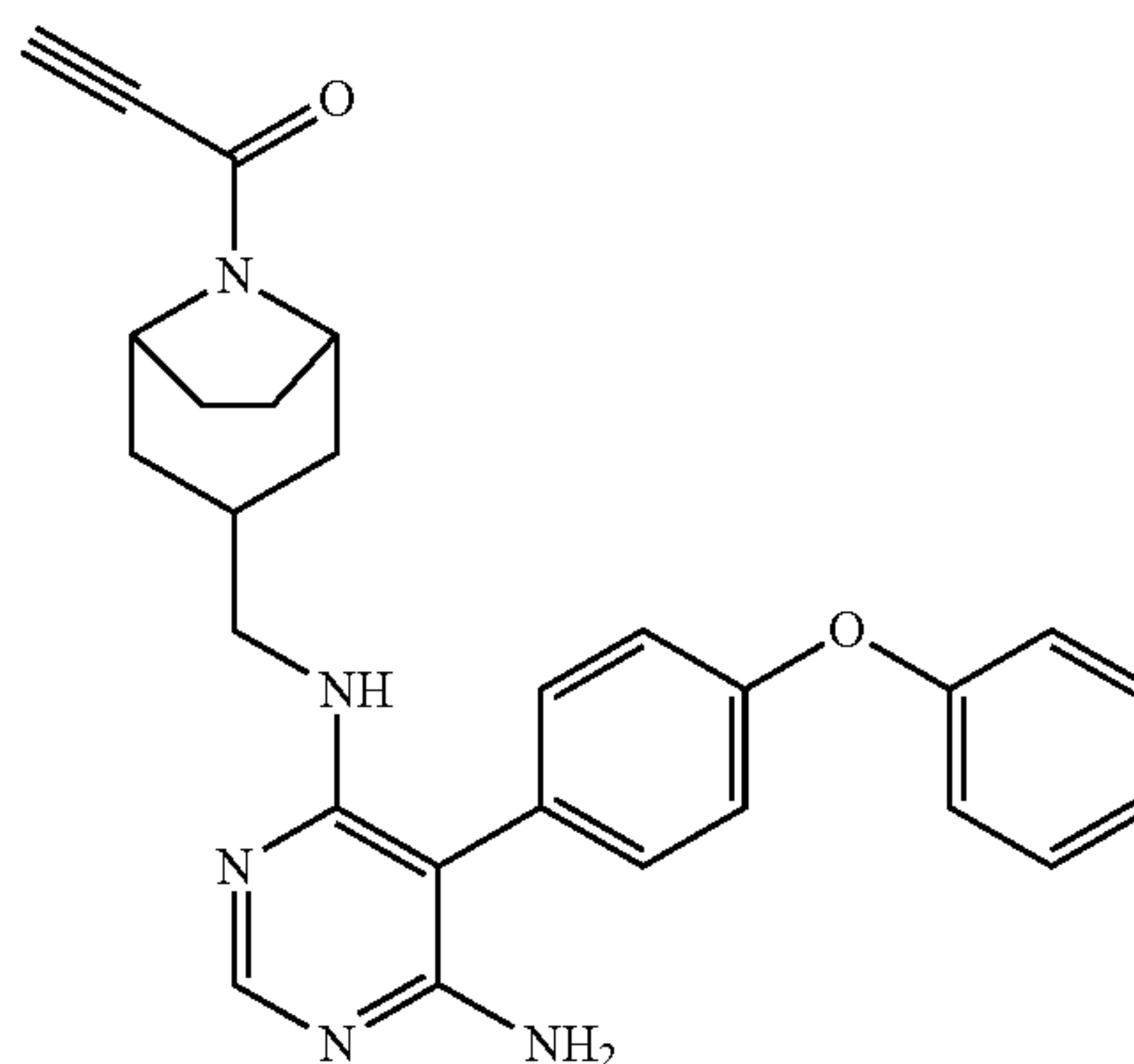
1-(3-(((6-amino-5-(4-phenoxyphenyl)pyrimidin-4-yl)amino)methyl)-8-azabicyclo[3.2.1]octan-8-yl)prop-2-yn-1-one (A68)
