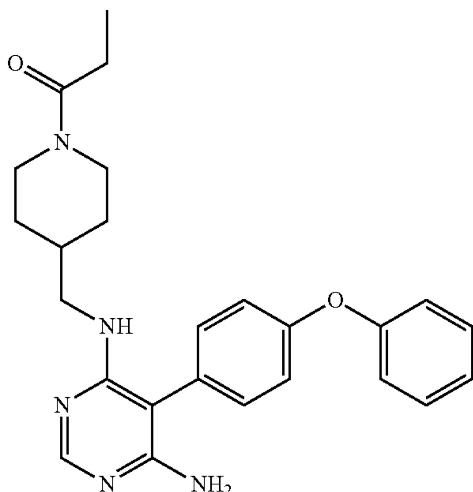
1-(4-(((6-amino-5-(4-phenoxyphenyl)pyrimidin-4-yl)amino)methyl)piperidin-1-yl)propan-1-one (A333)
