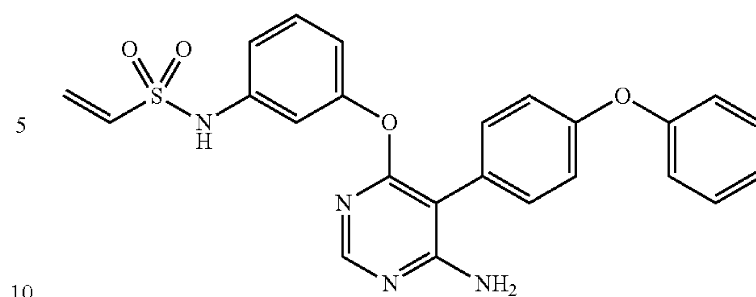
N-(3-(((6-amino-5-(4-phenoxyphenyl)pyrimidin-4-yl)oxy)phenyl)ethanesulfonamide (A58)
