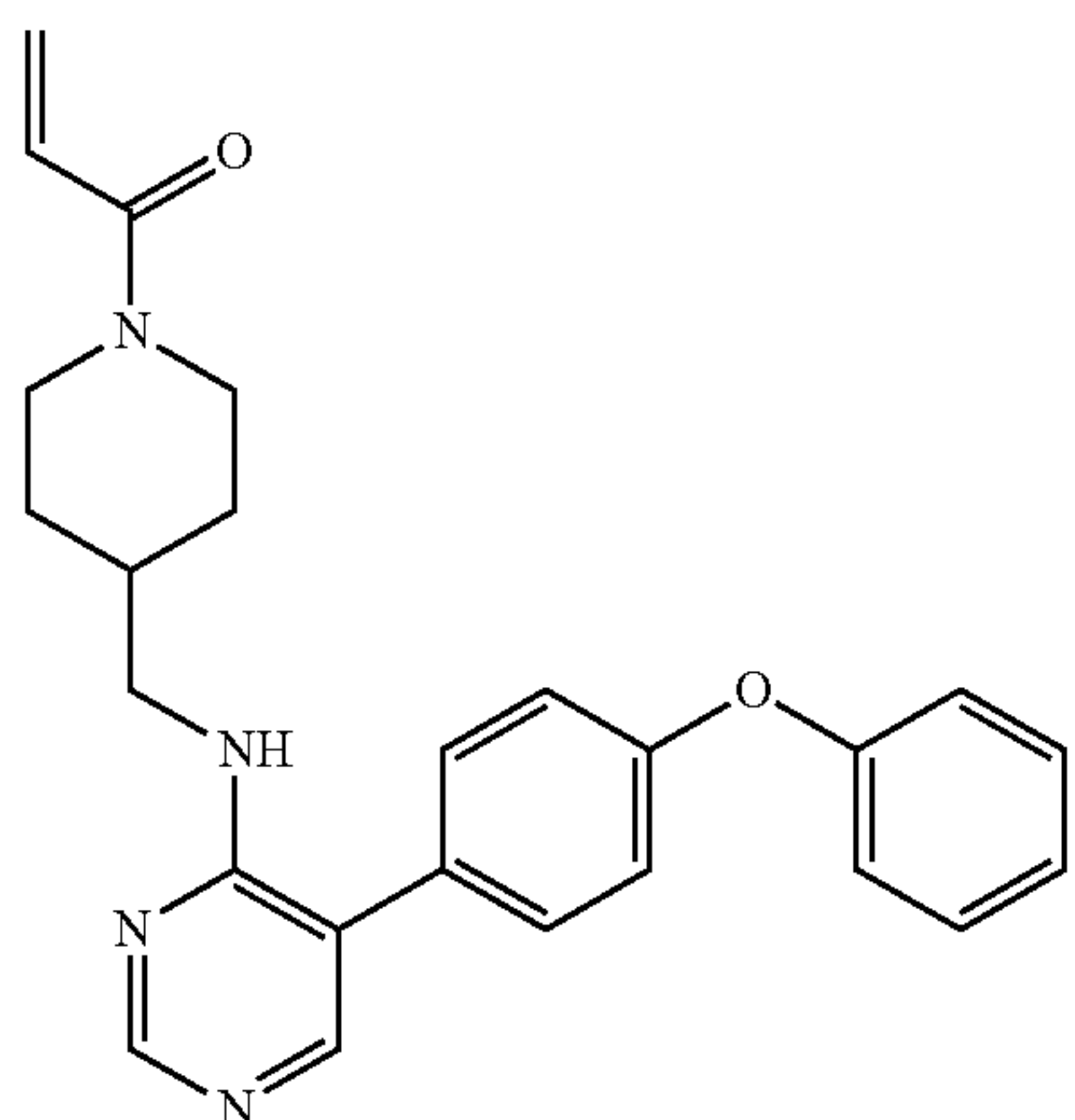
1-(4-(((5-(4-phenoxyphenyl)pyrimidin-4-yl)amino)methyl)piperidin-1-yl)prop-2-en-1-one (A334)
