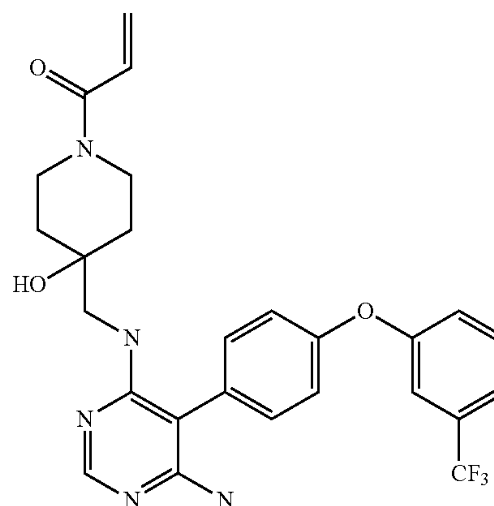
1-(4-(((6-amino-5-(4-(3-(trifluoromethyl)phenoxy)phenyl)pyrimidin-4-yl)amino)methyl)-4-hydroxypiperidin-1-yl)prop-2-en-1-one (A169)
