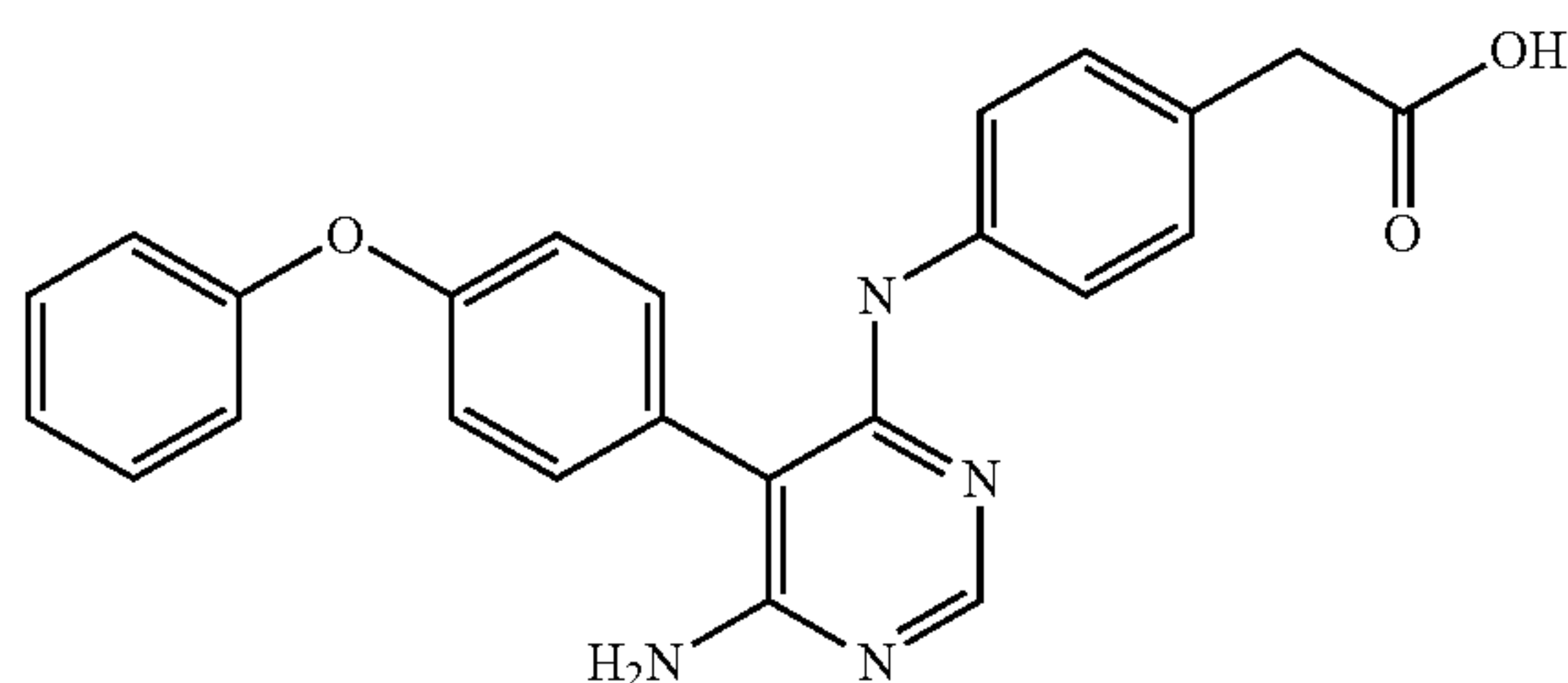
(4-(6-Amino-5-(4-phenoxyphenyl)-pyrimidin-4-ylamino)-phenyl)-acetic acid
