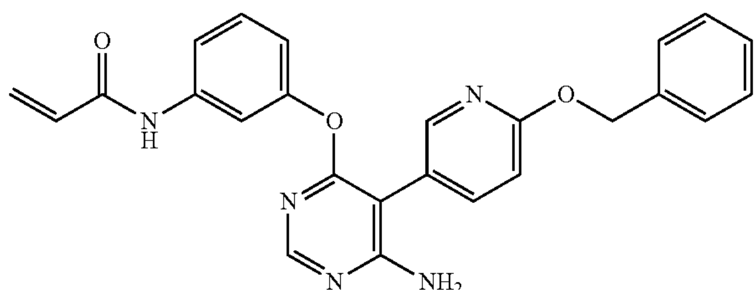
N-(3-((6-amino-5-(6-(benzyloxy)pyridin-3-yl)pyrimidin-4-yl)oxy)phenyl)acrylamide (A259)
