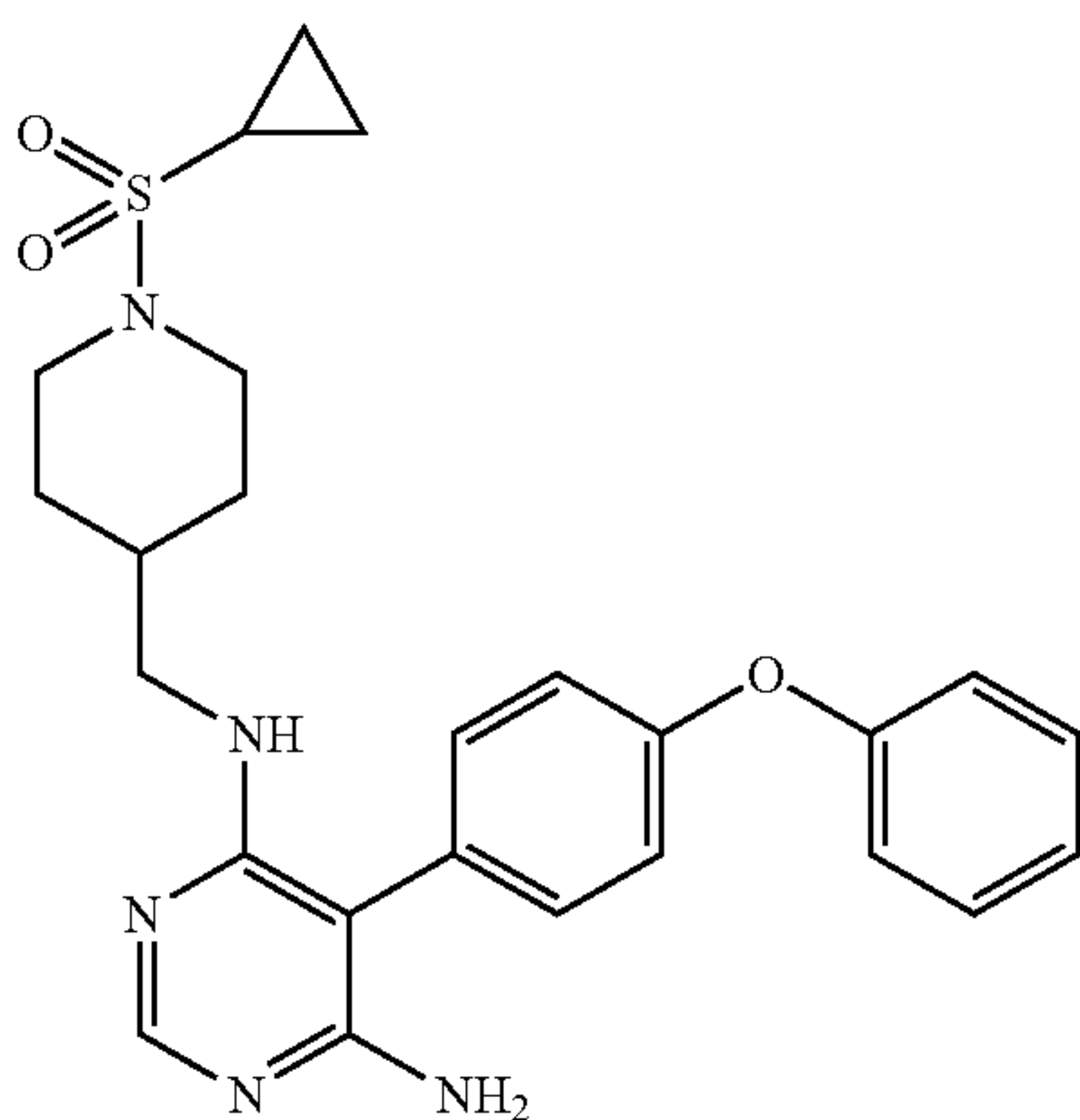
N4-((1-(cyclopropylsulfonyl)piperidin-4-yl)methyl)-5-(4-phenoxyphenyl)pyrimidine-4,6-diamine (A14)
