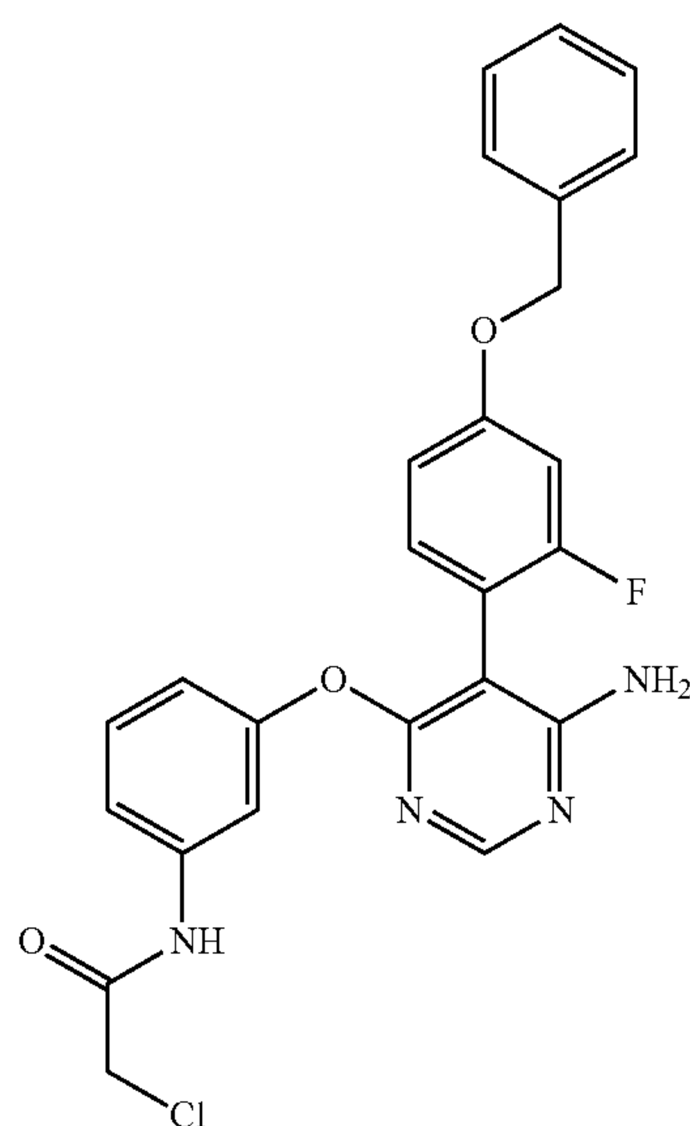
N-{3-(6-Amino-5-(4-benzyloxy-2-fluoro-phenyl)-pyrimidin-4-yloxy)-phenyl}-2-chloro-acetamide (A350)
