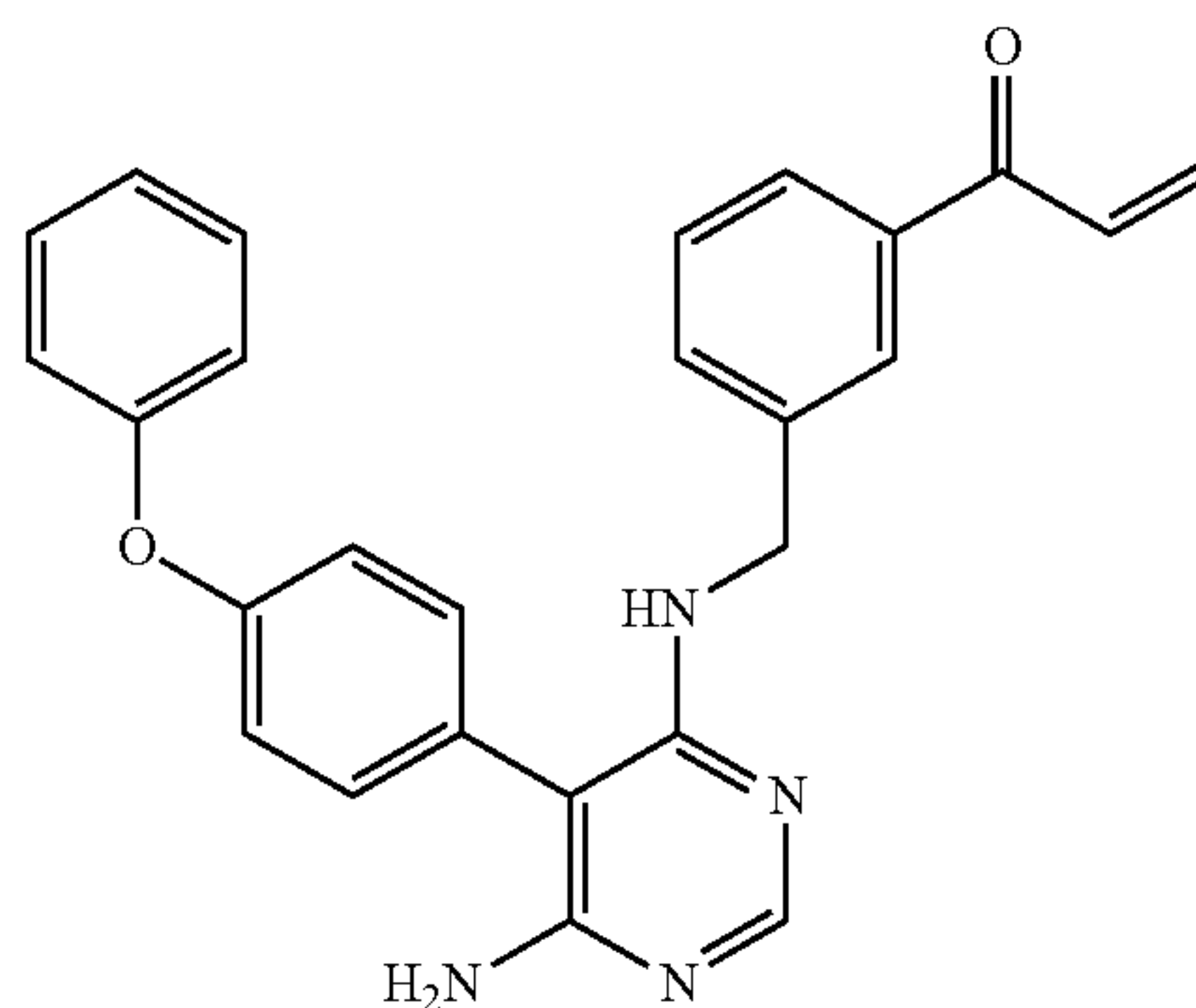
1-(3-((Amino-5-(4-phenoxyphenyl)-pyrimidin-4-ylamino)-methyl)-phenyl)-propanone
