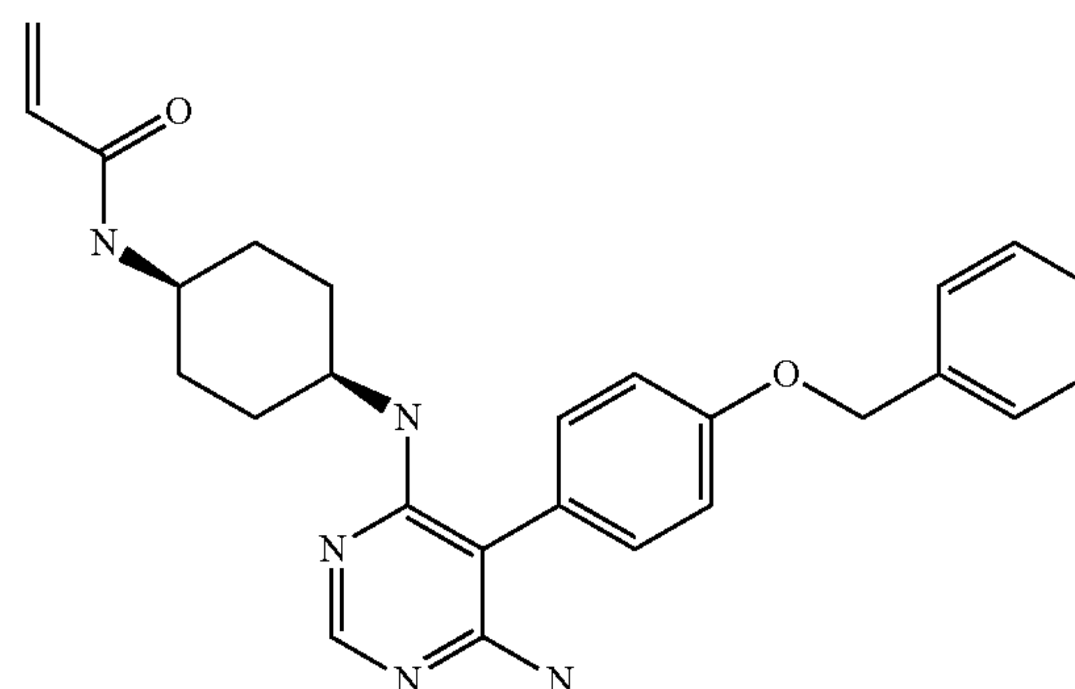
N-cis-4-((6-amino-5-(4-(benzyloxy)phenyl)pyrimidin-4-yl)amino)cyclohexylacrylamide (A154)
