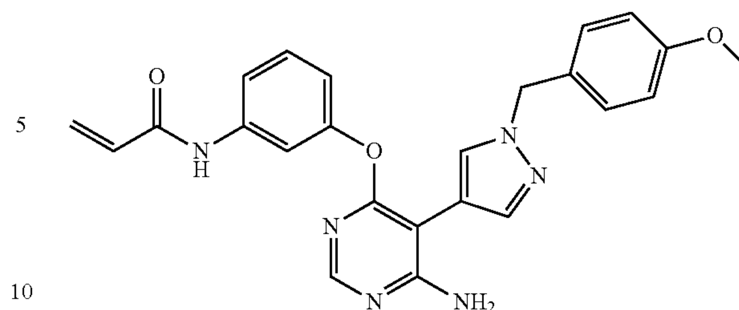
N-(3-((6-amino-5-(1-(4-methoxybenzyl)-1H-pyrazol-4-yl)pyrimidin-4-yl)oxy)phenyl)acrylamide (A72)
