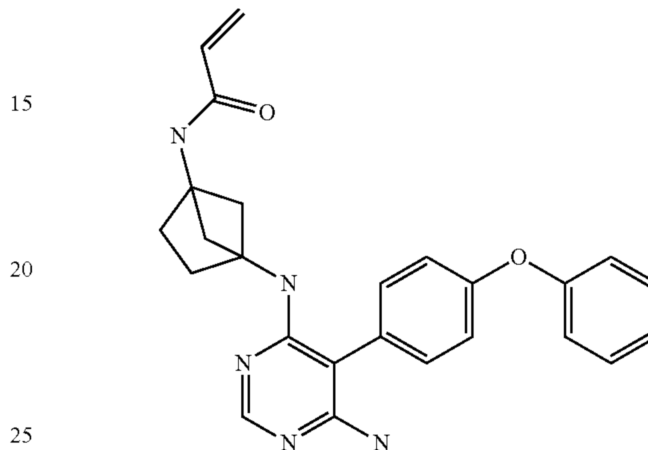
N-((1R,3S)-3-((6-amino-5-(4-phenoxyphenyl)pyrimidin-4-yl)amino)cyclohexyl)acrylamide (A174)
