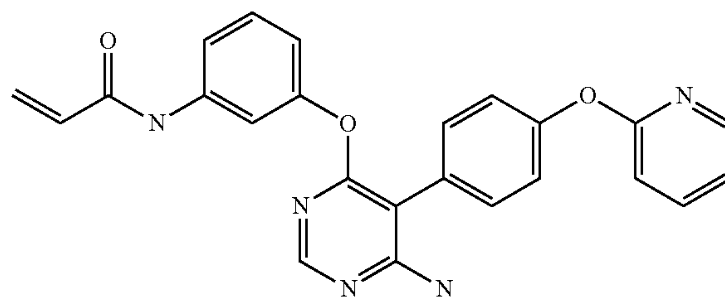
N-(3-((6-amino-5-(4-(pyridin-2-yloxy)phenyl)pyrimidin-4-yl)oxy)phenyl)acrylamide (A162)
