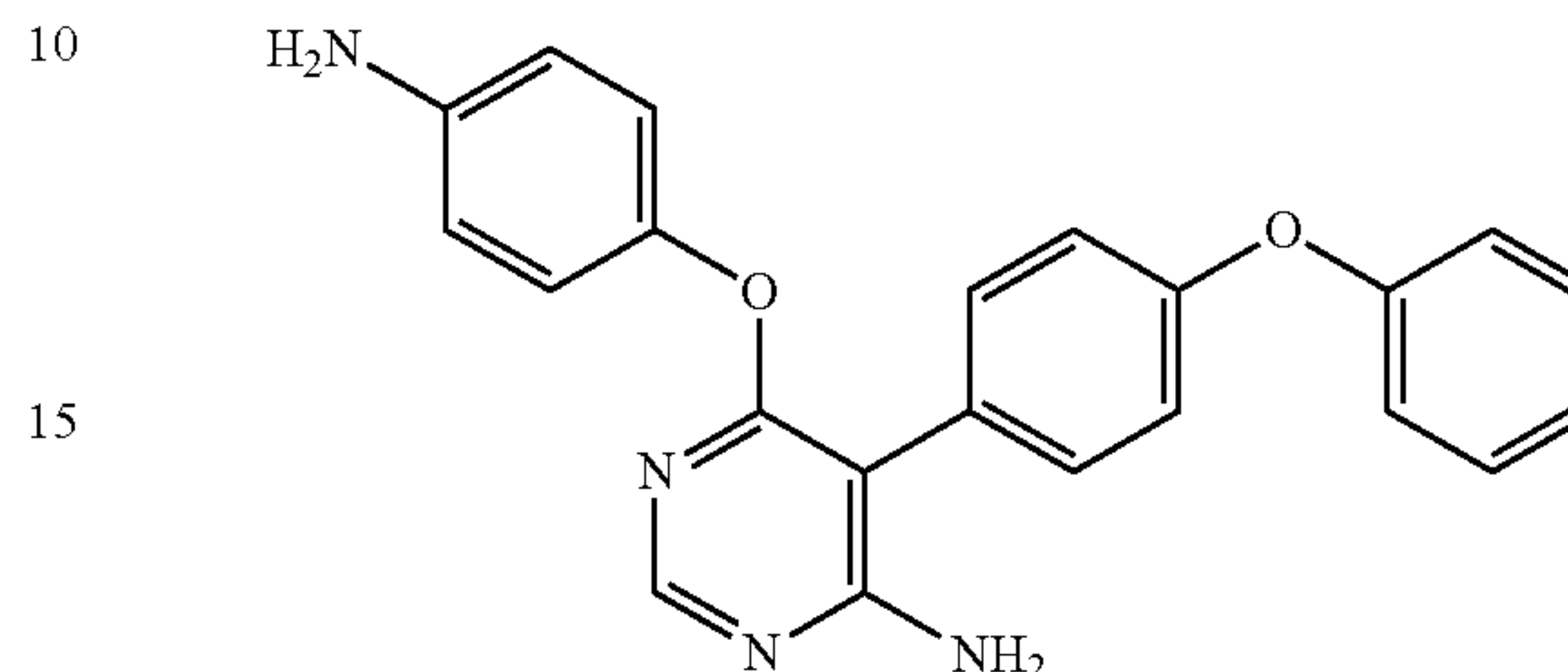
6-(4-aminophenoxy)-5-(4-phenoxyphenyl)pyrimidin-4-amine (A303)
