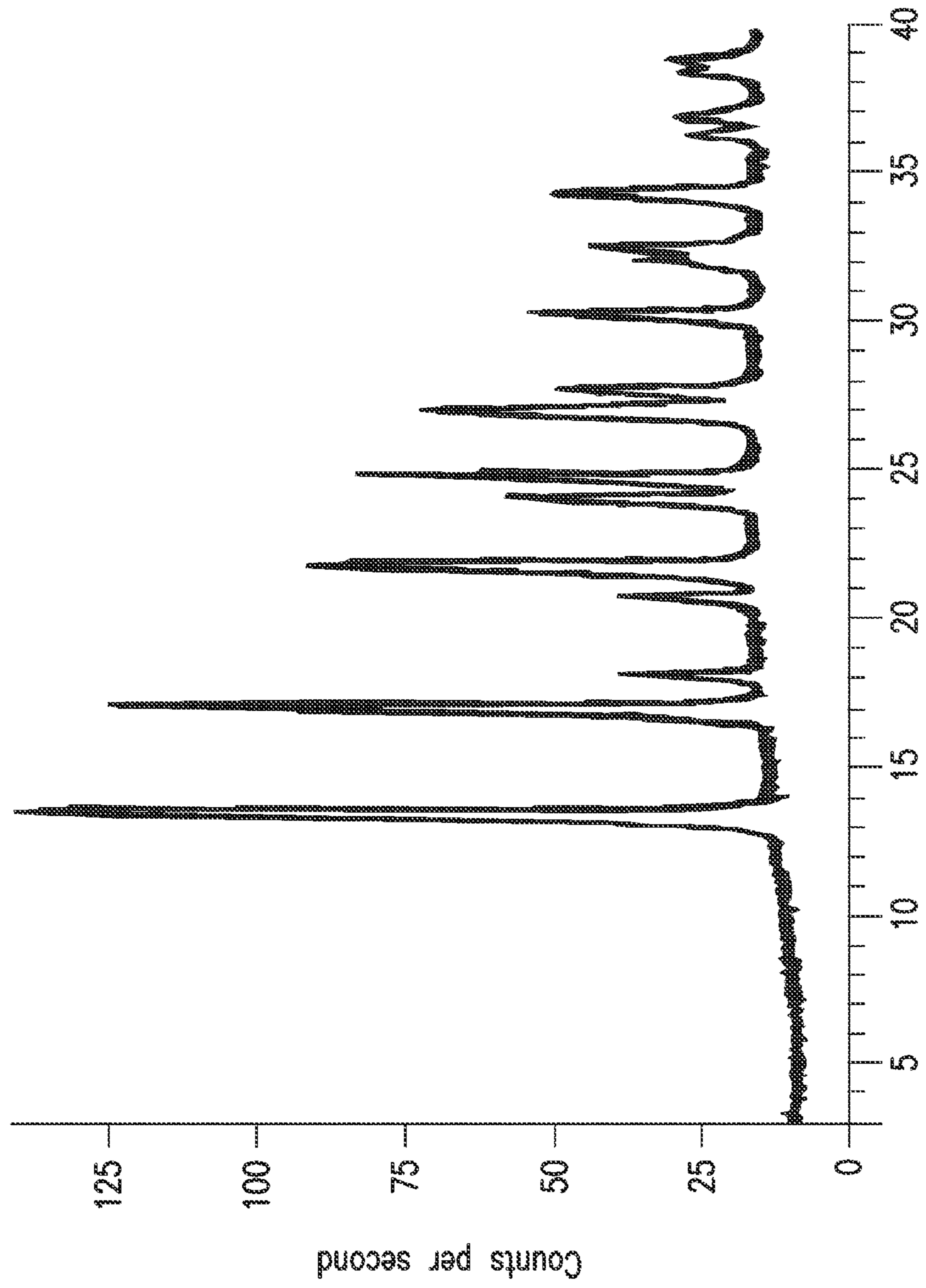
Degrees 2 theta
