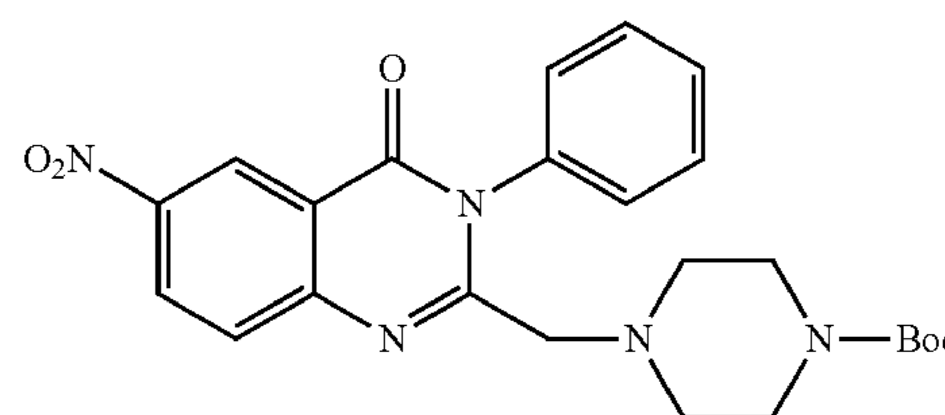
tert-Butyl 4-((6-nitro-4-oxo-3-phenyl-3,4-dihydroquinazolin-2-yl)methyl)piperazine-1-carboxylate
