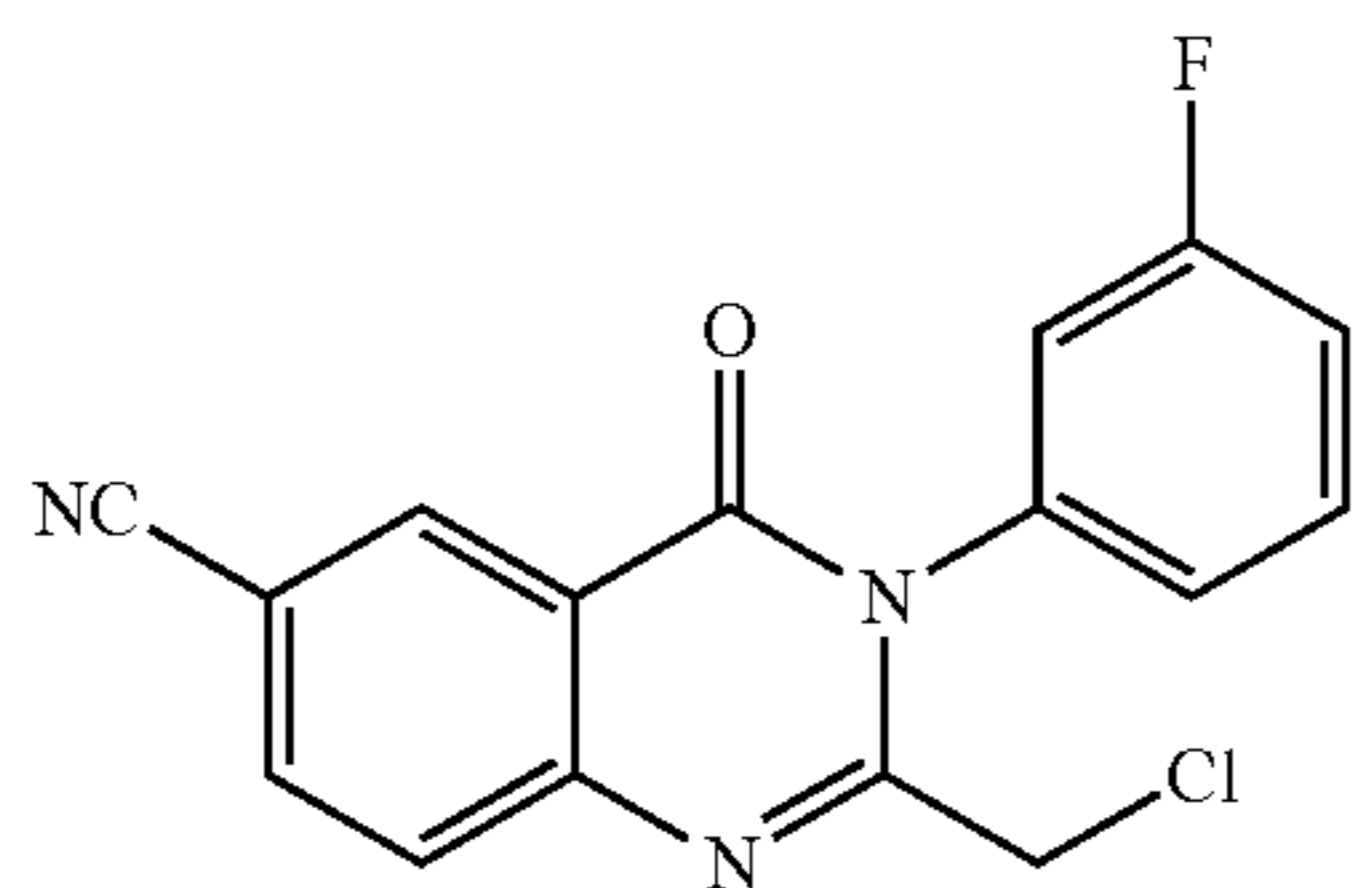
2-(chloromethyl)-3-(3-fluorophenyl)-4-oxo-3,4-dihydroquinazoline-6-carbonitrile
