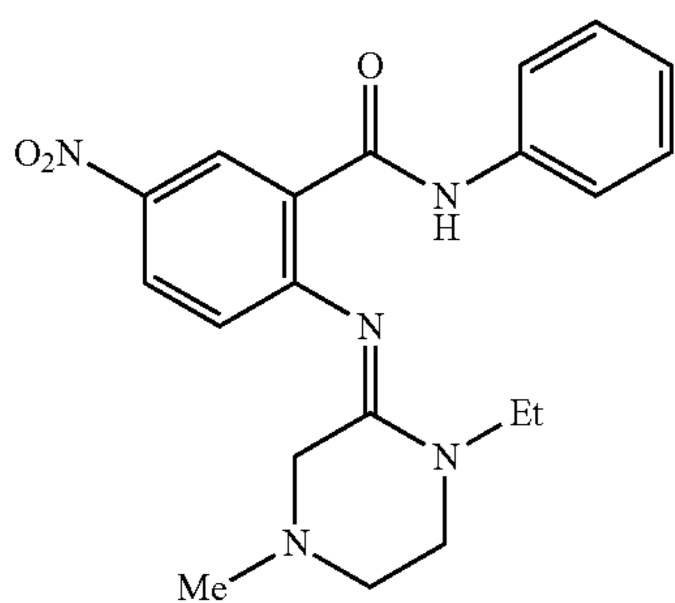
(E)-2-((1-ethyl-4-methylpiperazin-2-ylidene)amino)-5-nitro-N-phenylbenzamide
