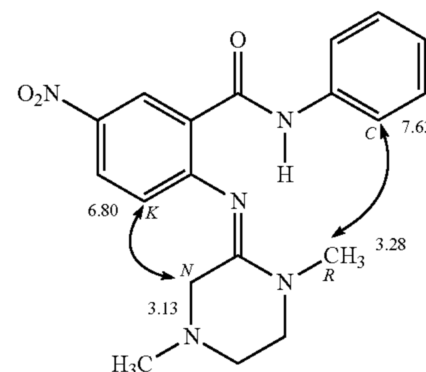
(E)-2-((1,4-dimethylpiperazin-2-ylidene)amino)-5-nitro-N-phenylbenzamide
