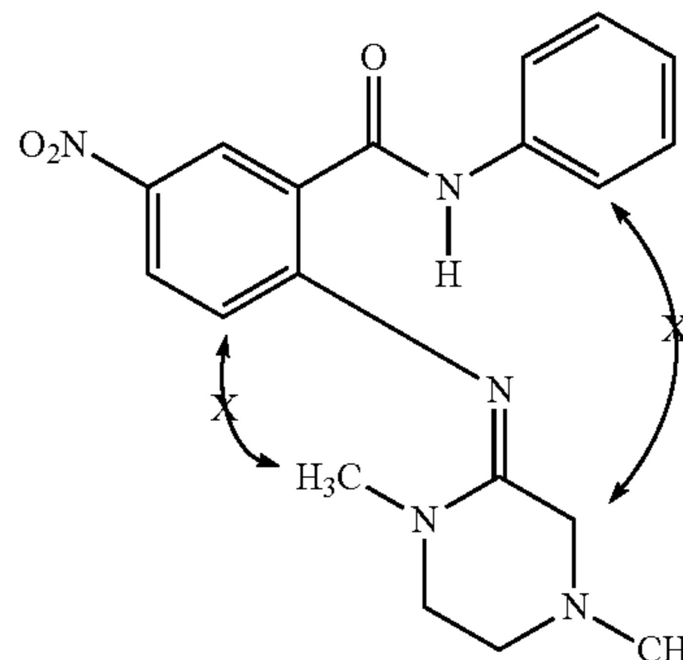
(Z)-2-((1,4-dimethylpiperazin-2-ylidene)amino)-5-nitro-N-phenylbenzamide
