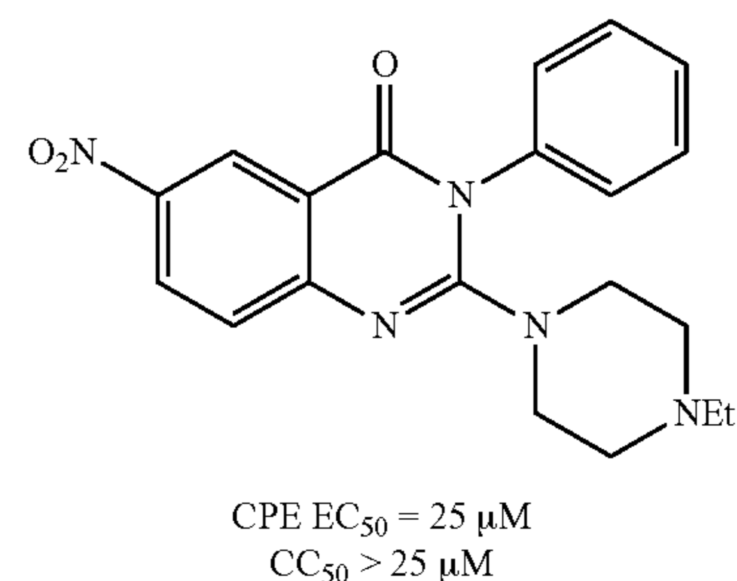
Scheme 4.
