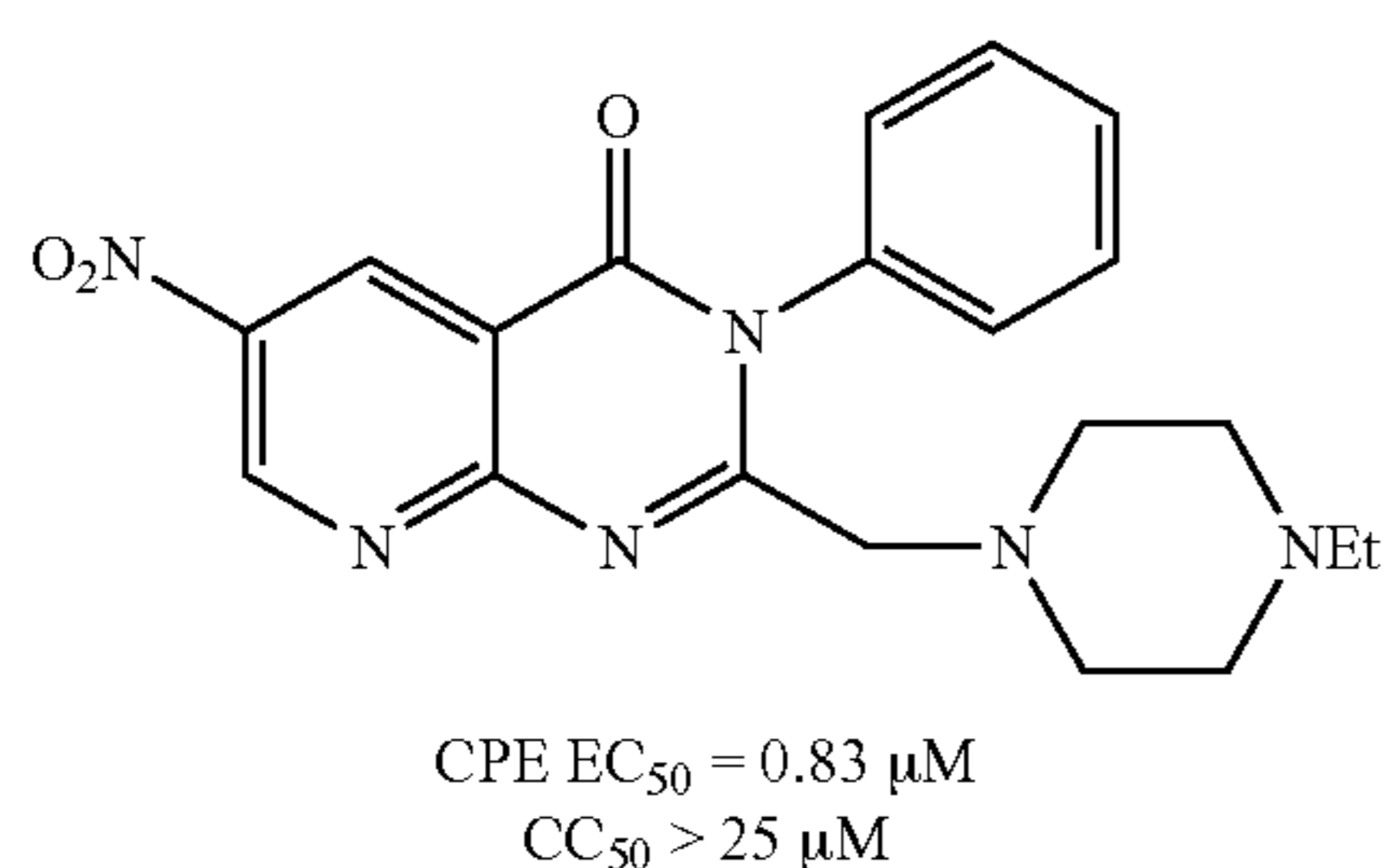
Scheme 3.
