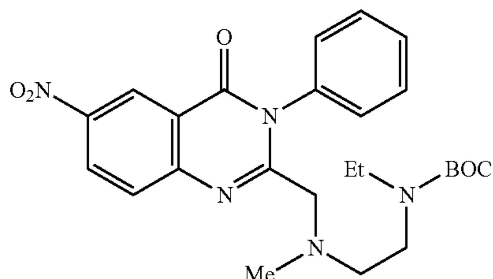
tert-Butyl ethyl(2-(methyl((6-nitro-4-oxo-3-phenyl-3,4-dihydroquinazolin-2-yl)methyl)amino)ethyl)carbamate
