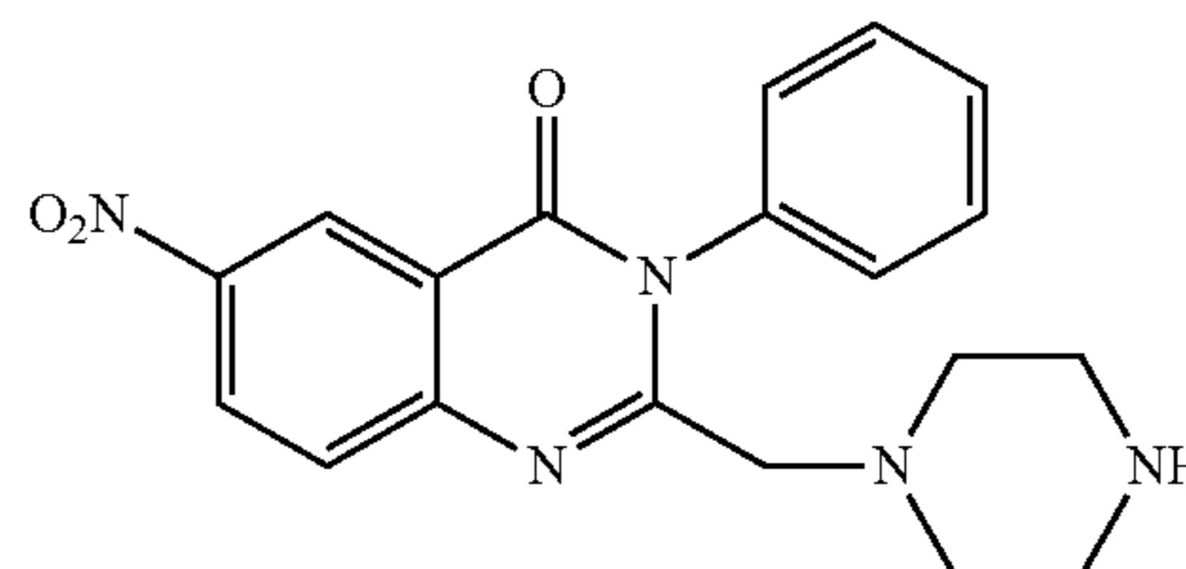
6-nitro-3-phenyl-2-(piperazin-1-ylmethyl)quinazolin-4(3H)-one
