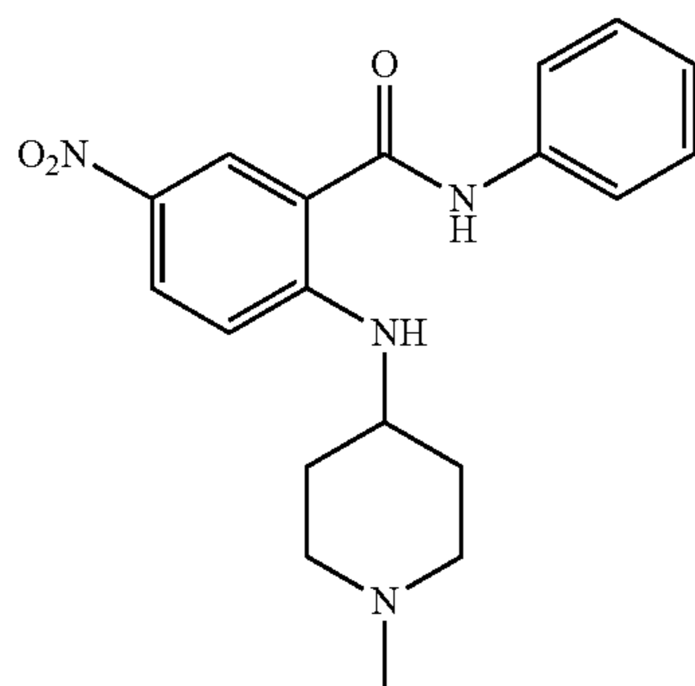
2-((1-methylpiperidin-4-yl)amino)-5-nitro-N-phenylbenzamide
