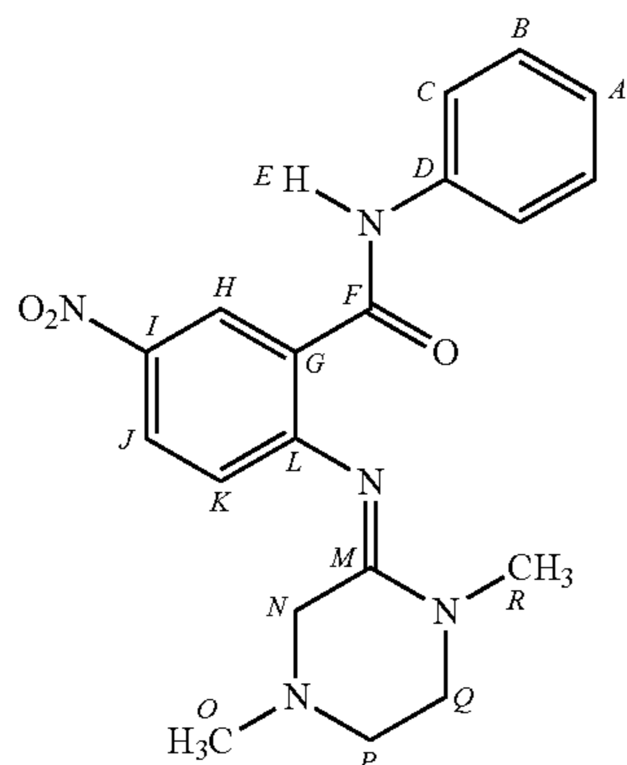
Diagram 1. Correlation assignments
