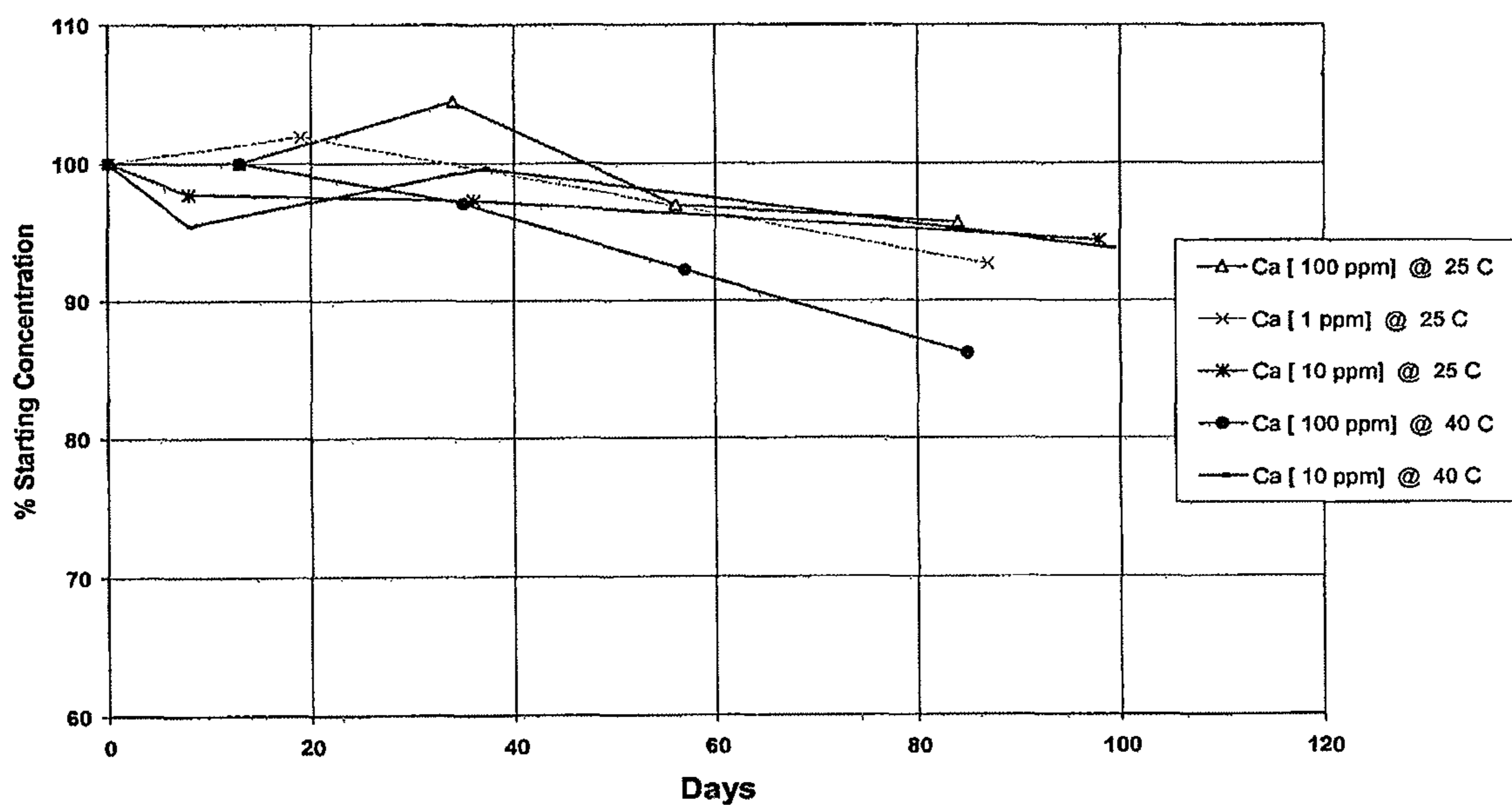
Figure 8 - Low Levels of CaCl2 in Deionized Water
