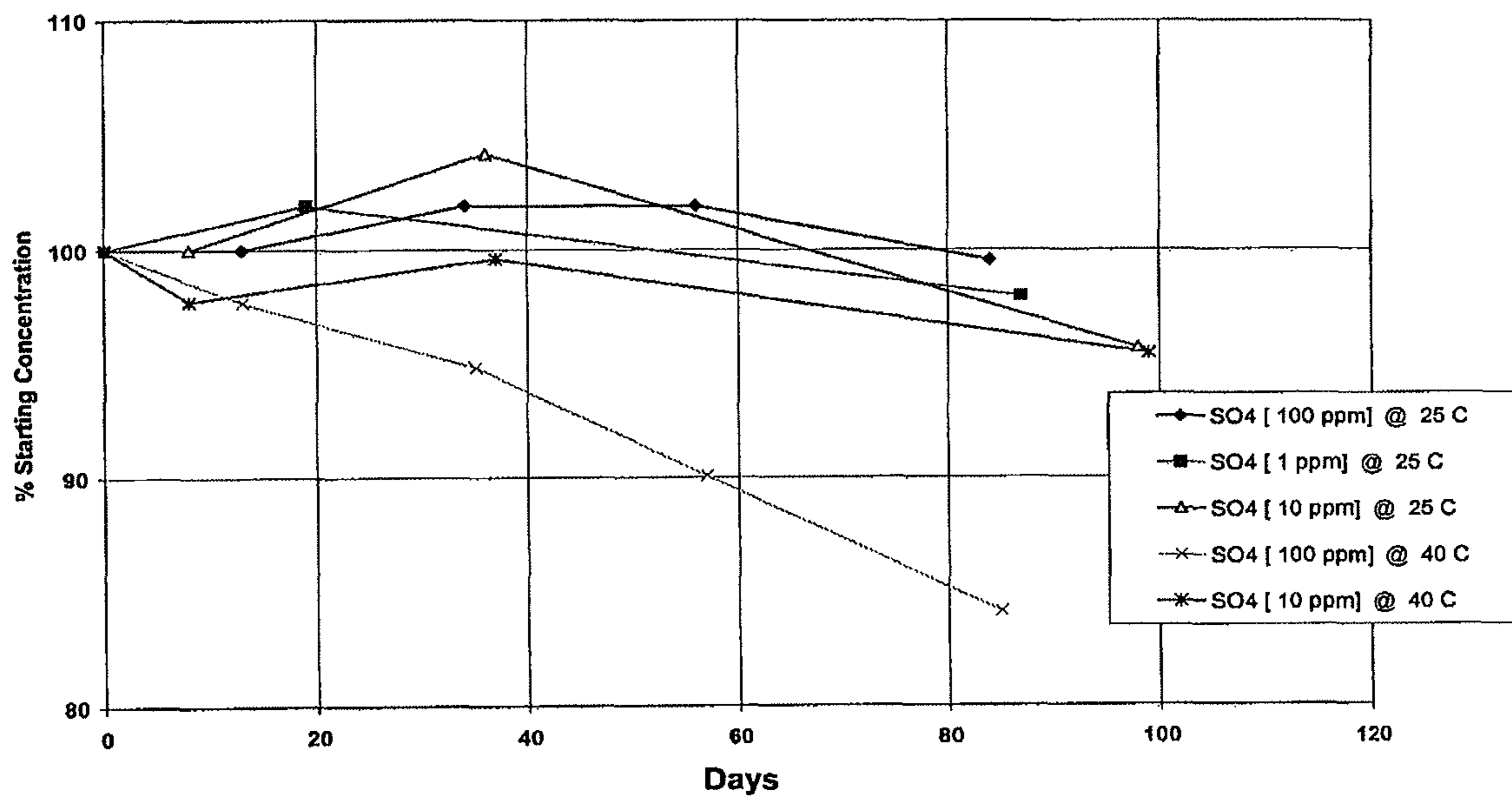
Figure 9 -Low Levels of Na 2 SO 4 in Deionized Water
