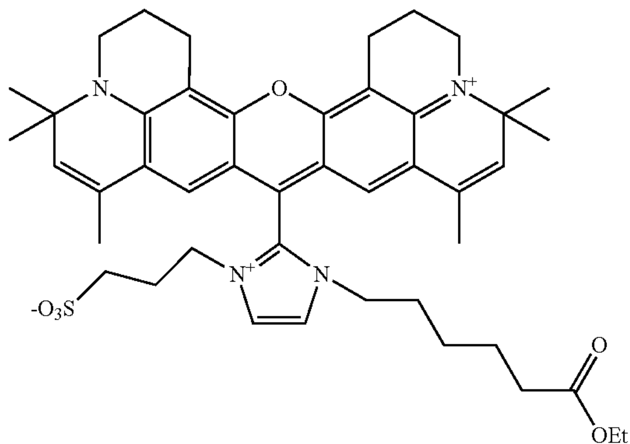
Compound No. 90
