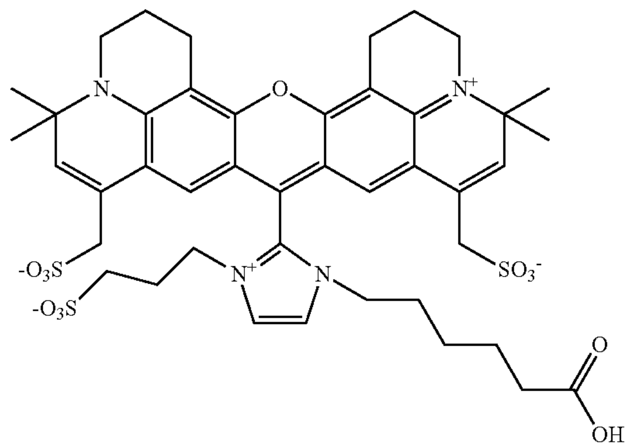
Compound No. 91
