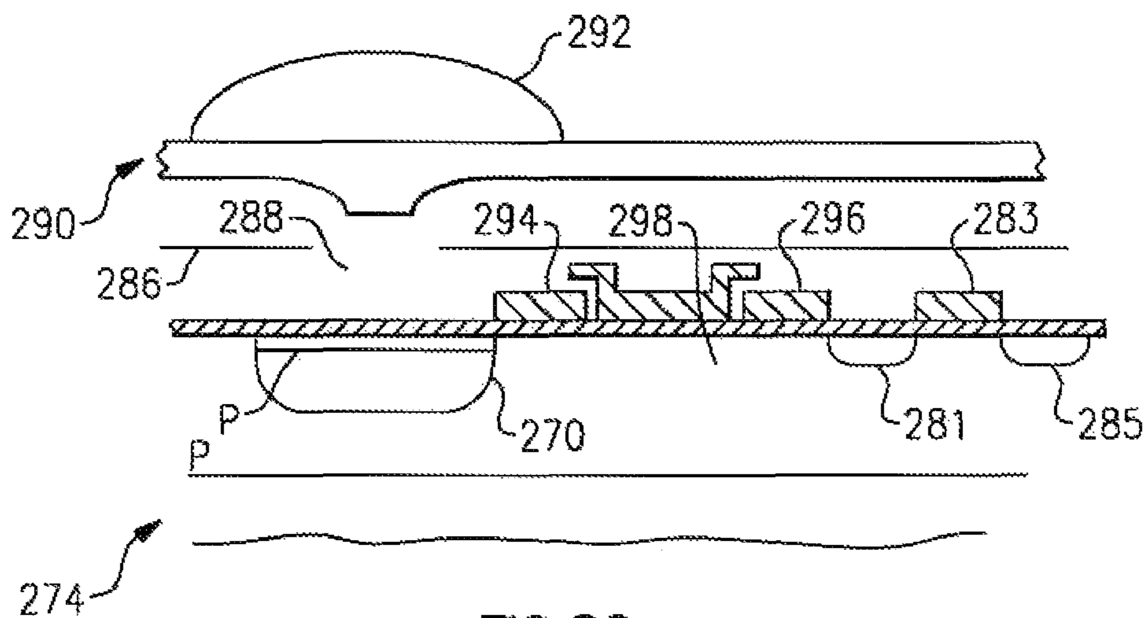
FIG. 8C Prior Art
