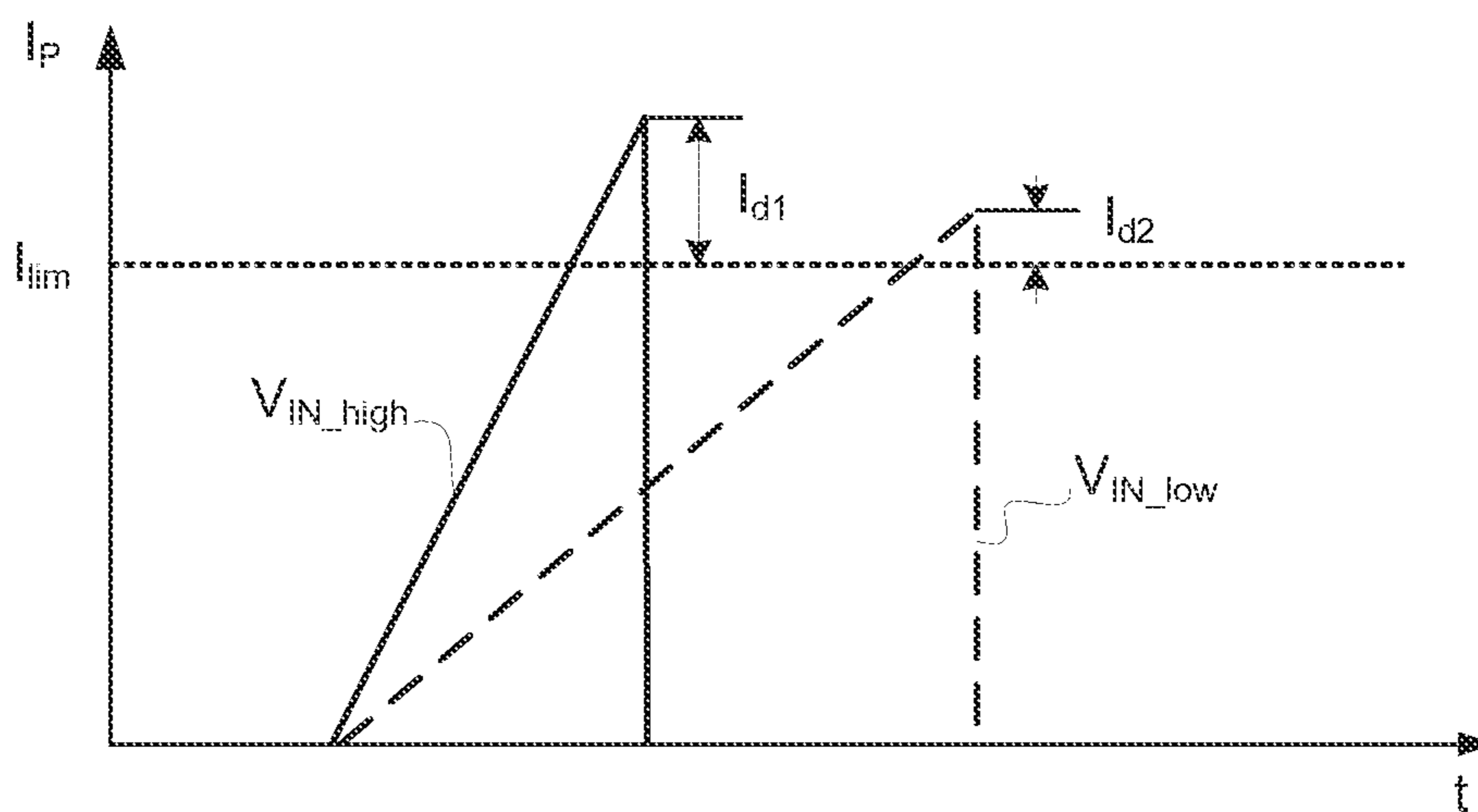
FIG. 9 (Prior Art)
