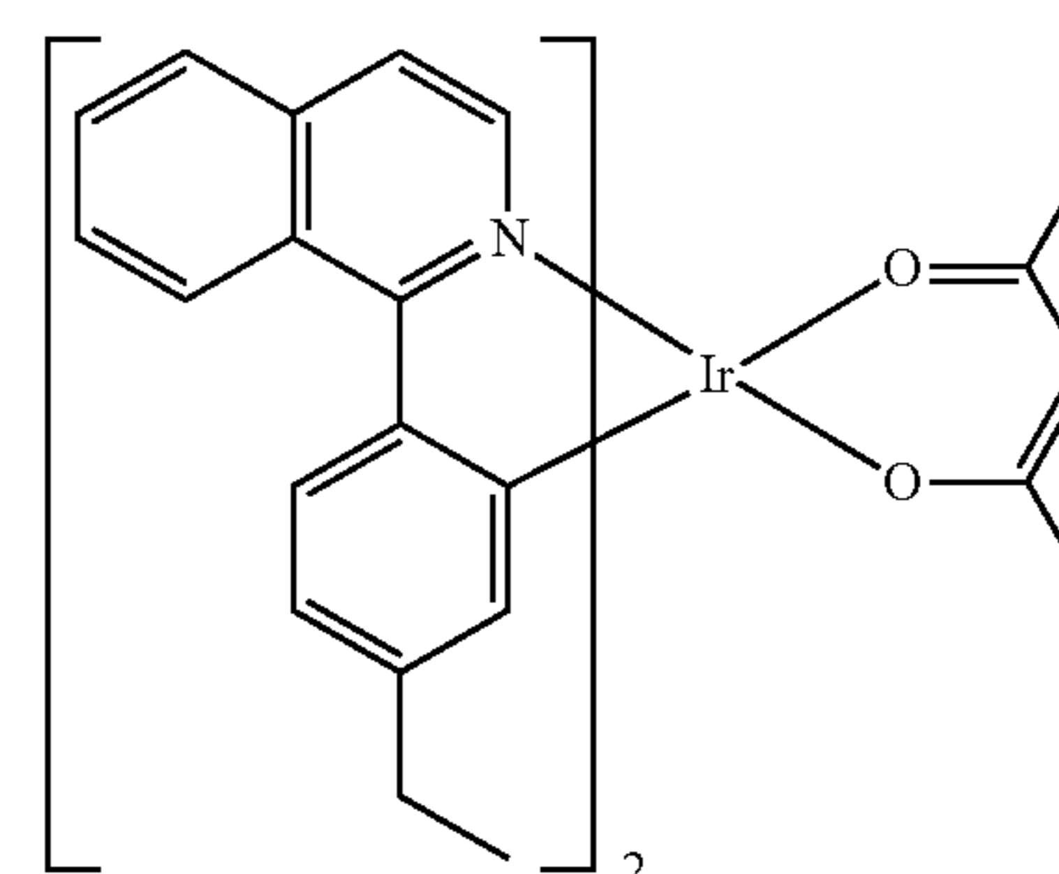
Compound 10
