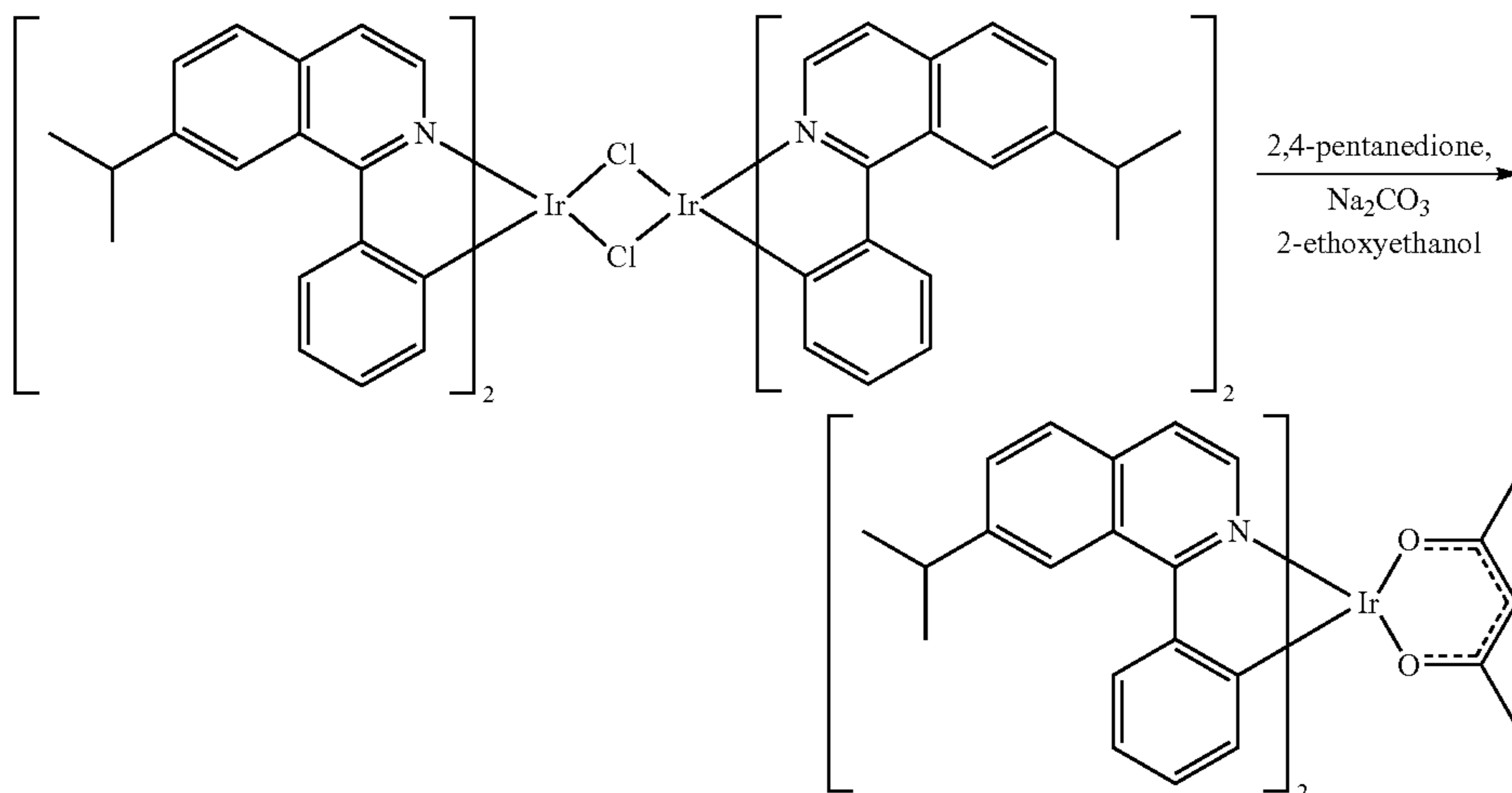
Compound 6
