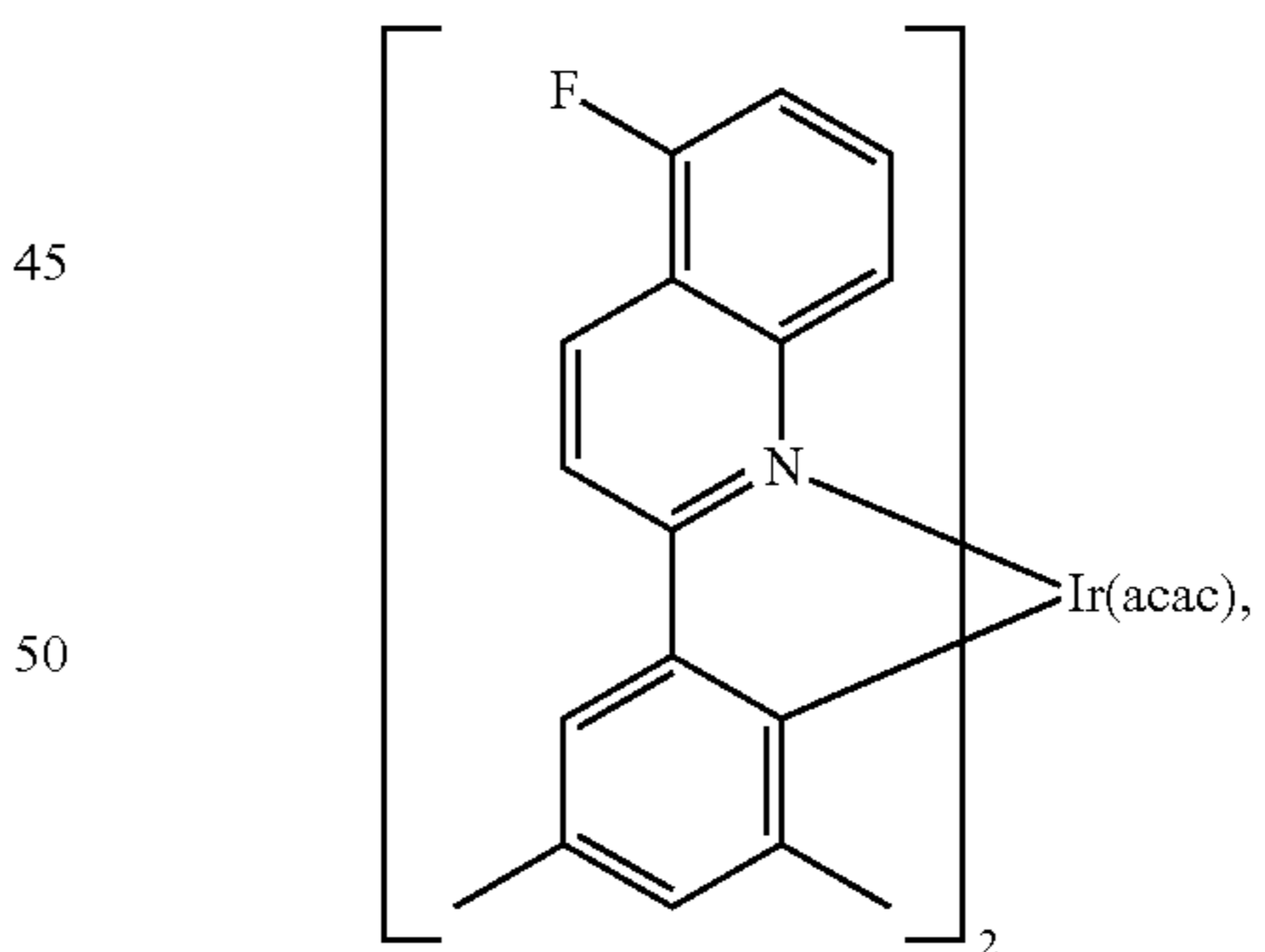
Compound 4
