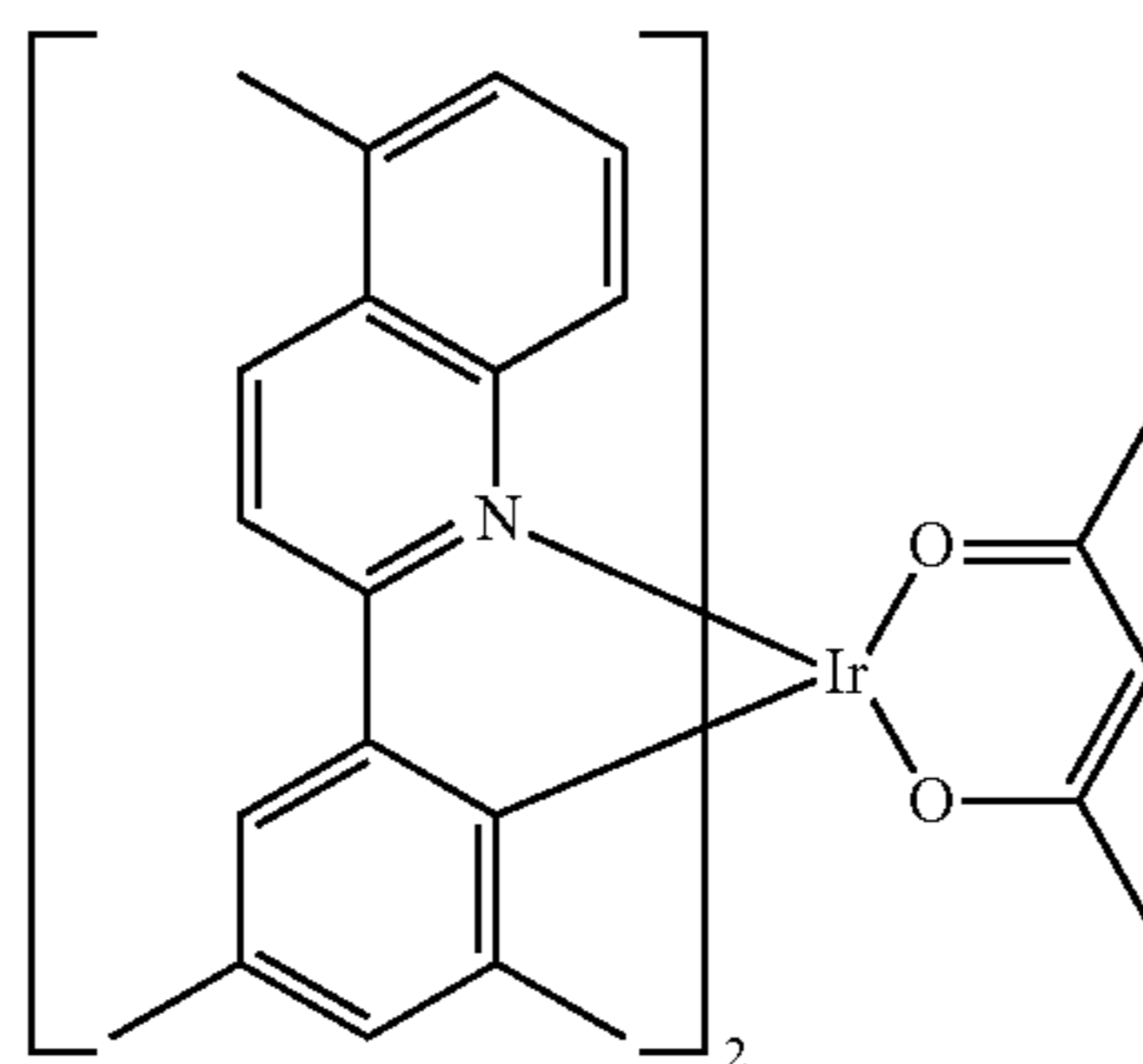
Compound 15
