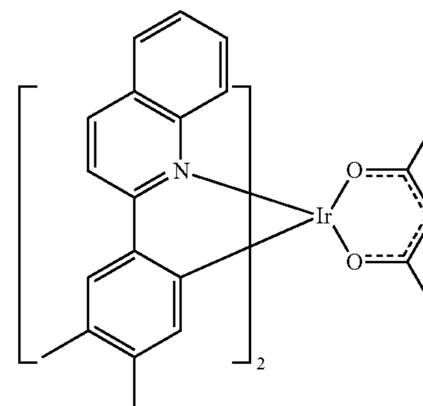
Compound 13
