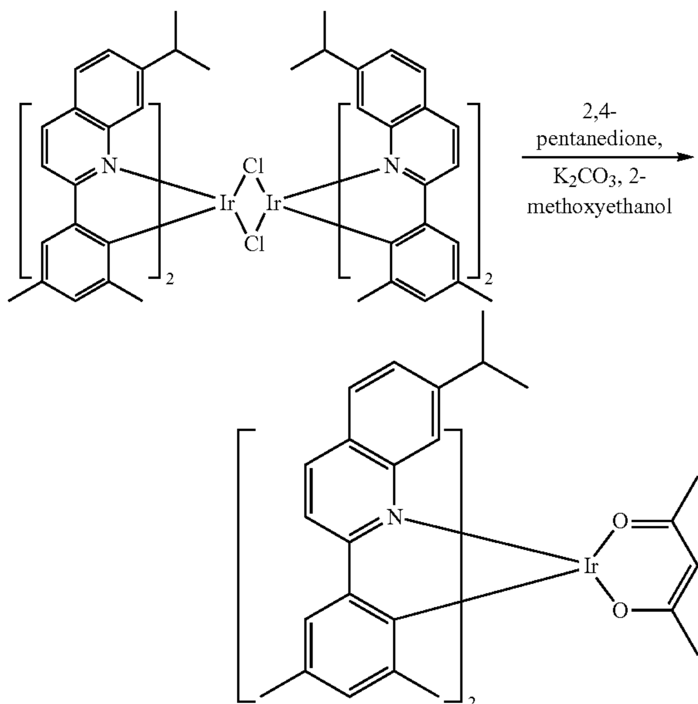
Compound 17
