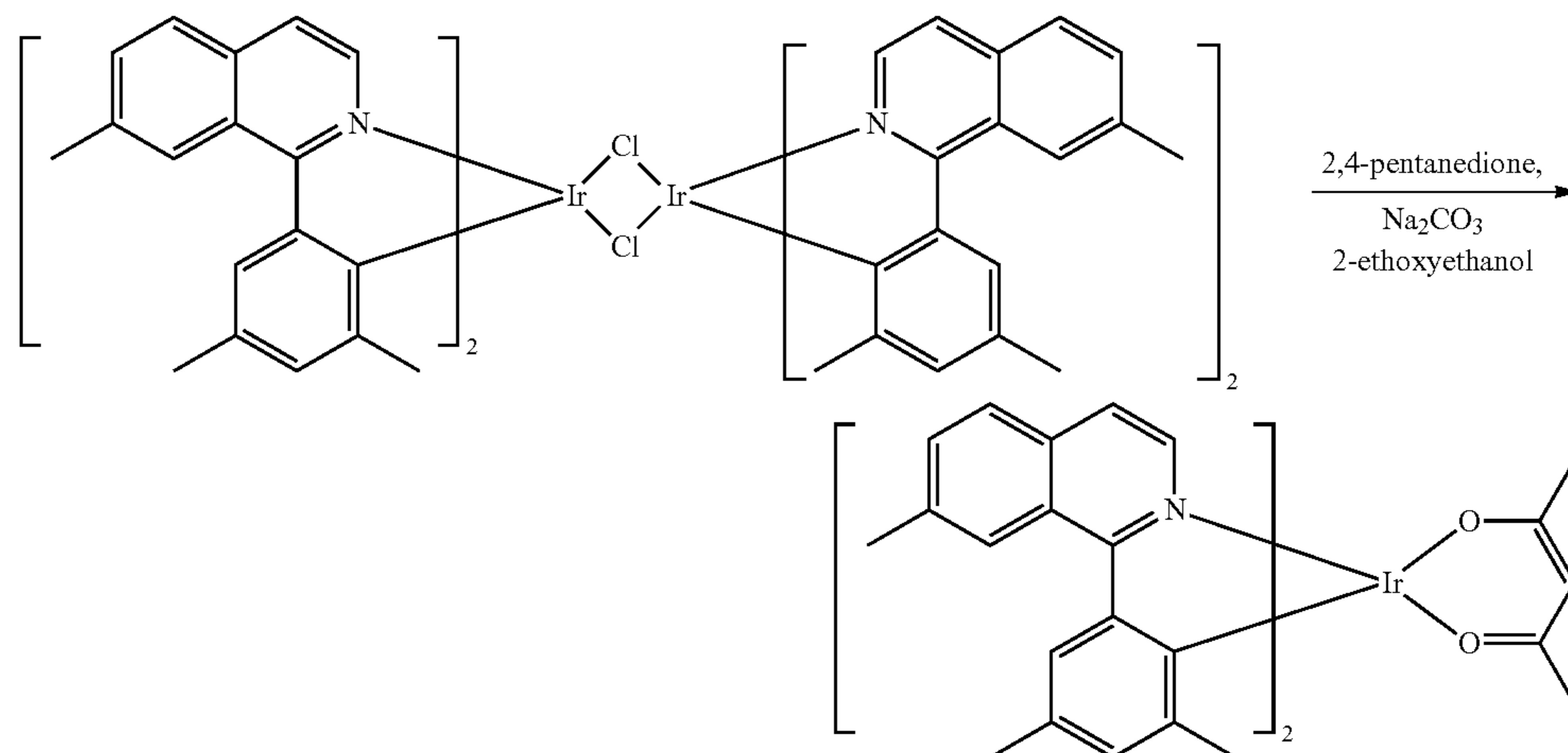
Compound 24
