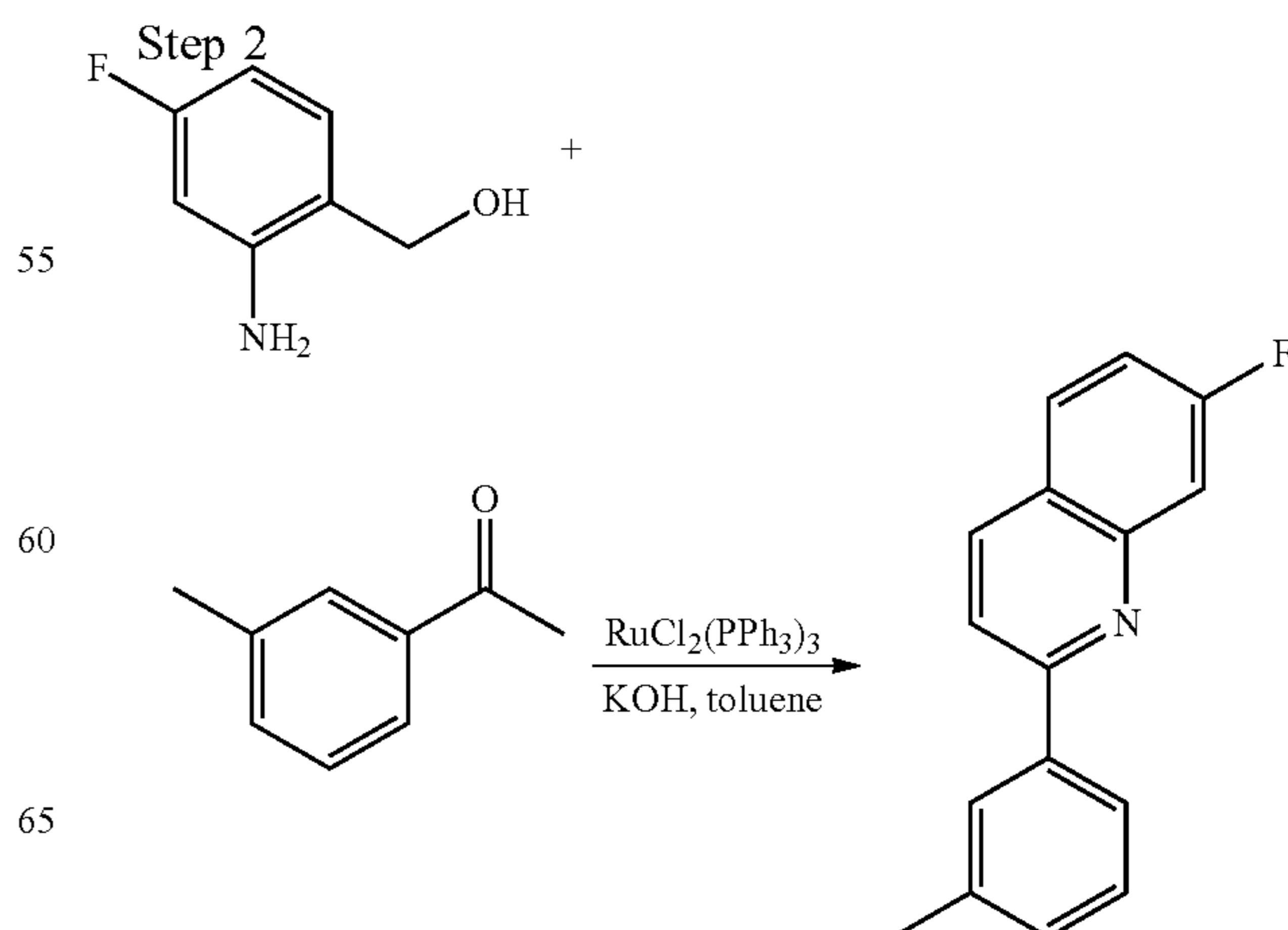
Compound 6
