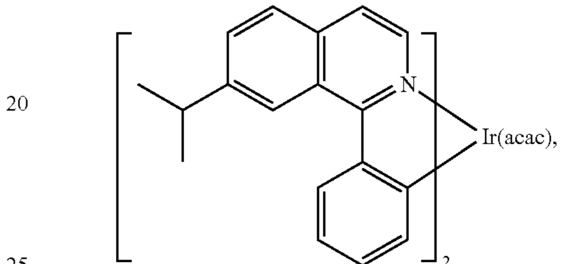
Compound 2
