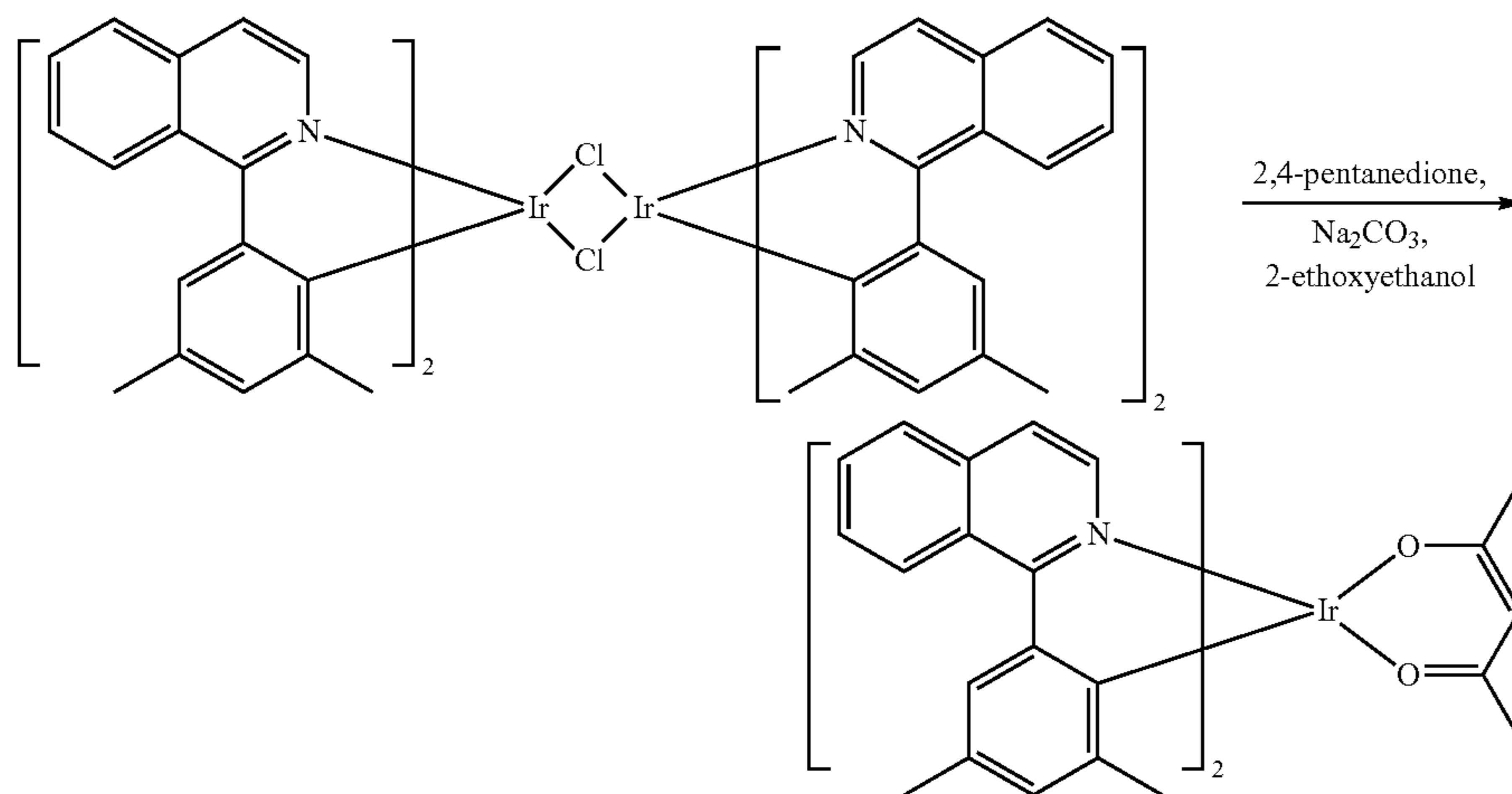
Compound 22
