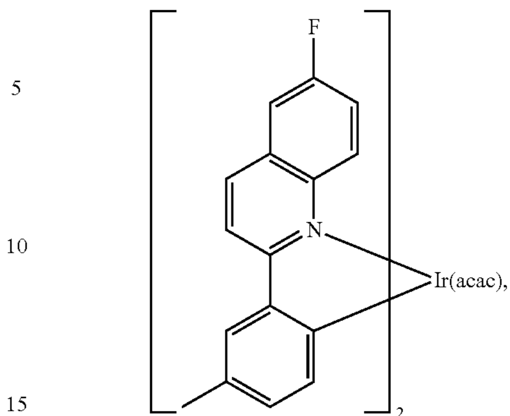
Compound 1
