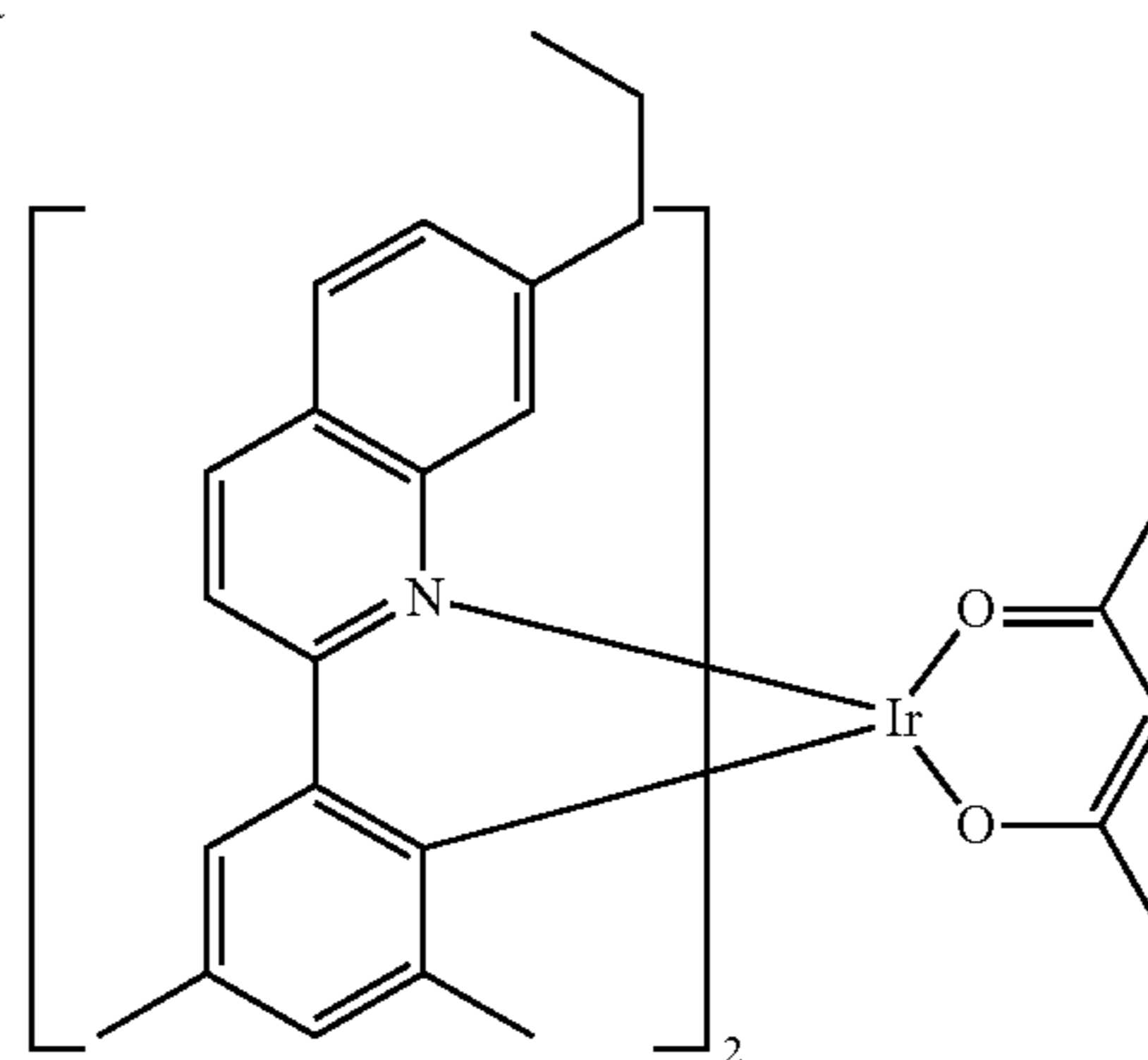
Compound 16
