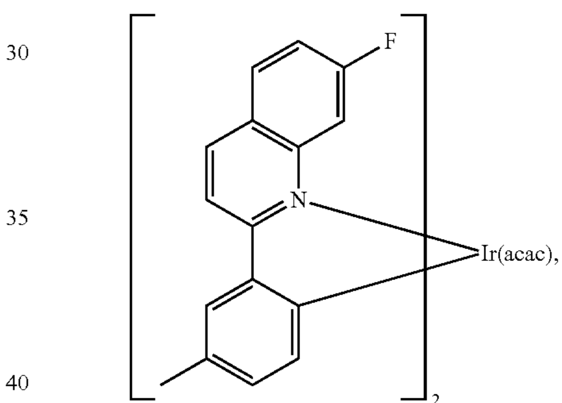
Compound 3
