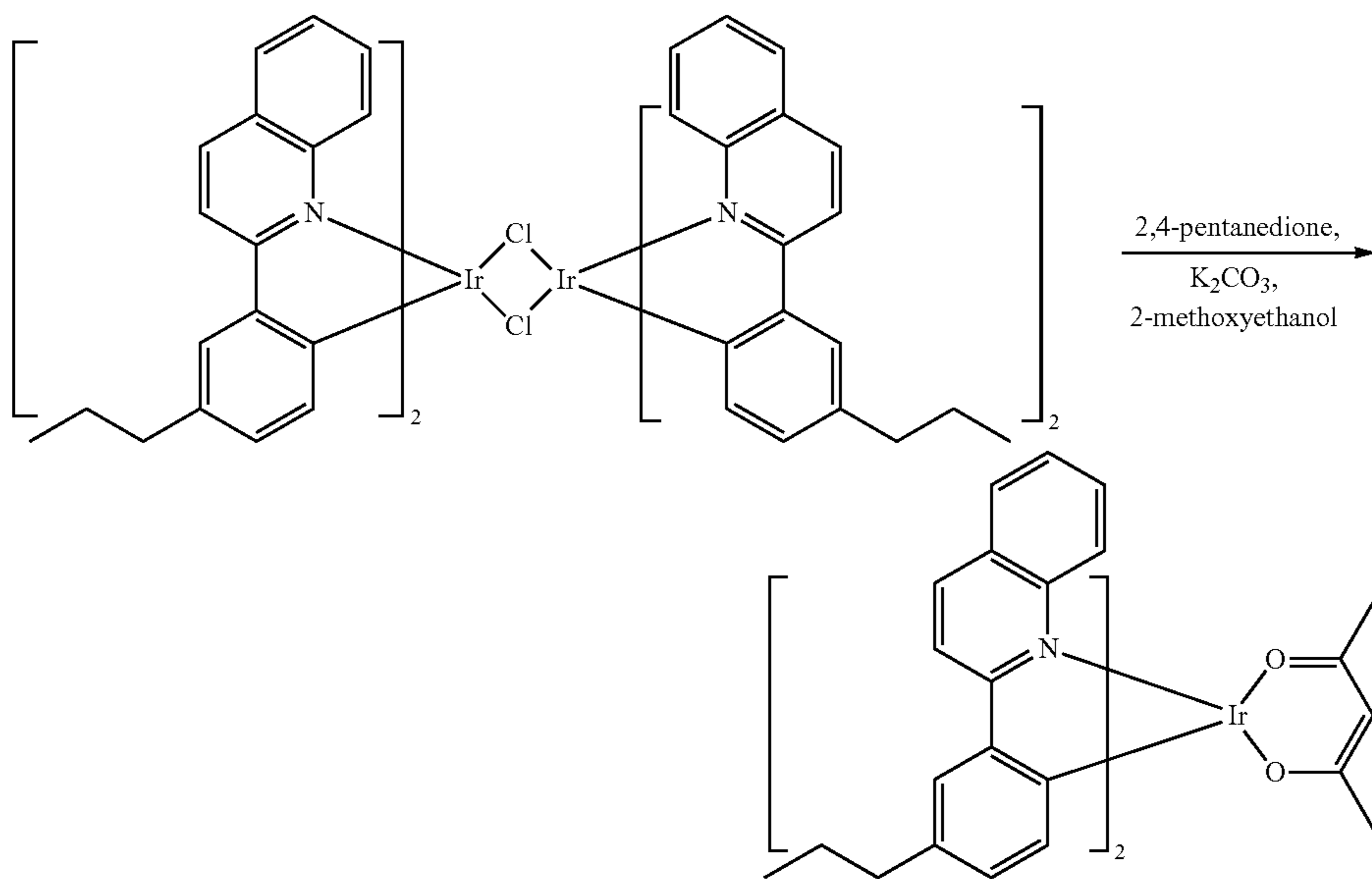
Compound 21
