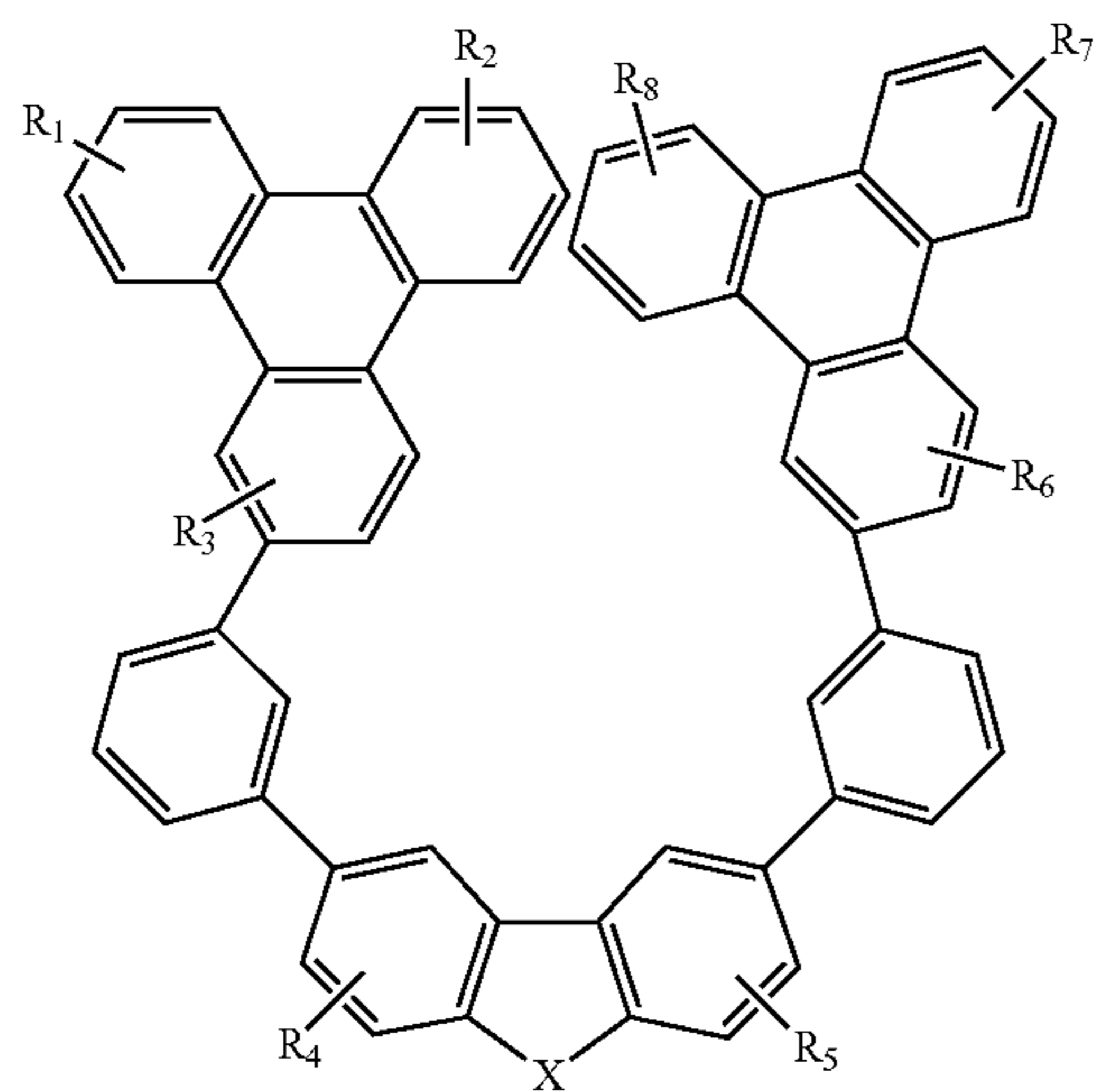
Compound 39G
