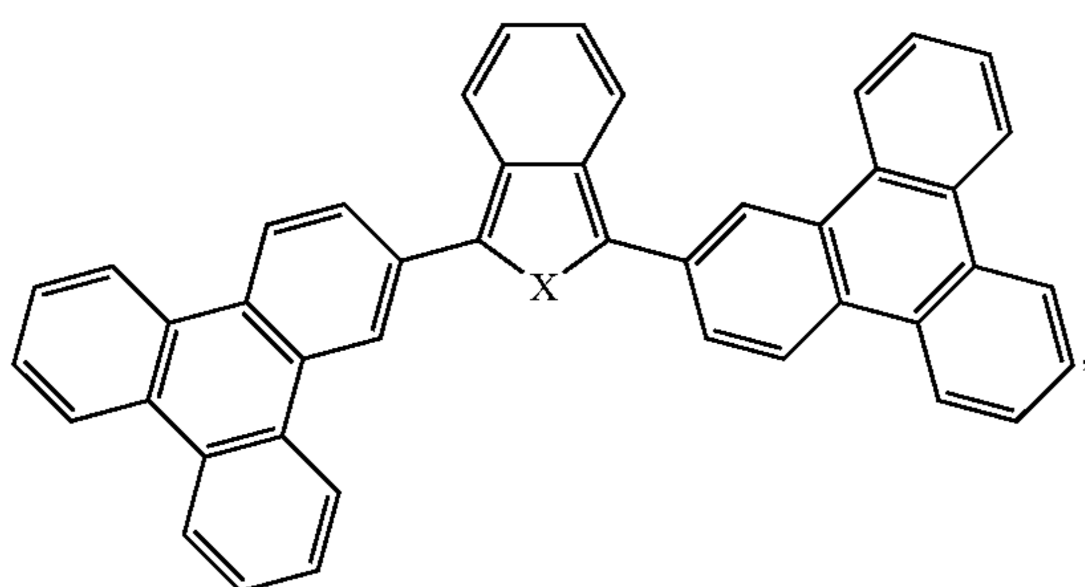
Compound 11
