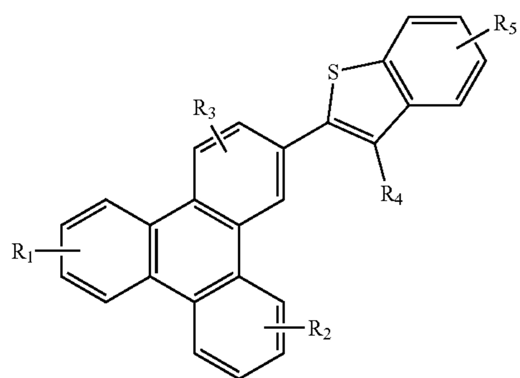
Compound 14'G
