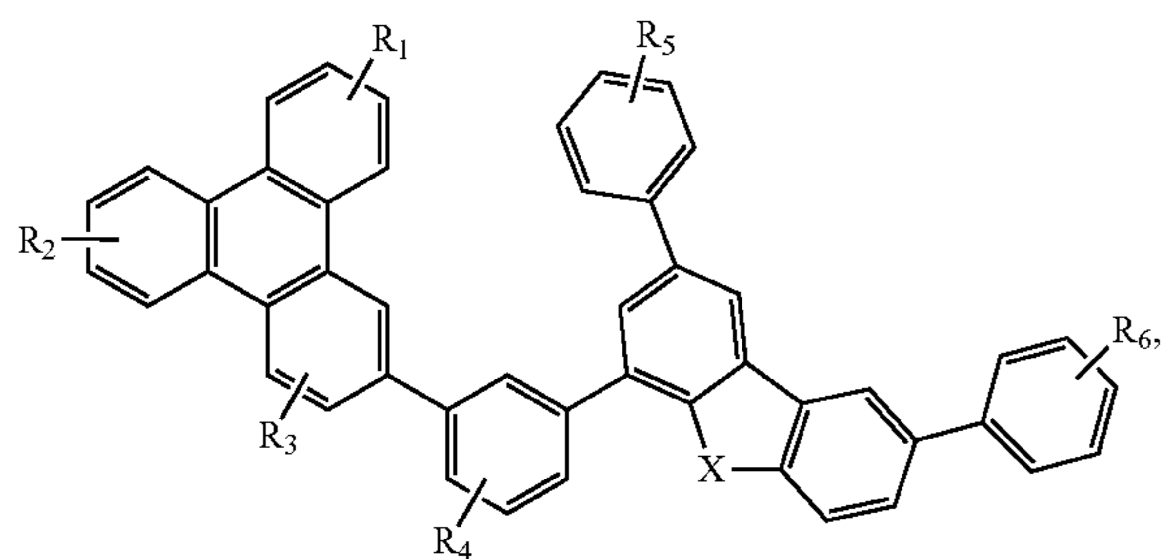
Compound 24G
