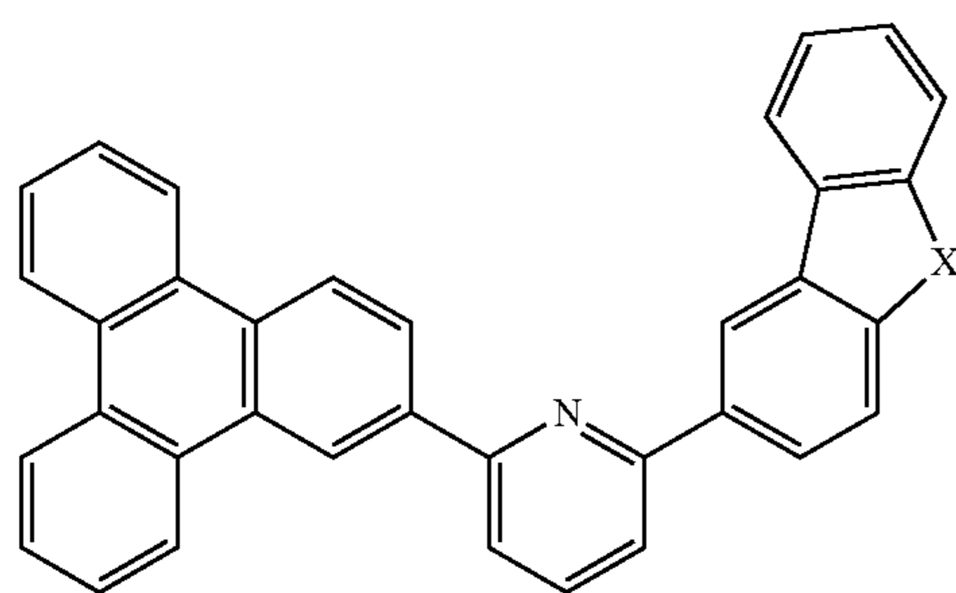
Compound 44 G
