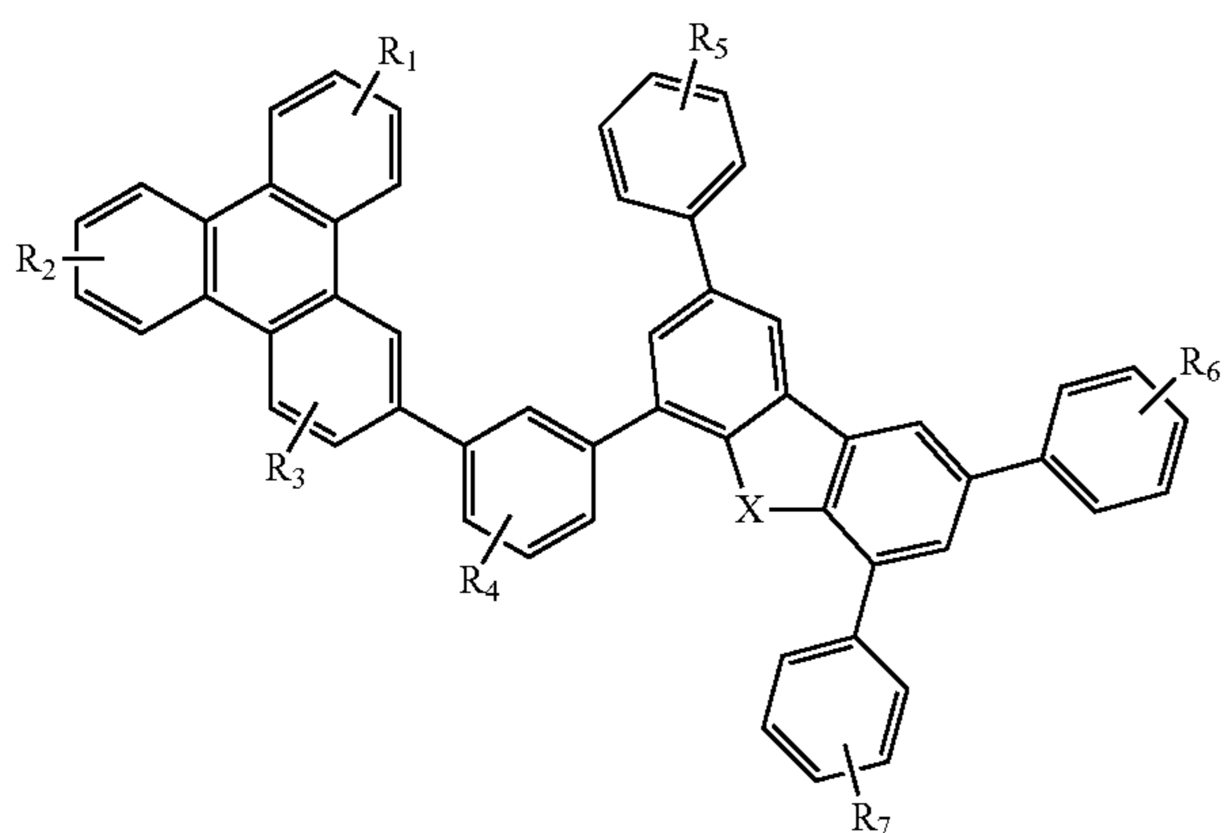
Compound 25 G
