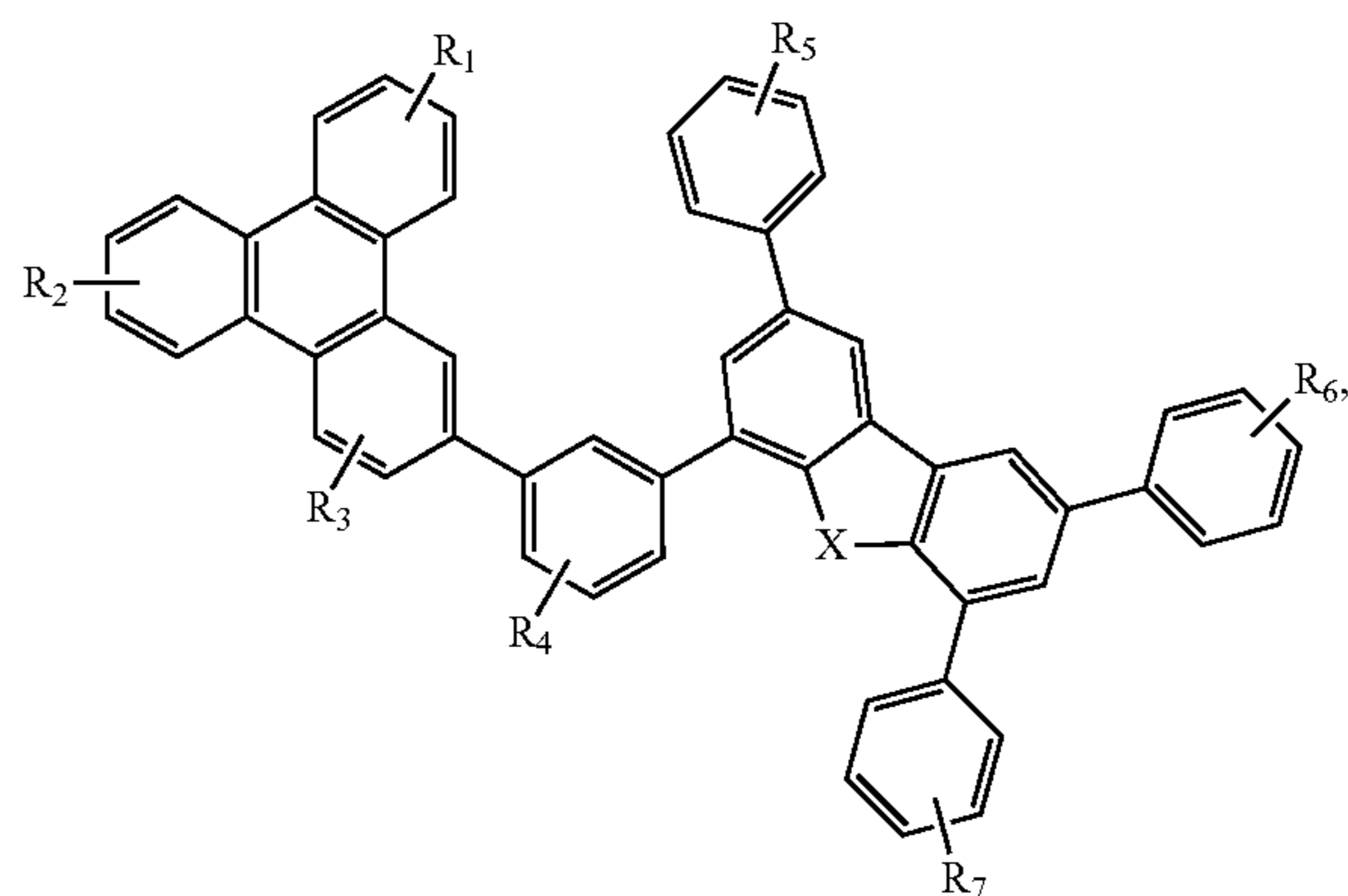
Compound 21G 55
