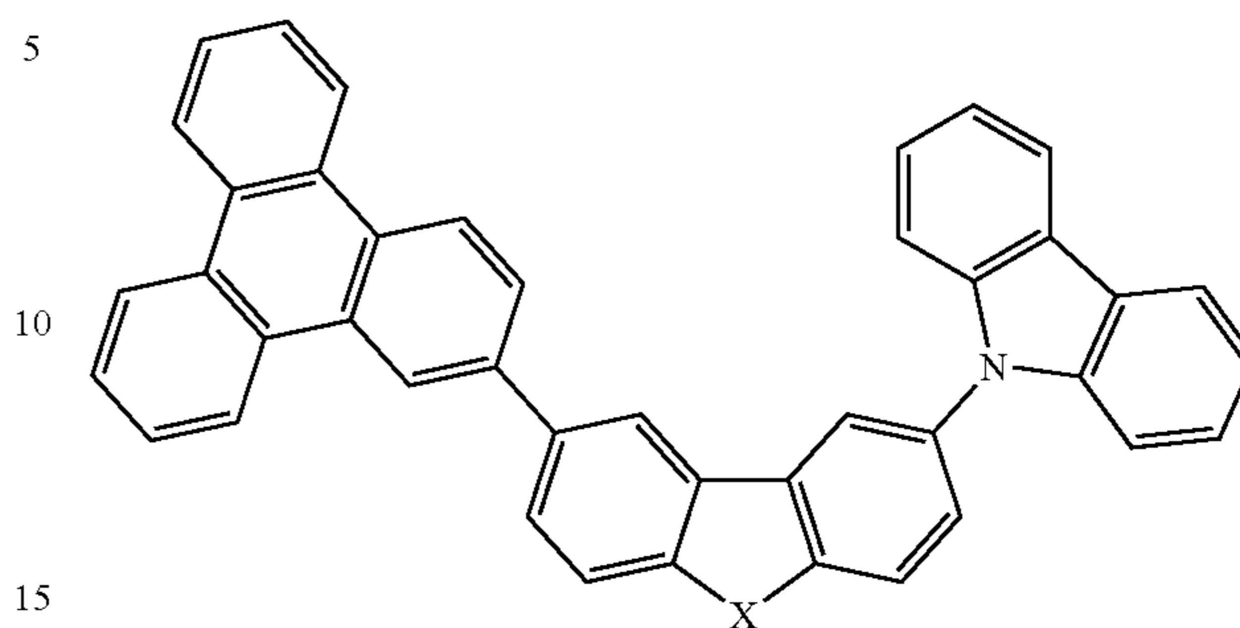
Compound 15
