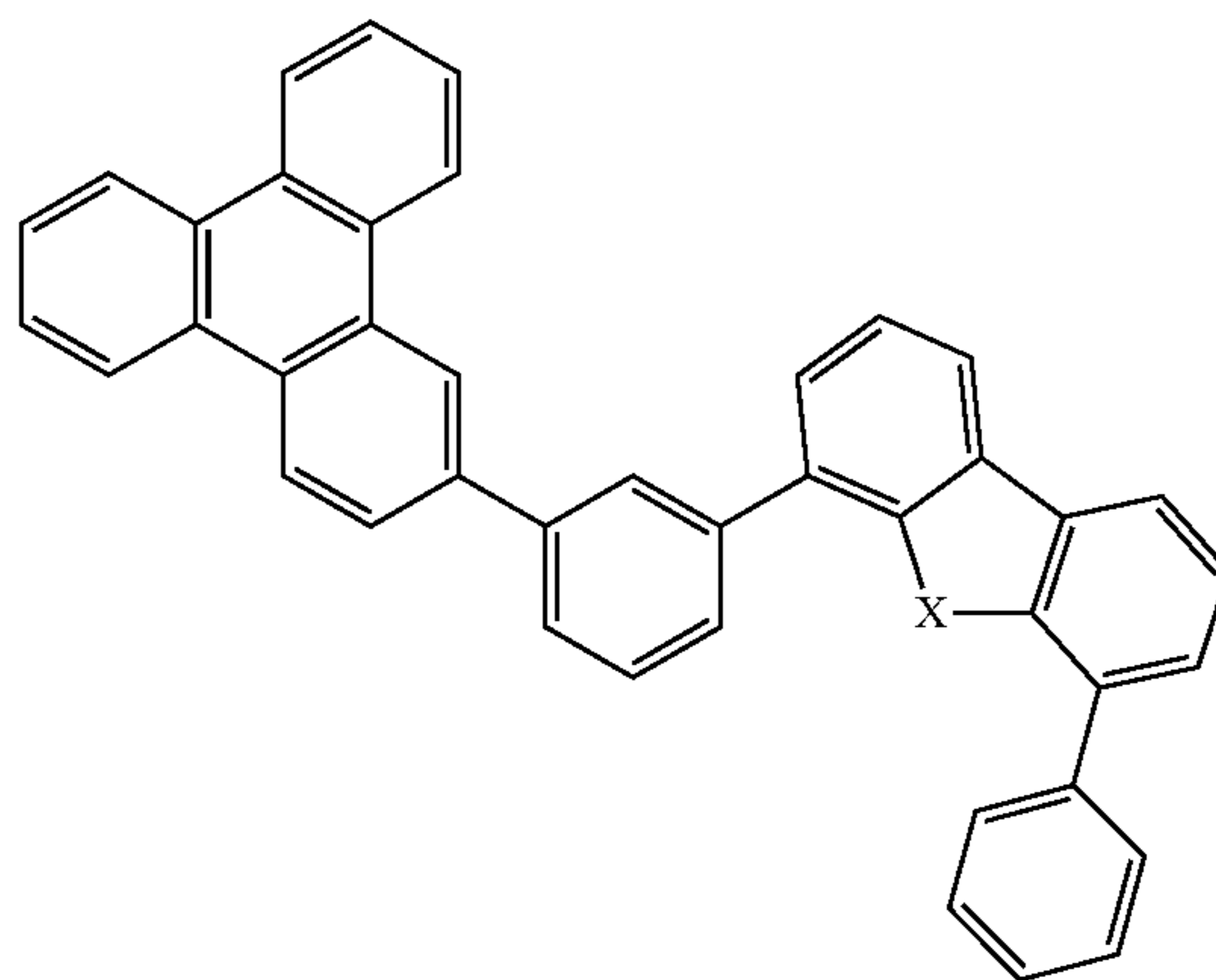
Compound 23
