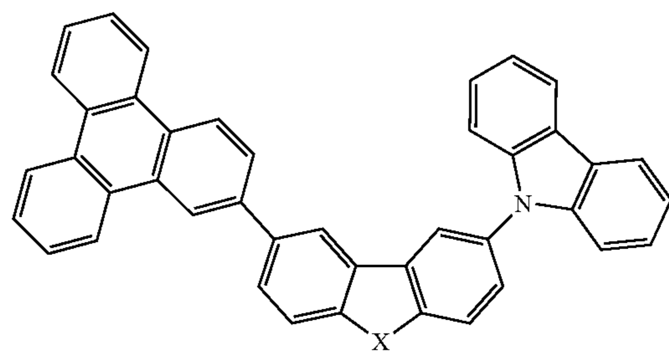
Compound 16
