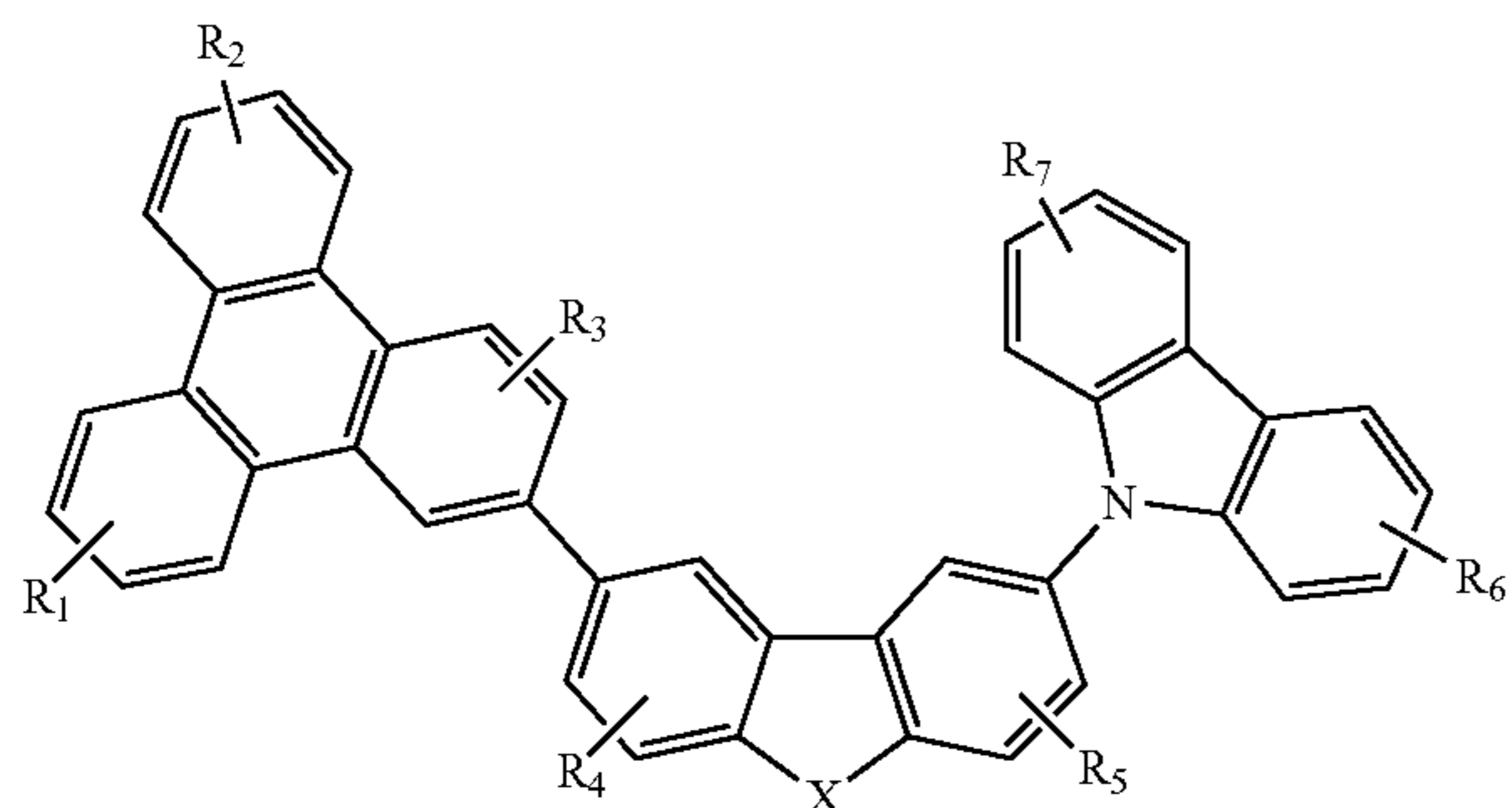
Compound 15G
