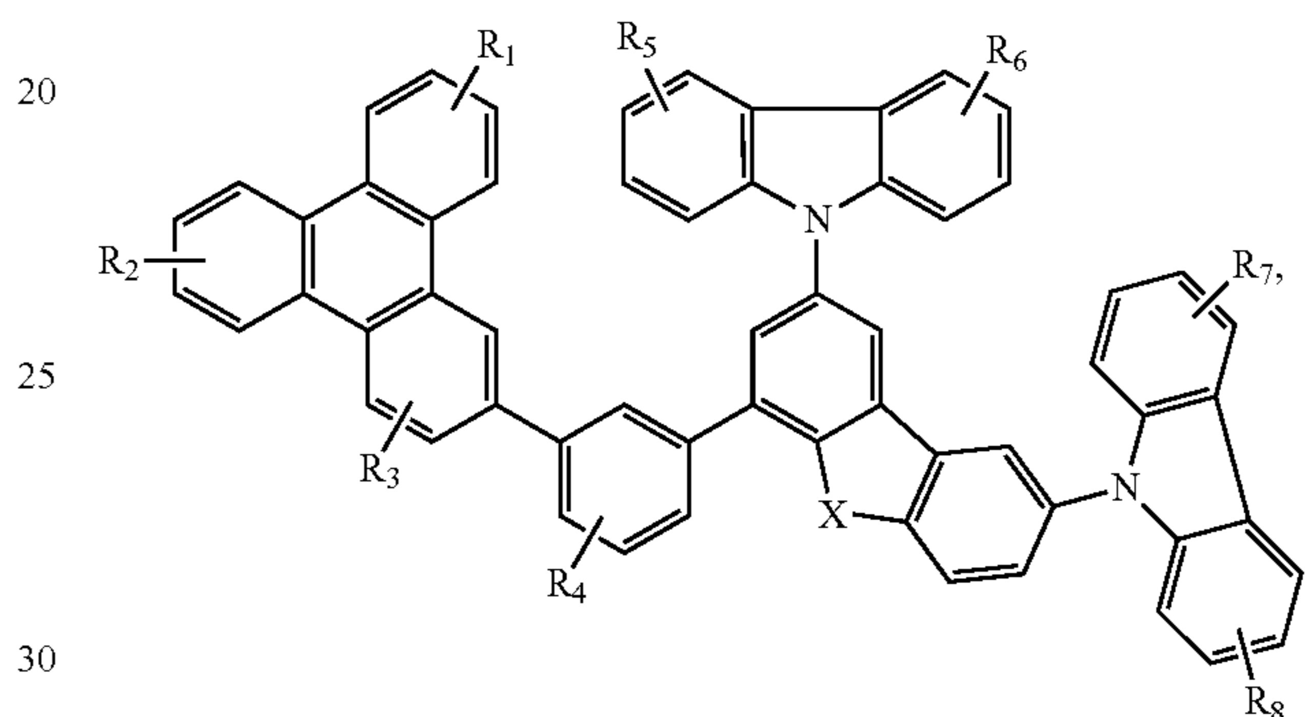
Compound 27G
