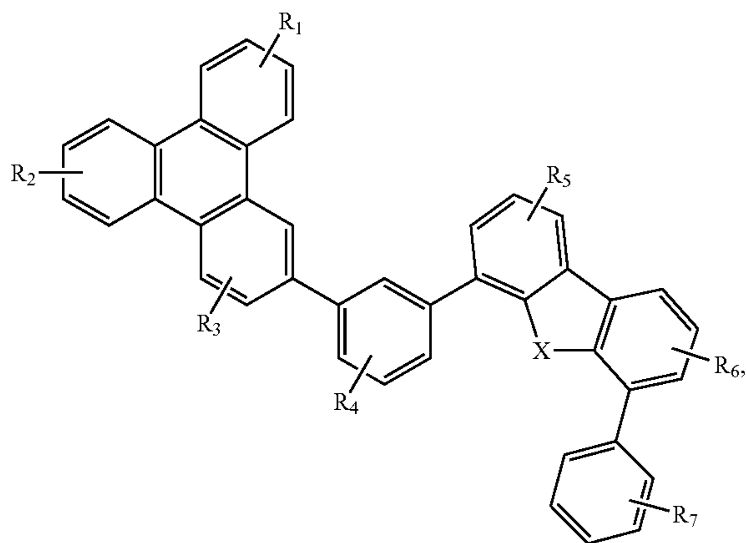
Compound 23G
