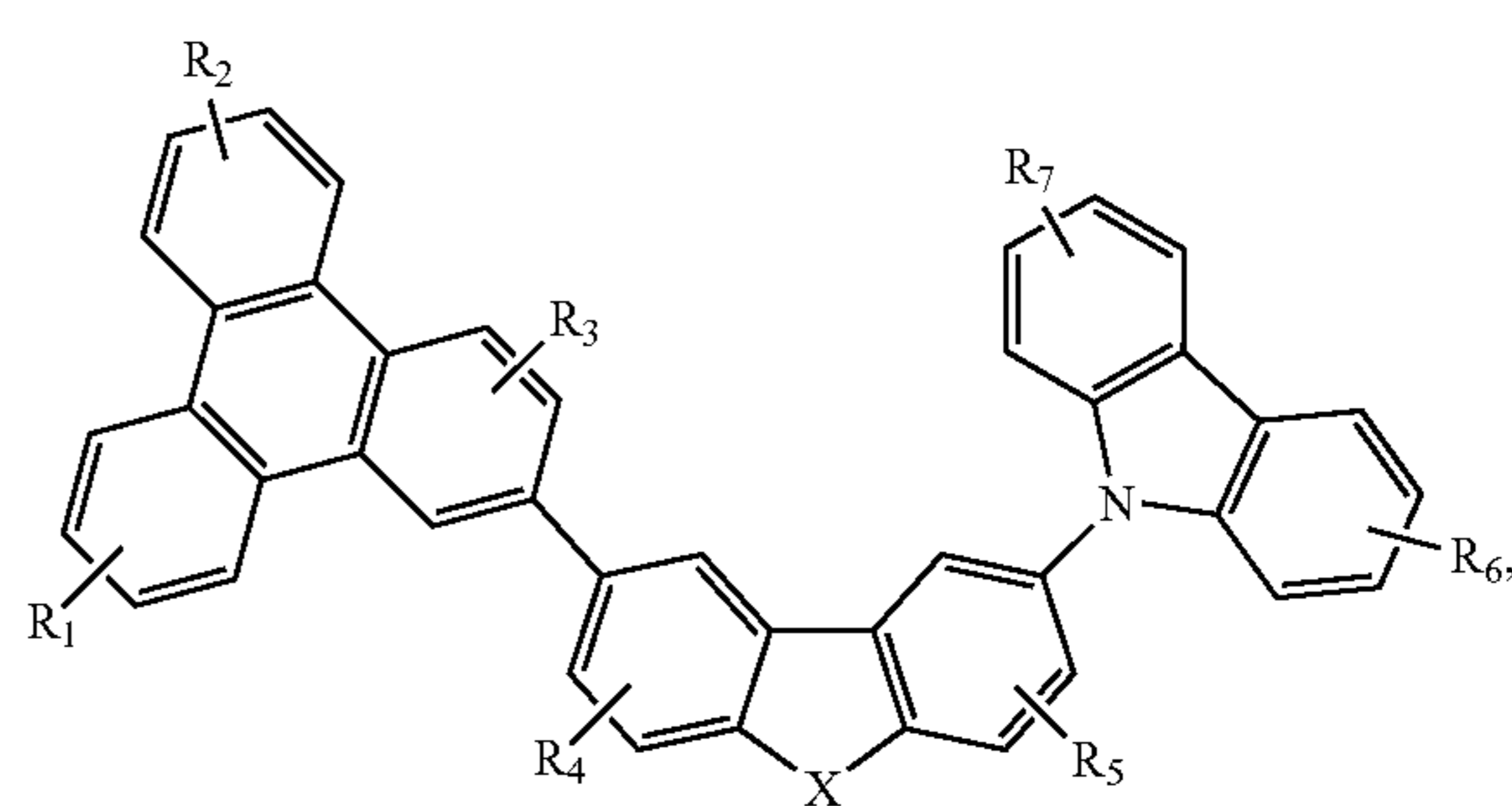
Compound 15G
