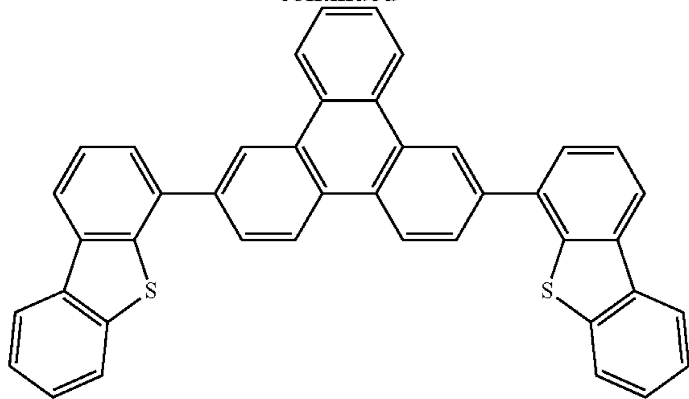
Compound 19S
