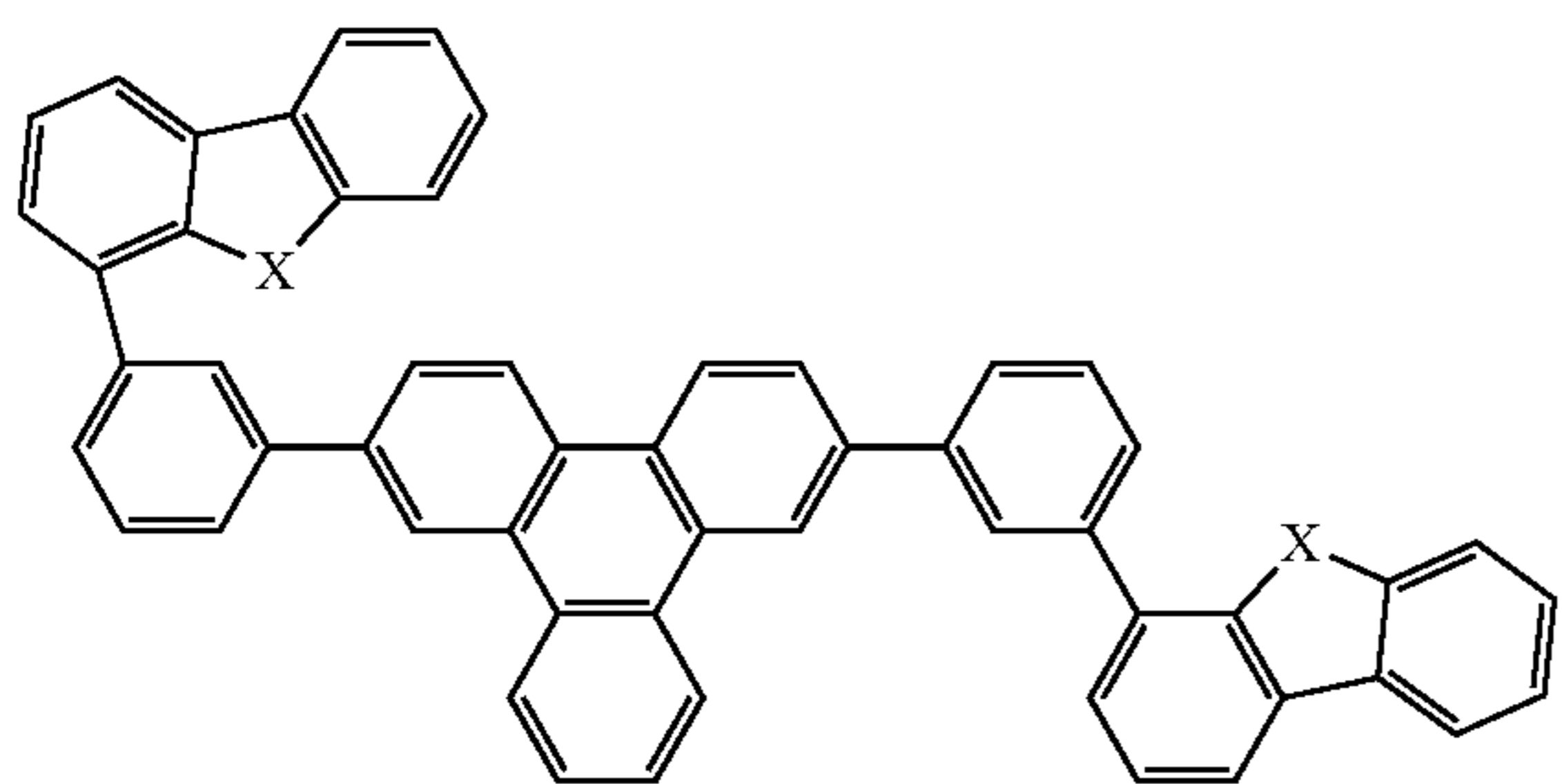
Compound 26
