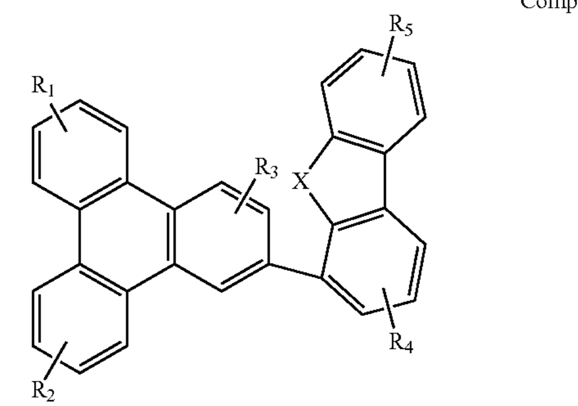
Compound 42G
