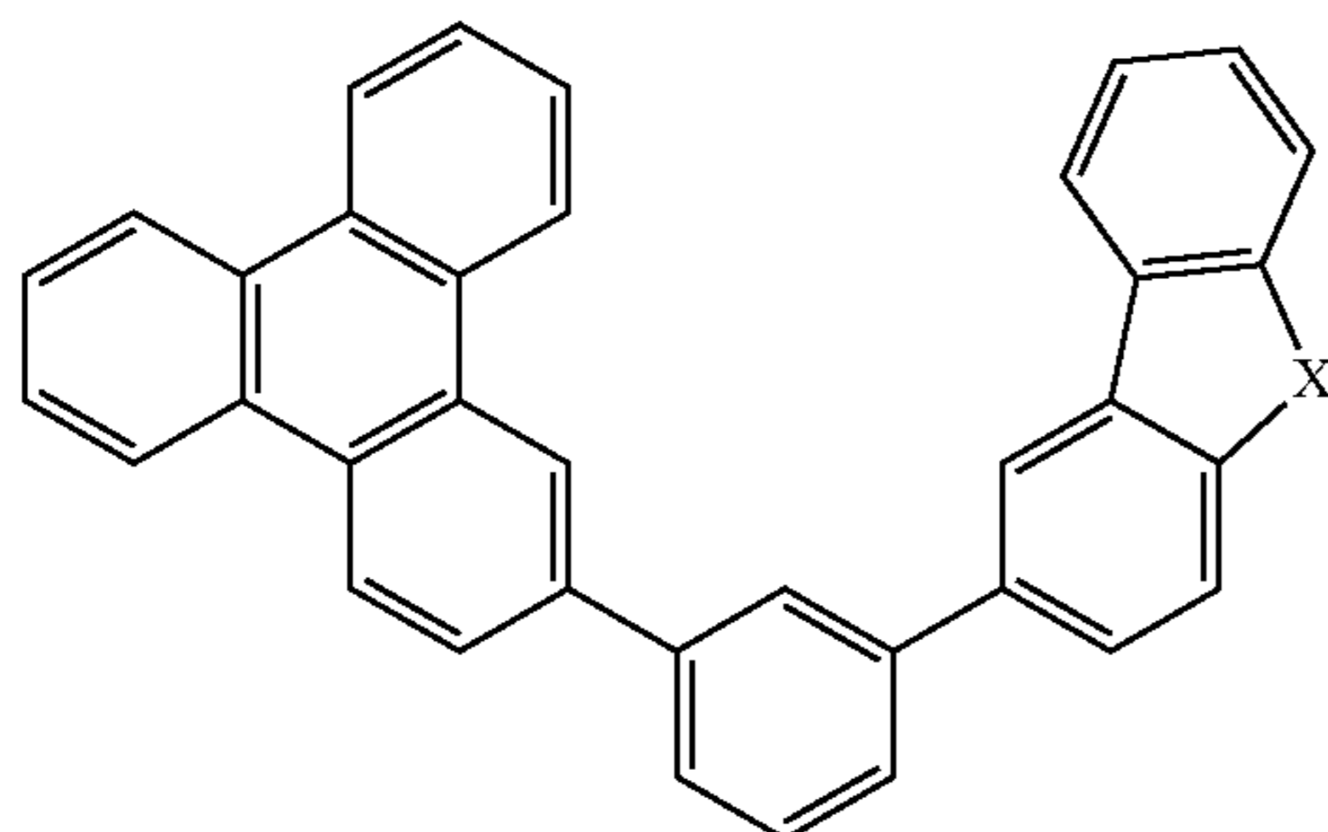
Compound 20
