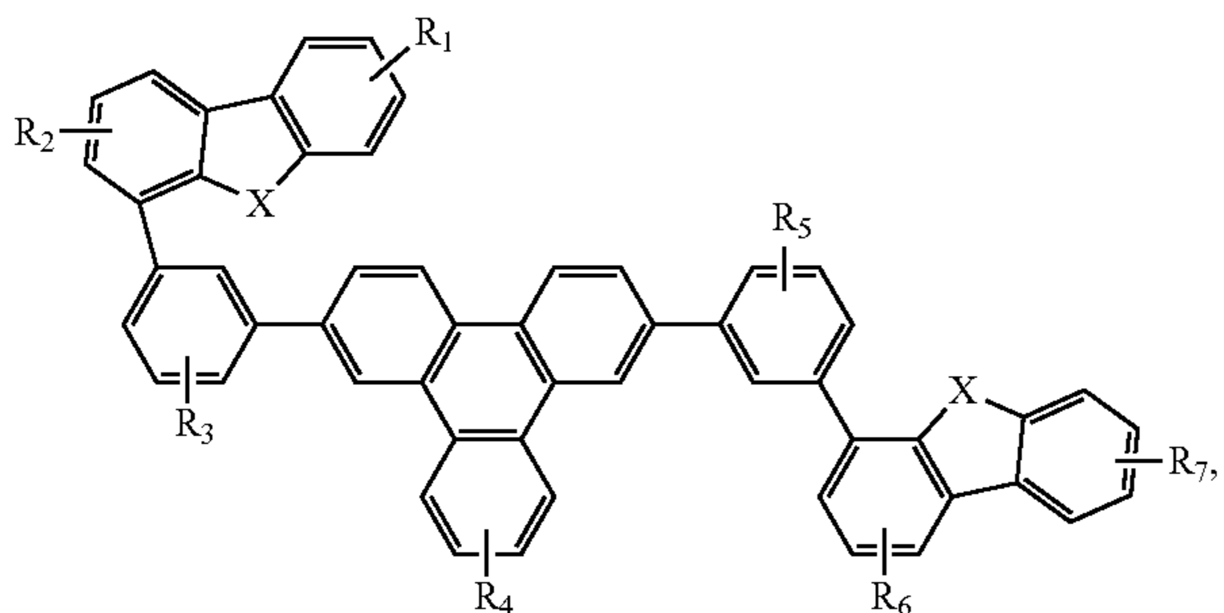
Compound 26G
