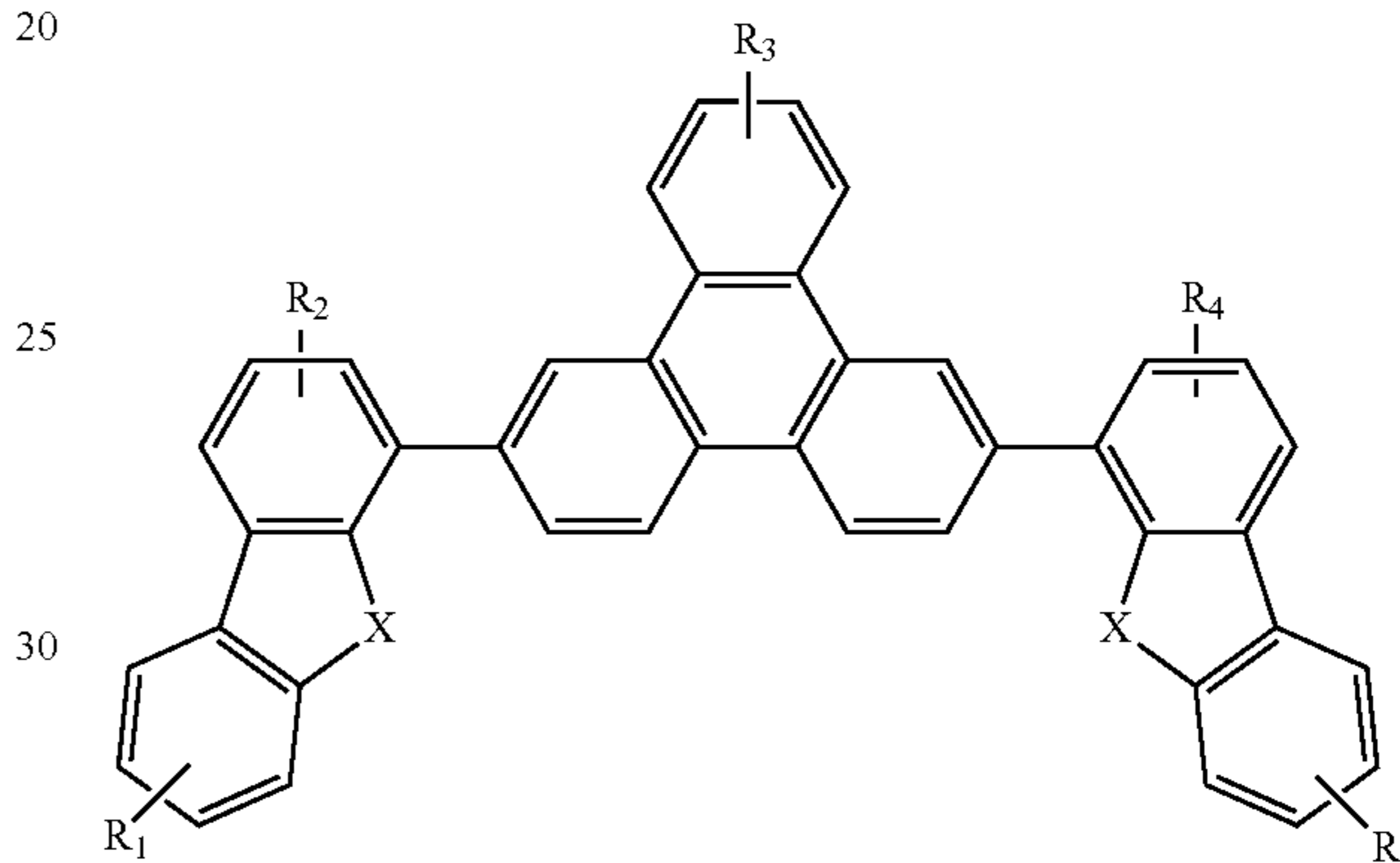
Compound 19 G
