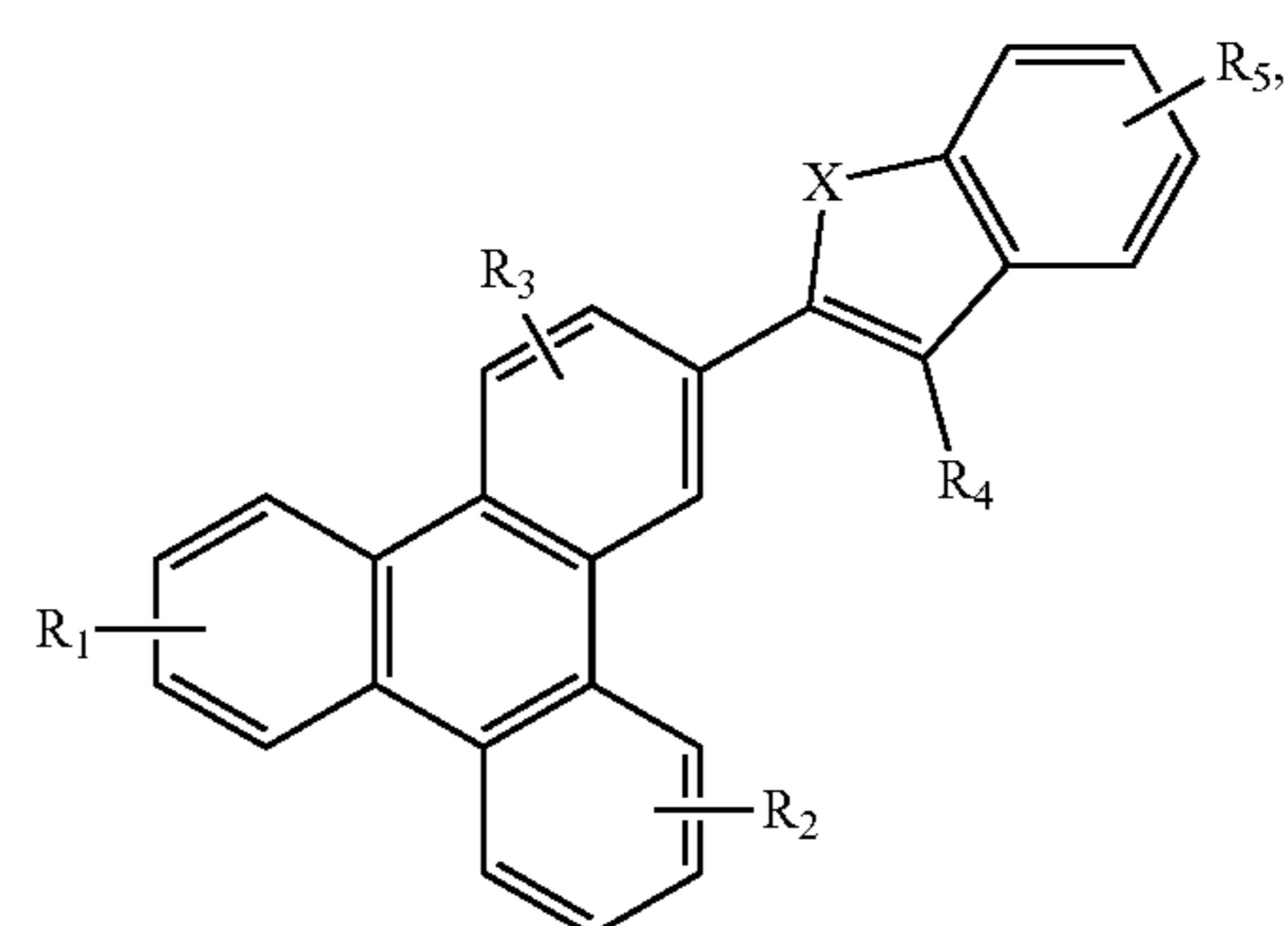
Compound 14G
