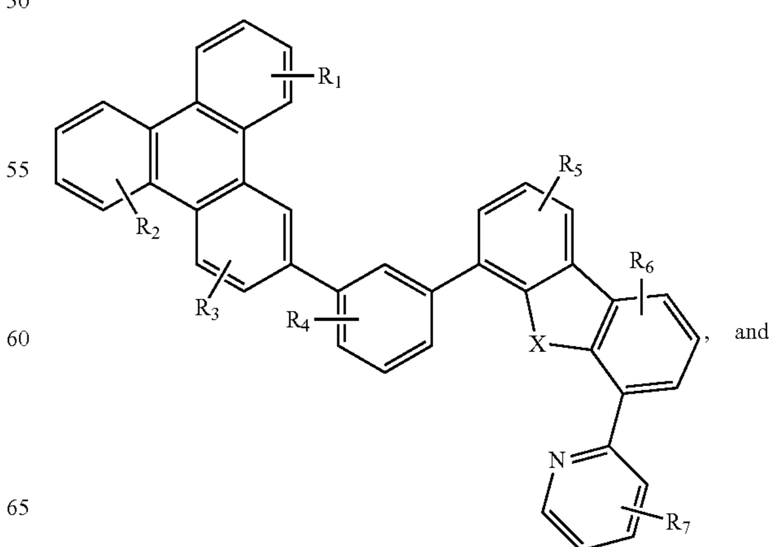
Compound 47G
