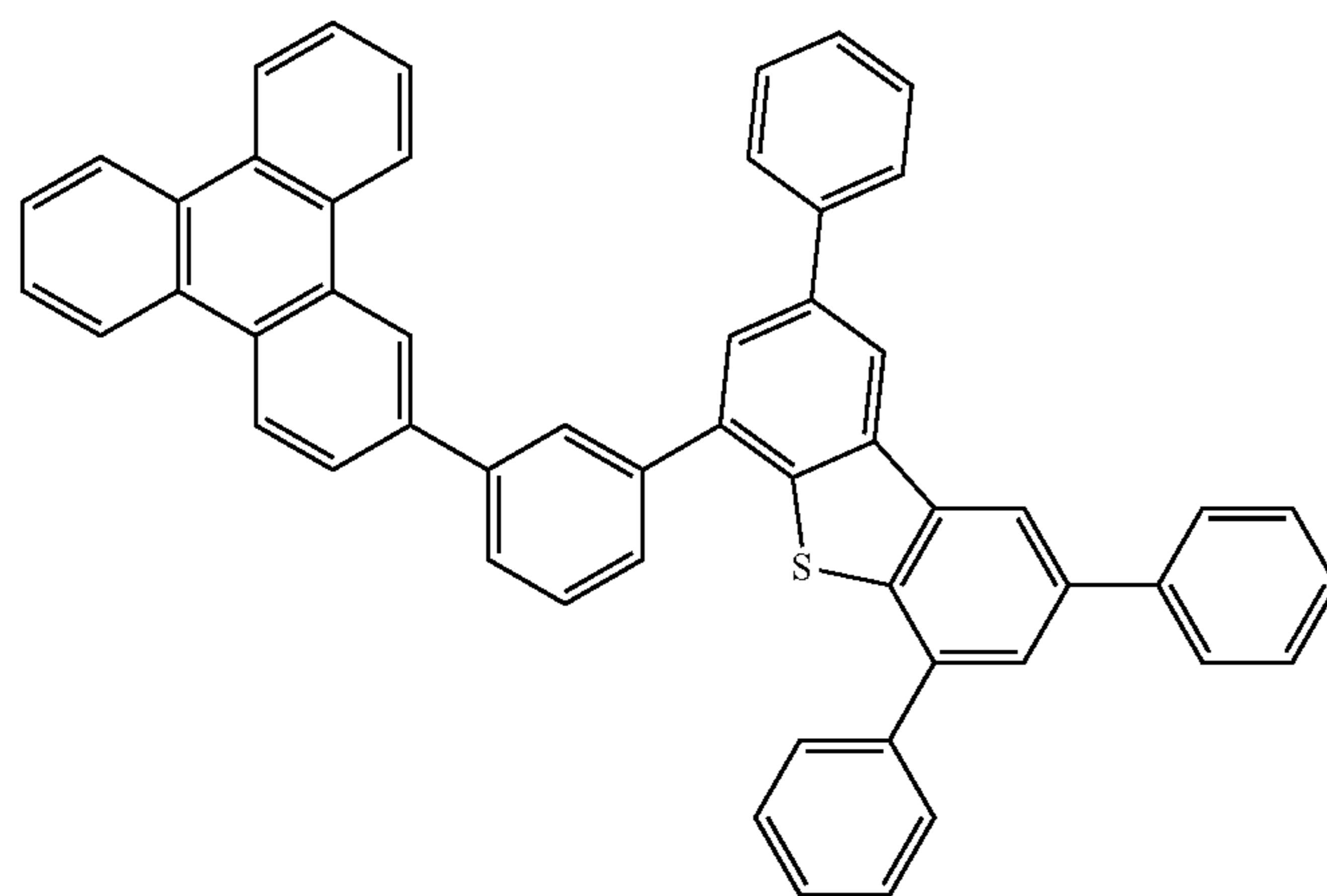
Compound 25S
