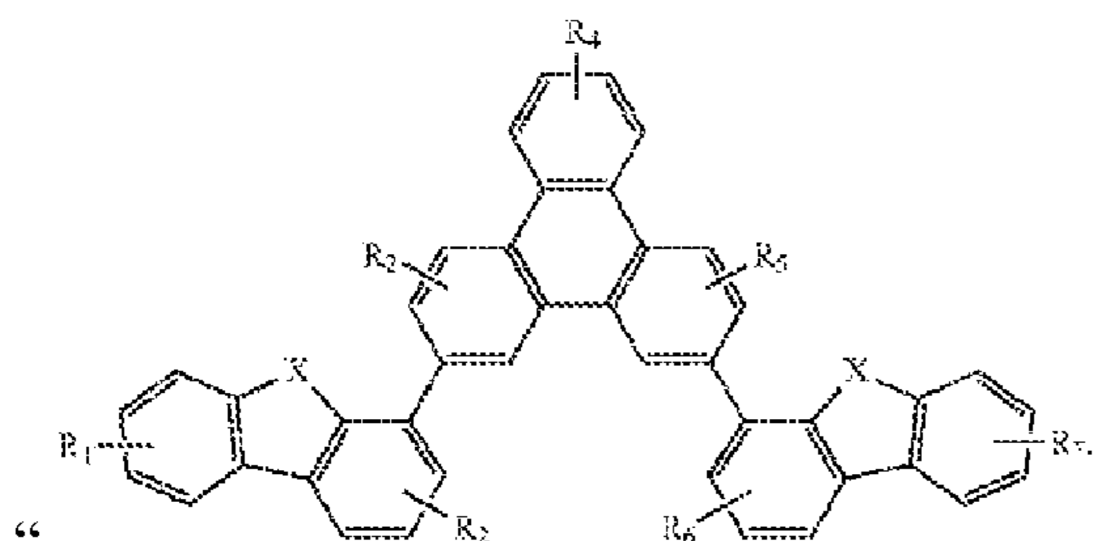
Compound 10G
