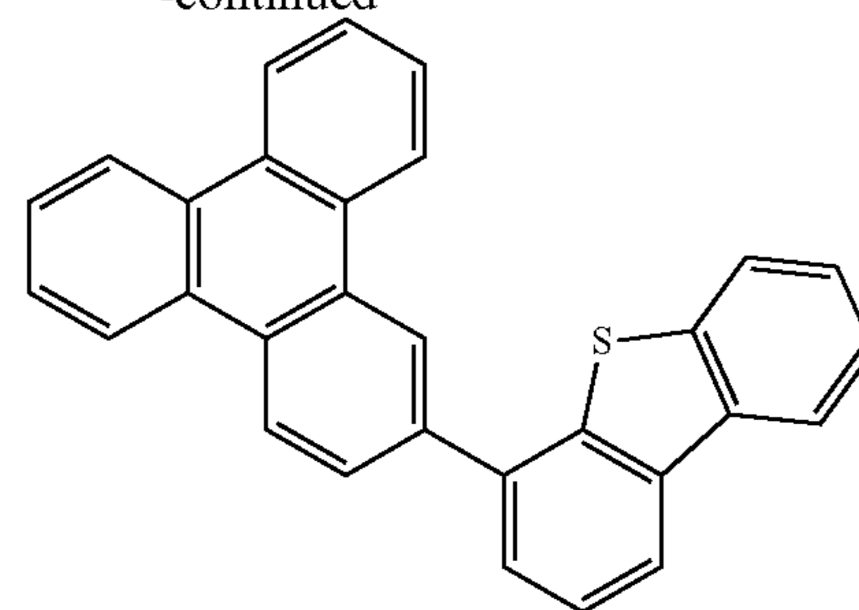
Compound 1S
