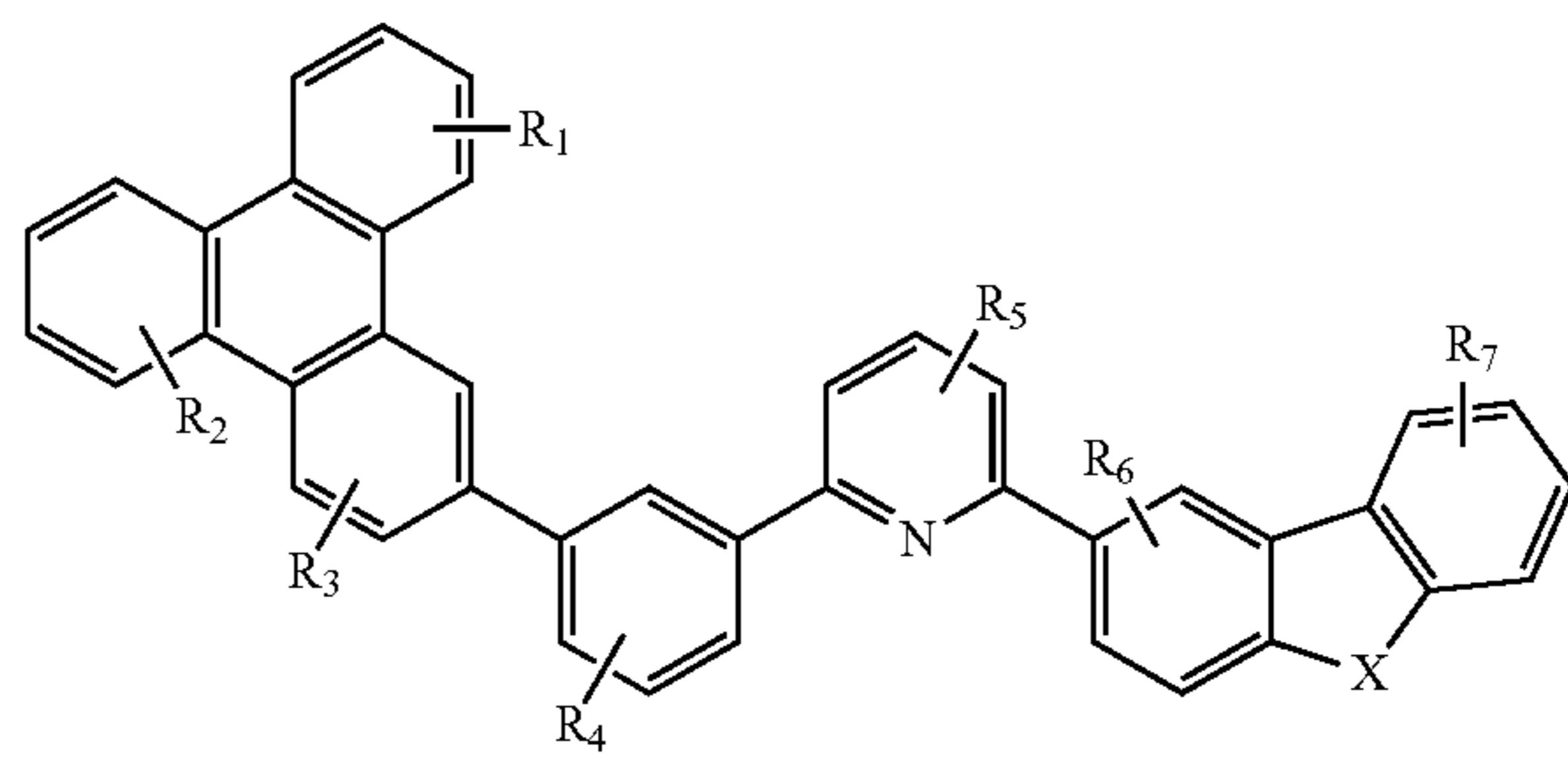
Compound 44 G
