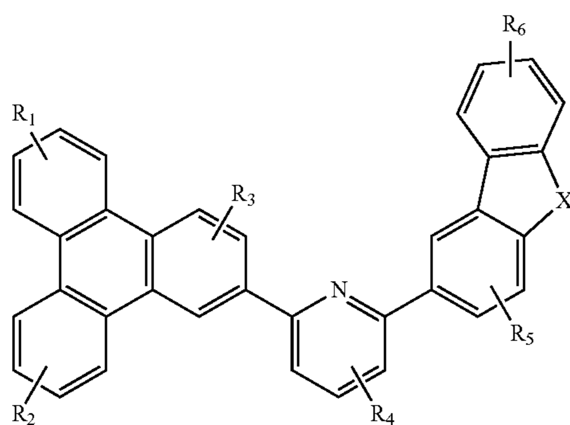
Compound 43
