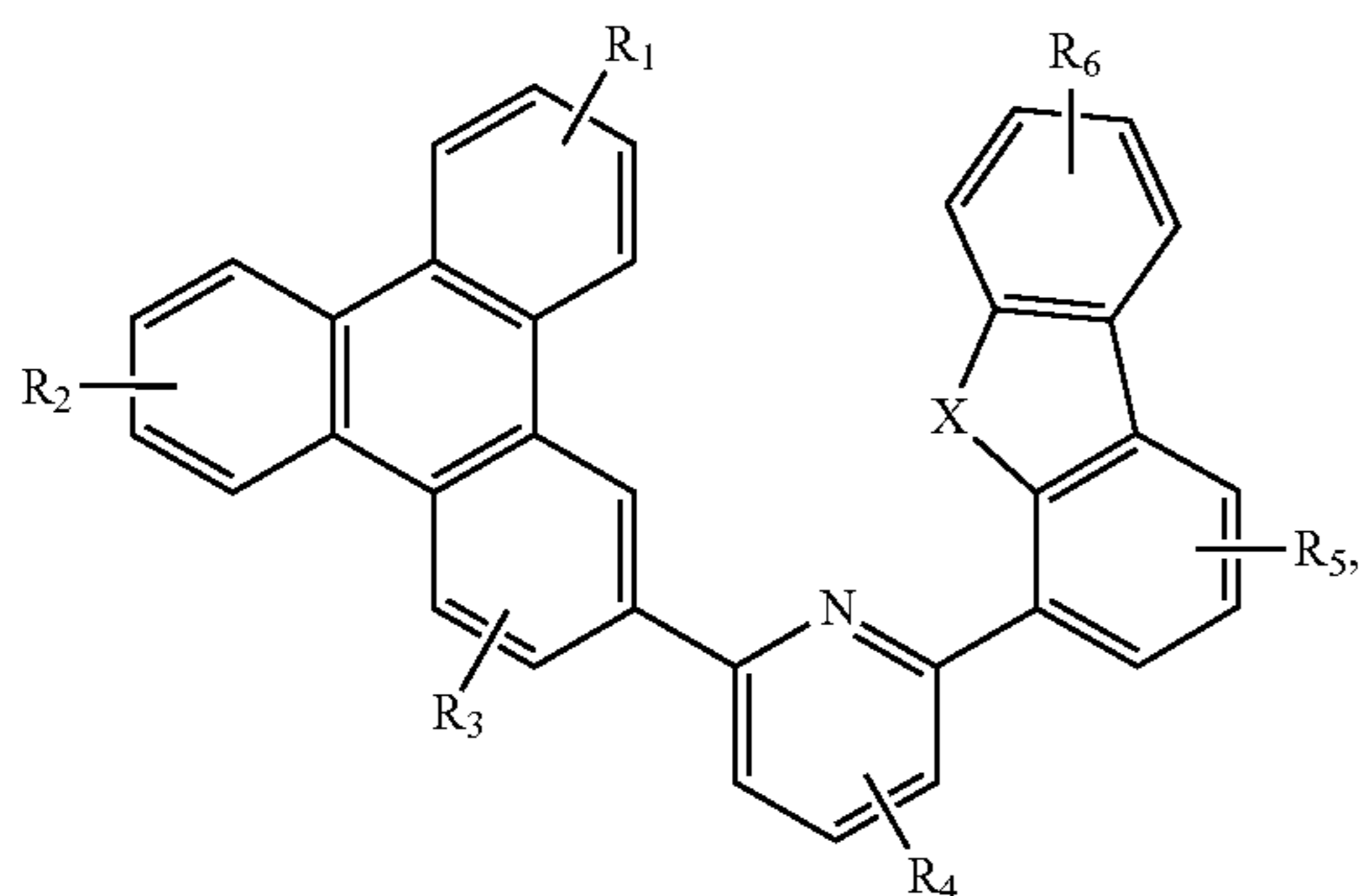
Compound 22G
