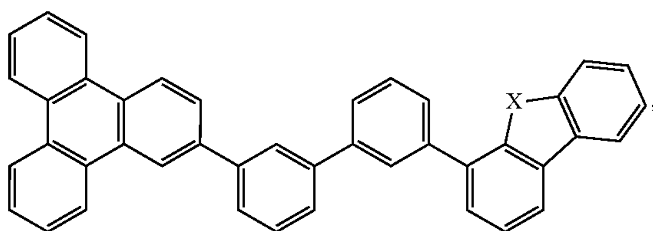
Compound 9
