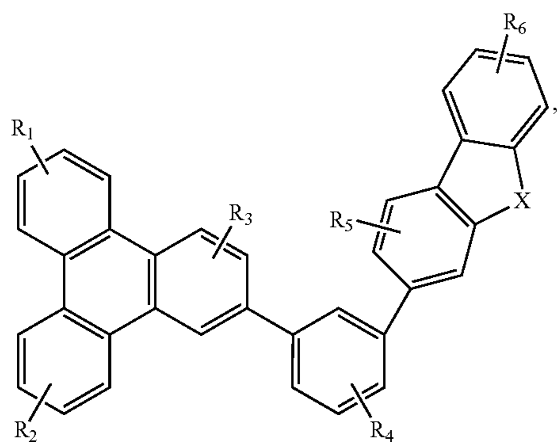
Compound 41G
