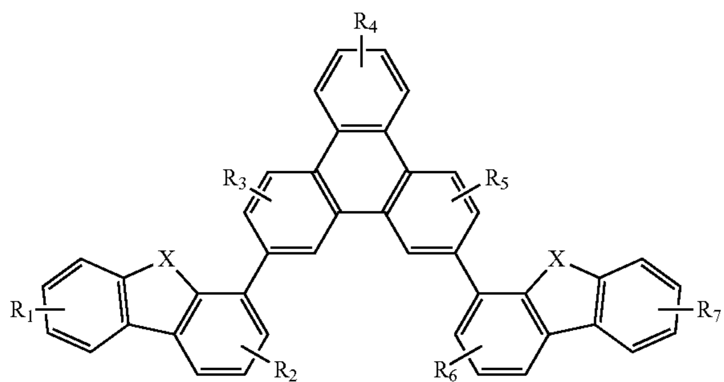
Compound 10G
