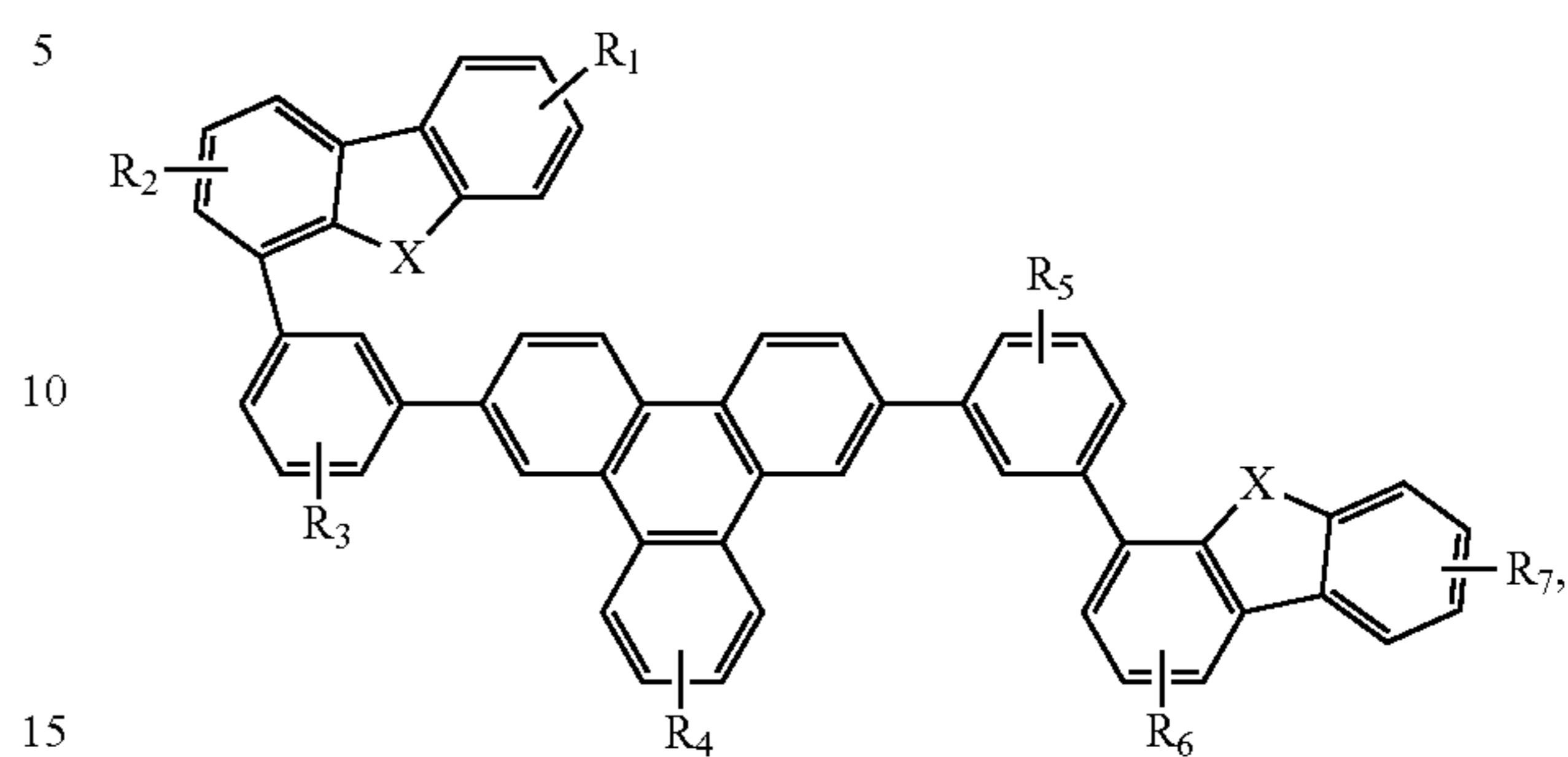
Compound 26G
