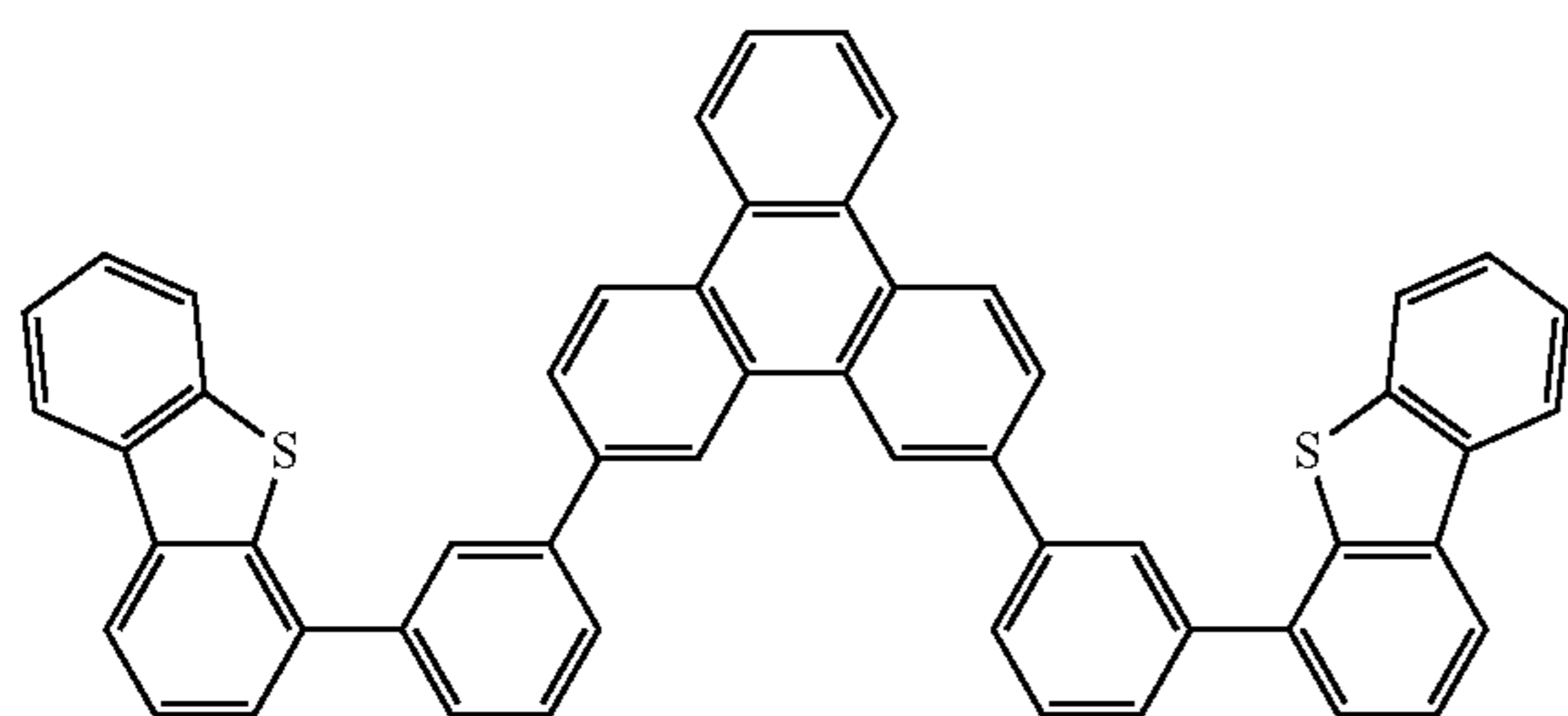
Compound 4S
