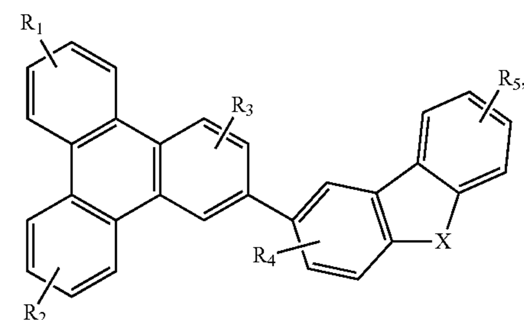
Compound 42G
