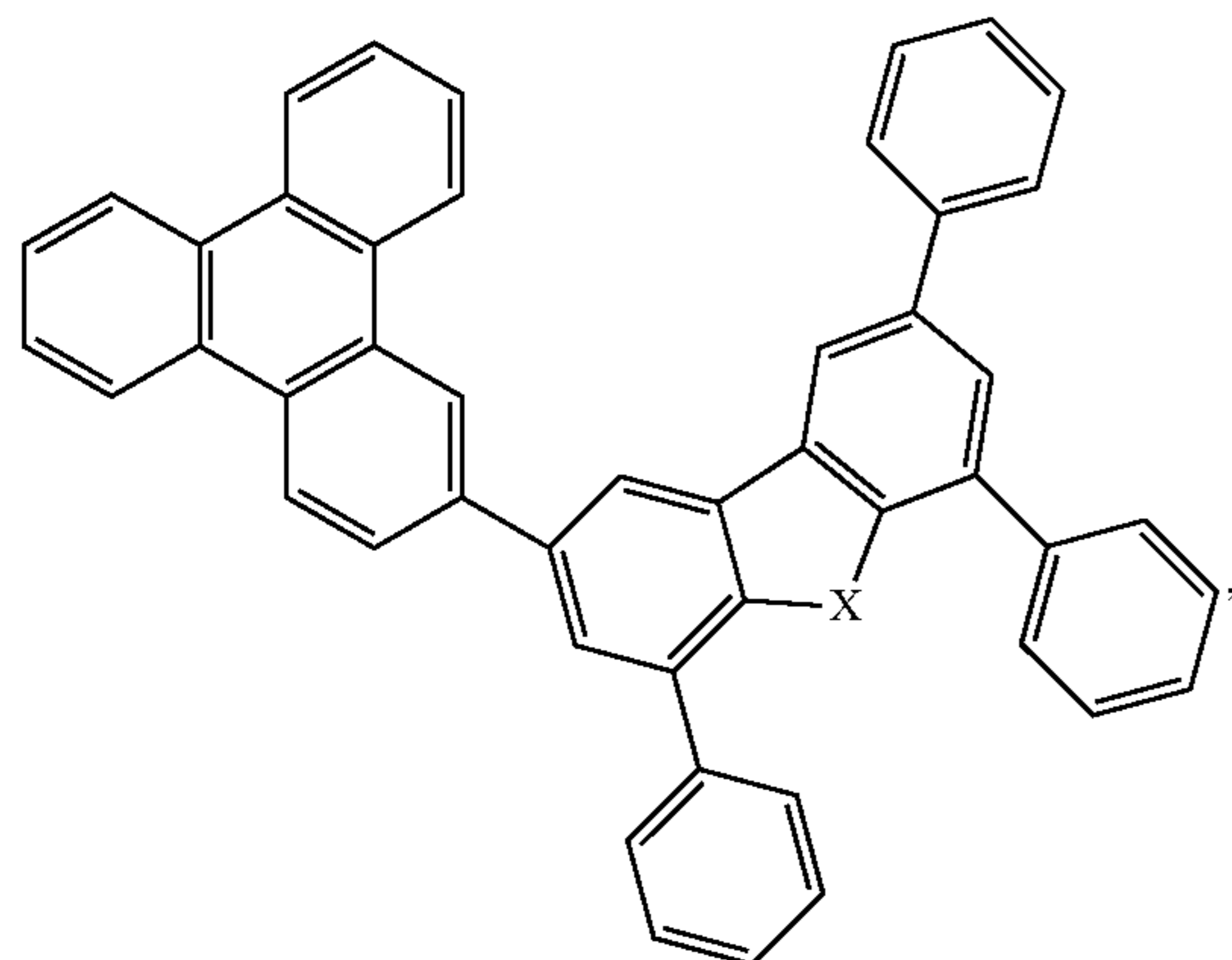
Compound 35
