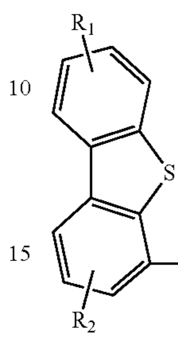
Compound 2'G
