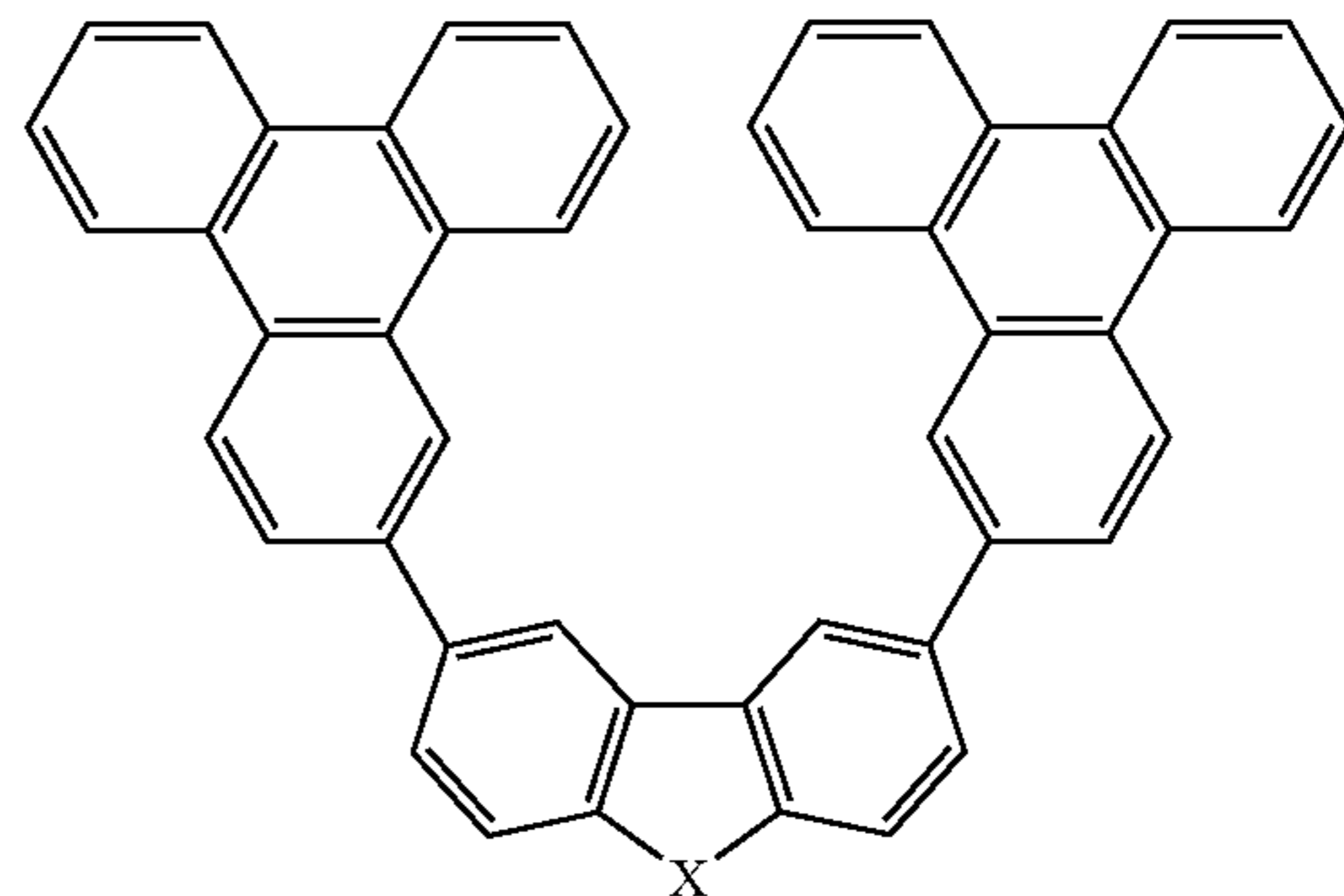
Compound 5
