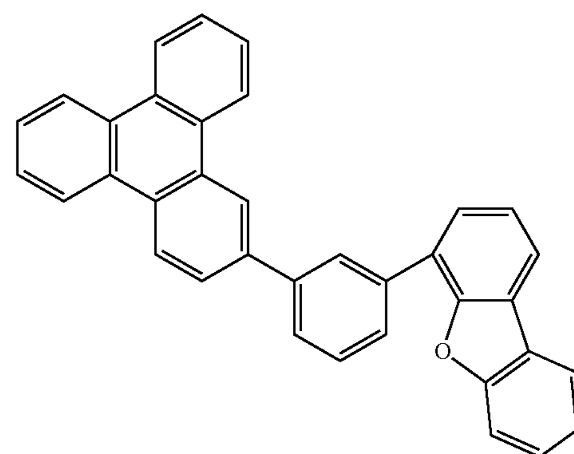
Compound 20
