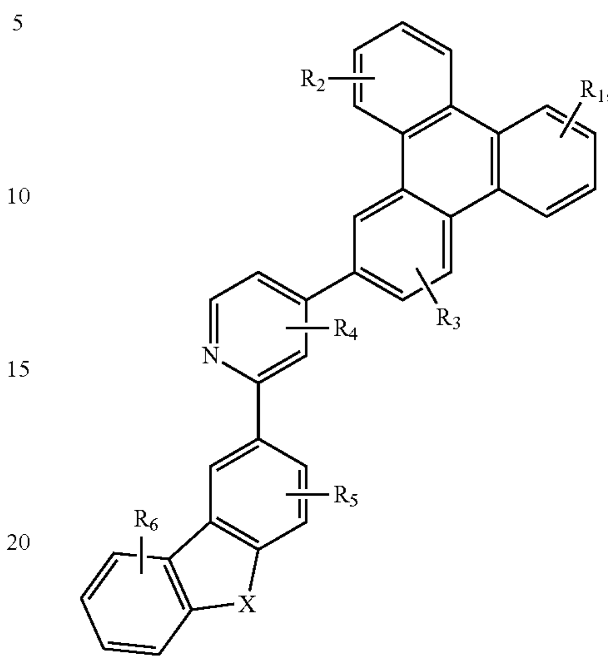
Compound 41G
