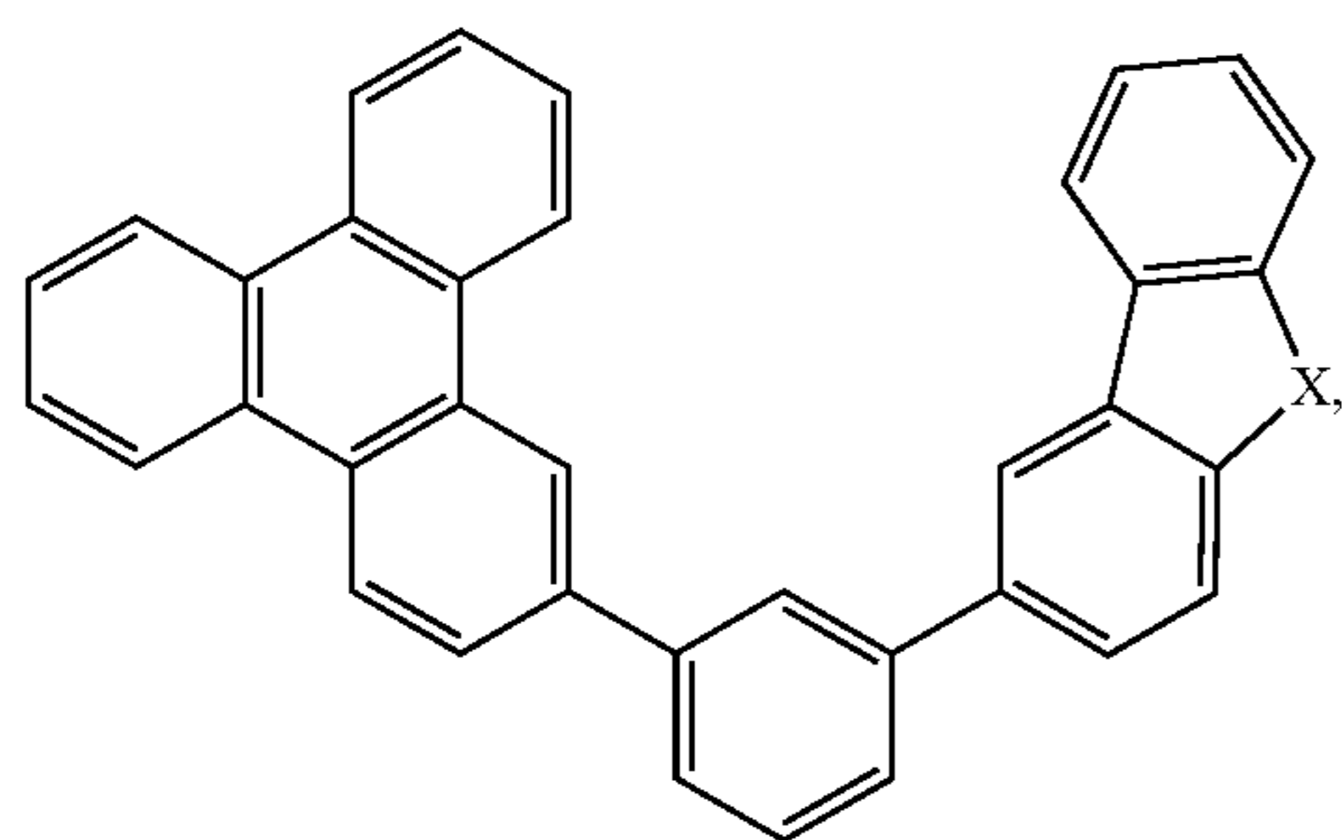
Compound 20
