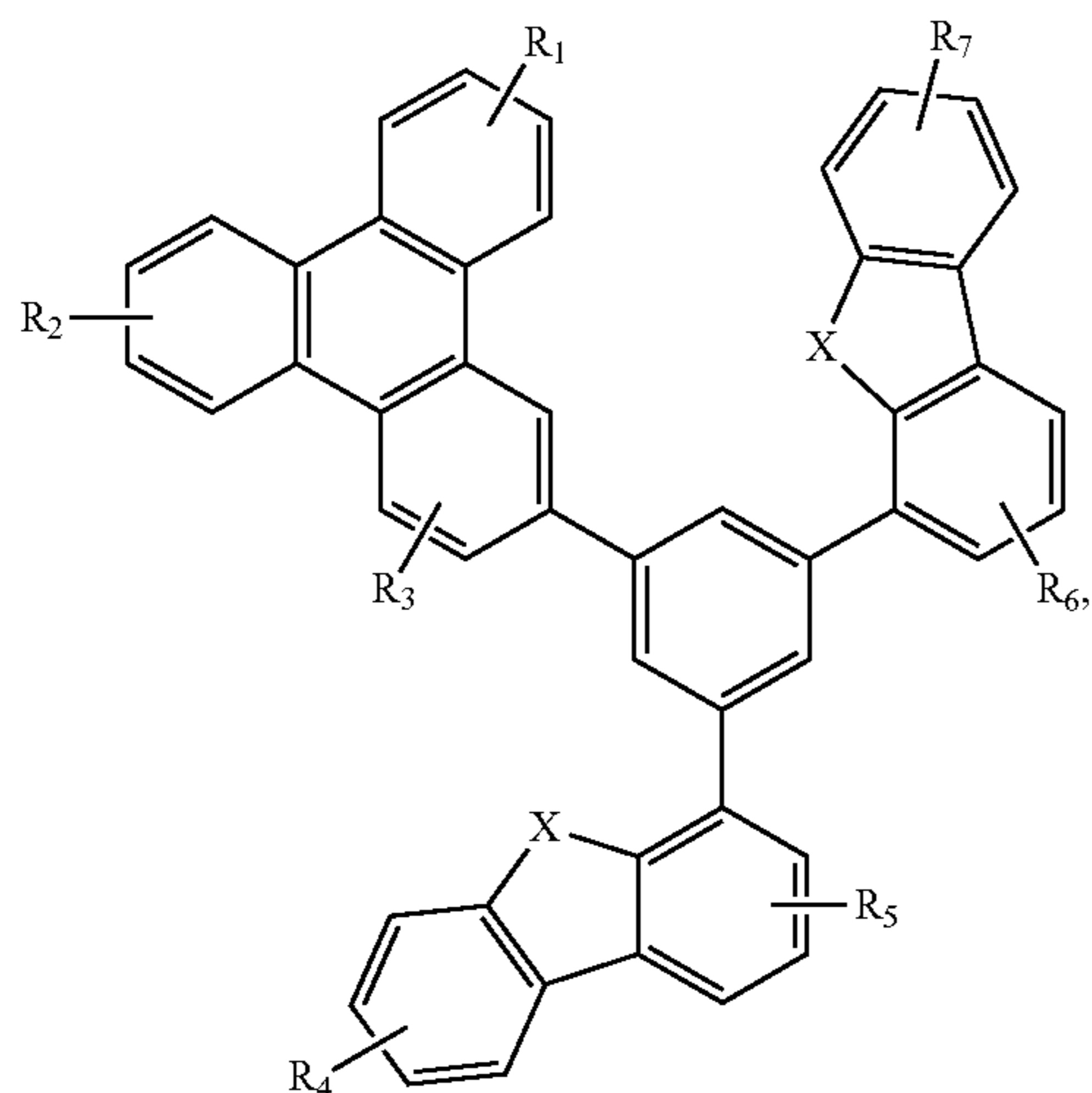
Compound 37G
