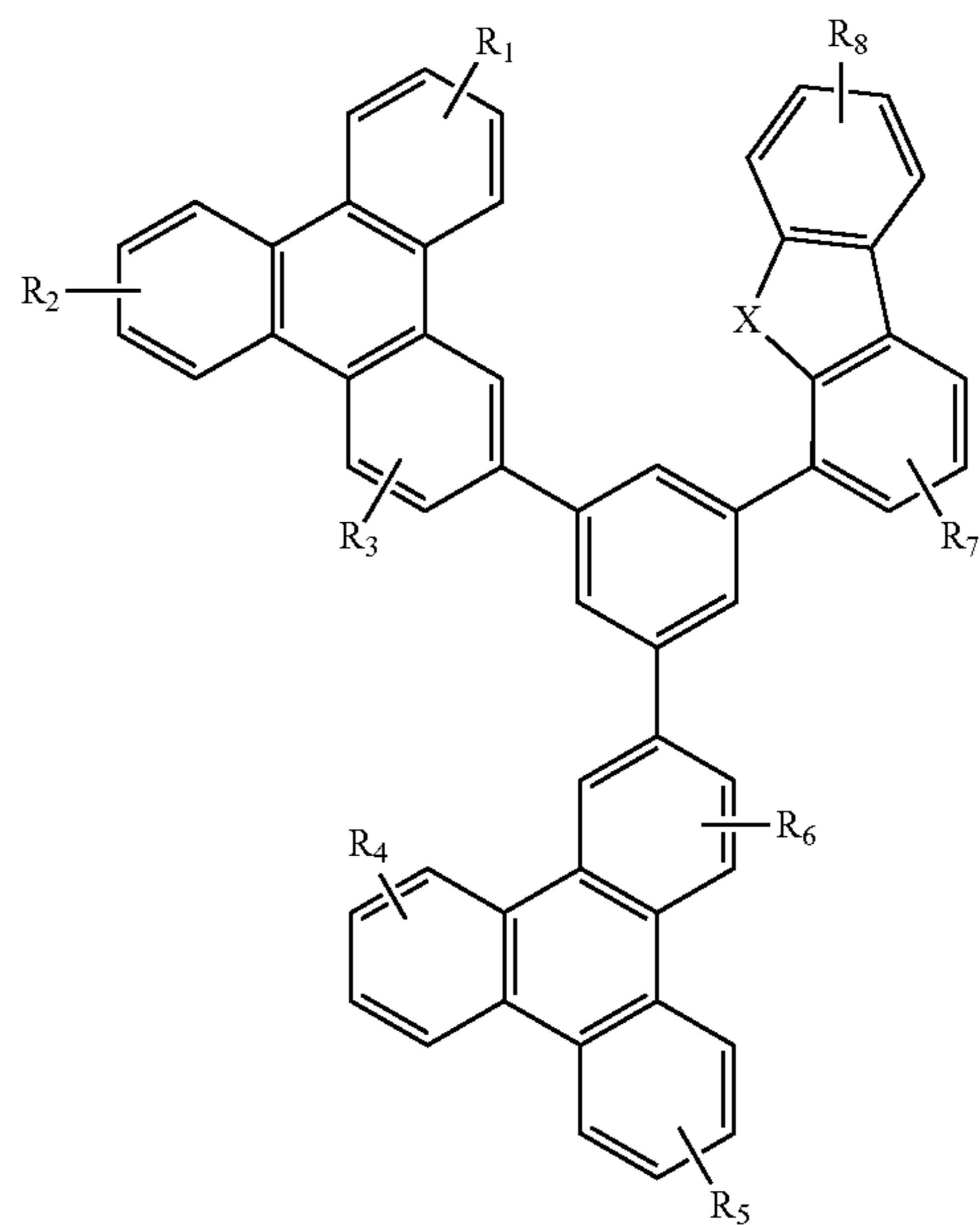
Compound 38G
