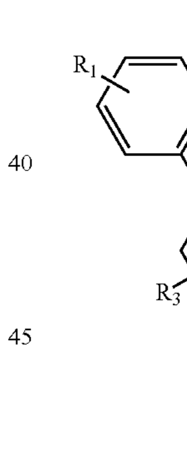
Compound 3'G
