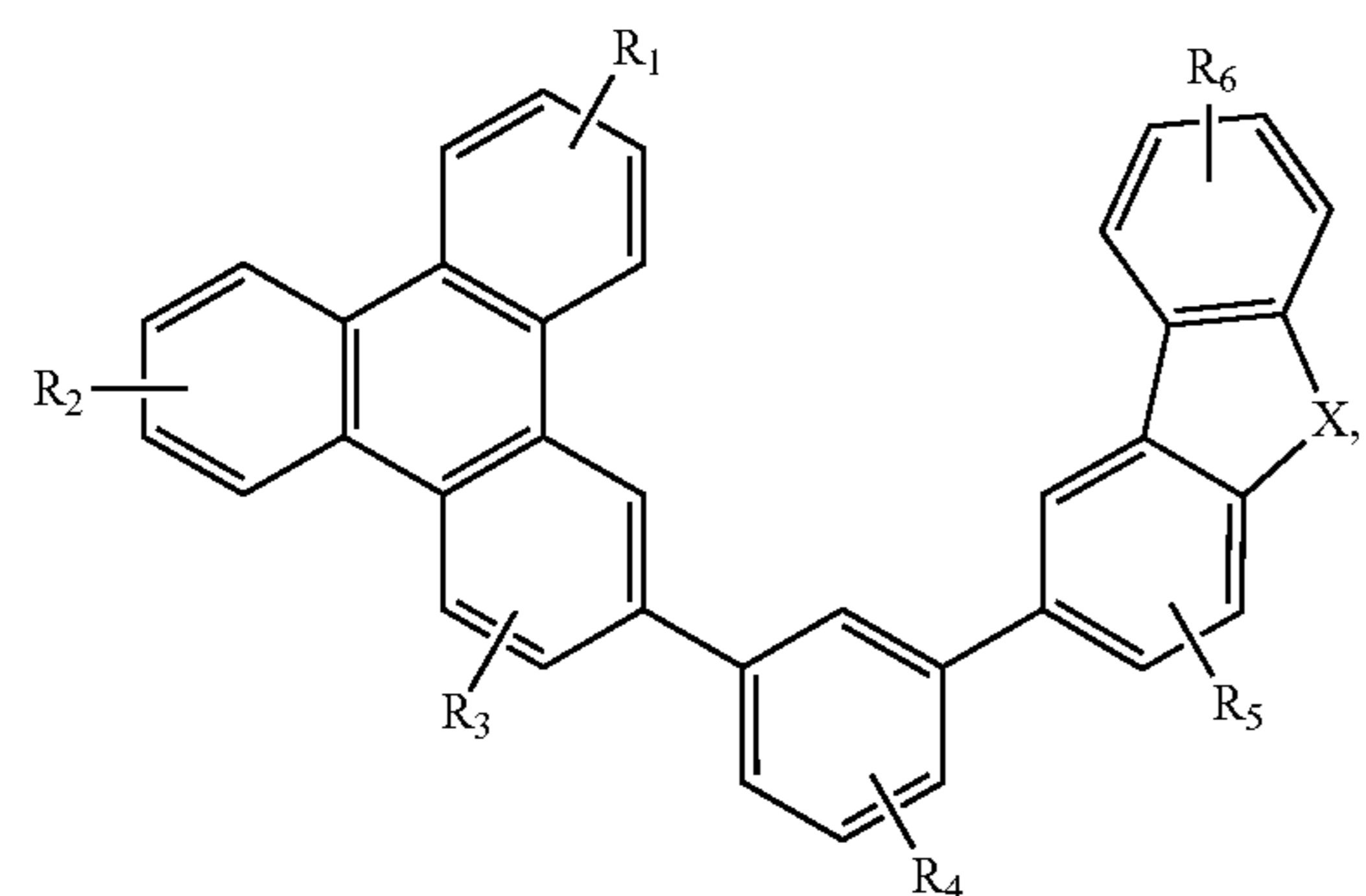
Compound 20G 40
