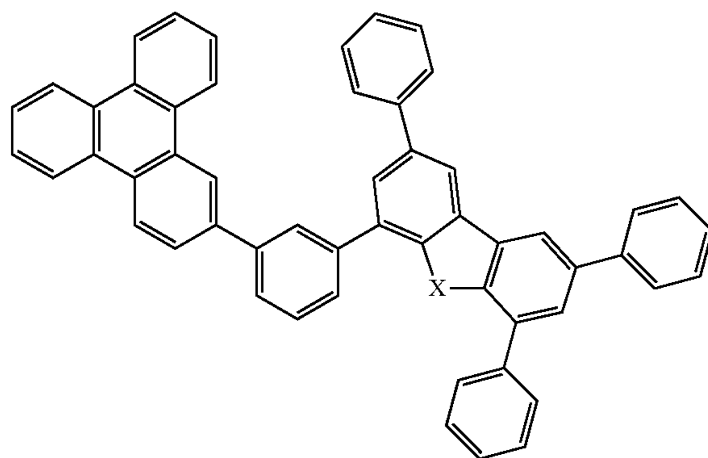
Compound 25
