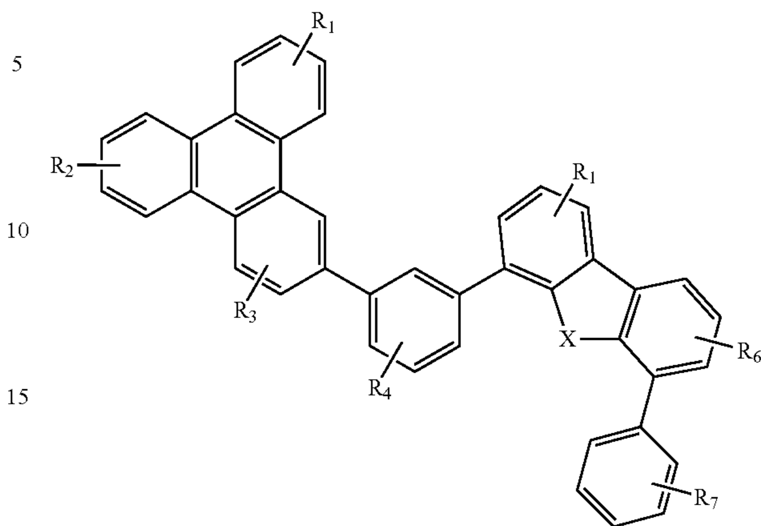
Compound 23 G
