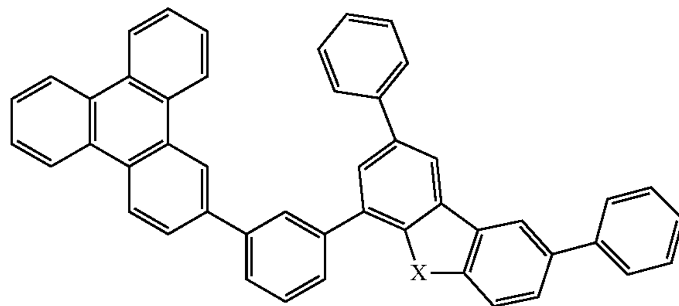
Compound 24
