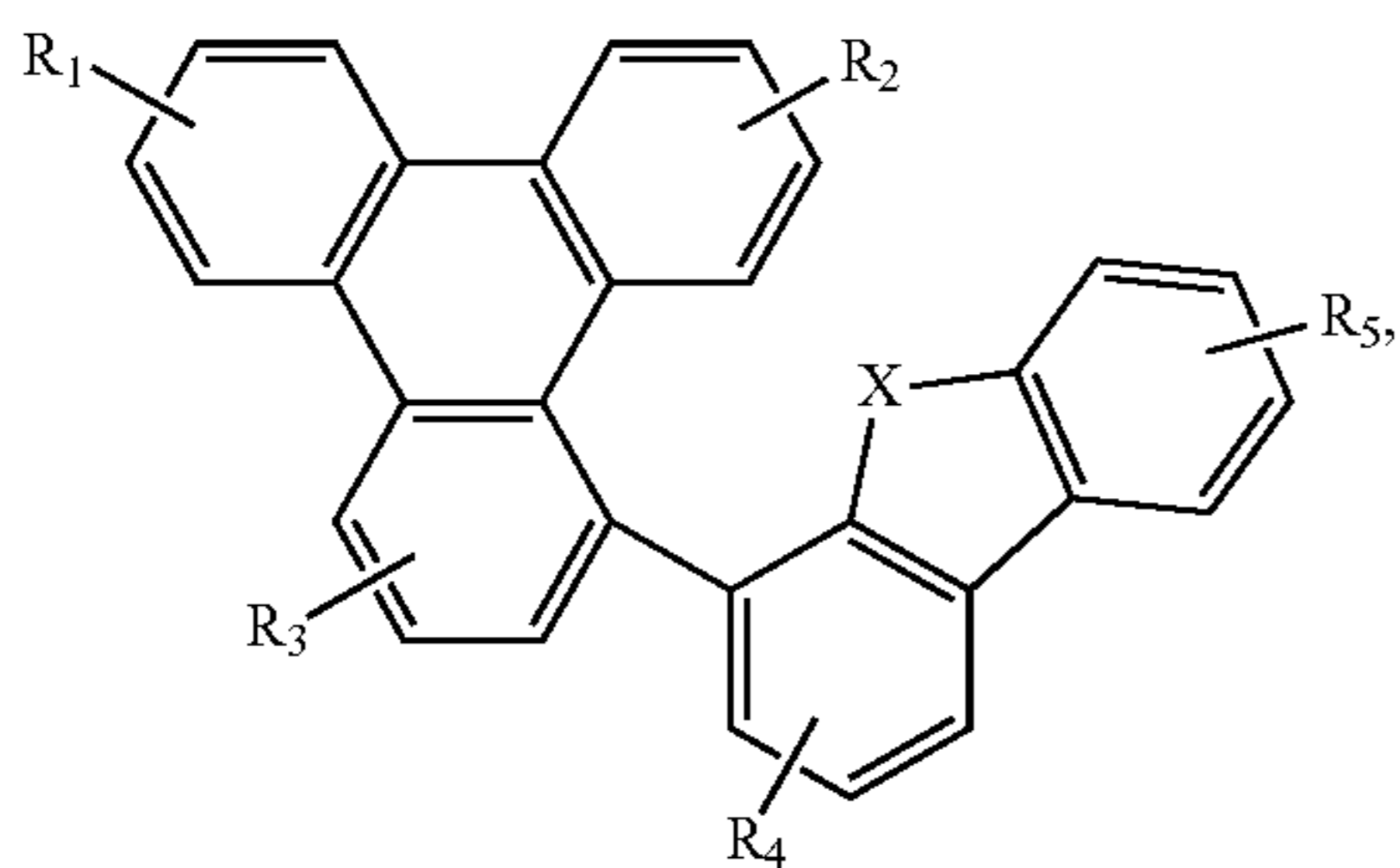
Compound 34G
