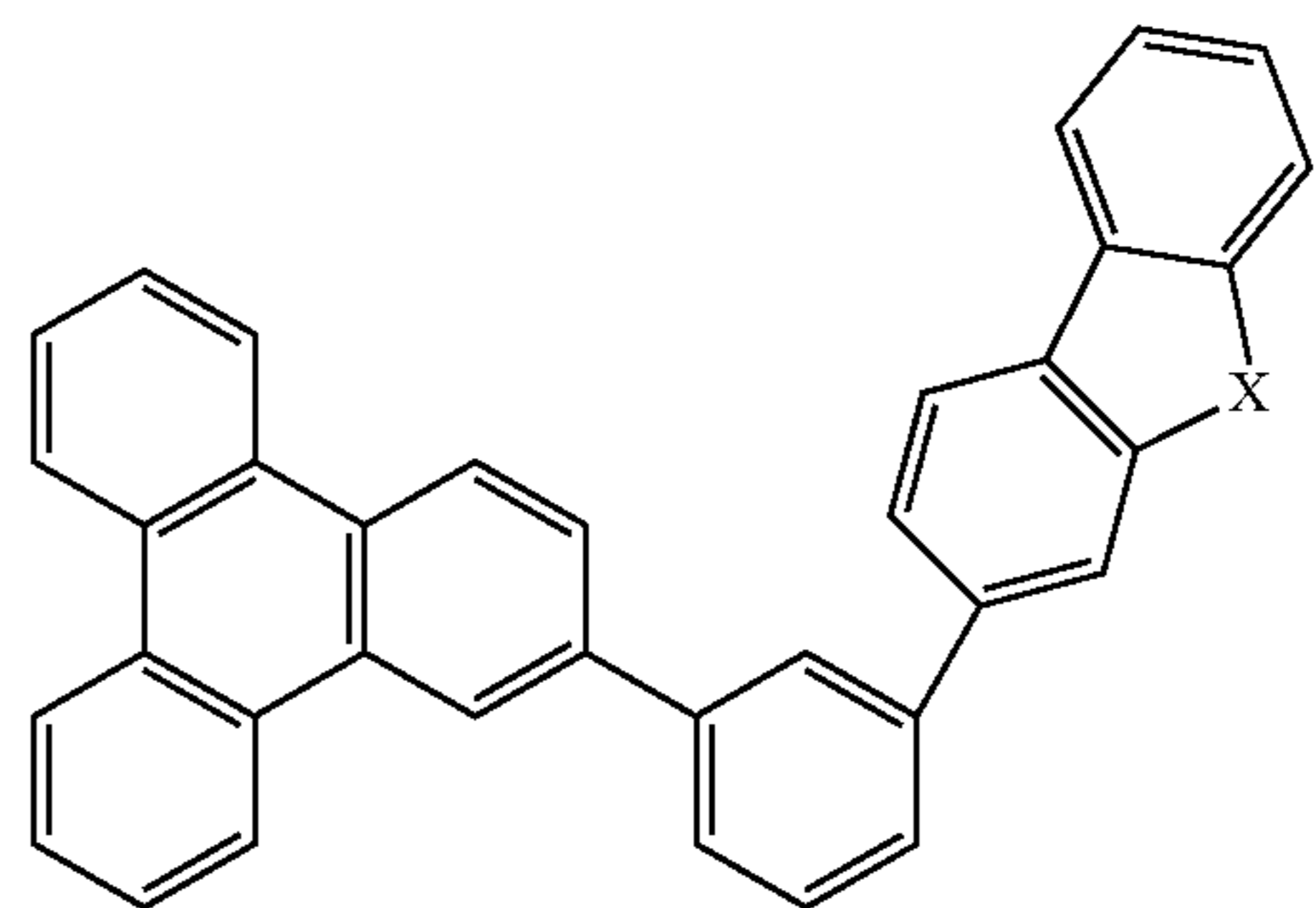
Compound 41
