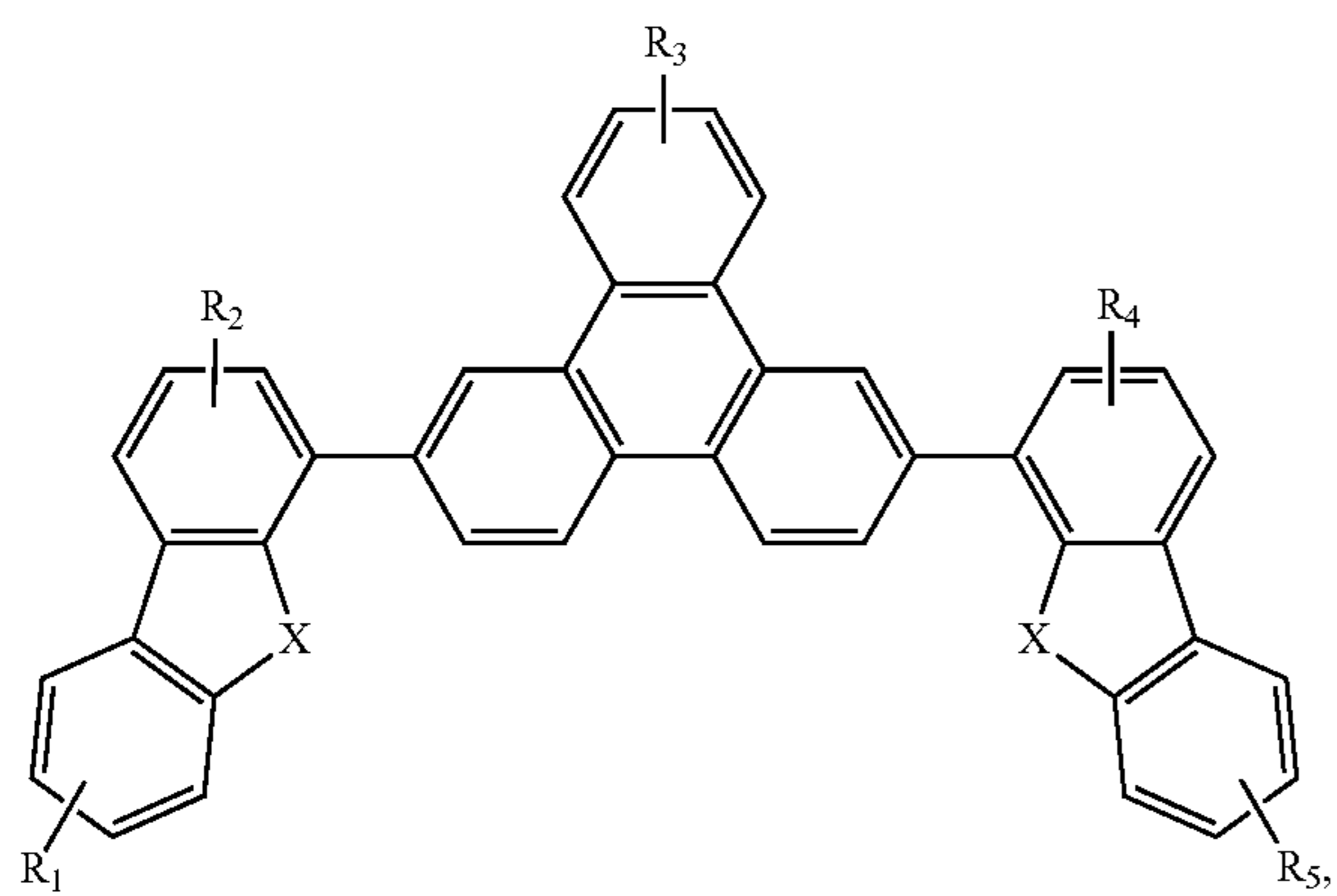
Compound 19G 20
