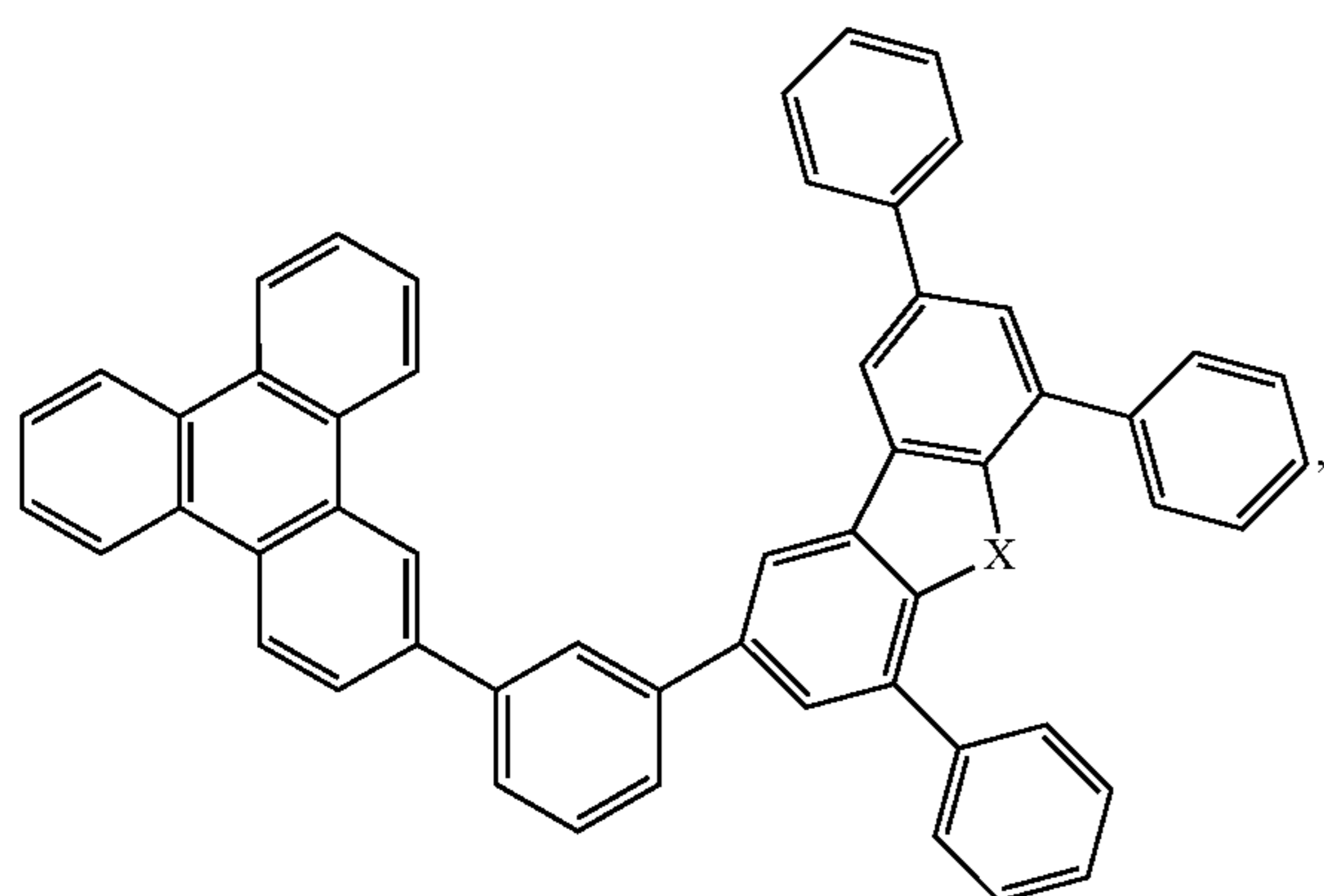
Compound 37
