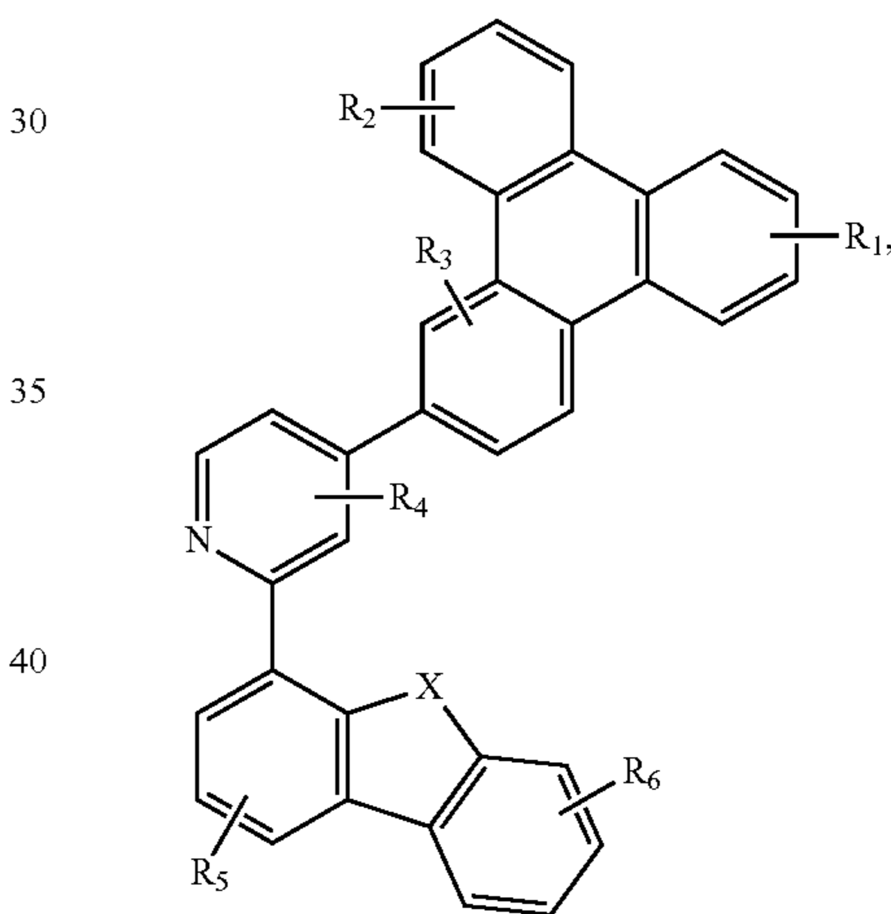
Compound 42G
