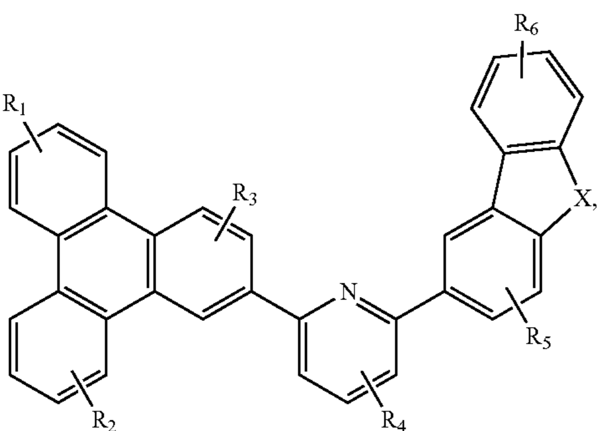
Compound 44G
