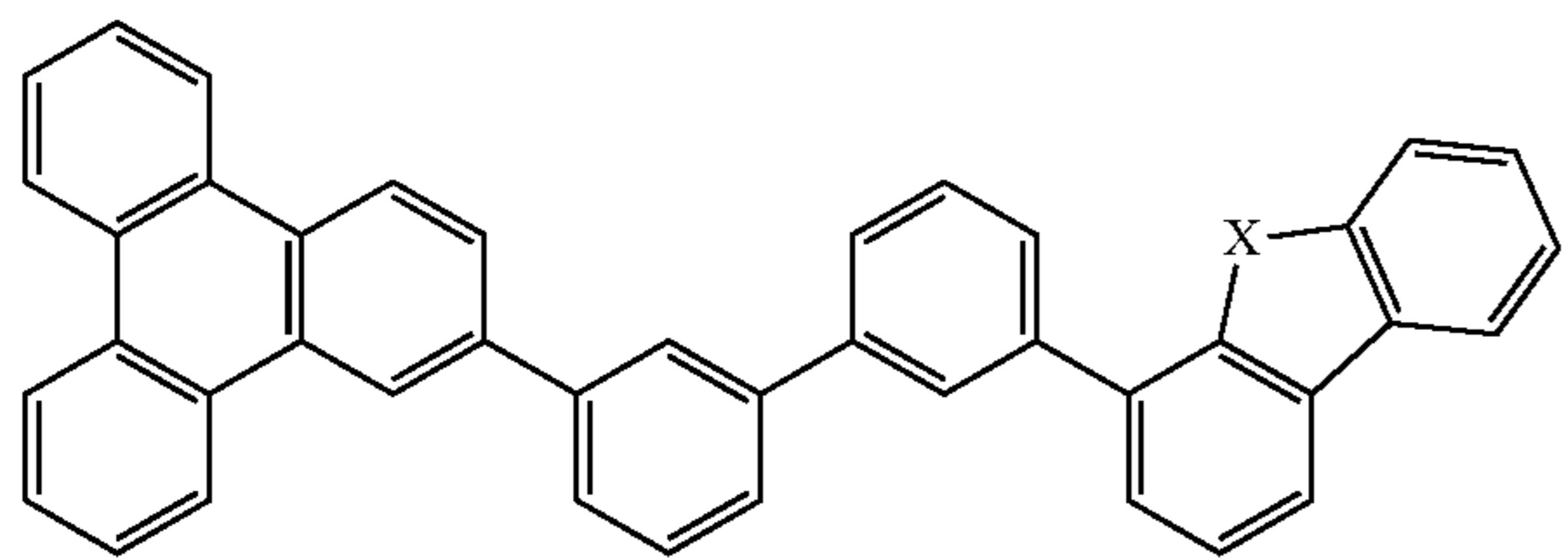
Compound 10G
