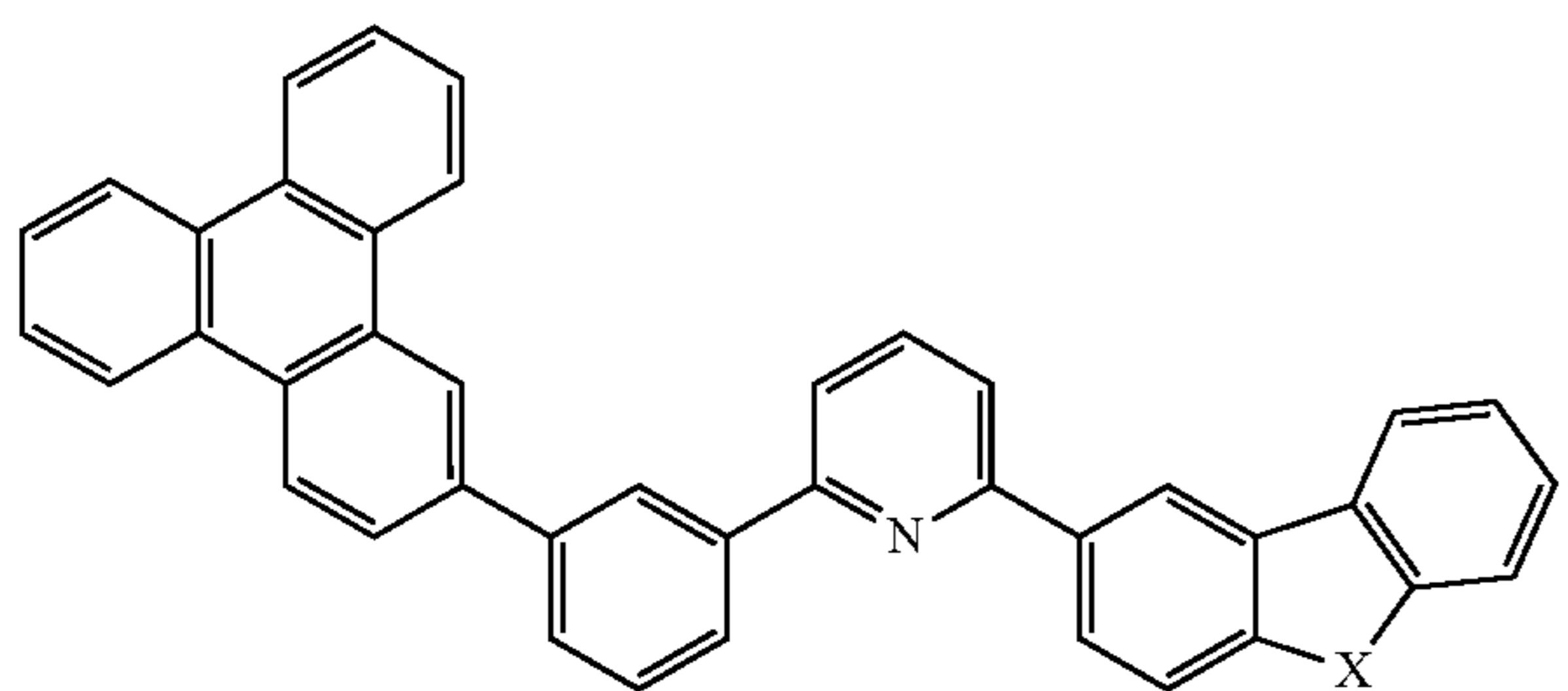
Compound 44
