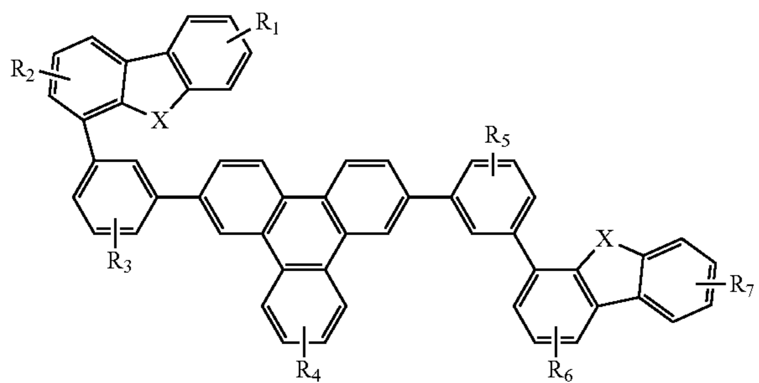
Compound 26G
