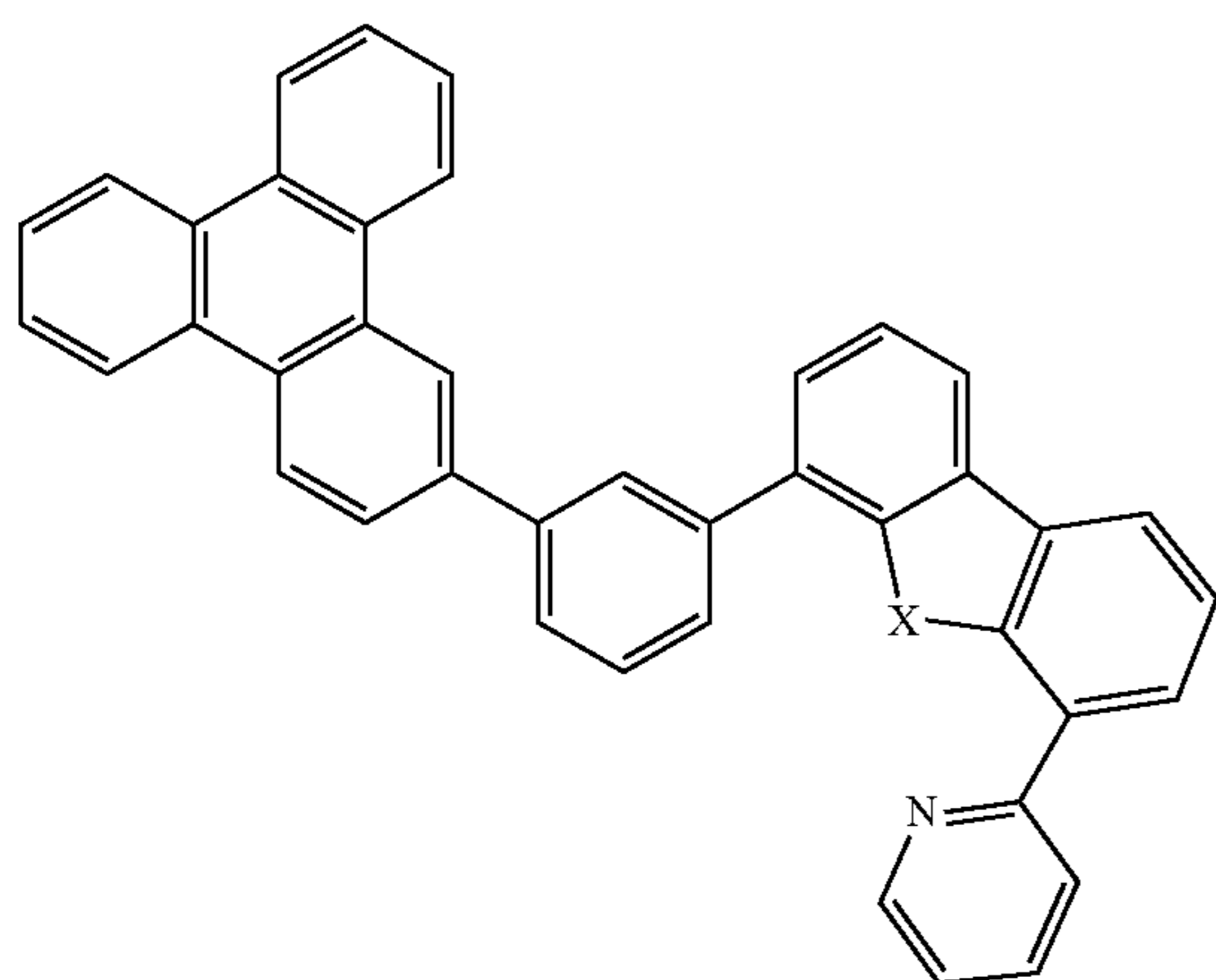
Compound 47
