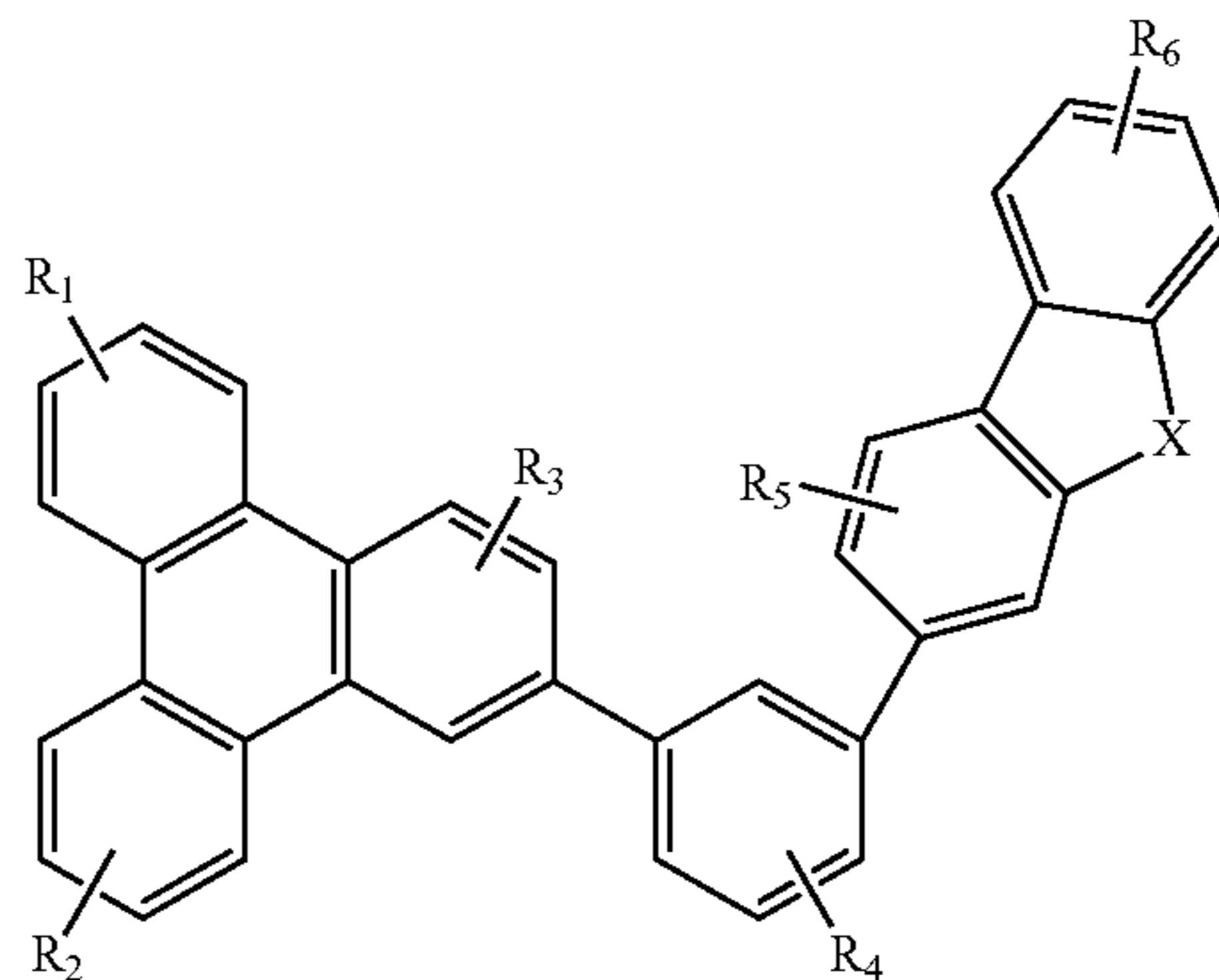
Compound 41G
