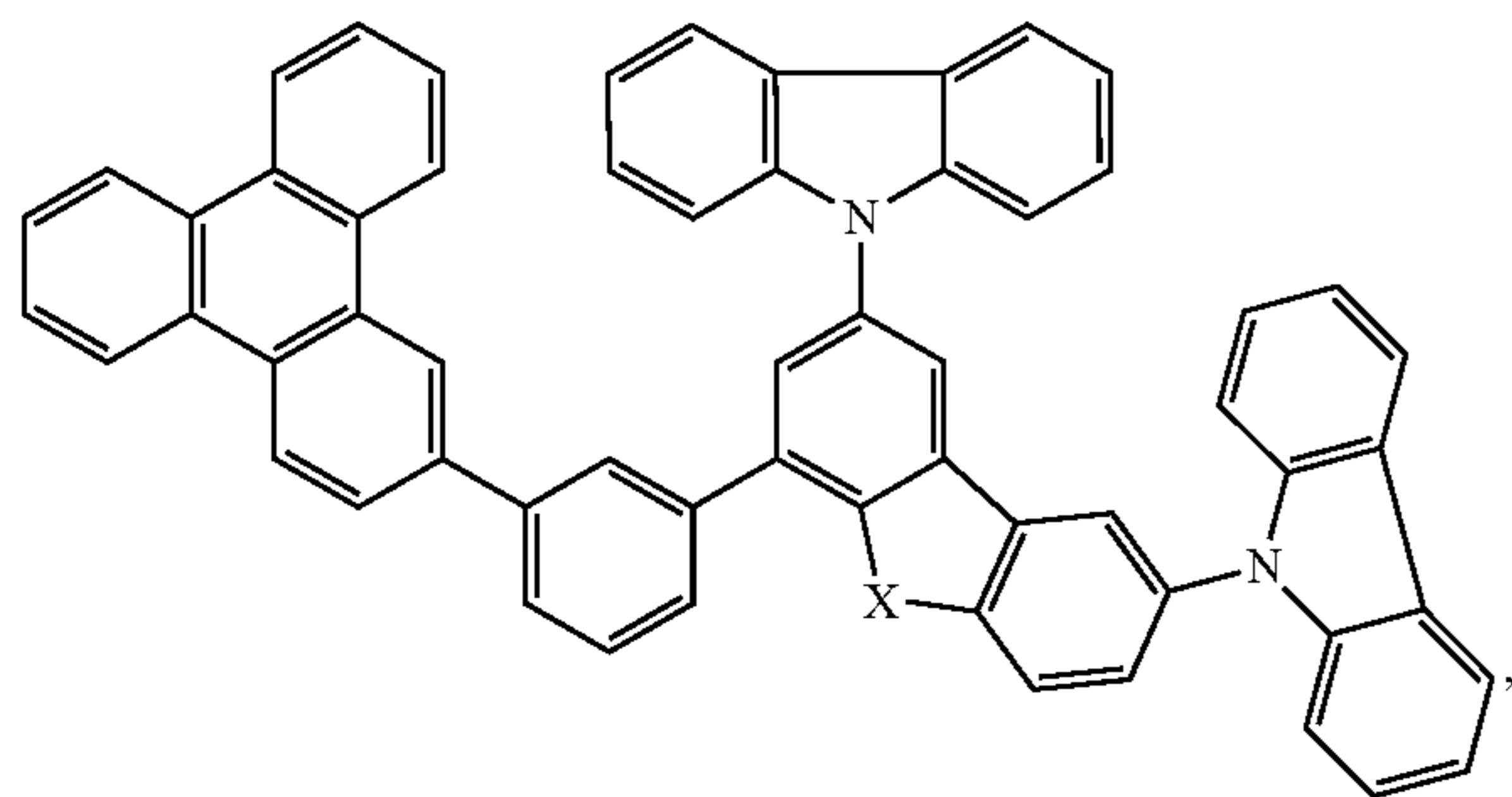
Compound 27
