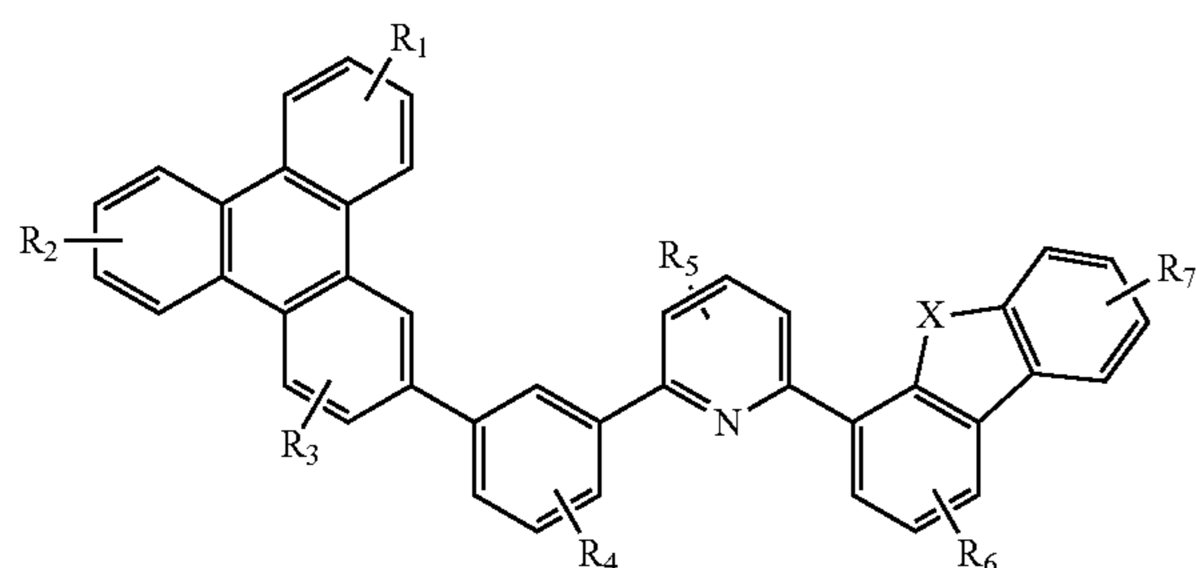
Compound 21 G
