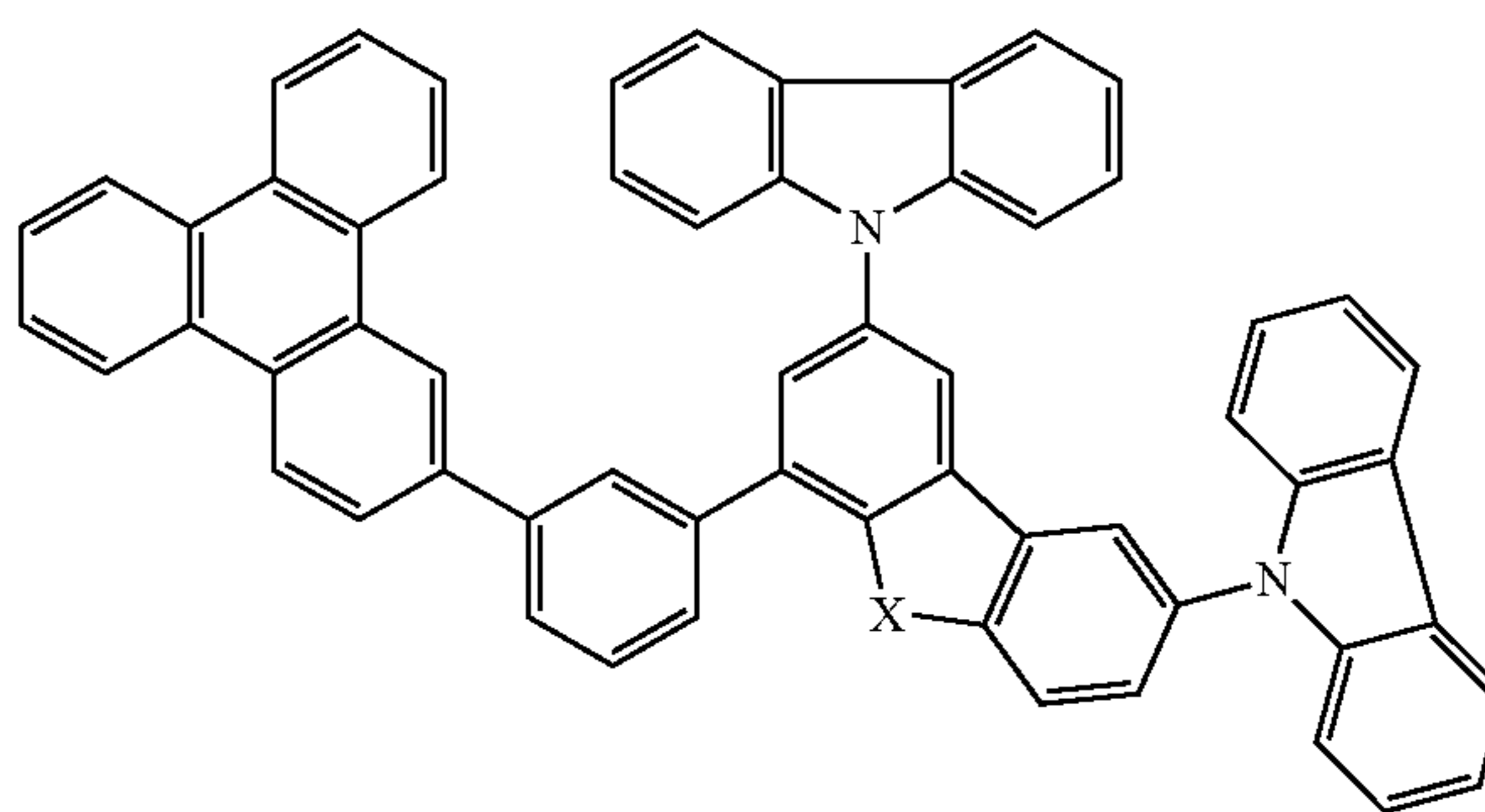
Compound 27
