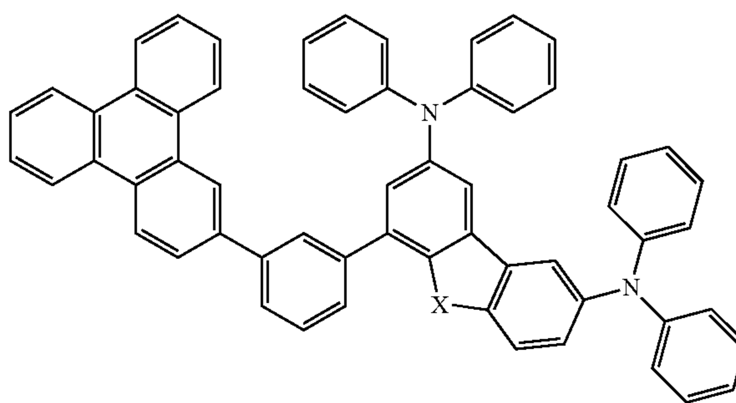
Compound 28
