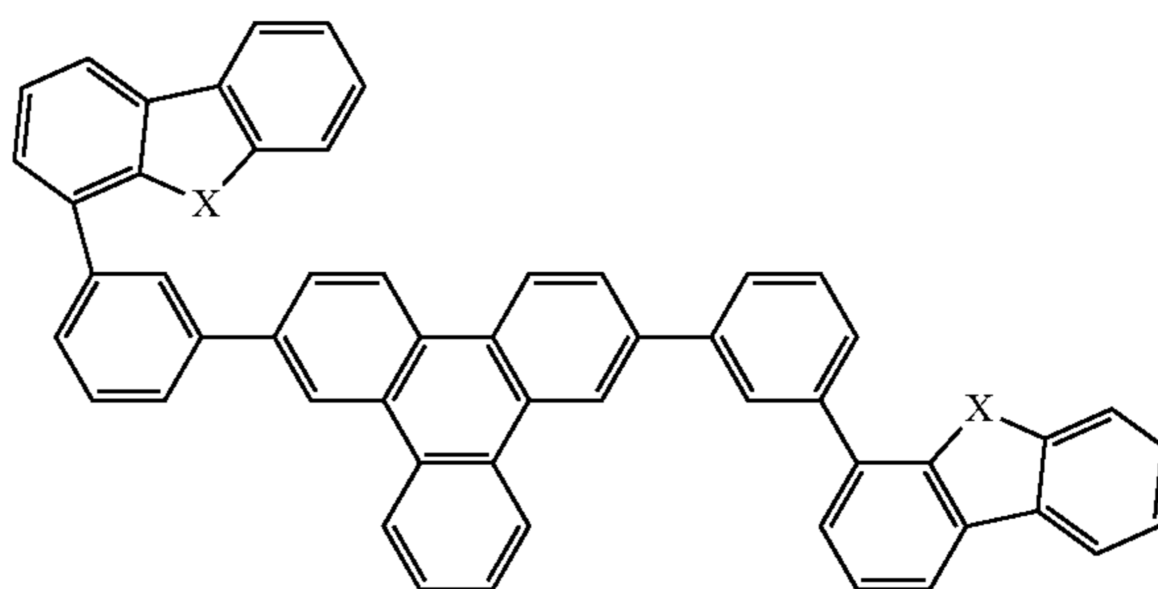
Compound 26
