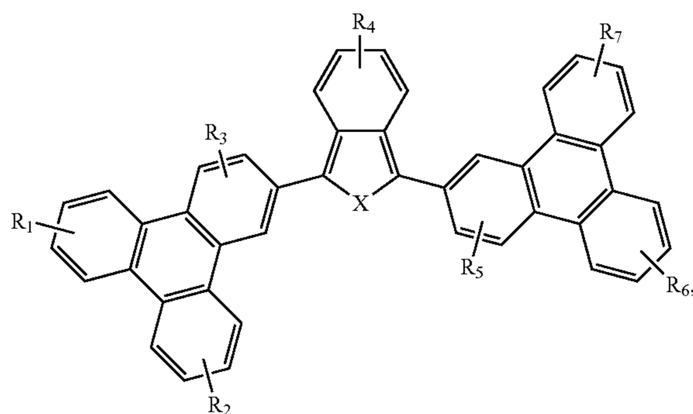
Compound 11G
