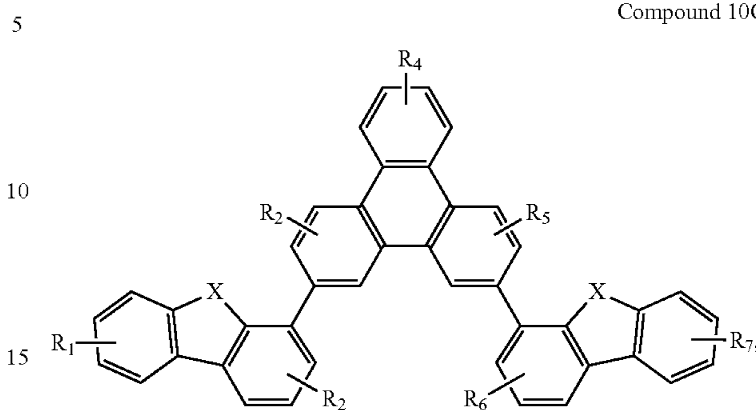
Compound 10G
