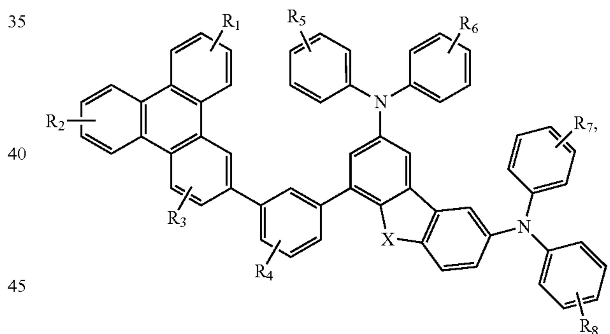
Compound 28 G
