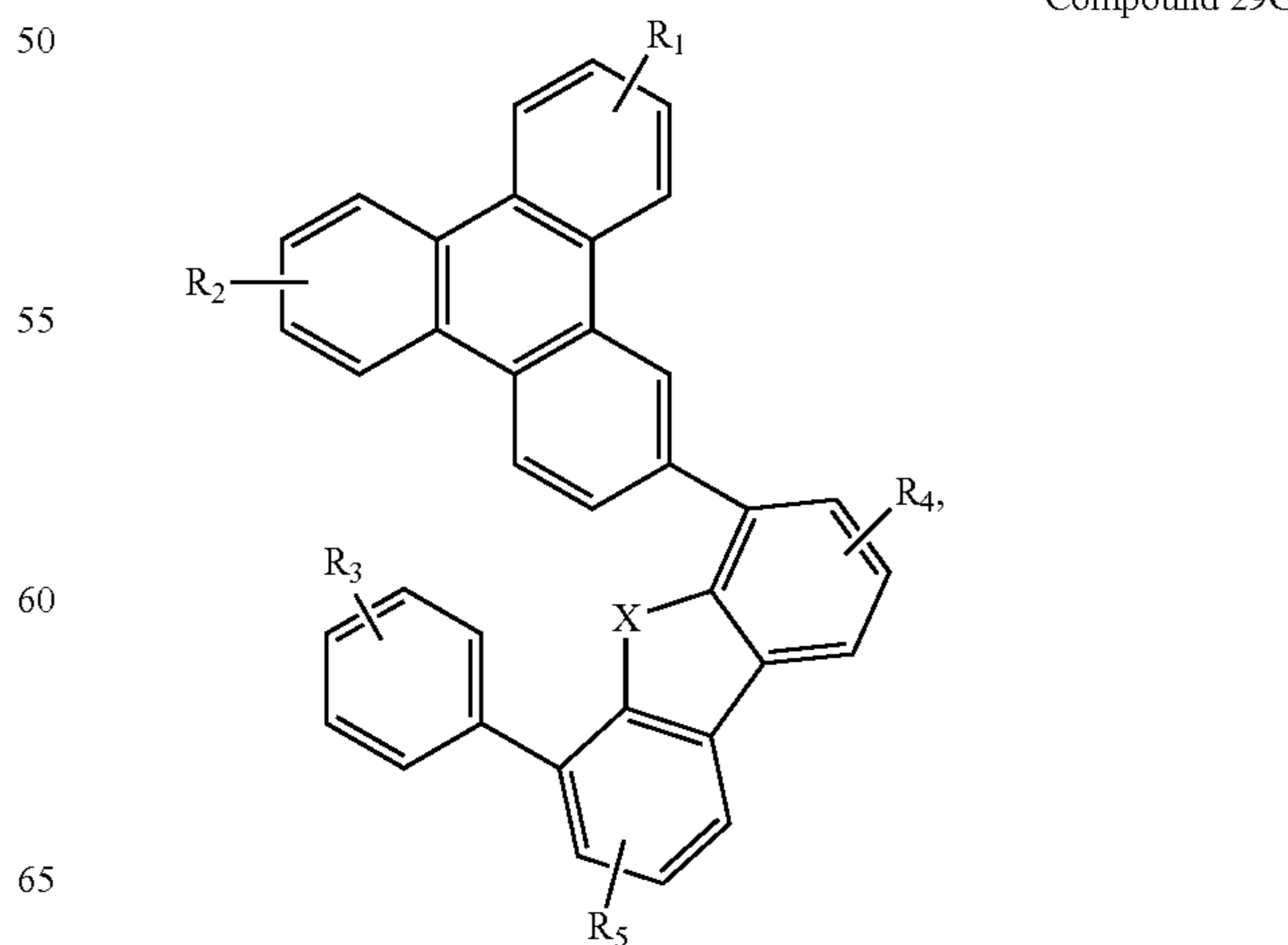
Compound 29G
