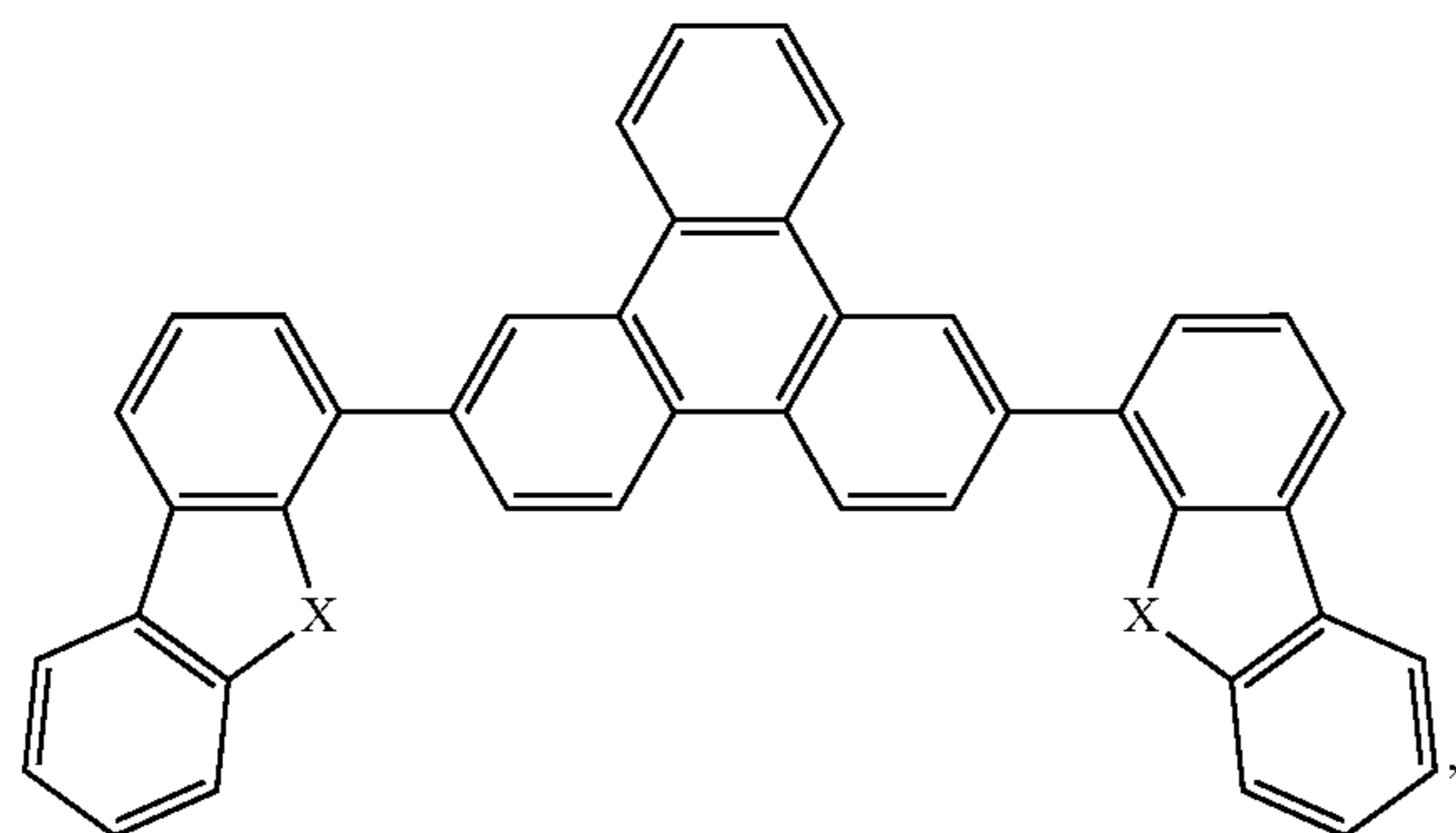
Compound 19
