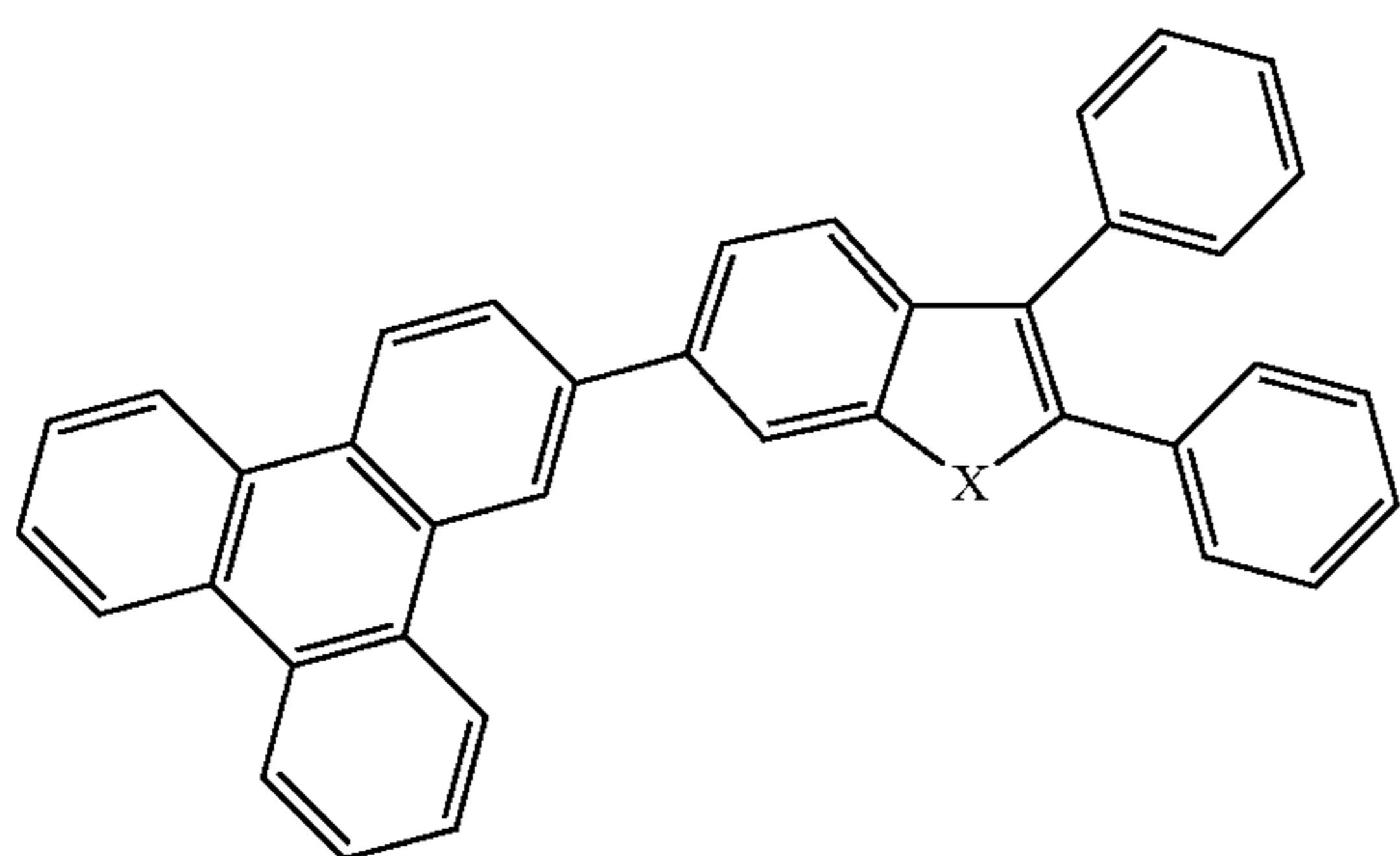
Compound 17
