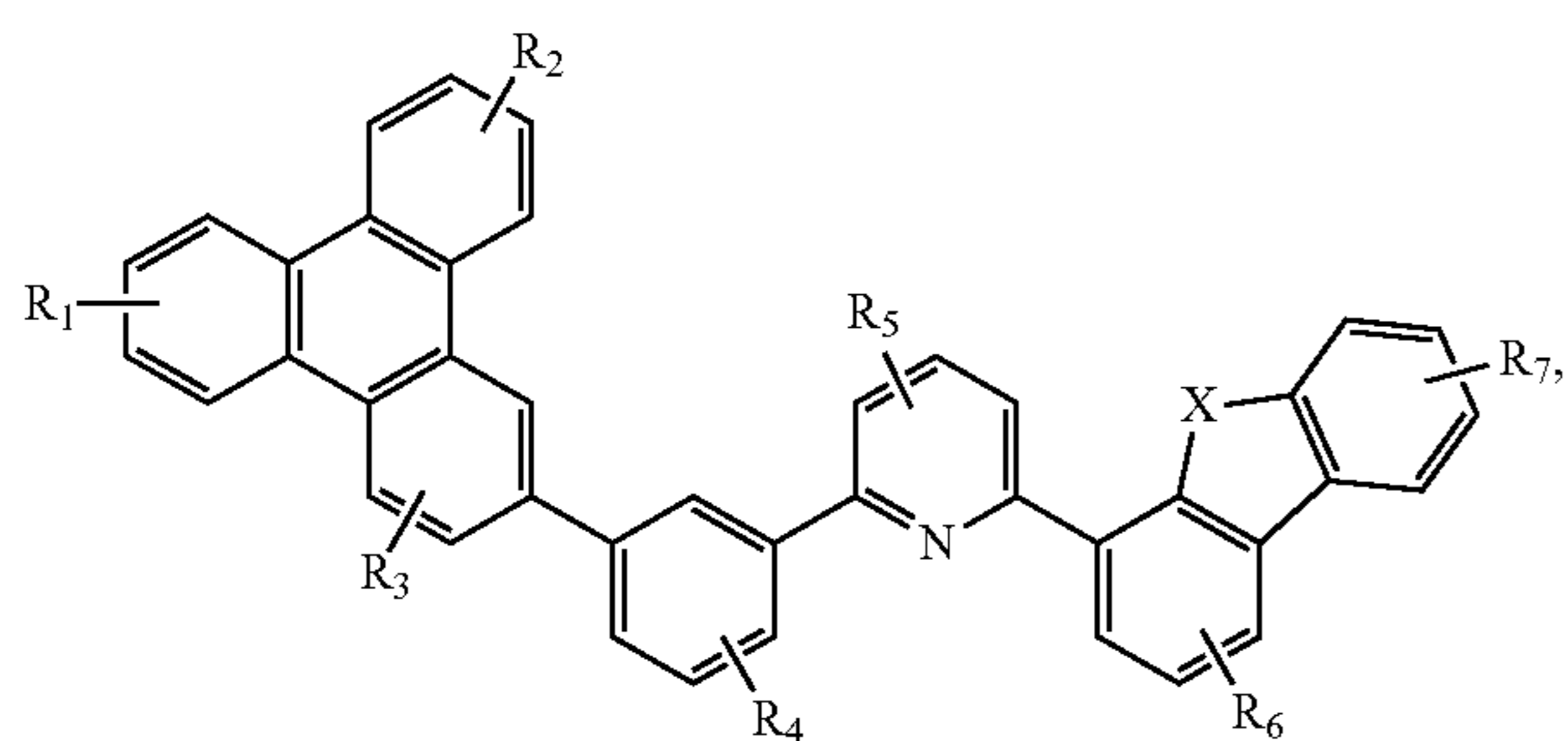
Compound 21G 55
