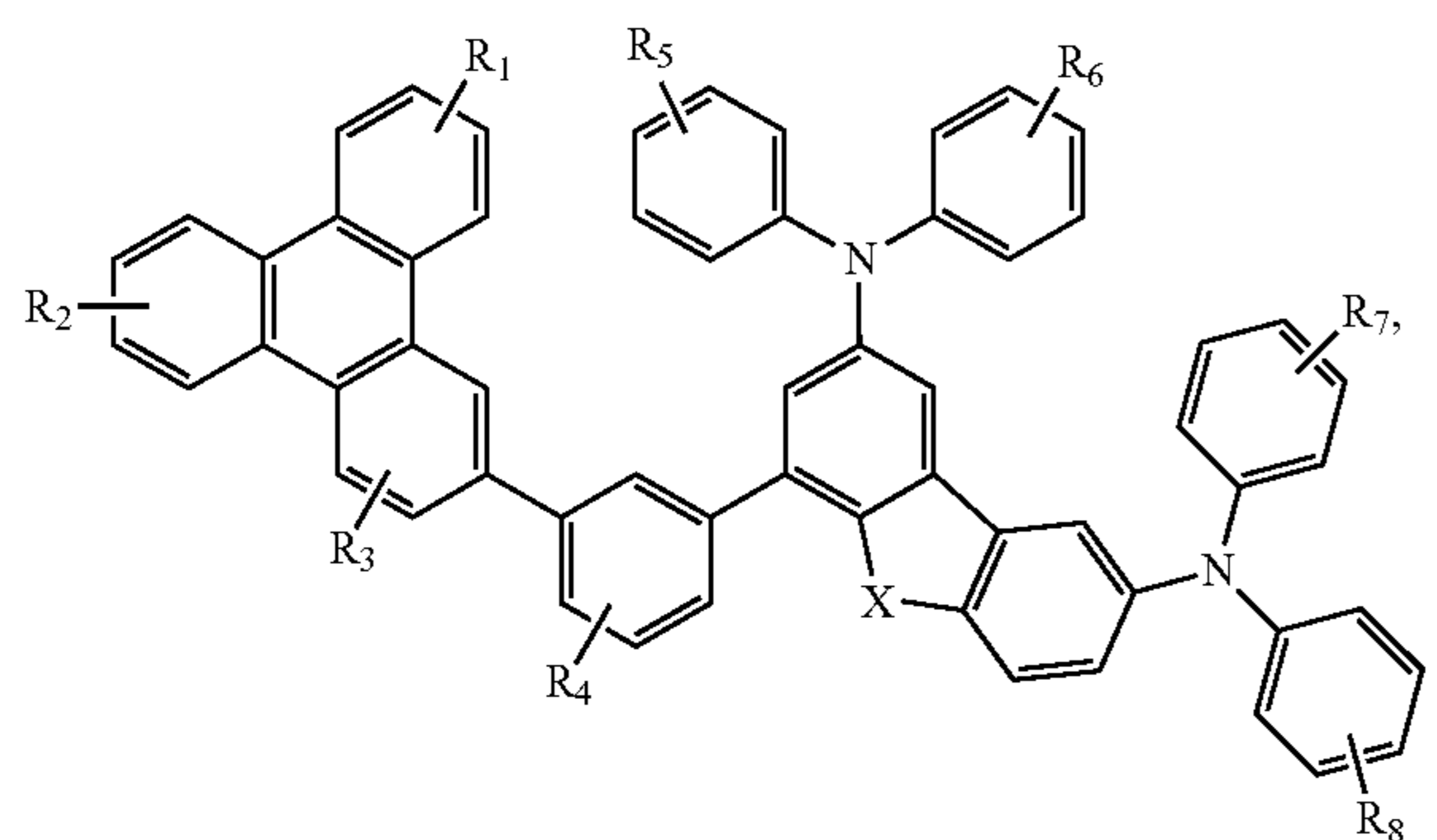
Compound 28G
