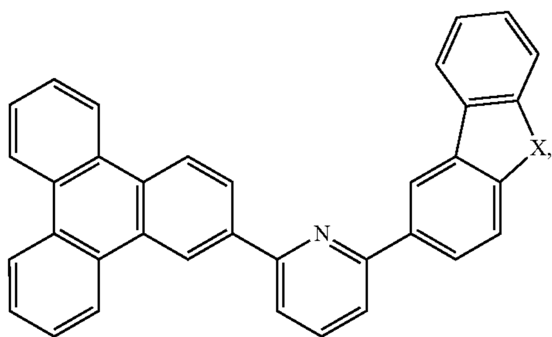
Compound 43
