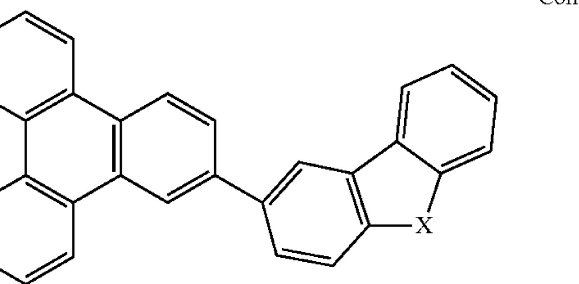
Compound 41
