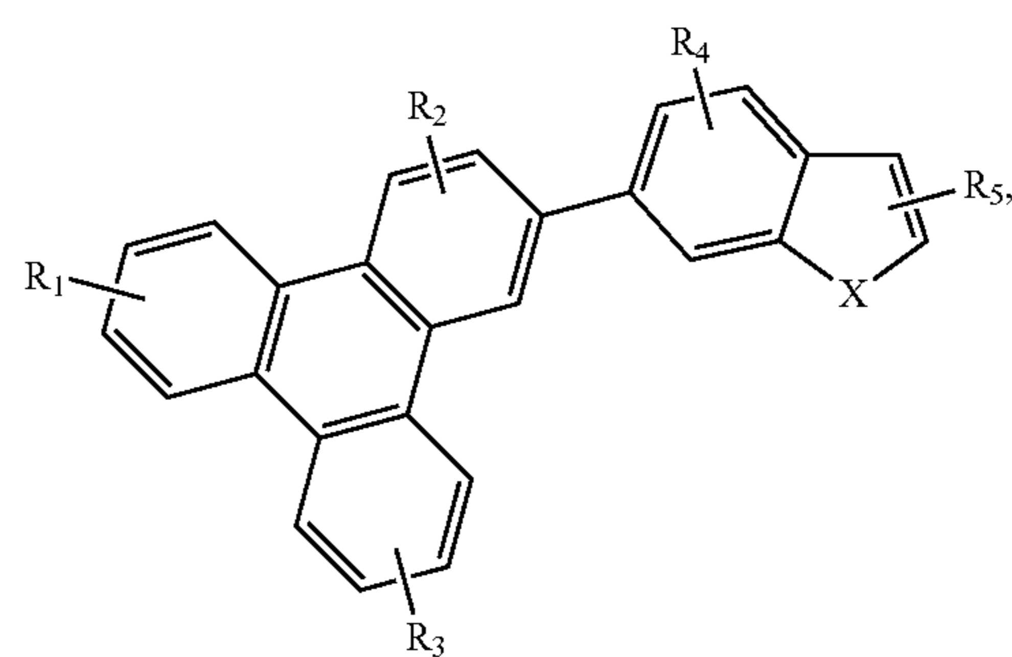
Compound 17G
