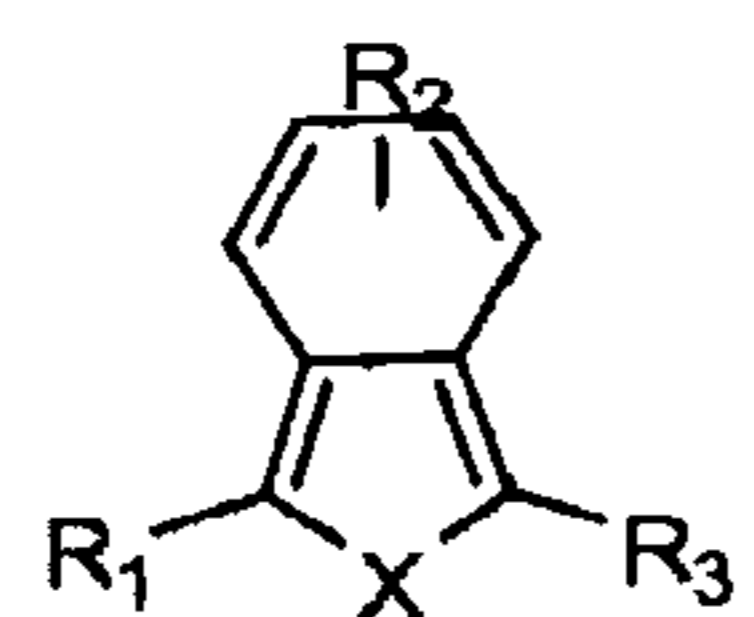
Formula (IV)
