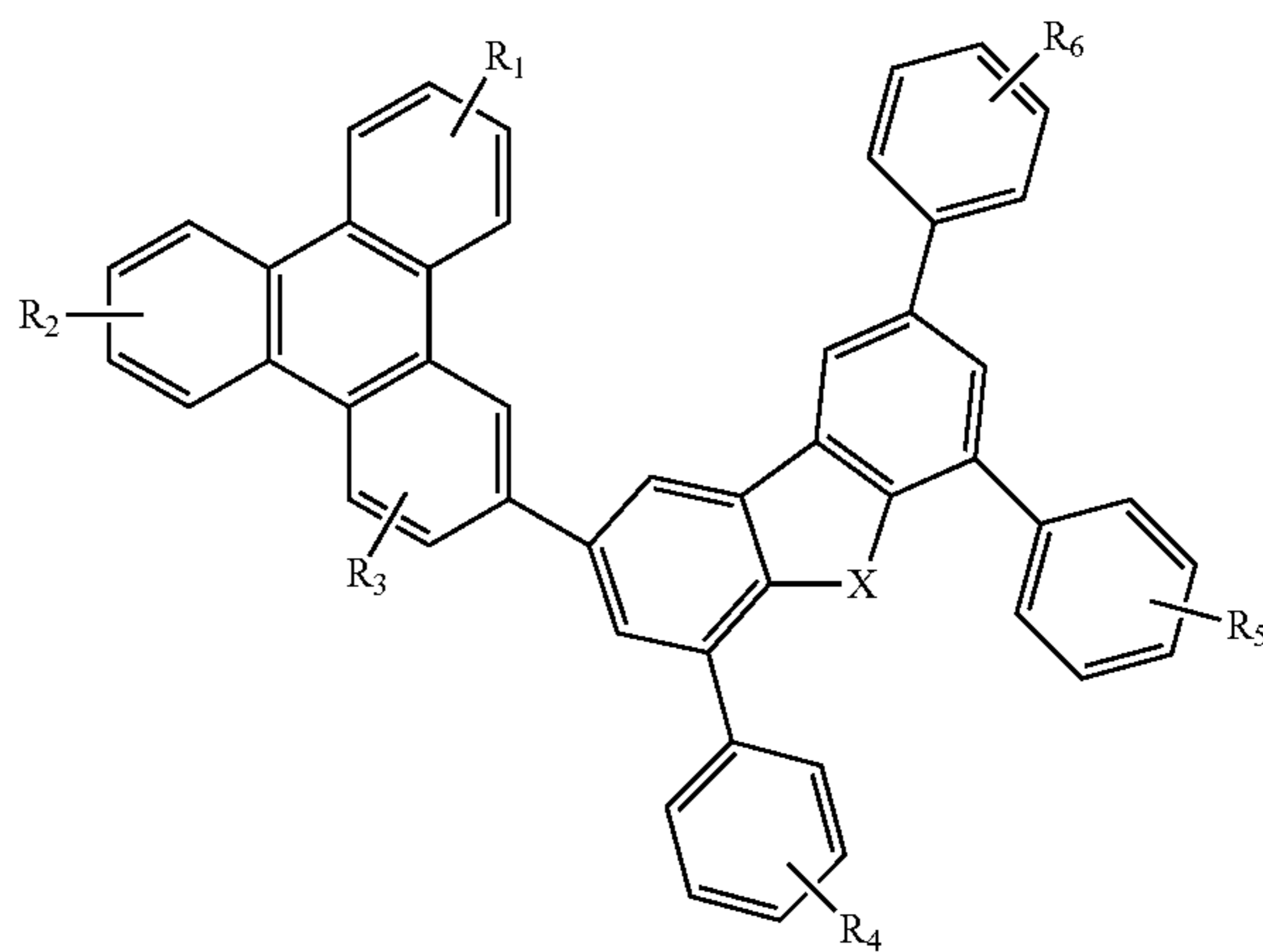
Compound 35G
