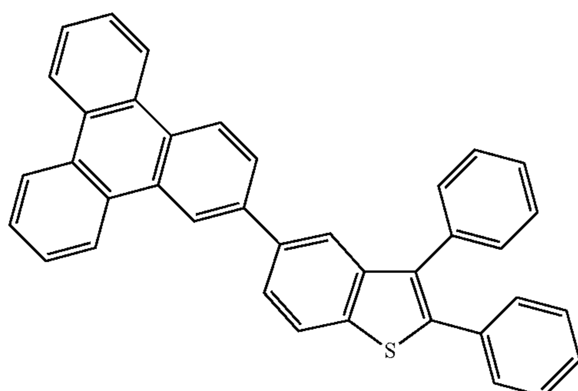
Compound 13' 20
