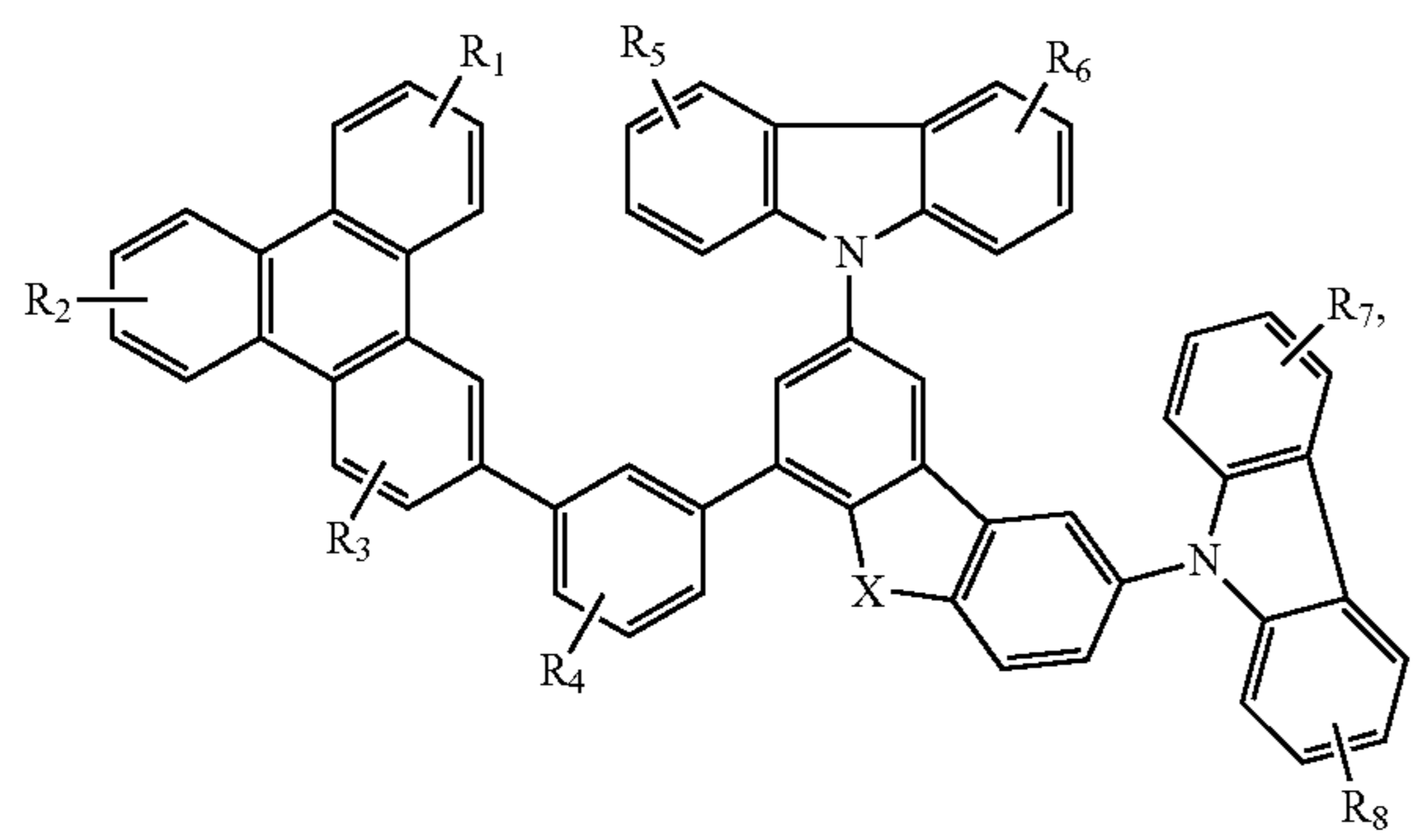
Compound 27G
