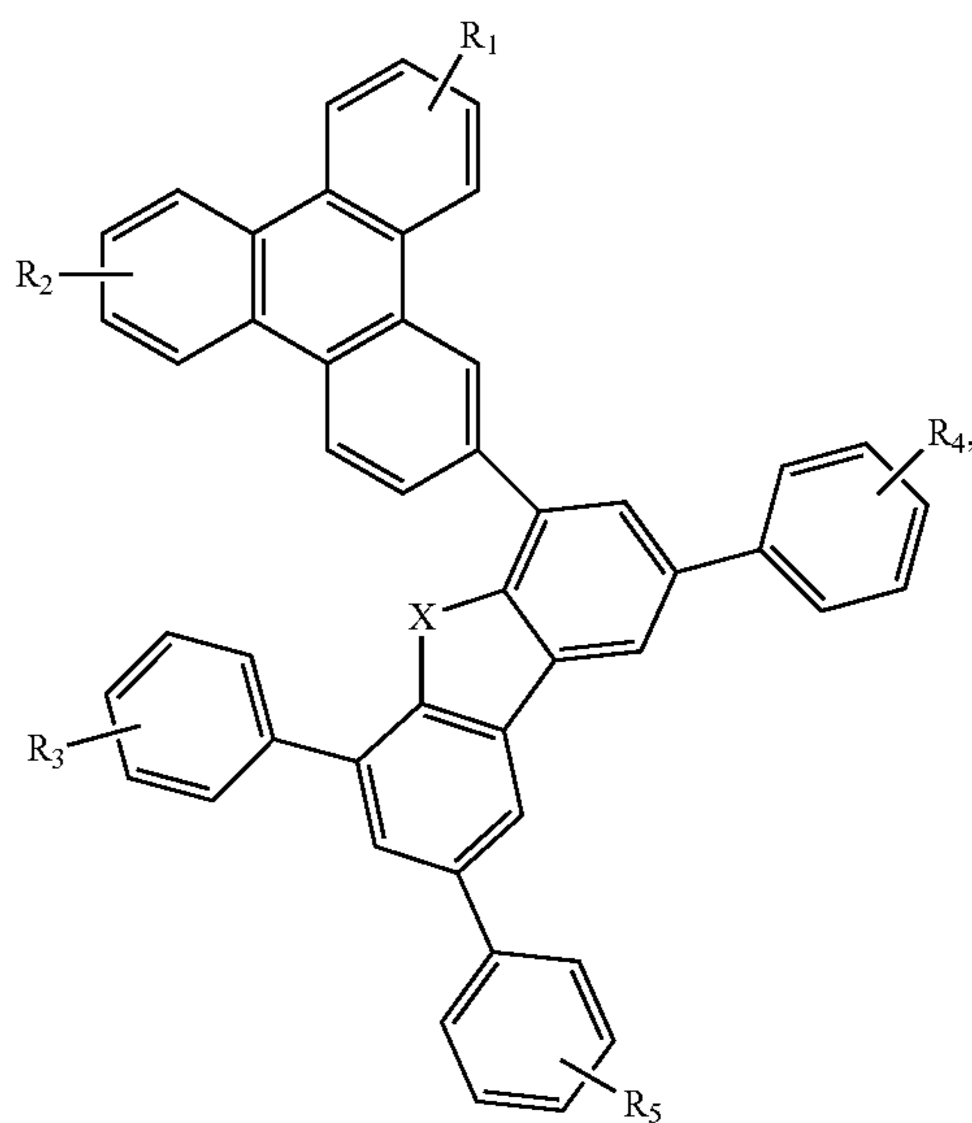
Compound 32G
