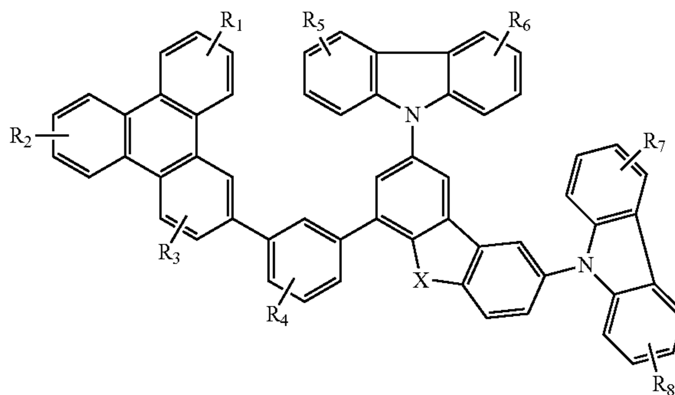
Compound 27 G
