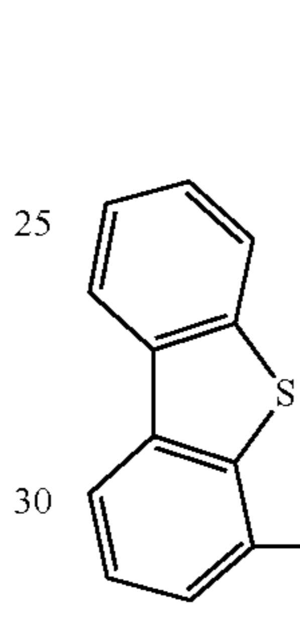
Compound 2'
