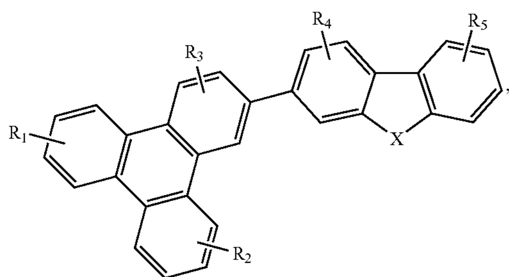
Compound 9G
