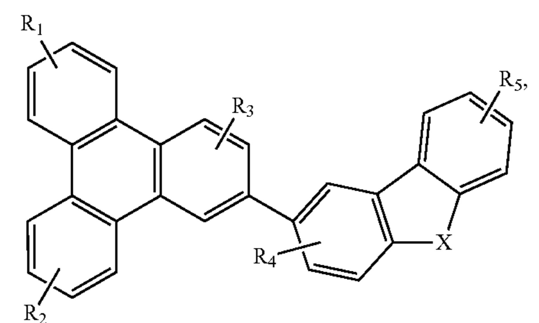
Compound 42G
