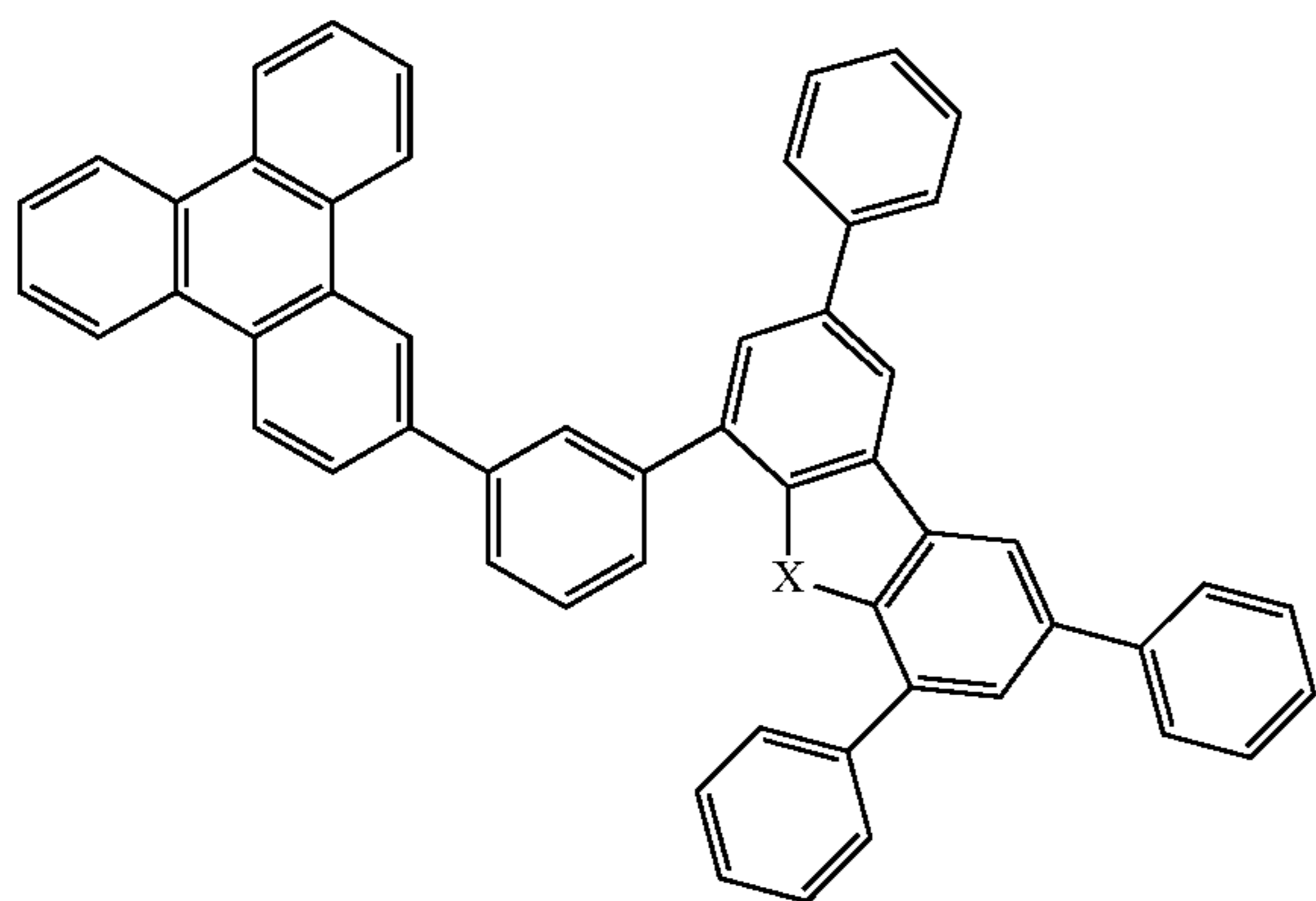
Compound 25
