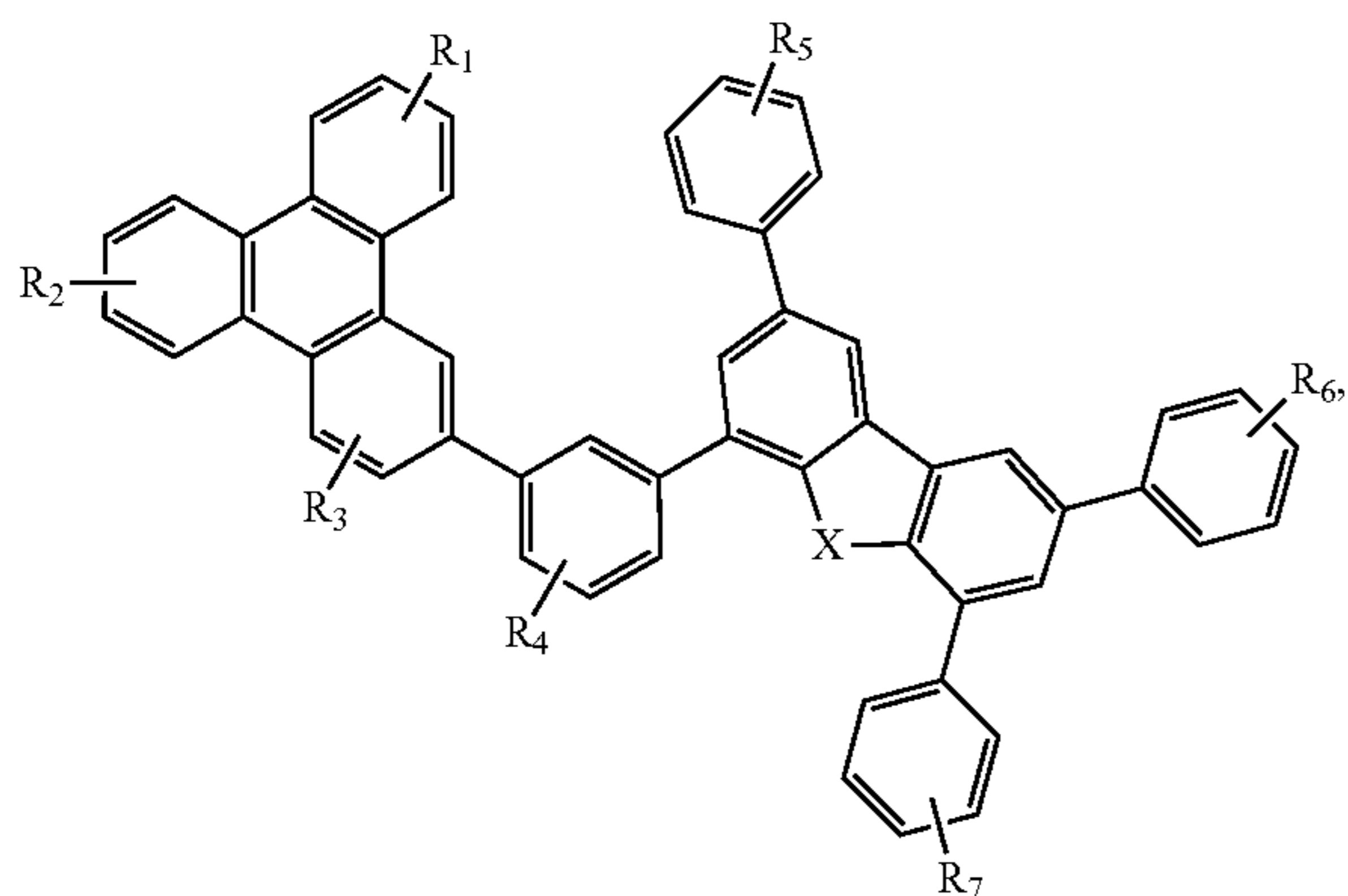
Compound 25G
