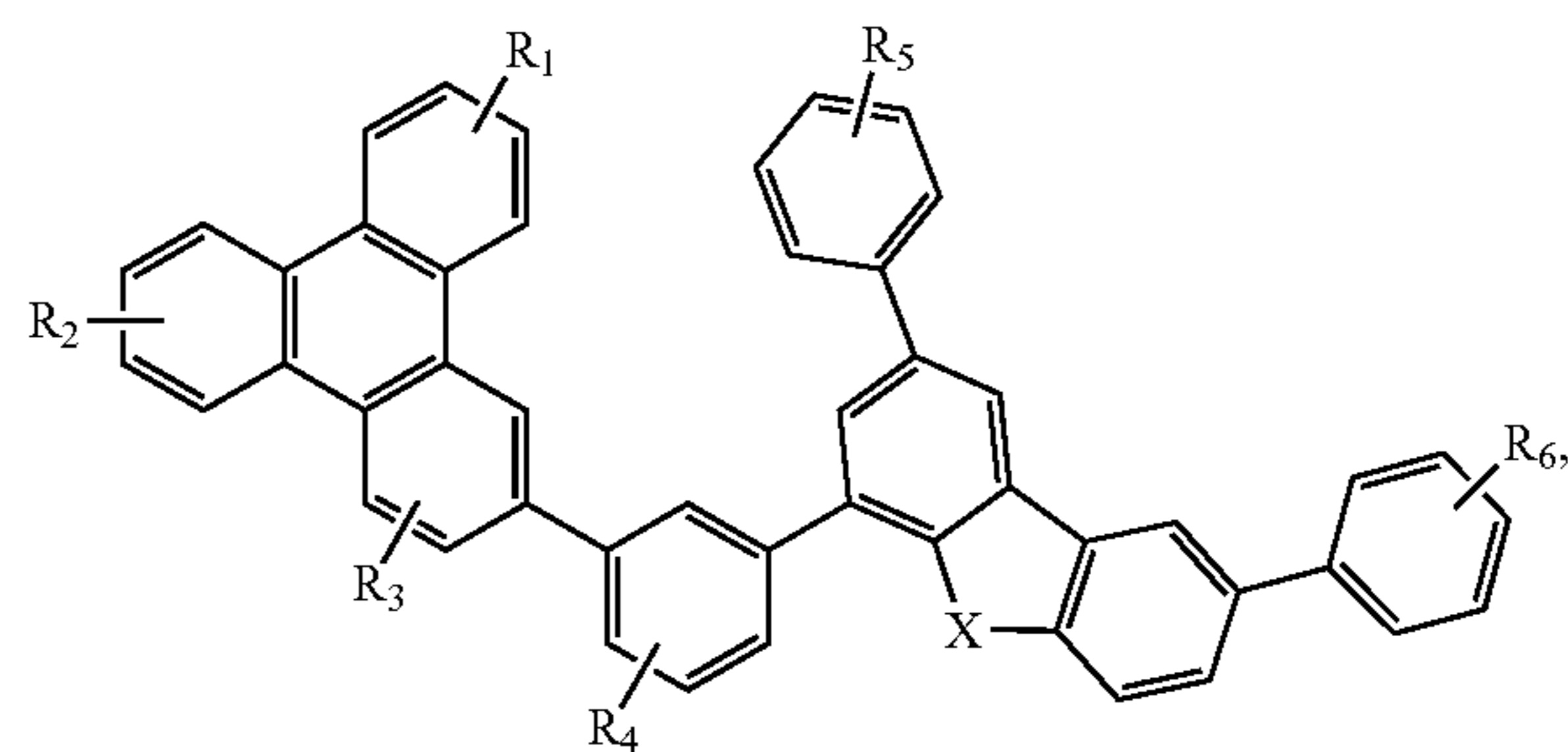
Compound 20G 40
