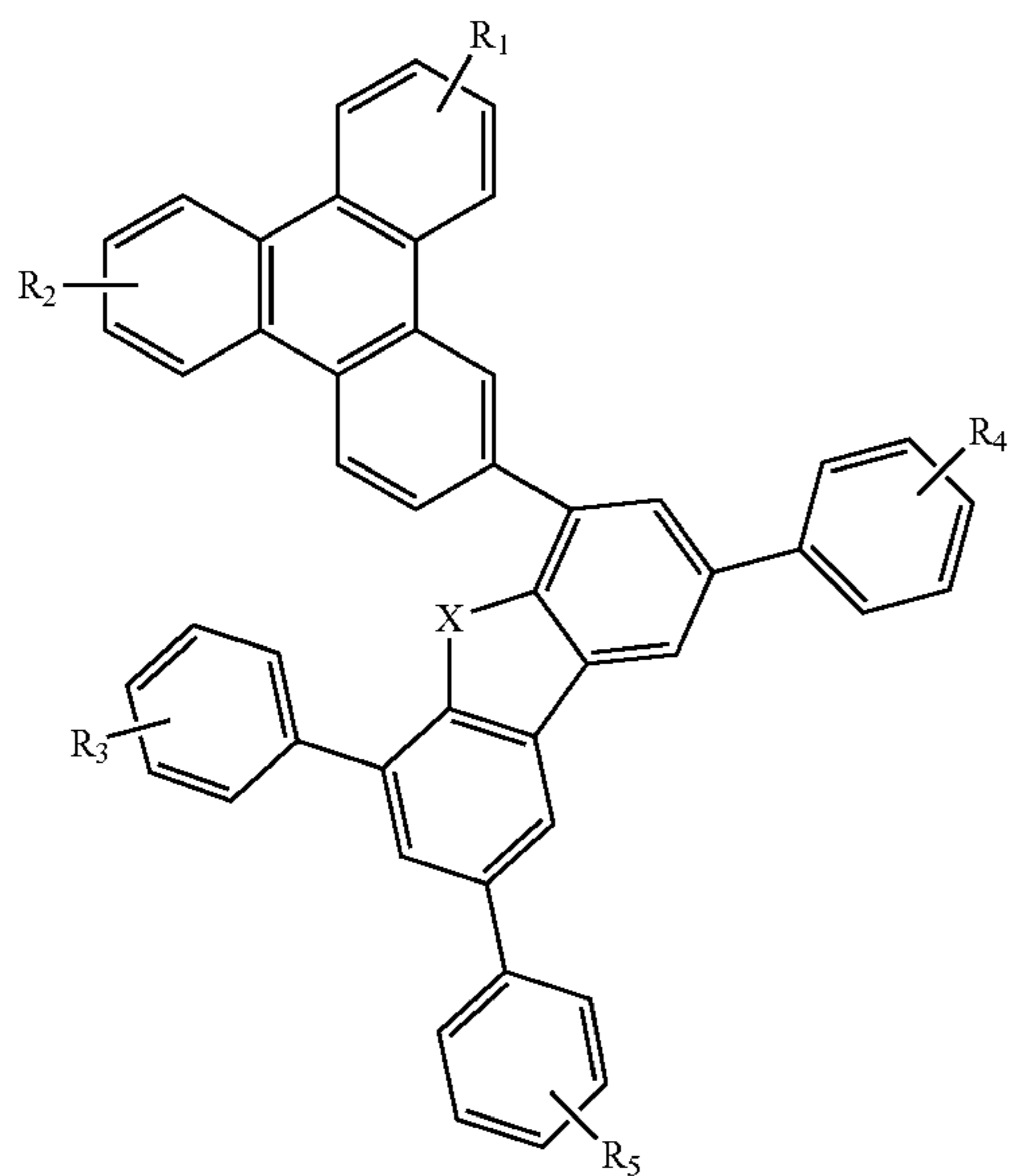
Compound 32G
