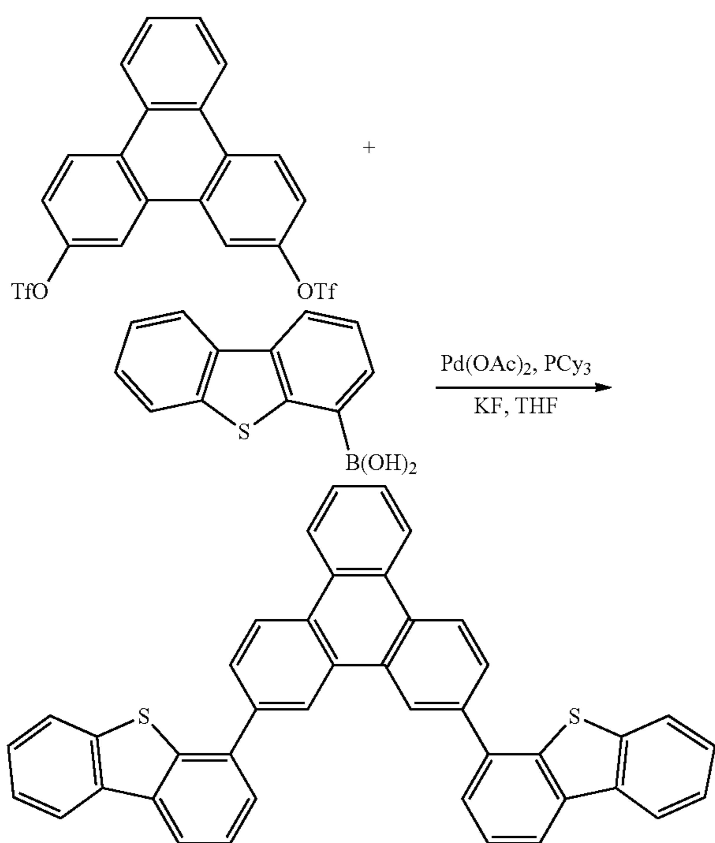
Compound 10S
