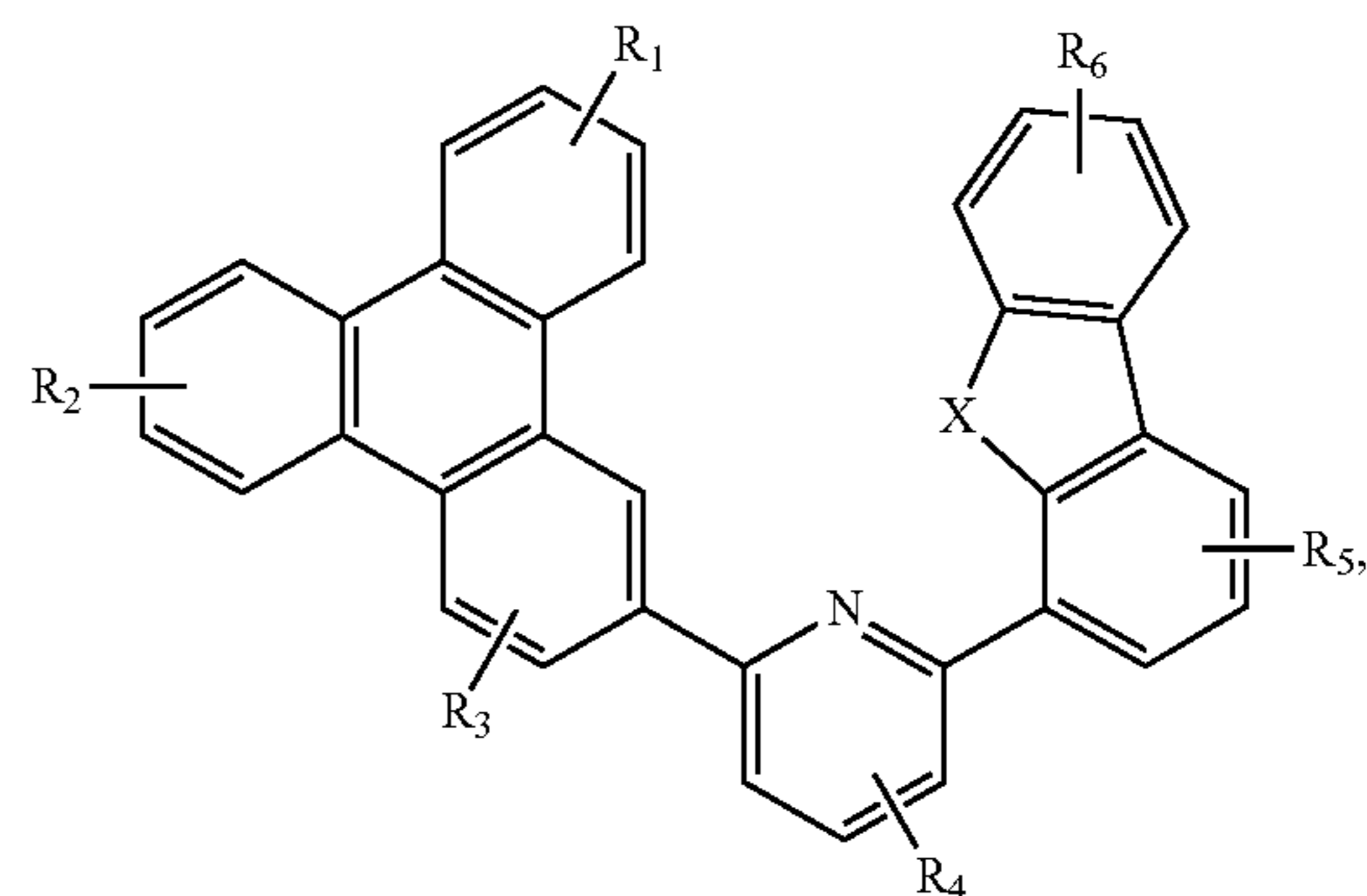
Compound 18G 5
