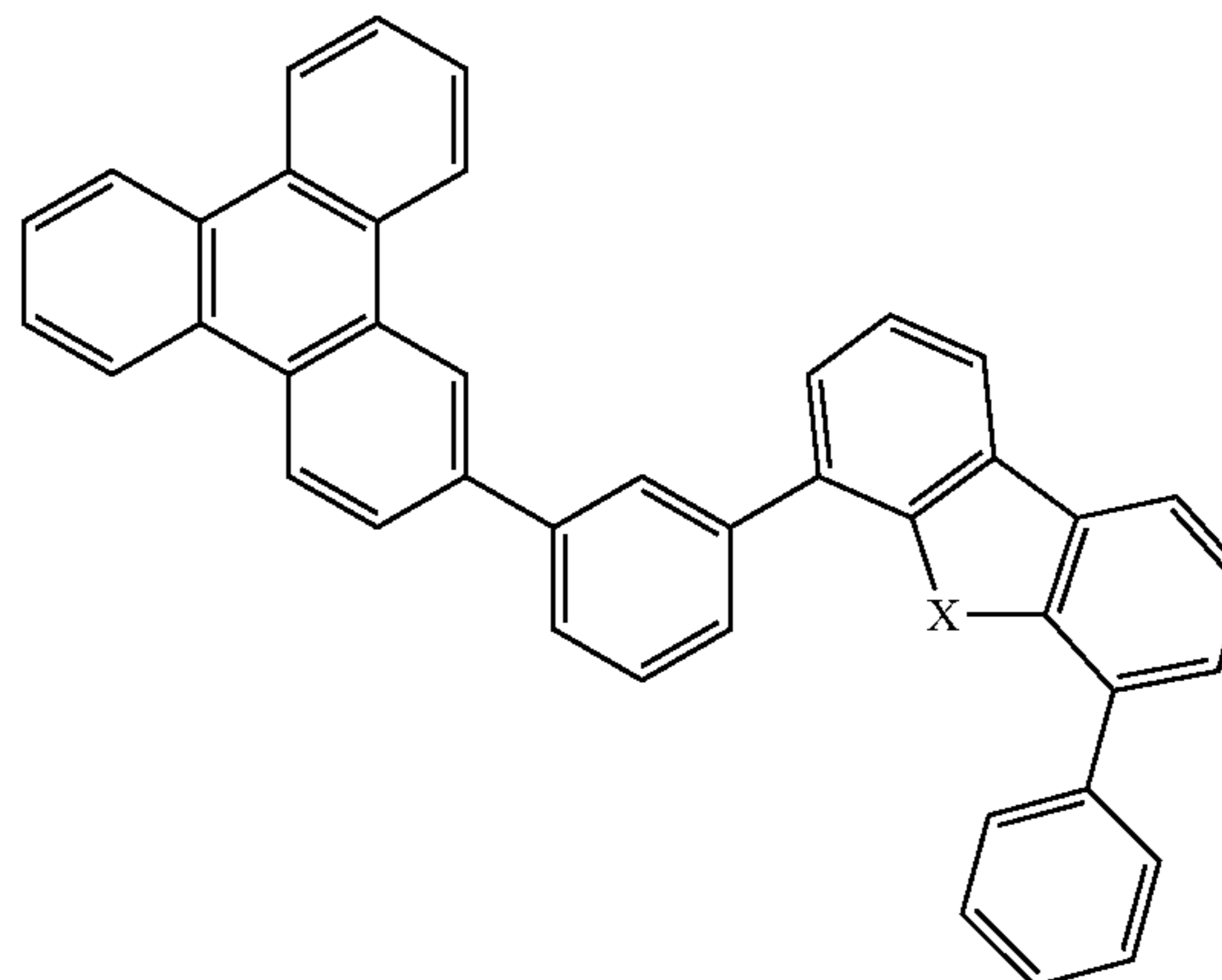
Compound 23
