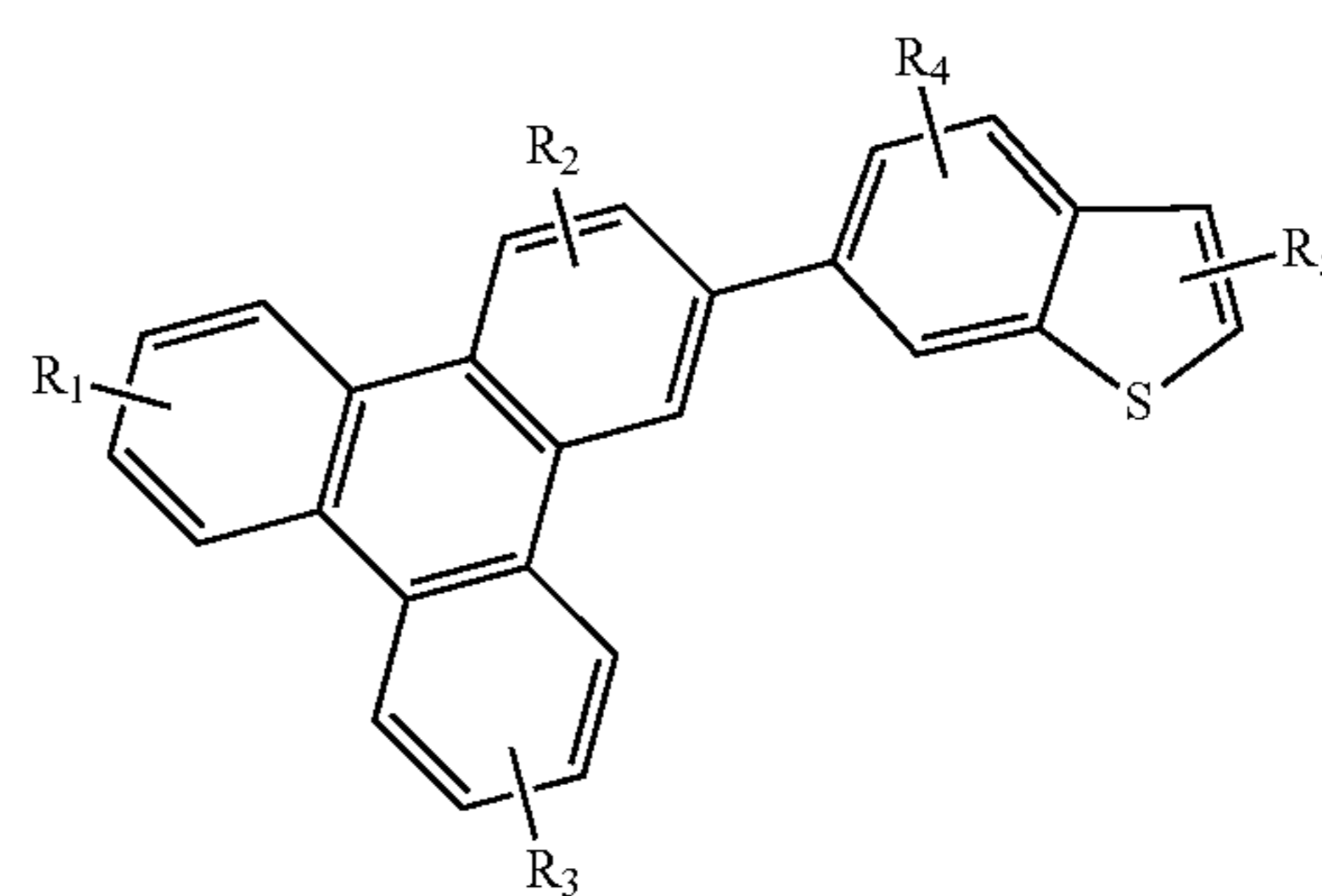
Compound 17'G
