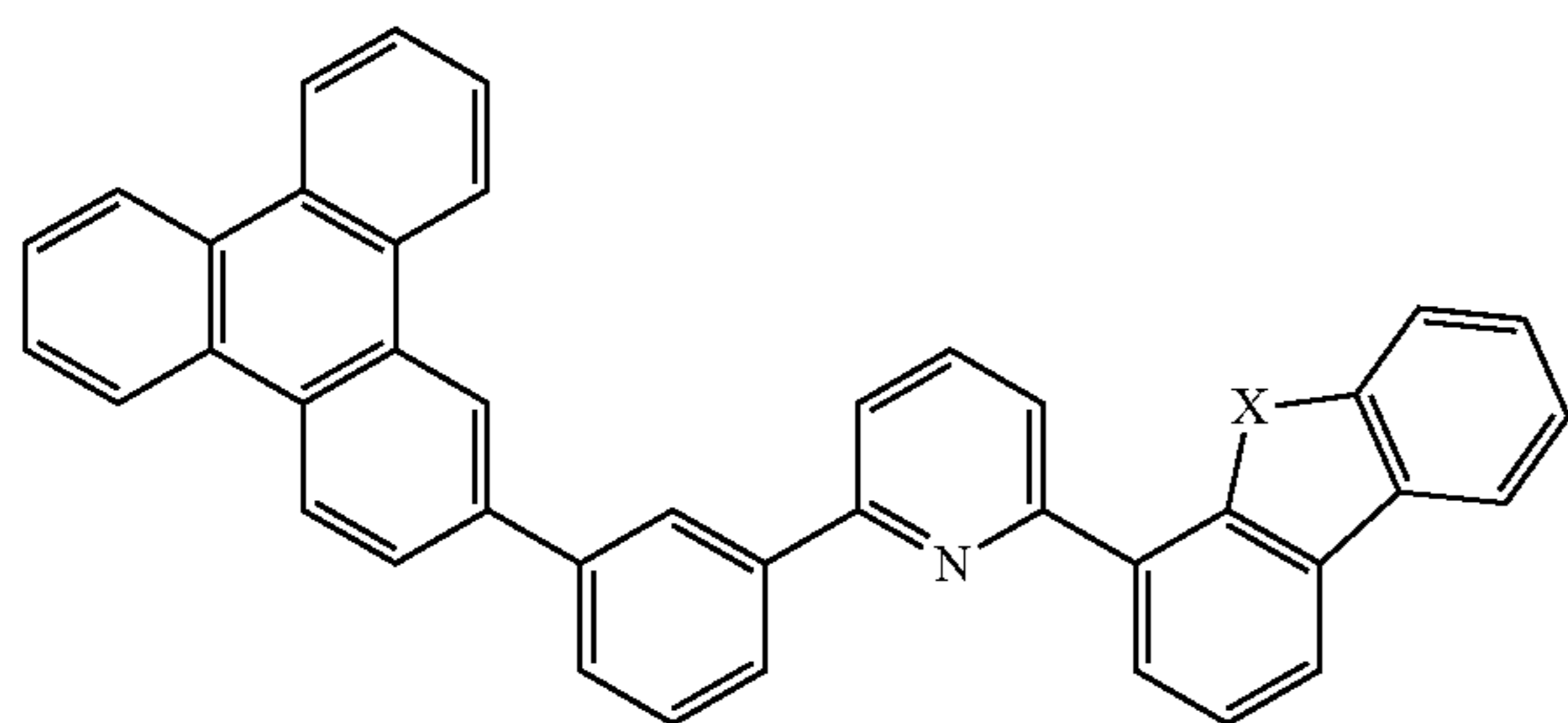
Compound 22 G
