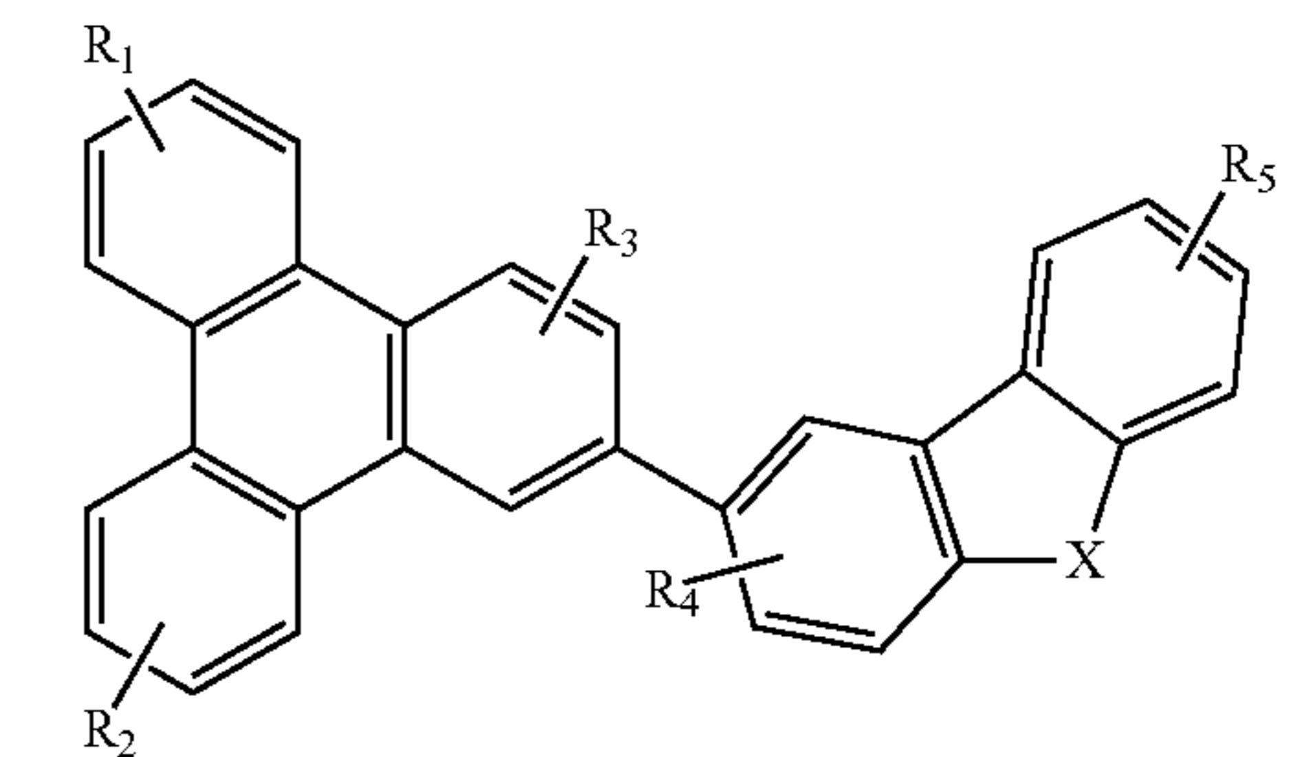
Compound 41G
