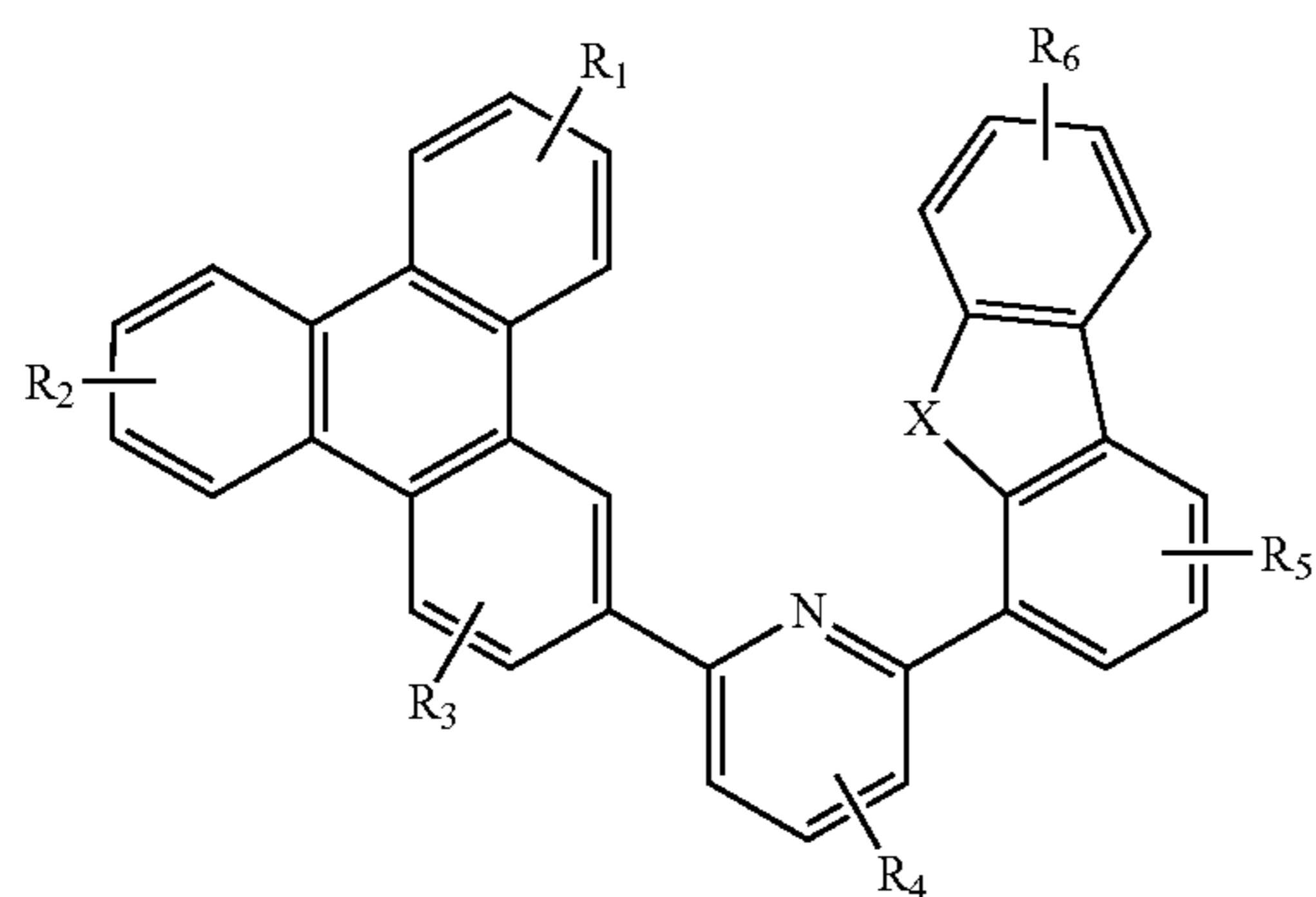
Compound 22
