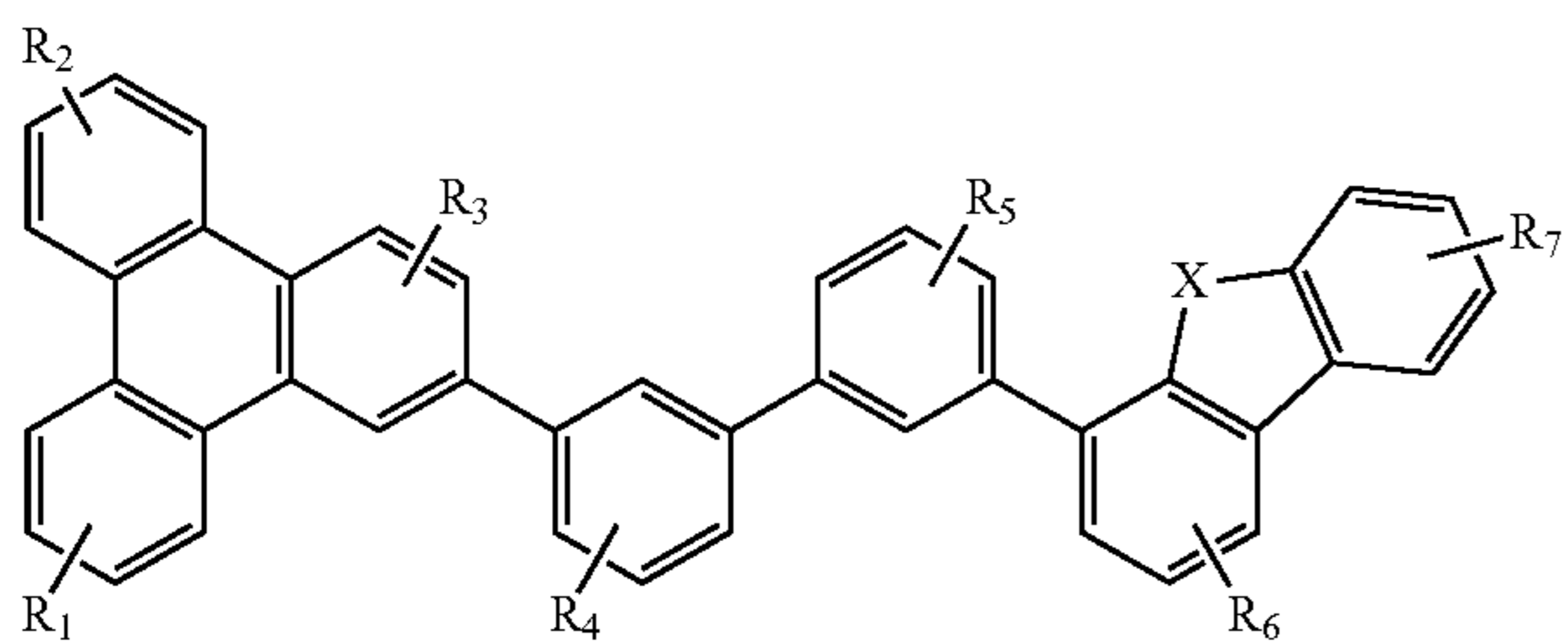
Compound 9G
