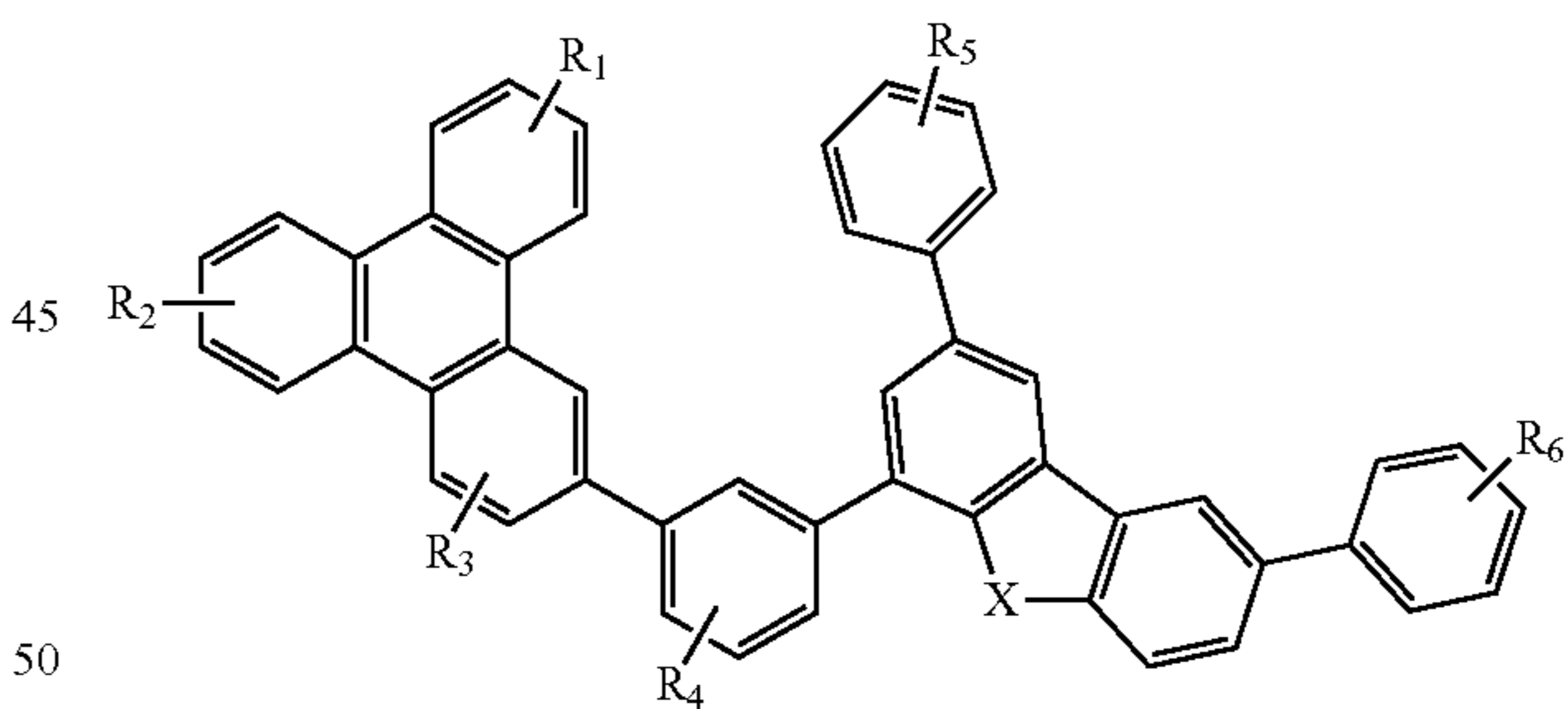
Compound 24 G
