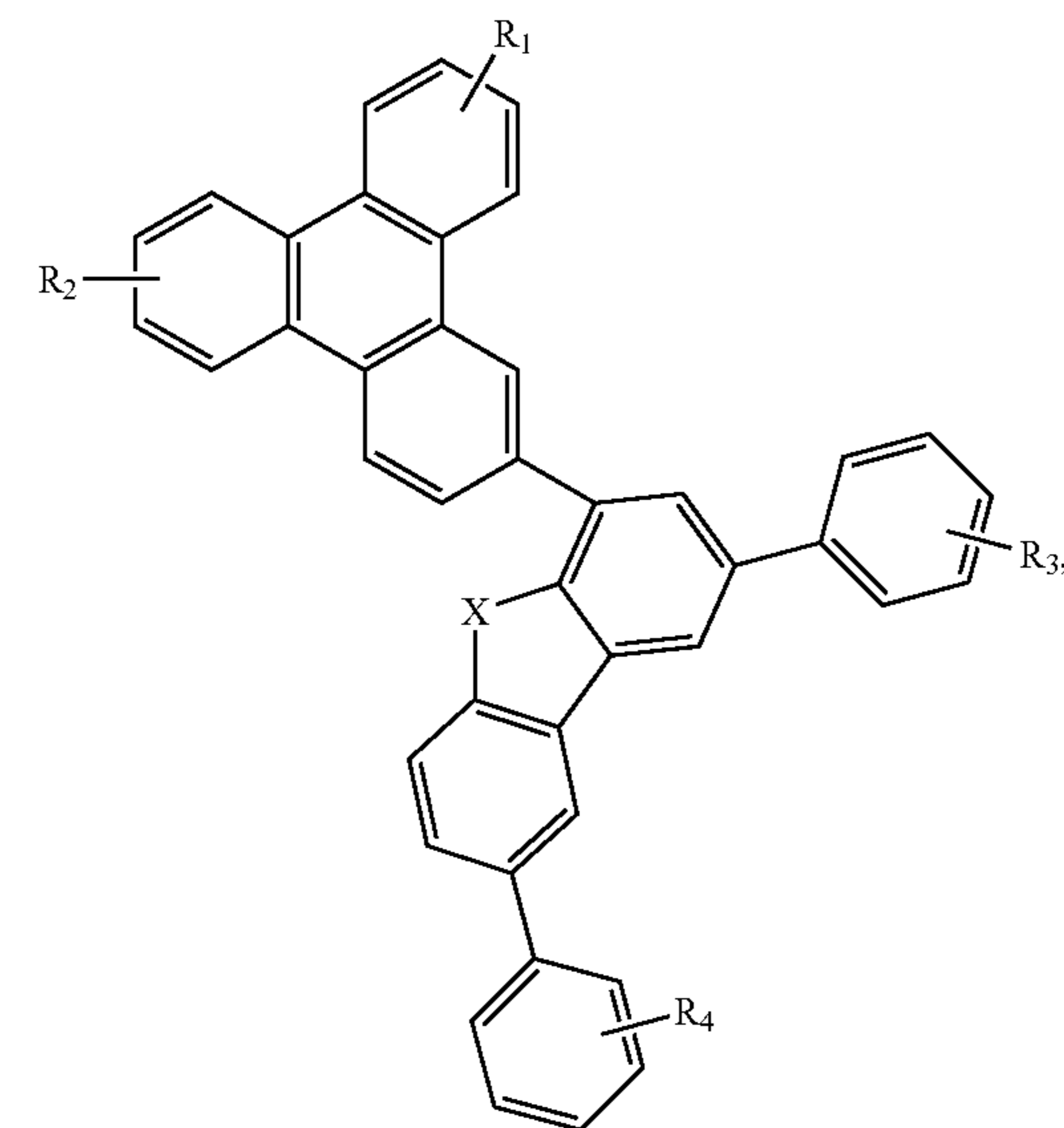
Compound 32G
