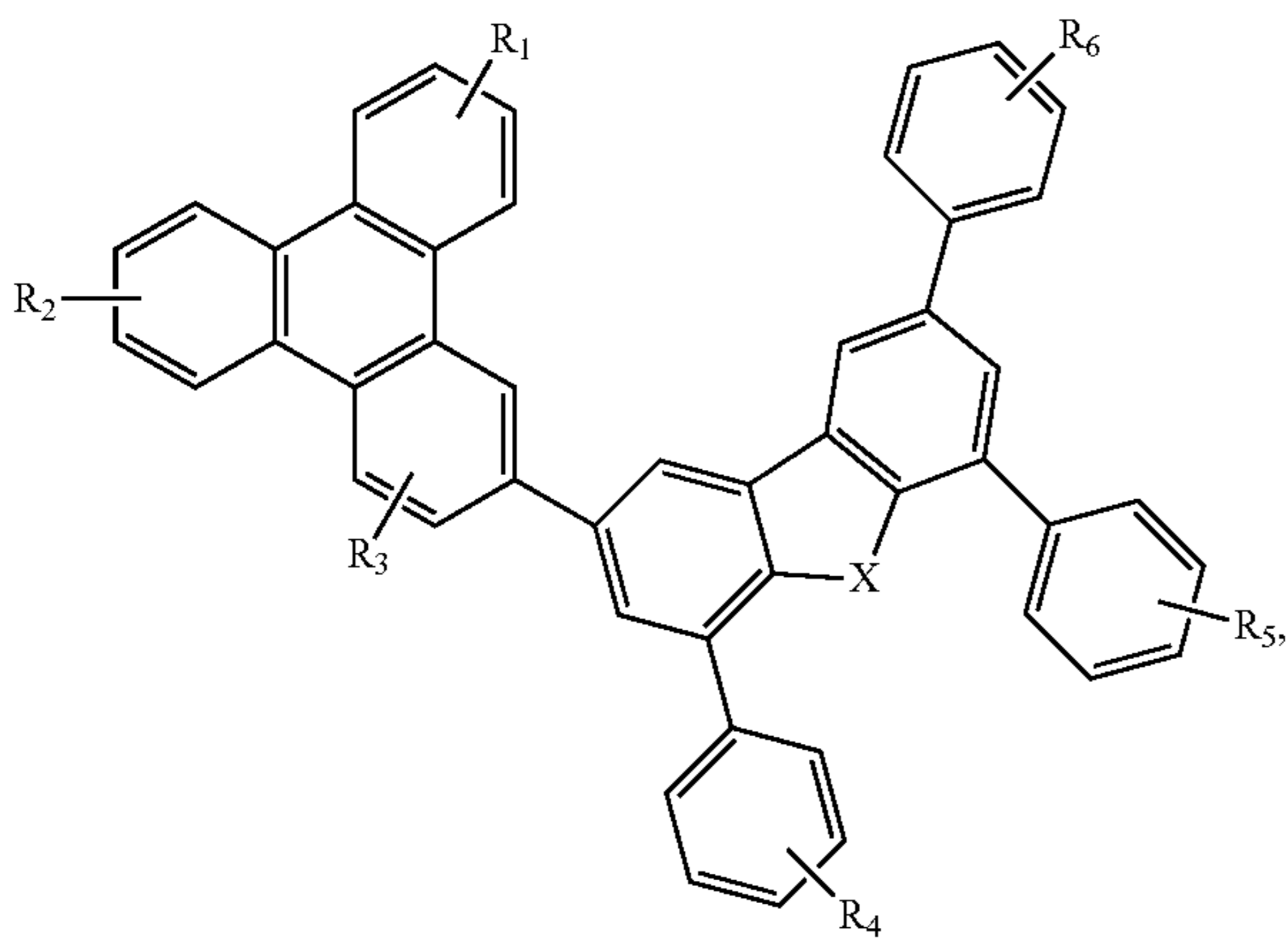
Compound 35G
