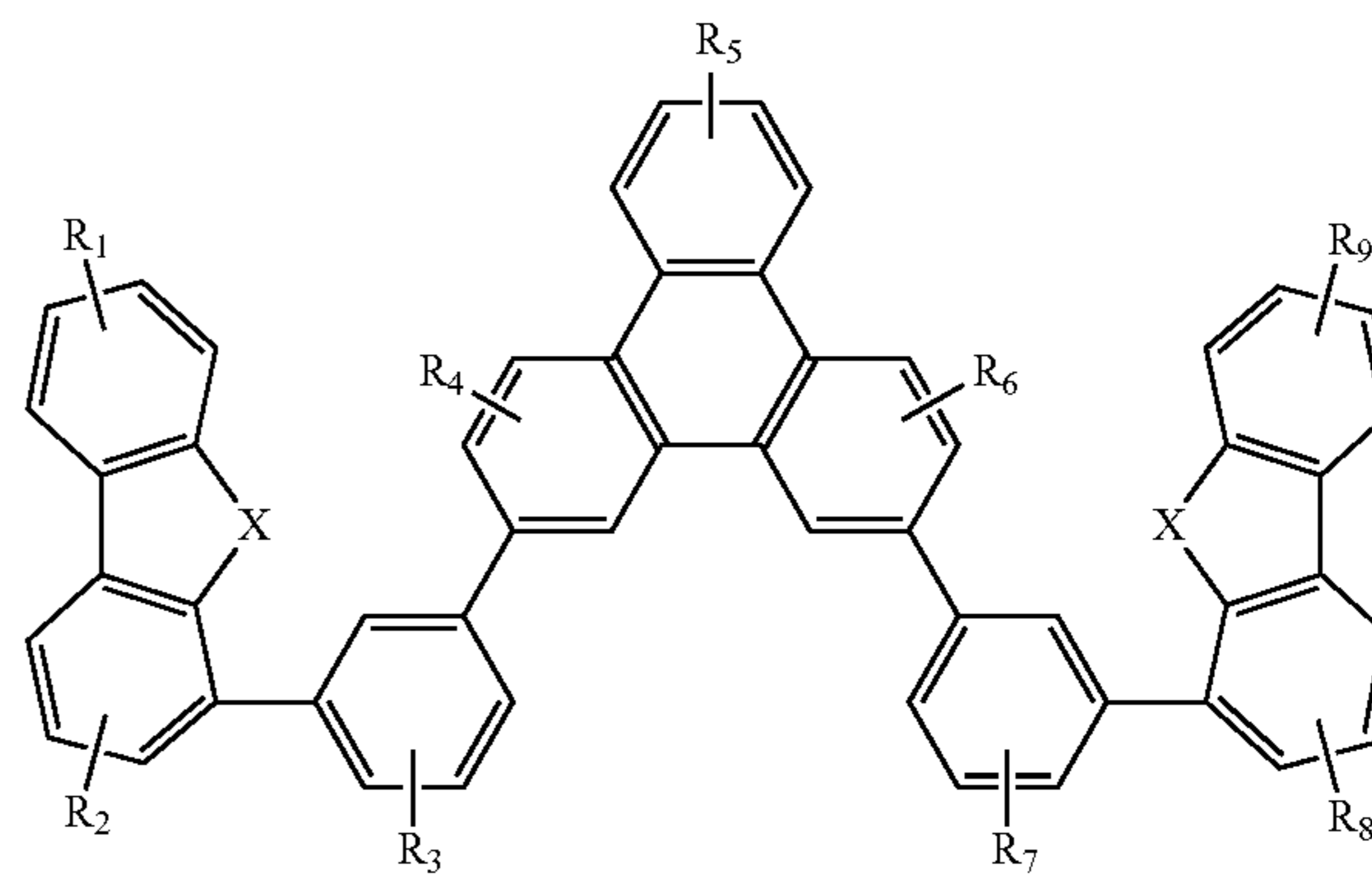
Compound 4G
