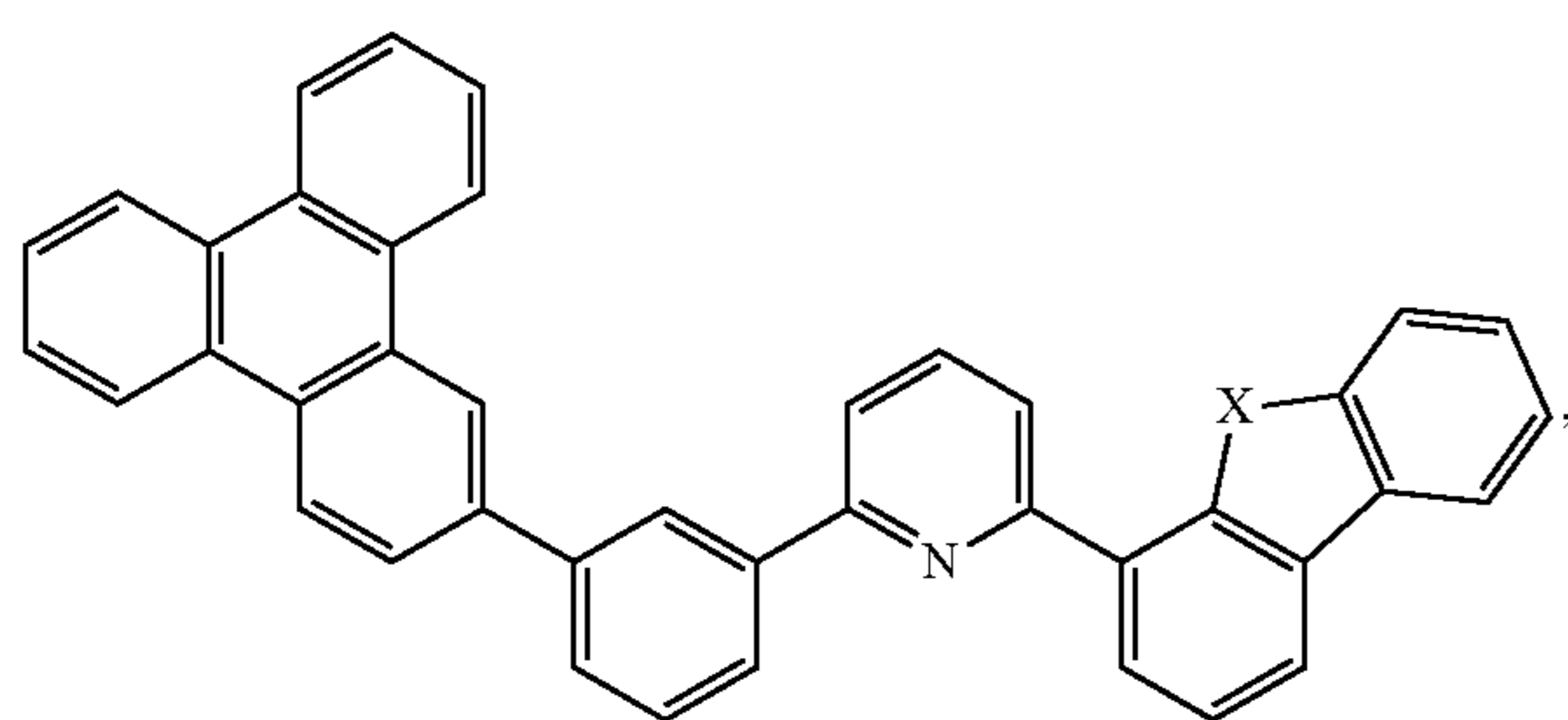
Compound 21
