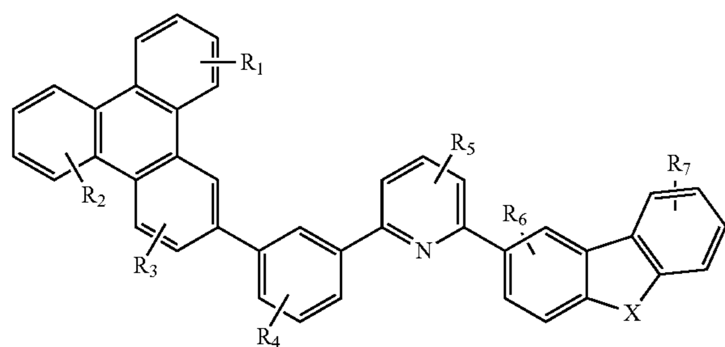
Compound 44
