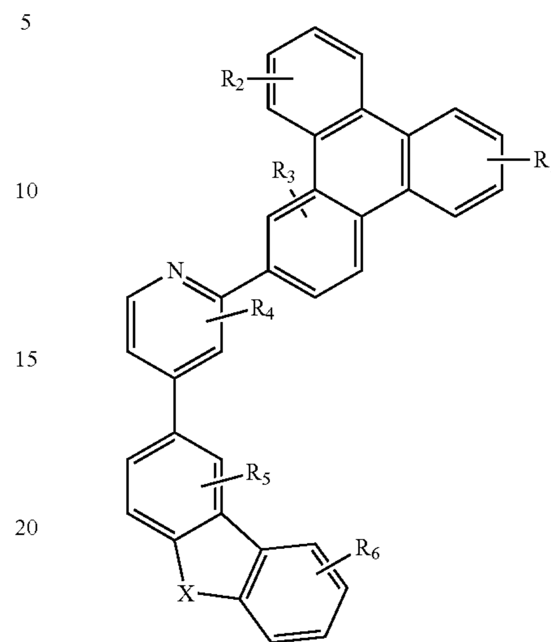
Compound 46
