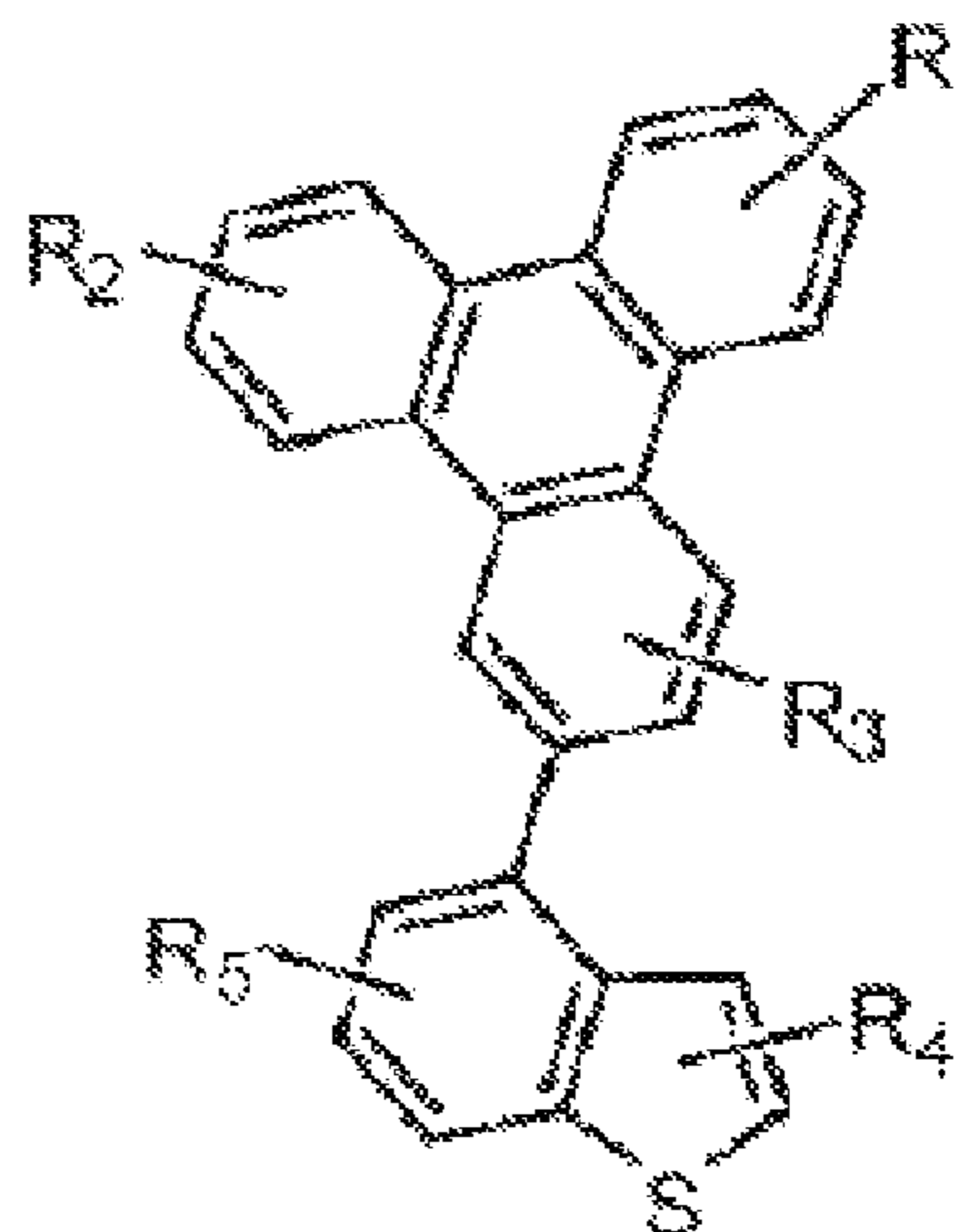
Compound 16'G
