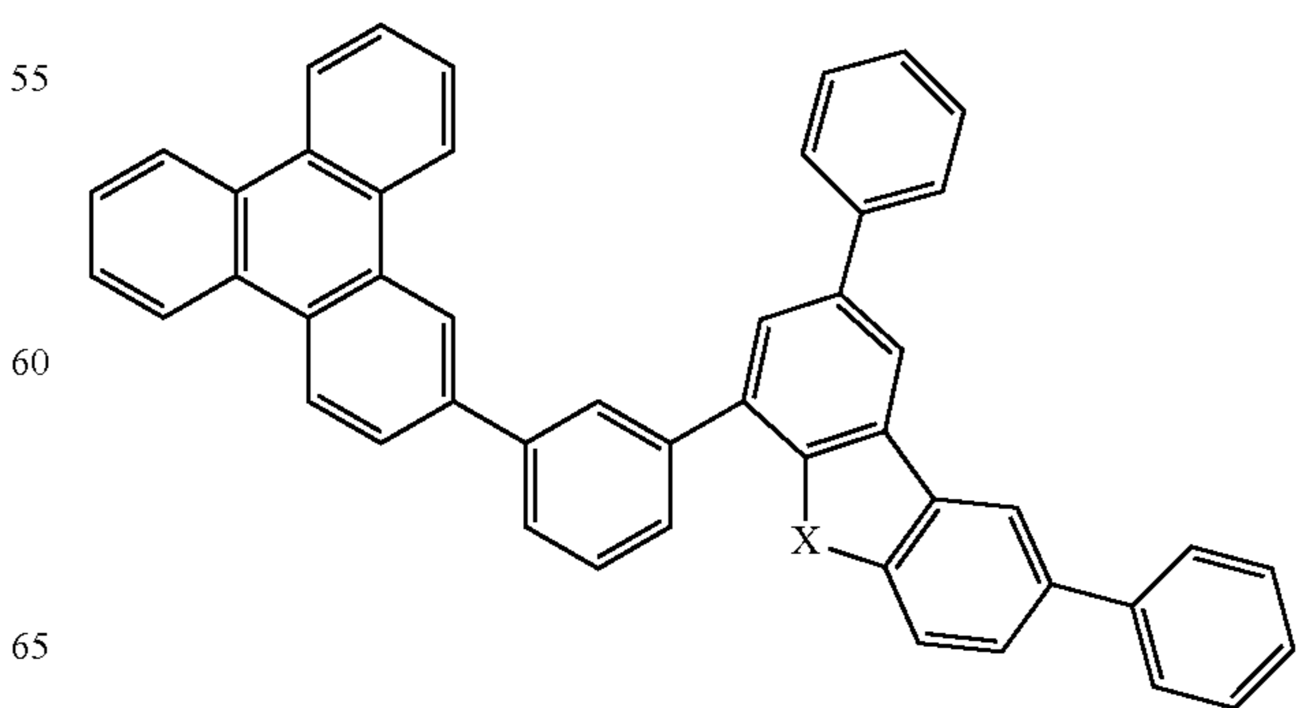
Compound 24
