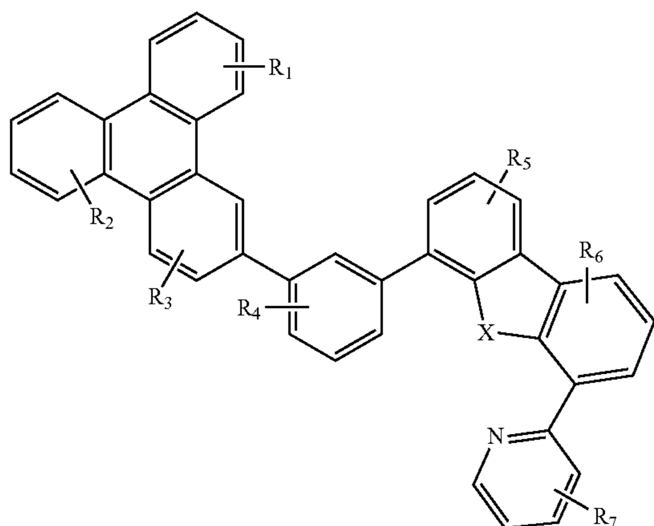
Compound 47 G
