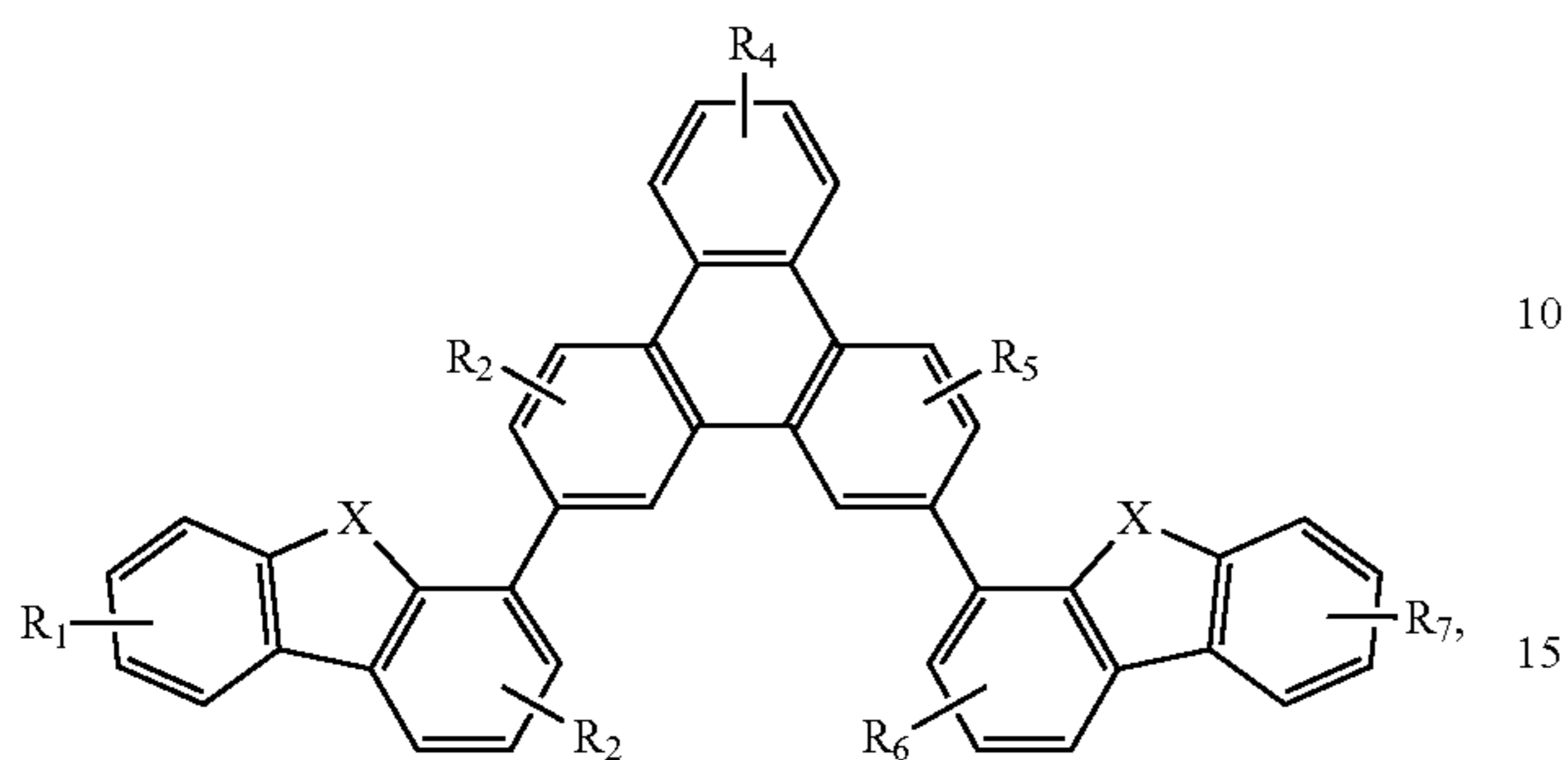
Compound 10G 5
