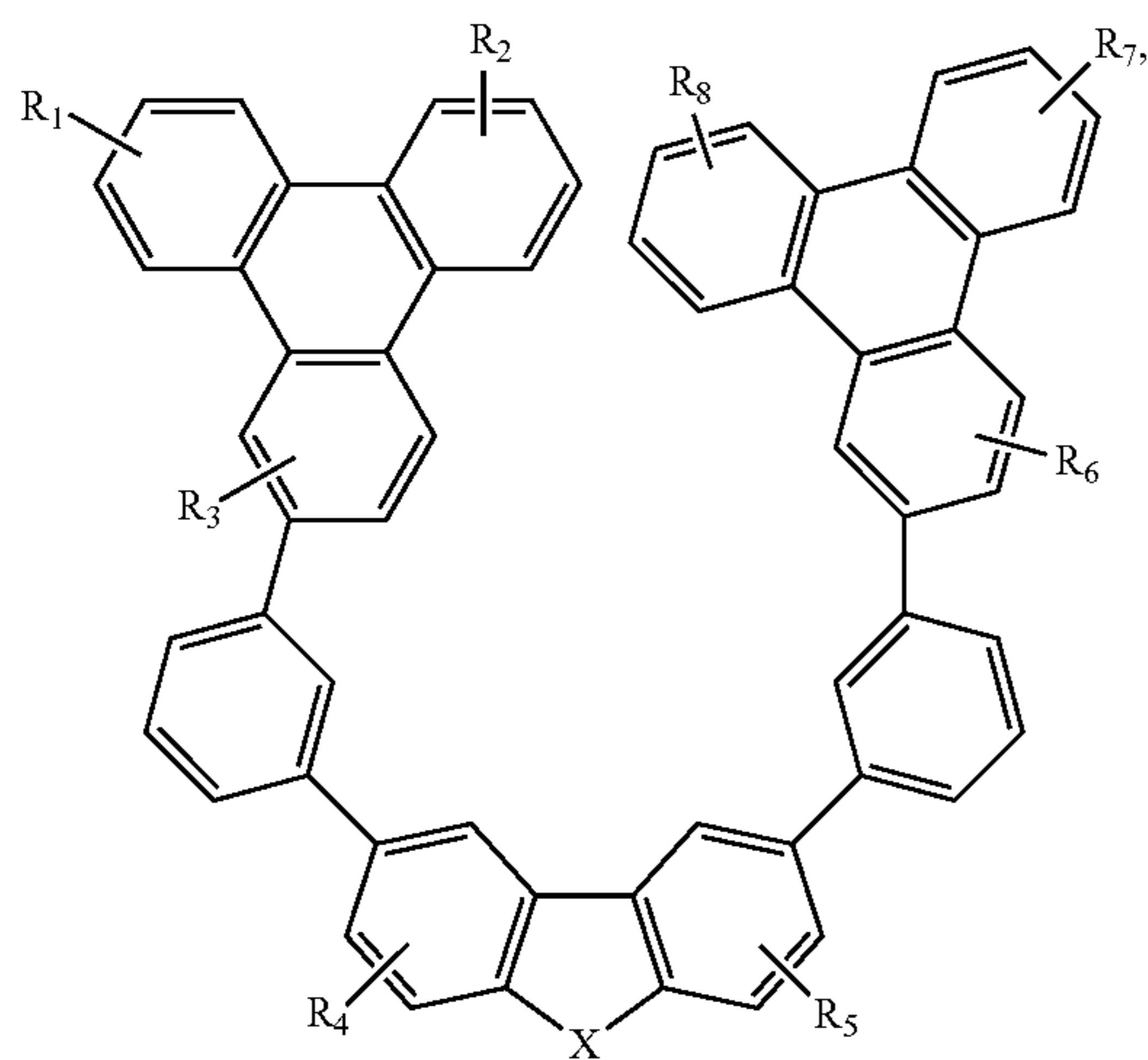
Compound 39G
