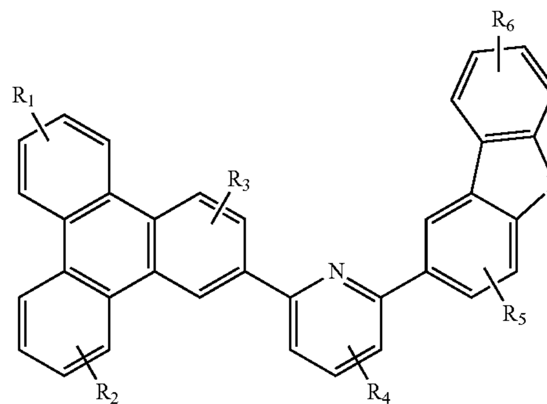
Compound 44 G
