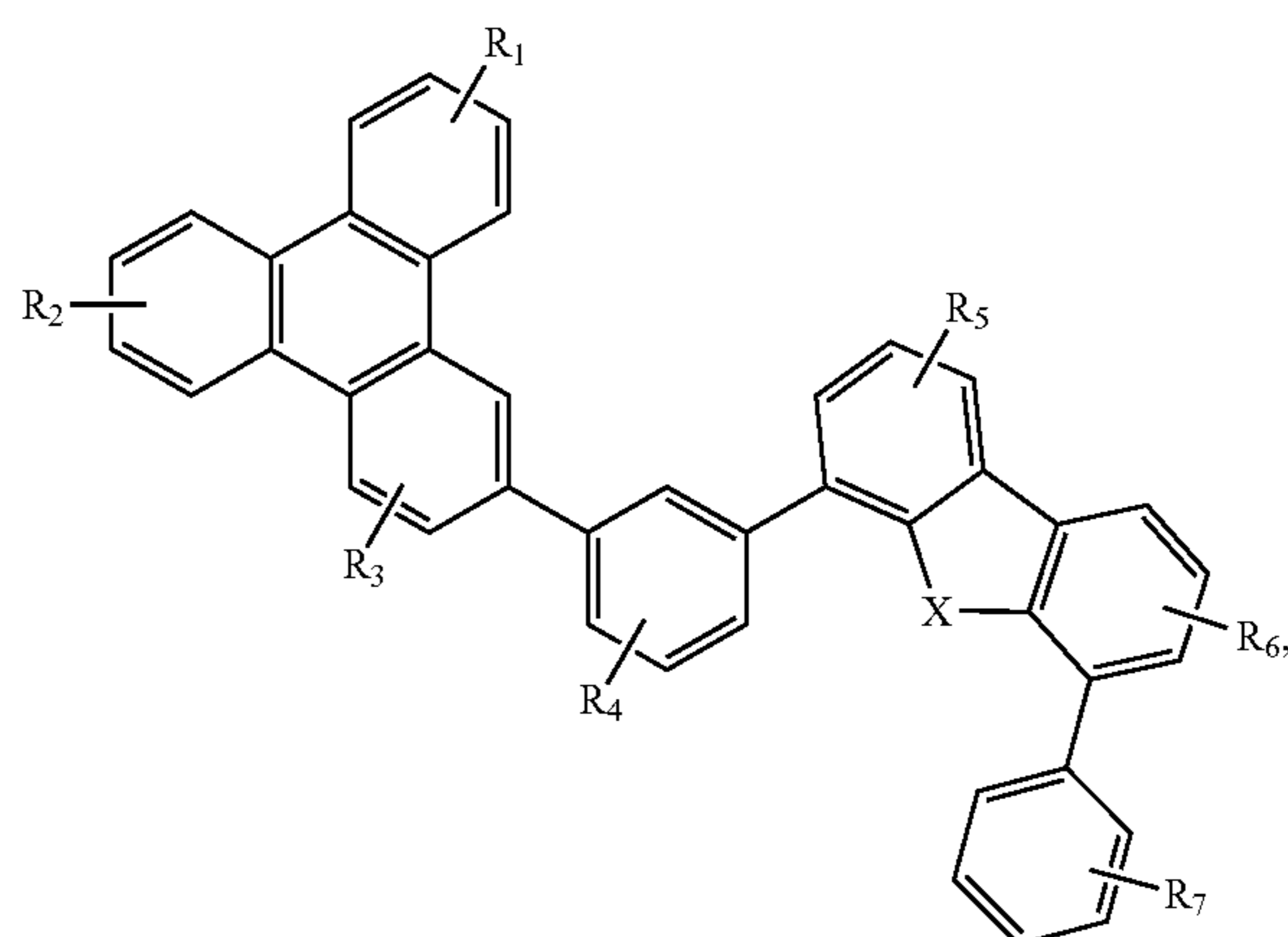
Compound 19G 20
