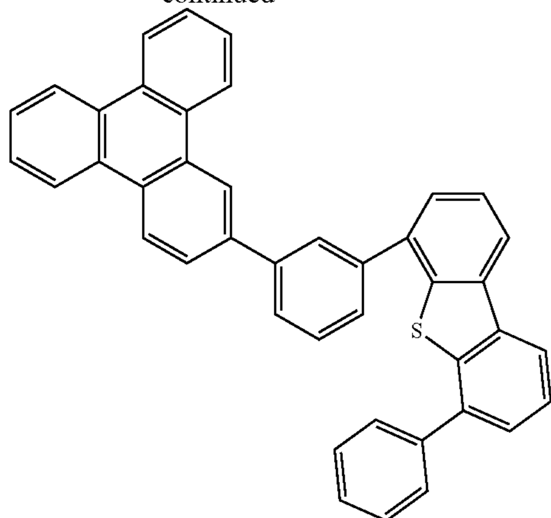
Compound 23S
