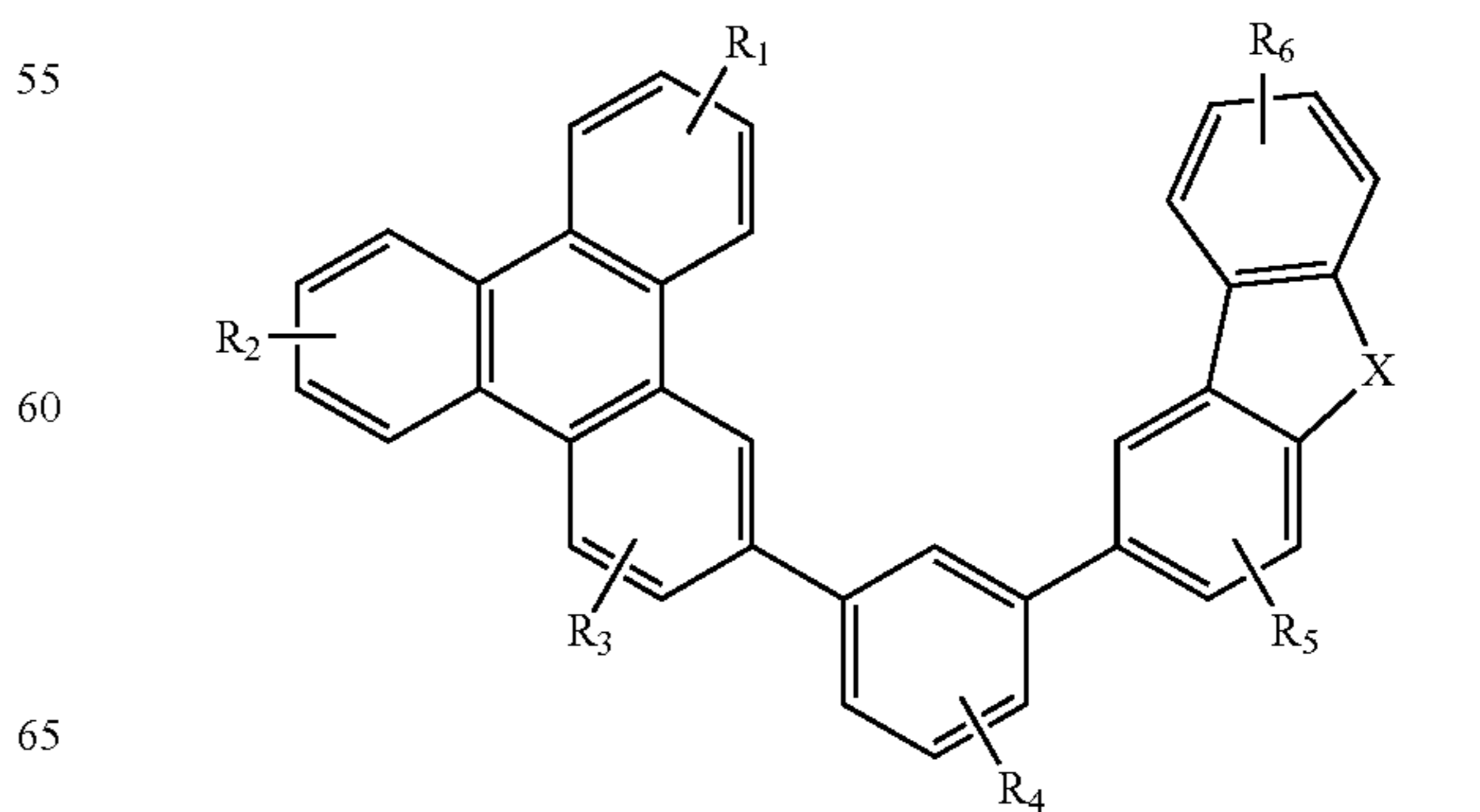
Compound 20 G
