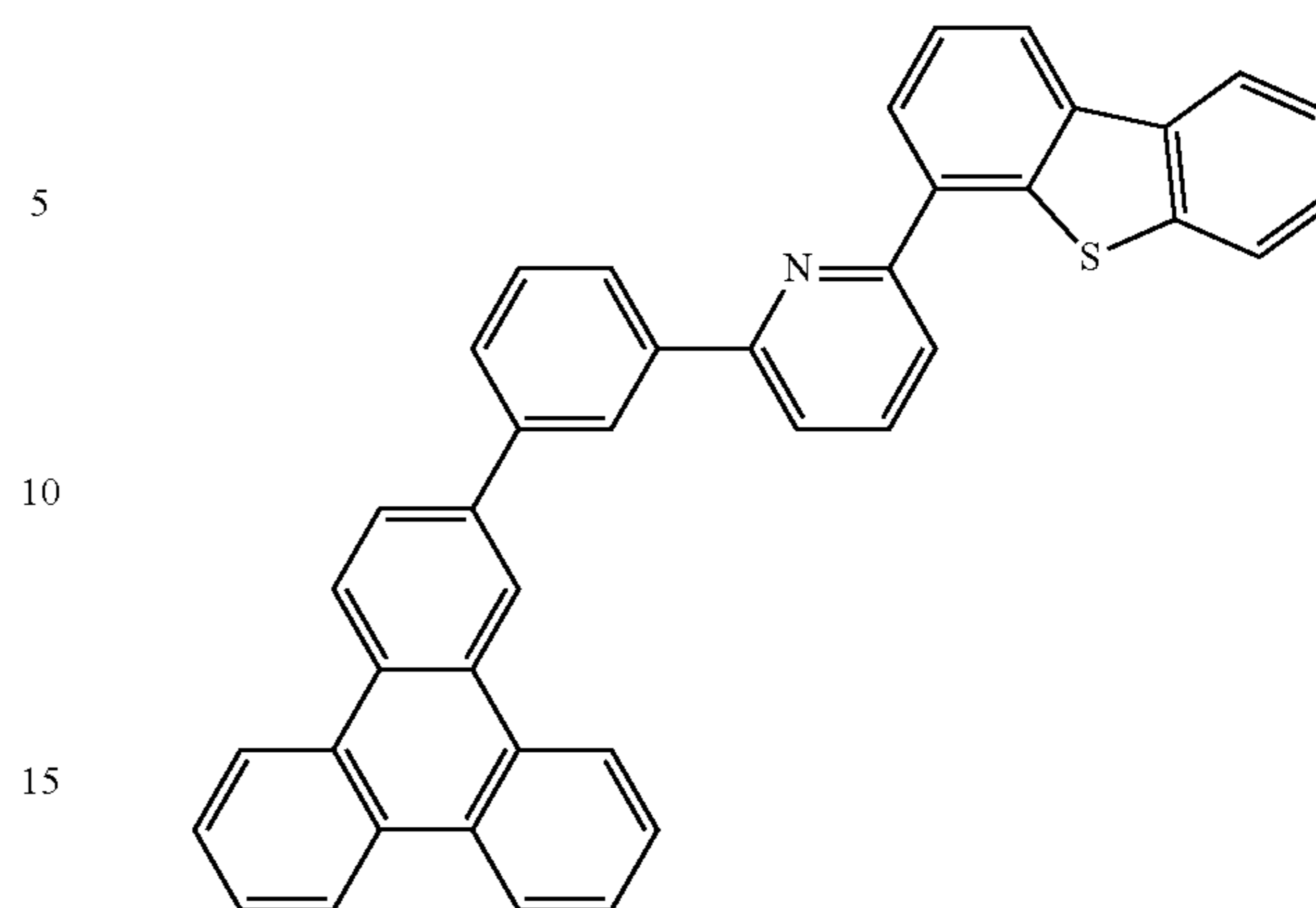
Compound 21S
