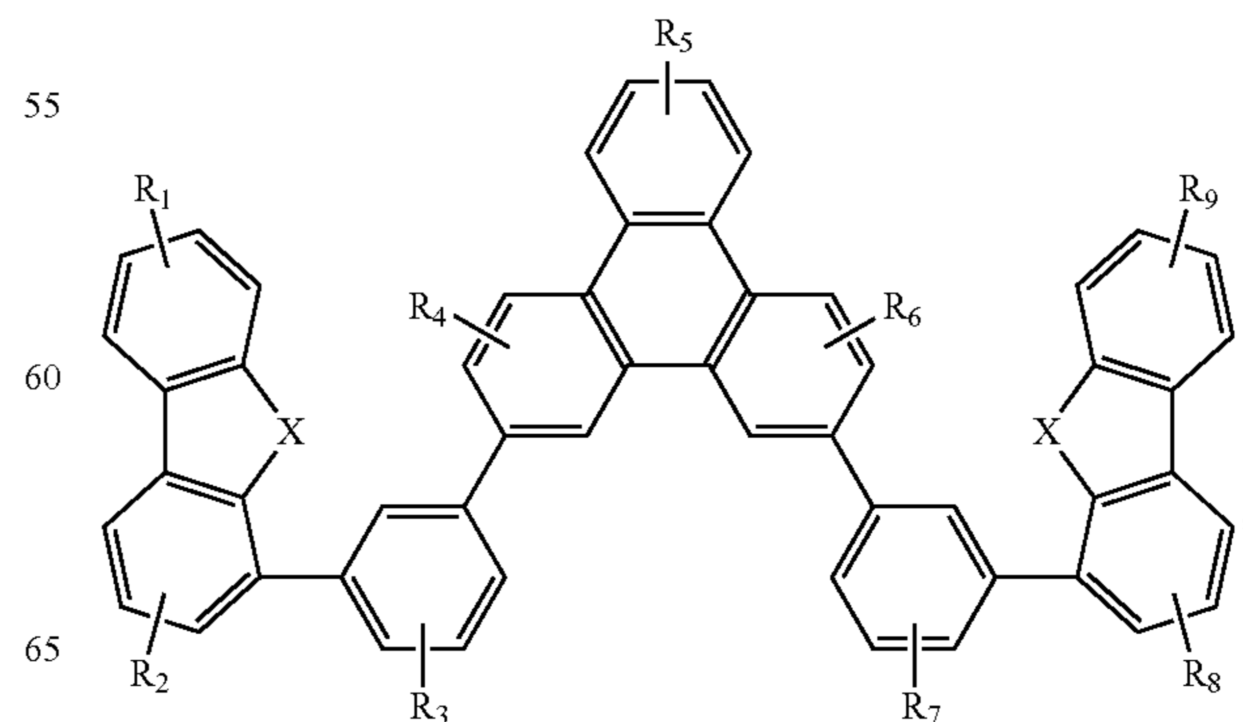
Compound 1G
