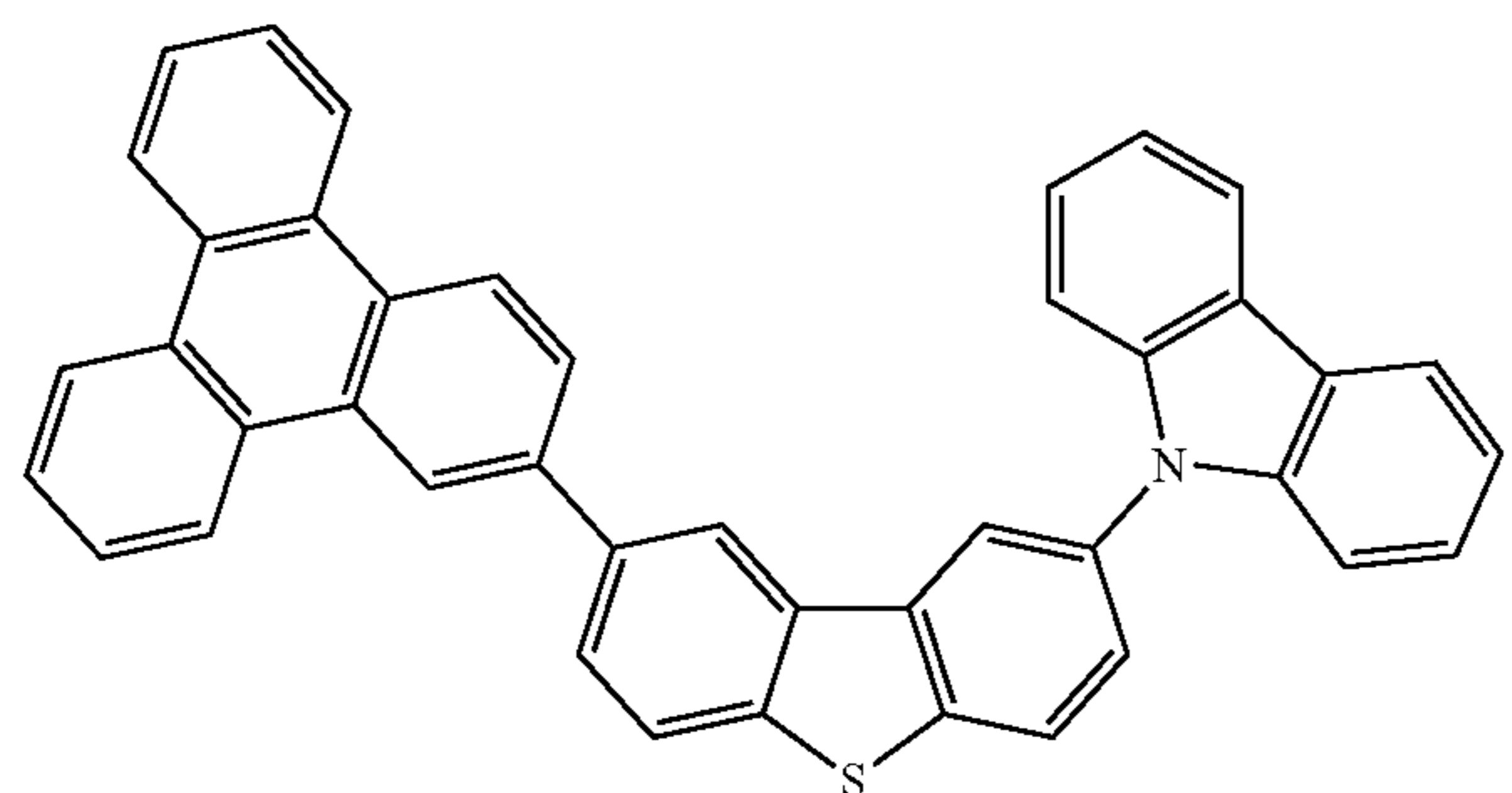
Compound 15'
