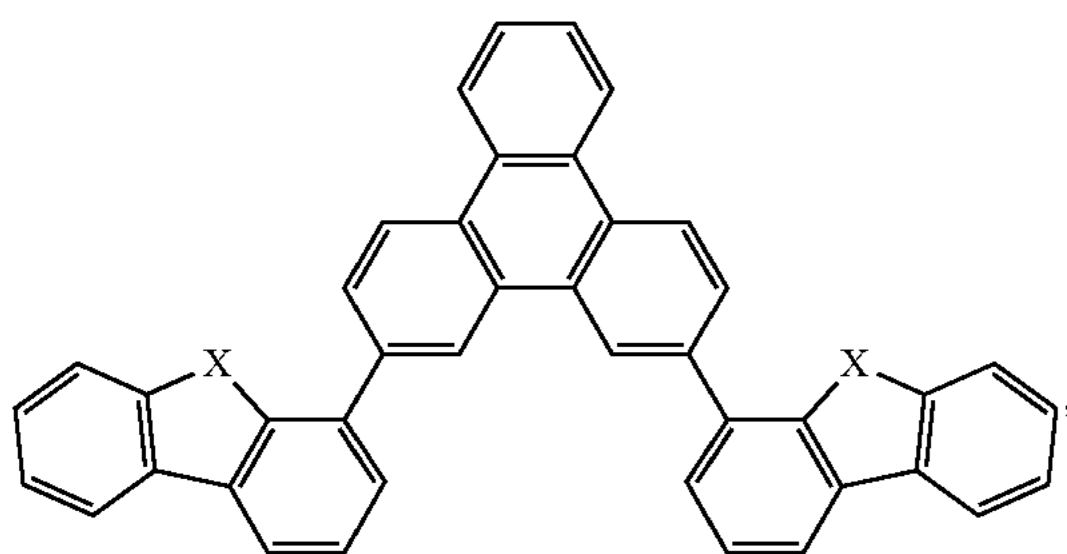
Compound 10
