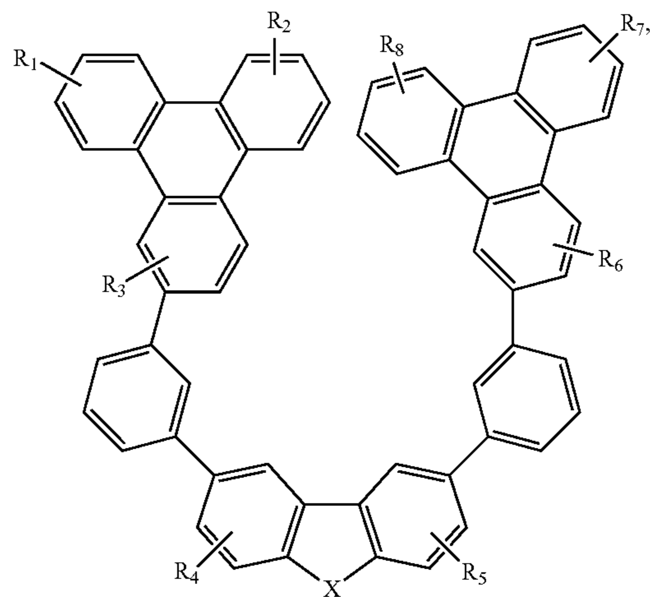
Compound 39G
