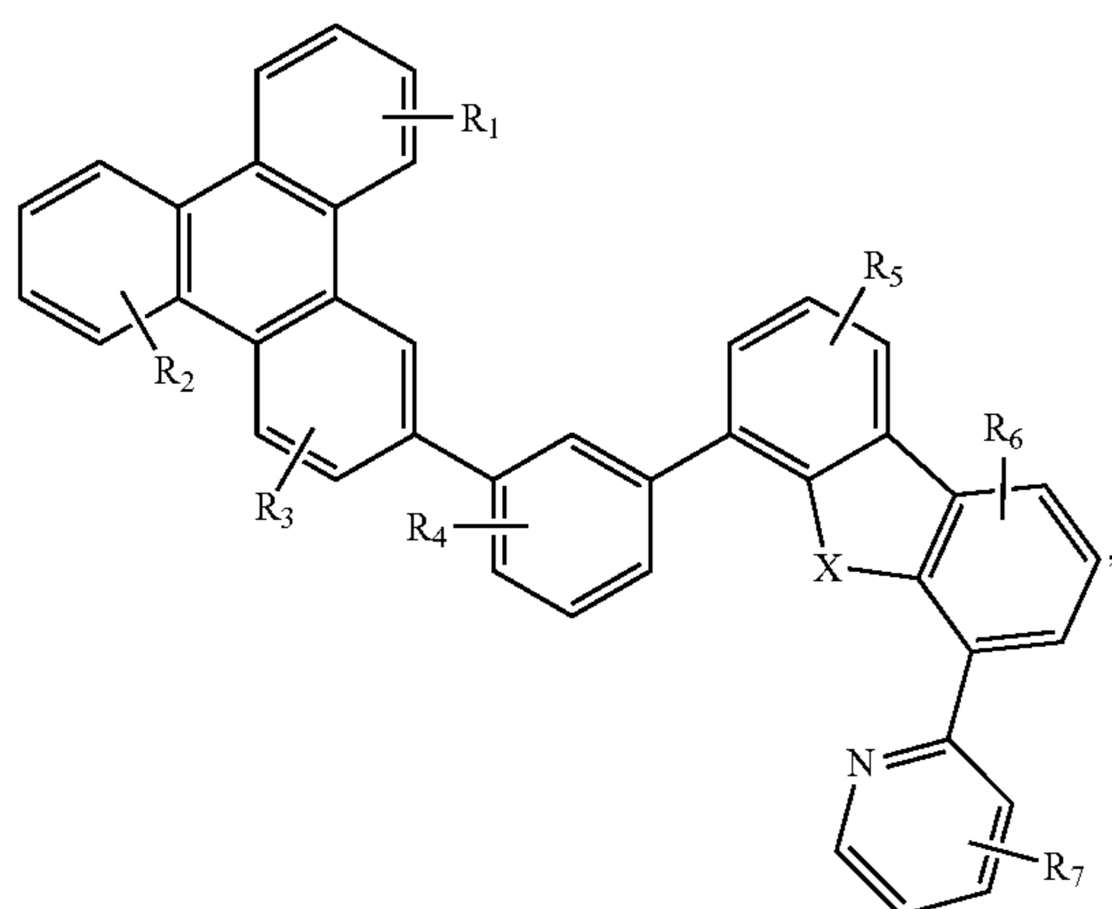
Compound 47 G
