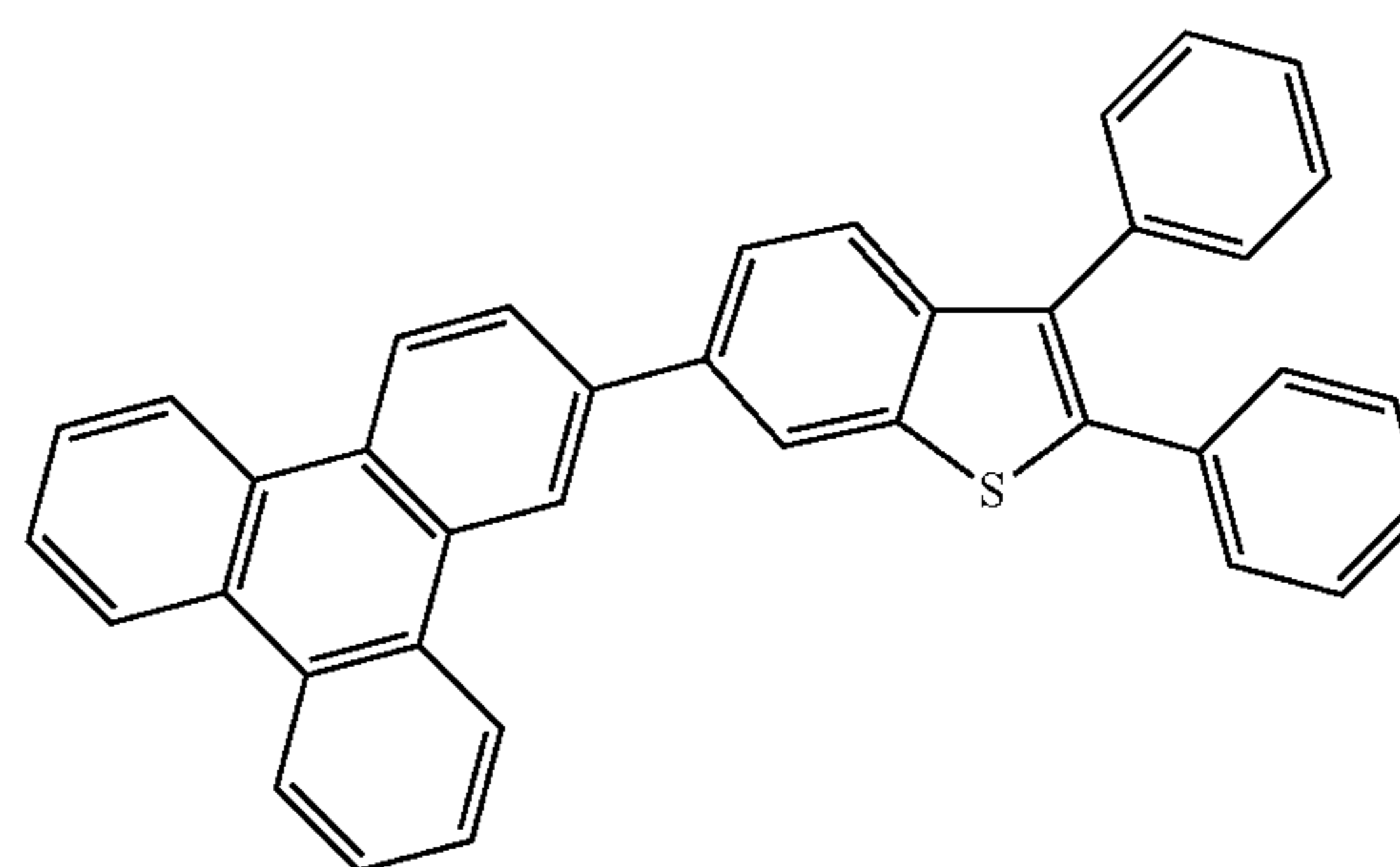
Compound 17'
