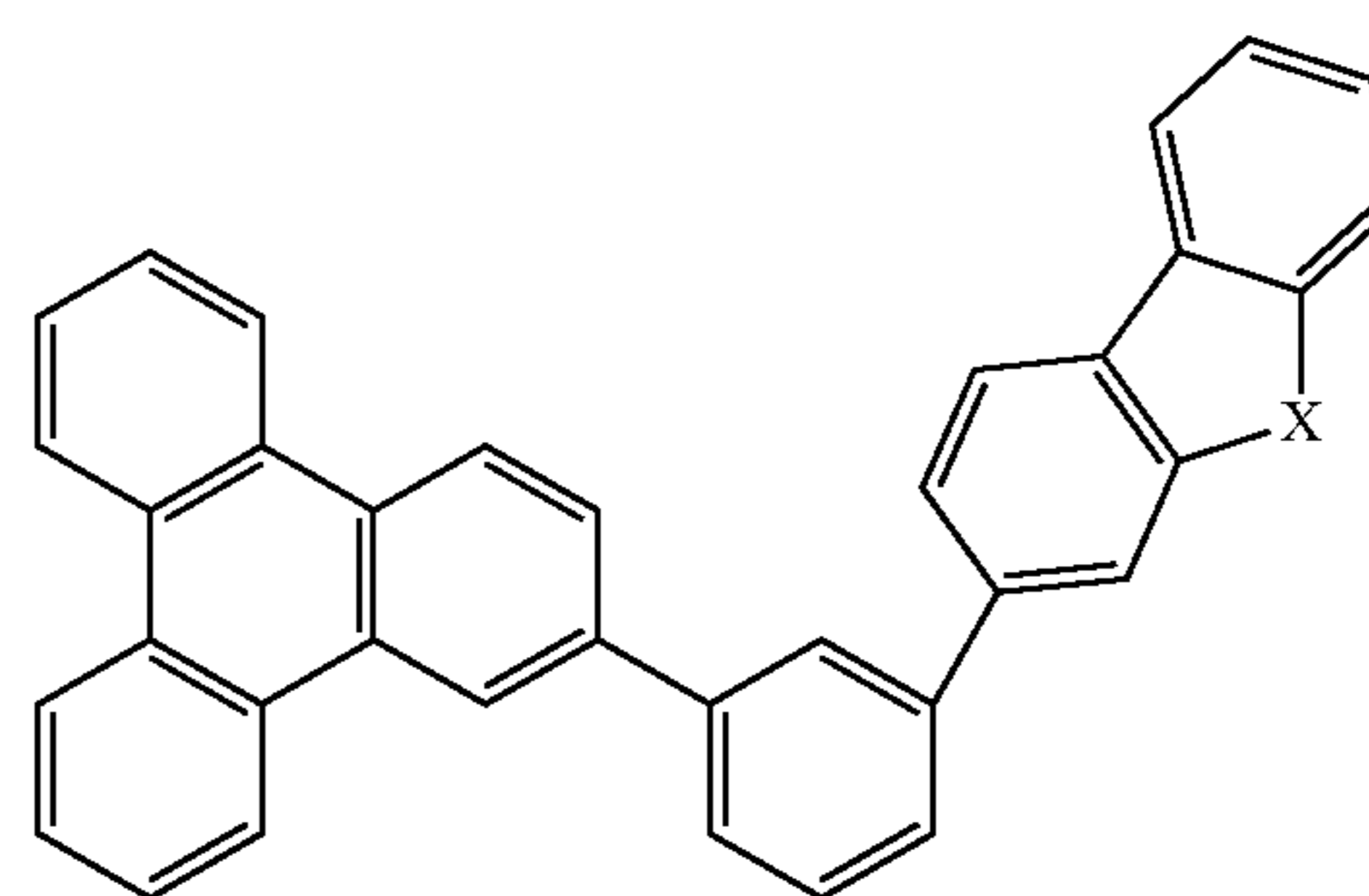
Compound 40
