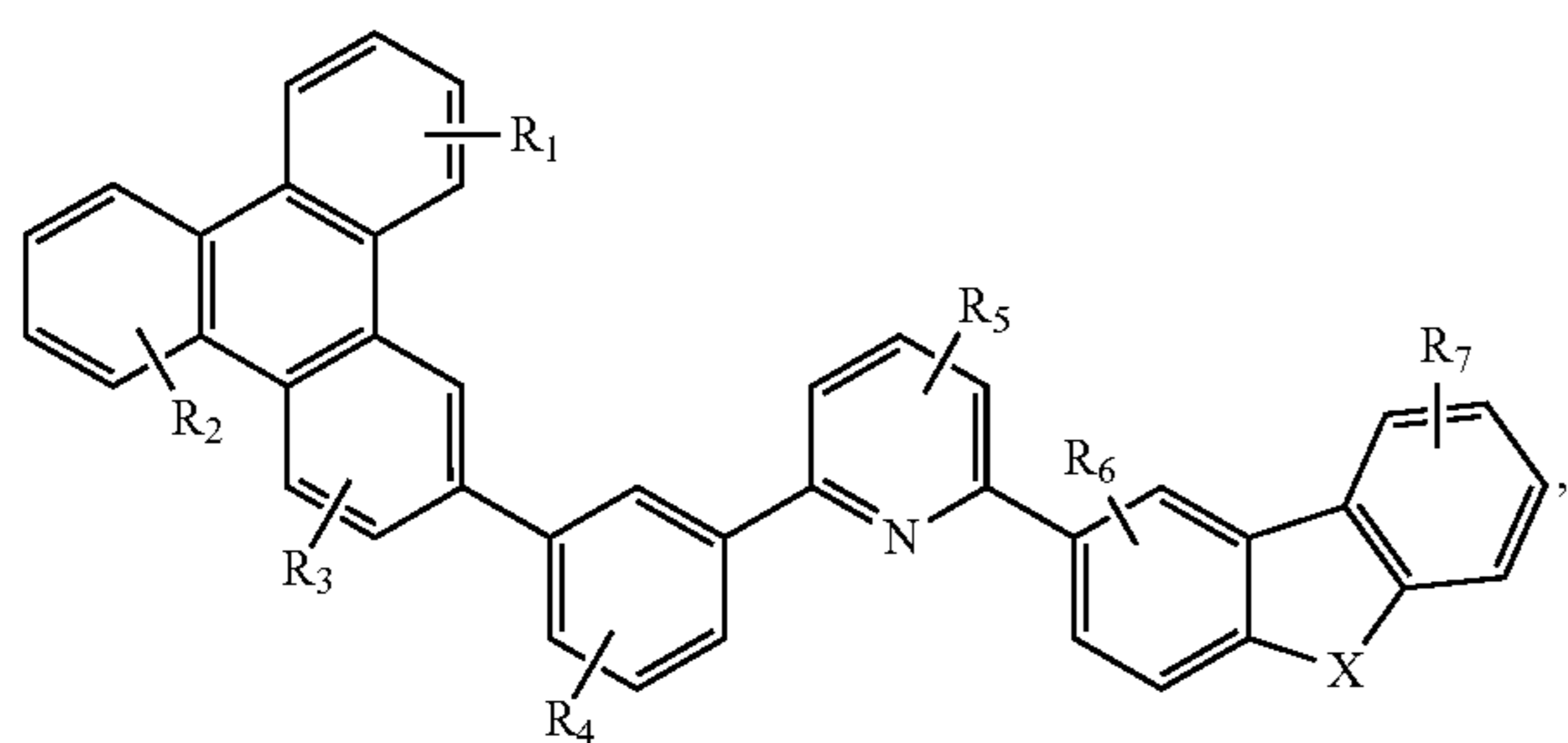
Compound 44G
