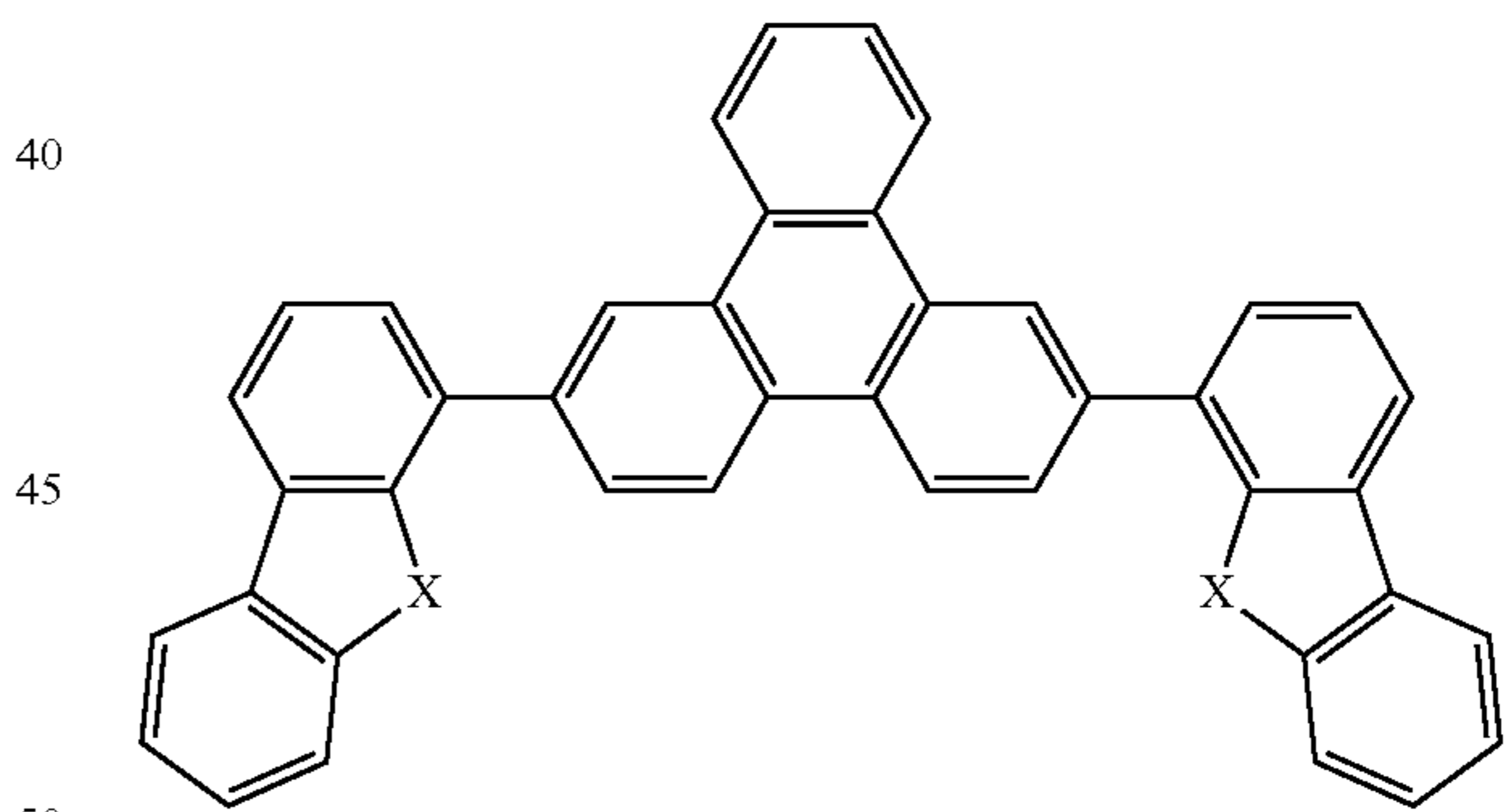
Compound 19
