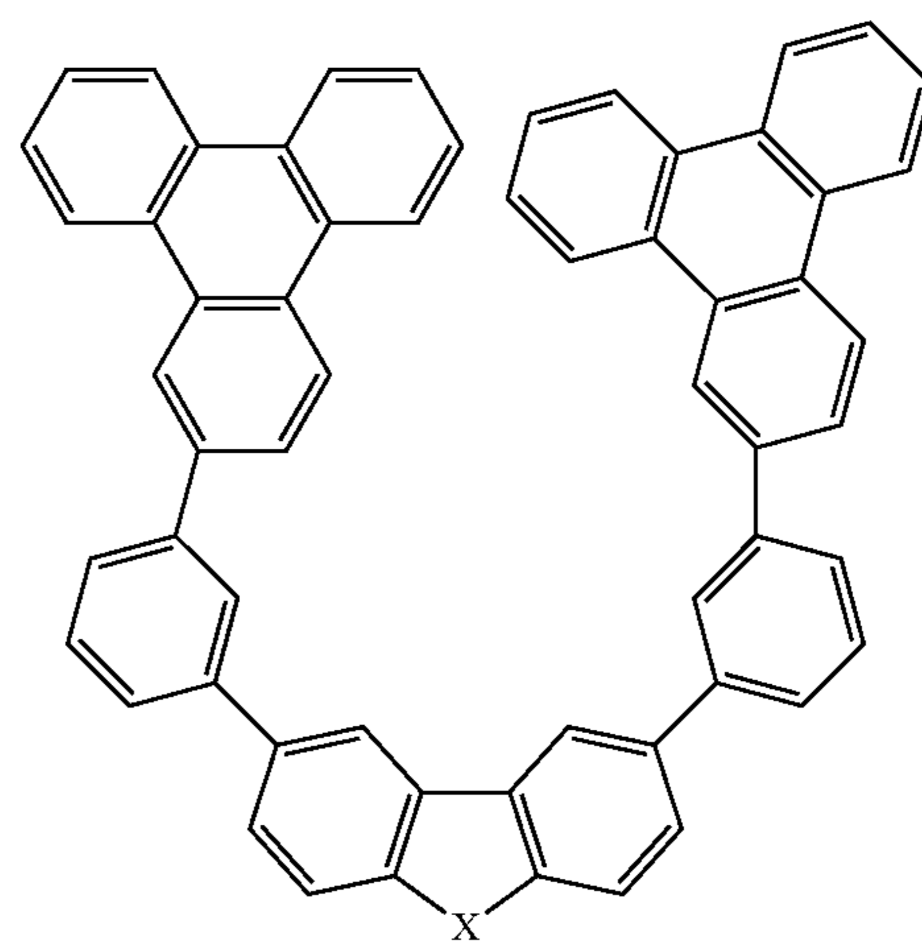
Compound 40
