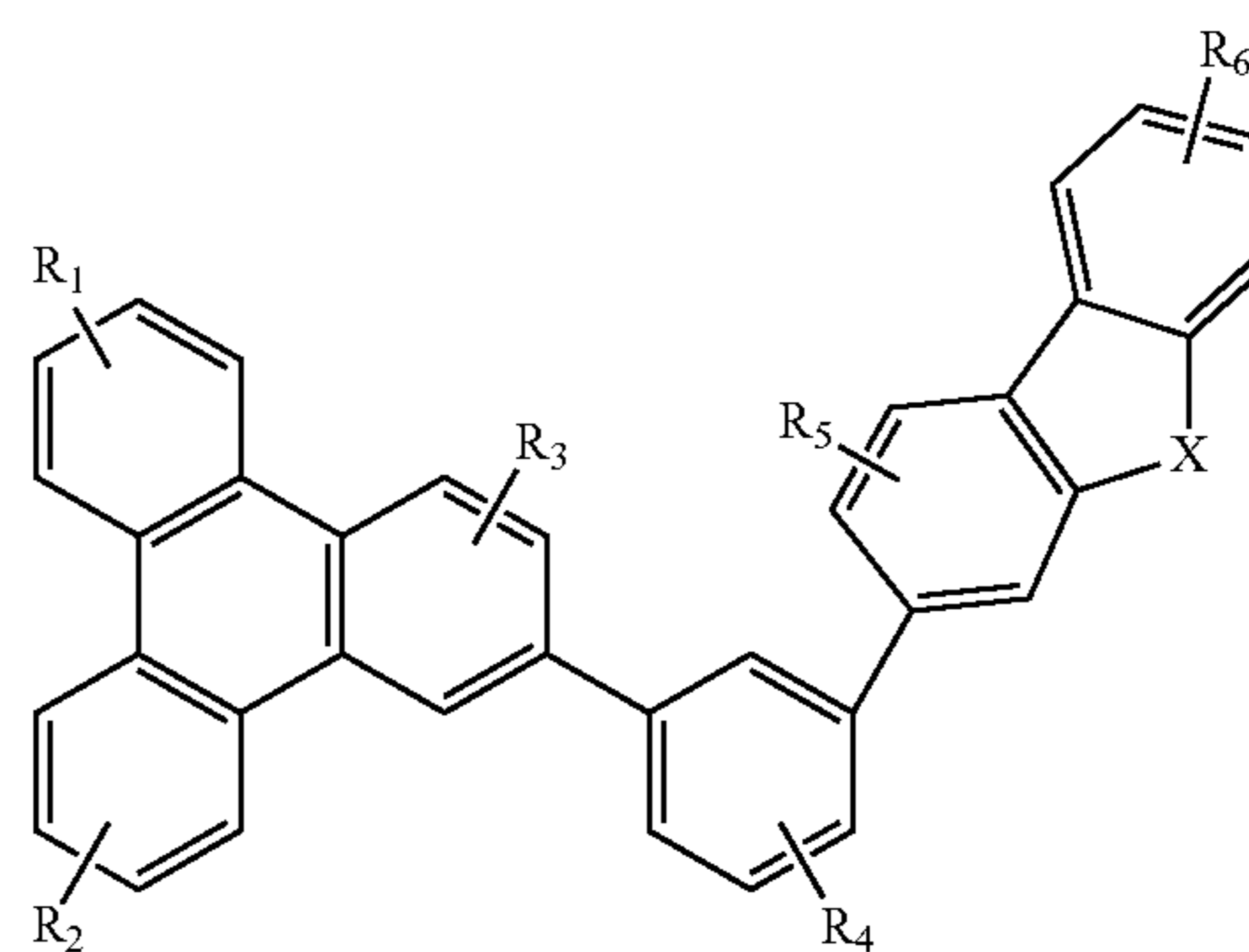
Compound 40G
