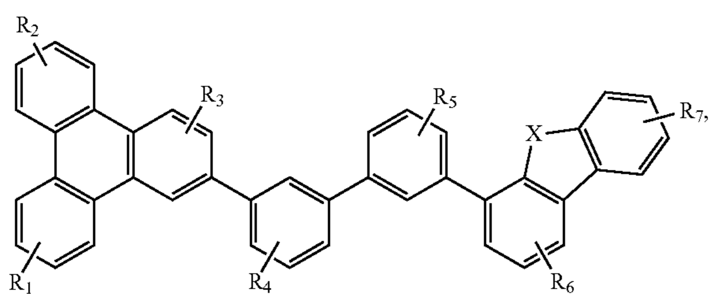
Compound 9G
