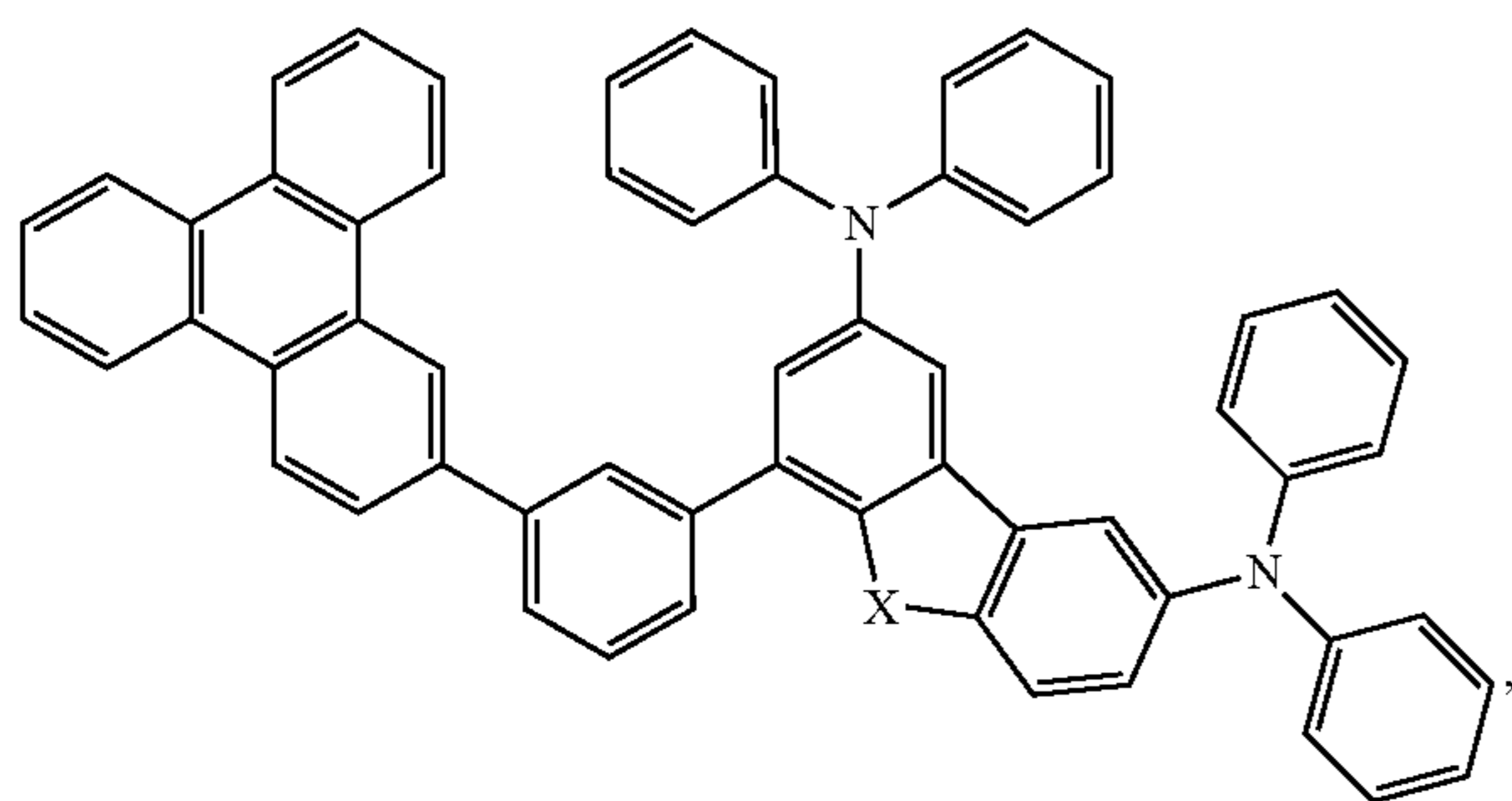
Compound 28
