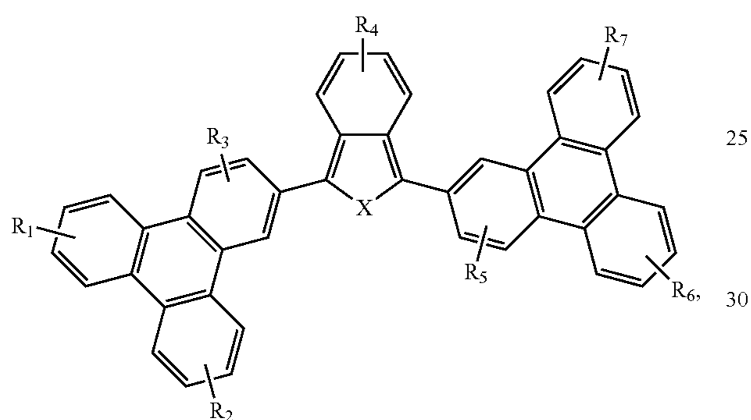
Compound 11G 20
