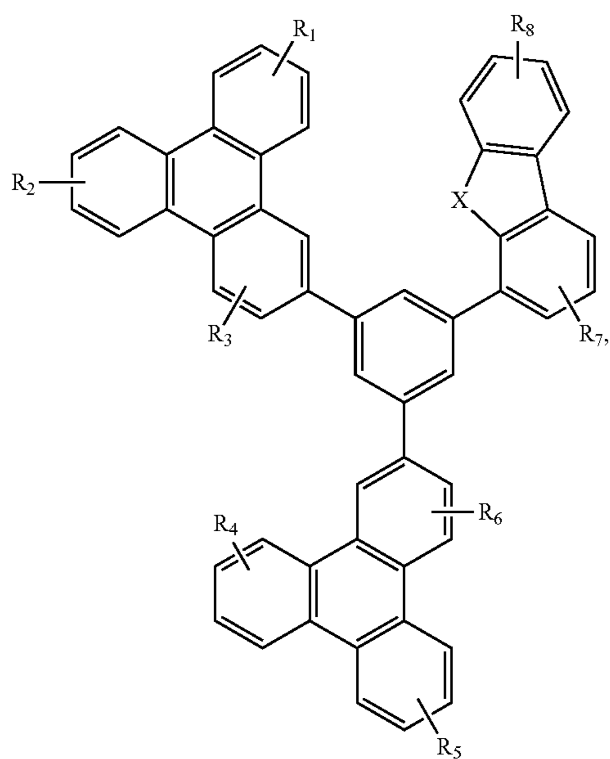
Compound 38G
