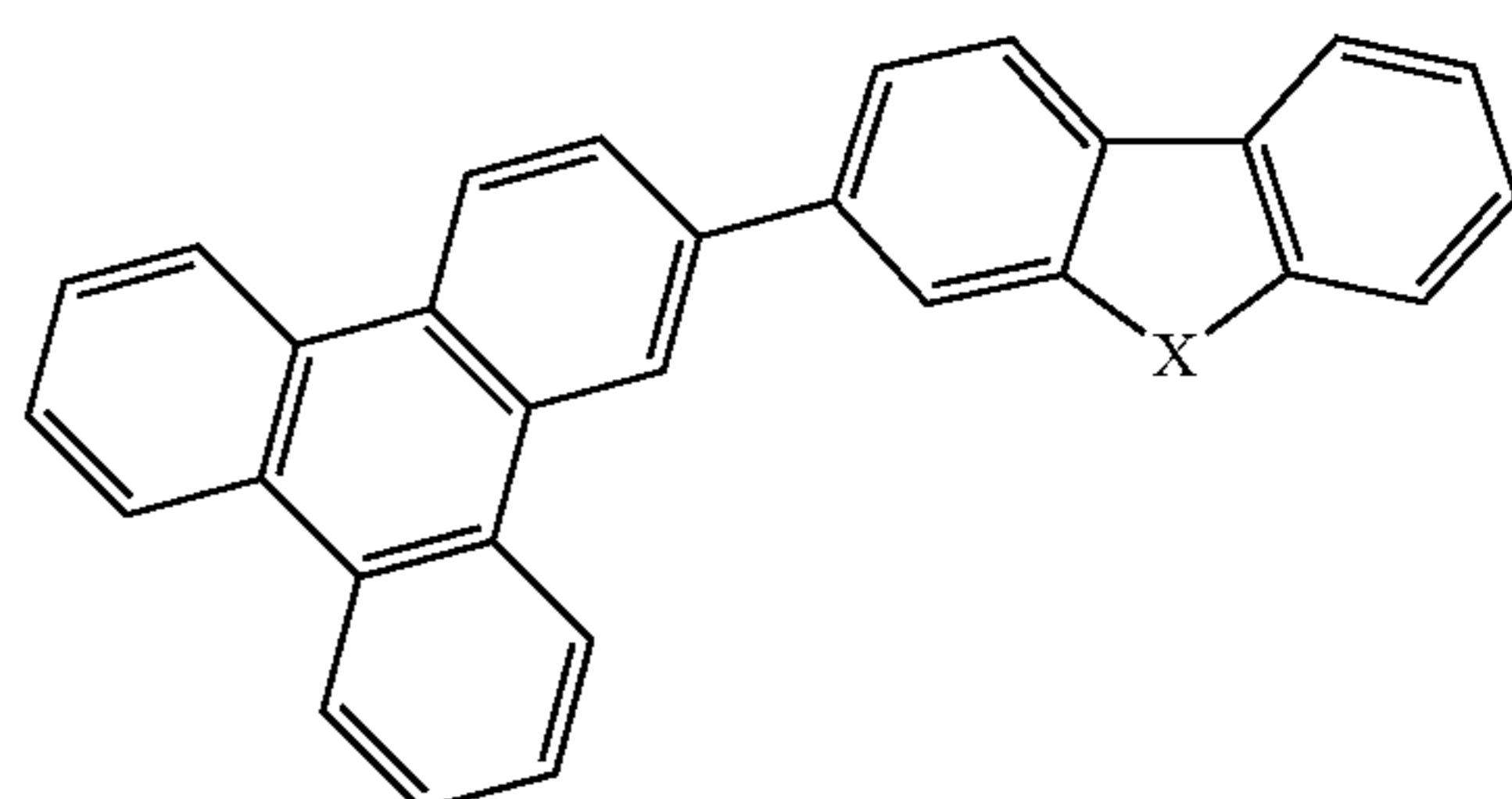
Compound 8
