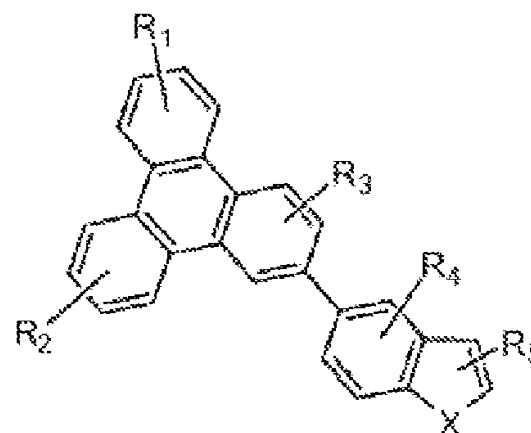
Compound 13G
