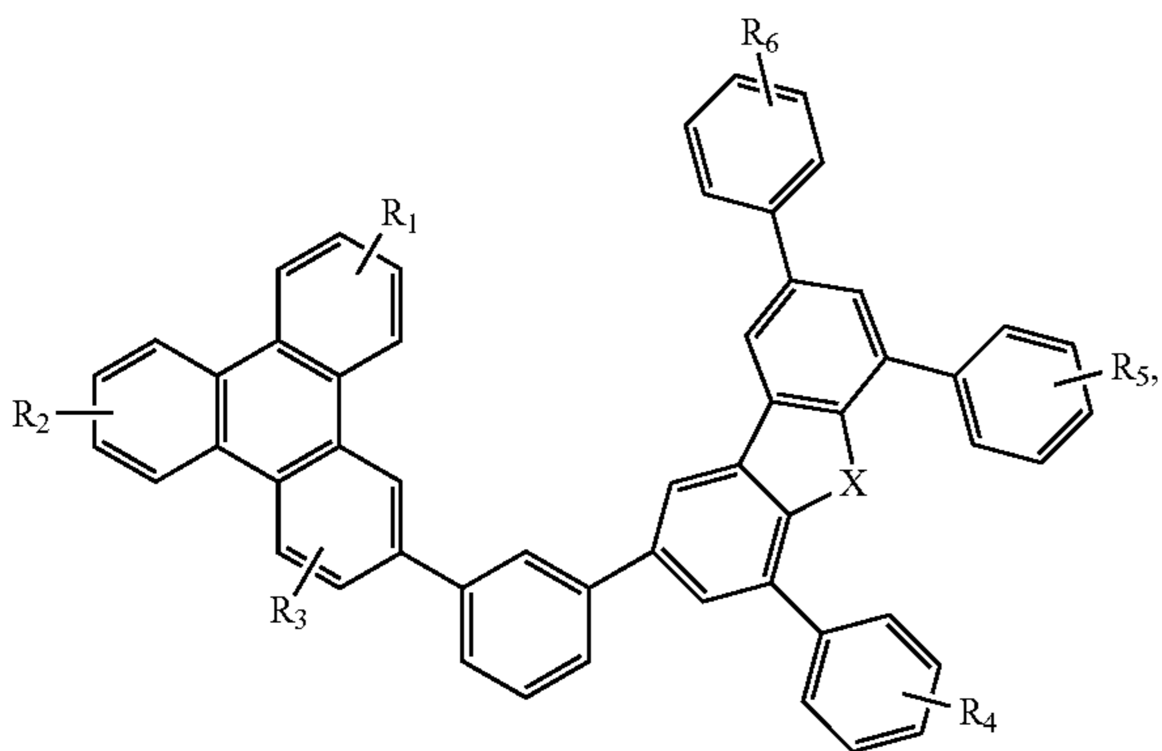
Compound 36G
