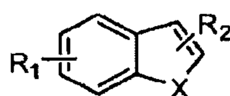
Formula (V)
