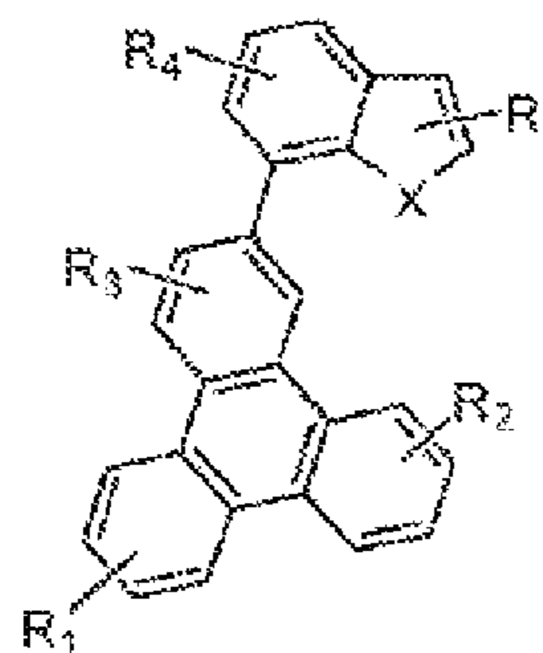
Compound 12G
