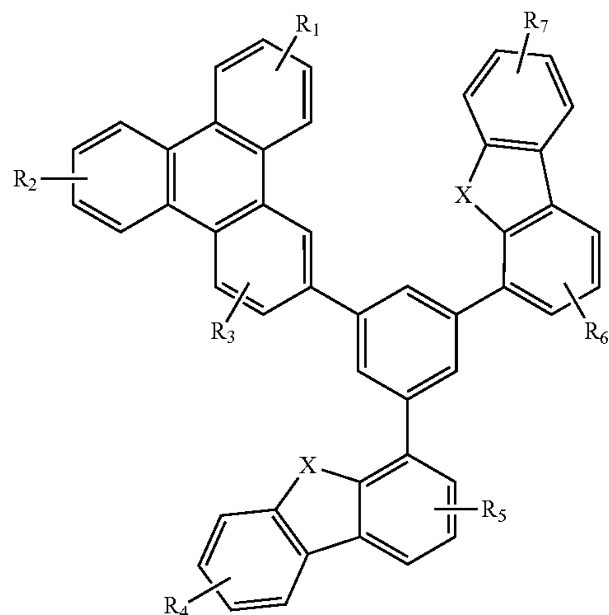
Compound 37G
