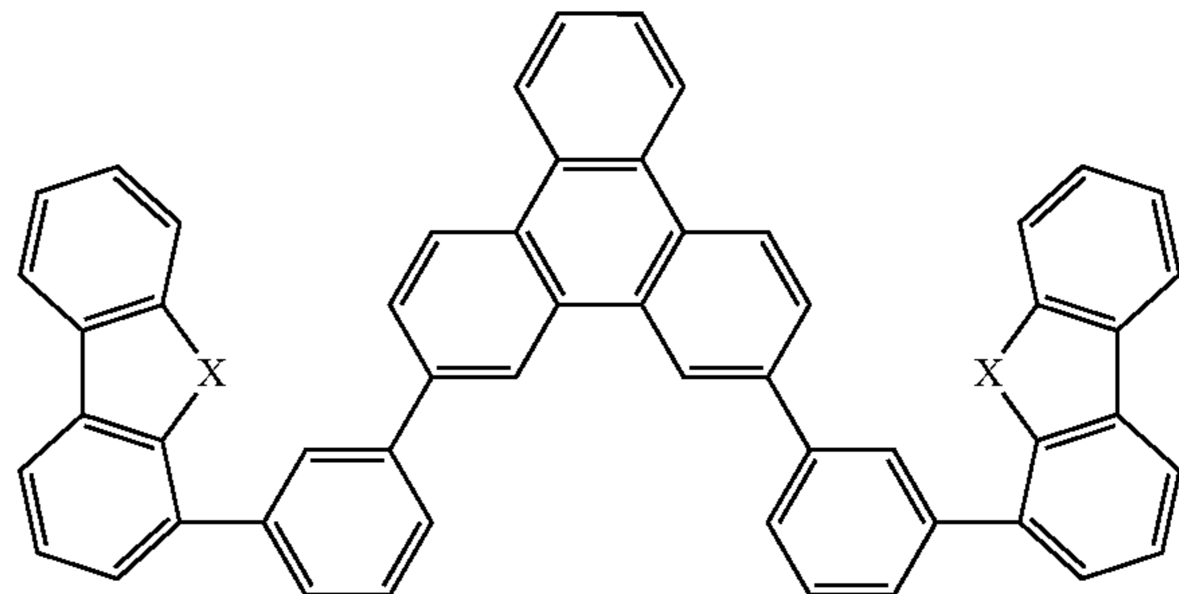
Compound 5
