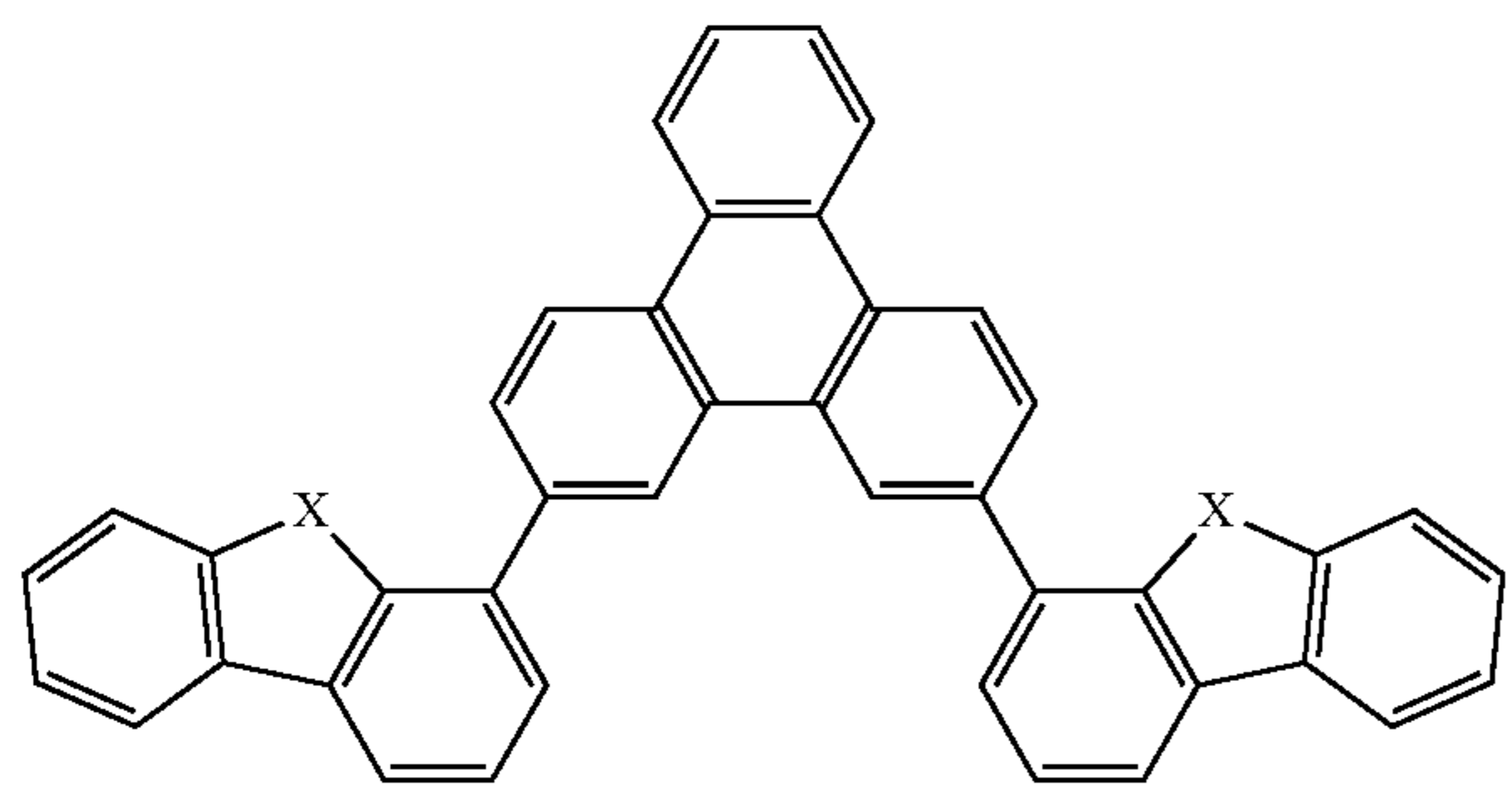
Compound 10
