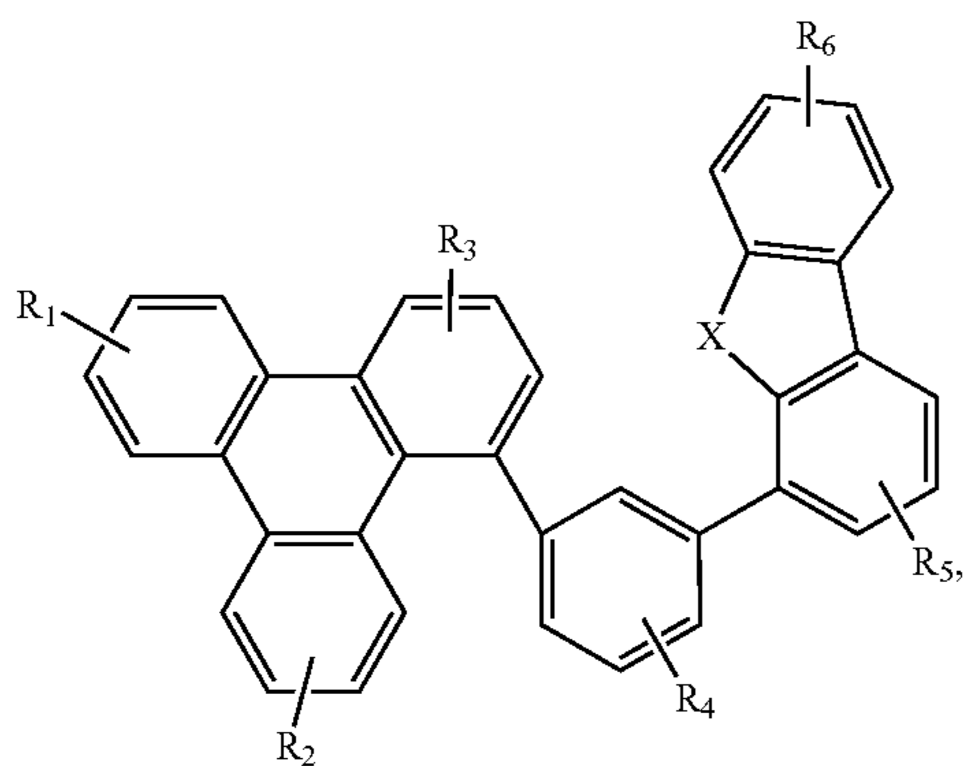
Compound 33G
