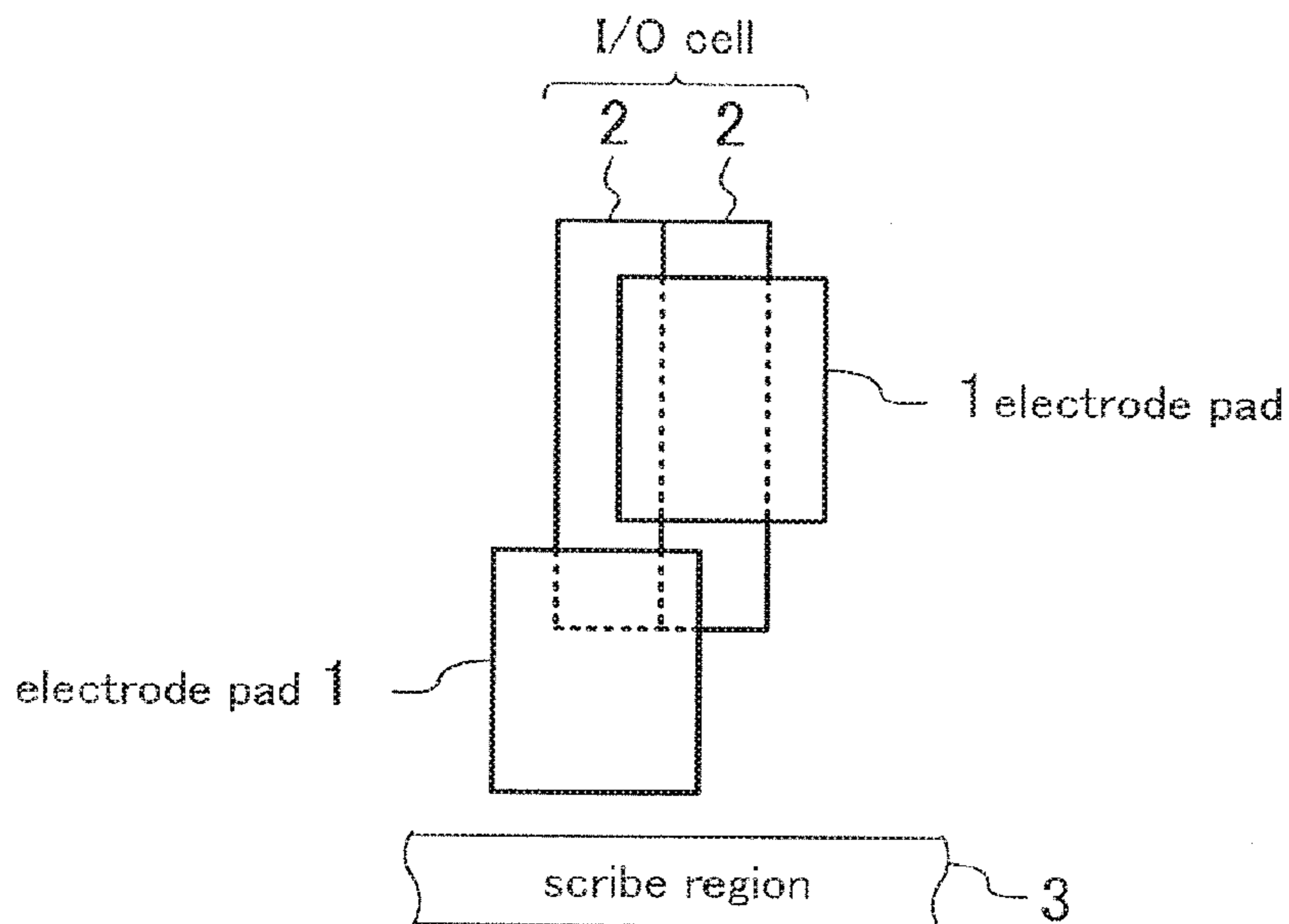
FIG.20 PRIOR ART
