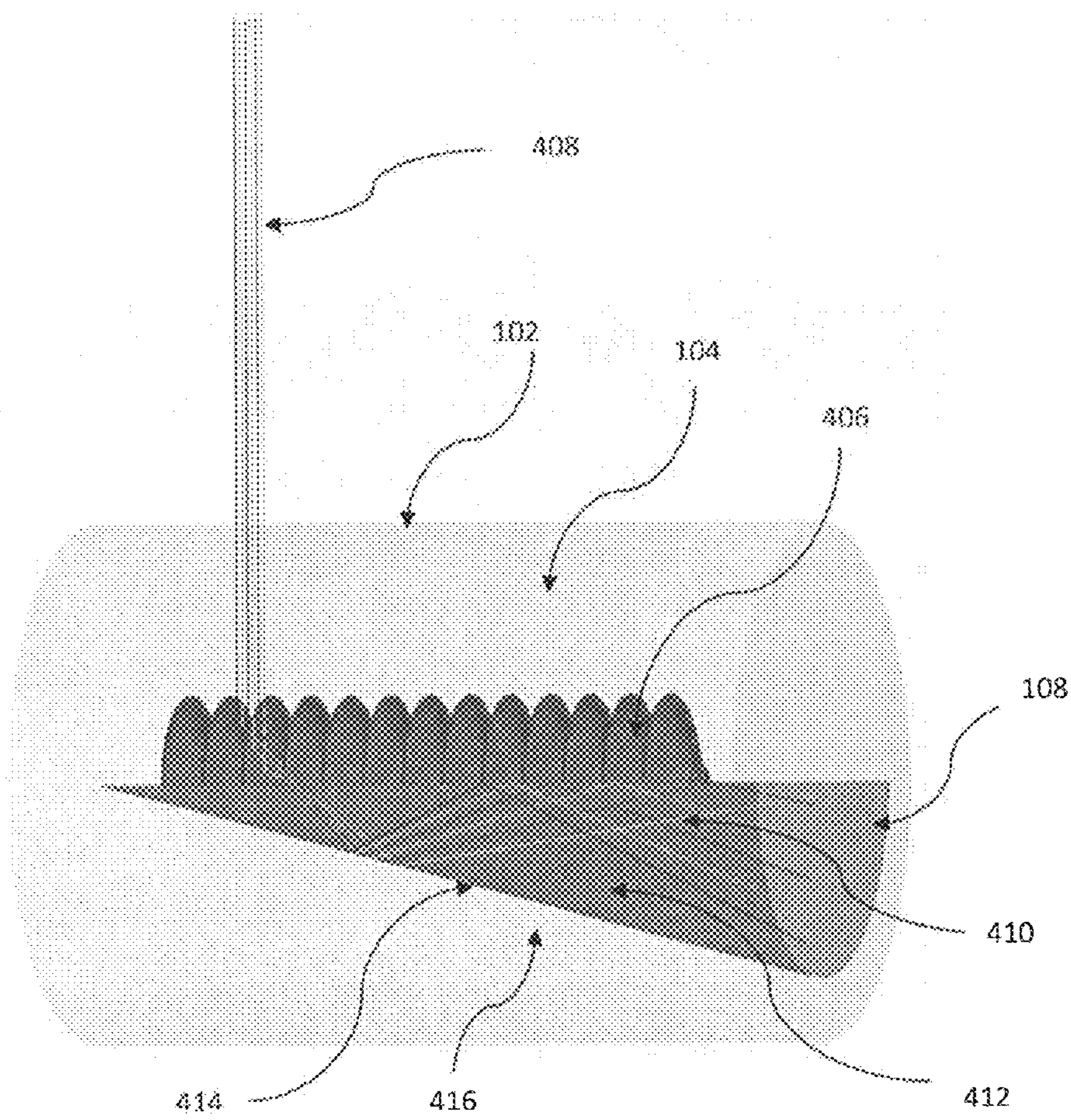
Figure 4 (a) Ray traces of light in the cladding and core
