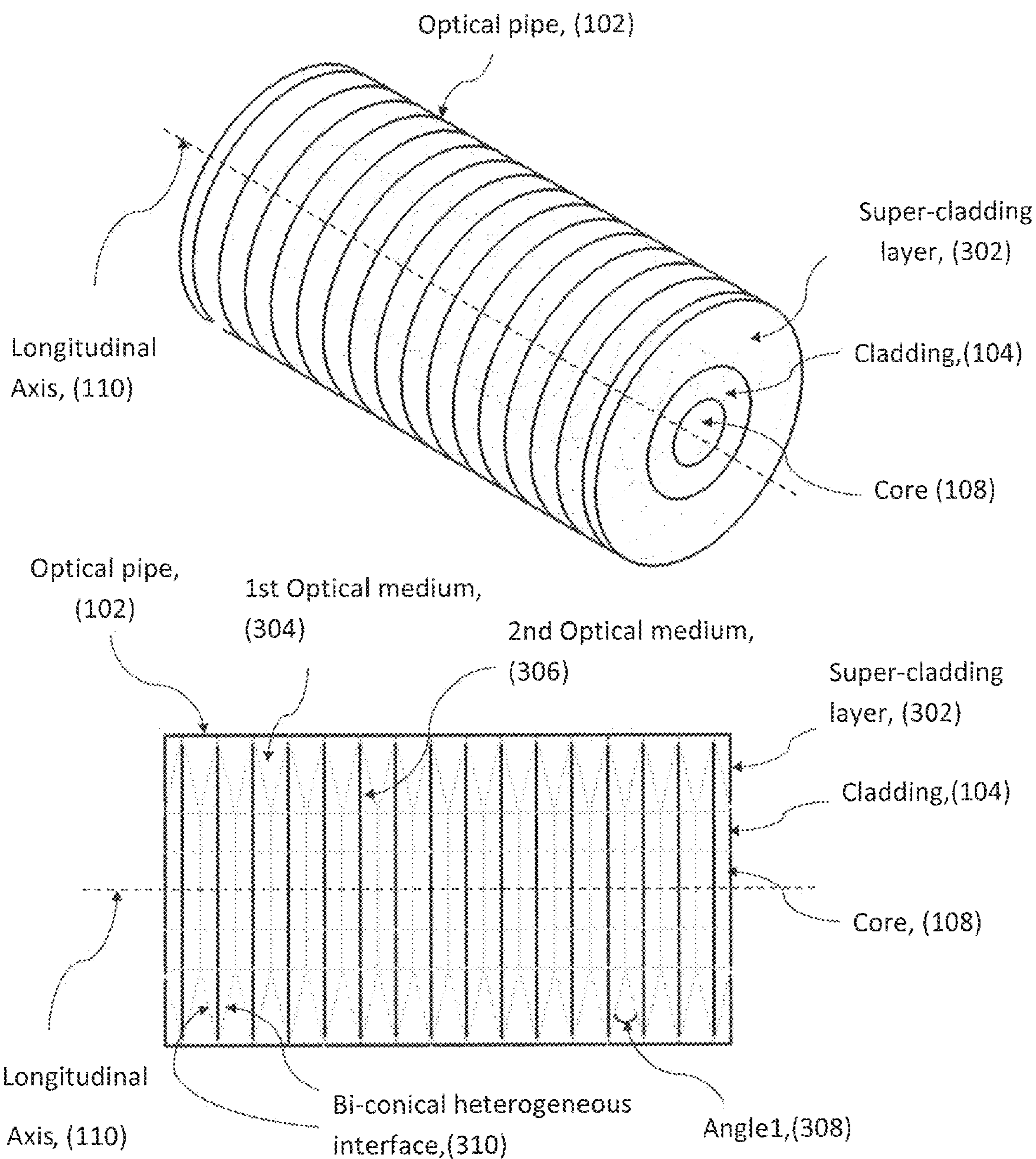
Figure 3. Super-cladding layer
