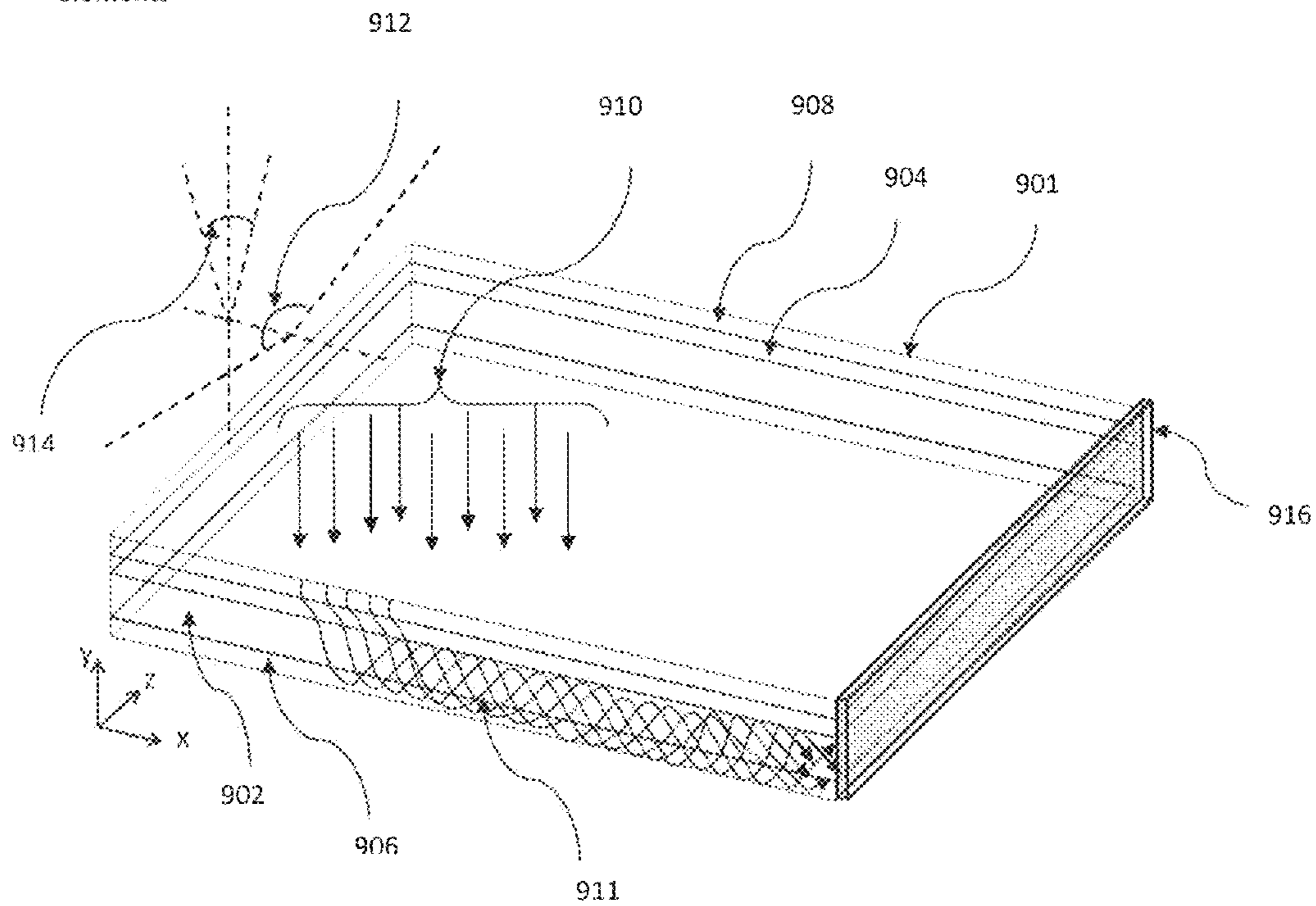
Figure 9(a) A Planar light guide concentrator using array of cladding, core and super-cladding elements
