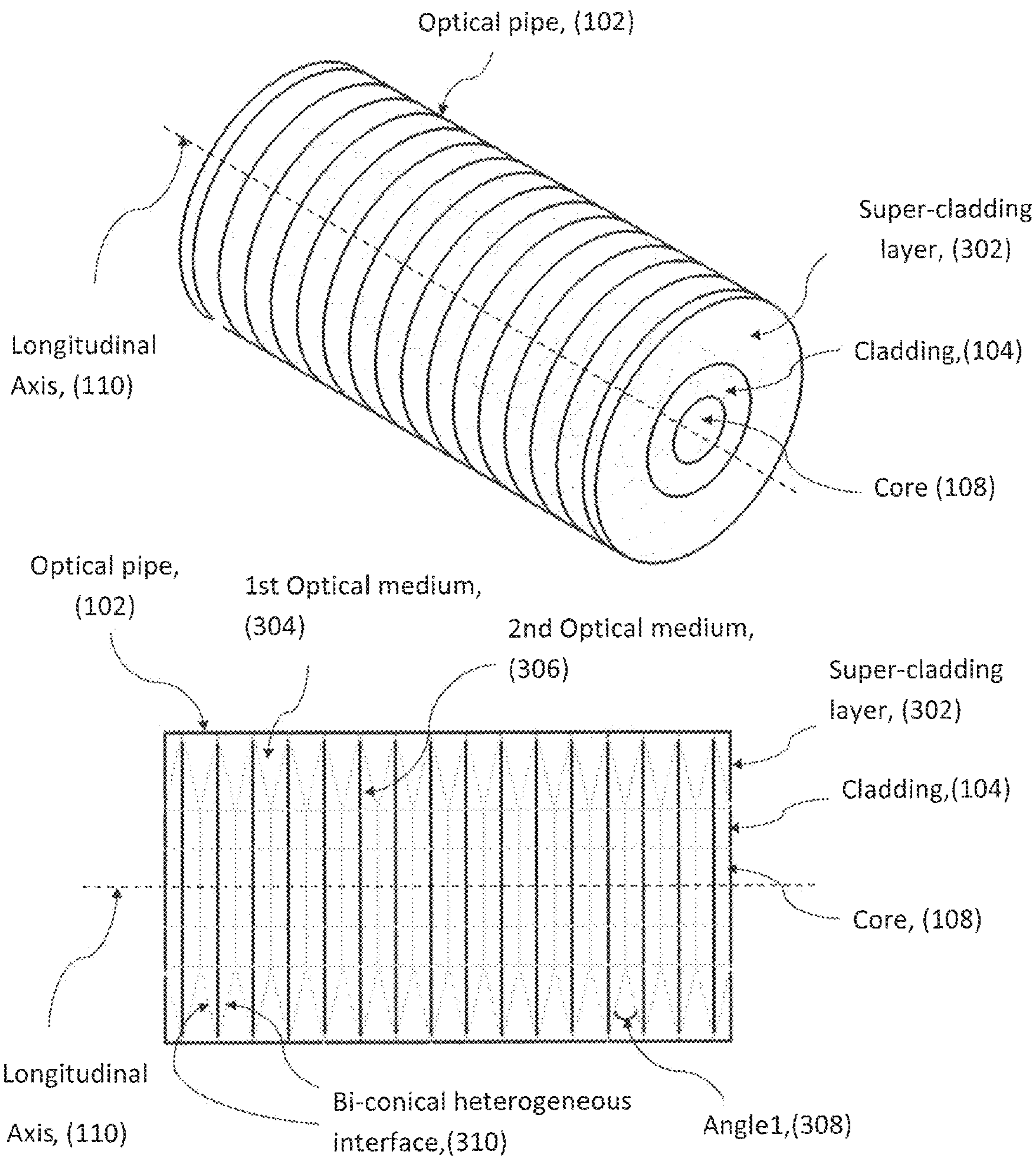
Figure 3. Super-cladding layer
