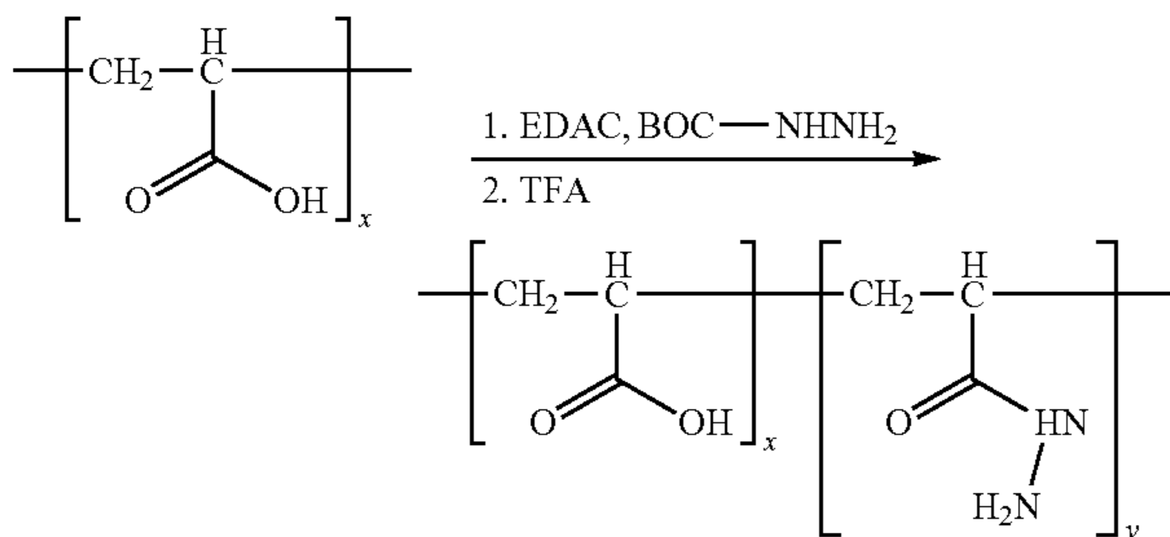
Scheme 4 Polyacrylic Acid Synthesis
