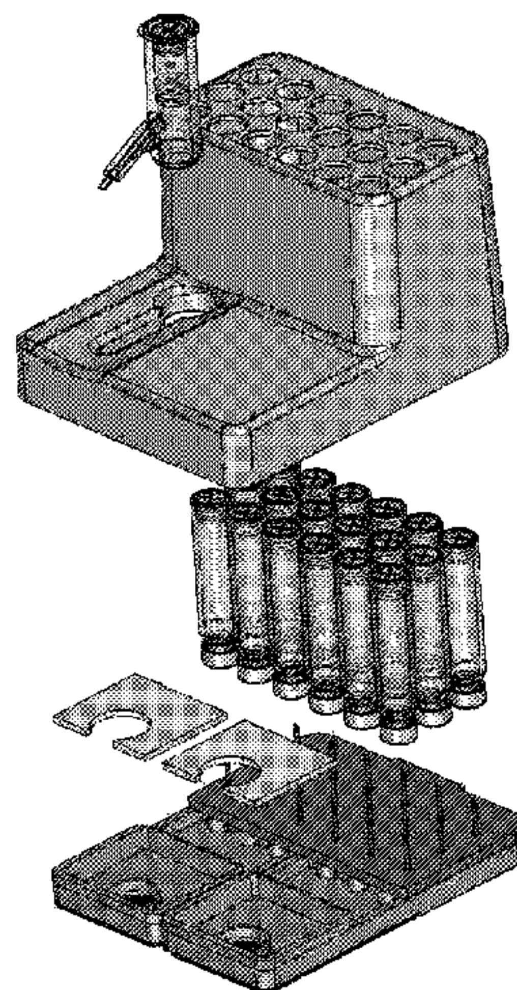
Assembly of Device
