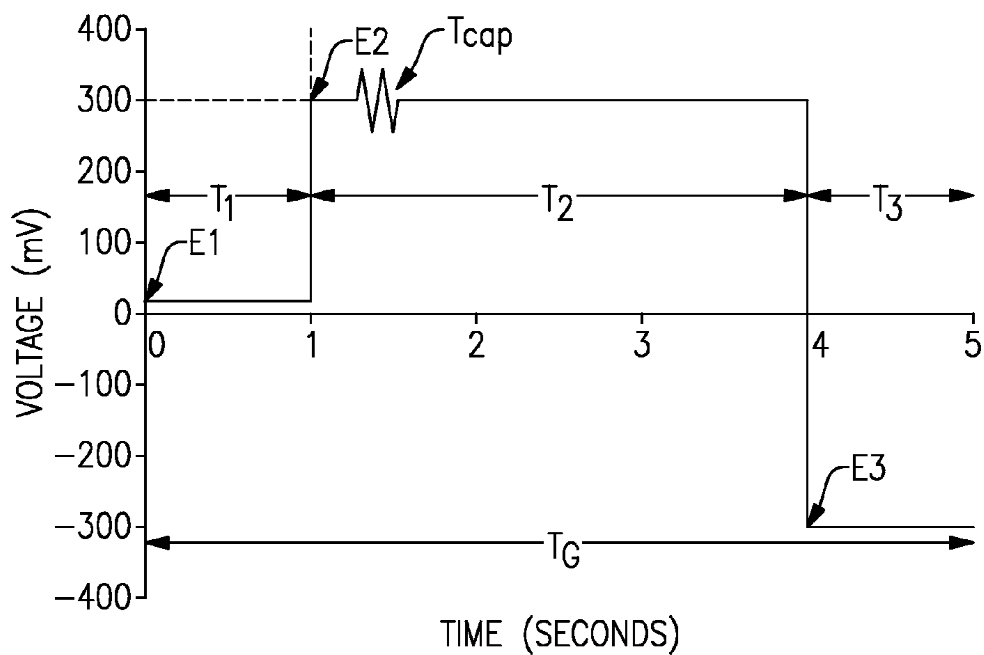
FIG.8A
