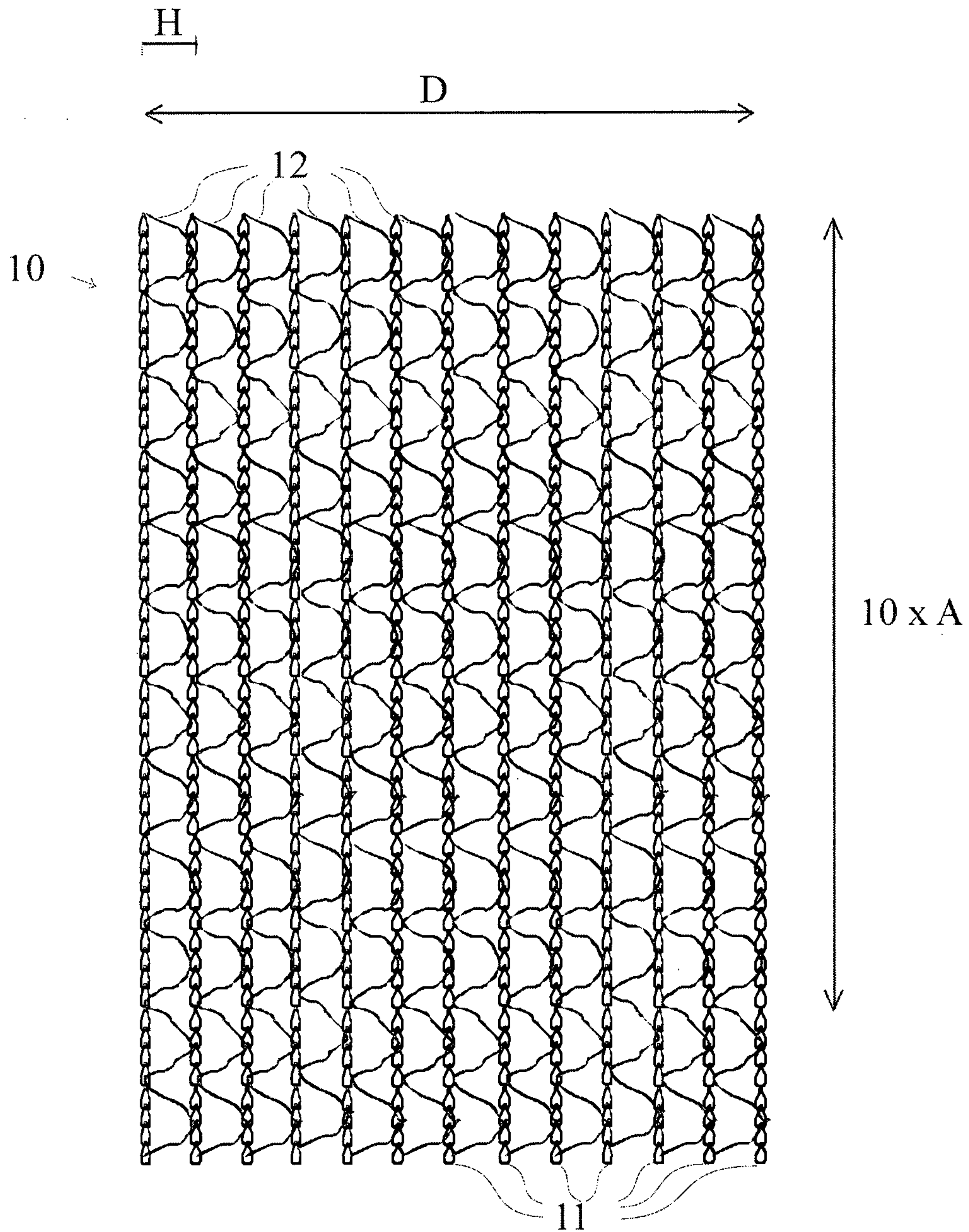
Fig. 10 (Prior Art)
