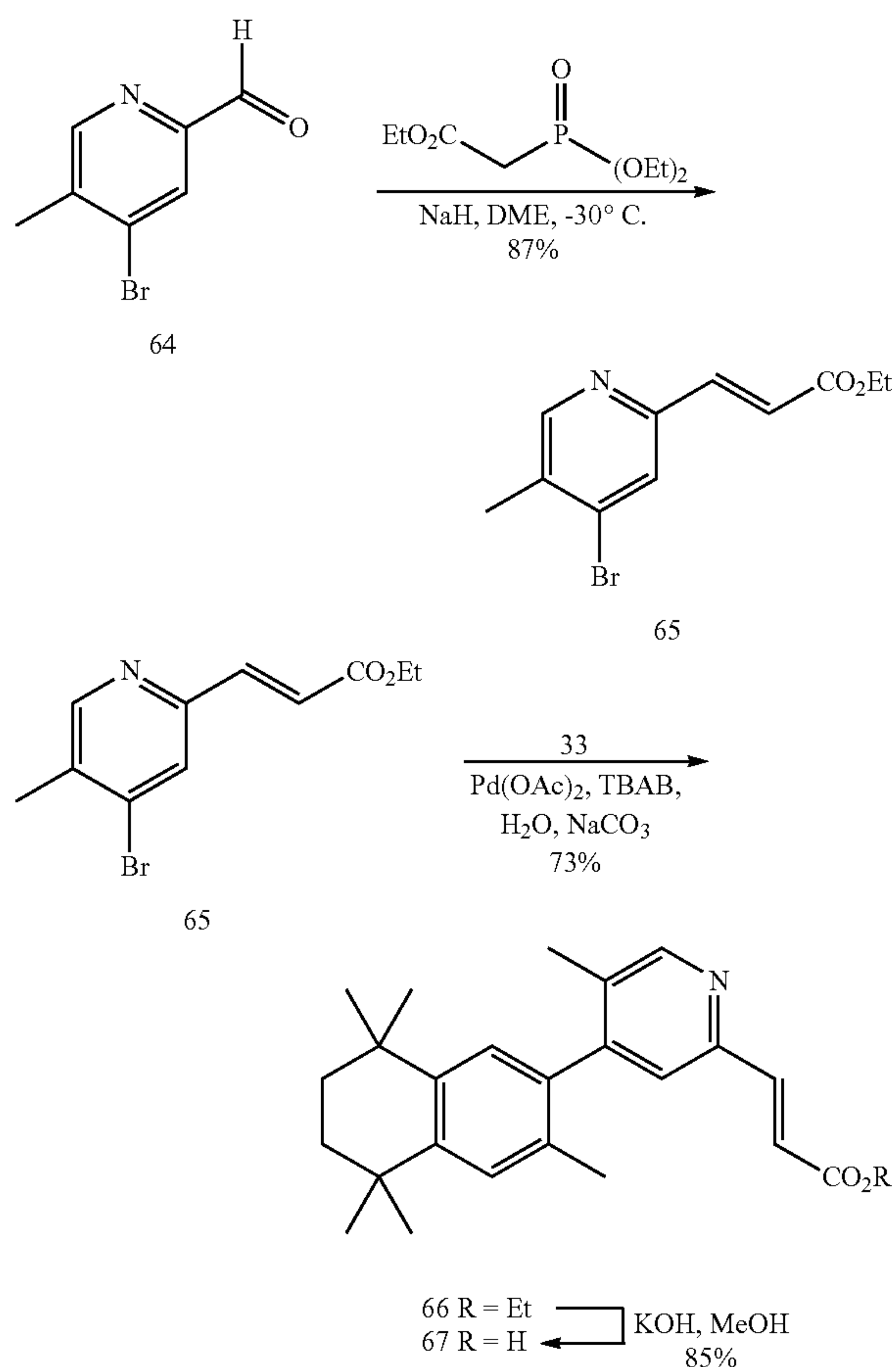
(E)-ethyl 3-(4-bromo-5-methylpyridin-2-yl)acrylate (65)
