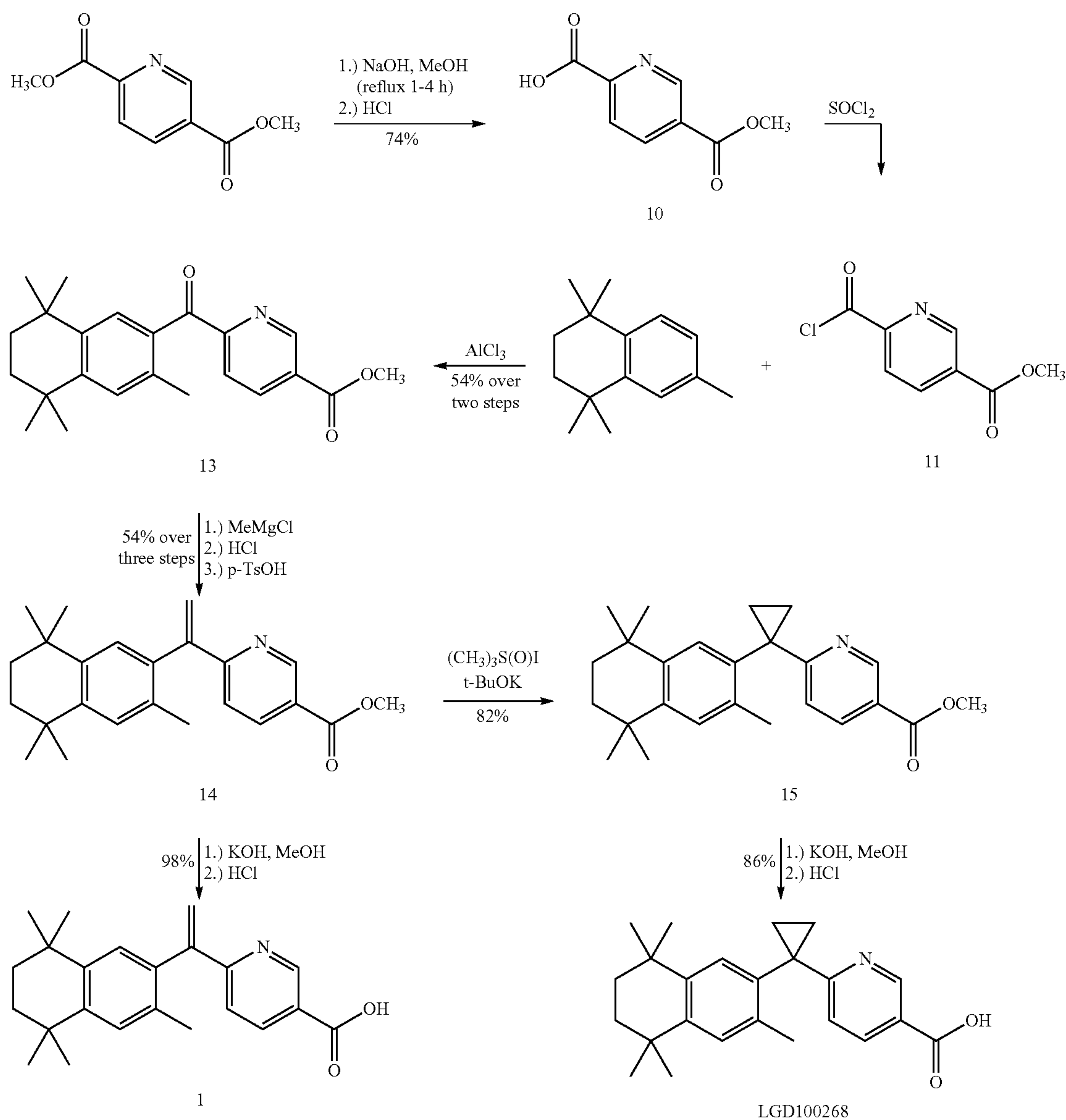
Scheme 1
