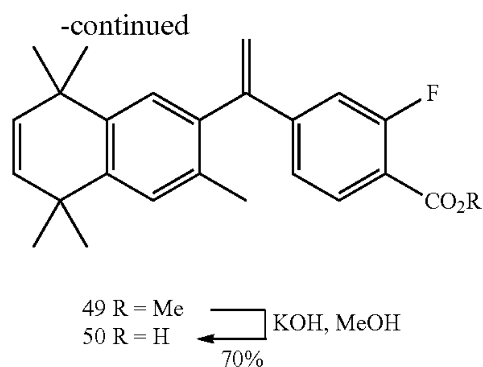
1-(4-(methoxycarbonyl)-3-fluorophenyl)vinyl trifluoromethanesulfonate (48)
