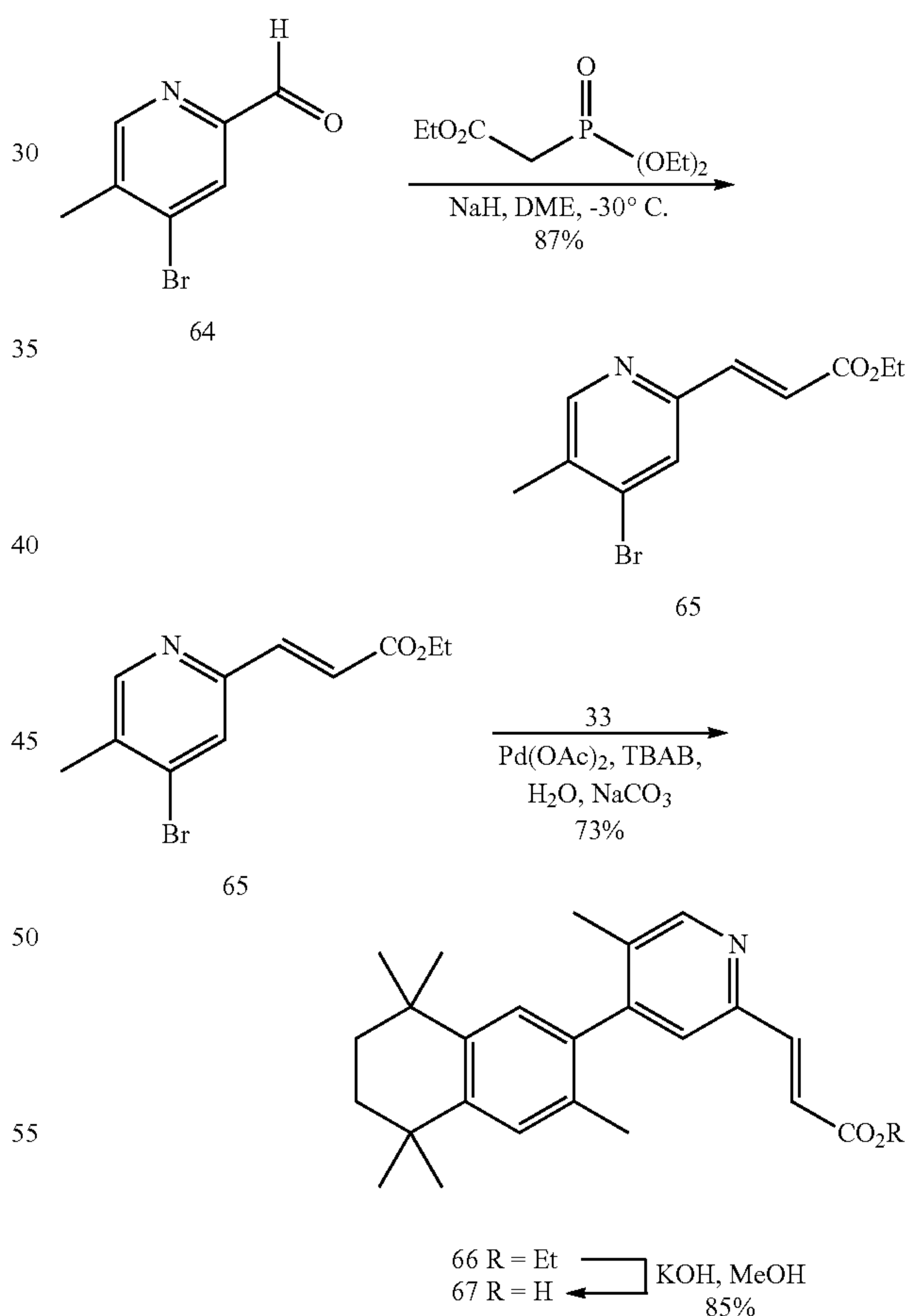
(E)-ethyl 3-(4-bromo-5-methylpyridin-2-yl)acrylate (65)
